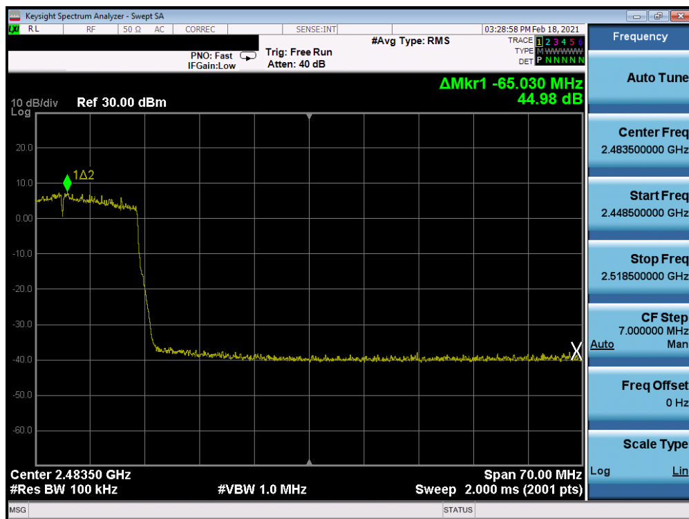
Plot 7-276. Band Edge Plot Antenna 8 (802.11ax (SU – 2.4GHz) – Ch. 9) – MCS3
