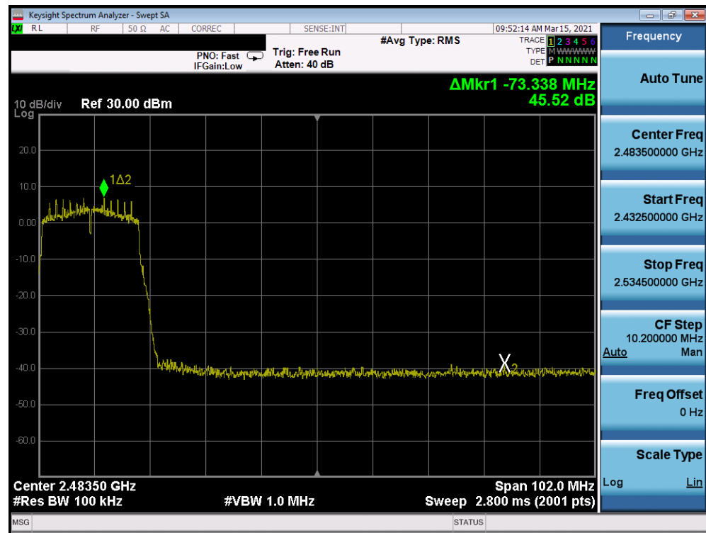
Plot 7-230. Band Edge Plot Antenna 8 (802.11n (2.4GHz) - Ch. 7) - MCS0
