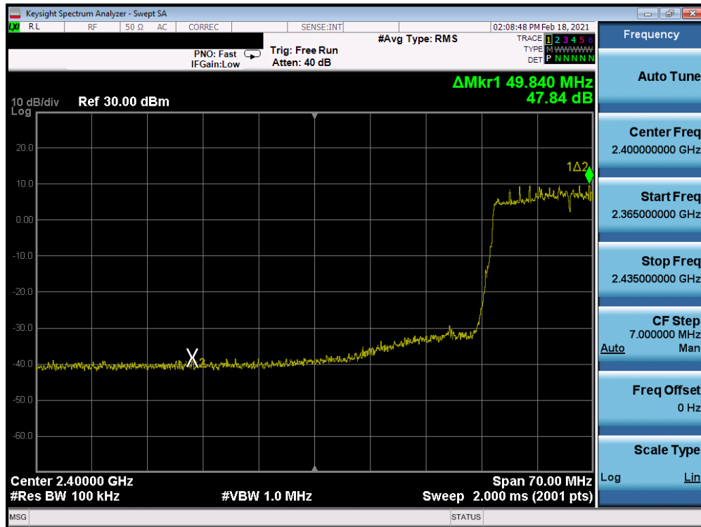
Plot 7-263. Band Edge Plot Antenna 8 (802.11ax (SU – 2.4GHz) – Ch. 5) – MCS0
