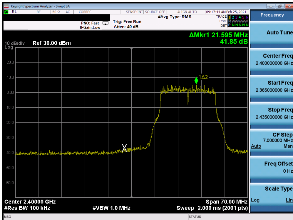
Plot 7-296. Band Edge Plot Antenna 7 (802.11g- Ch. 2) – 54Mbps
