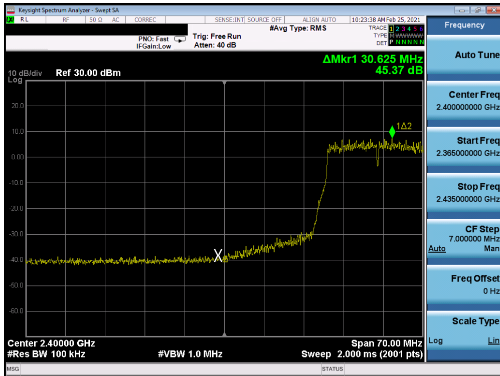
Plot 7-226. Band Edge Plot Antenna 8 (802.11n (2.4GHz) – Ch. 4) – MCS7
