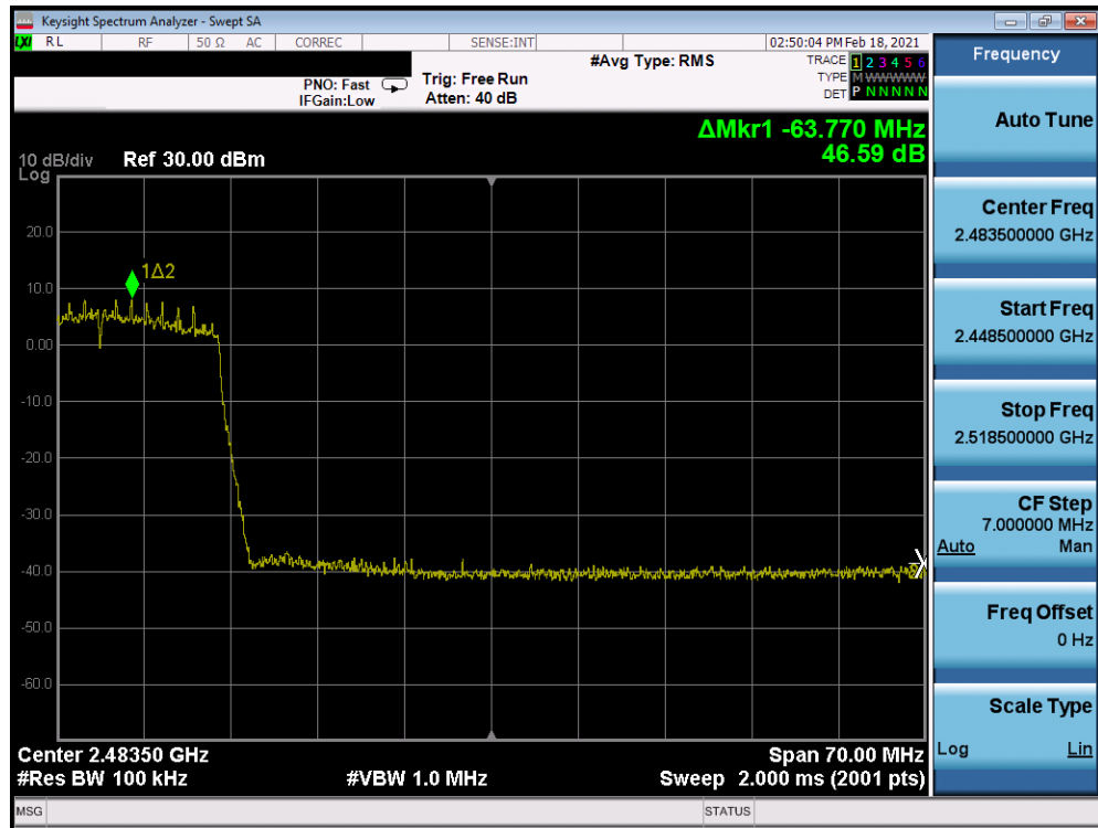
Plot 7-275: Band Edge Plot Antenna 8 (802.11ax (SU – 2.4GHz) – Ch. 9) – MCS0
