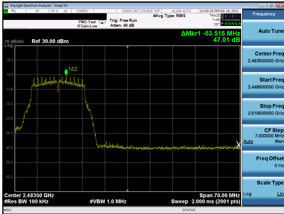
Plot 7-207. Band Edge Plot Antenna 8 (802.11g - Ch. 11) - 18Mbps
