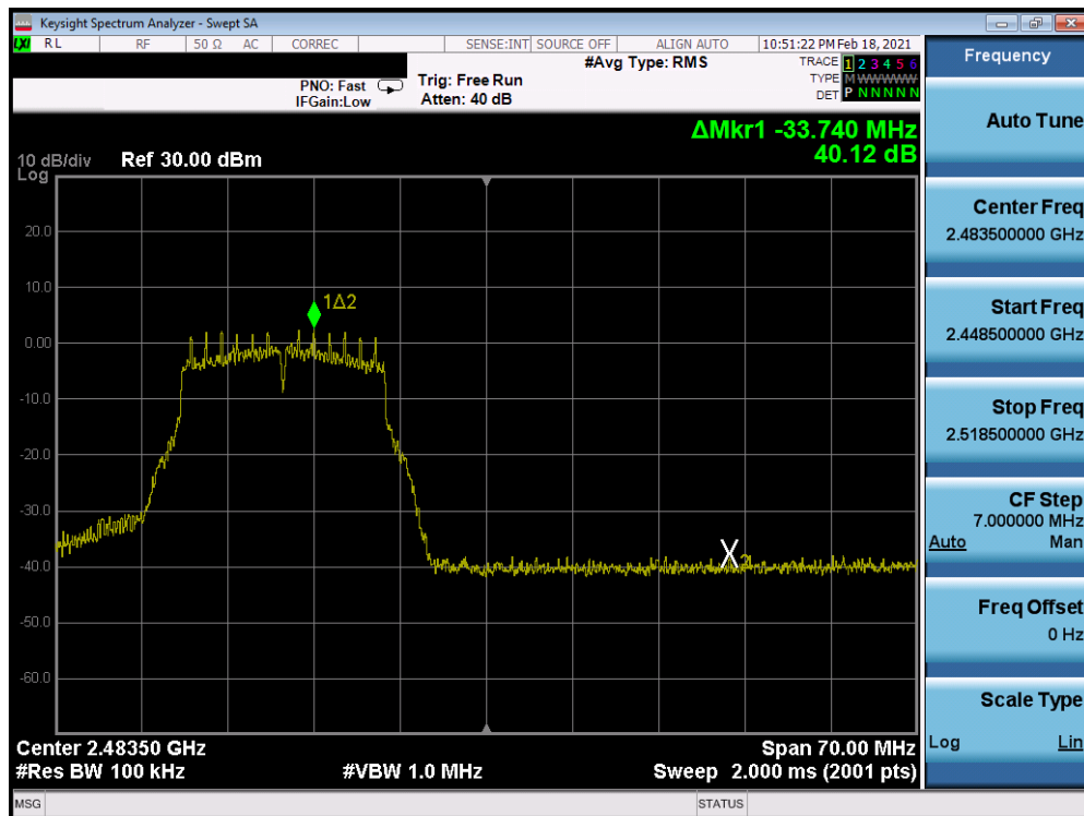
Plot 7-210. Band Edge Plot Antenna 8 (802.11g - Ch. 12) - 18Mbps
