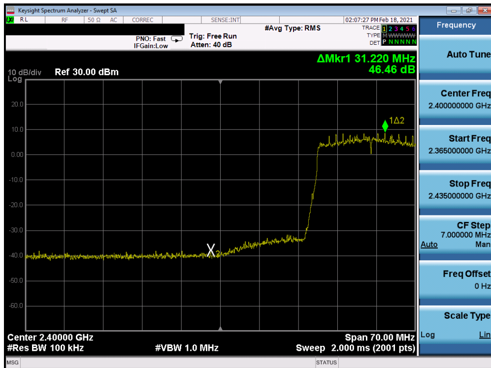
Plot 7-260: Band Edge Plot Antenna 8 (802.11ax (SU – 2.4GHz) – Ch. 4) – MCS0
