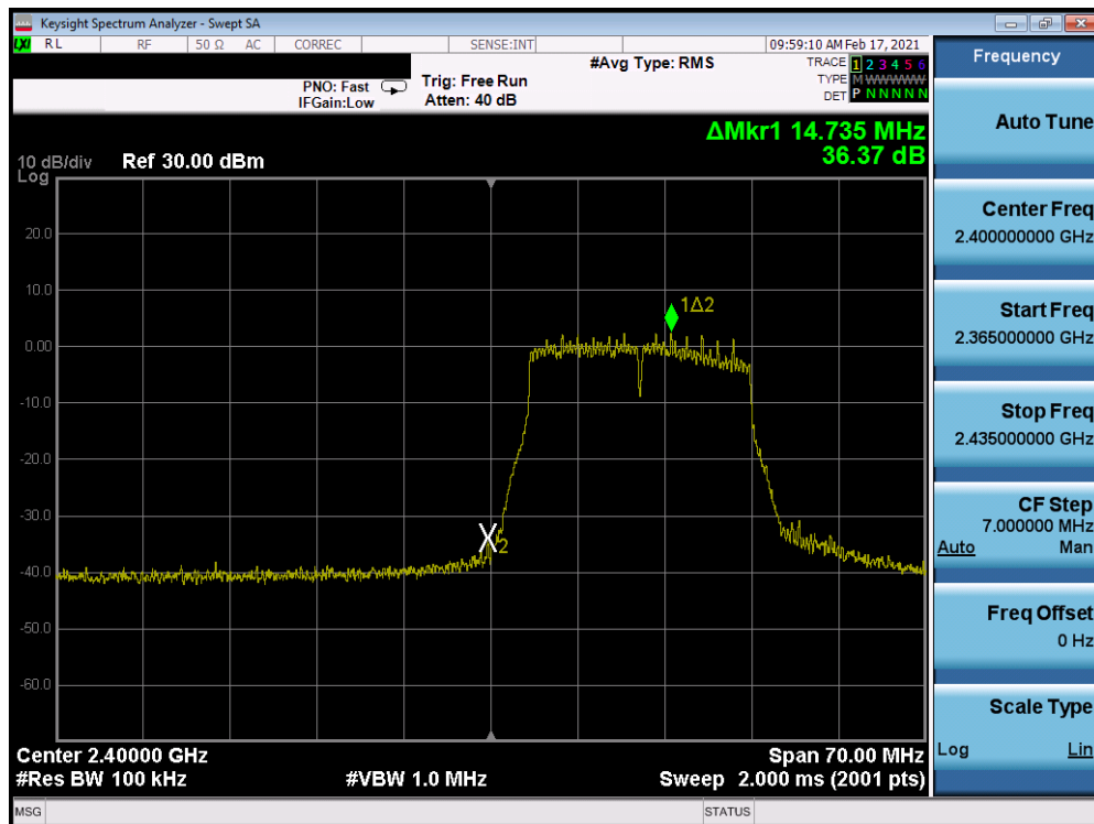
Plot 7-216. Band Edge Plot Antenna 8 (802.11n (2.4GHz) – Ch. 1) – MCS3
