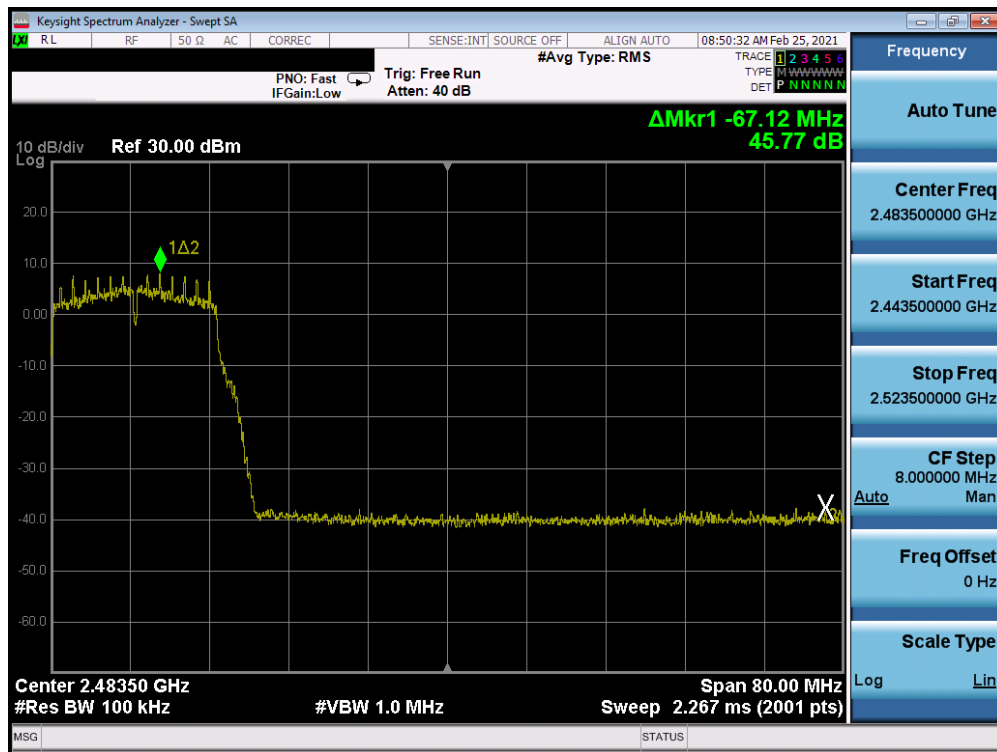
Plot 7-200. Band Edge Plot Antenna 8 (802.11g – Ch. 9) – 6Mbps
