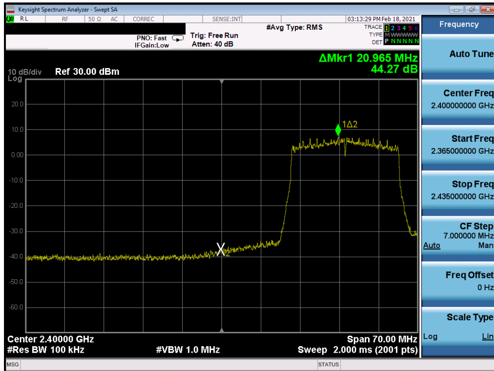
Plot 7-258. Band Edge Plot Antenna 8 (802.11ax (SU – 2.4GHz) – Ch. 3) – MCS3
