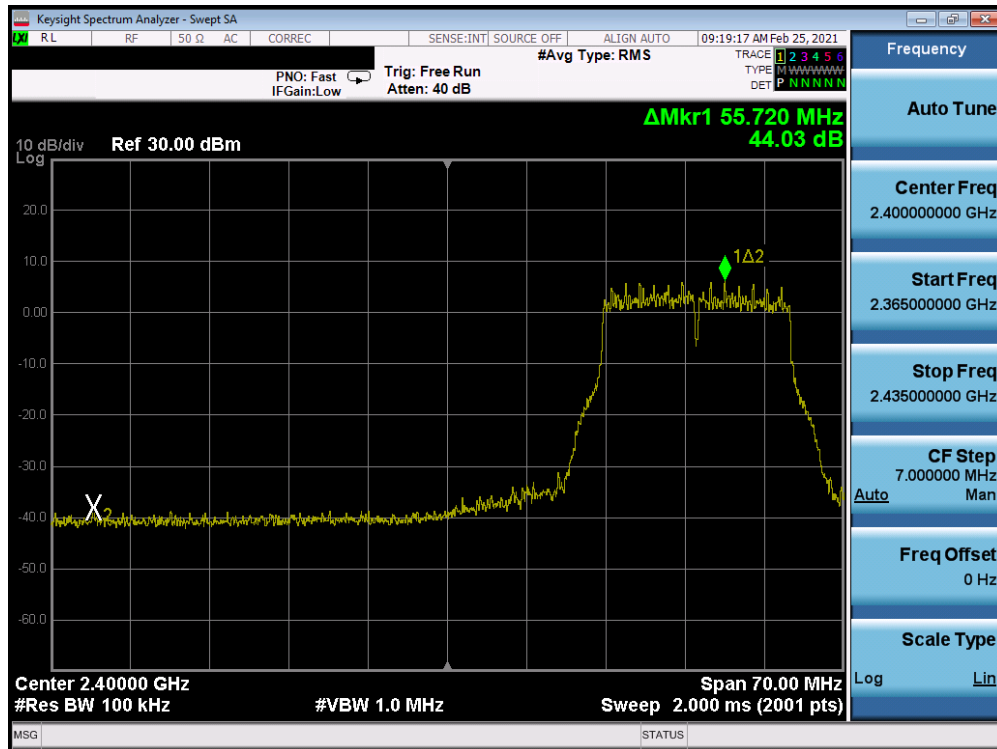
Plot 7-299: Band Edge Plot Antenna 7 (802.11g- Ch. 3) - 54Mbps
