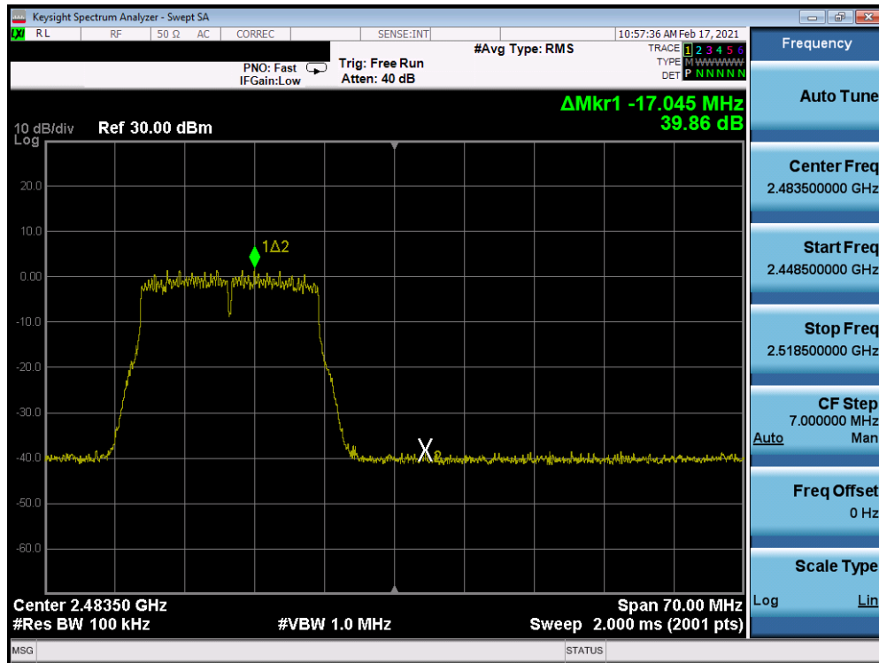
Plot 7-247. Band Edge Plot Antenna 8 (802.11n (2.4GHz) – Ch. 12) – MCS7
