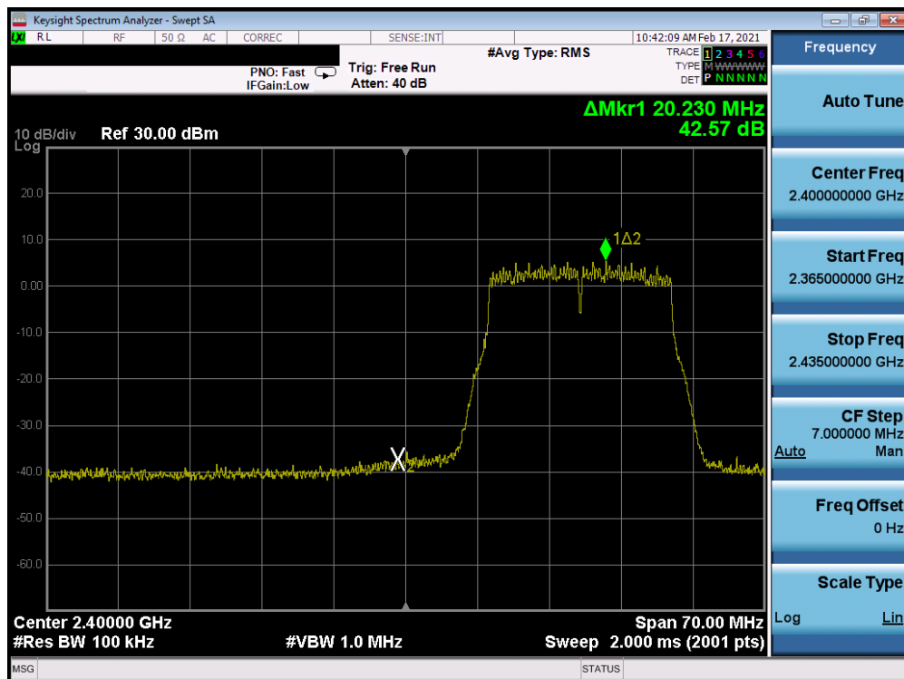
Plot 7-220. Band Edge Plot Antenna 8 (802.11n (2.4GHz) – Ch. 2) – MCS7
