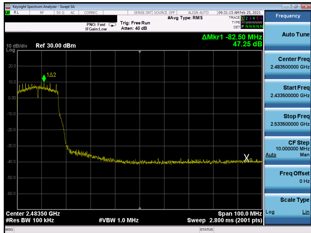
Plot 7-306:Band Edge Plot Antenna 7 (802.11g – Ch. 7) – 6Mbps
