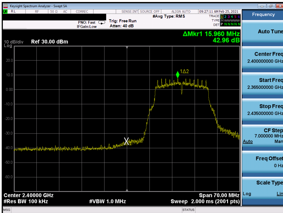
Plot 7-294. Band Edge Plot Antenna 7 (802.11g- Ch. 2) – 6Mbps
