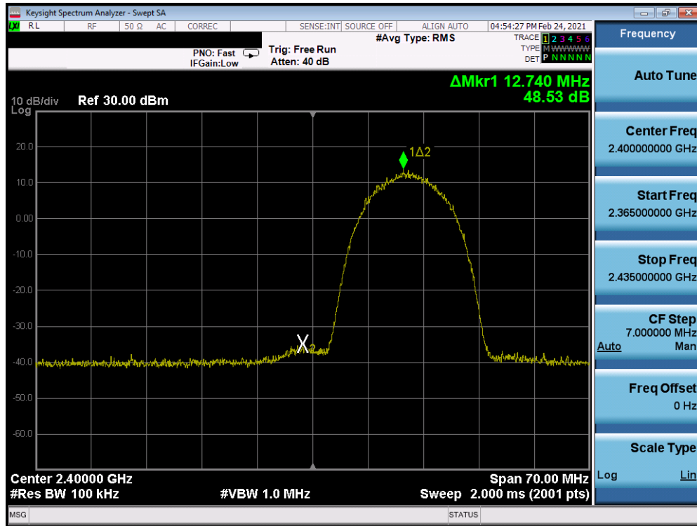
Plot 7-287. Band Edge Plot Antenna 7 (802.11b – Ch. 1) – 11Mbps
