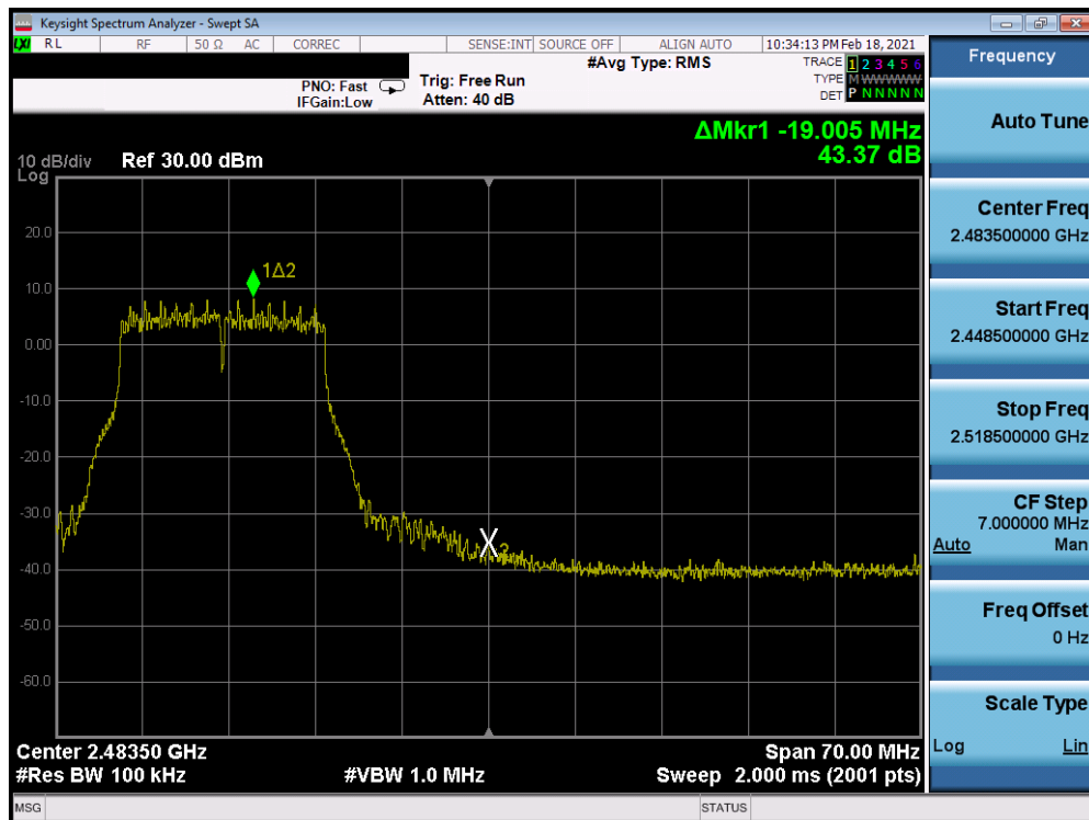
Plot 7-208. Band Edge Plot Antenna 8 (802.11g - Ch. 11) - 54Mbps
