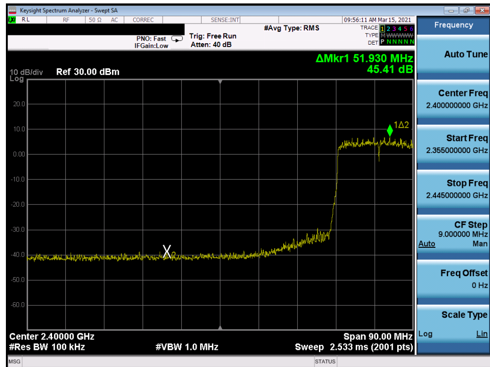
Plot 7-266: Band Edge Plot Antenna 8 (802.11ax (SU – 2.4GHz) – Ch. 6) – MCS5
