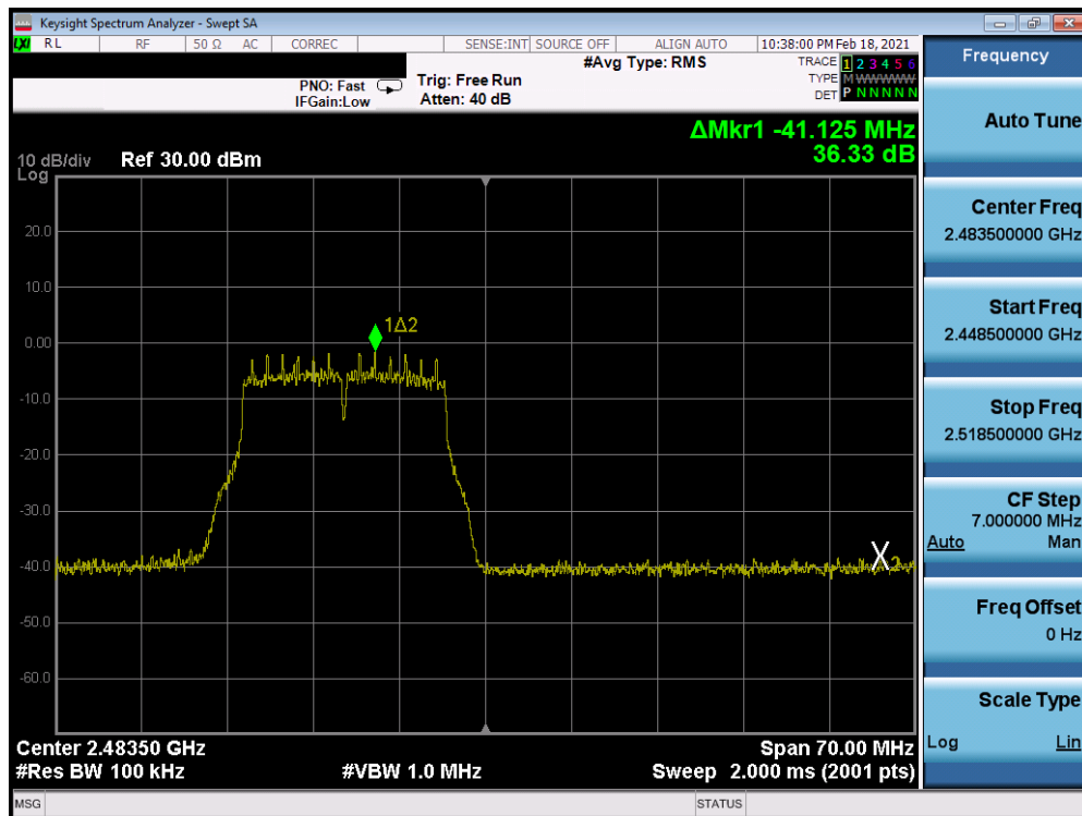
Plot 7-214. Band Edge Plot Antenna 8 (802.11g - Ch. 13) - 54Mbps
