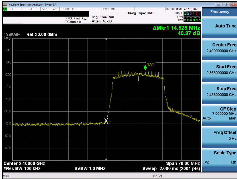
Plot 7-251. Band Edge Plot Antenna 8 (802.11ax (SU – 2.4GHz) – Ch. 1) – MCS0
