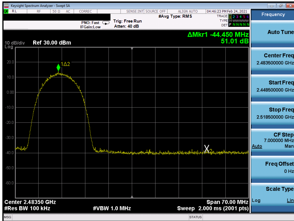
Plot 7-288. Band Edge Plot Antenna 7 (802.11b – Ch. 11) – 11Mbps
