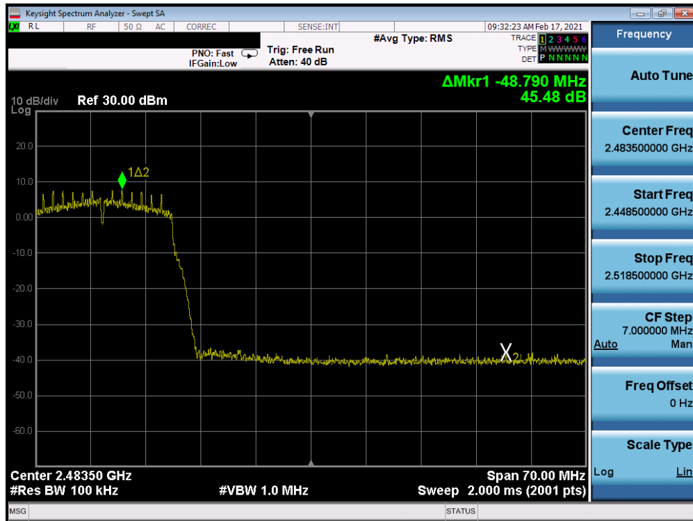
Plot 7-239. Band Edge Plot Antenna 8 (802.11n (2.4GHz) – Ch. 10) – MCS0
