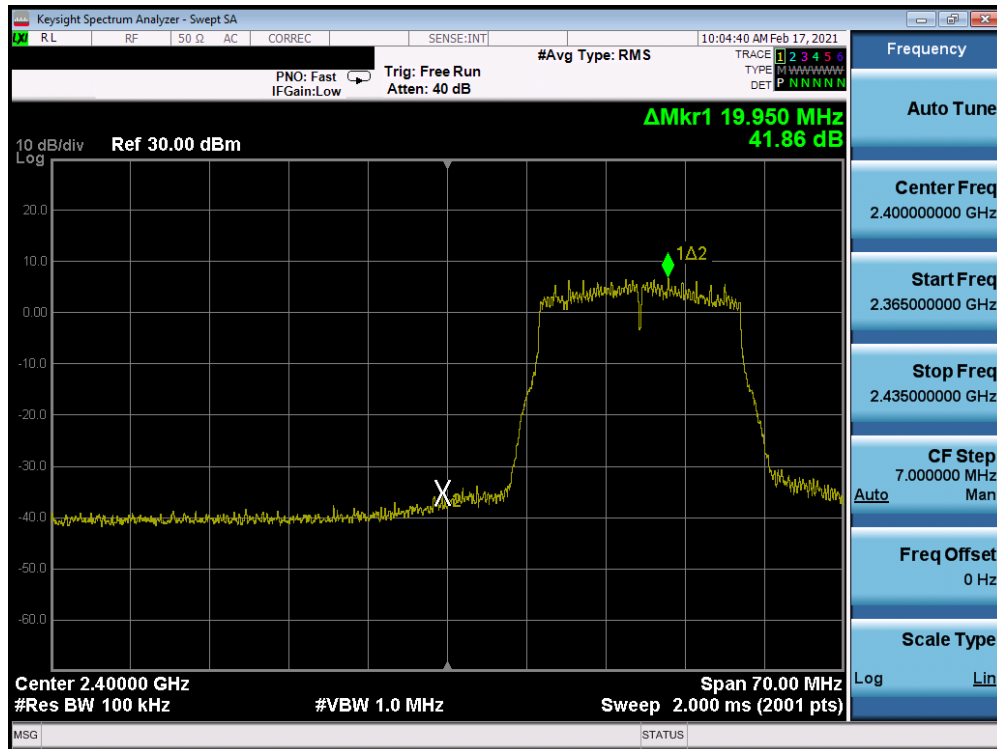
Plot 7-219. Band Edge Plot Antenna 8 (802.11n (2.4GHz) – Ch. 2) – MCS3
