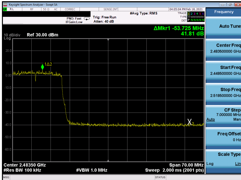
Plot 7-280. Band Edge Plot Antenna 8 (802.11ax (SU – 2.4GHz) – Ch. 10) – MCS5
