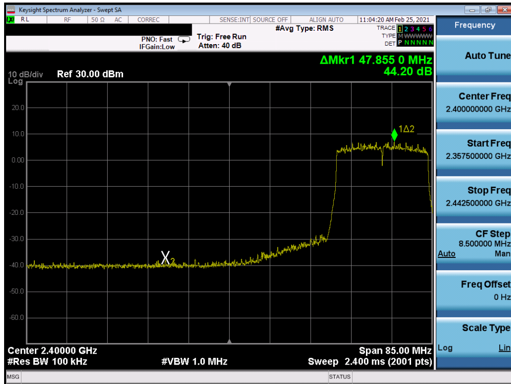
Plot 7-265. Band Edge Plot Antenna 8 (802.11ax (SU – 2.4GHz) – Ch. 5) – MCS5
