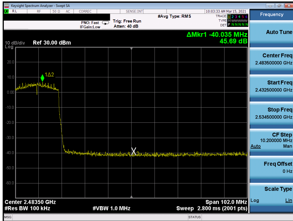
Plot 7-270: Band Edge Plot Antenna 8 (802.11ax (SU – 2.4GHz) – Ch. 7) – MCS3
