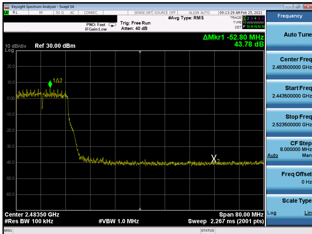
Plot 7-202. Band Edge Plot Antenna 8 (802.11g - Ch. 9) - 54Mbps
