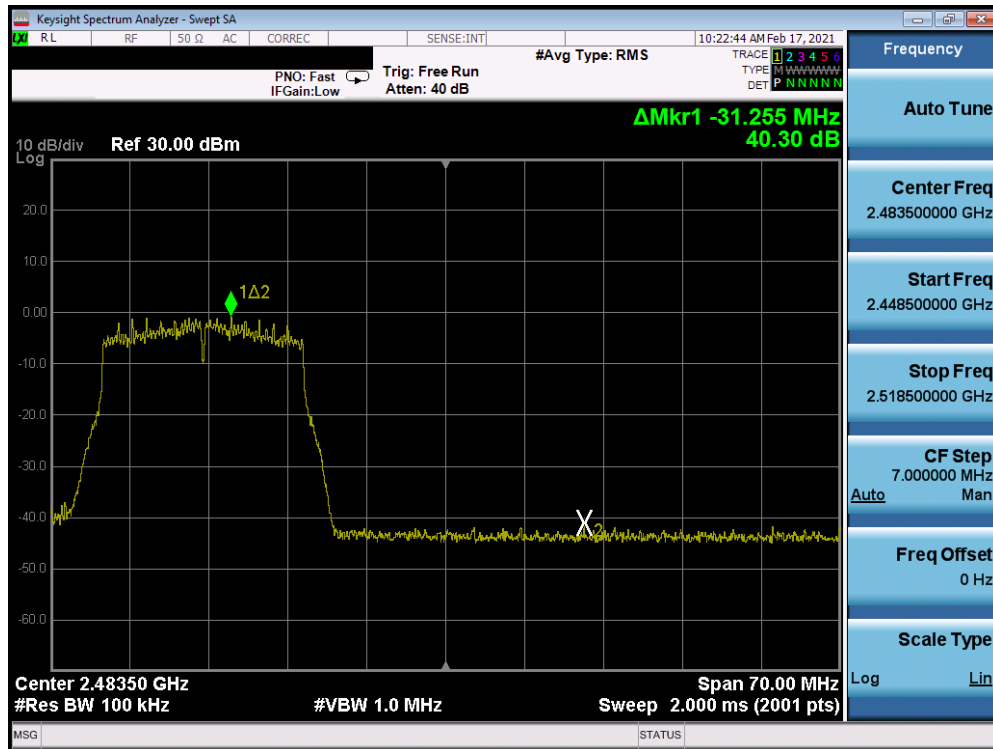
Plot 7-243. Band Edge Plot Antenna 8 (802.11n (2.4GHz) – Ch. 11) – MCS3
