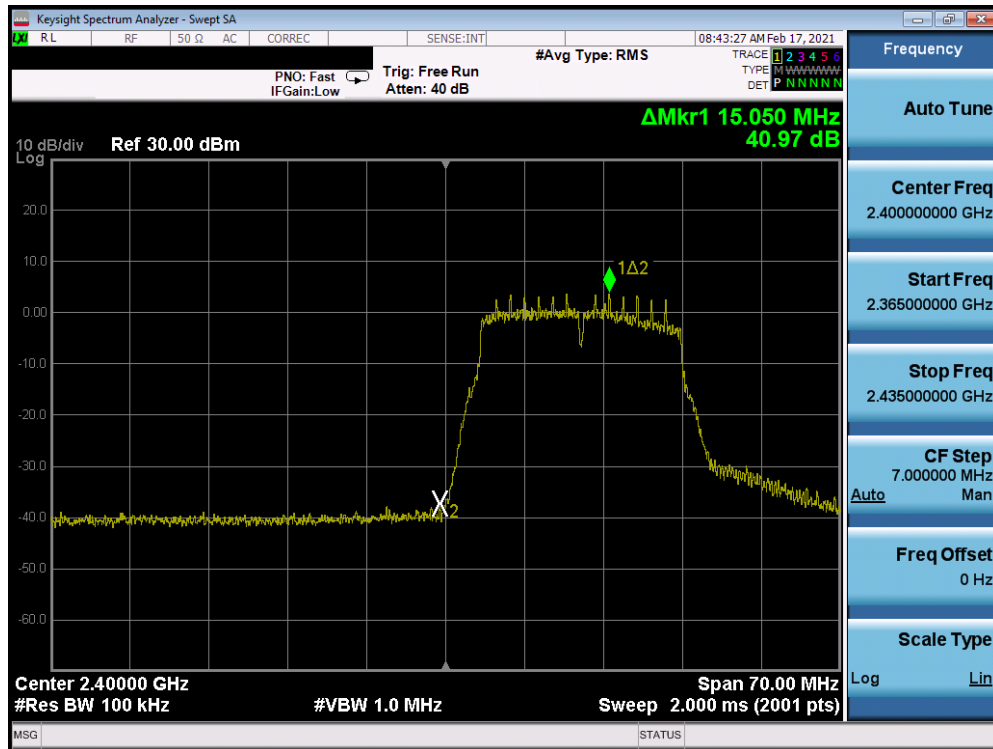
Plot 7-215. Band Edge Plot Antenna 8 (802.11n (2.4GHz) – Ch. 1) – MCS0
