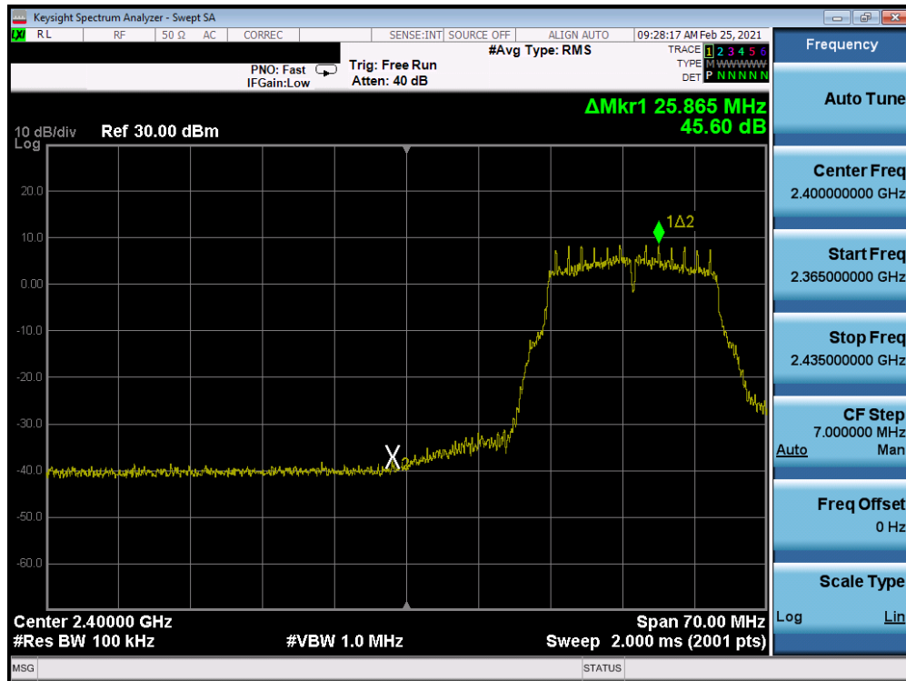
Plot 7-297. Band Edge Plot Antenna 7 (802.11g- Ch. 3) – 6Mbps
