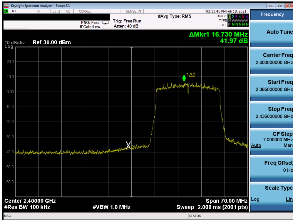
Plot 7-255. Band Edge Plot Antenna 8 (802.11ax (SU – 2.4GHz) – Ch. 2) – MCS3
