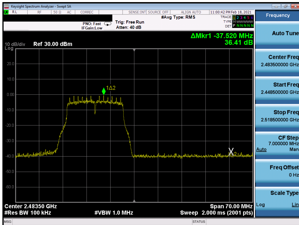
Plot 7-212. Band Edge Plot Antenna 8 (802.11g – Ch. 13) – 6Mbps
