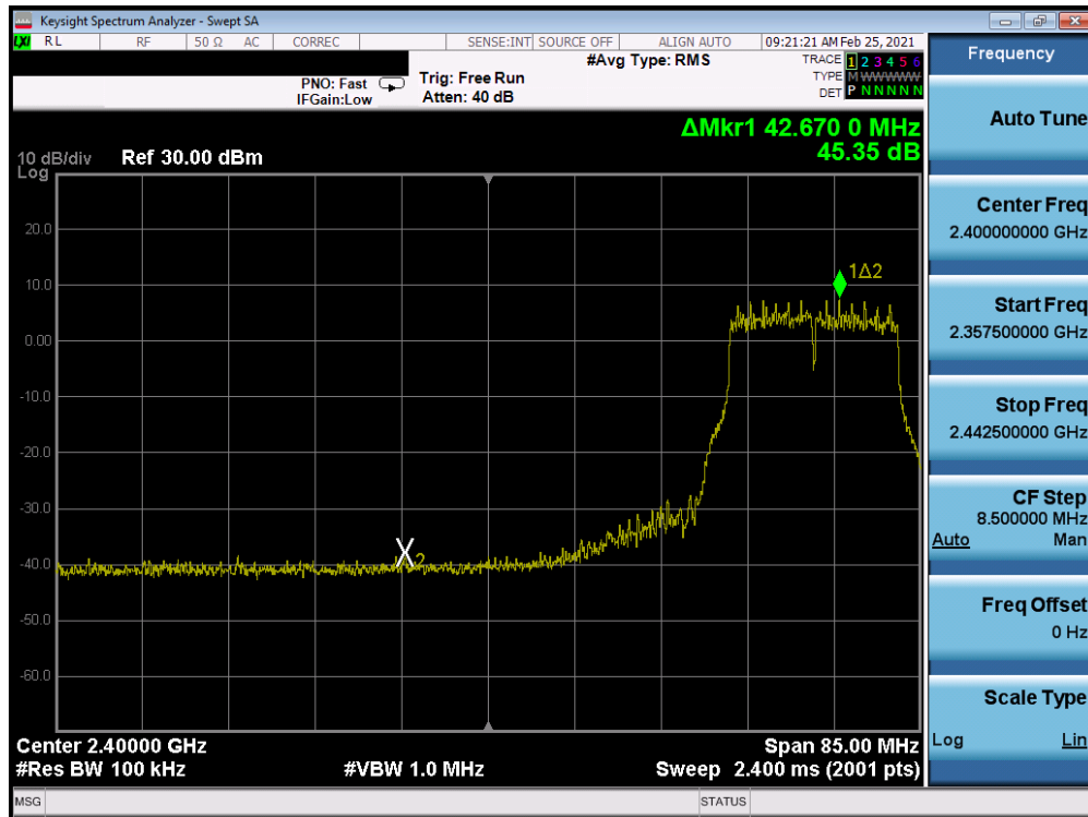
Plot 7-305. Band Edge Plot Antenna 7 (802.11g- Ch. 5) – 54Mbps
