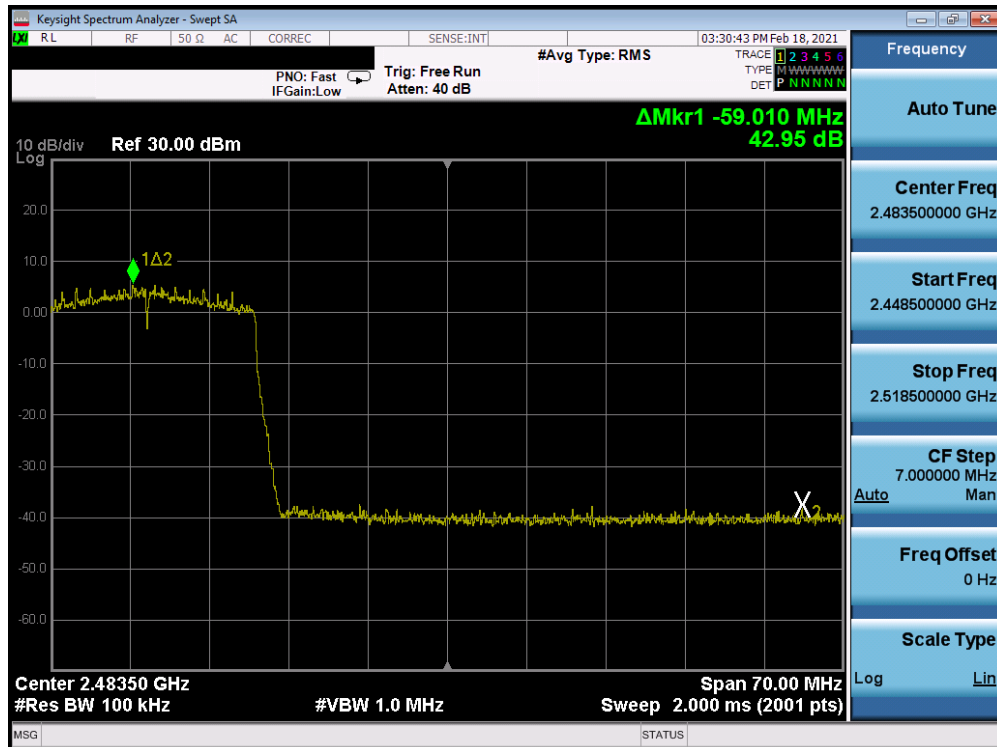
Plot 7-279. Band Edge Plot Antenna 8 (802.11ax (SU – 2.4GHz) – Ch. 10) – MCS3
