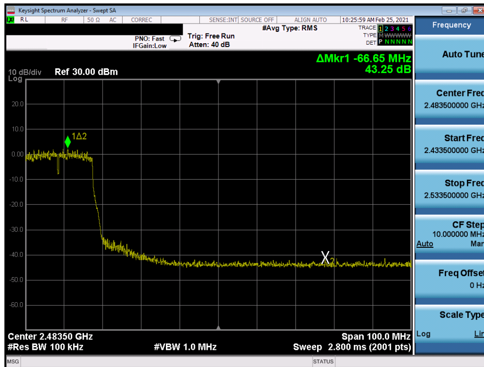
Plot 7-232. Band Edge Plot Antenna 8 (802.11n (2.4GHz) – Ch. 7) – MCS7
