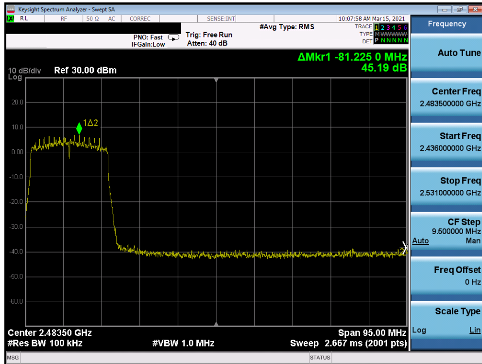
Plot 7-272: Band Edge Plot Antenna 8 (802.11ax (SU – 2.4GHz) – Ch. 8) – MCS0
