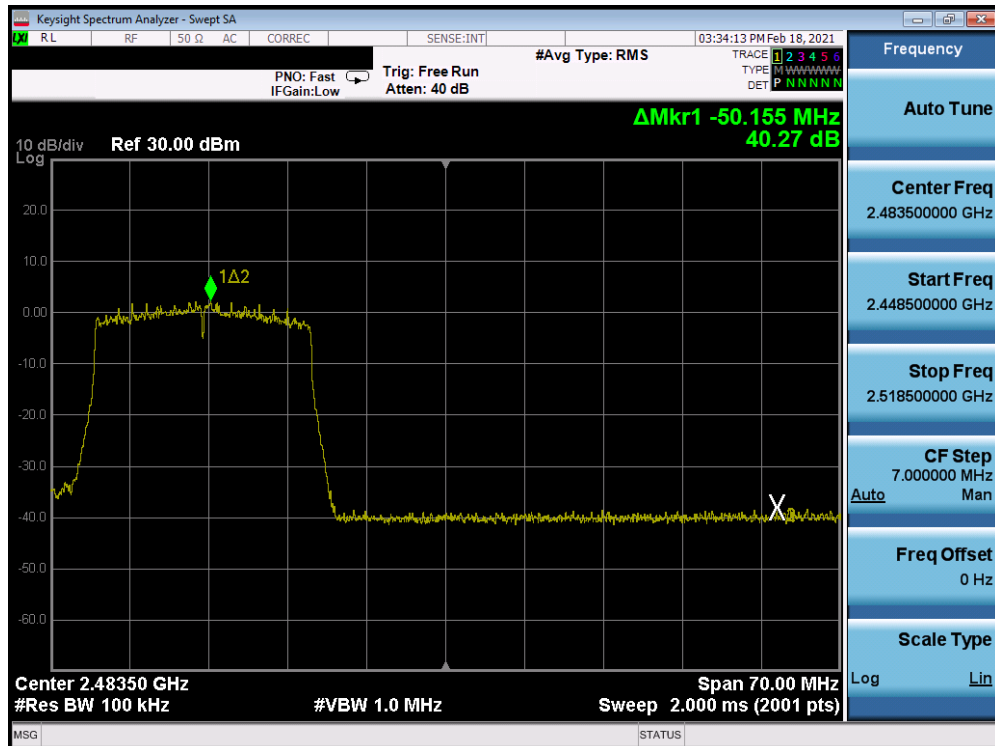
Plot 7-282. Band Edge Plot Antenna 8 (802.11ax (SU – 2.4GHz) – Ch. 11) – MCS3
