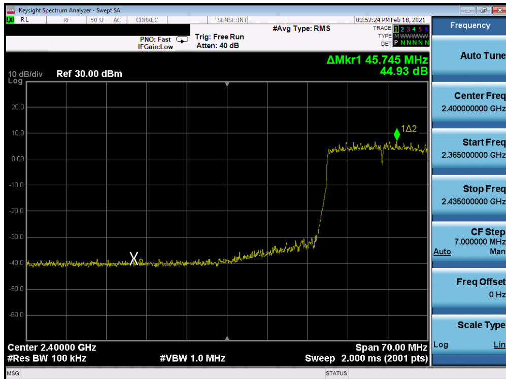
Plot 7-262. Band Edge Plot Antenna 8 (802.11ax (SU – 2.4GHz) – Ch. 4) – MCS5
