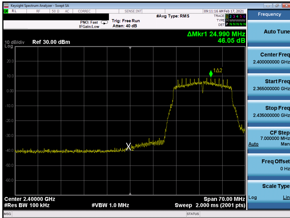
Plot 7-221. Band Edge Plot Antenna 8 (802.11n (2.4GHz) – Ch. 3) – MCS0
