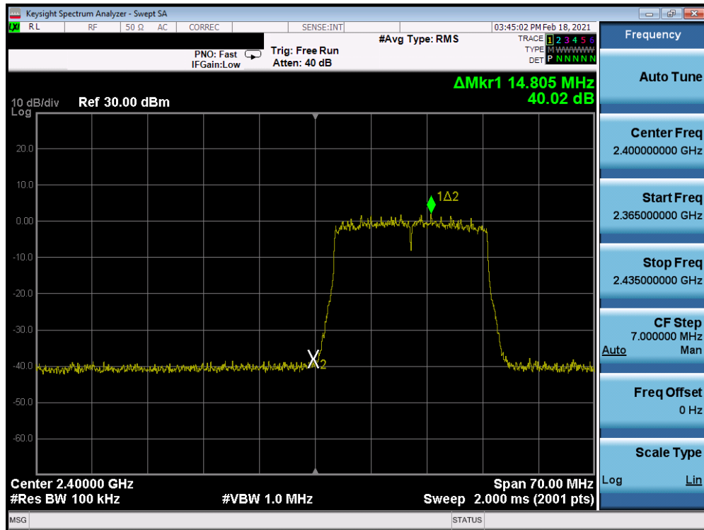
Plot 7-253. Band Edge Plot Antenna 8 (802.11ax (SU – 2.4GHz) – Ch. 1) – MCS5
