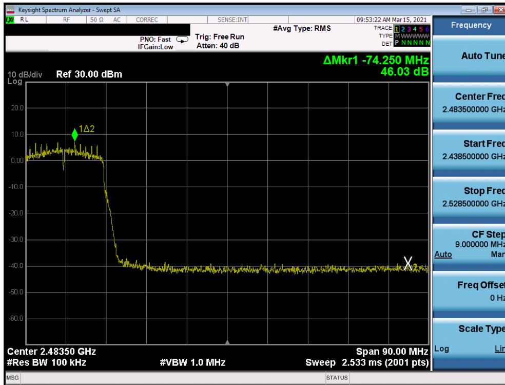
Plot 7-233: Band Edge Plot Antenna 8 (802.11n (2.4GHz) – Ch. 8) – MCS0
