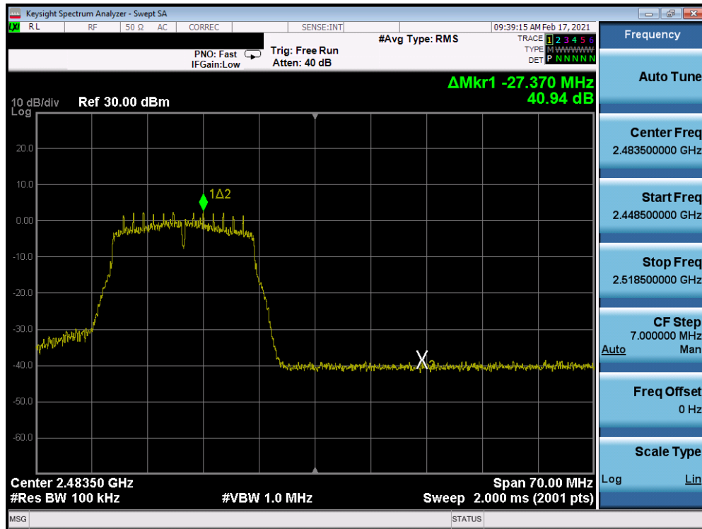
Plot 7-245. Band Edge Plot Antenna 8 (802.11n (2.4GHz) – Ch. 12) – MCS0
