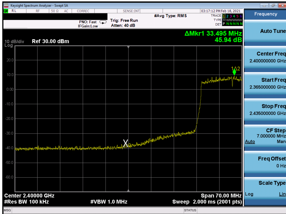
Plot 7-264. Band Edge Plot Antenna 8 (802.11ax (SU – 2.4GHz) – Ch. 5) – MCS3
