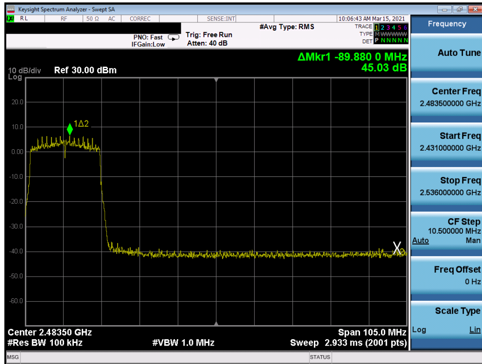
Plot 7-269: Band Edge Plot Antenna 8 (802.11ax (SU – 2.4GHz) – Ch. 7) – MCS0
