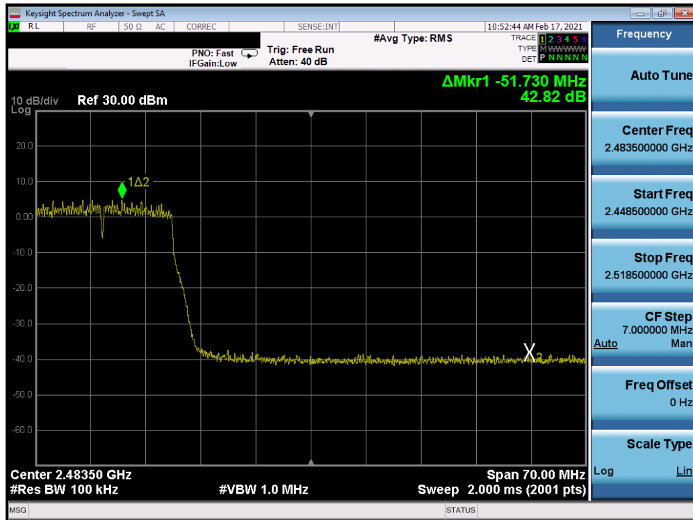
Plot 7-241. Band Edge Plot Antenna 8 (802.11n (2.4GHz) – Ch. 10) – MCS7
