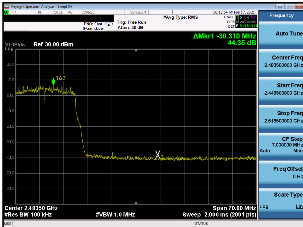
Plot 7-240. Band Edge Plot Antenna 8 (802.11n (2.4GHz) – Ch. 10) – MCS3
