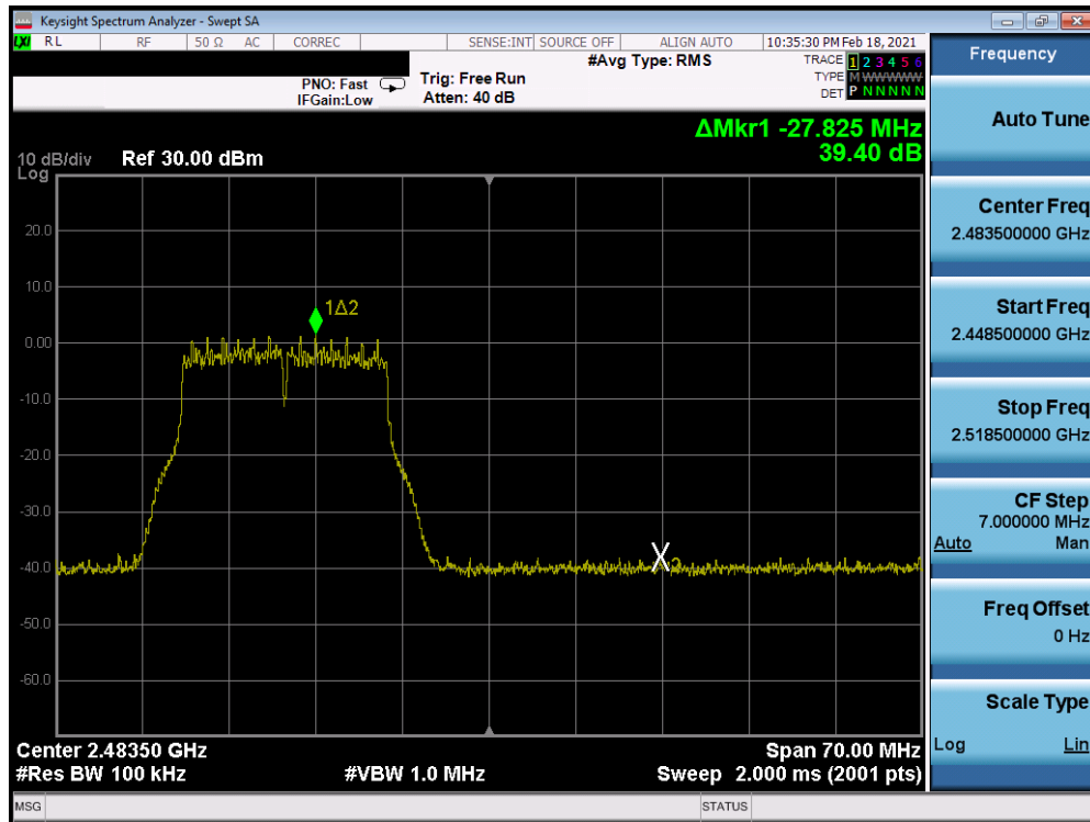
Plot 7-211. Band Edge Plot Antenna 8 (802.11g – Ch. 12) – 54Mbps
