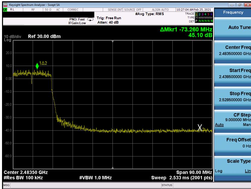
Plot 7-235. Band Edge Plot Antenna 8 (802.11n (2.4GHz) – Ch. 8) – MCS7
