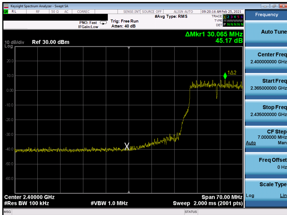
Plot 7-302. Band Edge Plot Antenna 7 (802.11g- Ch. 4) – 54Mbps
