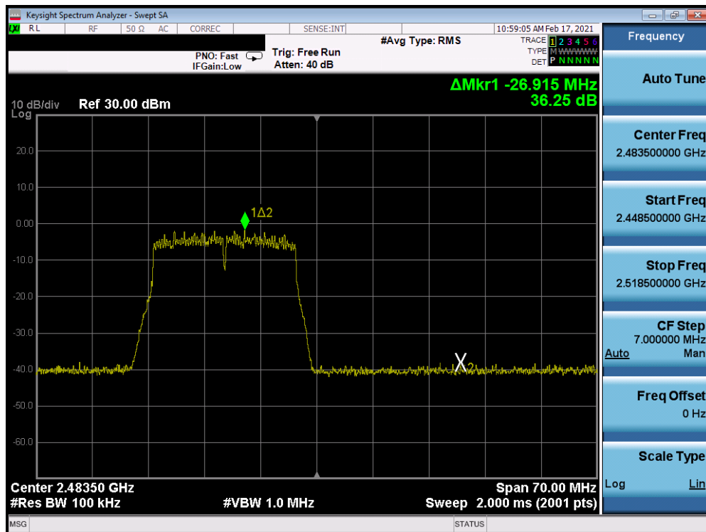
Plot 7-250. Band Edge Plot Antenna 8 (802.11n (2.4GHz) – Ch. 13) – MCS7
