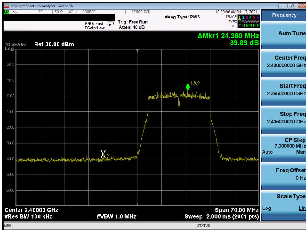
Plot 7-217. Band Edge Plot Antenna 8 (802.11n (2.4GHz) – Ch. 1) – MCS7
