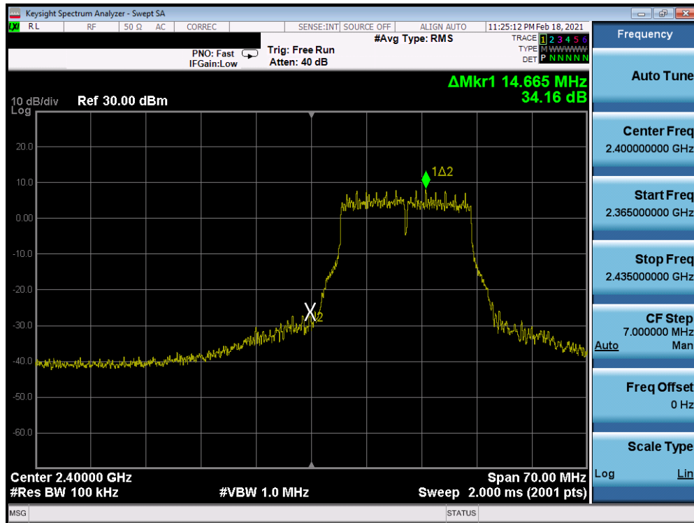
Plot 7-293. Band Edge Plot Antenna 7 (802.11g- Ch. 1) – 54Mbps
