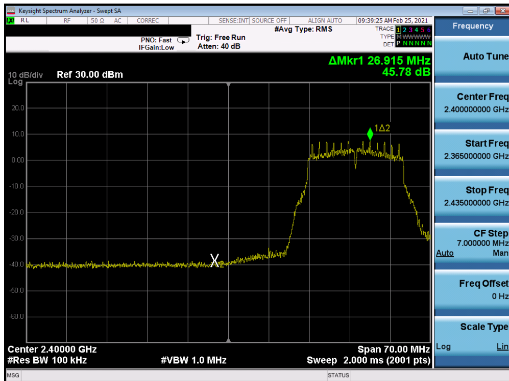
Plot 7-298. Band Edge Plot Antenna 7 (802.11g- Ch. 3) – 18Mbps
