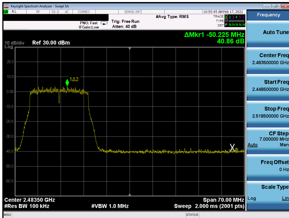
Plot 7-244. Band Edge Plot Antenna 8 (802.11n (2.4GHz) – Ch. 11) – MCS7
