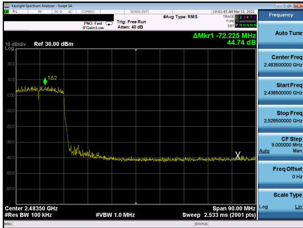
Plot 7-274: Band Edge Plot Antenna 8 (802.11ax (SU – 2.4GHz) – Ch. 8) – MCS5
