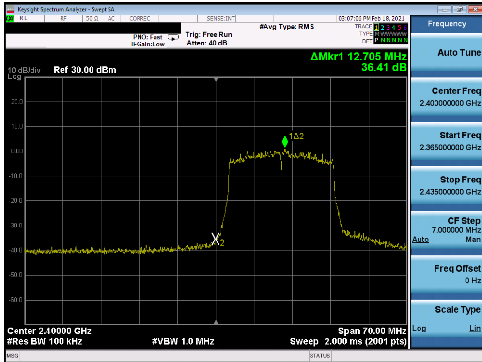
Plot 7-252. Band Edge Plot Antenna 8 (802.11ax (SU – 2.4GHz) – Ch. 1) – MCS3
