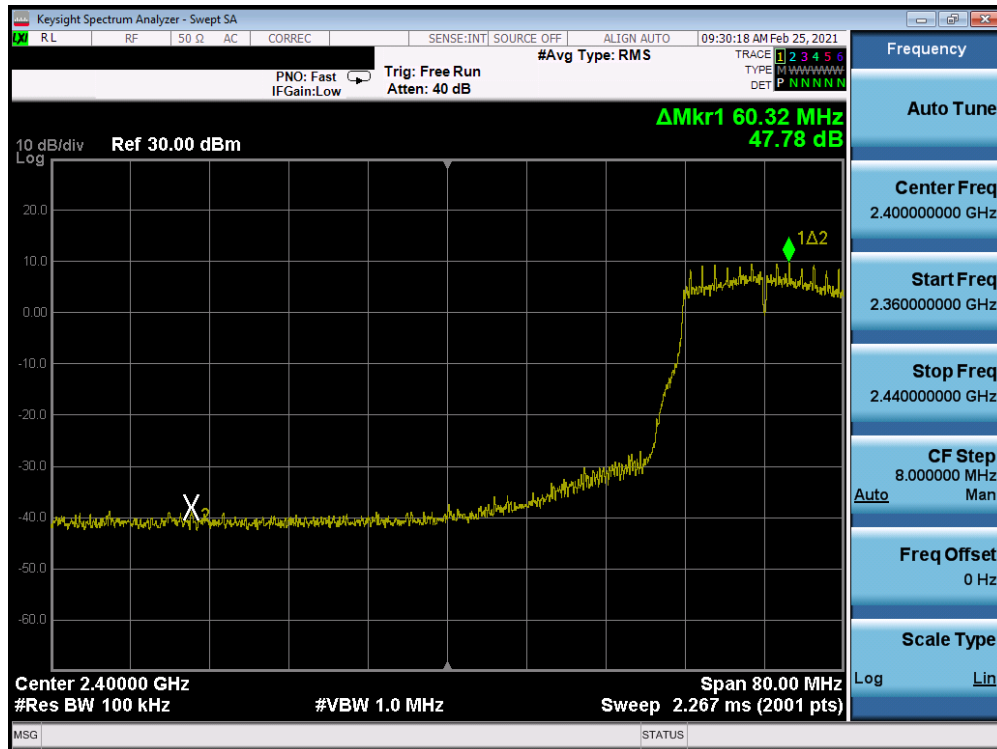
Plot 7-303. Band Edge Plot Antenna 7 (802.11g- Ch. 5) – 6Mbps
