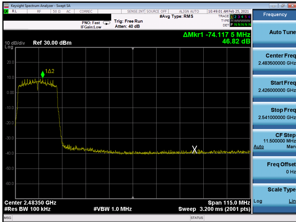
Plot 7-267: Band Edge Plot Antenna 8 (802.11ax (SU – 2.4GHz) – Ch. 6) – MCS0
