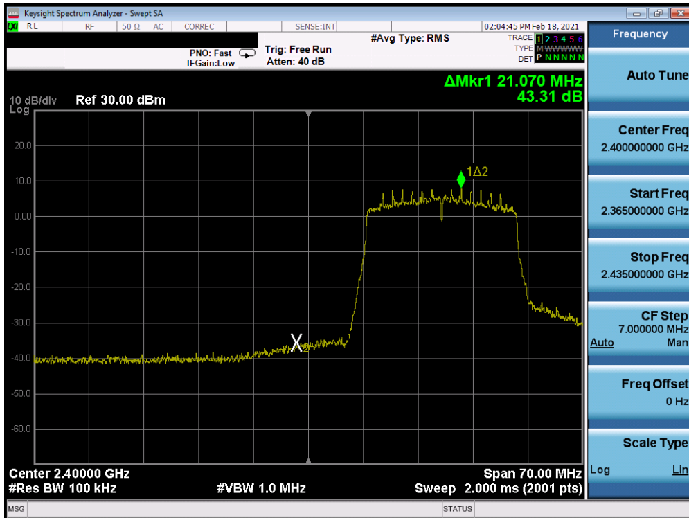
Plot 7-254. Band Edge Plot Antenna 8 (802.11ax (SU – 2.4GHz) – Ch. 2) – MCS0
