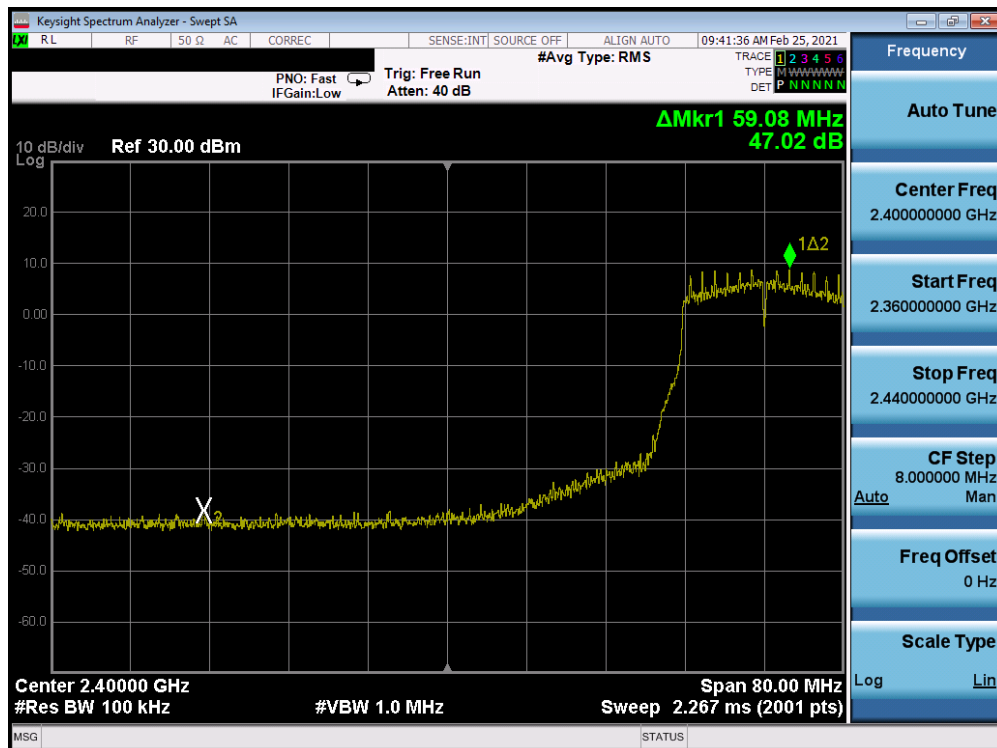
Plot 7-304. Band Edge Plot Antenna 7 (802.11g- Ch. 5) – 18Mbps
