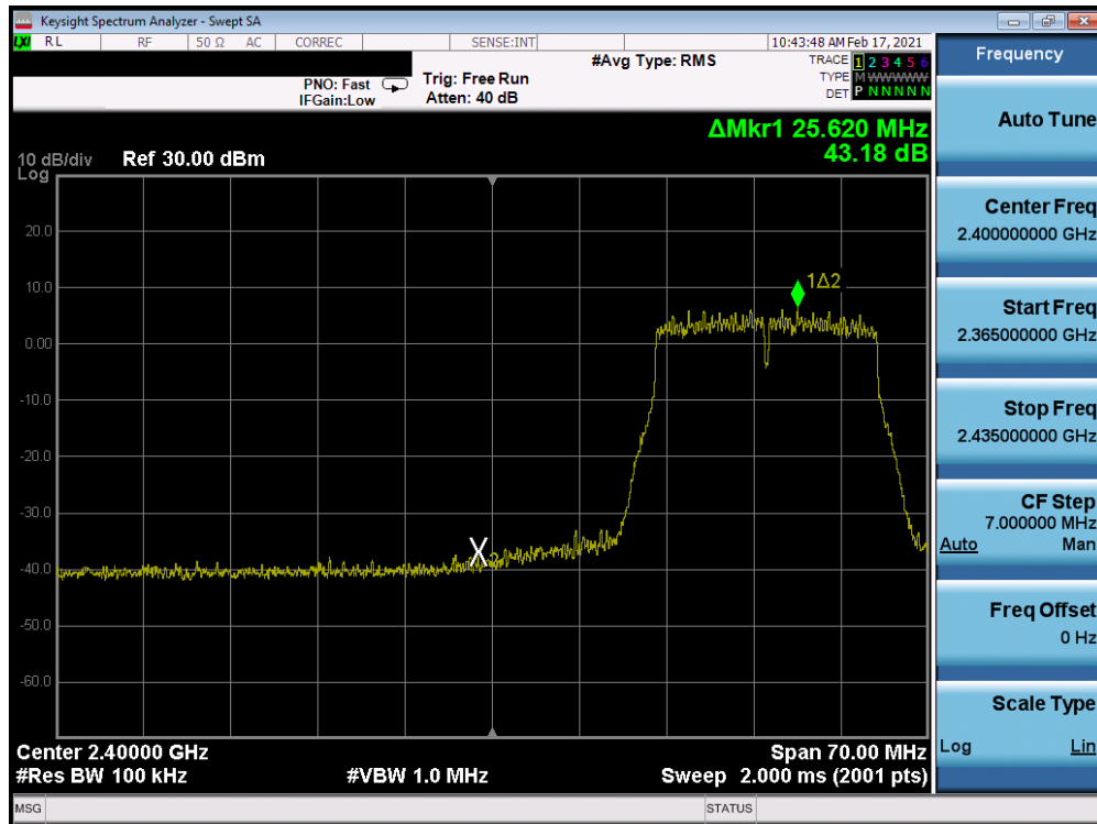
Plot 7-223. Band Edge Plot Antenna 8 (802.11n (2.4GHz) – Ch. 3) – MCS7
