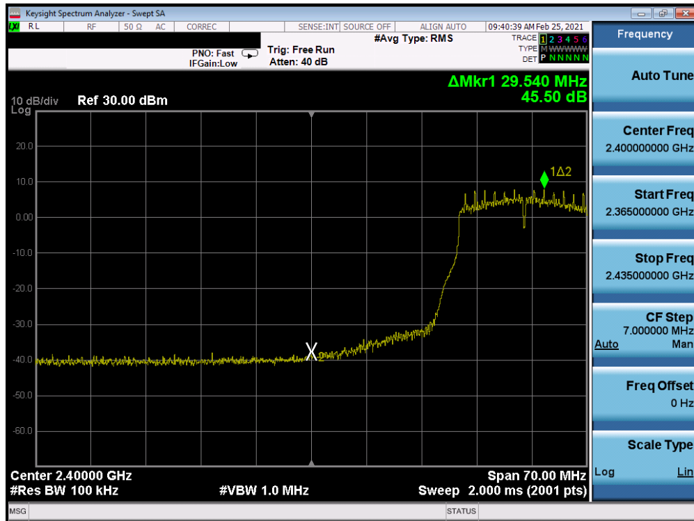
Plot 7-301. Band Edge Plot Antenna 7 (802.11g- Ch. 4) – 18Mbps
