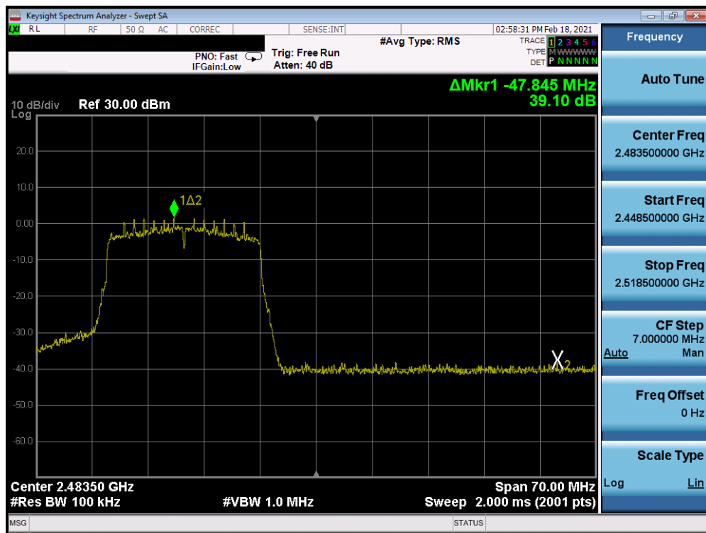
Plot 7-284. Band Edge Plot Antenna 8 (802.11ax (SU – 2.4GHz) – Ch. 12) – MCS0
