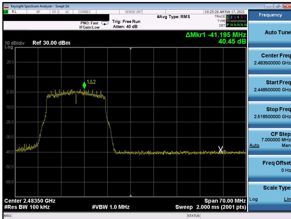
Plot 7-246. Band Edge Plot Antenna 8 (802.11n (2.4GHz) – Ch. 12) – MCS3
