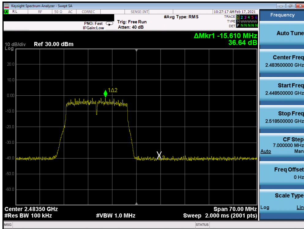
Plot 7-249. Band Edge Plot Antenna 8 (802.11n (2.4GHz) – Ch. 13) – MCS3
