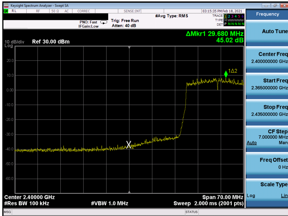
Plot 7-261. Band Edge Plot Antenna 8 (802.11ax (SU – 2.4GHz) – Ch. 4) – MCS3
