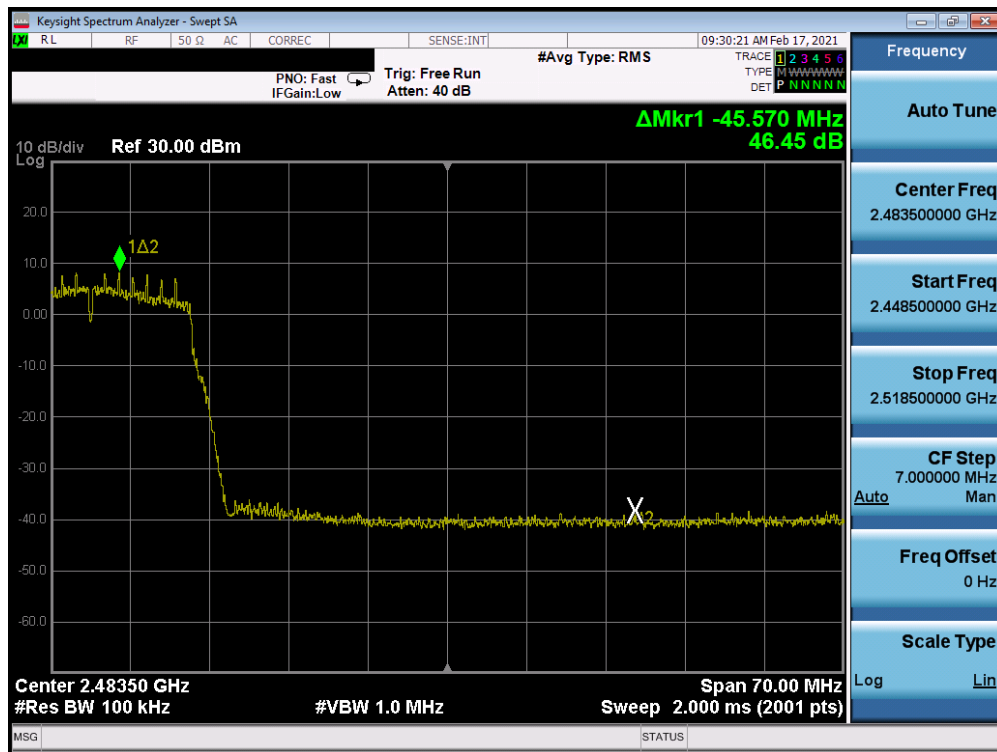
Plot 7-236. Band Edge Plot Antenna 8 (802.11n (2.4GHz) – Ch. 9) – MCS0
