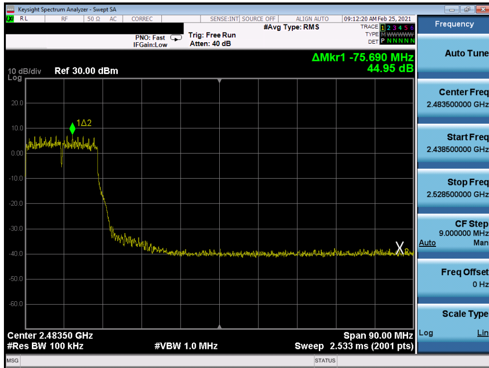
Plot 7-199. Band Edge Plot Antenna 8 (802.11g – Ch. 8) – 54Mbps
