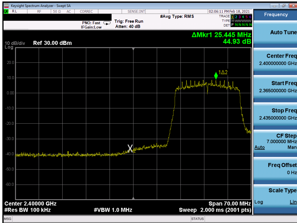
Plot 7-257. Band Edge Plot Antenna 8 (802.11ax (SU – 2.4GHz) – Ch. 3) – MCS0
