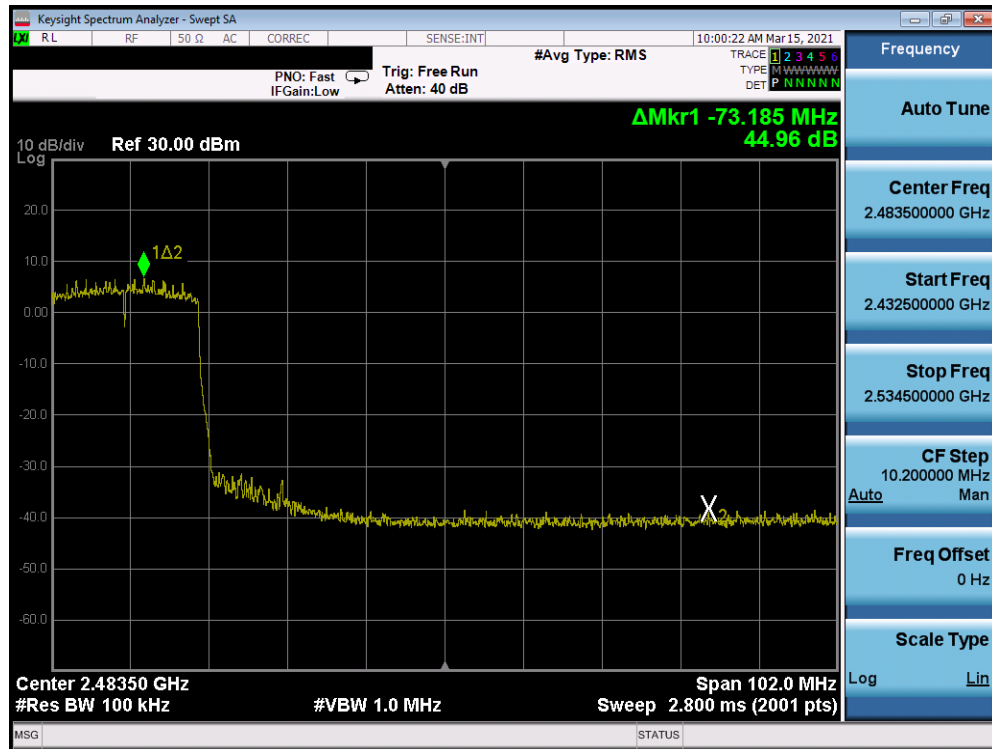
Plot 7-271: Band Edge Plot Antenna 8 (802.11ax (SU – 2.4GHz) – Ch. 7) – MCS5
