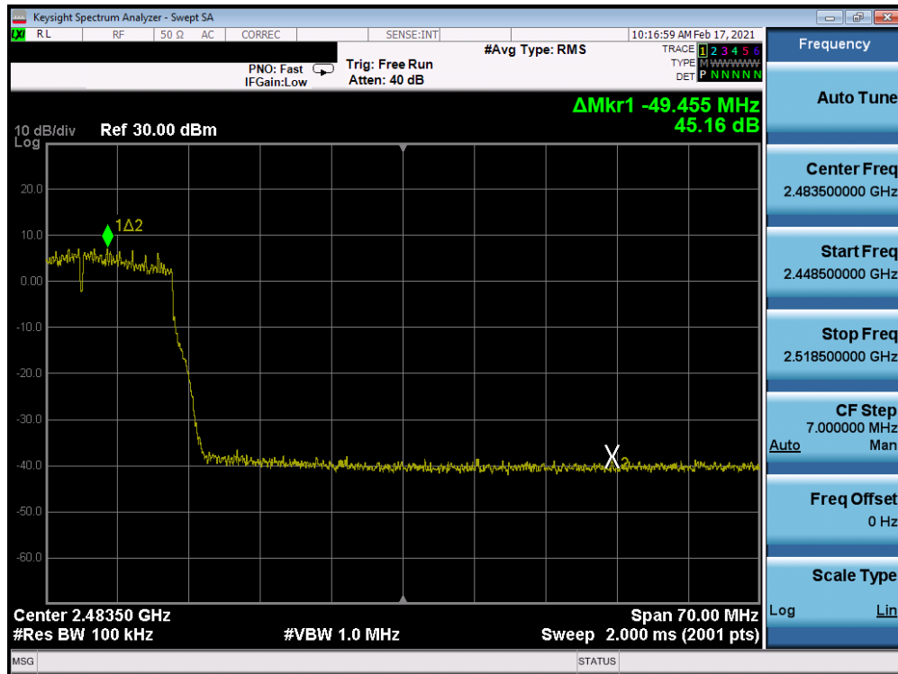
Plot 7-237. Band Edge Plot Antenna 8 (802.11n (2.4GHz) – Ch. 9) – MCS3
