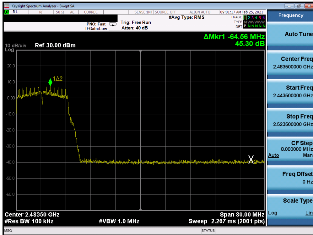
Plot 7-201. Band Edge Plot Antenna 8 (802.11g - Ch. 9) - 18Mbps
