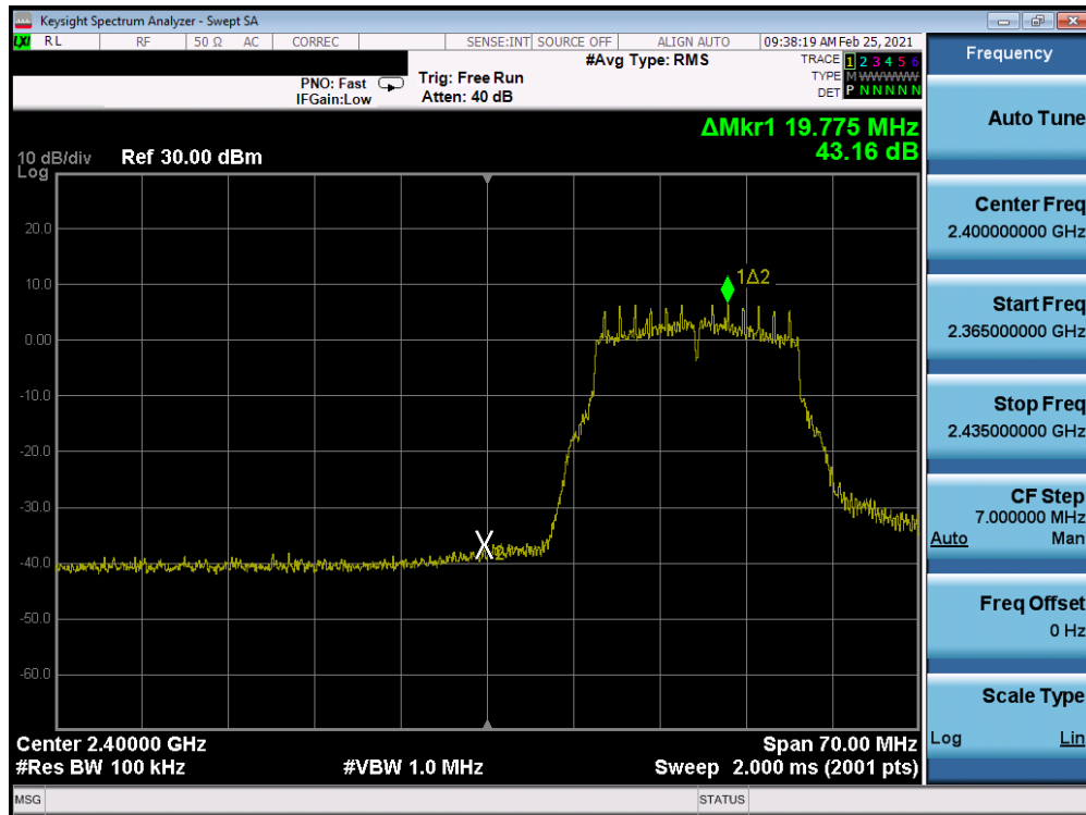
Plot 7-295. Band Edge Plot Antenna 7 (802.11g- Ch. 2) – 18Mbps
