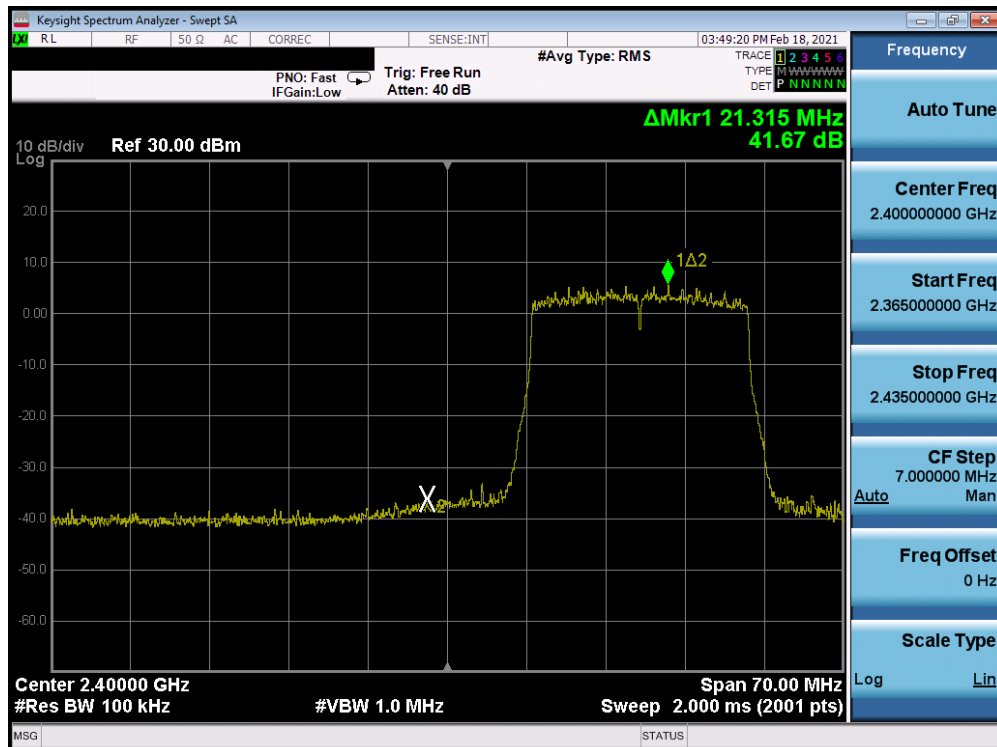
Plot 7-256. Band Edge Plot Antenna 8 (802.11ax (SU – 2.4GHz) – Ch. 2) – MCS5
