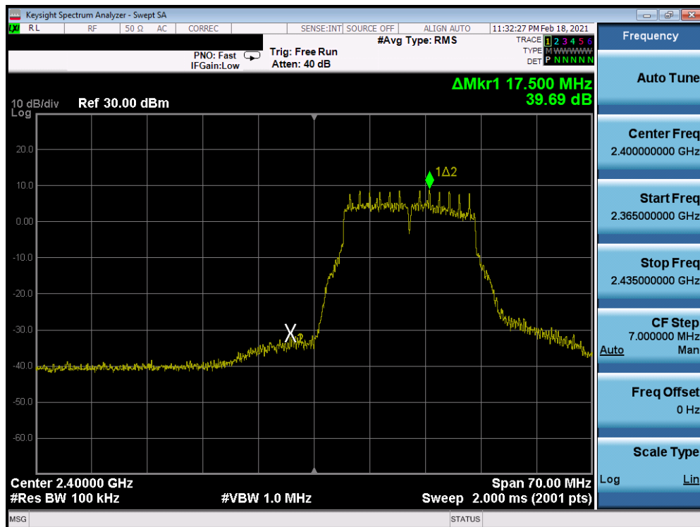
Plot 7-292. Band Edge Plot Antenna 7 (802.11g- Ch. 1) – 18Mbps
