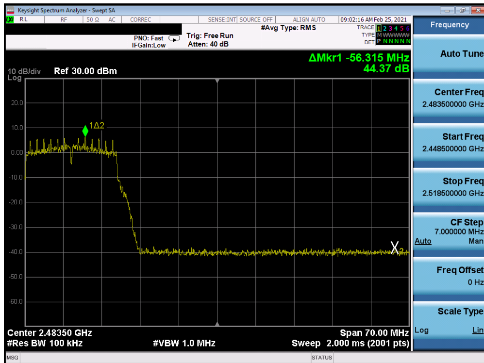
Plot 7-204. Band Edge Plot Antenna 8 (802.11g - Ch. 10) - 18Mbps
