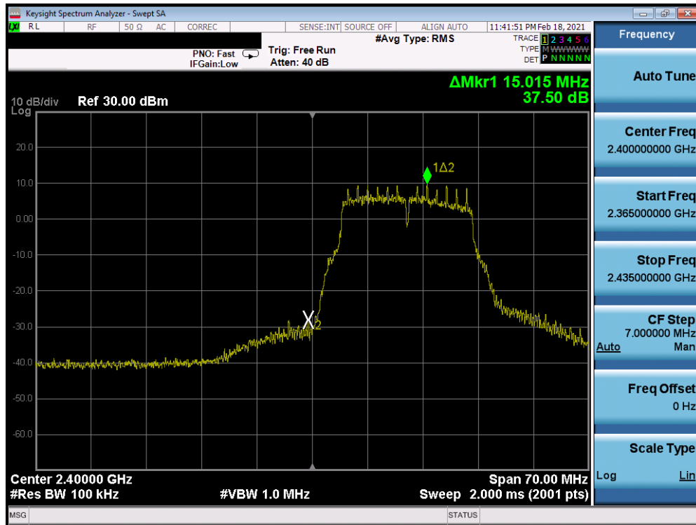
Plot 7-291. Band Edge Plot Antenna 7 (802.11g- Ch. 1) – 6Mbps
