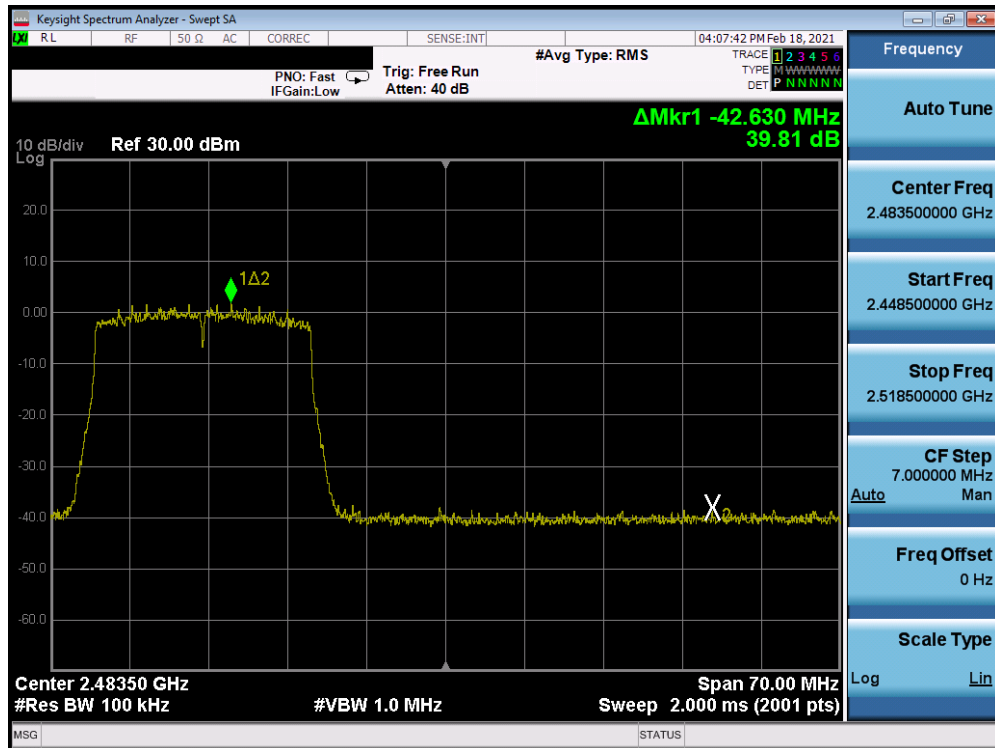
Plot 7-283. Band Edge Plot Antenna 8 (802.11ax (SU – 2.4GHz) – Ch. 11) – MCS5
