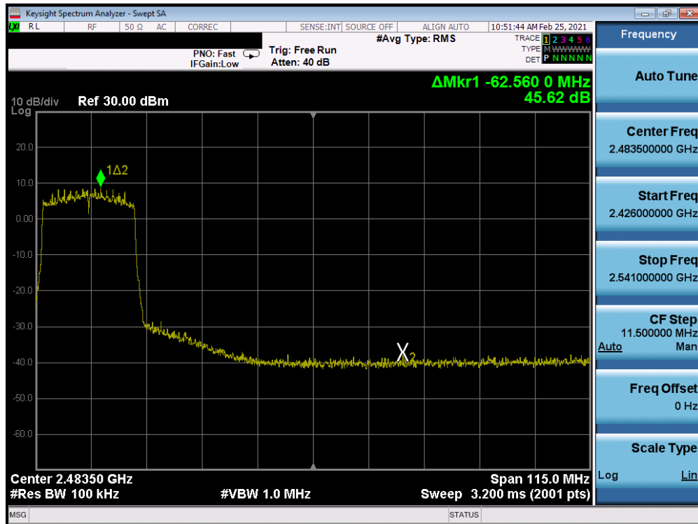
Plot 7-268: Band Edge Plot Antenna 8 (802.11ax (SU – 2.4GHz) – Ch. 6) – MCS3
