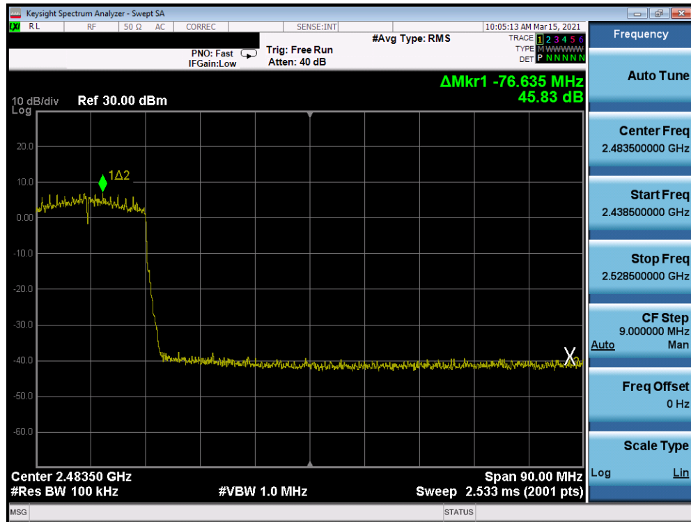
Plot 7-273: Band Edge Plot Antenna 8 (802.11ax (SU – 2.4GHz) – Ch. 8) – MCS3
