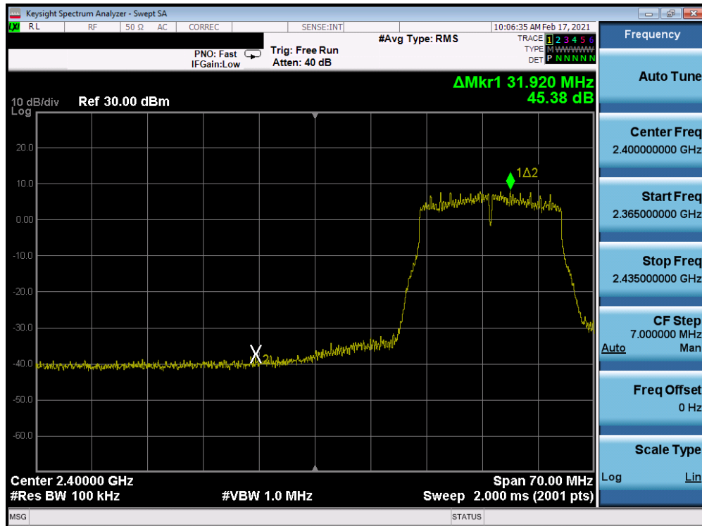
Plot 7-222. Band Edge Plot Antenna 8 (802.11n (2.4GHz) – Ch. 3) – MCS3
