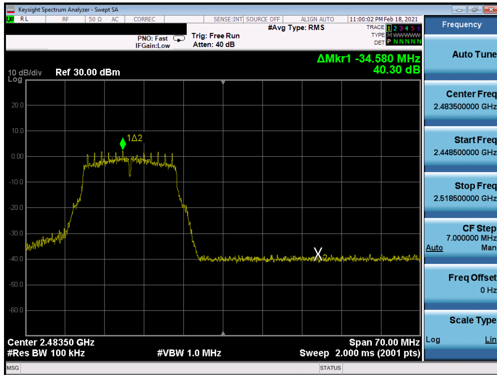
Plot 7-209. Band Edge Plot Antenna 8 (802.11g - Ch. 12) - 6Mbps
