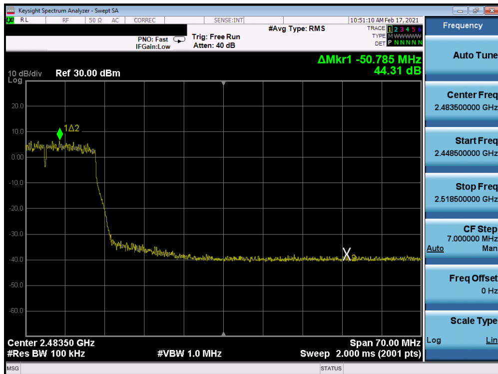
Plot 7-238. Band Edge Plot Antenna 8 (802.11n (2.4GHz) – Ch. 9) – MCS7
