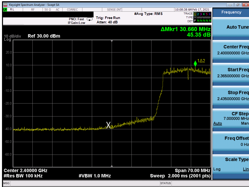
Plot 7-225. Band Edge Plot Antenna 8 (802.11n (2.4GHz) – Ch. 4) – MCS3
