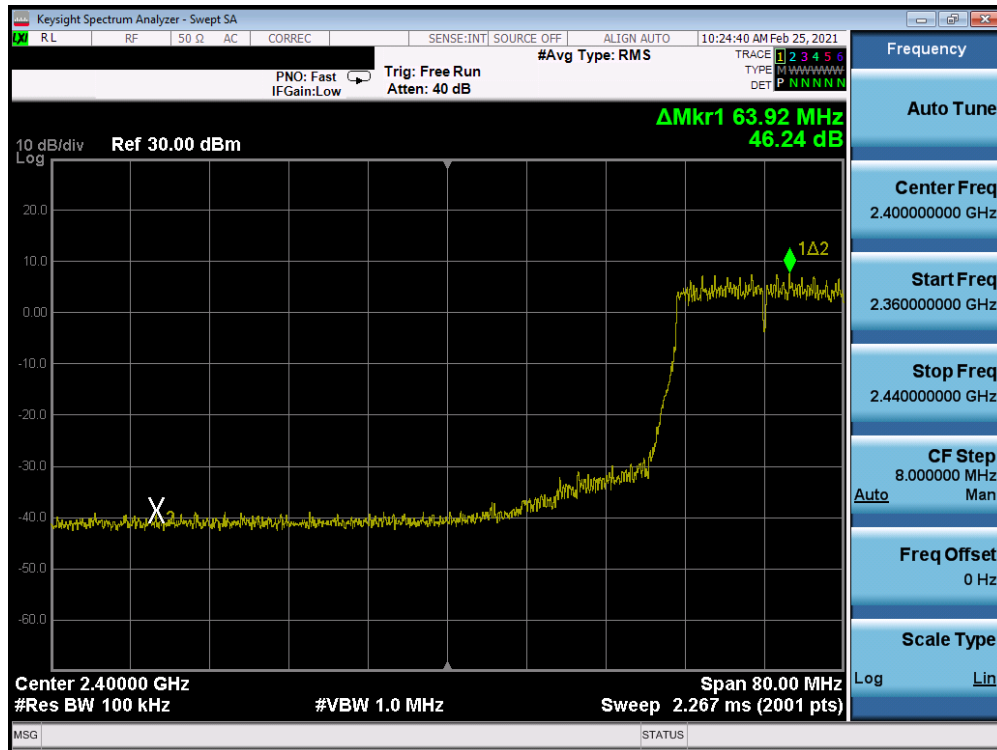
Plot 7-229. Band Edge Plot Antenna 8 (802.11n (2.4GHz) - Ch. 5) - MCS7
