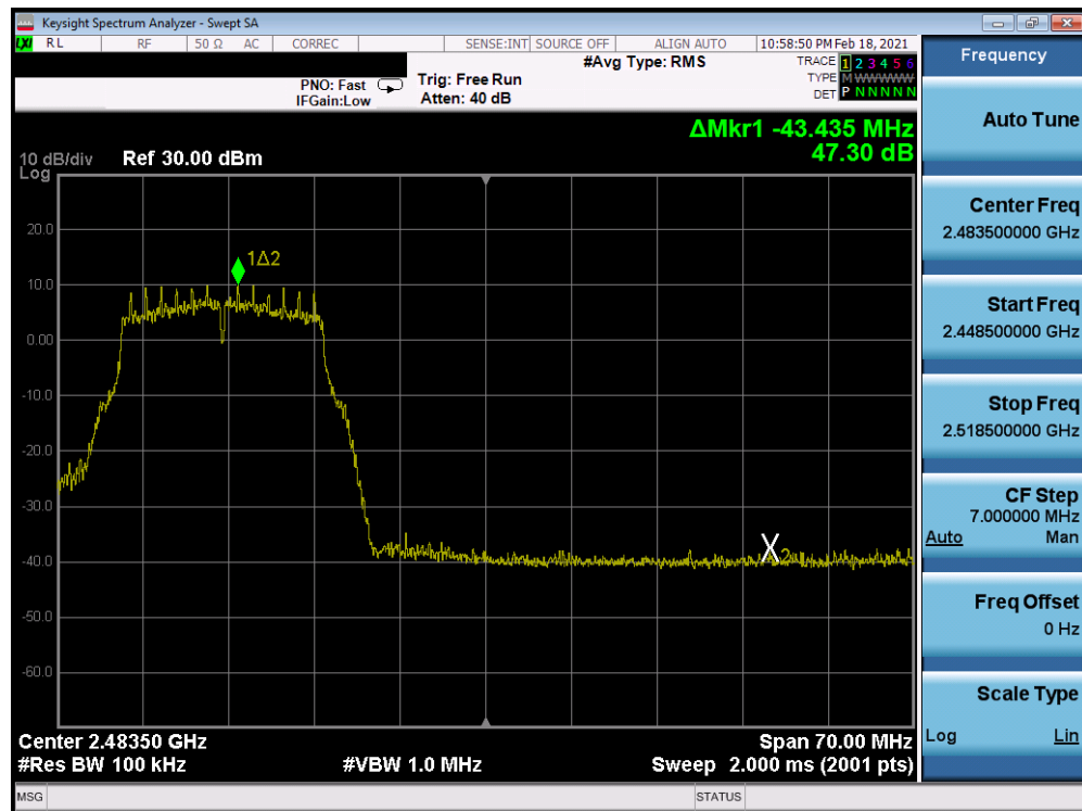
Plot 7-206. Band Edge Plot Antenna 8 (802.11g - Ch. 11) - 6Mbps
