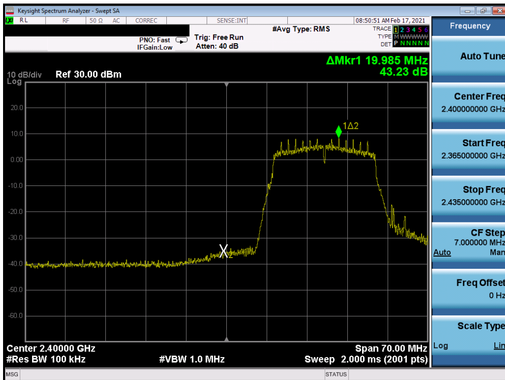
Plot 7-218. Band Edge Plot Antenna 8 (802.11n (2.4GHz) – Ch. 2) – MCS0
