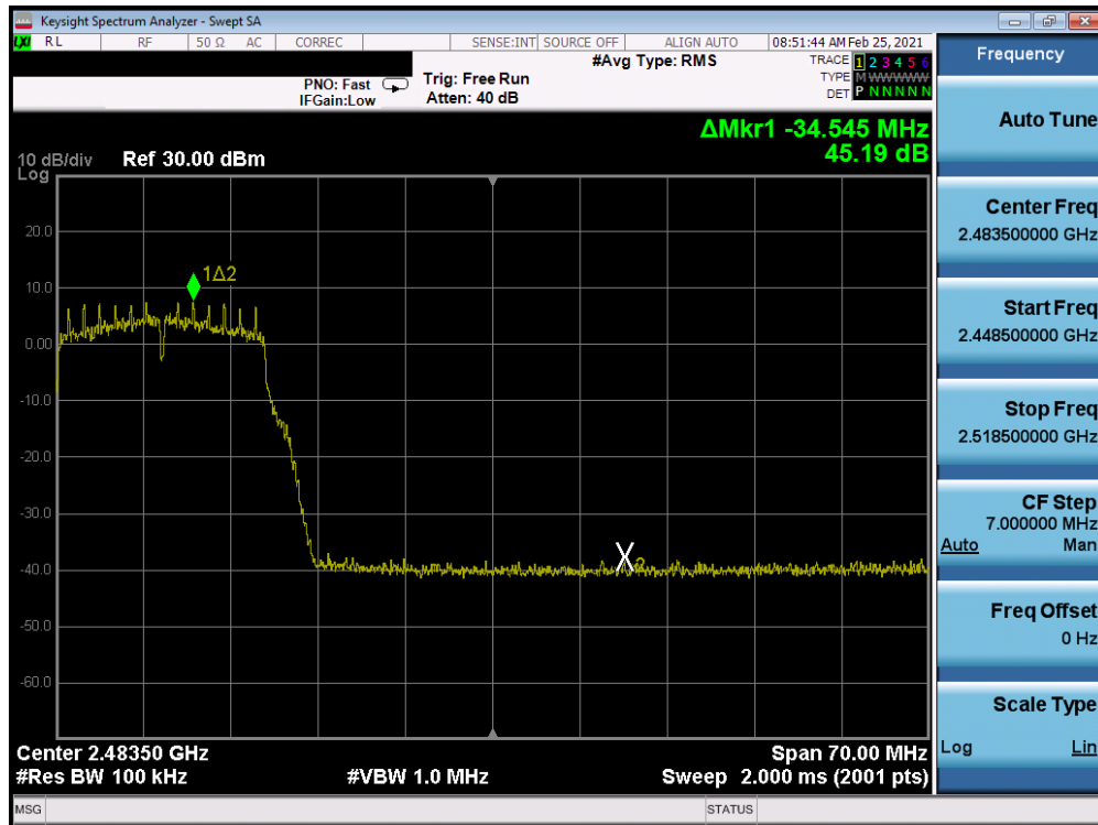
Plot 7-203. Band Edge Plot Antenna 8 (802.11g - Ch. 10) - 6Mbps
