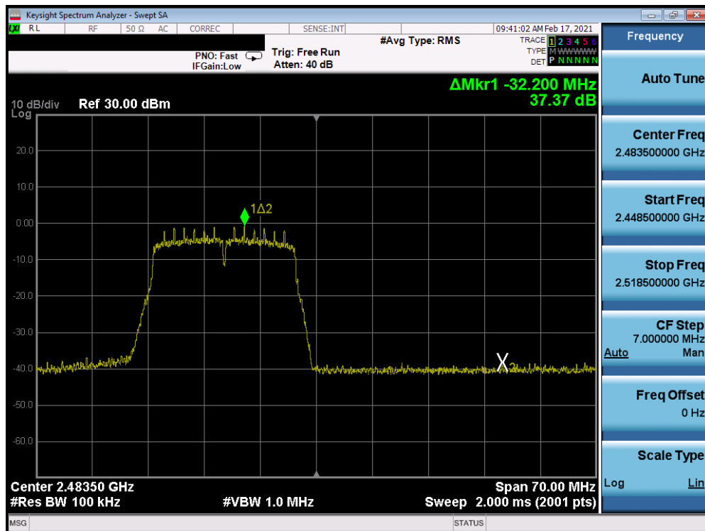
Plot 7-248. Band Edge Plot Antenna 8 (802.11n (2.4GHz) – Ch. 13) – MCS0
