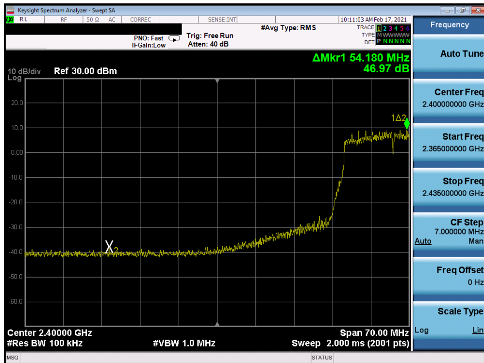
Plot 7-228. Band Edge Plot Antenna 8 (802.11n (2.4GHz) – Ch. 5) – MCS3
