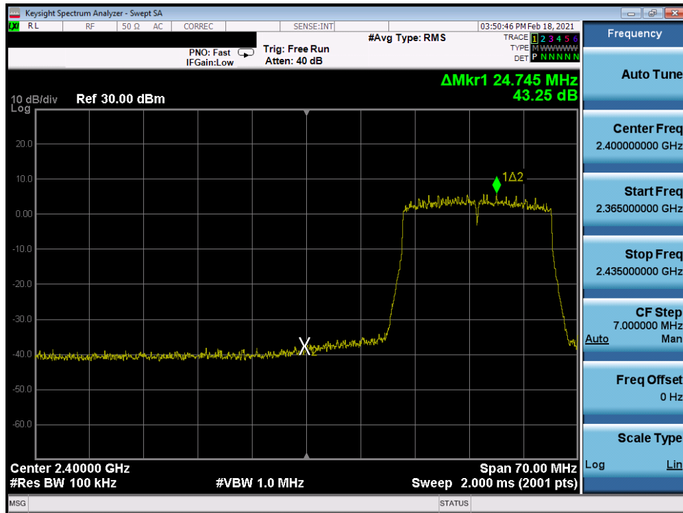
Plot 7-259: Band Edge Plot Antenna 8 (802.11ax (SU – 2.4GHz) – Ch. 3) – MCS5
