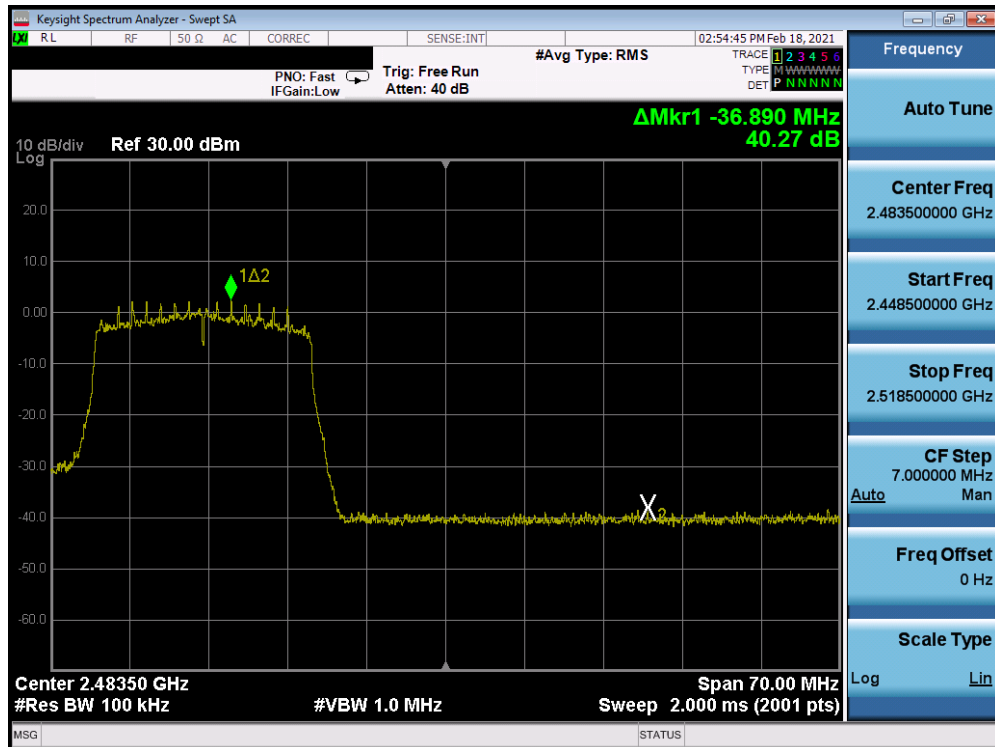
Plot 7-281. Band Edge Plot Antenna 8 (802.11ax (SU – 2.4GHz) – Ch. 11) – MCS0
