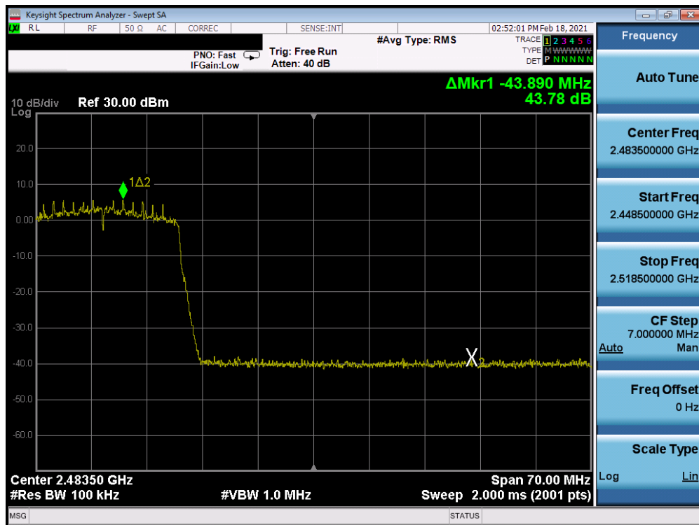
Plot 7-278. Band Edge Plot Antenna 8 (802.11ax (SU – 2.4GHz) – Ch. 10) – MCS0
