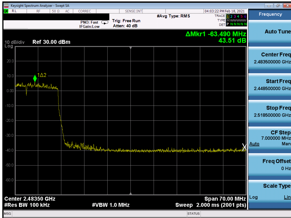
Plot 7-277. Band Edge Plot Antenna 8 (802.11ax (SU – 2.4GHz) – Ch. 9) – MCS5
