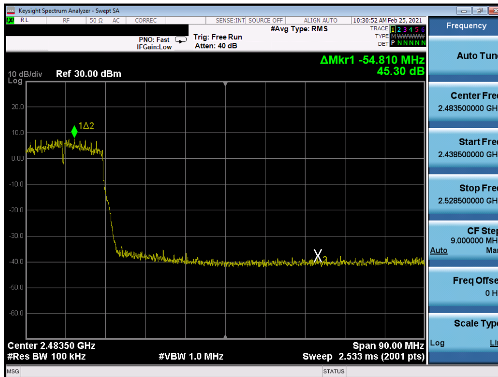
Plot 7-234. Band Edge Plot Antenna 8 (802.11n (2.4GHz) – Ch. 8) – MCS3
