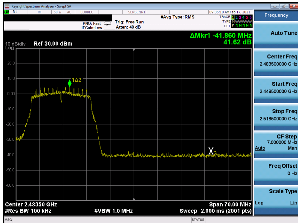
Plot 7-242. Band Edge Plot Antenna 8 (802.11n (2.4GHz) – Ch. 11) – MCS0
