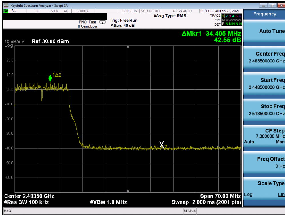
Plot 7-205. Band Edge Plot Antenna 8 (802.11g - Ch. 10) - 54Mbps
