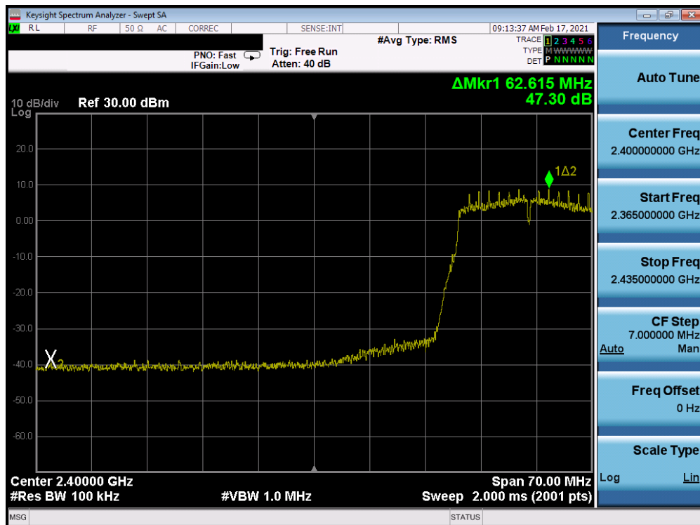
Plot 7-224: Band Edge Plot Antenna 8 (802.11n (2.4GHz) – Ch. 4) – MCS0
