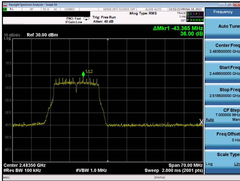
Plot 7-213. Band Edge Plot Antenna 8 (802.11g - Ch. 13) - 18Mbps
