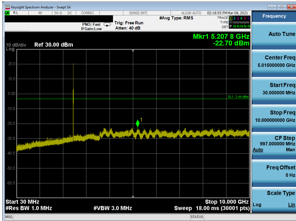
Plot 7-123. Conducted Spurious Plot Antenna 8 (802.11ax OFDMA – RU26 – Ch. 11)
