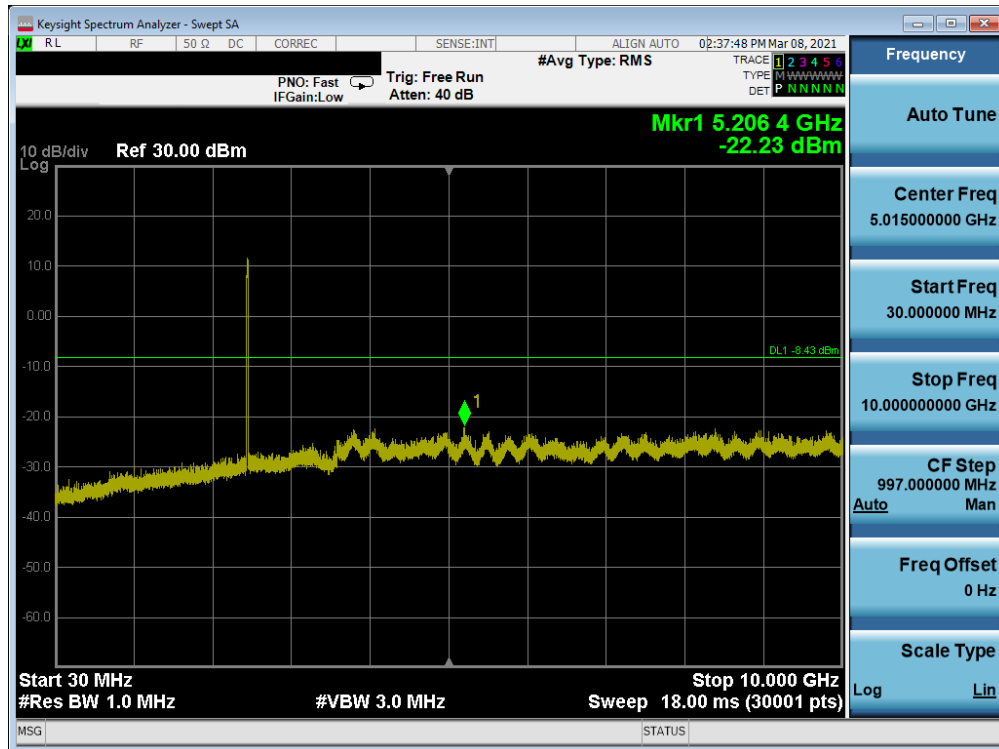
Plot 7-129. Conducted Spurious Plot Antenna 8 (802.11ax OFDMA – RU242 – Ch. 11)
