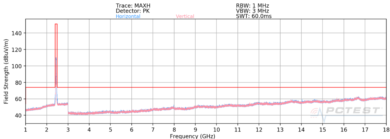
Plot 7-147. Radiated Spurious Emissions above 1GHz Antenna 8 (802.11ax OFDMA – RU242 – Ch. 6)
