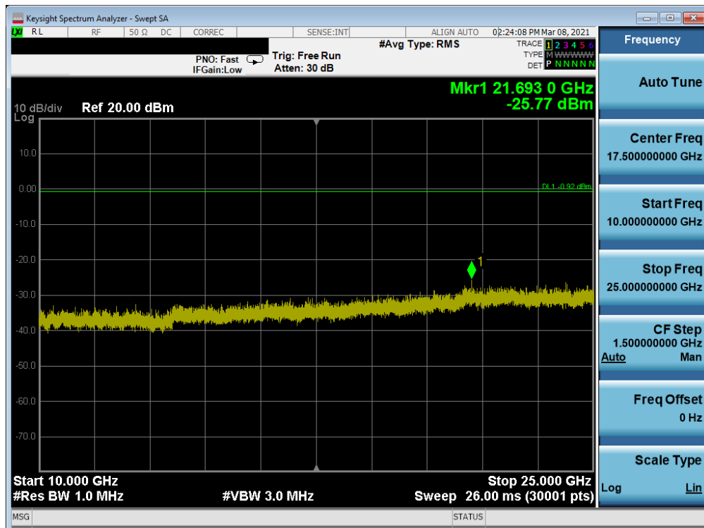
Plot 7-122. Conducted Spurious Plot Antenna 8 (802.11ax OFDMA – RU26 – Ch. 6)
