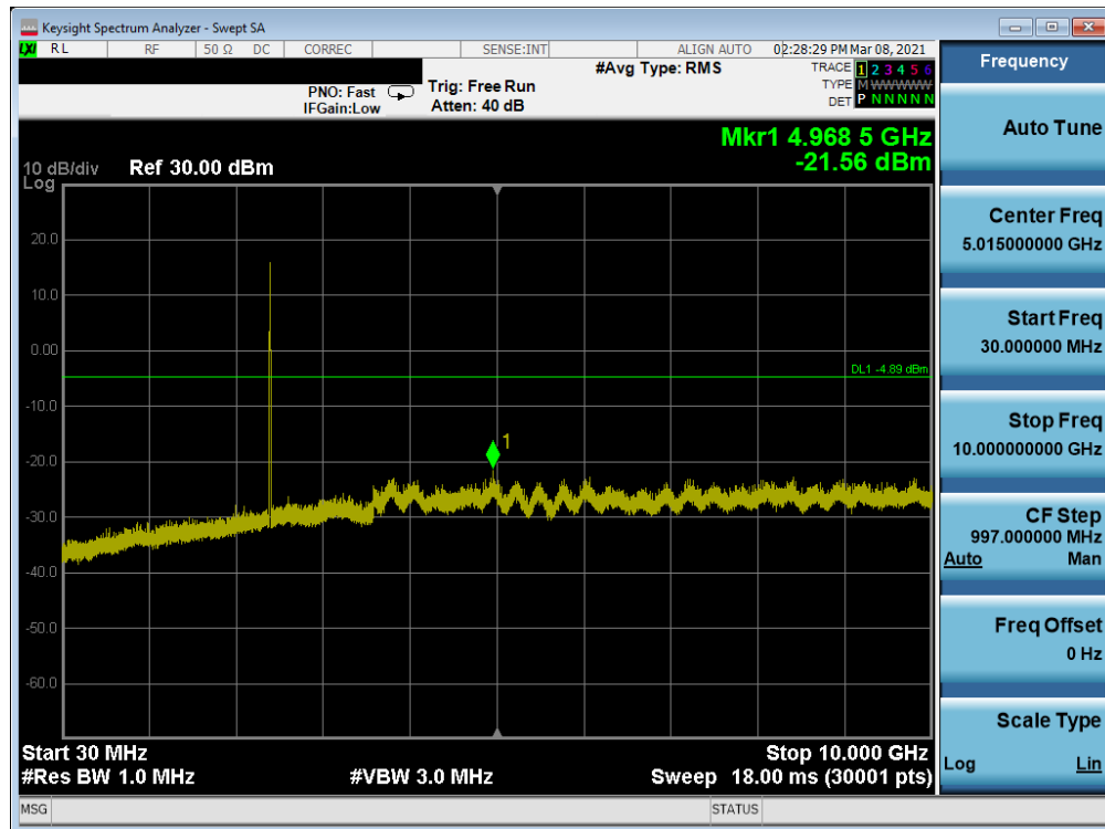
Plot 7-119. Conducted Spurious Plot Antenna 8 (802.11ax OFDMA – RU26 – Ch. 1)
