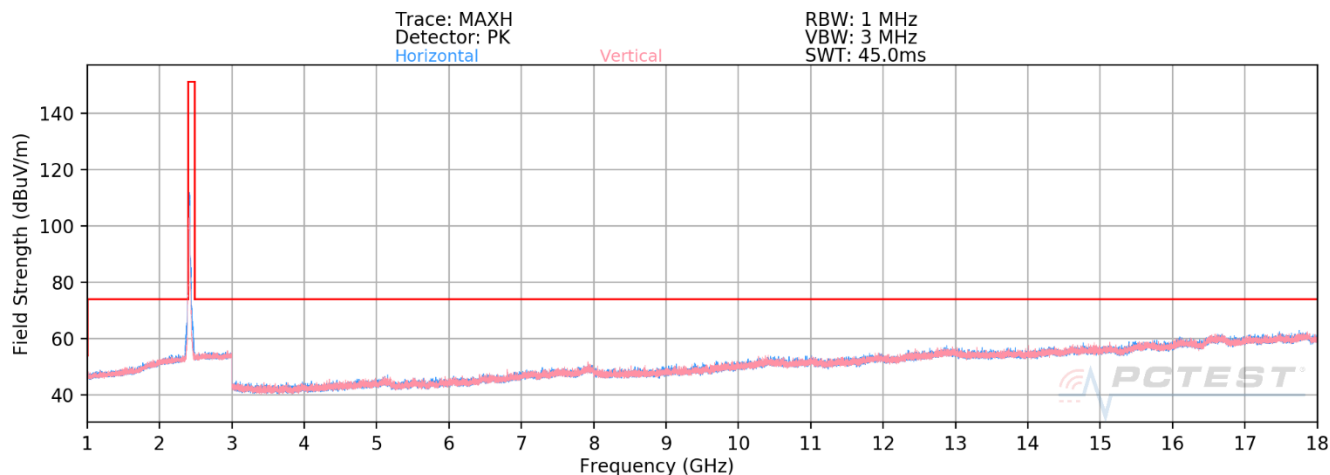
Plot 7-146. Radiated Spurious Emissions above 1GHz Antenna 8 (802.11ax OFDMA – RU242 – Ch. 1)
