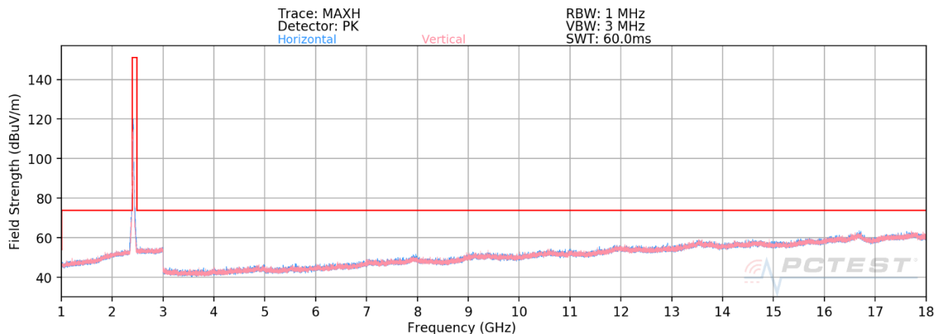
Plot 7-160. Radiated Spurious Emissions above 1GHz CDD (802.11ax OFDMA – RU242 – Ch. 1)
