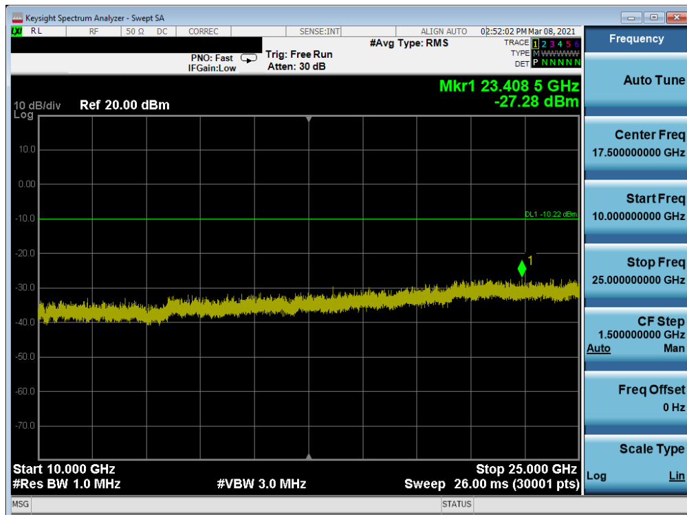
Plot 7-138. Conducted Spurious Plot Antenna 7 (802.11ax OFDMA – RU242 – Ch. 1)
