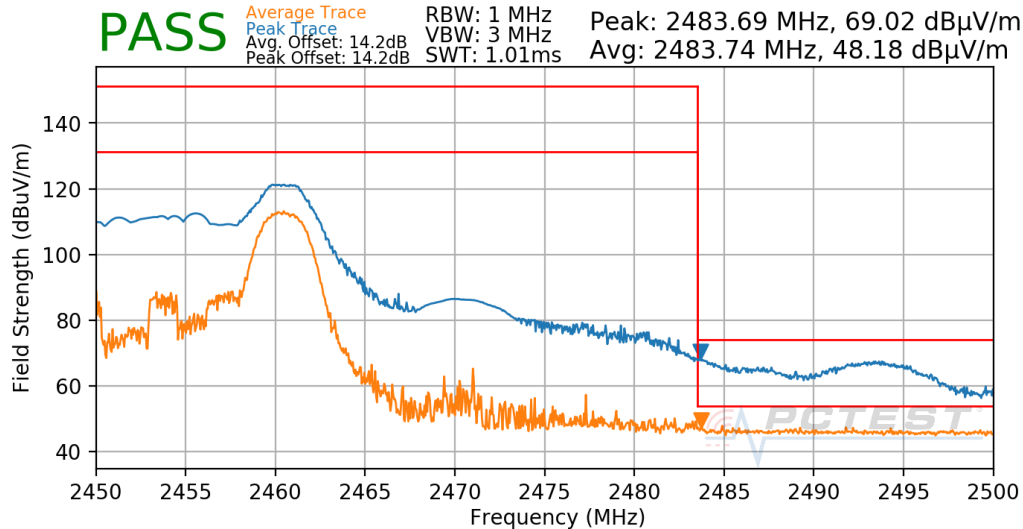
Plot 7-170. Radiated Restricted Upper Band Edge Measurement Antenna 8 (Peak & Average – RU26)
