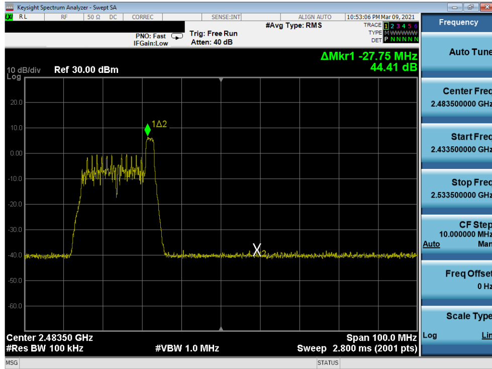
Plot 7-104. Band Edge Antenna 7 (802.11ax OFDMA – RU26 Index 8 – Ch. 10)
