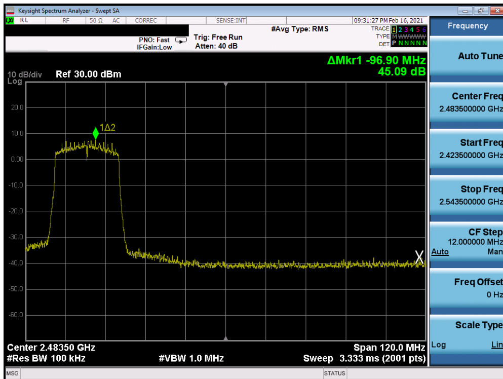
Plot 7-113. Band Edge Antenna 7 (802.11ax OFDMA – RU242 – Ch. 7)
