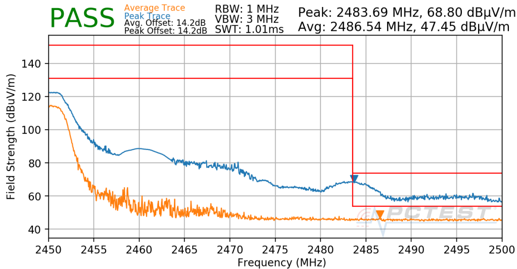
Plot 7-168. Radiated Restricted Upper Band Edge Measurement Antenna 8 (Peak & Average – RU26)
