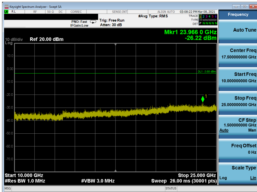
Plot 7-136. Conducted Spurious Plot Antenna 7 (802.11ax OFDMA – RU26 – Ch. 11)
