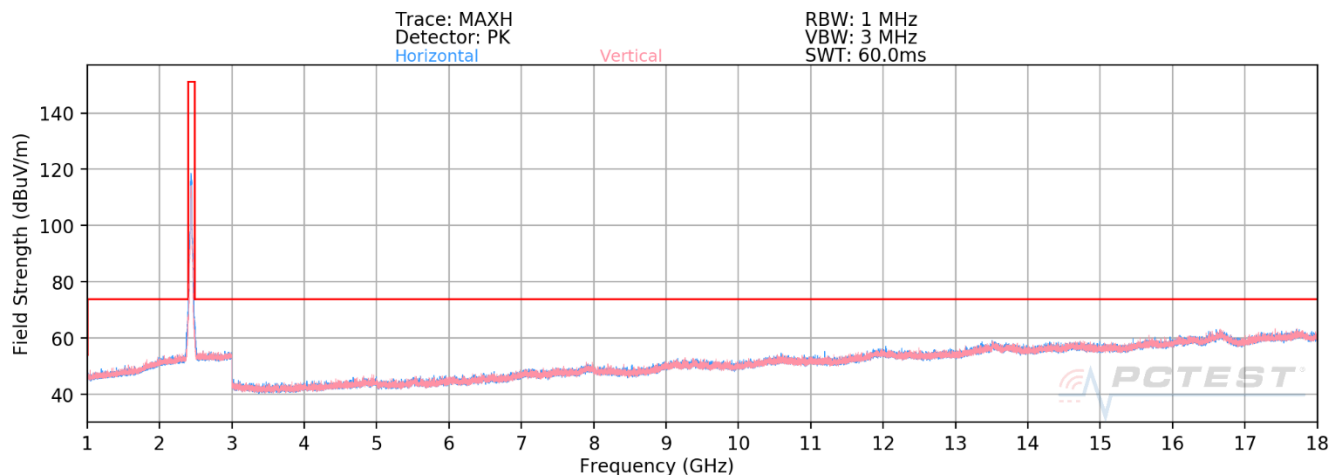
Plot 7-161. Radiated Spurious Emissions above 1GHz CDD (802.11ax OFDMA – RU242 – Ch. 6)
