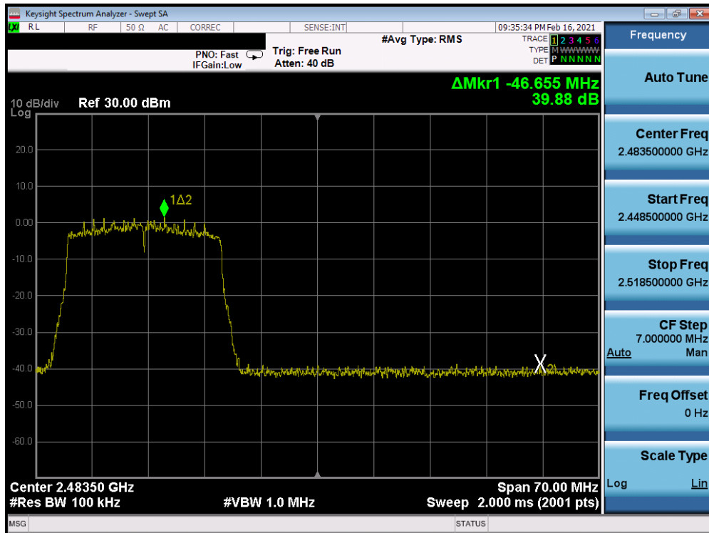
Plot 7-117. Band Edge Antenna 7 (802.11ax OFDMA – RU242 – Ch. 11)
