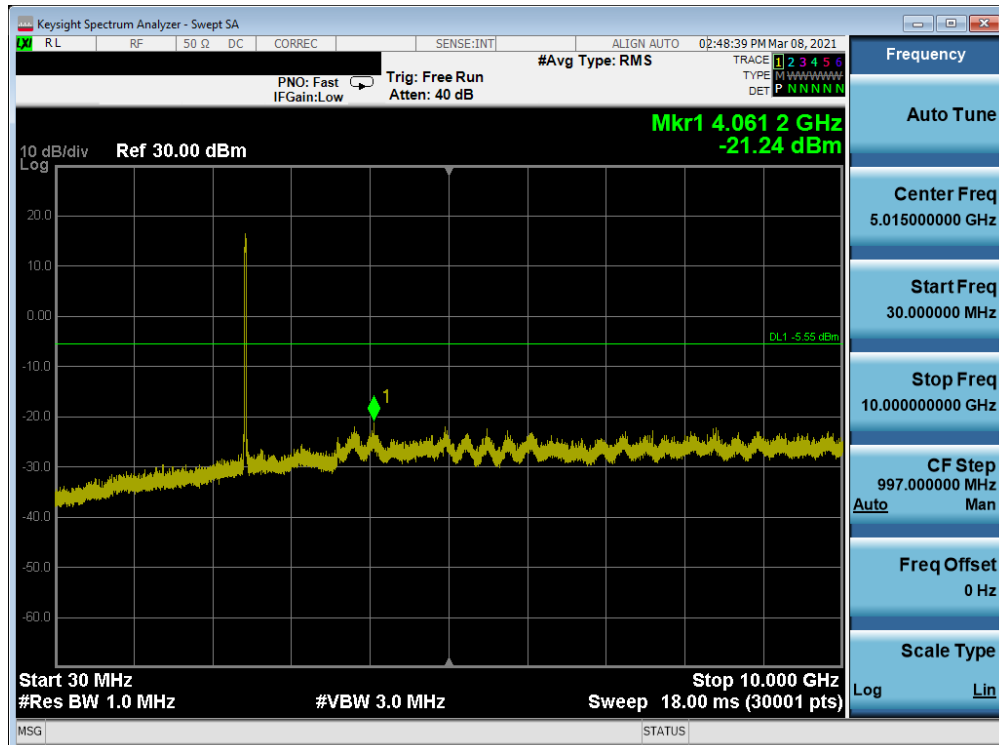
Plot 7-139. Conducted Spurious Plot Antenna 7 (802.11ax OFDMA – RU242 – Ch. 6)
