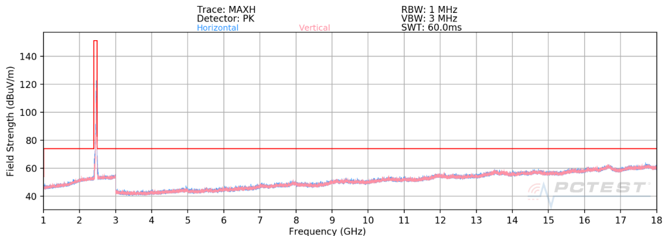
Plot 7-151. Radiated Spurious Emissions above 1GHz Antenna 7 (802.11ax OFDMA – RU26 – Ch. 11)
