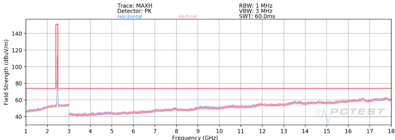
Plot 7-145. Radiated Spurious Emissions above 1GHz Antenna 8 (802.11ax OFDMA – RU26 – Ch. 11)
