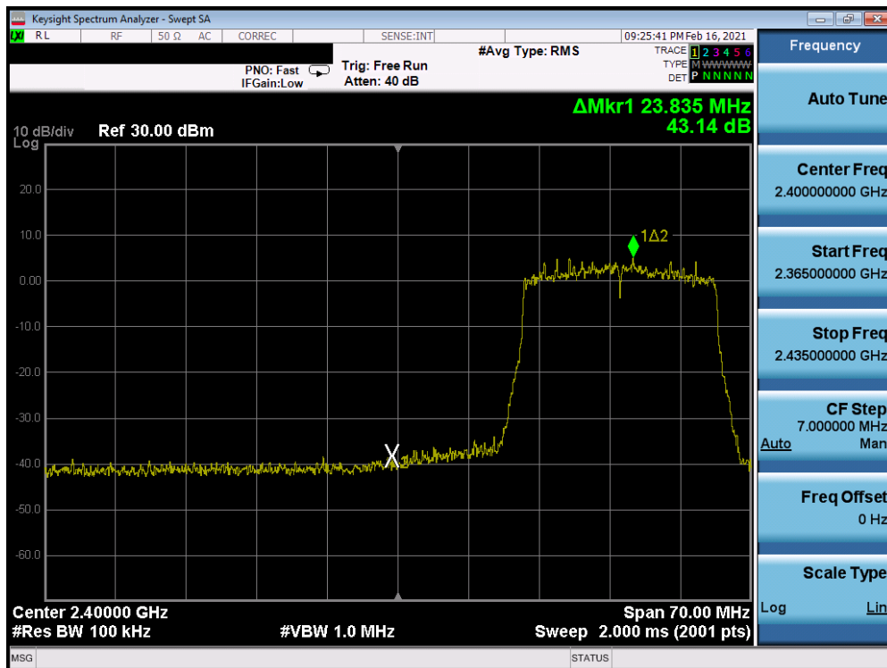
Plot 7-109. Band Edge Antenna 7 (802.11ax OFDMA - RU242 - Ch. 3)
