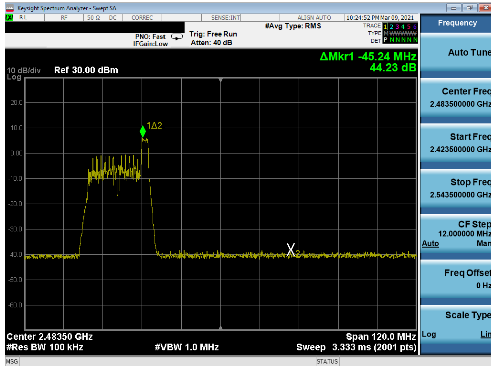
Plot 7-103. Band Edge Antenna 7 (802.11ax OFDMA – RU26 Index 8 – Ch. 9)
