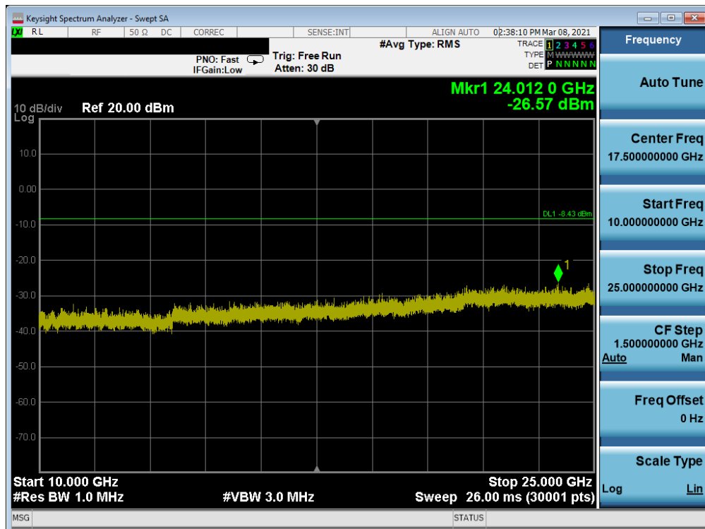
Plot 7-130. Conducted Spurious Plot Antenna 8 (802.11ax OFDMA – RU242 – Ch. 11)
