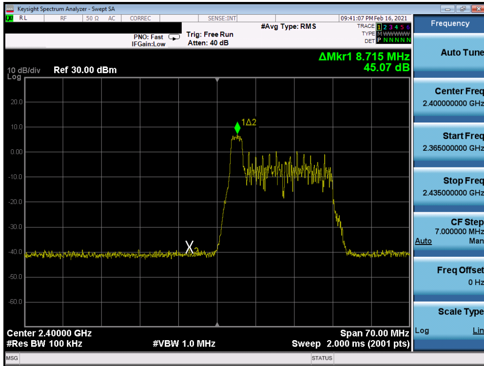
Plot 7-96. Band Edge Antenna 7 (802.11ax OFDMA – RU26 Index 0 – Ch. 1)
