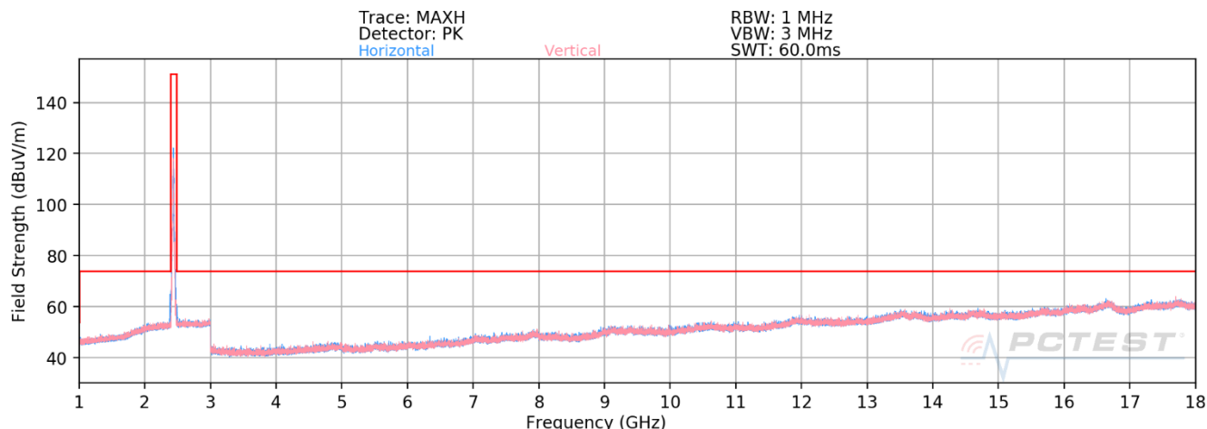
Plot 7-150. Radiated Spurious Emissions above 1GHz Antenna 7 (802.11ax OFDMA – RU26 – Ch. 6)
