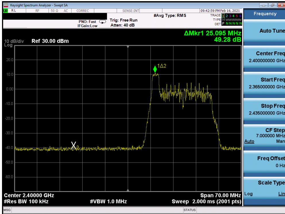
Plot 7-97. Band Edge Antenna 7 (802.11ax OFDMA – RU26 Index 0 – Ch. 2)
