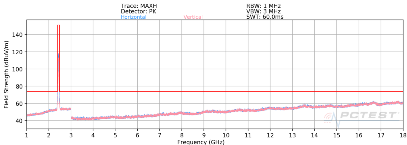
Plot 7-153. Radiated Spurious Emissions above 1GHz Antenna 7 (802.11ax OFDMA – RU242 – Ch. 6)
