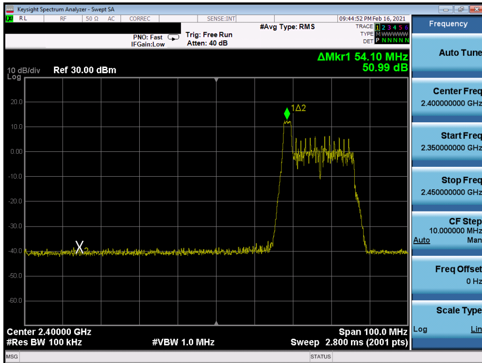
Plot 7-99. Band Edge Antenna 7 (802.11ax OFDMA – RU26 Index 0 – Ch. 4)
