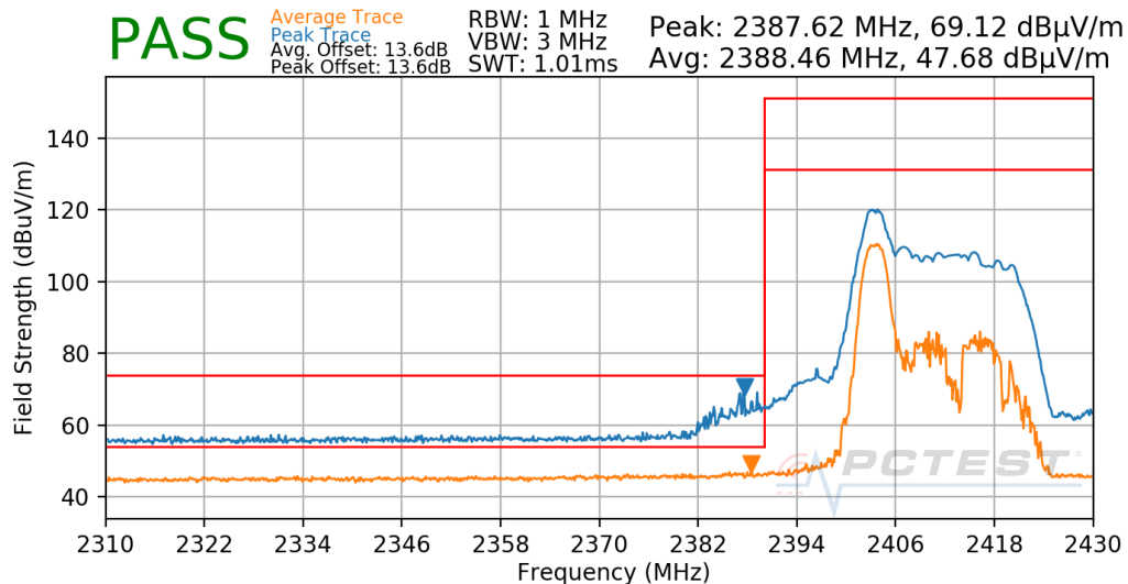
Plot 7-163. Radiated Restricted Lower Band Edge Measurement Antenna 8 (Peak & Average – RU26)
