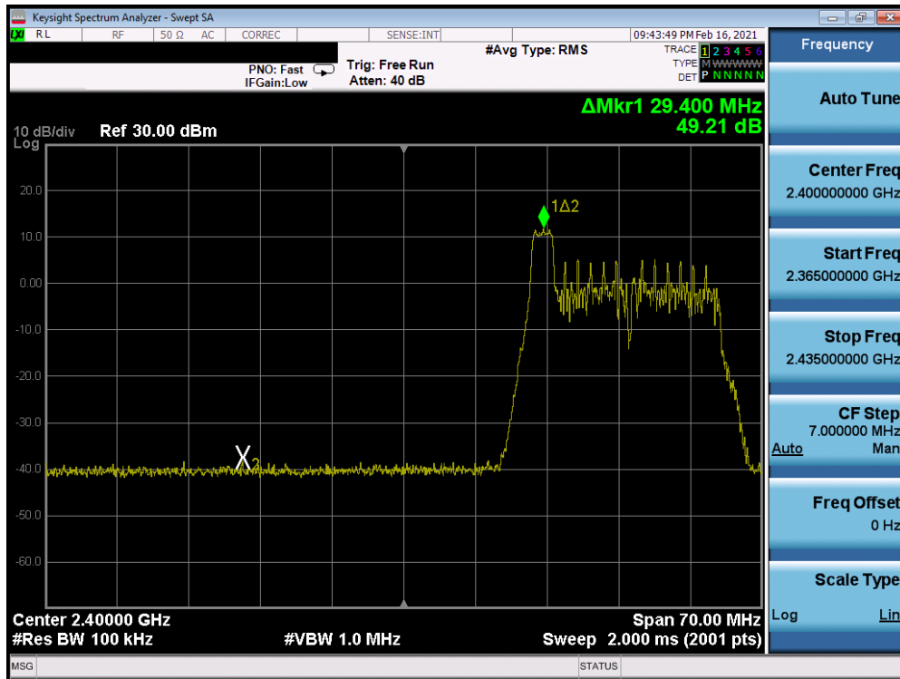
Plot 7-98. Band Edge Antenna 7 (802.11ax OFDMA – RU26 Index 0 – Ch. 3)
