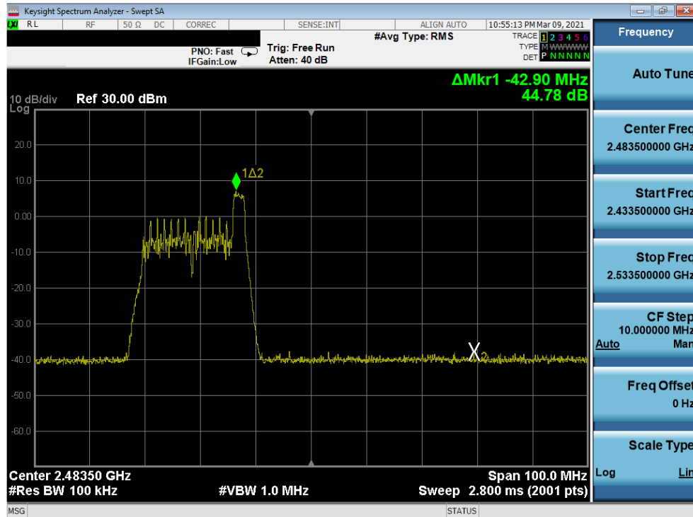
Plot 7-105. Band Edge Antenna 7 (802.11ax OFDMA – RU26 Index 8 – Ch. 11)
