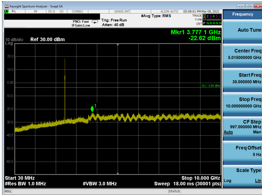
Plot 7-135. Conducted Spurious Plot Antenna 7 (802.11ax OFDMA – RU26 – Ch. 11)
