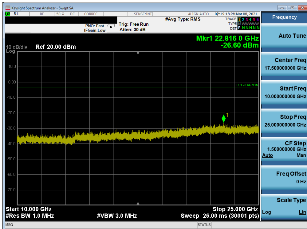
Plot 7-124. Conducted Spurious Plot Antenna 8 (802.11ax OFDMA – RU26 – Ch. 11)
