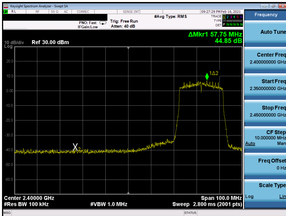
Plot 7-111. Band Edge Antenna 7 (802.11ax OFDMA – RU242 – Ch. 5)
