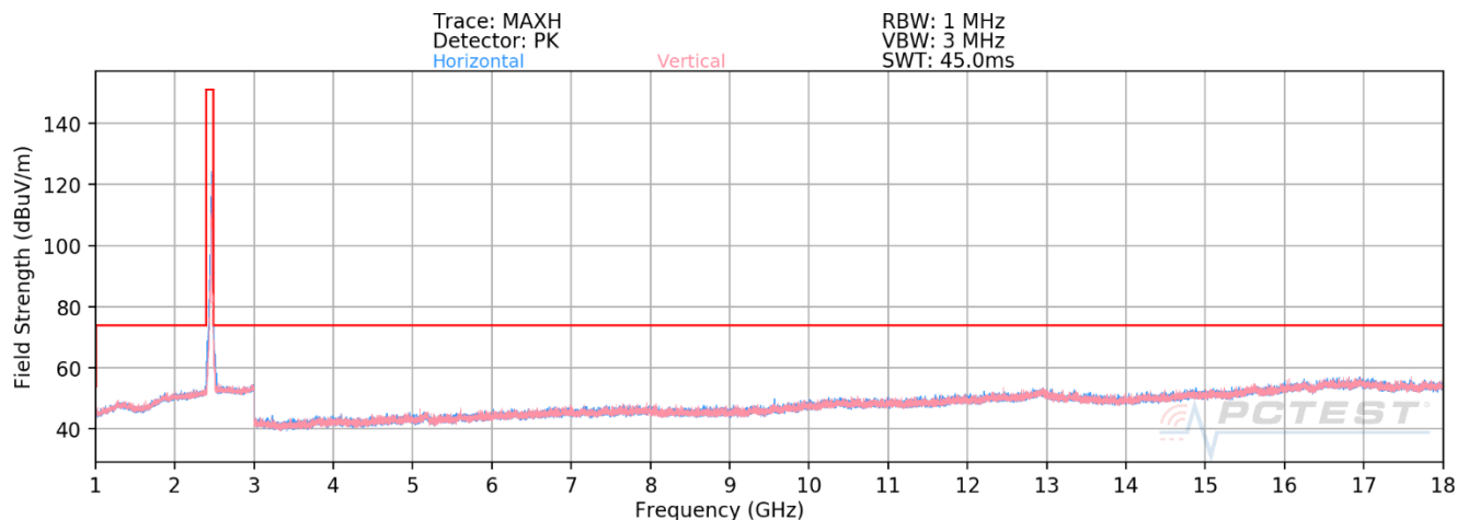
Plot 7-159. Radiated Spurious Emissions above 1GHz CDD (802.11ax OFDMA – RU26 – Ch. 11)
