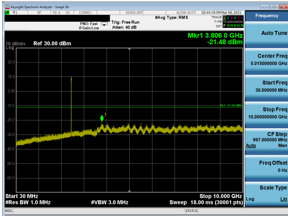
Plot 7-141. Conducted Spurious Plot Antenna 7 (802.11ax OFDMA – RU242 – Ch. 11)
