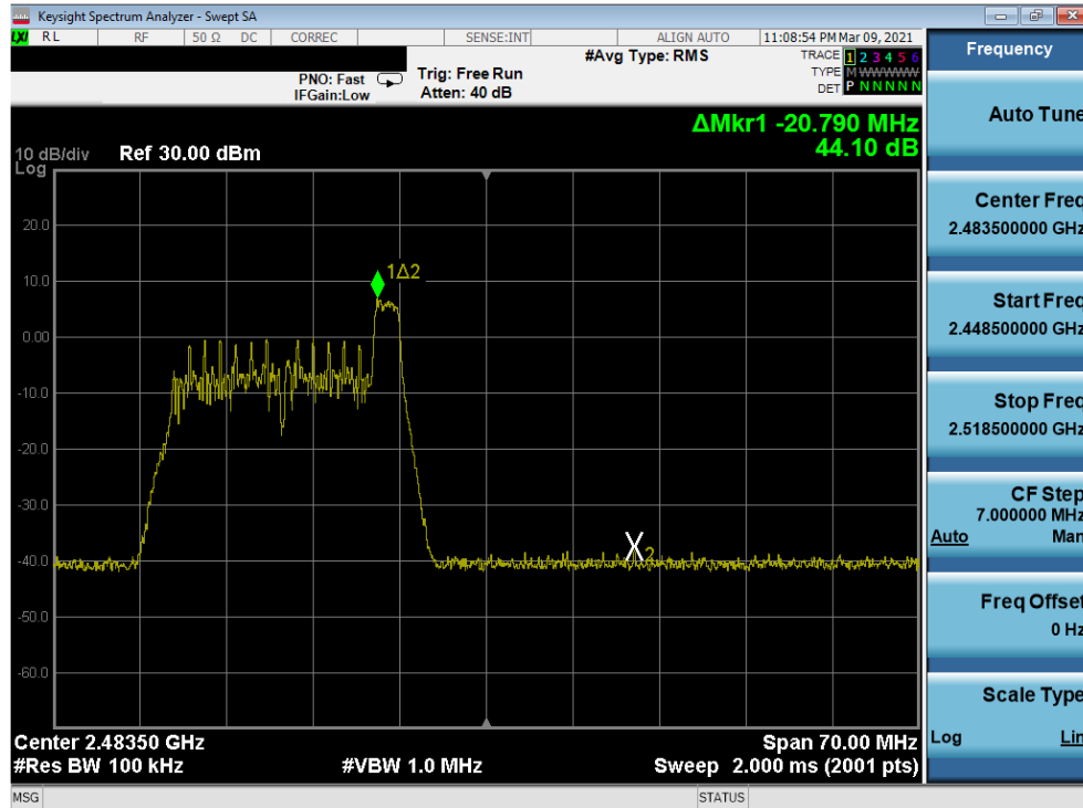
Plot 7-106. Band Edge Antenna 7 (802.11ax OFDMA – RU26 Index 8 – Ch. 12)
