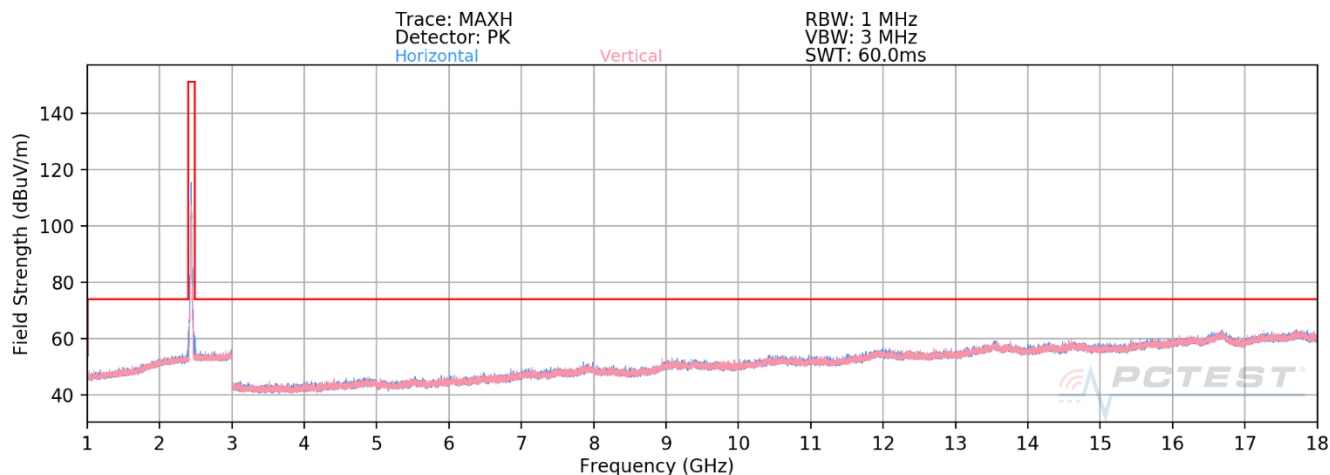
Plot 7-144. Radiated Spurious Emissions above 1GHz Antenna 8 (802.11ax OFDMA – RU26 – Ch. 6)
