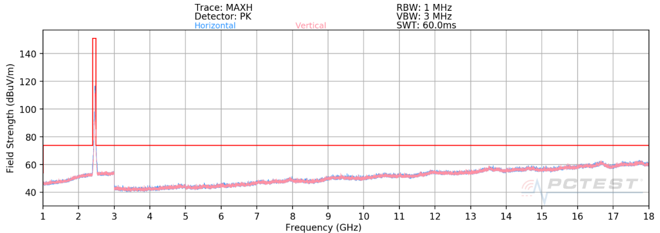
Plot 7-154. Radiated Spurious Emissions above 1GHz Antenna 7 (802.11ax OFDMA – RU242 – Ch. 11)
