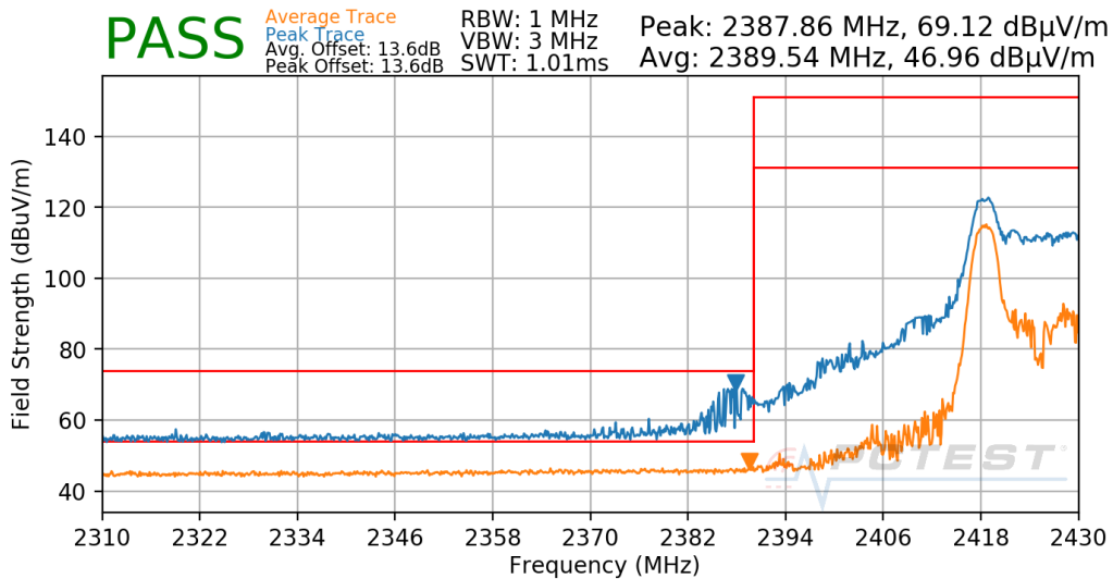
Plot 7-166. Radiated Restricted Lower Band Edge Measurement Antenna 8 (Peak & Average – RU26)
