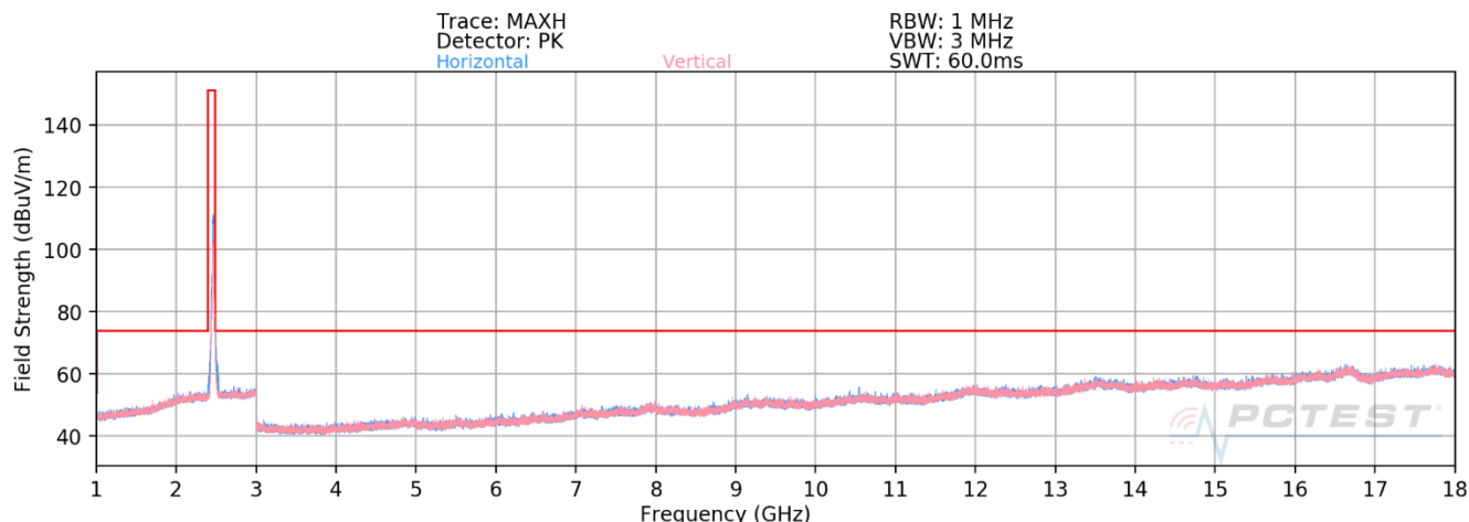
Plot 7-148. Radiated Spurious Emissions above 1GHz Antenna 8 (802.11ax OFDMA – RU242 – Ch. 11)
