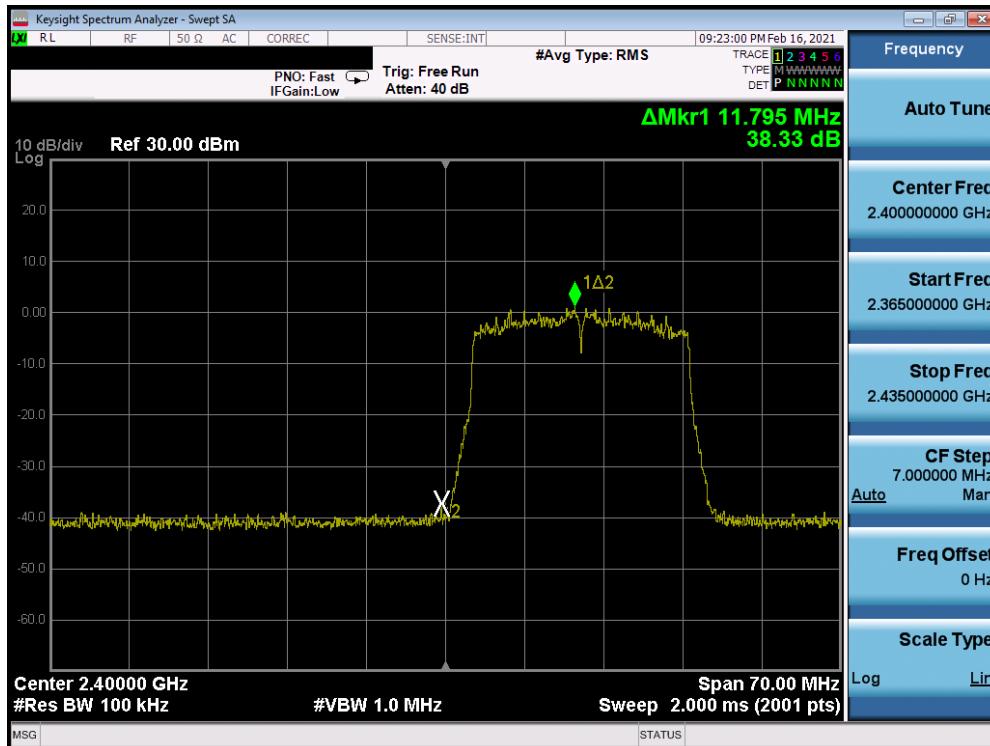
Plot 7-107. Band Edge Antenna 7 (802.11ax OFDMA – RU242 – Ch. 1)
