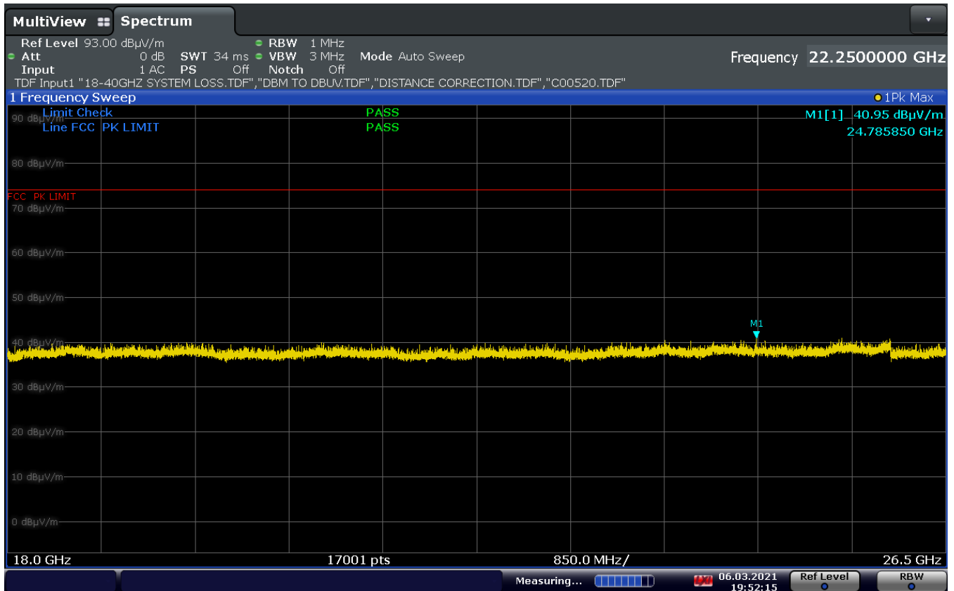
Plot 7-158. Radiated Spurious Emissions above 18GHz CDD (802.11ax, Ch.6 – RU26, Pol V)
