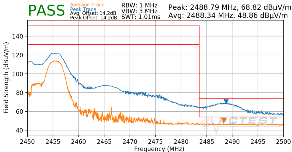
Plot 7-169. Radiated Restricted Upper Band Edge Measurement Antenna 8 (Peak & Average – RU26)
