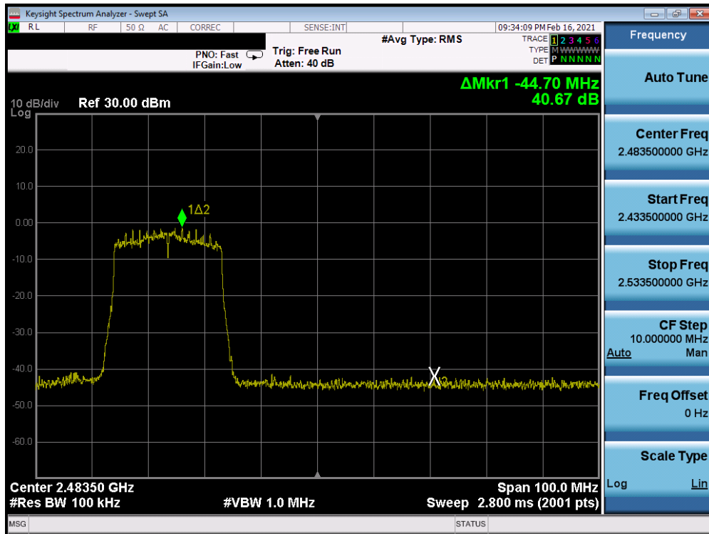
Plot 7-116. Band Edge Antenna 7 (802.11ax OFDMA – RU242 – Ch. 10)
