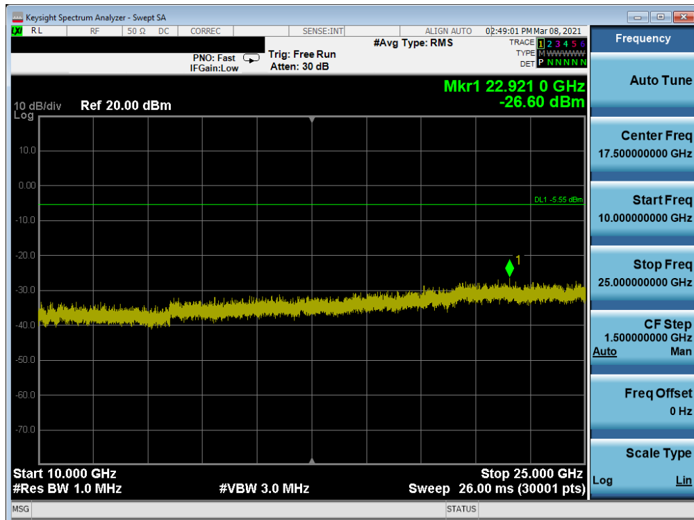
Plot 7-140. Conducted Spurious Plot Antenna 7 (802.11ax OFDMA – RU242 – Ch. 6)
