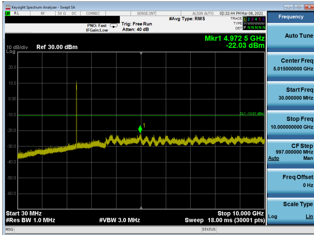
Plot 7-125. Conducted Spurious Plot Antenna 8 (802.11ax OFDMA – RU242 – Ch. 1)
