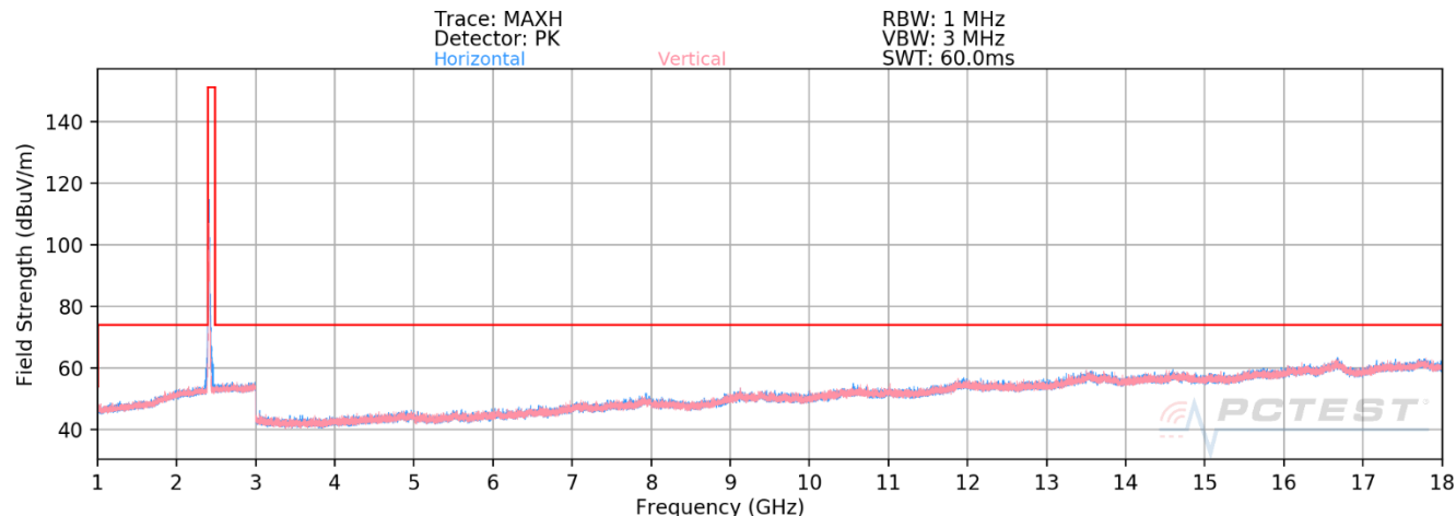
Plot 7-143. Radiated Spurious Emissions above 1GHz Antenna 8 (802.11ax OFDMA – RU26 – Ch. 1)
