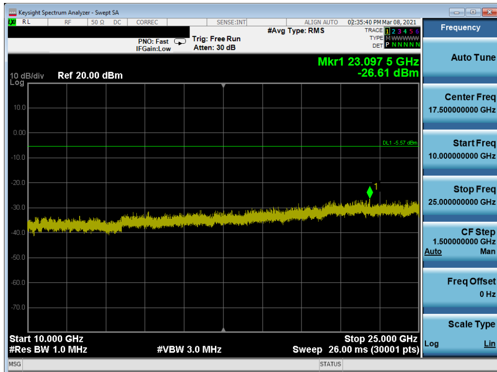
Plot 7-128. Conducted Spurious Plot Antenna 8 (802.11ax OFDMA – RU242 – Ch. 6)
