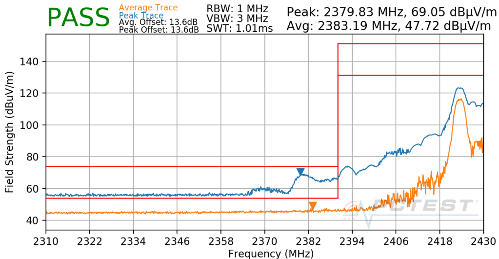
Plot 7-167. Radiated Restricted Lower Band Edge Measurement Antenna 8 (Peak & Average – RU26)
