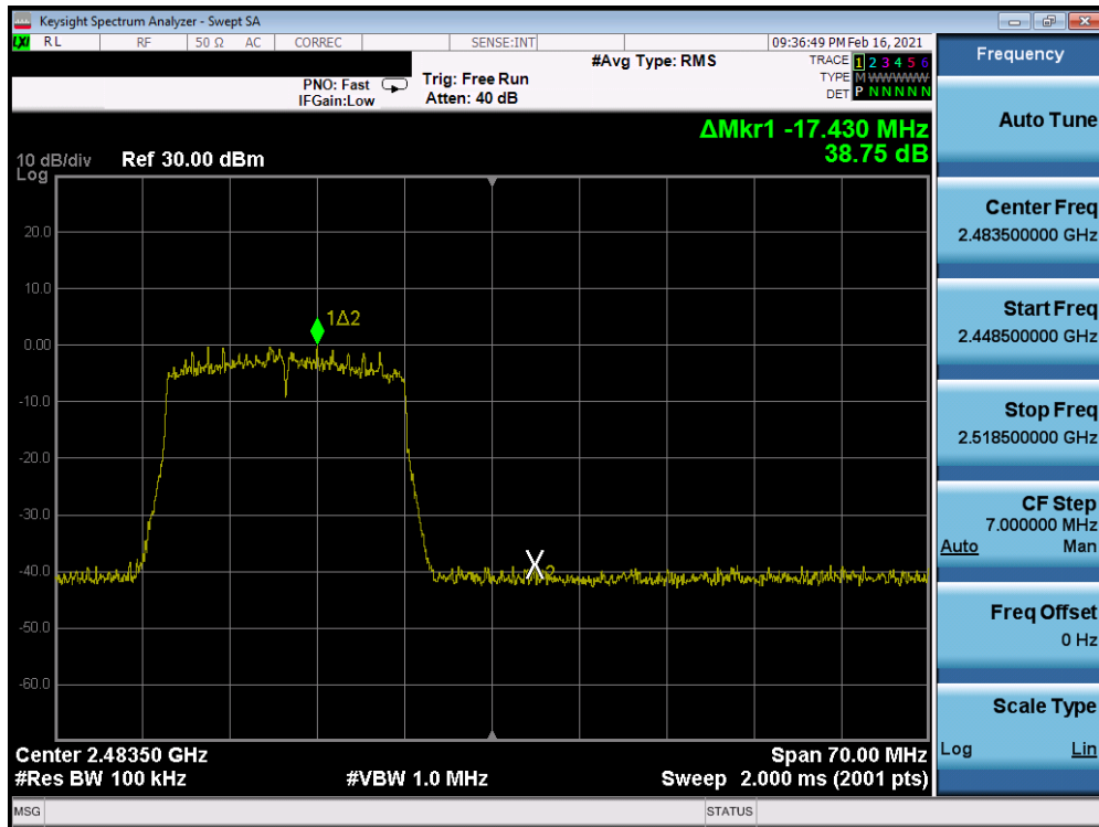
Plot 7-118. Band Edge Antenna 7 (802.11ax OFDMA – RU242 – Ch. 12)
