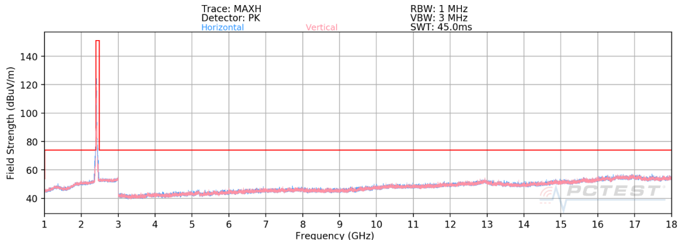
Plot 7-155. Radiated Spurious Emissions above 1GHz CDD (802.11ax OFDMA – RU26 – Ch. 1)
