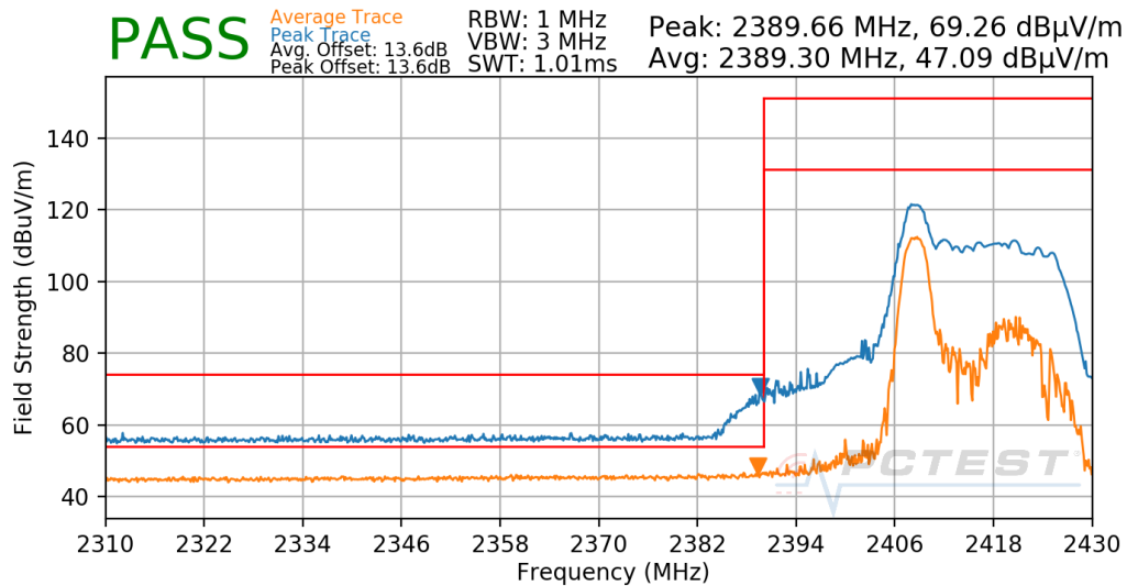
Plot 7-164. Radiated Restricted Lower Band Edge Measurement Antenna 8 (Peak & Average – RU26)
