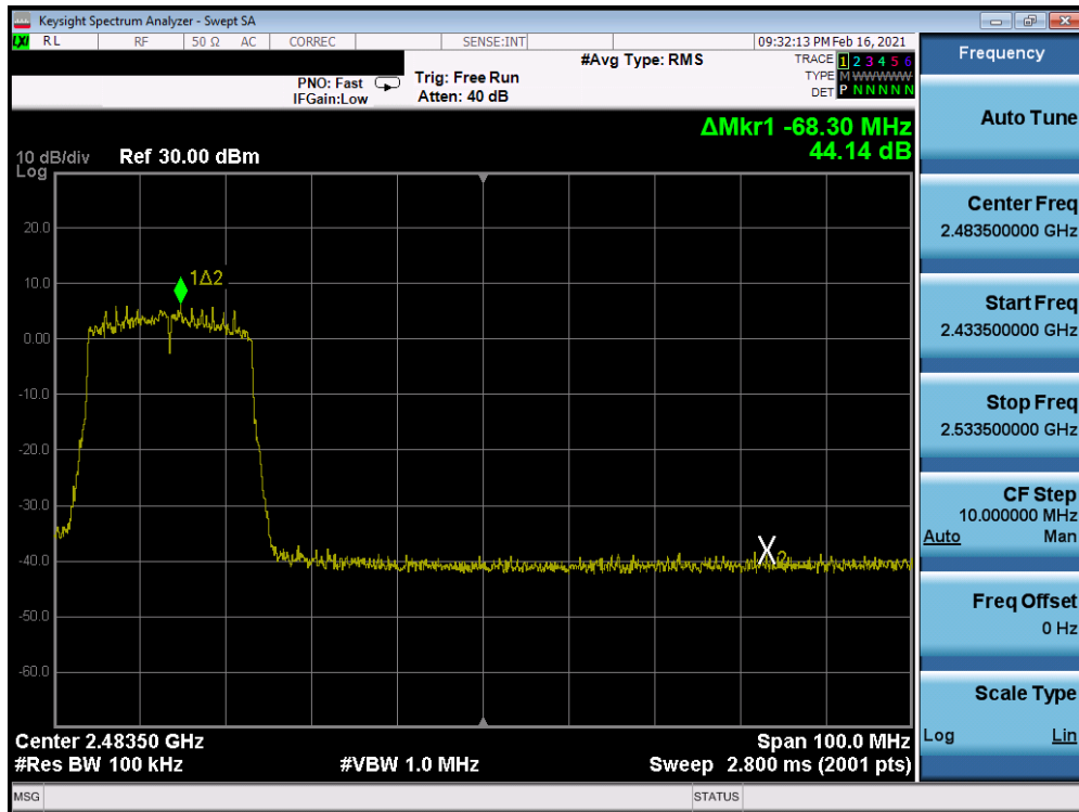
Plot 7-114. Band Edge Antenna 7 (802.11ax OFDMA – RU242 – Ch. 8)
