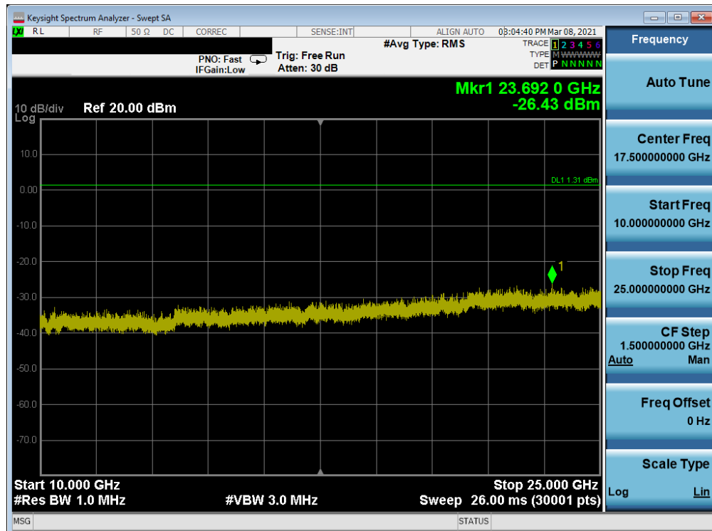
Plot 7-134. Conducted Spurious Plot Antenna 7 (802.11ax OFDMA – RU26 – Ch. 6)
