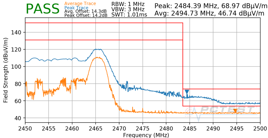
Plot 7-171. Radiated Restricted Upper Band Edge Measurement Antenna 8 (Peak & Average – RU26)
