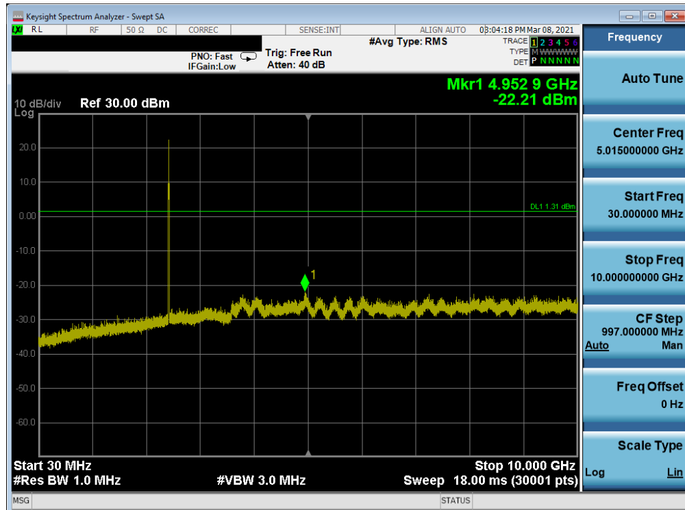
Plot 7-133. Conducted Spurious Plot Antenna 7 (802.11ax OFDMA – RU26 – Ch. 6)
