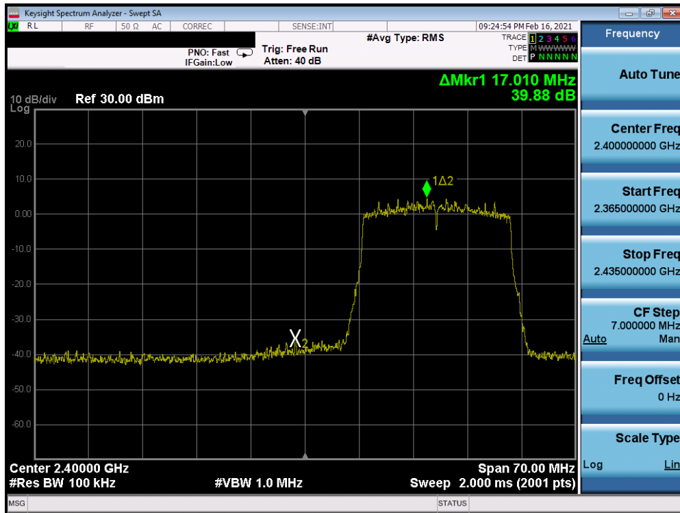
Plot 7-108. Band Edge Antenna 7 (802.11ax OFDMA - RU242 - Ch. 2)
