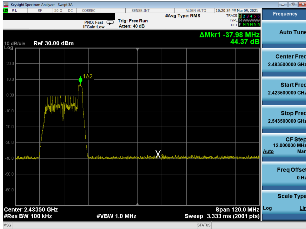
Plot 7-102. Band Edge Antenna 7 (802.11ax OFDMA – RU26 Index 8 – Ch. 8)
