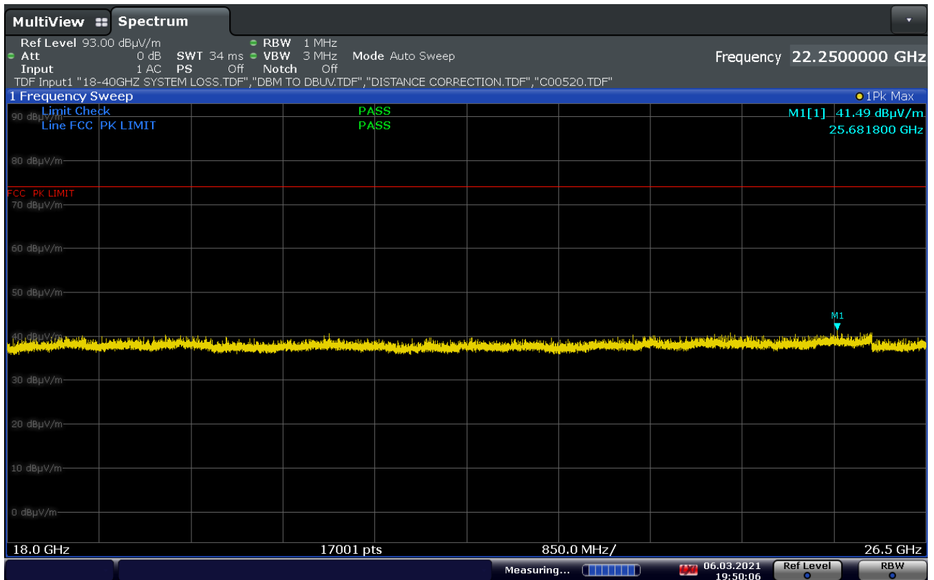
Plot 7-157. Radiated Spurious Emissions above 18GHz CDD (802.11ax, Ch.6 – RU26, Pol H)
