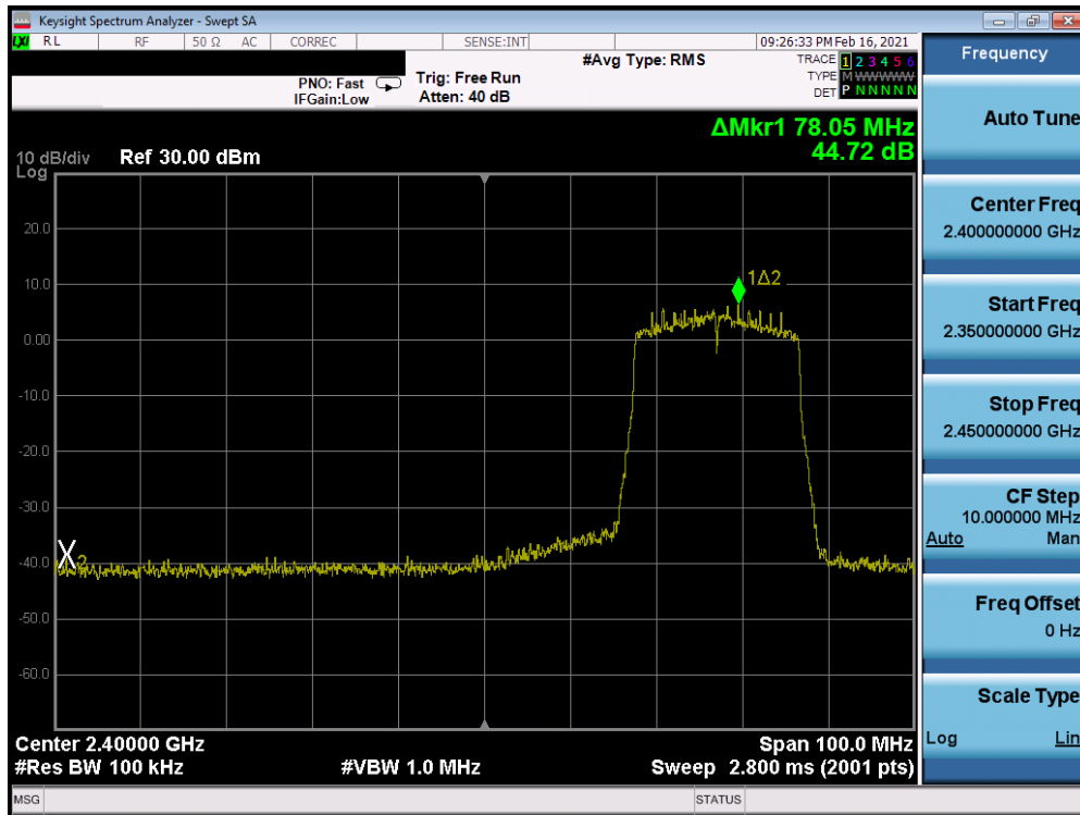
Plot 7-110. Band Edge Antenna 7 (802.11ax OFDMA – RU242 – Ch. 4)
