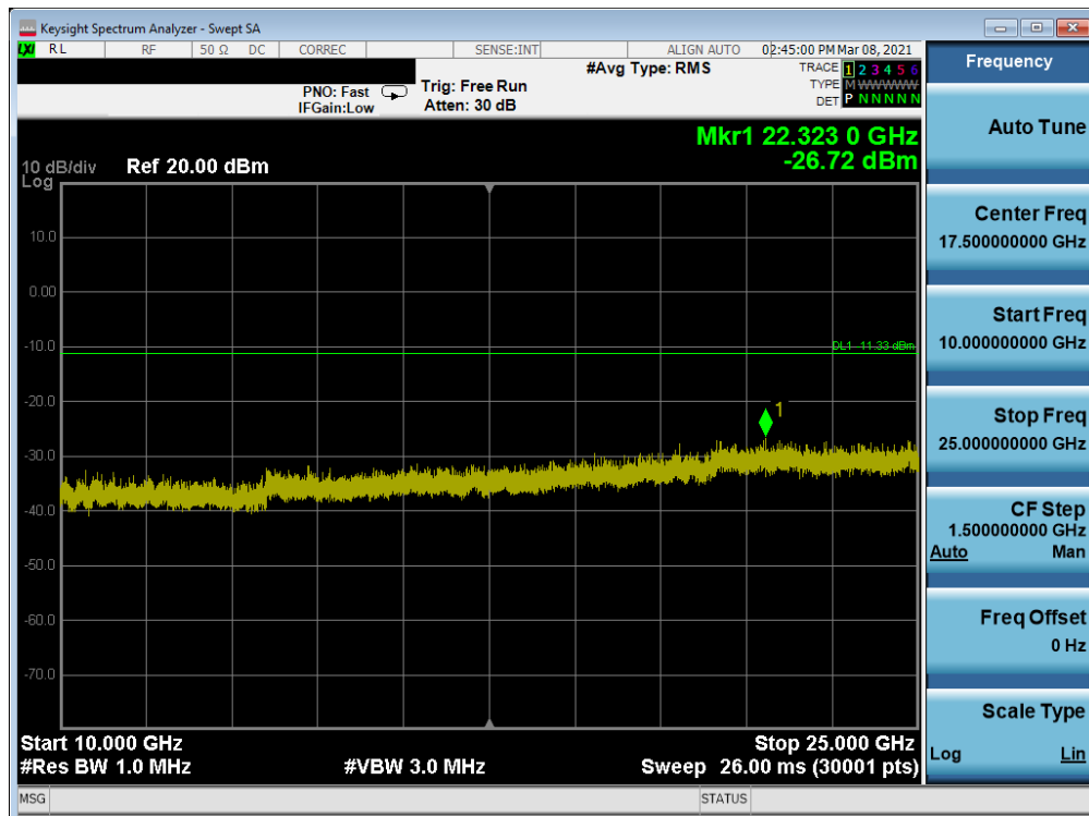
Plot 7-142. Conducted Spurious Plot Antenna 7 (802.11ax OFDMA – RU242 – Ch. 11)
