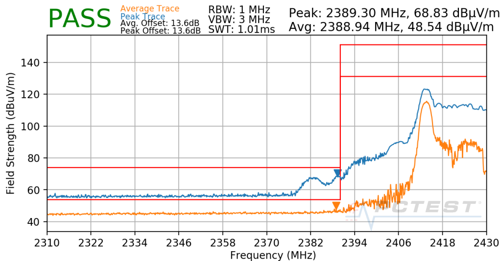
Plot 7-165. Radiated Restricted Lower Band Edge Measurement Antenna 8 (Peak & Average – RU26)
