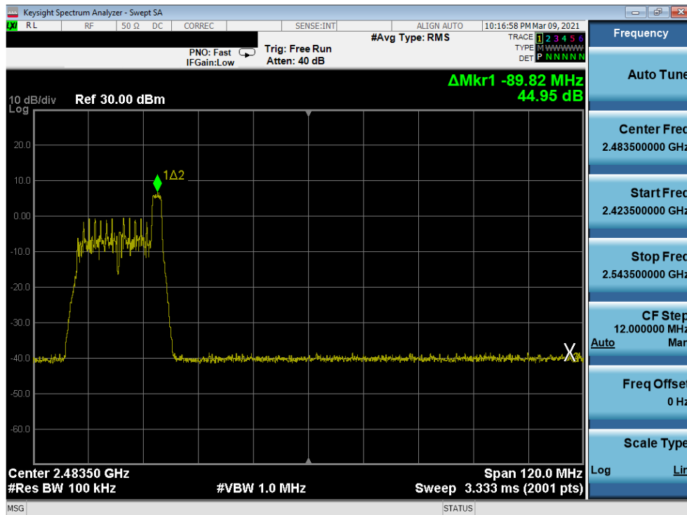
Plot 7-101. Band Edge Antenna 7 (802.11ax OFDMA – RU26 Index 8 – Ch. 7)
