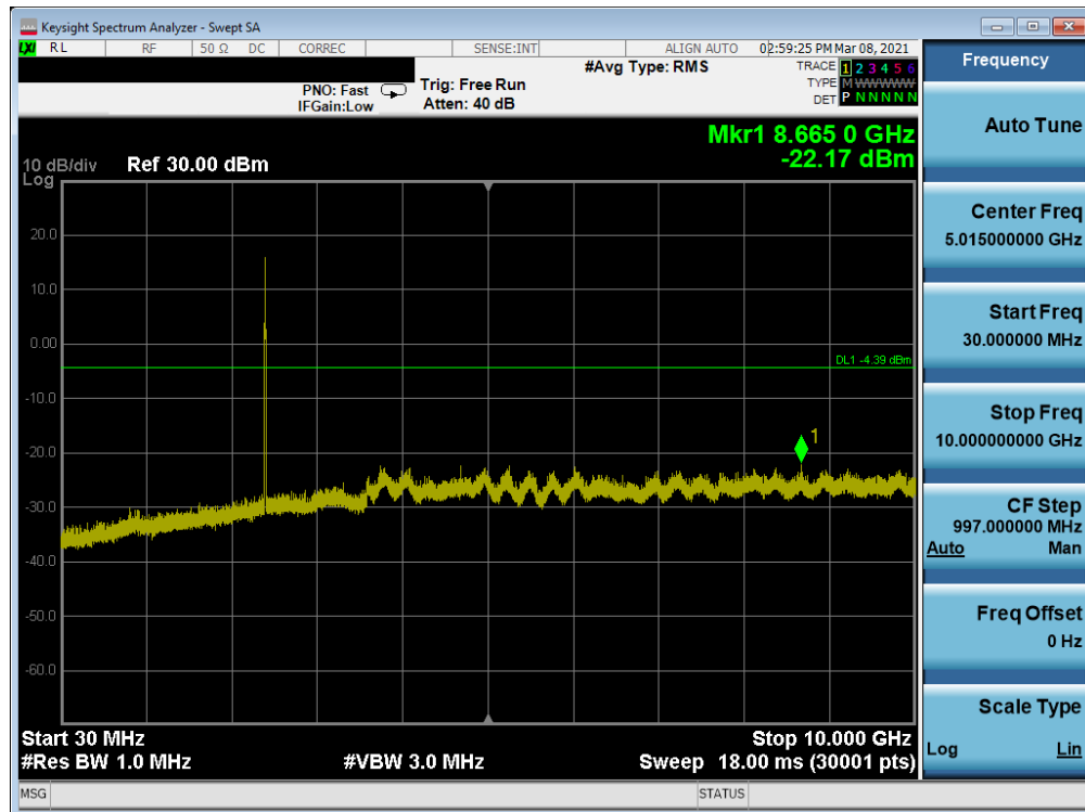
Plot 7-131. Conducted Spurious Plot Antenna 7 (802.11ax OFDMA – RU26 – Ch. 1)
