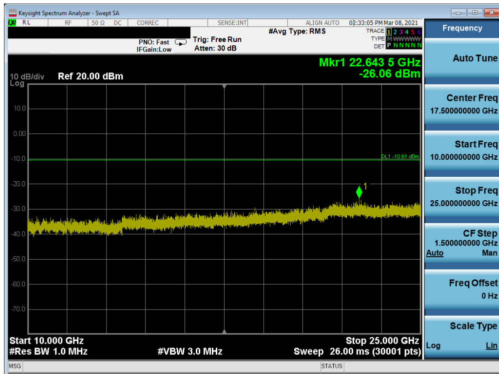
Plot 7-126. Conducted Spurious Plot Antenna 8 (802.11ax OFDMA – RU242 – Ch. 1)
