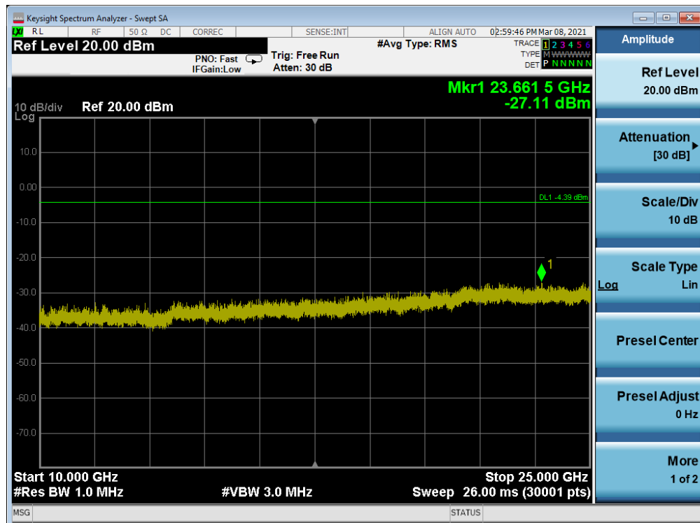
Plot 7-132. Conducted Spurious Plot Antenna 7 (802.11ax OFDMA – RU26 – Ch. 1)
