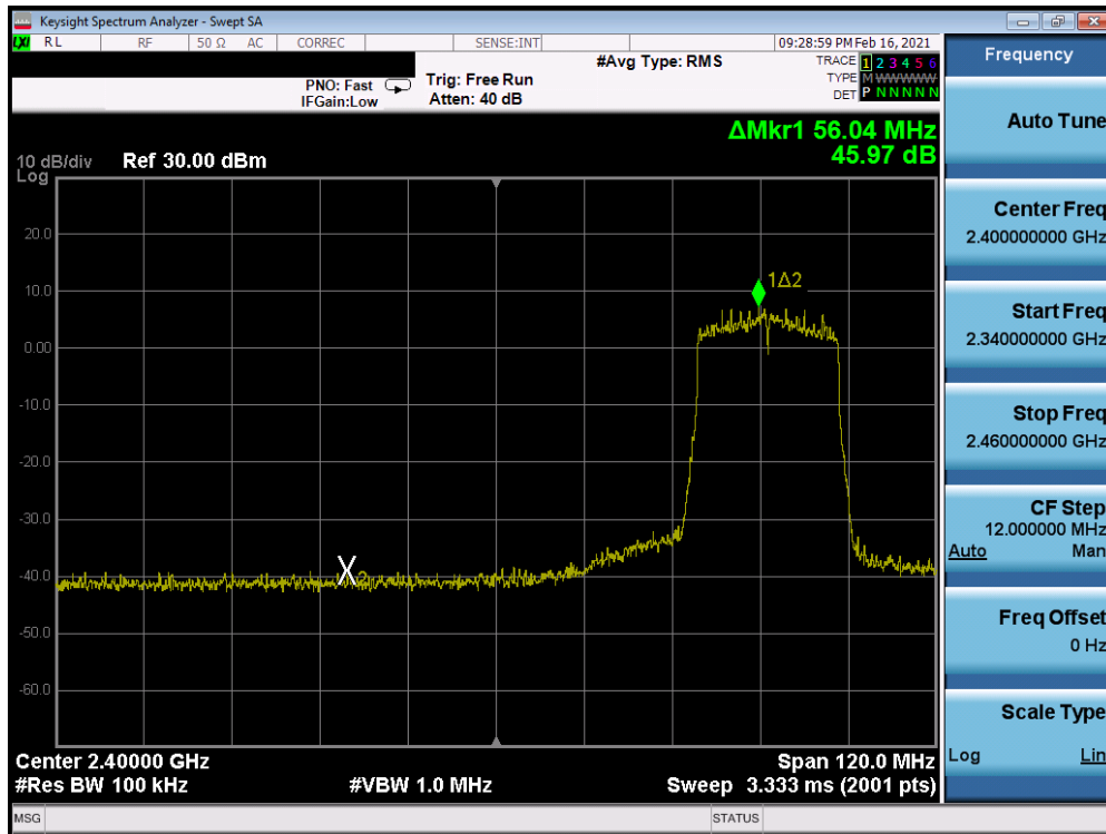
Plot 7-112. Band Edge Antenna 7 (802.11ax OFDMA – RU242 – Ch. 6)
