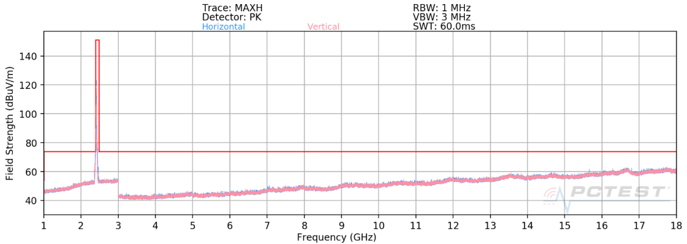
Plot 7-149. Radiated Spurious Emissions above 1GHz Antenna 7 (802.11ax OFDMA – RU26 – Ch. 1)
