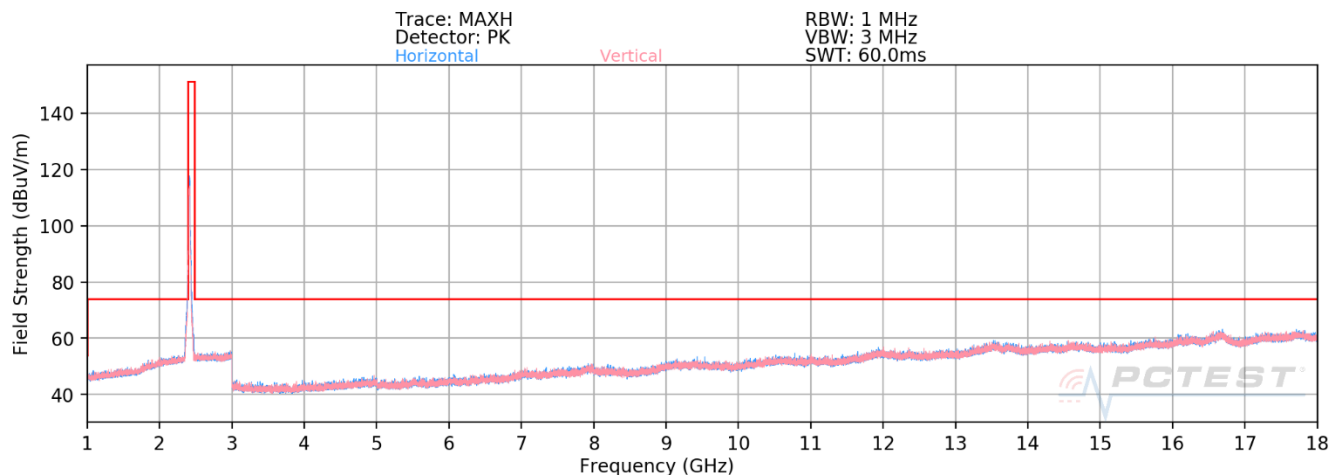
Plot 7-152. Radiated Spurious Emissions above 1GHz Antenna 7 (802.11ax OFDMA – RU242 – Ch. 1)
