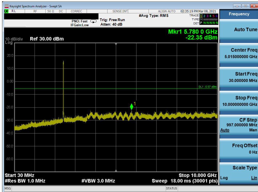
Plot 7-127. Conducted Spurious Plot Antenna 8 (802.11ax OFDMA – RU242 – Ch. 6)
