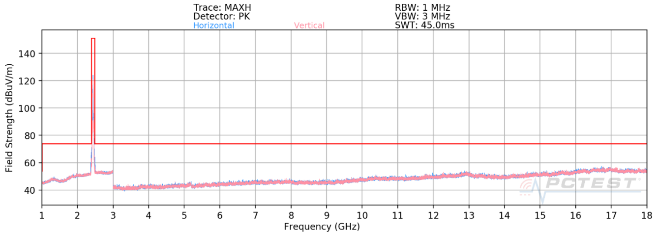
Plot 7-156. Radiated Spurious Emissions above 1GHz CDD (802.11ax OFDMA – RU26 – Ch. 6)
