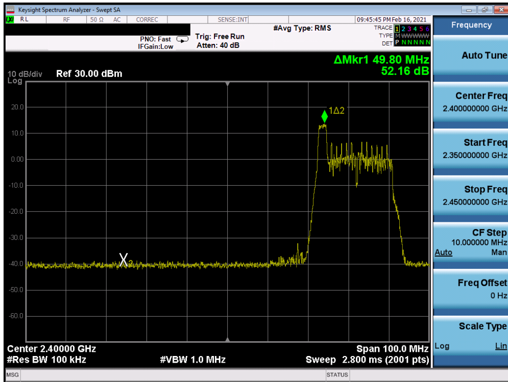
Plot 7-100. Band Edge Antenna 7 (802.11ax OFDMA – RU26 Index 0 – Ch. 5)
