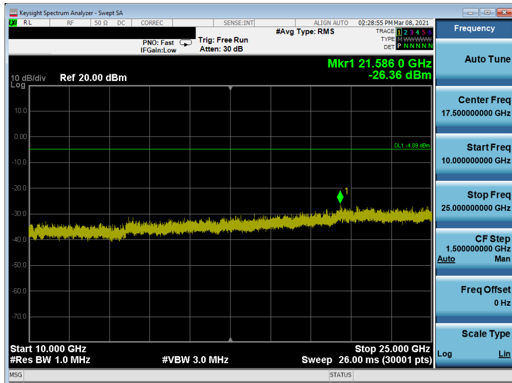
Plot 7-120. Conducted Spurious Plot Antenna 8 (802.11ax OFDMA – RU26 – Ch. 1)
