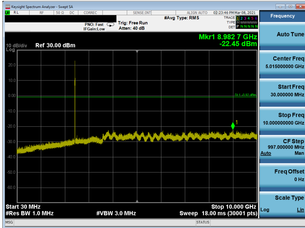
Plot 7-121. Conducted Spurious Plot Antenna 8 (802.11ax OFDMA – RU26 – Ch. 6)
