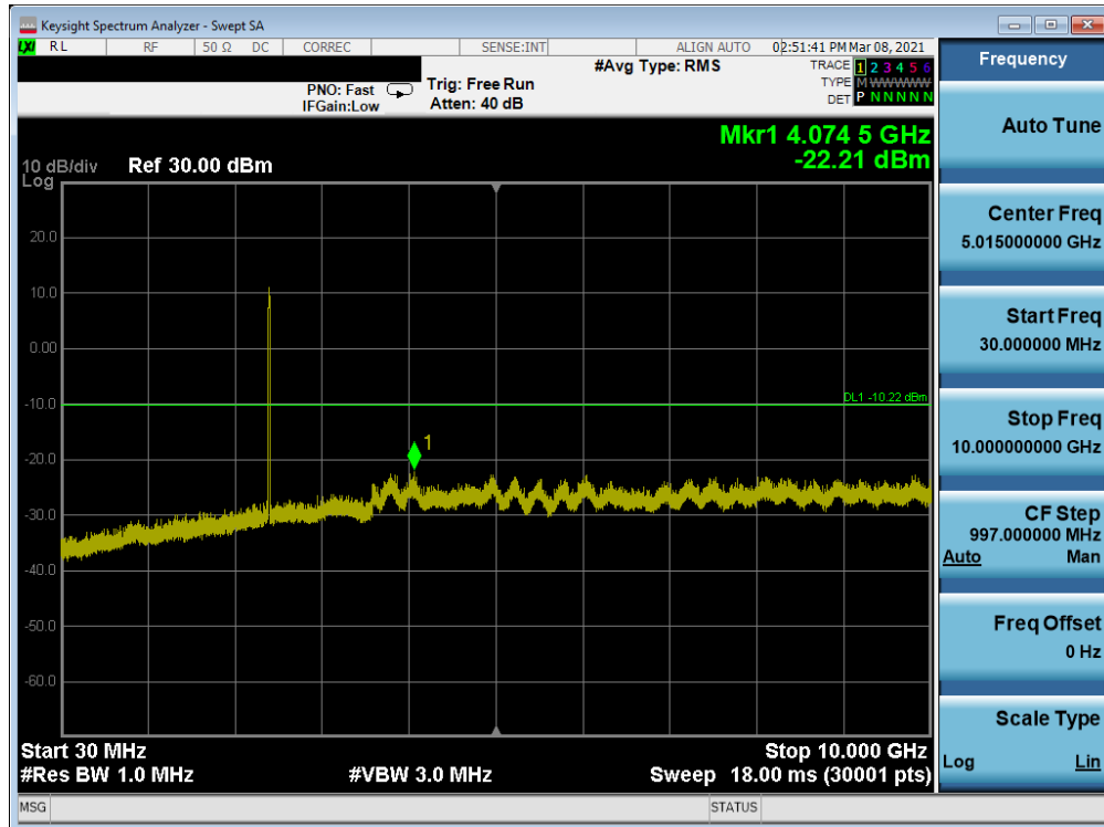
Plot 7-137. Conducted Spurious Plot Antenna 7 (802.11ax OFDMA – RU242 – Ch. 1)
