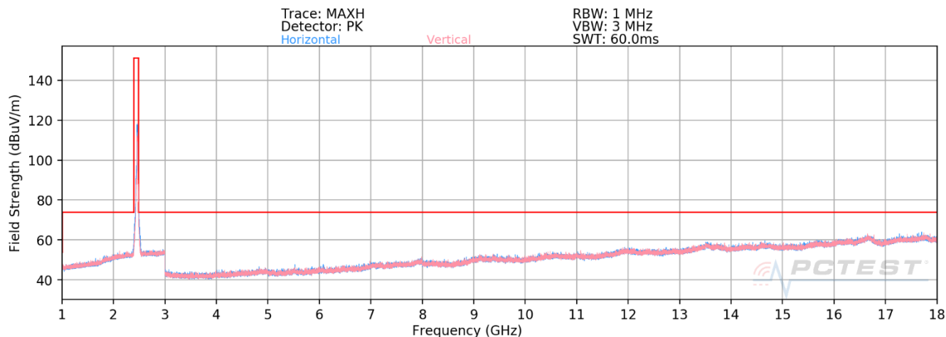
Plot 7-162. Radiated Spurious Emissions above 1GHz CDD (802.11ax OFDMA – RU242 – Ch. 11)
