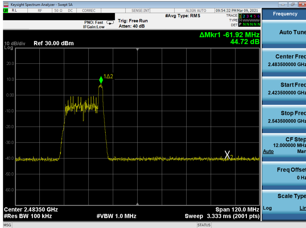
Plot 7-81. Band Edge Antenna 8 (802.11ax OFDMA – RU26 Index 8 – Ch. 10)
