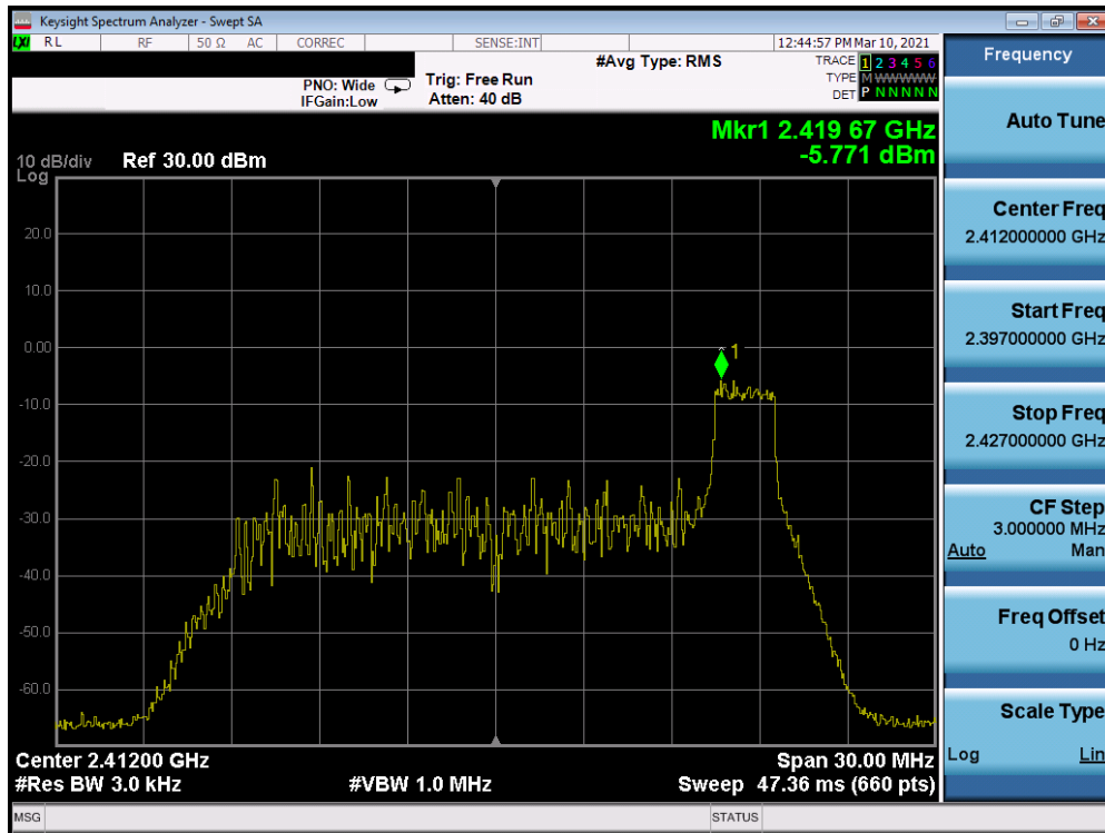
Plot 7-27. Power Spectral Density Plot Antenna 8 (802.11ax OFDMA – RU26 Index 8 – Ch. 1)
