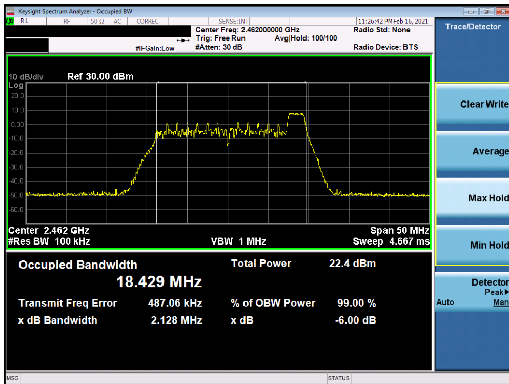
Plot 7-21. 6dB BW & 99% OBW Plot Antenna 7 (802.11ax OFDMA – RU26 Index 8 – Ch. 11)
