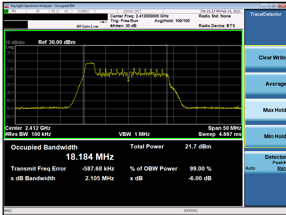
Plot 7-1. 6dB BW & 99% OBW Plot Antenna 8 (802.11ax OFDMA – RU26 Index 0 – Ch. 1)
