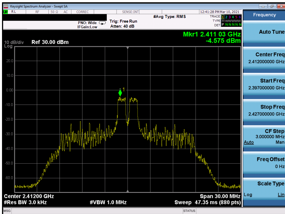
Plot 7-26. Power Spectral Density Plot Antenna 8 (802.11ax OFDMA – RU26 Index 4 – Ch. 1)
