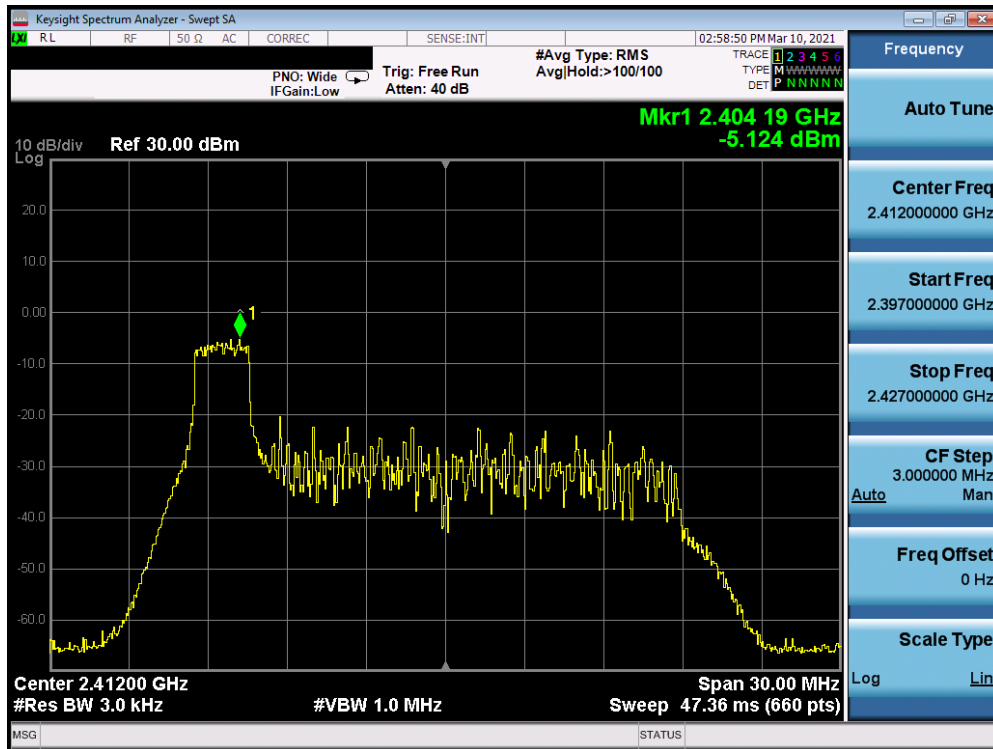
Plot 7-37. Power Spectral Density Plot Antenna 7 (802.11ax OFDMA – RU26 Index 0 – Ch. 1)
