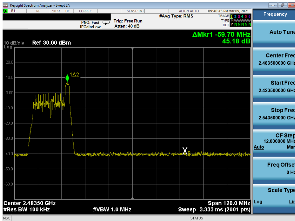
Plot 7-78. Band Edge Antenna 8 (802.11ax OFDMA – RU26 Index 8 – Ch. 7)
