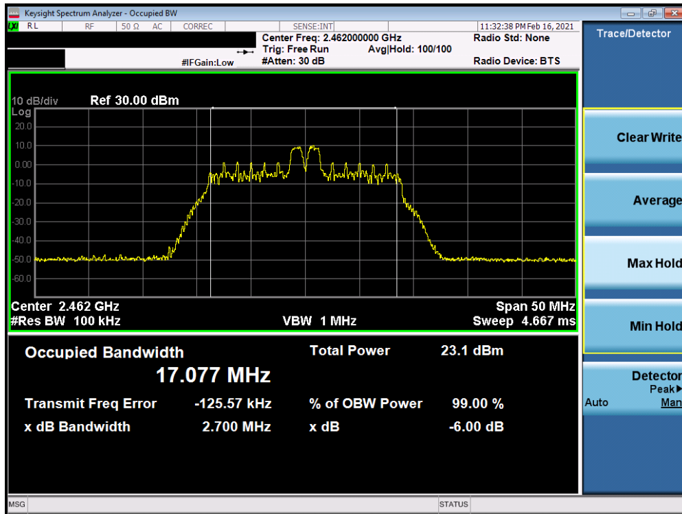
Plot 7-20. 6dB BW & 99% OBW Plot Antenna 7 (802.11ax OFDMA – RU26 Index 4 – Ch. 11)
