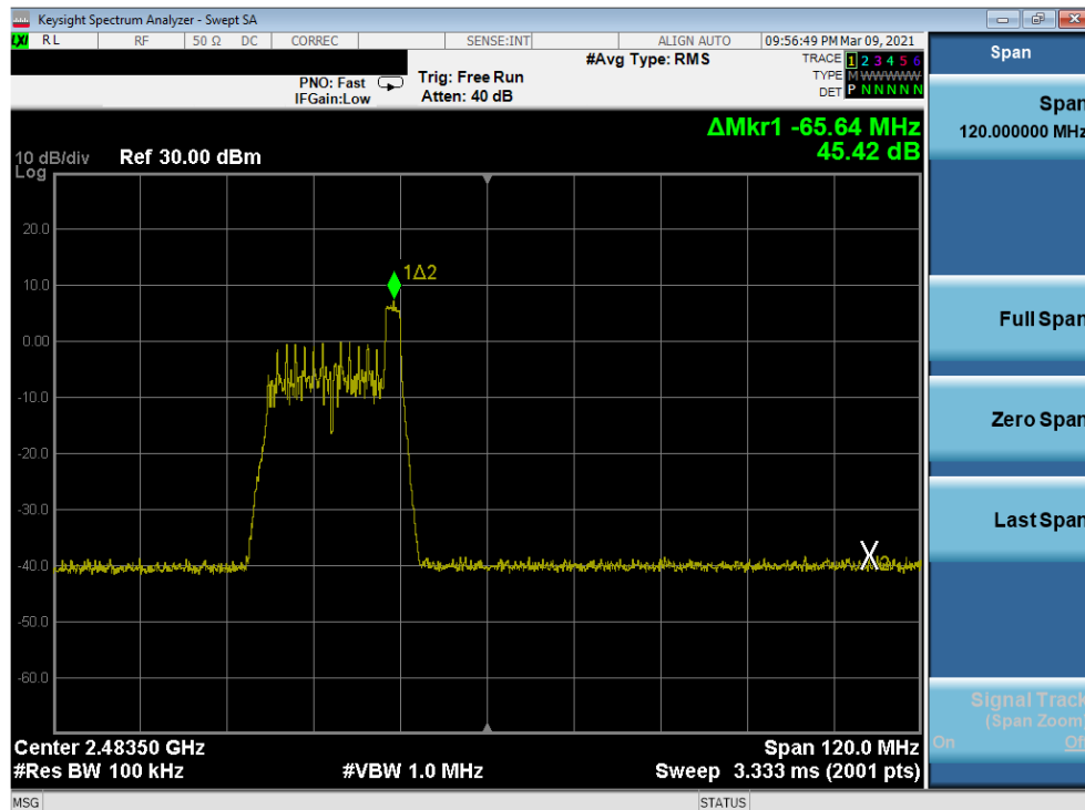
Plot 7-82. Band Edge Antenna 8 (802.11ax OFDMA – RU26 Index 8 – Ch. 11)
