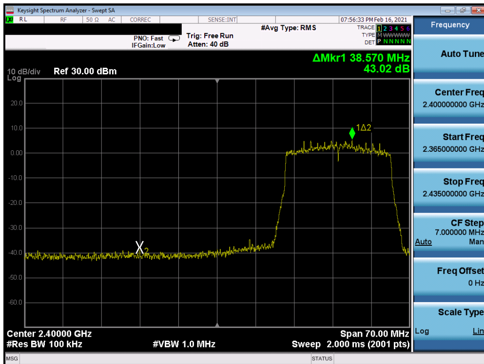
Plot 7-86. Band Edge Antenna 8 (802.11ax OFDMA – RU242 – Ch. 3)
