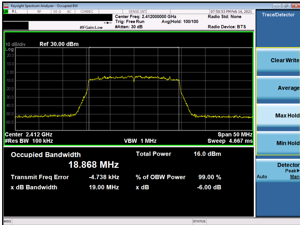
Plot 7-10. 6dB BW & 99% OBW Plot Antenna 8 (802.11ax OFDMA – RU242 – Ch. 1)
