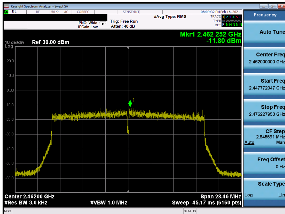
Plot 7-36. Power Spectral Density Plot Antenna 8 (802.11ax OFDMA – RU242 – Ch. 11)
