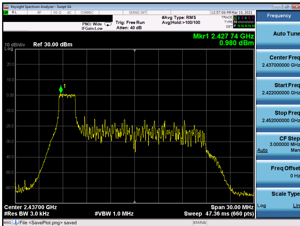
Plot 7-28. Power Spectral Density Plot Antenna 8 (802.11ax OFDMA – RU26 Index 0 – Ch. 6)
