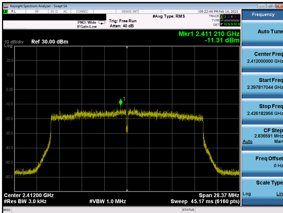
Plot 7-46. Power Spectral Density Plot Antenna 7 (802.11ax OFDMA – RU242 – Ch. 1)
