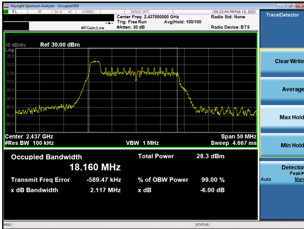
Plot 7-4. 6dB BW & 99% OBW Plot Antenna 8 (802.11ax OFDMA – RU26 Index 0 – Ch. 6)
