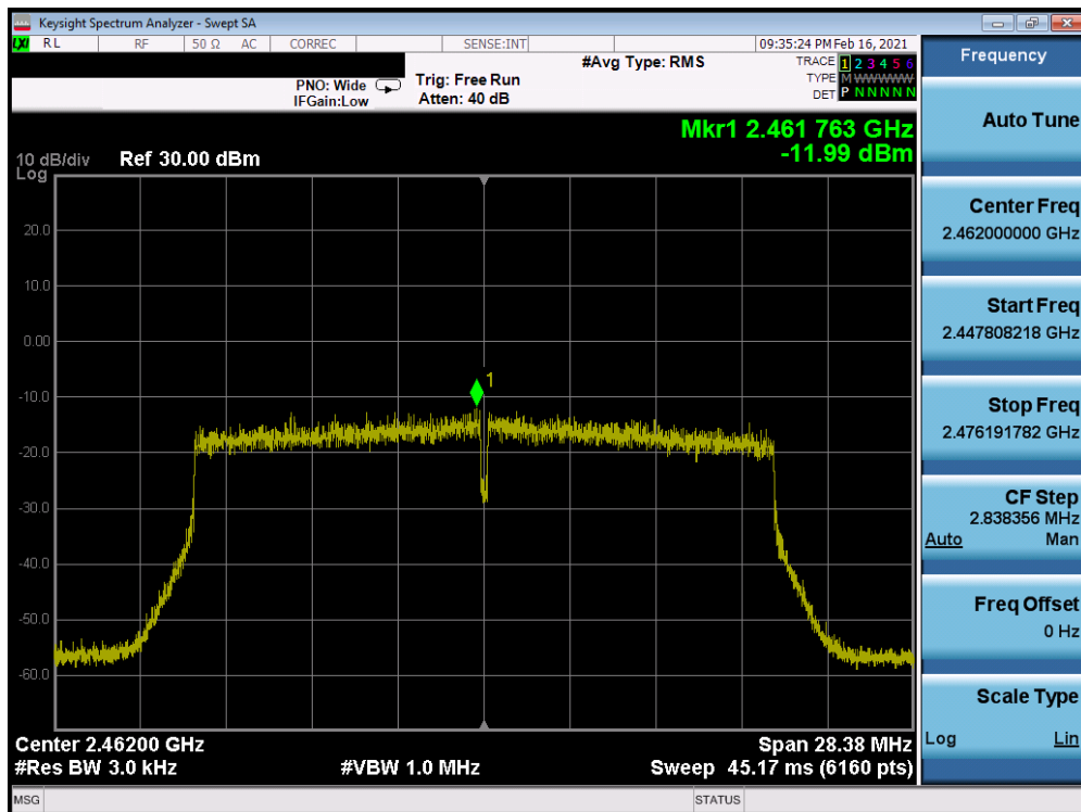
Plot 7-48. Power Spectral Density Plot Antenna 7 (802.11ax OFDMA – RU242 – Ch. 11)
