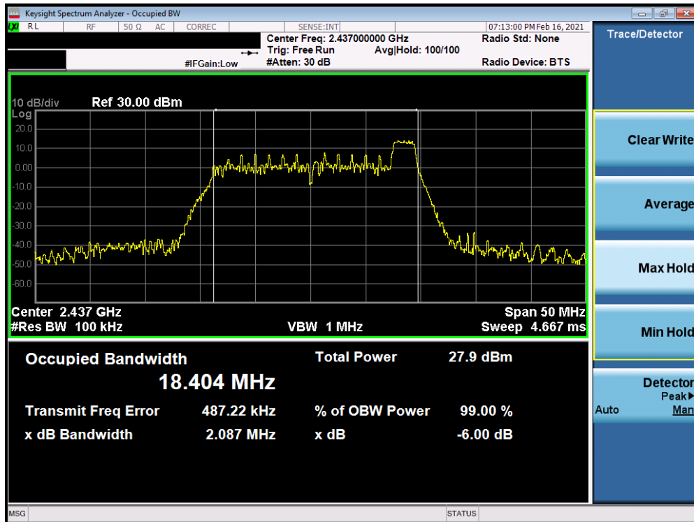
Plot 7-6. 6dB BW & 99% OBW Antenna 8 (802.11ax OFDMA – RU26 Index 8 – Ch. 6)
