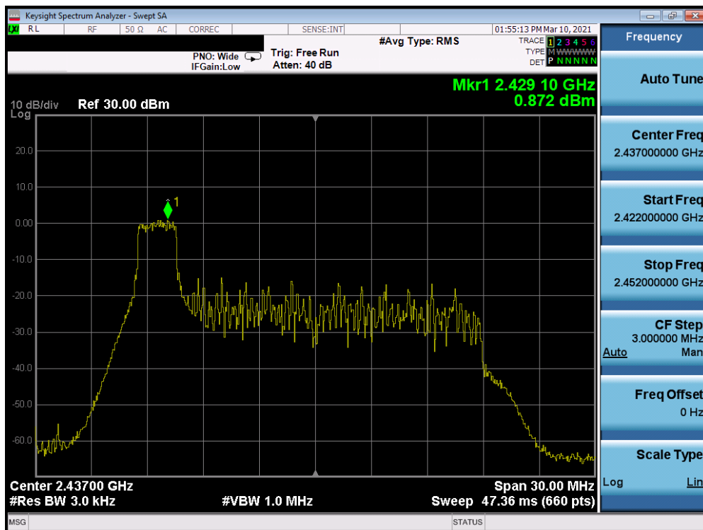
Plot 7-56. Power Spectral Density Plot CDD Antenna 7 (802.11ax OFDMA – RU26 Index 0 – Ch. 6)
