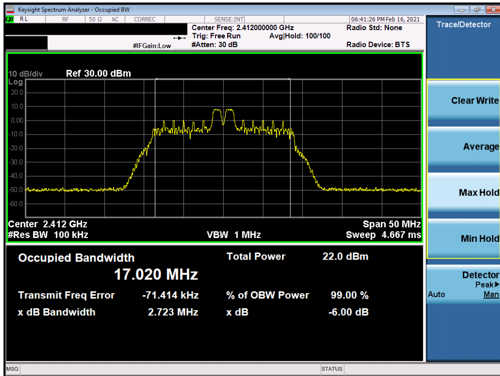
Plot 7-2. 6dB BW & 99% OBW Plot Antenna 8 (802.11ax OFDMA – RU26 Index 4 – Ch. 1)
