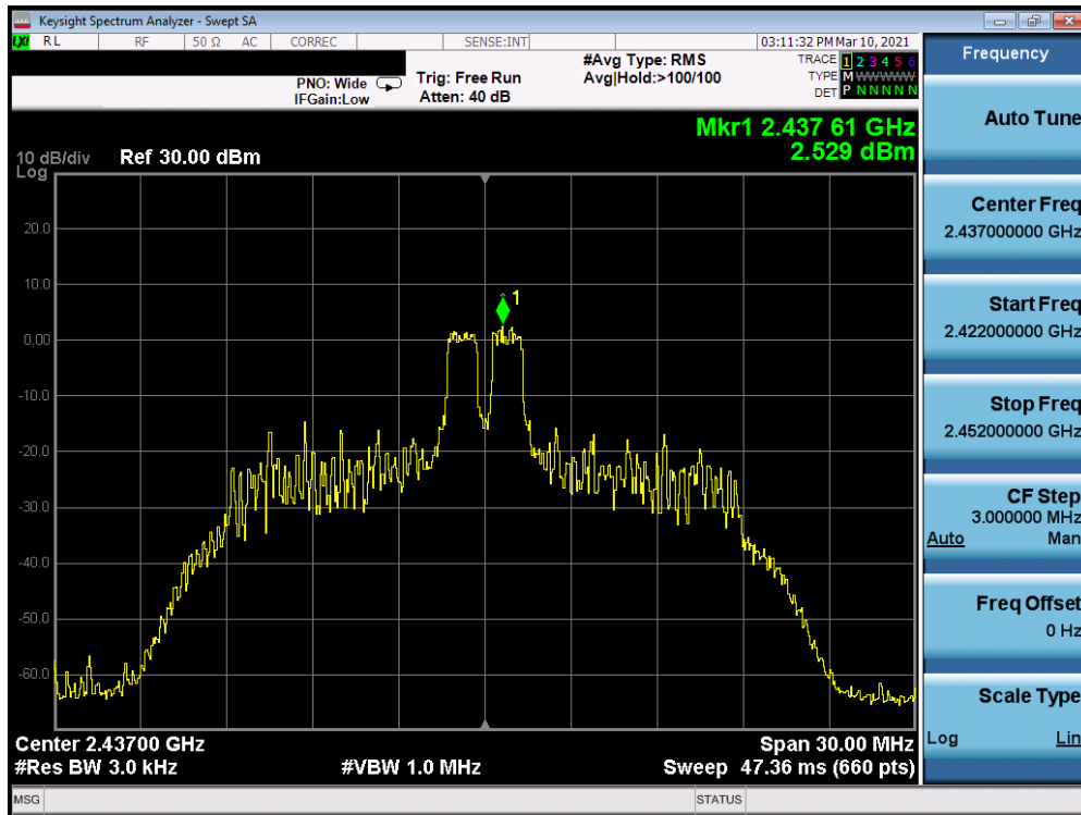
Plot 7-41. Power Spectral Density Plot Antenna 7 (802.11ax OFDMA – RU26 Index 4 – Ch. 6)
