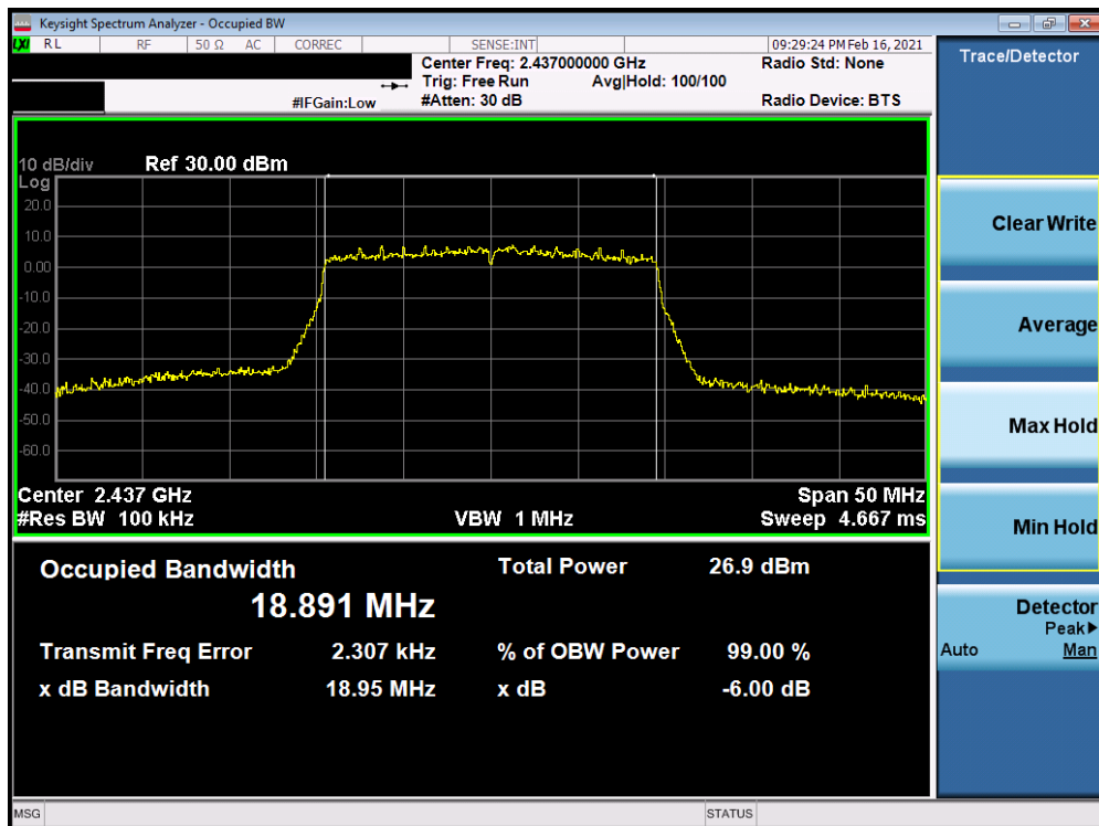
Plot 7-23. 6dB BW & 99% OBW Plot Antenna 7 (802.11ax OFDMA – RU242 – Ch. 6)
