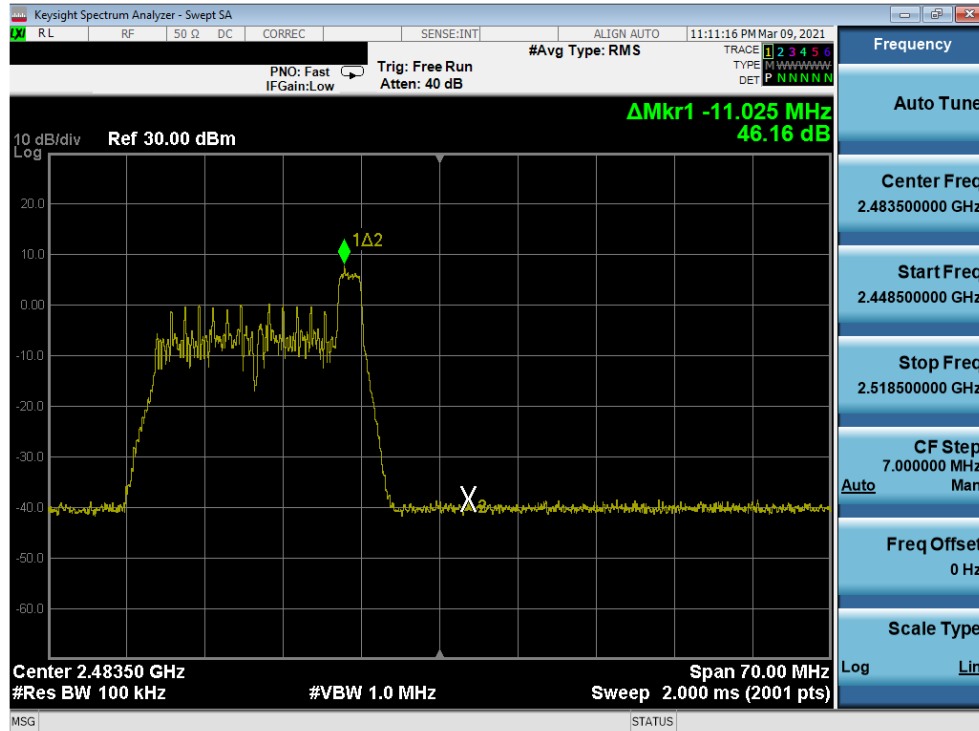
Plot 7-83. Band Edge Antenna 8 (802.11ax OFDMA – RU26 Index 8 – Ch. 12)
