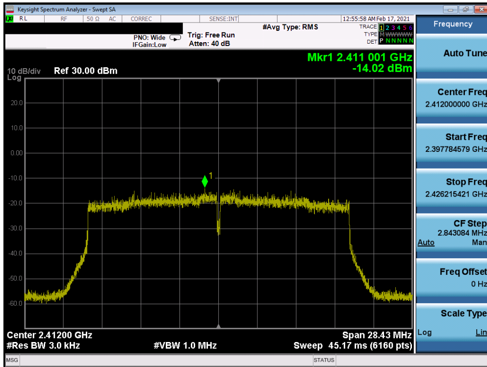
Plot 7-67. Power Spectral Density Plot CDD Antenna 8 (802.11ax OFDMA – RU242 – Ch. 1)
