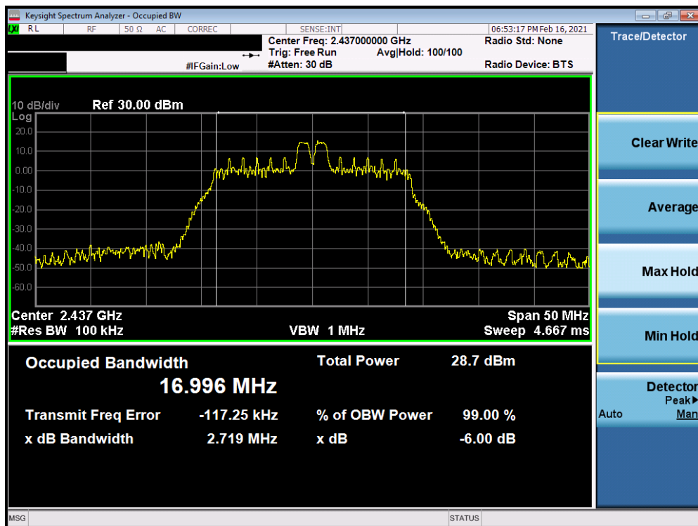
Plot 7-5. 6dB BW & 99% OBW Plot Antenna 8 (802.11ax OFDMA – RU26 Index 4 – Ch. 6)
