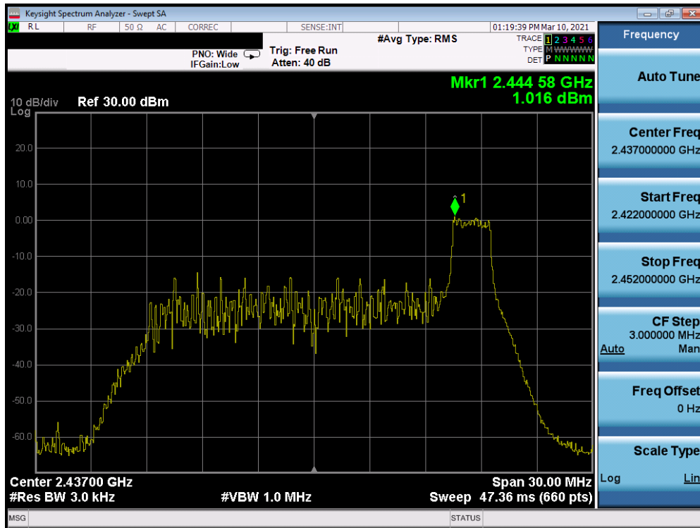
Plot 7-59. Power Spectral Density Plot CDD Antenna 8 (802.11ax OFDMA – RU26 Index 8 – Ch. 6)
