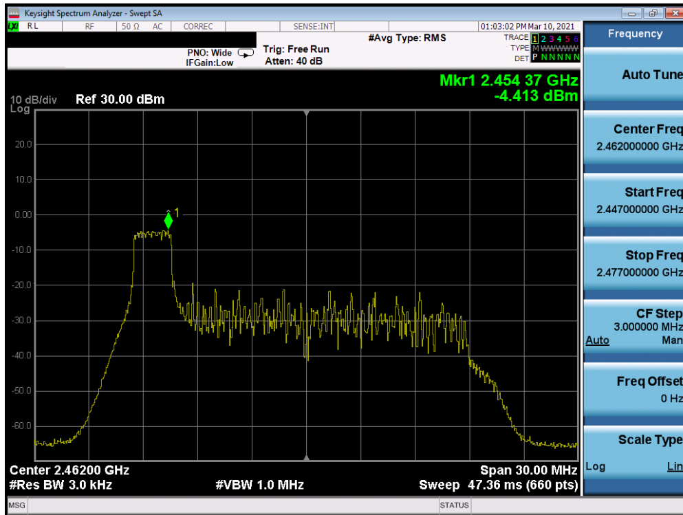
Plot 7-31. Power Spectral Density Plot Antenna 8 (802.11ax OFDMA – RU26 Index 0 – Ch. 11)
