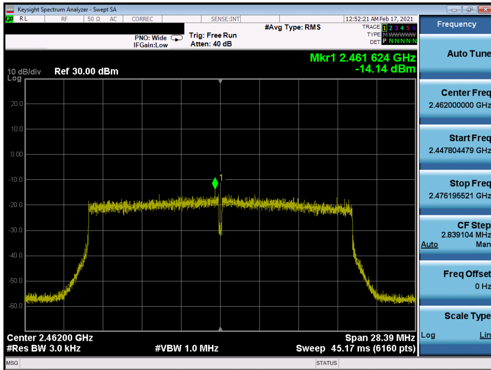
Plot 7-71. Power Spectral Density Plot CDD Antenna 8 (802.11ax OFDMA – RU242 – Ch. 11)
