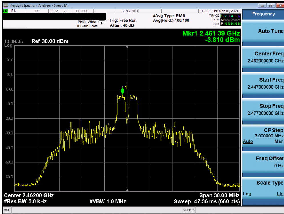
Plot 7-63. Power Spectral Density Plot CDD Antenna 8 (802.11ax OFDMA – RU26 Index 4 – Ch. 11)
