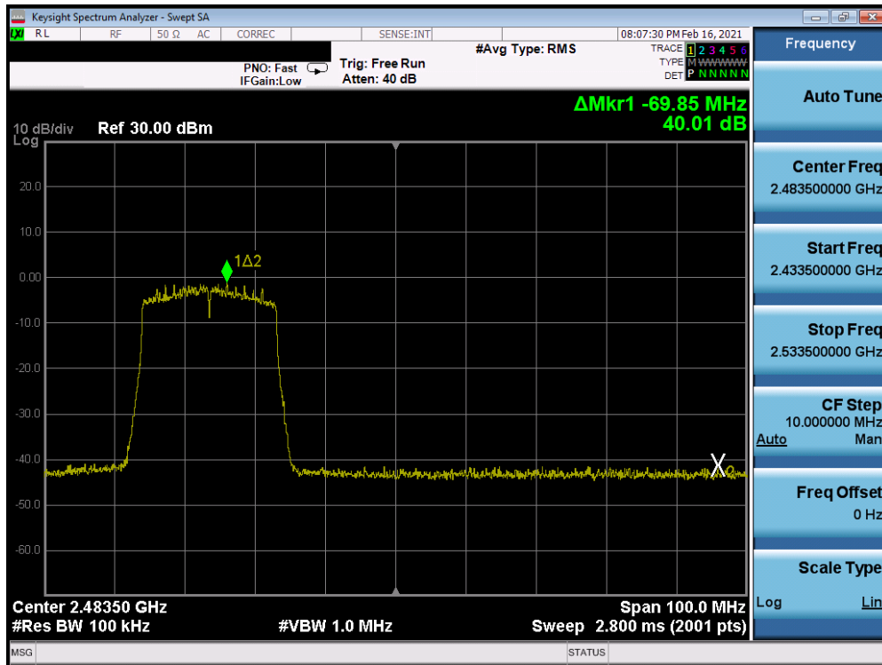
Plot 7-93. Band Edge Antenna 8 (802.11ax OFDMA – RU242 – Ch. 10)
