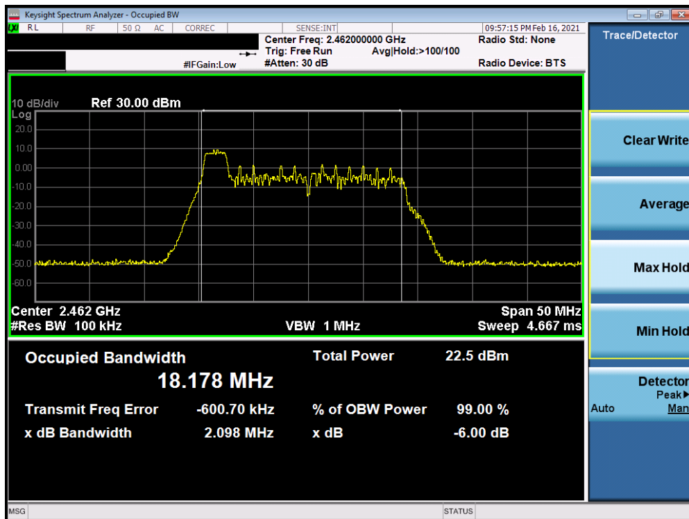
Plot 7-19. 6dB BW & 99% OBW Plot Antenna 7 (802.11ax OFDMA – RU26 Index 0 – Ch. 11)
