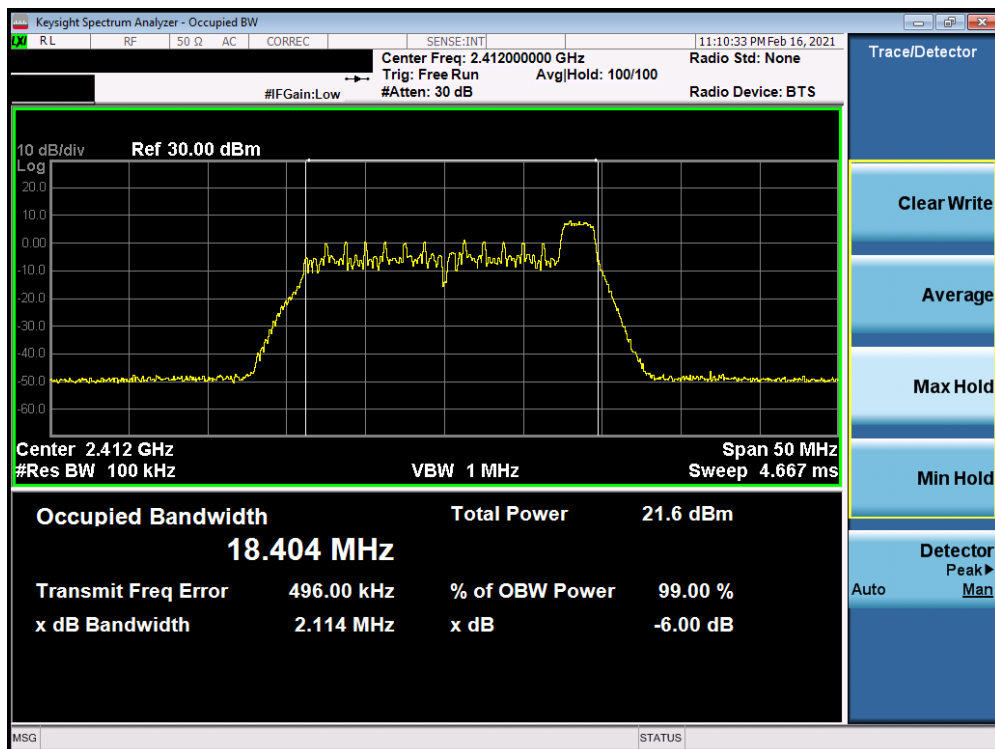
Plot 7-15. 6dB BW & 99% OBW Plot Antenna 7 (802.11ax OFDMA – RU26 Index 8 – Ch. 1)
