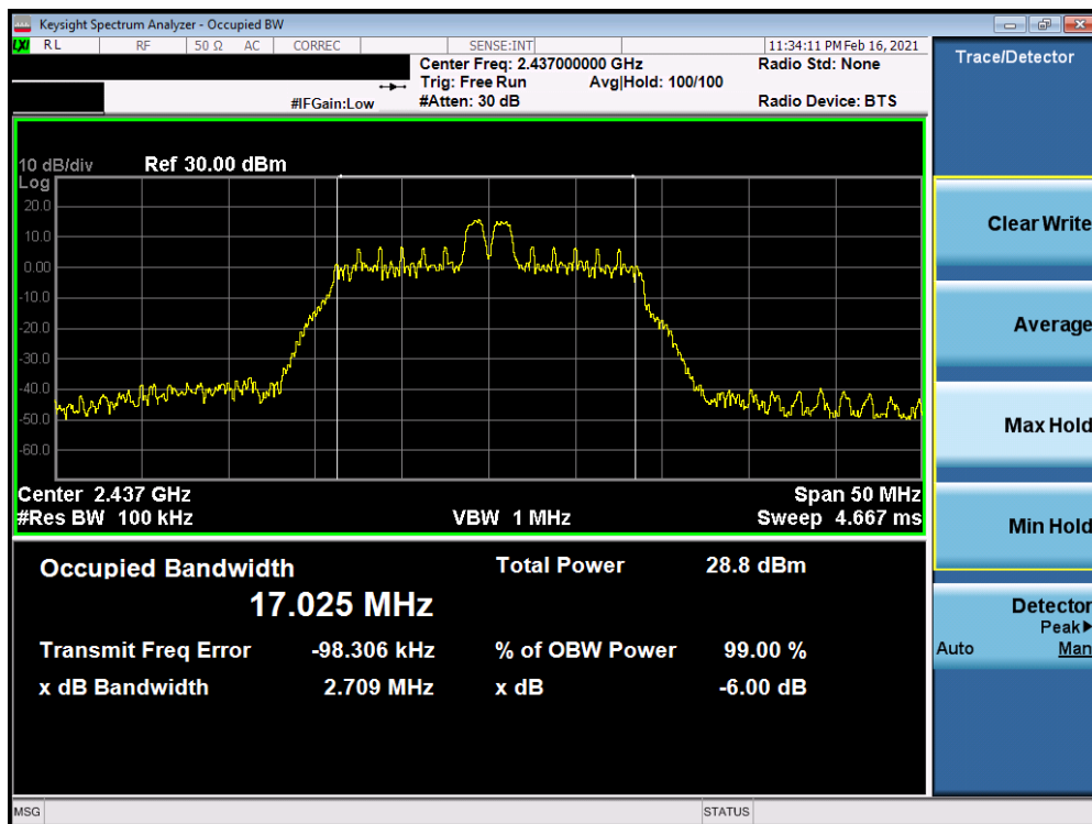
Plot 7-17. 6dB BW & 99% OBW Plot Antenna 7 (802.11ax OFDMA – RU26 Index 4 – Ch. 6)
