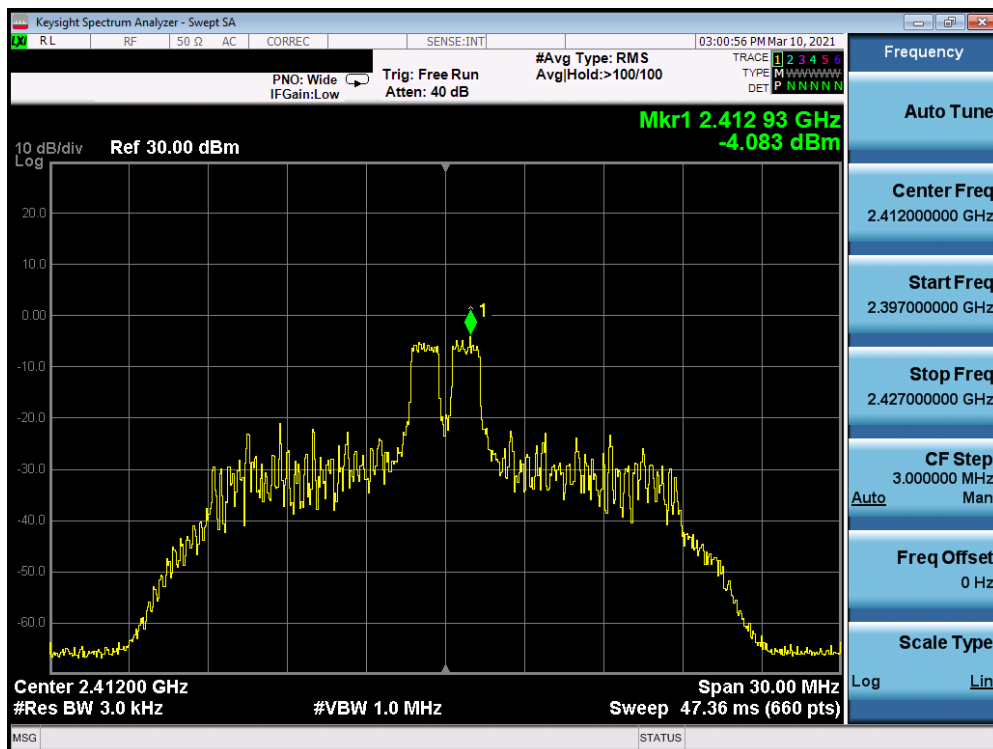
Plot 7-38. Power Spectral Density Plot Antenna 7 (802.11ax OFDMA – RU26 Index 4 – Ch. 1)
