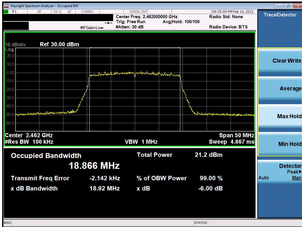
Plot 7-24. 6dB BW & 99% OBW Plot Antenna 7 (802.11ax OFDMA – RU242 – Ch. 11)
