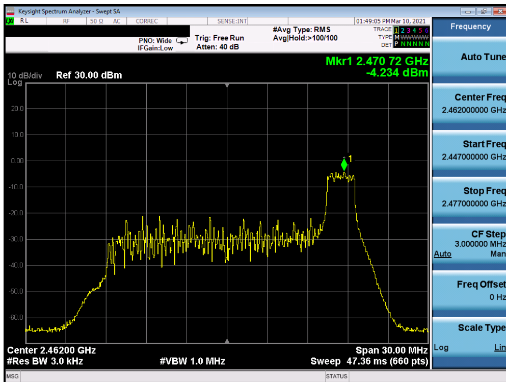
Plot 7-66. Power Spectral Density Plot CDD Antenna 7 (802.11ax OFDMA – RU26 Index 8 – Ch. 11)
