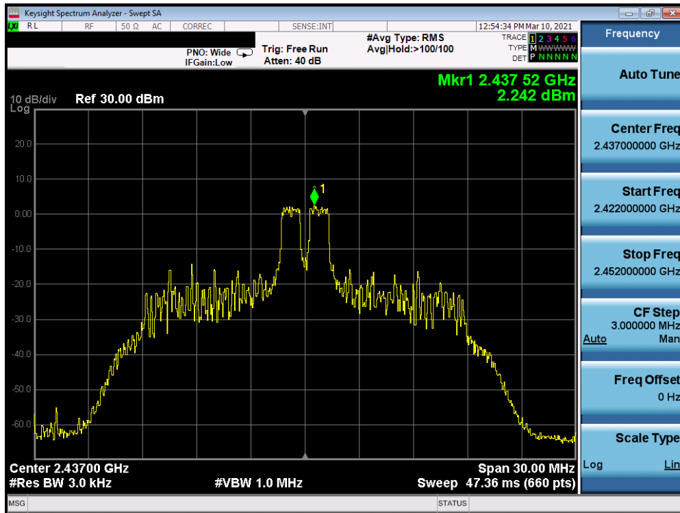
Plot 7-29. Power Spectral Density Plot Antenna 8 (802.11ax OFDMA – RU26 Index 4 – Ch. 6)
