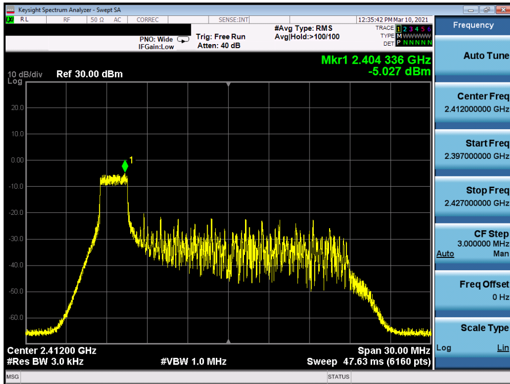
Plot 7-25. Power Spectral Density Plot Antenna 8 (802.11ax OFDMA – RU26 Index 0 – Ch. 1)
