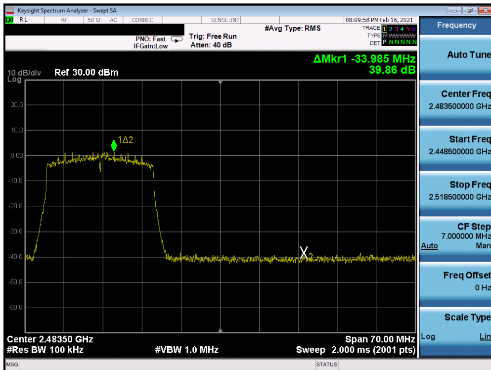
Plot 7-94. Band Edge Antenna 8 (802.11ax OFDMA – RU242 – Ch. 11)
