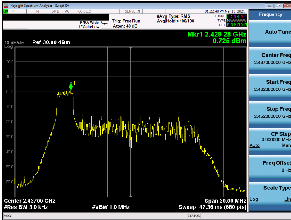
Plot 7-55. Power Spectral Density Plot CDD Antenna 8 (802.11ax OFDMA – RU26 Index 0 – Ch. 6)
