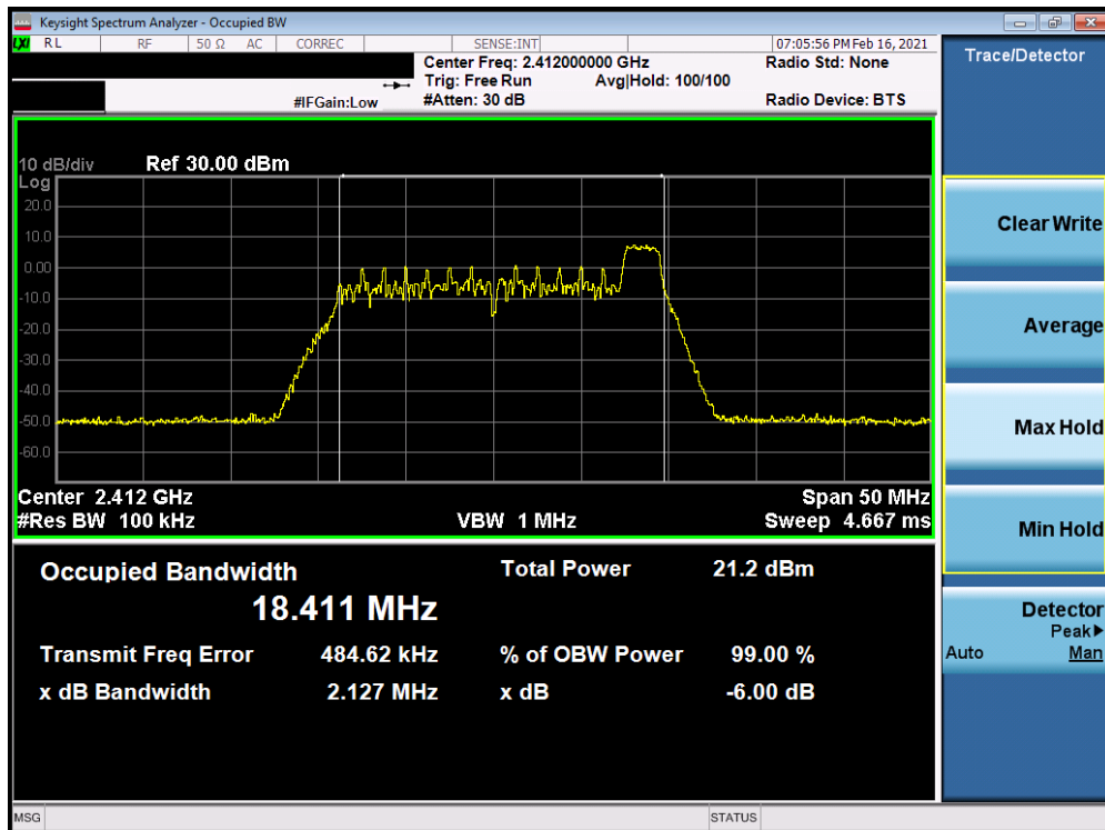
Plot 7-3. 6dB BW & 99% OBW Plot Antenna 8 (802.11ax OFDMA – RU26 Index 8 – Ch. 1)
