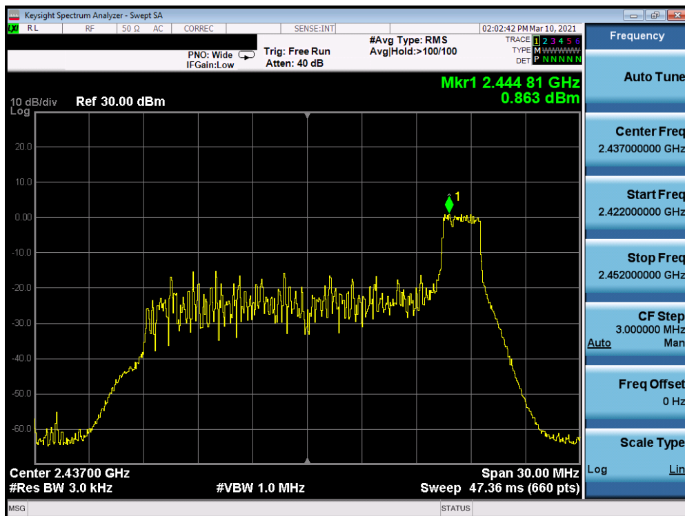
Plot 7-60. Power Spectral Density Plot CDD Antenna 7 (802.11ax OFDMA – RU26 Index 8 – Ch. 6)
