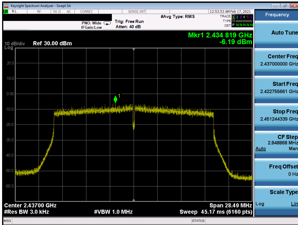
Plot 7-69. Power Spectral Density Plot CDD Antenna 8 (802.11ax OFDMA – RU242 – Ch. 6)
