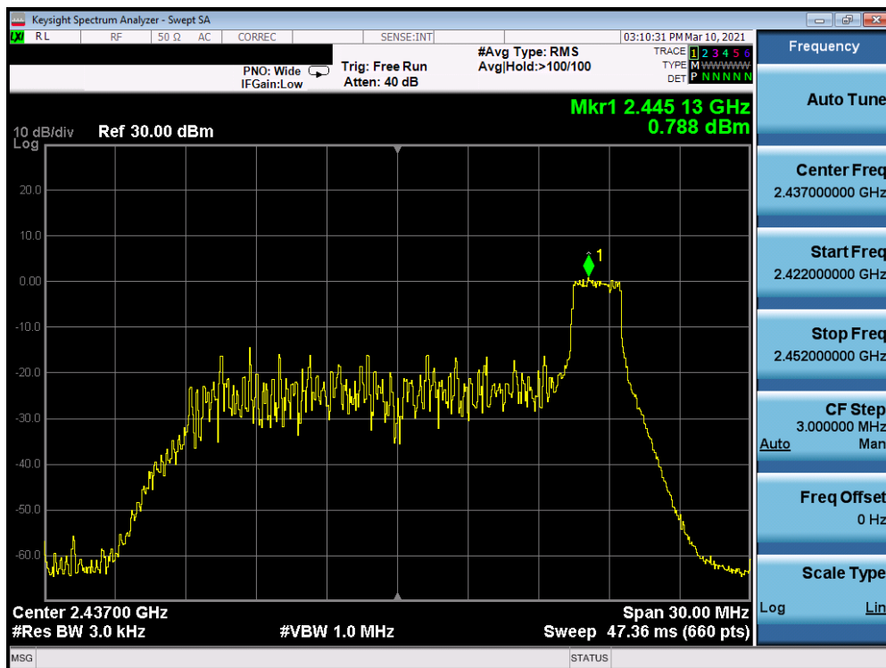
Plot 7-42. Power Spectral Density Plot Antenna 7 (802.11ax OFDMA – RU26 Index 8 – Ch. 6)
