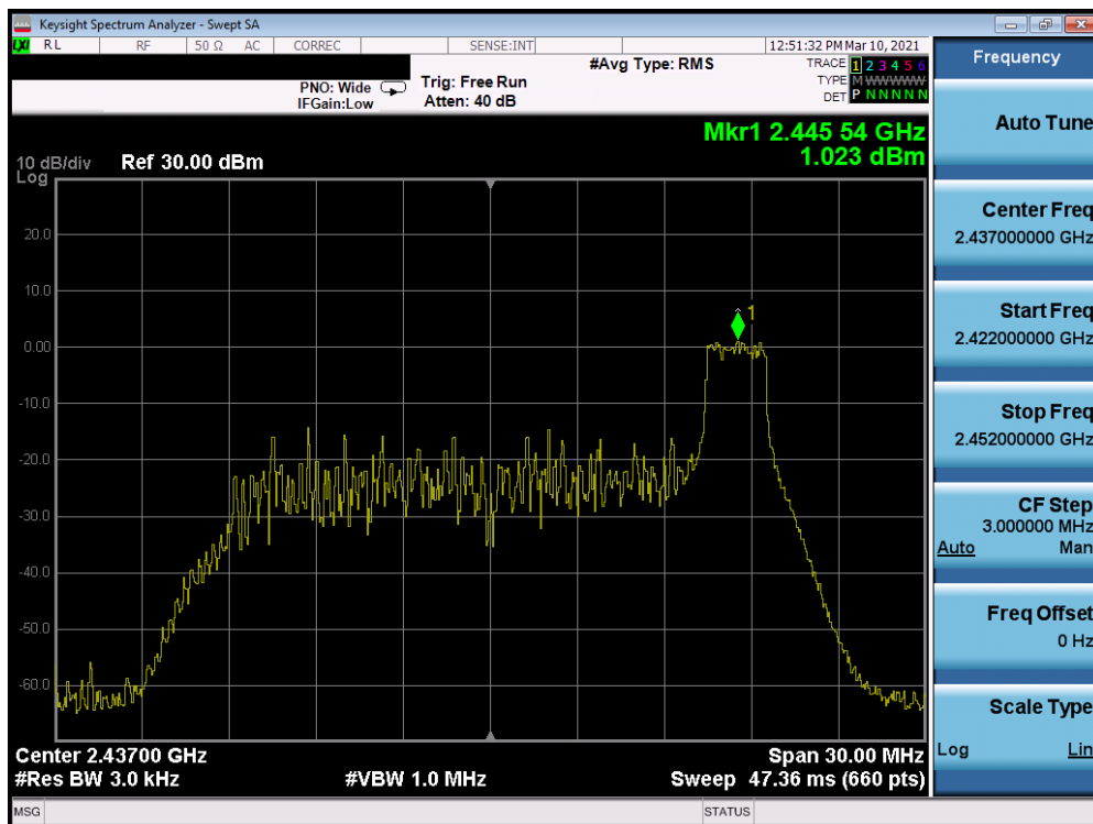
Plot 7-30. Power Spectral Density Plot Antenna 8 (802.11ax OFDMA – RU26 Index 8 – Ch. 6)
