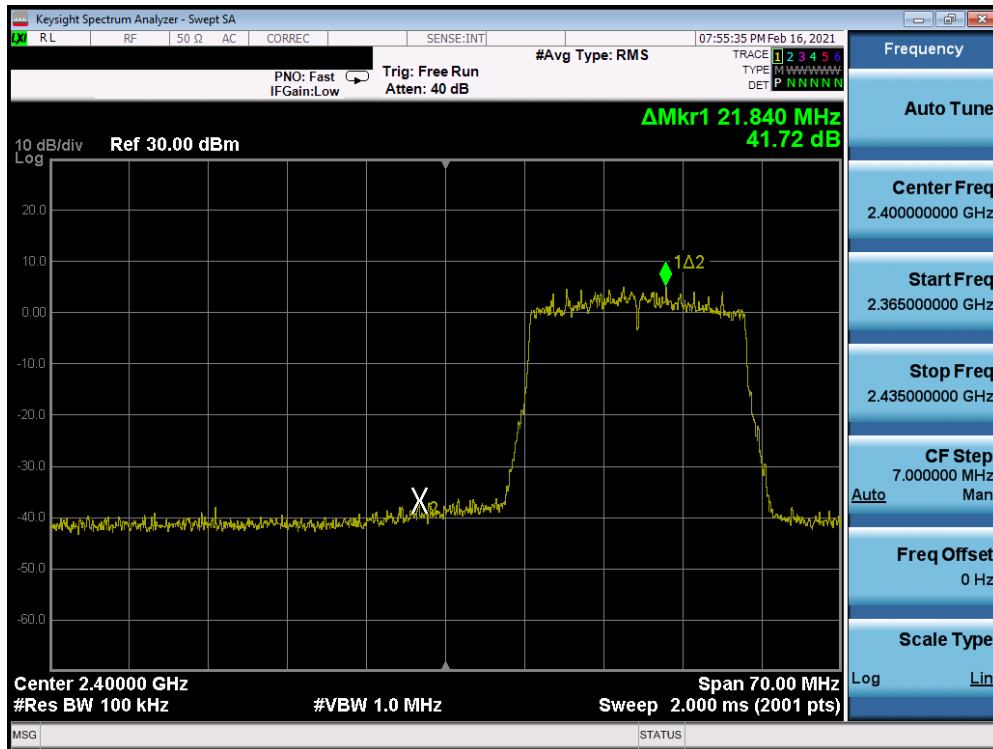
Plot 7-85. Band Edge Antenna 8 (802.11ax OFDMA – RU242 – Ch. 2)
