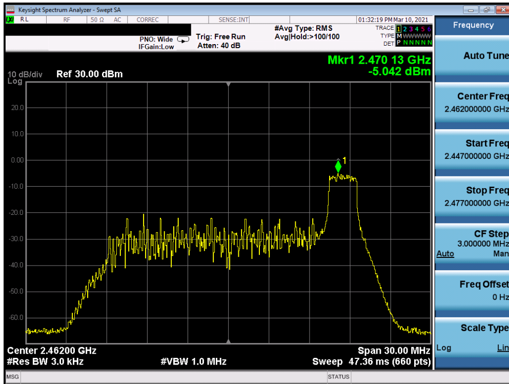
Plot 7-65. Power Spectral Density Plot CDD Antenna 8 (802.11ax OFDMA – RU26 Index 8 – Ch. 11)
