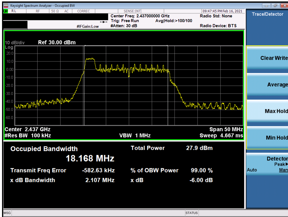
Plot 7-16. 6dB BW & 99% OBW Plot Antenna 7 (802.11ax OFDMA – RU26 Index 0 – Ch. 6)
