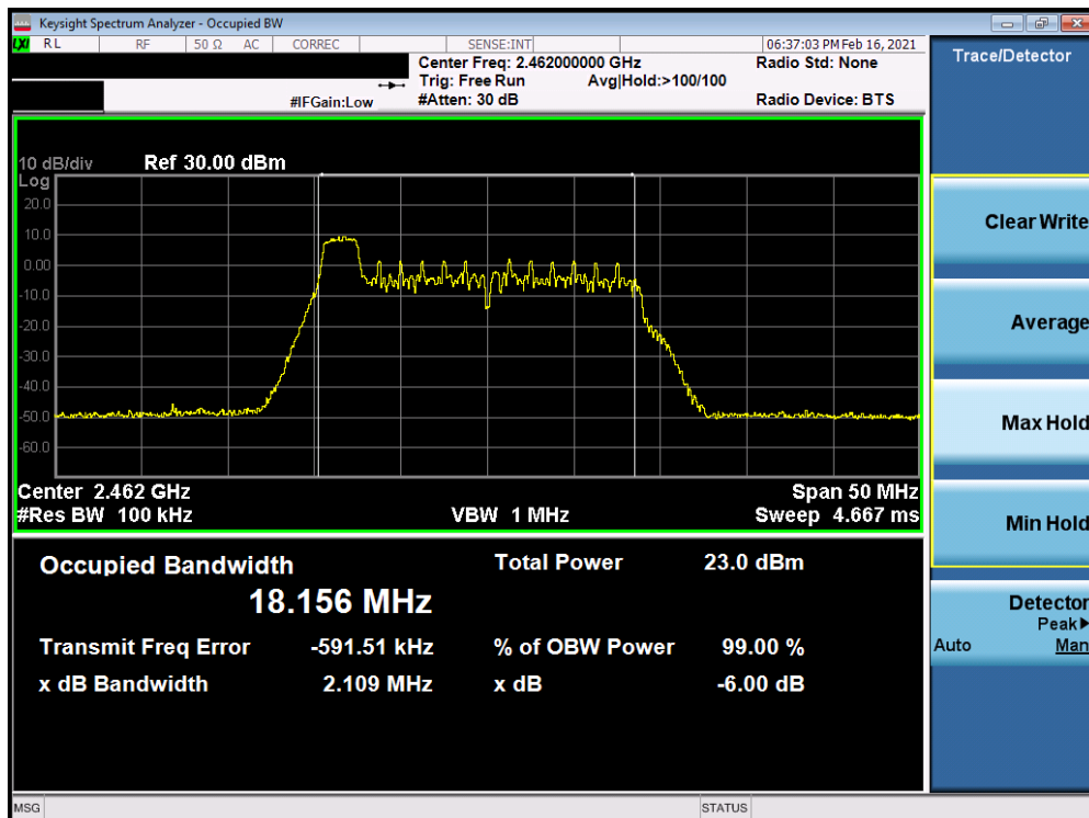
Plot 7-7. 6dB BW & 99% OBW Antenna 8 (802.11ax OFDMA – RU26 Index 0 – Ch. 11)
