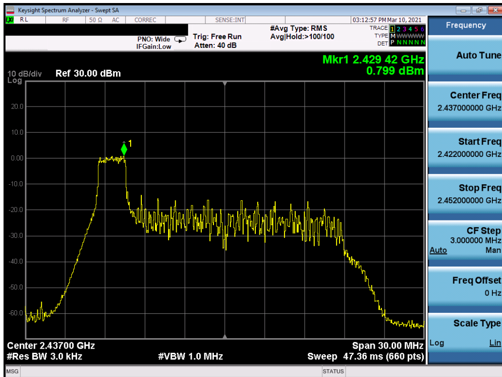
Plot 7-40. Power Spectral Density Plot Antenna 7 (802.11ax OFDMA – RU26 Index 0 – Ch. 6)
