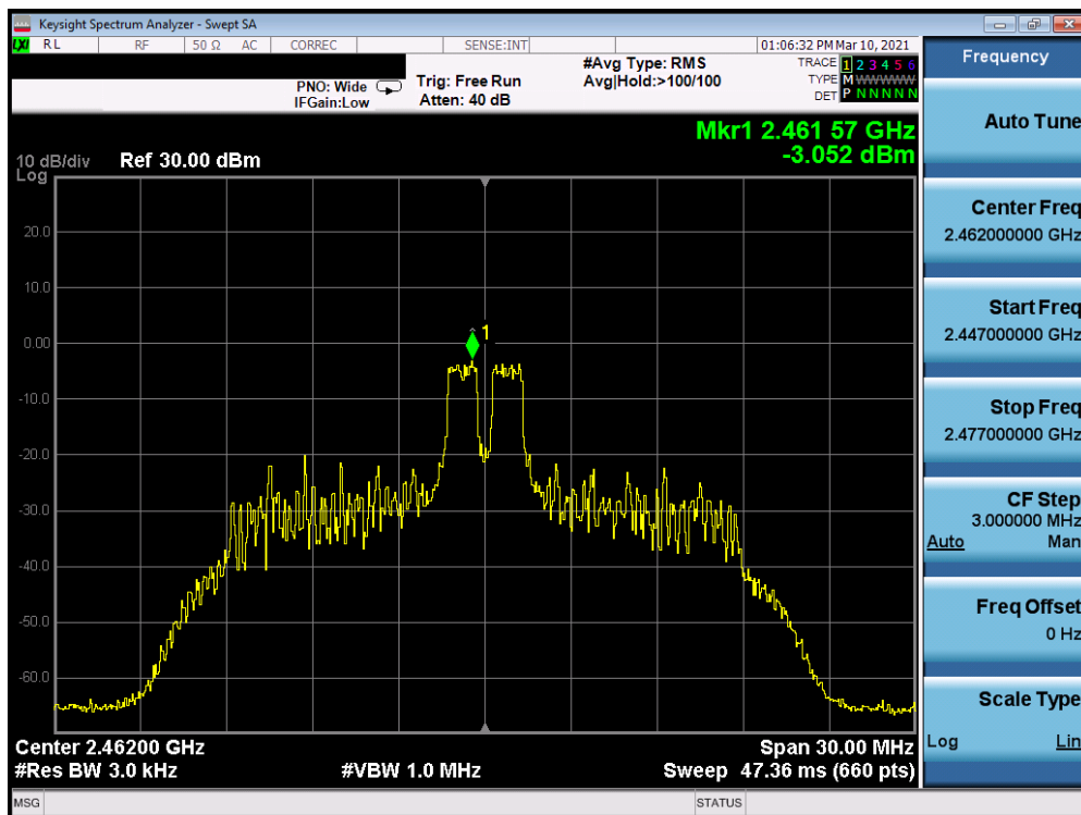
Plot 7-32. Power Spectral Density Plot Antenna 8 (802.11ax OFDMA – RU26 Index 4 – Ch. 11)
