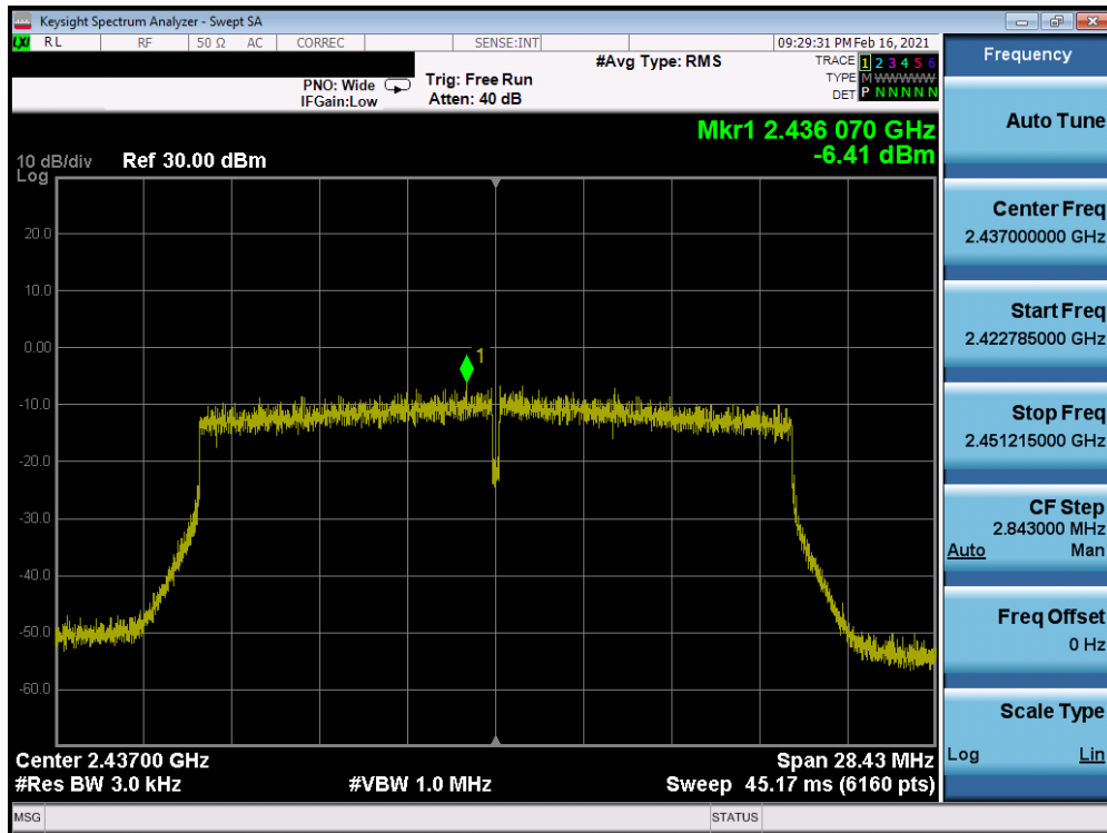
Plot 7-47. Power Spectral Density Plot Antenna 7 (802.11ax OFDMA – RU242 – Ch. 6)
