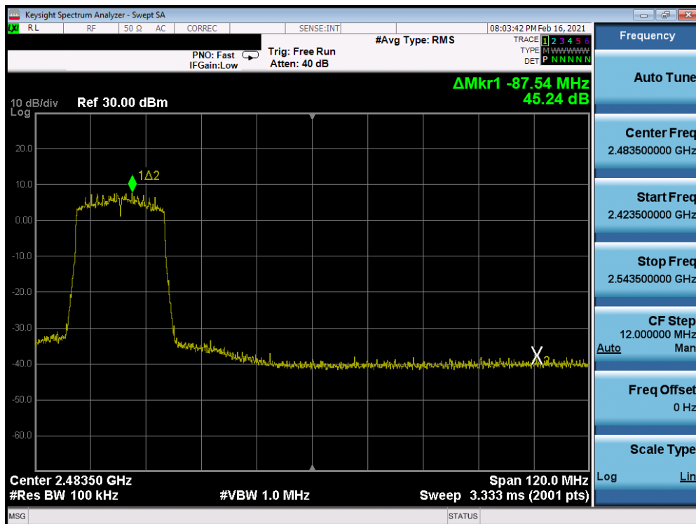
Plot 7-90. Band Edge Antenna 8 (802.11ax OFDMA – RU242 – Ch. 7)
