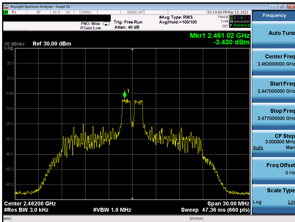
Plot 7-44. Power Spectral Density Plot Antenna 7 (802.11ax OFDMA – RU26 Index 4 – Ch. 11)
