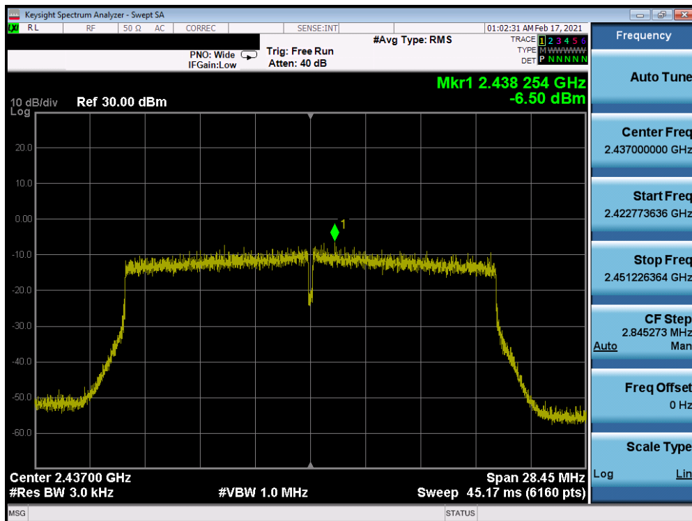
Plot 7-70. Power Spectral Density Plot CDD Antenna 7 (802.11ax OFDMA – RU242 – Ch. 6)
