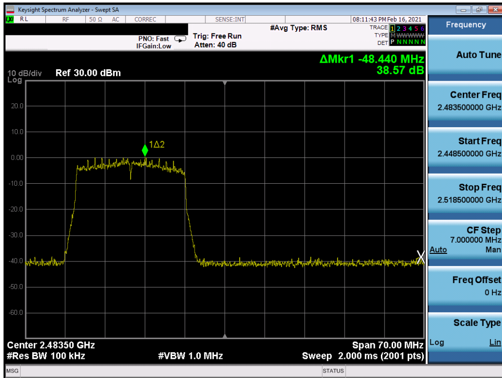
Plot 7-95. Band Edge Antenna 8 (802.11ax OFDMA – RU242 – Ch. 12)
