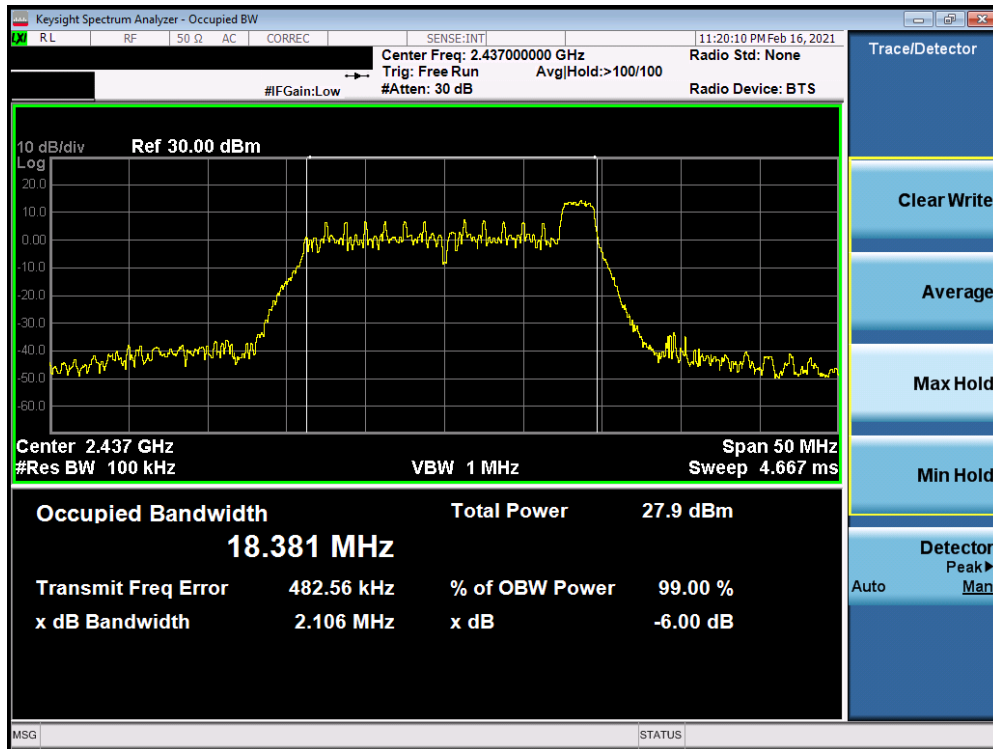
Plot 7-18. 6dB BW & 99% OBW Plot Antenna 7 (802.11ax OFDMA – RU26 Index 8 – Ch. 6)
