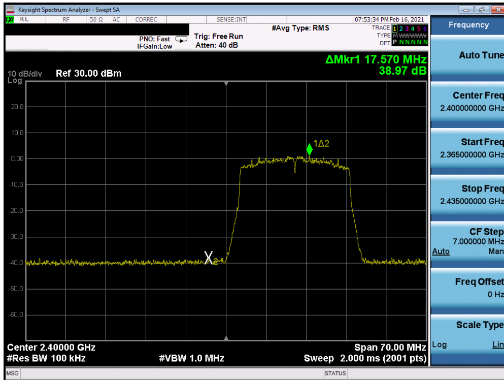
Plot 7-84. Band Edge Antenna 8 (802.11ax OFDMA – RU242 – Ch. 1)
