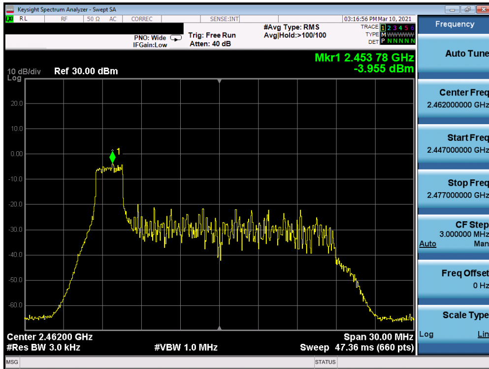
Plot 7-43. Power Spectral Density Plot Antenna 7 (802.11ax OFDMA – RU26 Index 0 – Ch. 11)
