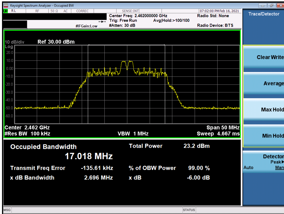
Plot 7-8. 6dB BW & 99% OBW Antenna 8 (802.11ax OFDMA – RU26 Index 4 – Ch. 11)
