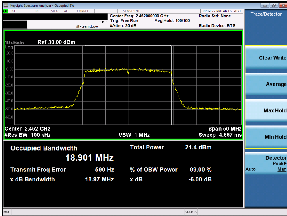
Plot 7-12. 6dB BW & 99% OBW Plot Antenna 8 (802.11ax OFDMA – RU242 – Ch. 11)
