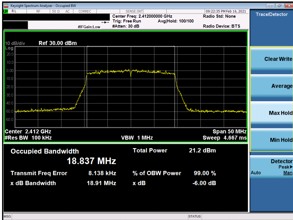
Plot 7-22. 6dB BW & 99% OBW Plot Antenna 7 (802.11ax OFDMA – RU242 – Ch. 1)
