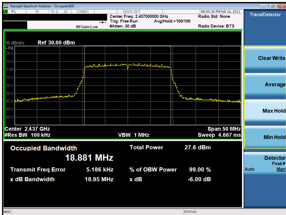
Plot 7-11. 6dB BW & 99% OBW Plot Antenna 8 (802.11ax OFDMA – RU242 – Ch. 6)
