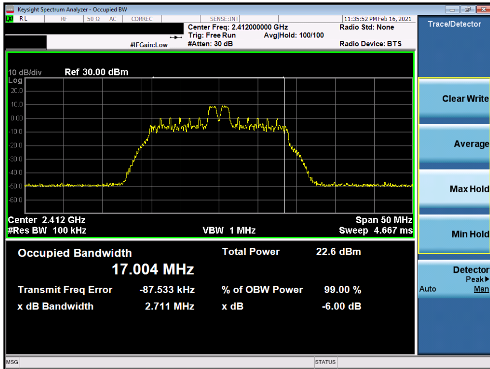
Plot 7-14. 6dB BW & 99% OBW Plot Antenna 7 (802.11ax OFDMA – RU26 Index 4 – Ch. 1)
