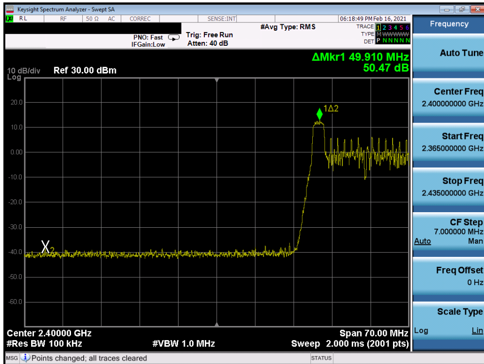
Plot 7-76. Band Edge Antenna 8 (802.11ax OFDMA – RU26 Index 0 – Ch. 4)
