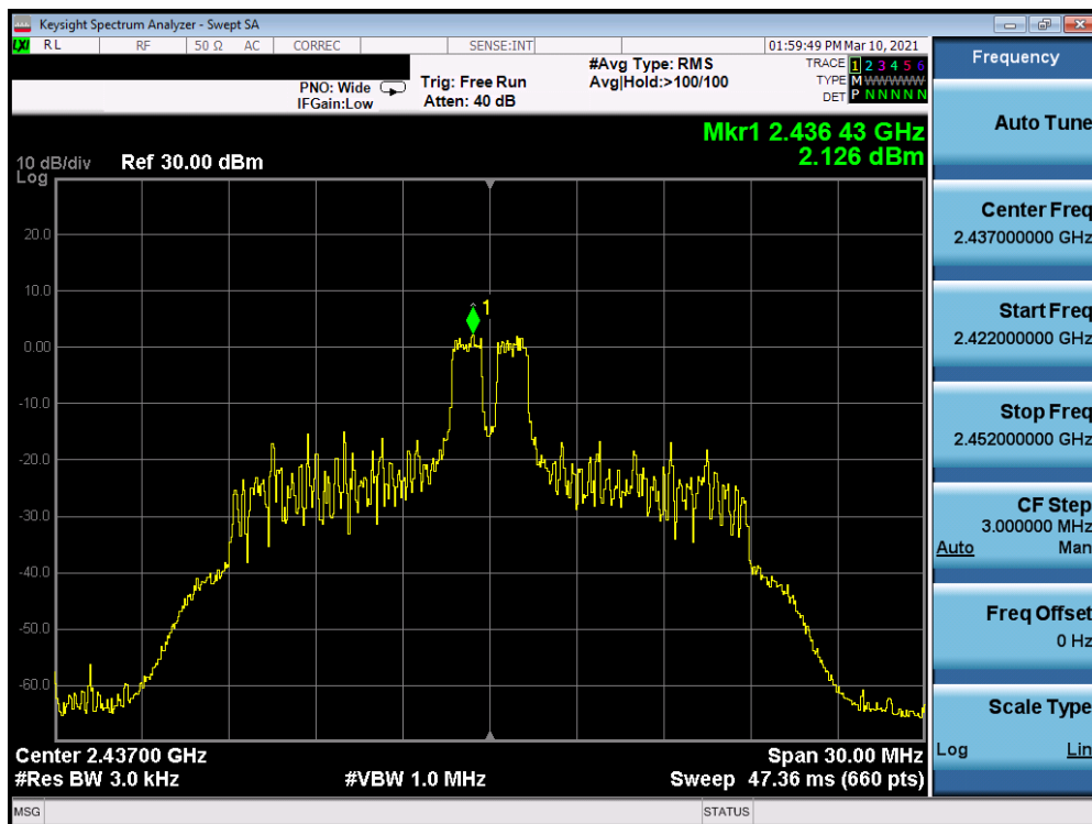
Plot 7-58. Power Spectral Density Plot CDD Antenna 7 (802.11ax OFDMA – RU26 Index 4 – Ch. 6)
