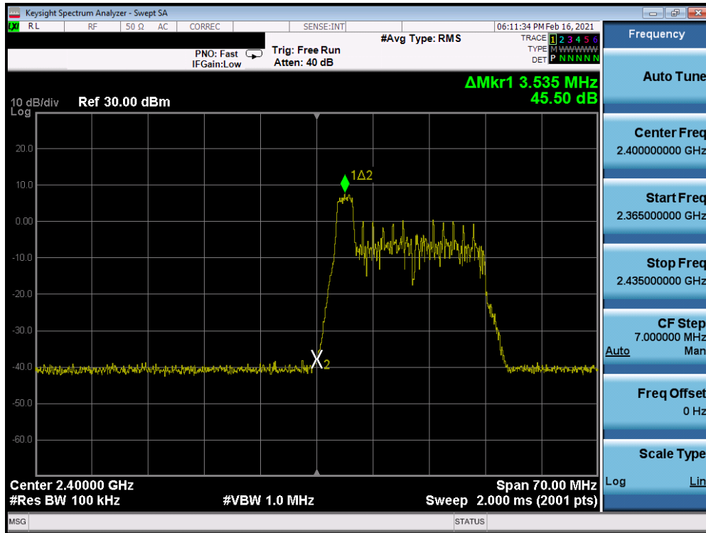
Plot 7-73. Band Edge Antenna 8 (802.11ax OFDMA – RU26 Index 0 – Ch. 1)
