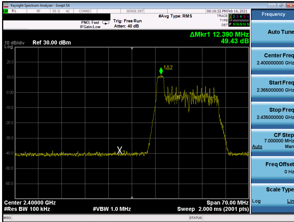
Plot 7-74. Band Edge Antenna 8 (802.11ax OFDMA – RU26 Index 0 – Ch. 2)
