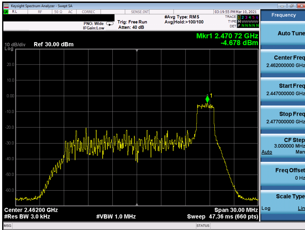
Plot 7-45. Power Spectral Density Plot Antenna 7 (802.11ax OFDMA – RU26 Index 8 – Ch. 11)
