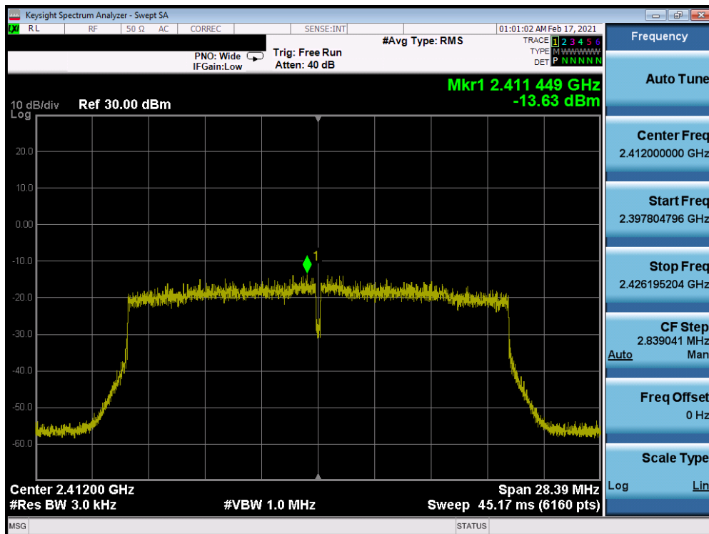
Plot 7-68. Power Spectral Density Plot CDD Antenna 7 (802.11ax OFDMA – RU242 – Ch. 1)
