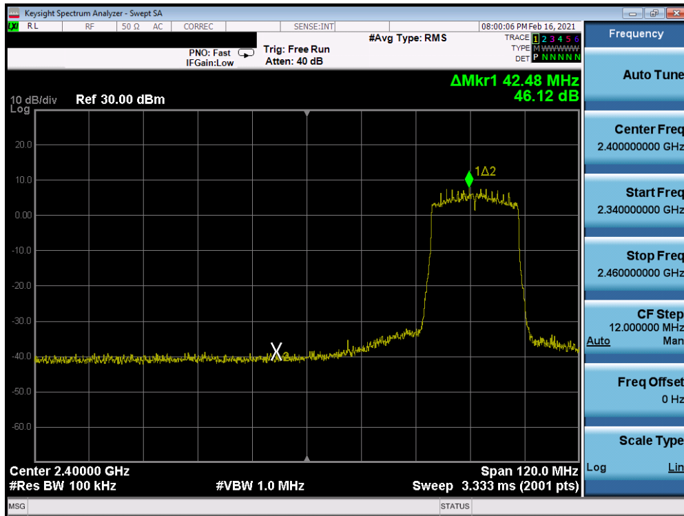
Plot 7-89. Band Edge Antenna 8 (802.11ax OFDMA – RU242 – Ch. 6)
