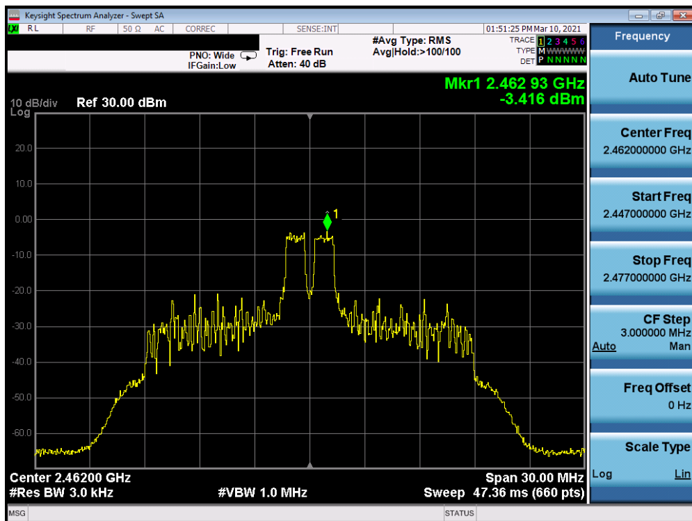
Plot 7-64. Power Spectral Density Plot CDD Antenna 7 (802.11ax OFDMA – RU26 Index 4 – Ch. 11)
