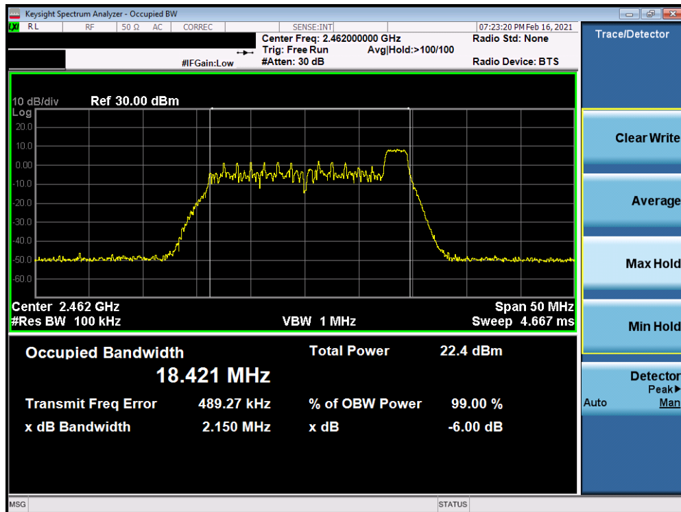
Plot 7-9. 6dB BW & 99% OBW Plot Antenna 8 (802.11ax OFDMA – RU26 Index 8 – Ch. 11)
