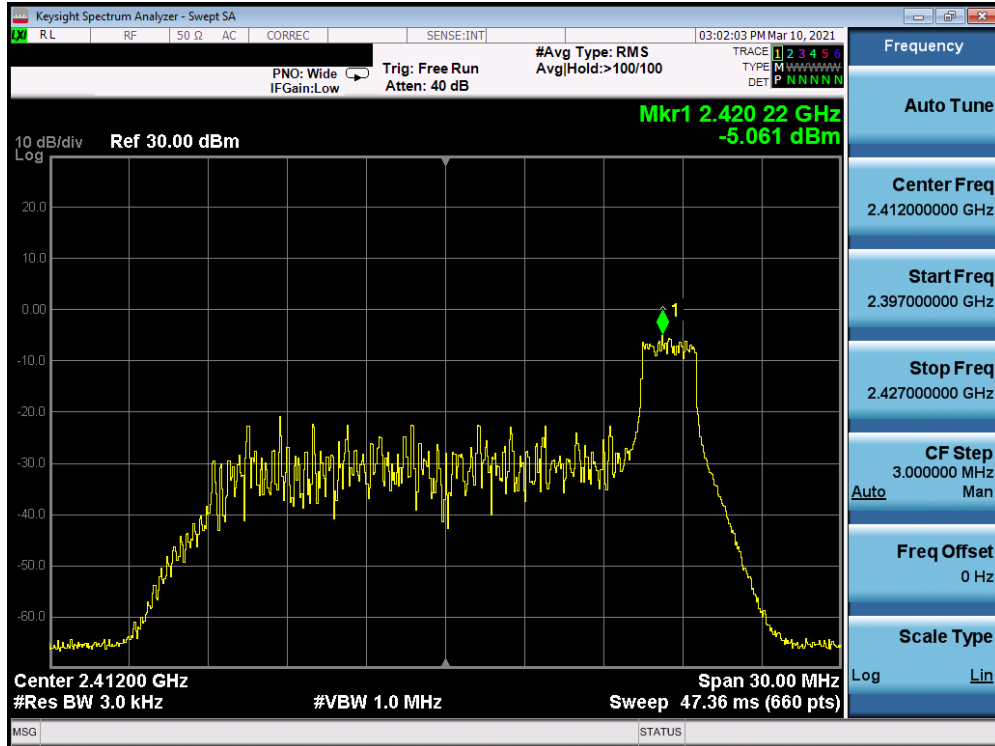
Plot 7-39. Power Spectral Density Plot Antenna 7 (802.11ax OFDMA – RU26 Index 8 – Ch. 1)
