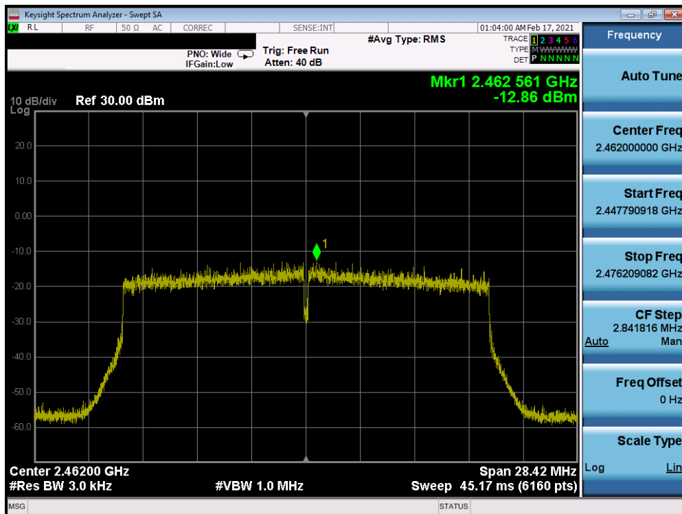
Plot 7-72. Power Spectral Density Plot CDD Antenna 7 (802.11ax OFDMA – RU242 – Ch. 11)
