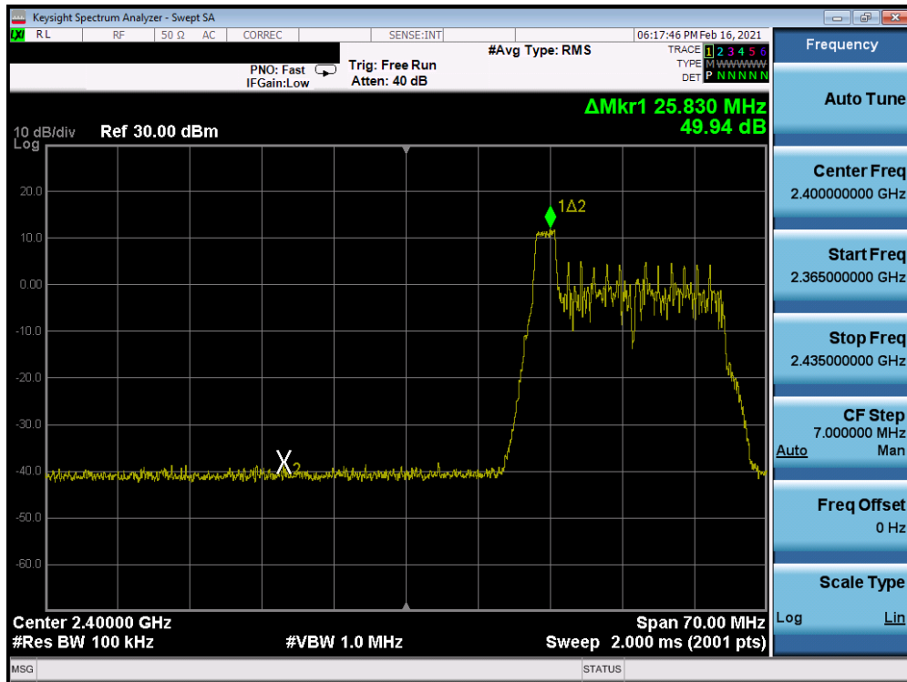
Plot 7-75. Band Edge Antenna 8 (802.11ax OFDMA – RU26 Index 0 – Ch. 3)
