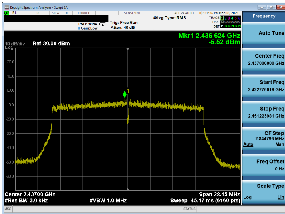
Plot 7-35. Power Spectral Density Plot Antenna 8 (802.11ax OFDMA – RU242 – Ch. 6)
