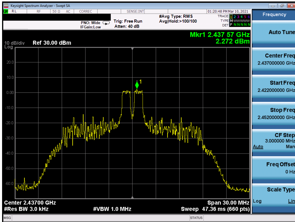
Plot 7-57. Power Spectral Density Plot CDD Antenna 8 (802.11ax OFDMA – RU26 Index 4 – Ch. 6)
