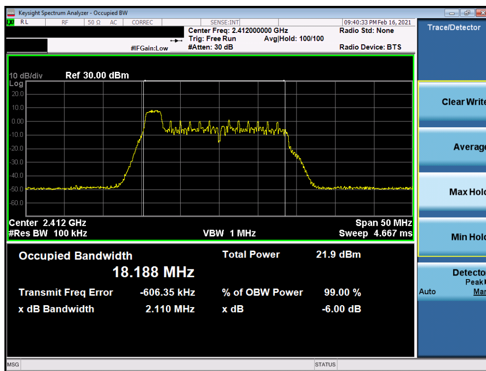
Plot 7-13. 6dB BW & 99% OBW Plot Antenna 7 (802.11ax OFDMA – RU26 Index 0 – Ch. 1)
