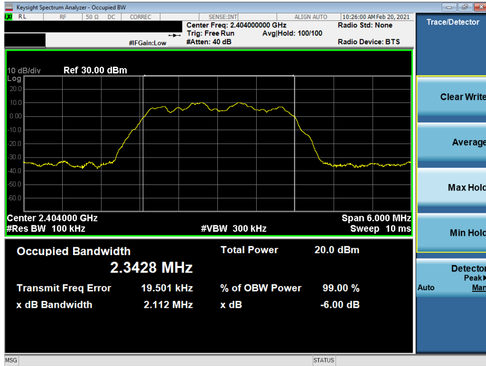
Plot 7-7. 6dB BW & 99% OBW Plot Antenna 7 (Bluetooth (HDR4), 4Mbps, ePA – Ch. 1)
