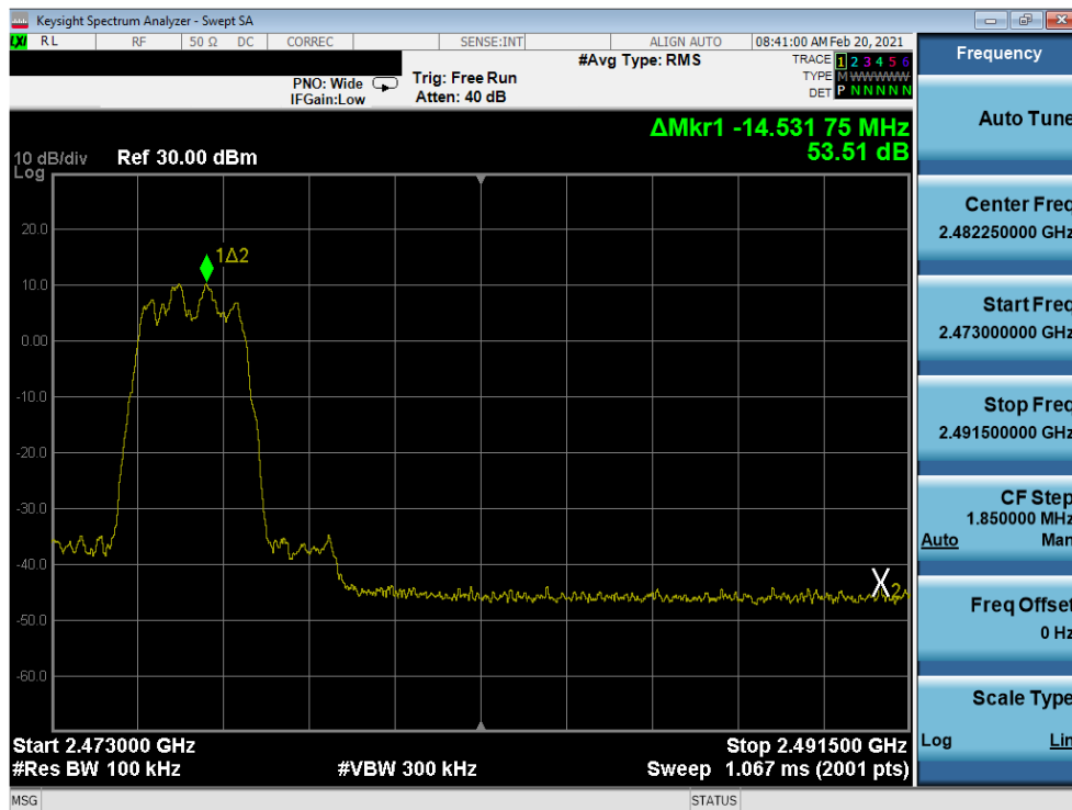
Plot 7-62. Band Edge Plot Antenna 8 (Bluetooth (HDR4), ePA – Ch. 73)
