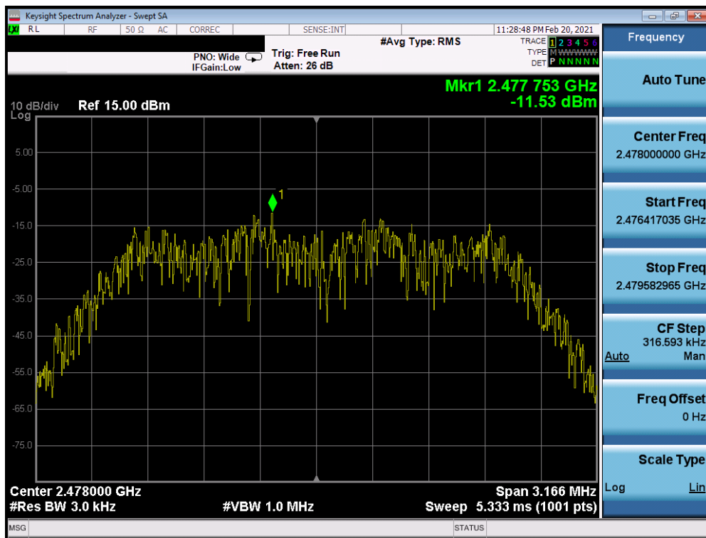
Plot 7-48. Power Spectral Density Plot TxBF Antenna 7 (Bluetooth (HDR4), 4Mbps, iPA – Ch. 73)
