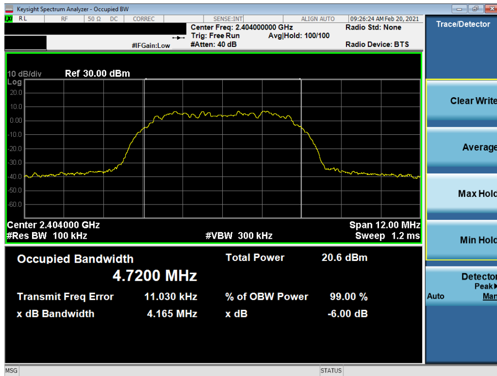
Plot 7-4. 6dB BW & 99% OBW Plot Antenna 8 (Bluetooth (HDR8), 8Mbps, ePA – Ch. 1)
