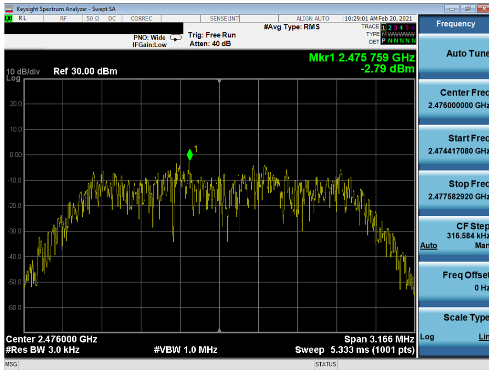
Plot 7-27. Power Spectral Density Plot Antenna 7 (Bluetooth (HDR4), 4Mbps, ePA – Ch. 73)
