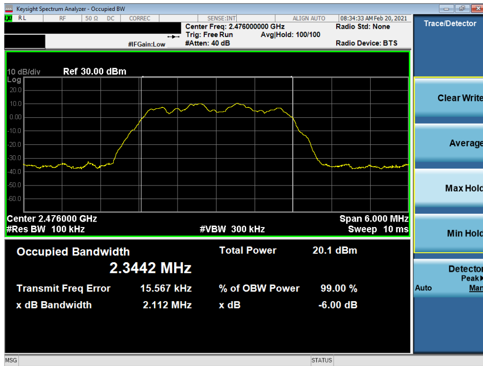
Plot 7-3. 6dB BW & 99% OBW Plot Antenna 8 (Bluetooth (HDR4), 4Mbps, ePA – Ch. 73)
