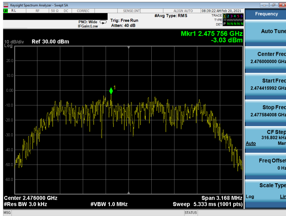
Plot 7-15. Power Spectral Density Plot Antenna 8 (Bluetooth (HDR4), 4Mbps, ePA – Ch. 73)
