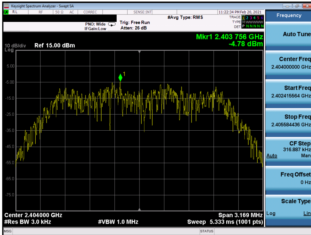
Plot 7-38. Power Spectral Density Plot TxBF Antenna 7 (Bluetooth (HDR4), 4Mbps, ePA – Ch. 1)
