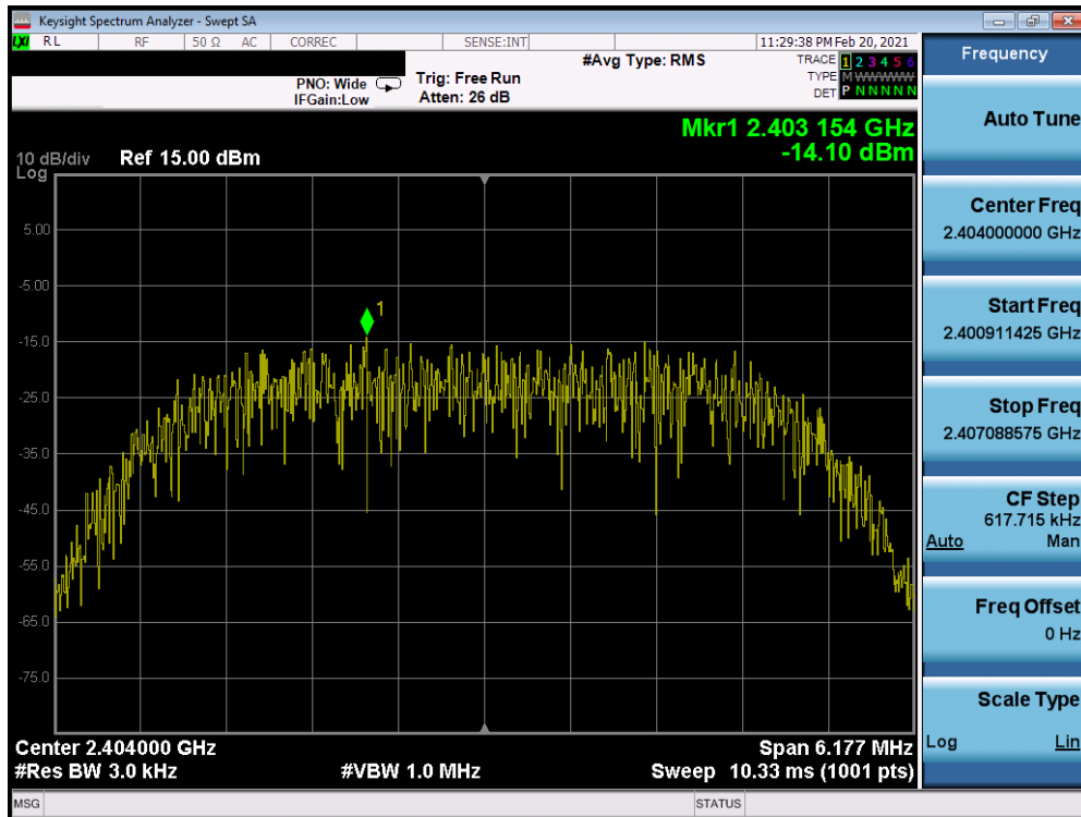
Plot 7-56. Power Spectral Density Plot TxBF Antenna 7 (Bluetooth (HDR8), 8Mbps, iPA – Ch. 1)
