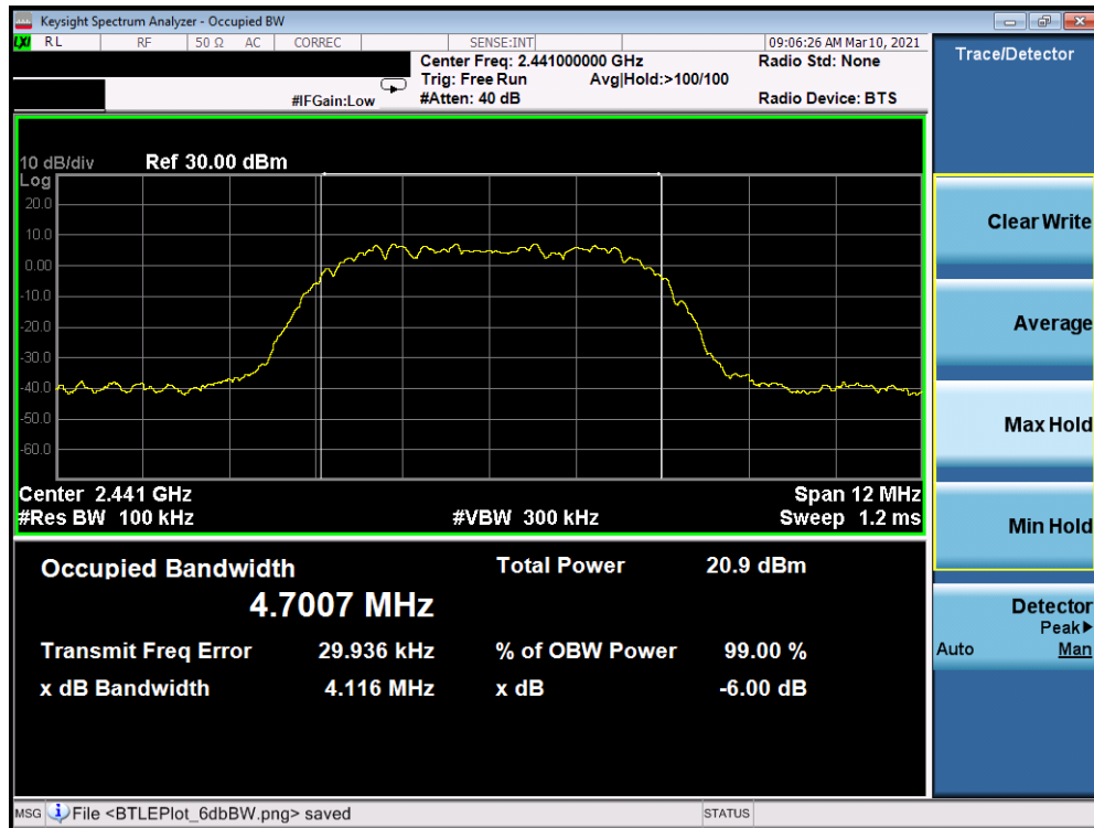
Plot 7-5. 6dB BW & 99% OBW Plot Antenna 8 (Bluetooth (HDR8), 8Mbps, ePA – Ch. 38)
