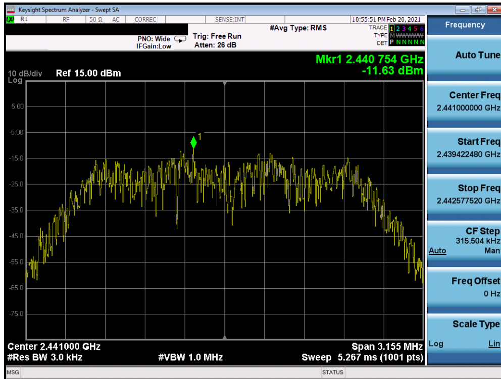
Plot 7-45. Power Spectral Density Plot TxBF Antenna 8 (Bluetooth (HDR4), 4Mbps, iPA – Ch. 38)
