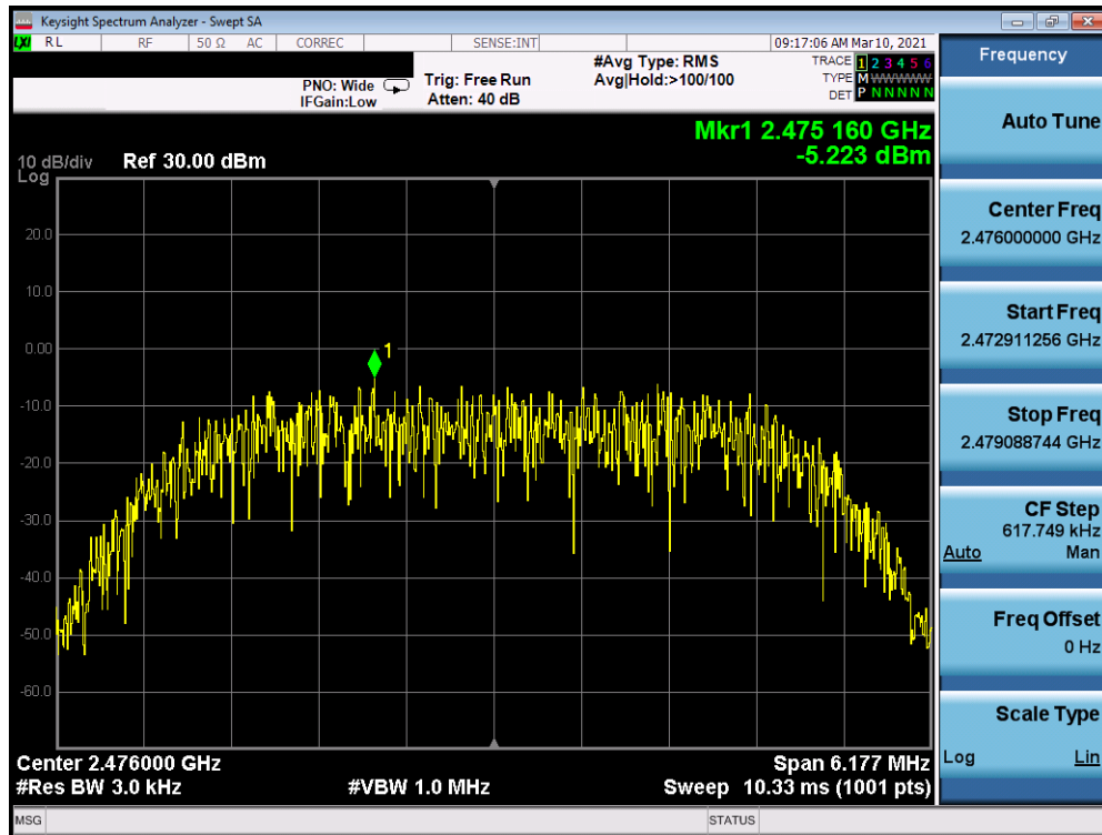
Plot 7-21. Power Spectral Density Plot Antenna 8 (Bluetooth (HDR8), 8Mbps, ePA – Ch. 73)
