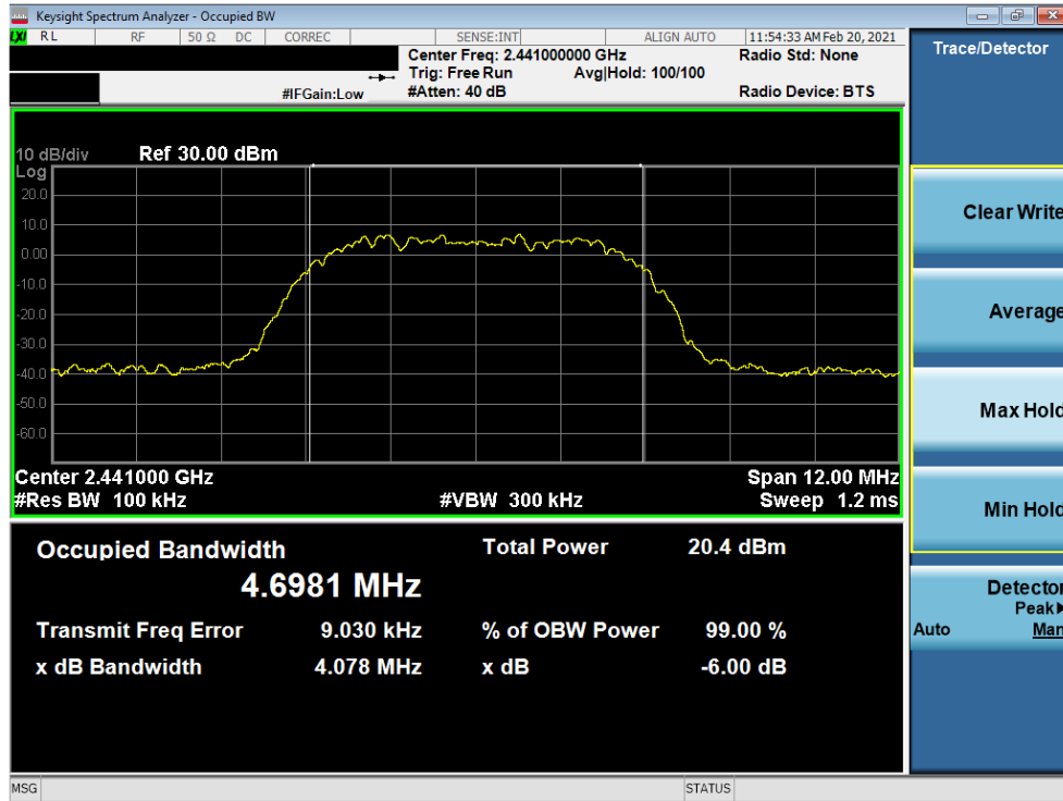
Plot 7-11. 6dB BW & 99% OBW Plot Antenna 7 (Bluetooth (HDR8), 8Mbps, ePA – Ch. 38)
