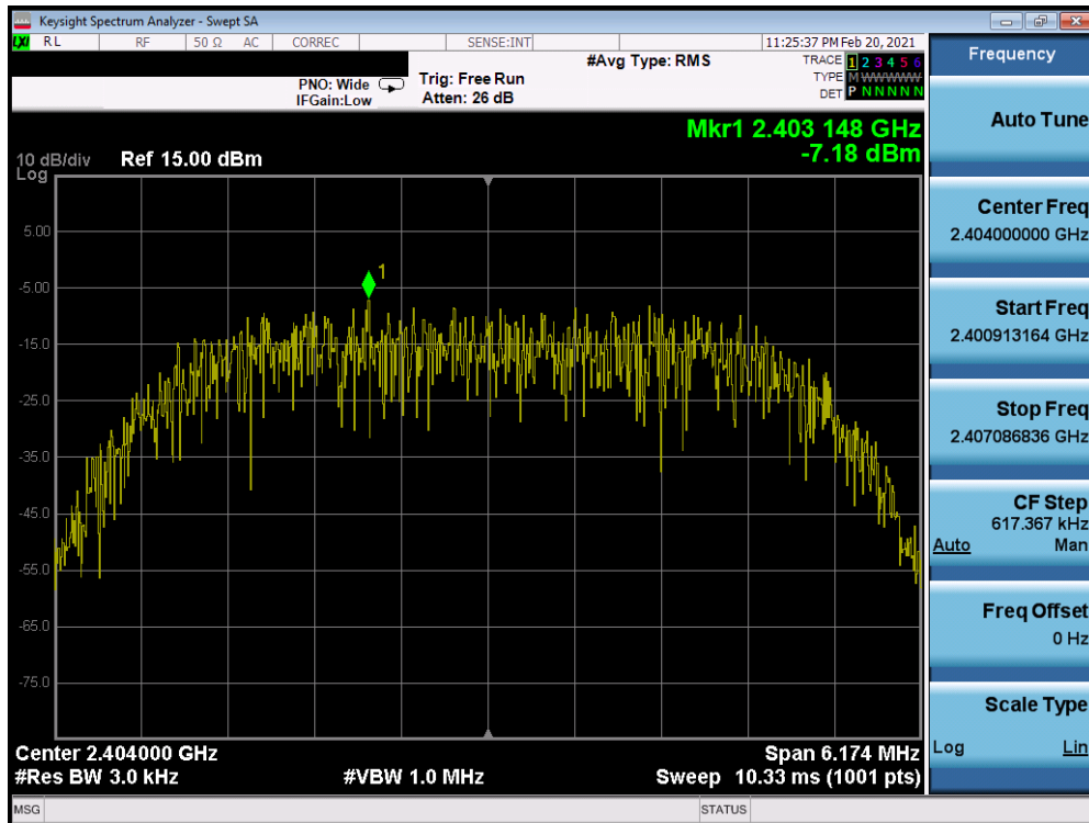
Plot 7-50. Power Spectral Density Plot TxBF Antenna 7 (Bluetooth (HDR8), 8Mbps, ePA – Ch. 1)
