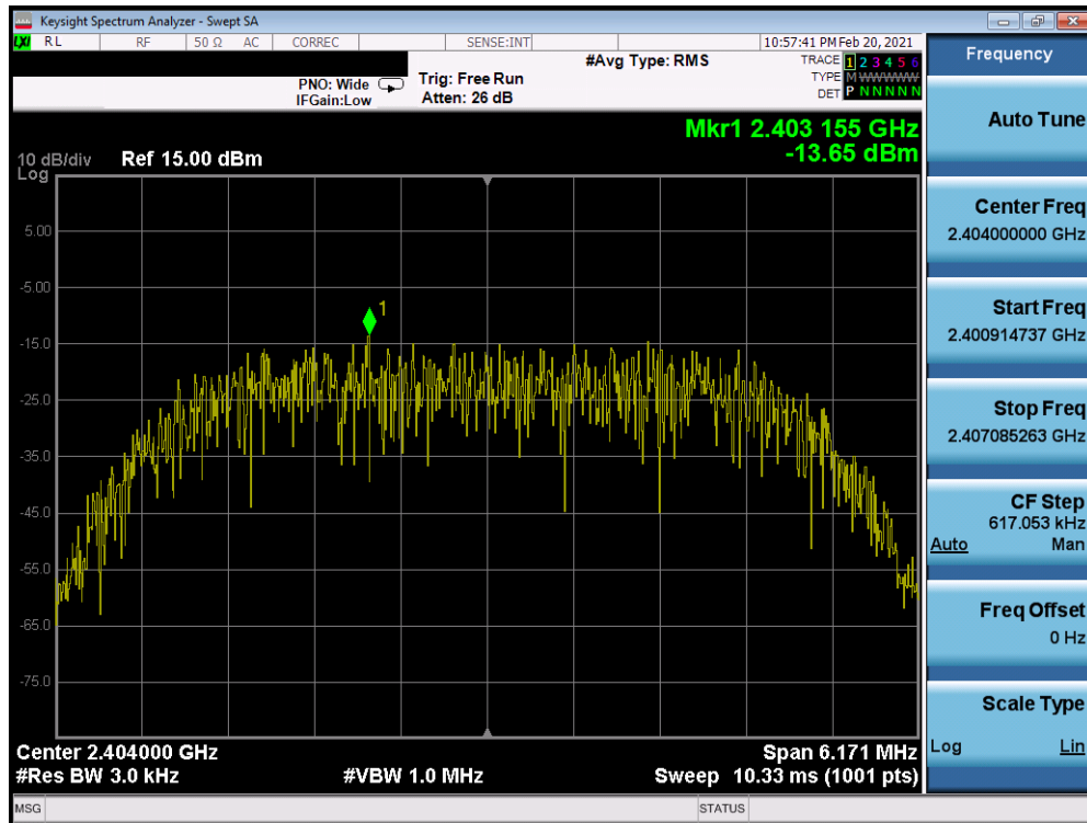
Plot 7-55. Power Spectral Density Plot TxBF Antenna 8 (Bluetooth (HDR8), 8Mbps, iPA – Ch. 1)
