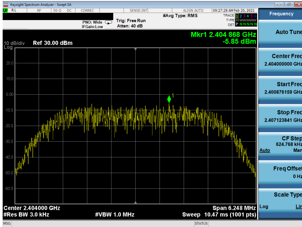
Plot 7-19. Power Spectral Density Plot Antenna 8 (Bluetooth (HDR8), 8Mbps, ePA – Ch. 1)
