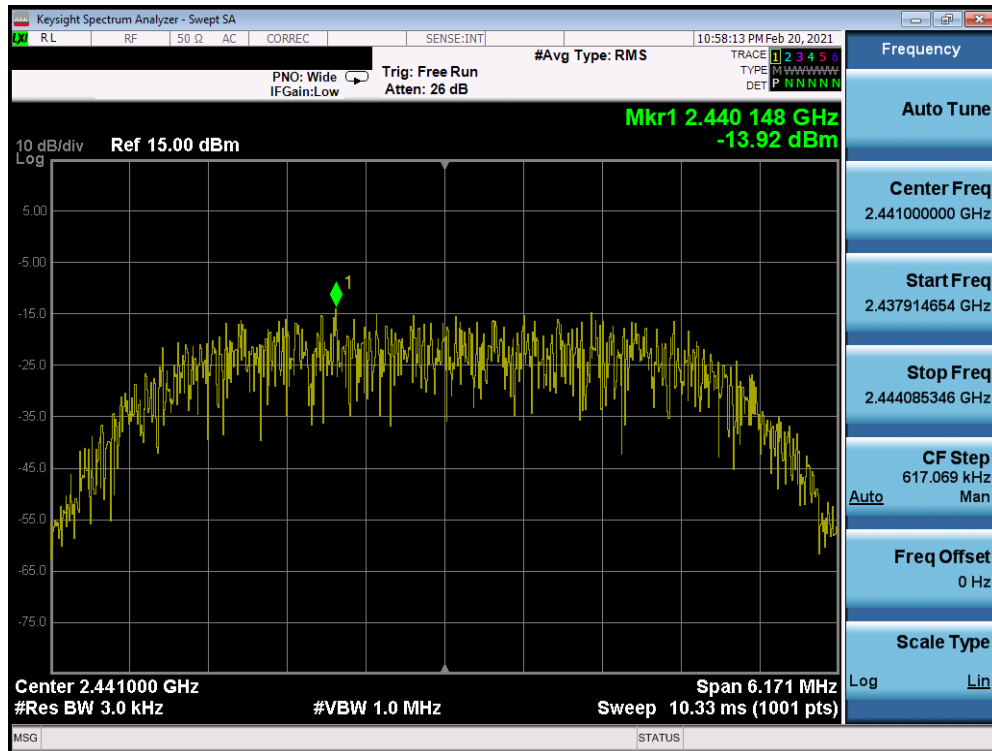
Plot 7-57. Power Spectral Density Plot TxBF Antenna 8 (Bluetooth (HDR8), 8Mbps, iPA – Ch. 38)
