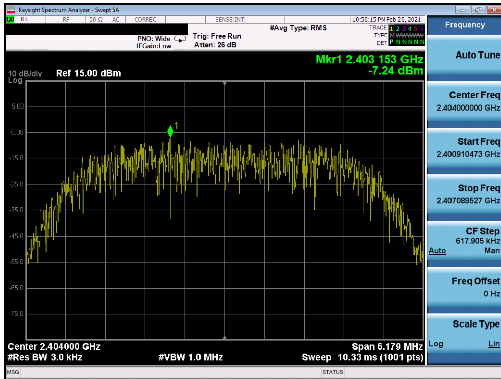
Plot 7-49. Power Spectral Density Plot TxBF Antenna 8 (Bluetooth (HDR8), 8Mbps, ePA – Ch. 1)
