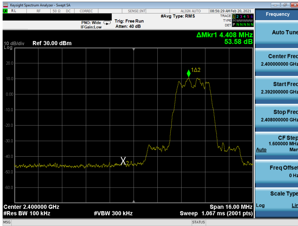
Plot 7-61. Band Edge Plot Antenna 8 (Bluetooth (HDR4), ePA – Ch. 1)
