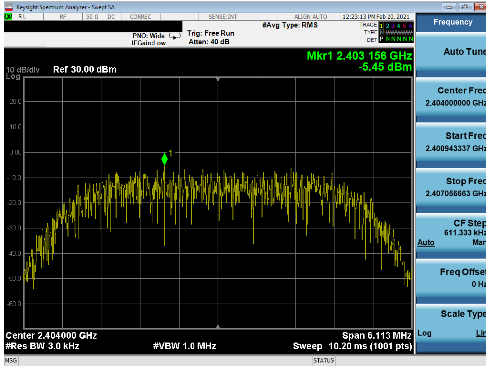
Plot 7-31. Power Spectral Density Plot Antenna 7 (Bluetooth (HDR8), 8Mbps, ePA – Ch. 1)
