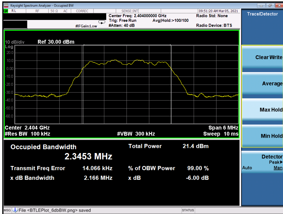
Plot 7-1. 6dB BW & 99% OBW Plot Antenna 8 (Bluetooth (HDR4), 4Mbps, ePA – Ch. 1)
