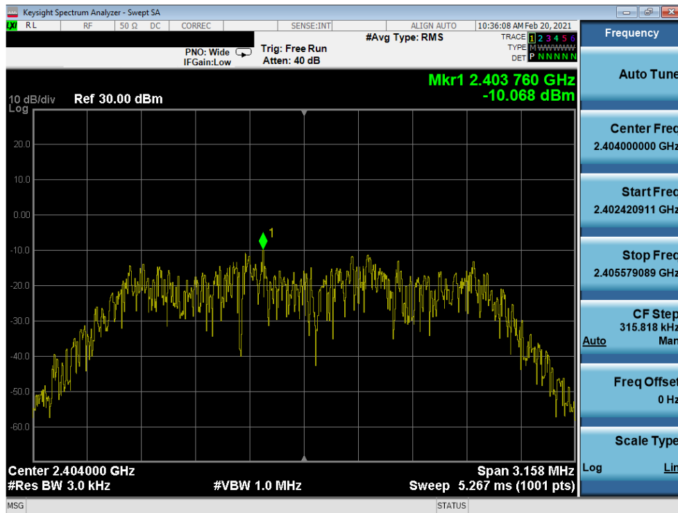
Plot 7-28. Power Spectral Density Plot Antenna 7 (Bluetooth (HDR4), 4Mbps, iPA – Ch. 1)
