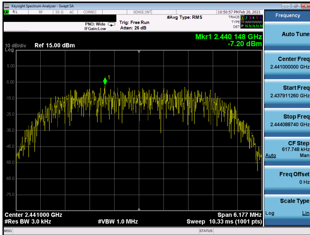
Plot 7-51. Power Spectral Density Plot TxBF Antenna 8 (Bluetooth (HDR8), 8Mbps, ePA – Ch. 38)
