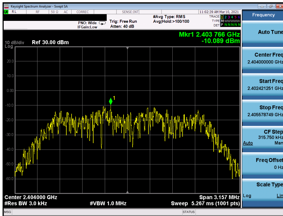
Plot 7-16. Power Spectral Density Plot Antenna 8 (Bluetooth (HDR4), 4Mbps, iPA – Ch. 1)
