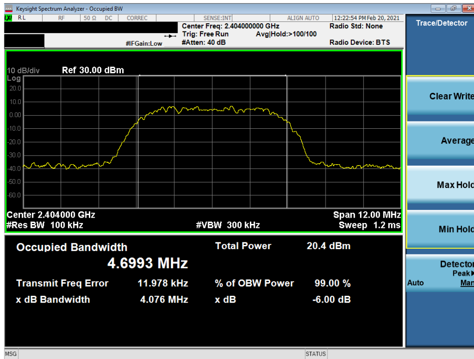
Plot 7-10. 6dB BW & 99% OBW Plot Antenna 7 (Bluetooth (HDR8), 8Mbps, ePA – Ch. 1)
