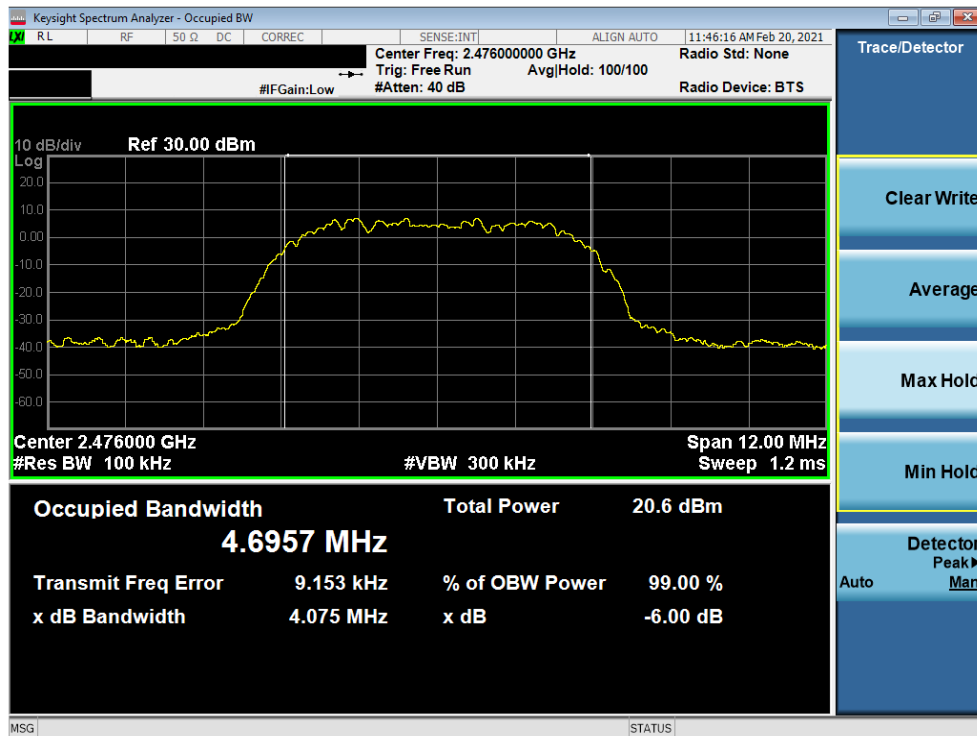
Plot 7-12. 6dB BW & 99% OBW Plot Antenna 7 (Bluetooth (HDR8), 8Mbps, ePA – Ch. 73)
