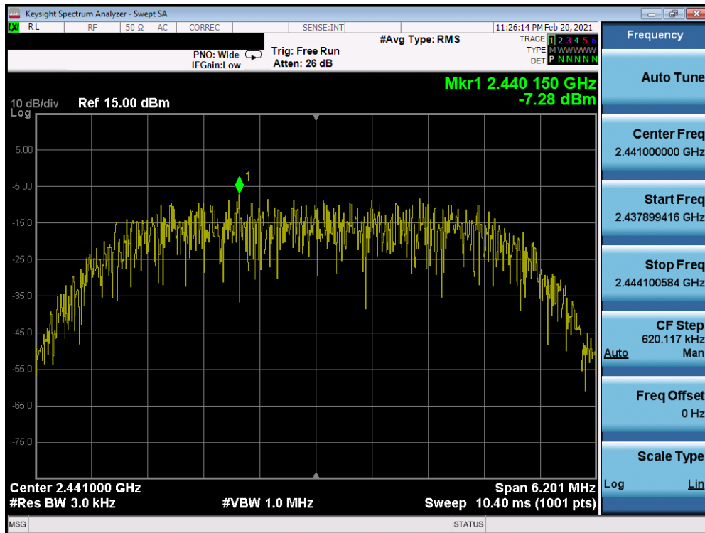
Plot 7-52. Power Spectral Density Plot TxBF Antenna 7 (Bluetooth (HDR8), 8Mbps, ePA – Ch. 38)
