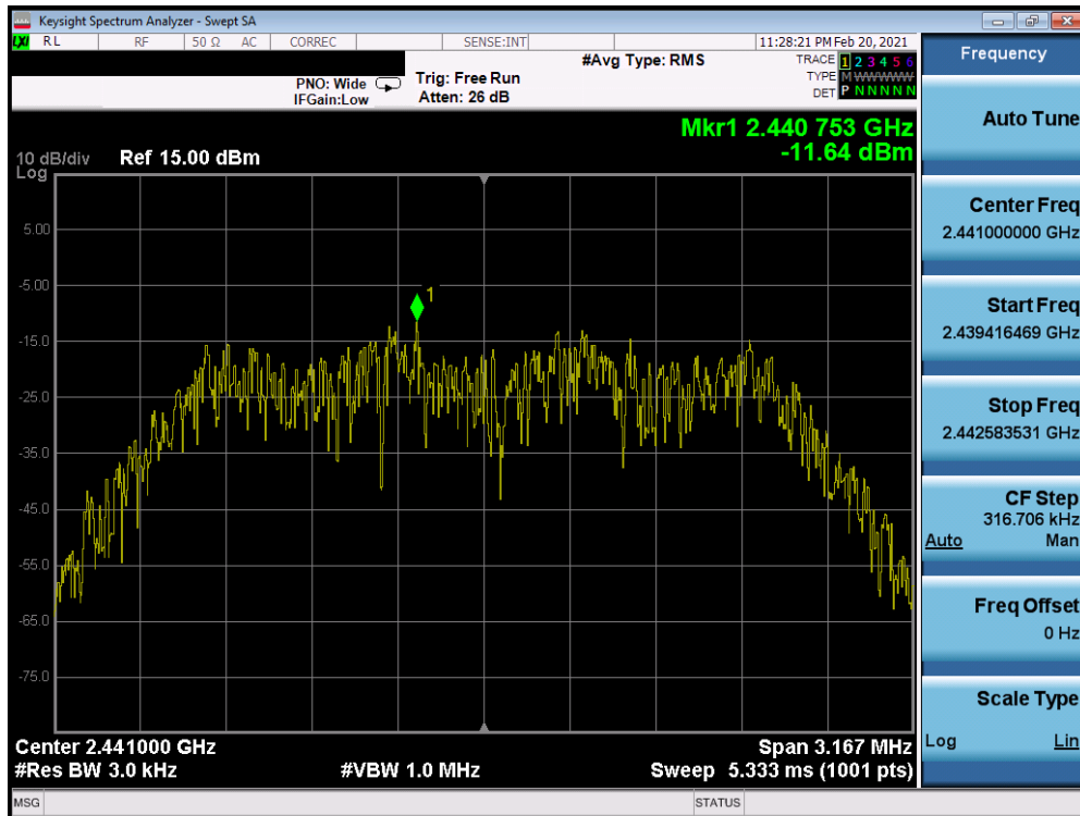
Plot 7-46. Power Spectral Density Plot TxBF Antenna 7 (Bluetooth (HDR4), 4Mbps, iPA – Ch. 38)
