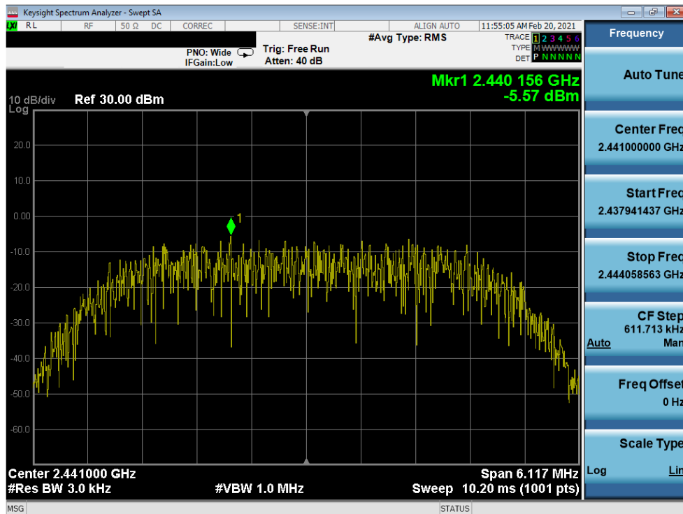
Plot 7-32. Power Spectral Density Plot Antenna 7 (Bluetooth (HDR8), 8Mbps, ePA – Ch. 38)
