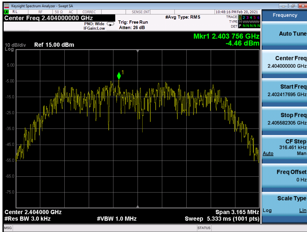
Plot 7-37. Power Spectral Density Plot TxBF Antenna 8 (Bluetooth (HDR4), 4Mbps, ePA – Ch. 1)
