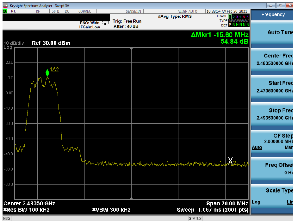
Plot 7-66. Band Edge Plot Antenna 7 (Bluetooth (HDR4), ePA – Ch. 73)
