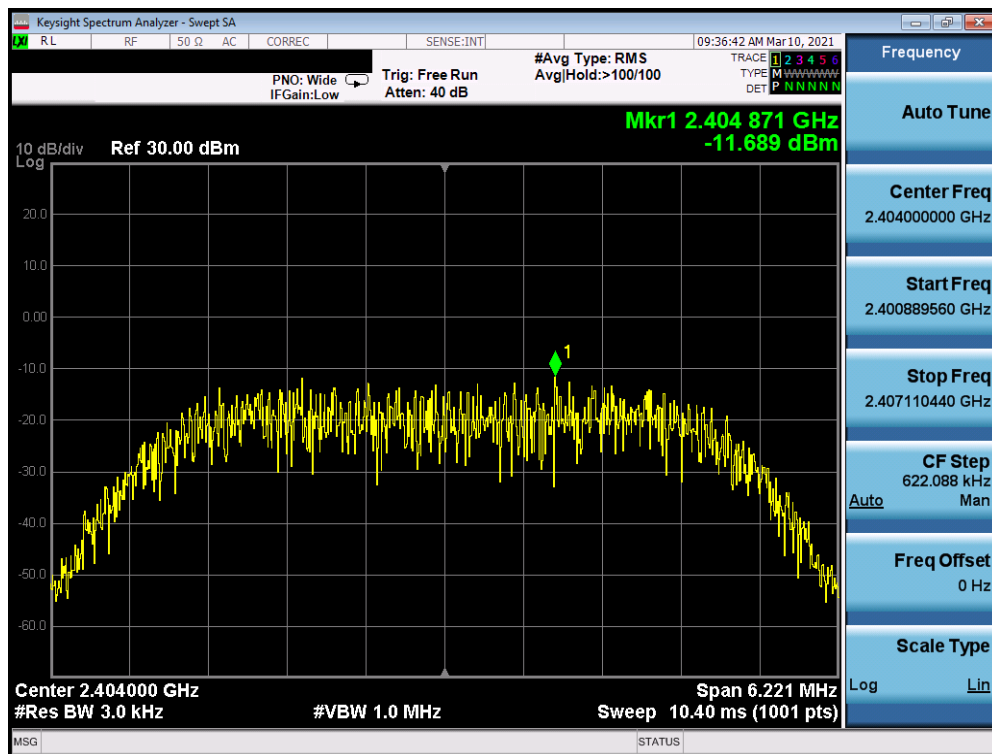
Plot 7-22. Power Spectral Density Plot Antenna 8 (Bluetooth (HDR8), 8Mbps, iPA – Ch. 1)
