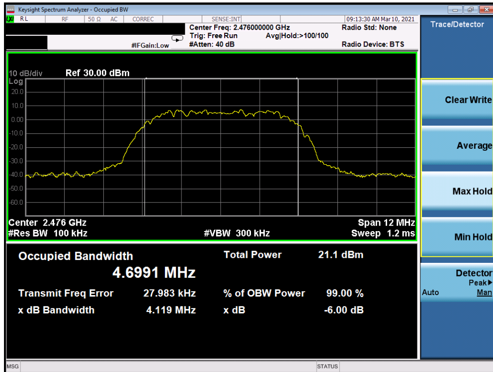
Plot 7-6. 6dB BW & 99% OBW Plot Antenna 8 (Bluetooth (HDR8), 8Mbps, ePA – Ch. 73)
