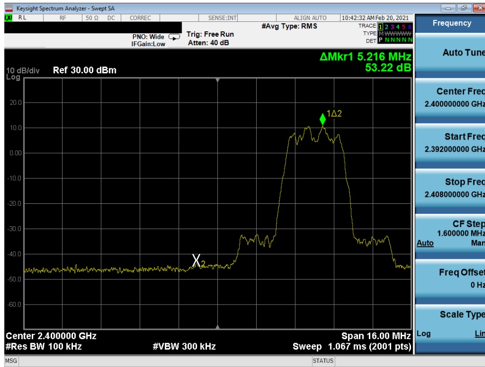
Plot 7-65. Band Edge Plot Antenna 7 (Bluetooth (HDR4), ePA – Ch. 1)
