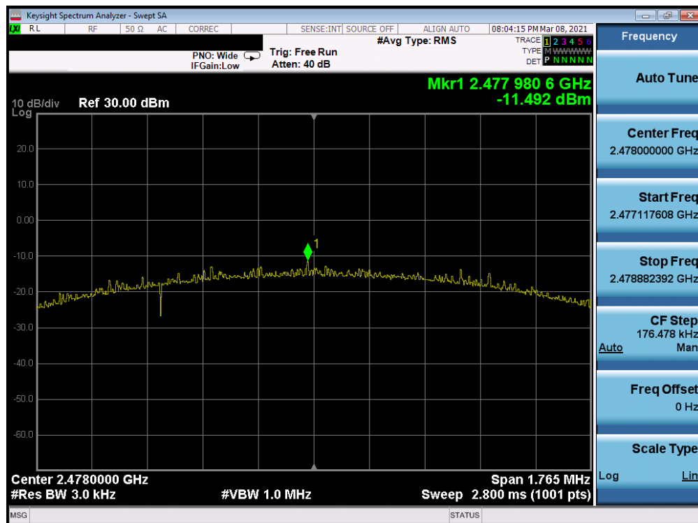
Plot 7-54. Power Spectral Density Plot Antenna 7 (Bluetooth (LE), 2Mbps, ePA – Ch. 38)
