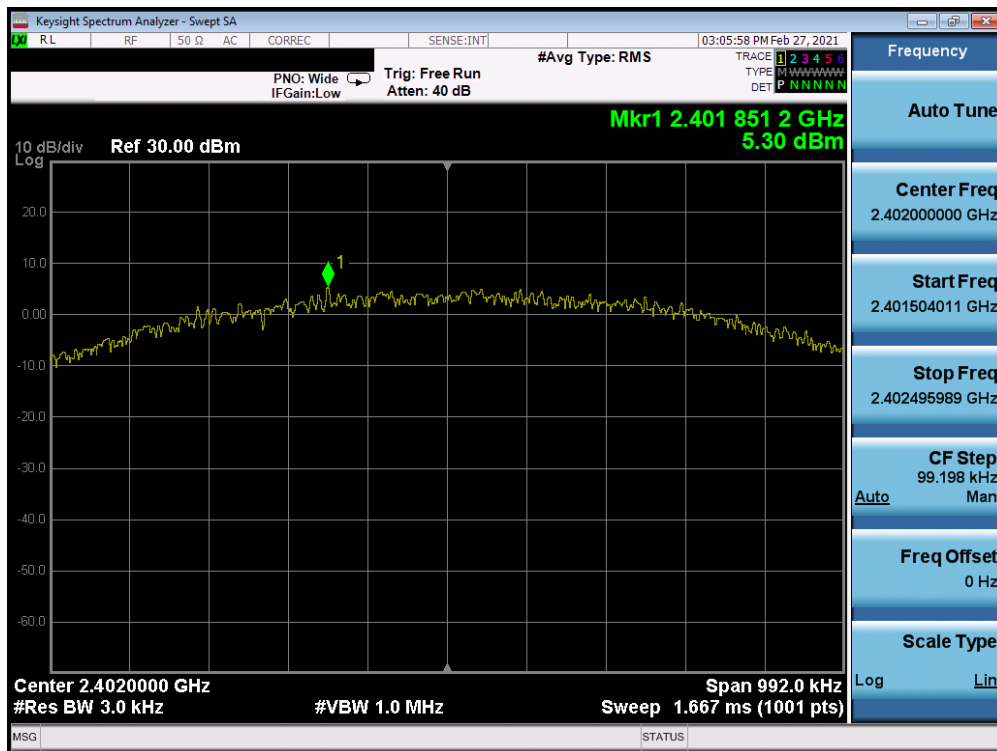
Plot 7-13. Power Spectral Density Plot Antenna 8 (Bluetooth (LE), 1Mbps, ePA – Ch. 0)
