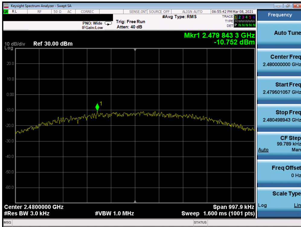
Plot 7-41. Power Spectral Density Plot Antenna 8 (Bluetooth (LE), 1Mbps, ePA – Ch. 39)
