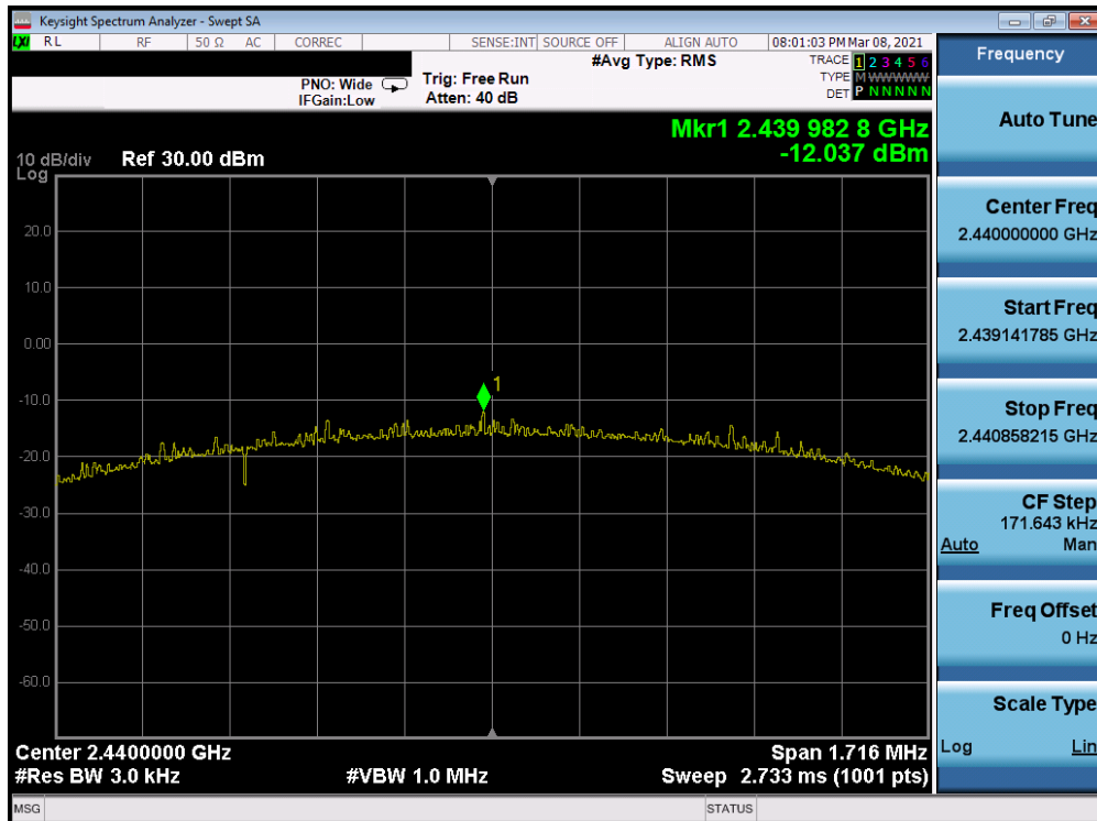
Plot 7-52. Power Spectral Density Plot Antenna 7 (Bluetooth (LE), 2Mbps, ePA – Ch. 19)
