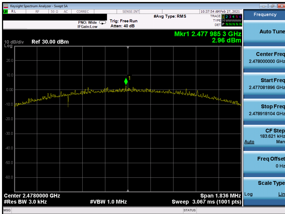
Plot 7-33. Power Spectral Density Plot Antenna 7 (Bluetooth (LE), 2Mbps, ePA – Ch. 38)
