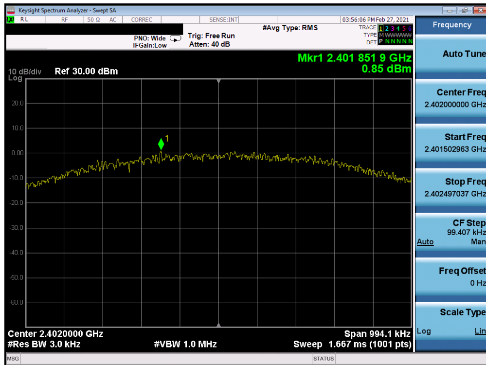
Plot 7-28. Power Spectral Density Plot Antenna 7 (Bluetooth (LE), 1Mbps, iPA – Ch. 0)
