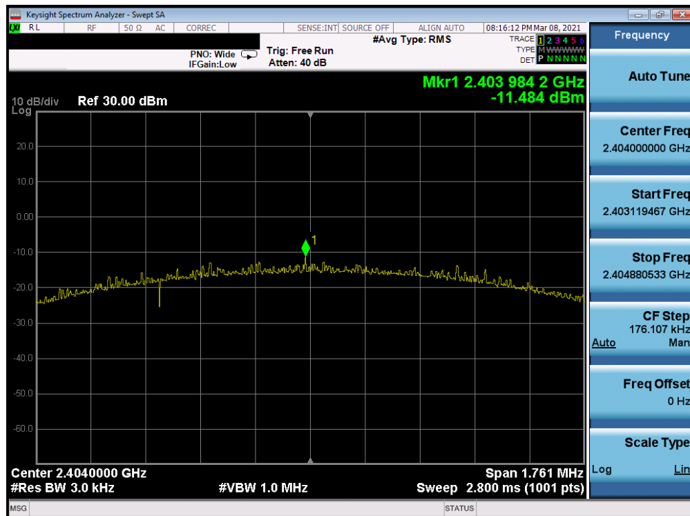
Plot 7-56. Power Spectral Density Plot Antenna 7 (Bluetooth (LE), 2Mbps, iPA – Ch. 1)
