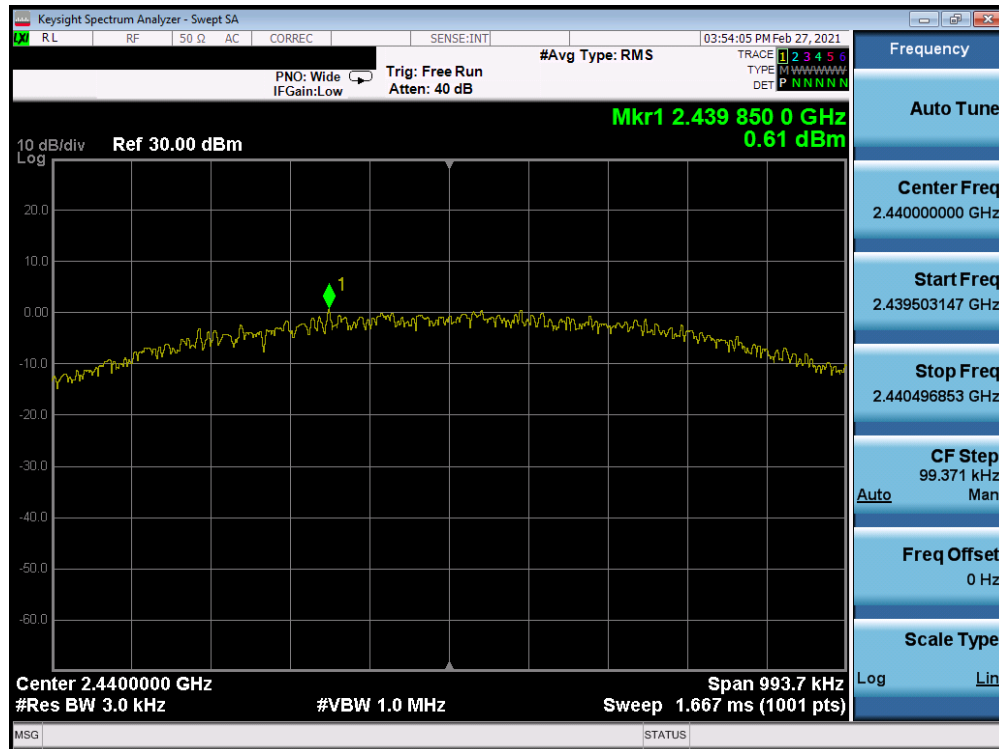
Plot 7-29. Power Spectral Density Plot Antenna 7 (Bluetooth (LE), 1Mbps, iPA – Ch. 19)
