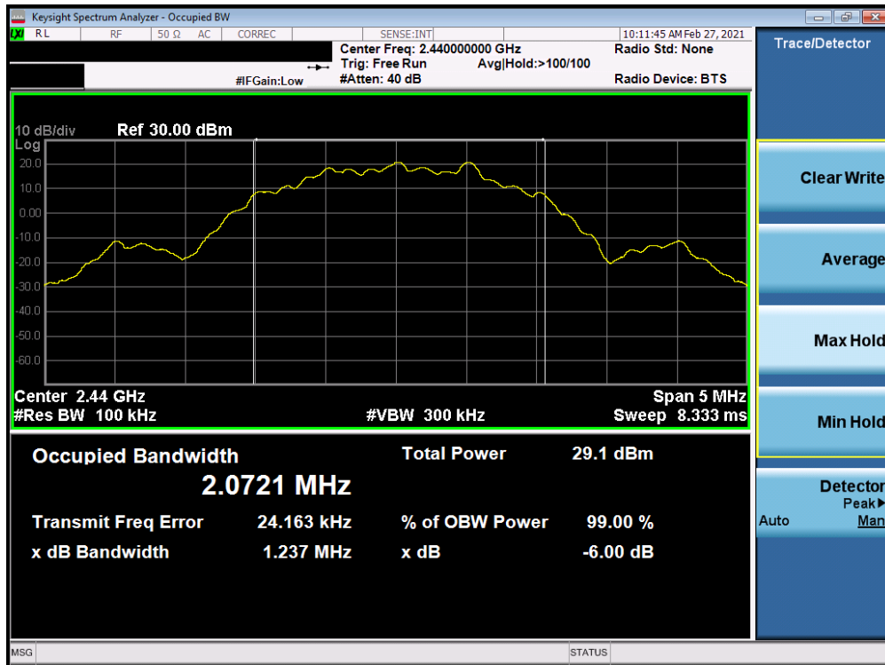
Plot 7-5. 6dB BW & 99% OBW Plot Antenna 8 (Bluetooth (LE), 2Mbps, ePA – Ch. 19)
