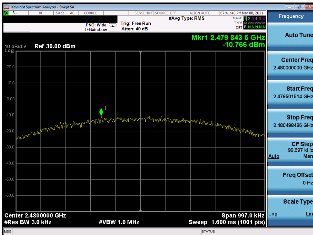
Plot 7-48. Power Spectral Density Plot Antenna 7 (Bluetooth (LE), 1Mbps, iPA – Ch. 39)
