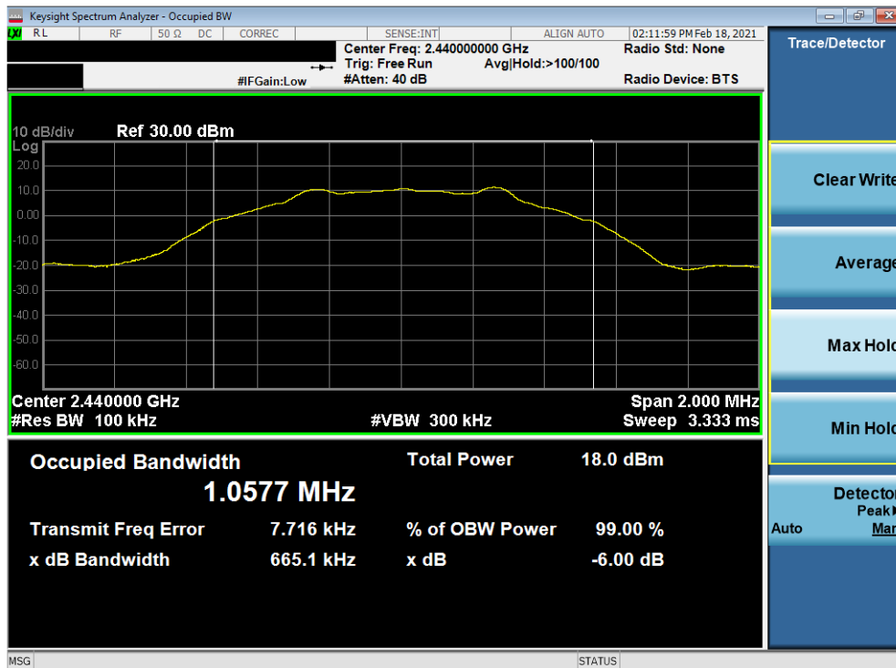
Plot 7-2. 6dB BW & 99% OBW Plot Antenna 8 (Bluetooth (LE), 1Mbps, ePA – Ch. 19)
