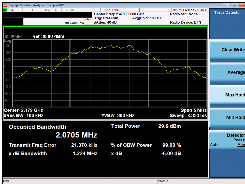
Plot 7-12. 6dB BW & 99% OBW Antenna 7 (Bluetooth (LE), 2Mbps, ePA – Ch. 38)
