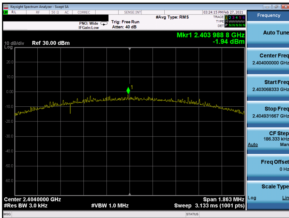
Plot 7-22. Power Spectral Density Plot Antenna 8 (Bluetooth (LE), 2Mbps, iPA – Ch. 1)
