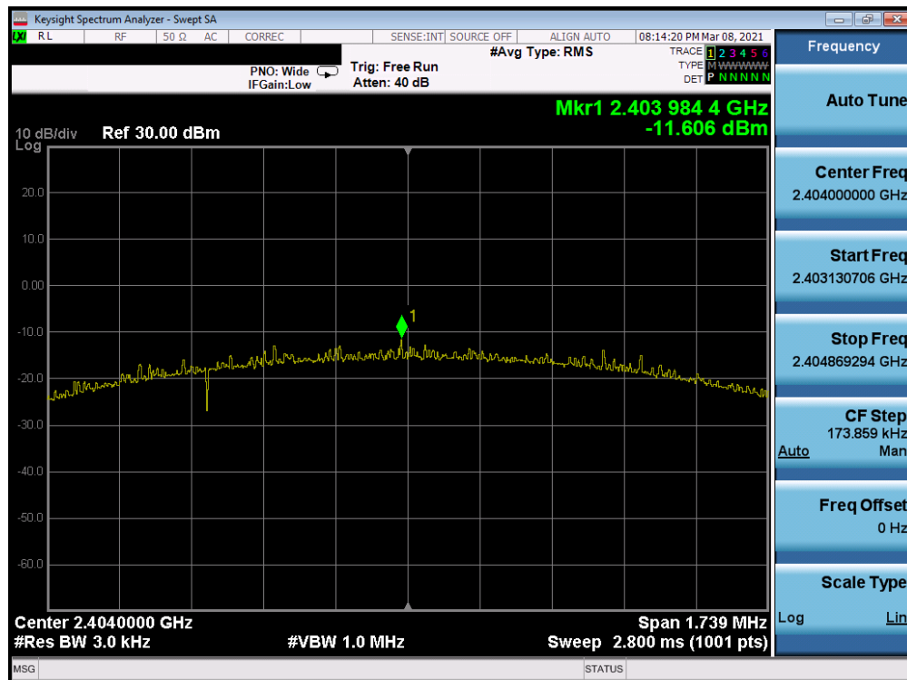
Plot 7-55. Power Spectral Density Plot Antenna 8 (Bluetooth (LE), 2Mbps, iPA – Ch. 1)
