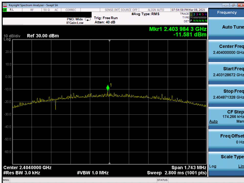
Plot 7-49. Power Spectral Density Plot Antenna 8 (Bluetooth (LE), 2Mbps, ePA – Ch. 1)
