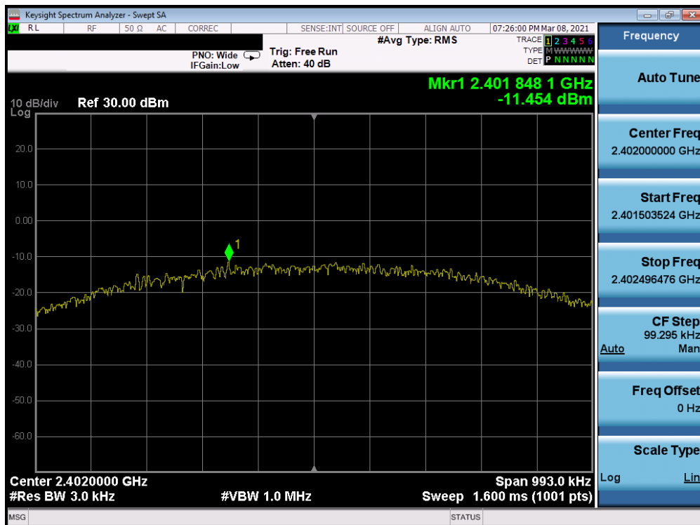
Plot 7-44. Power Spectral Density Plot Antenna 7 (Bluetooth (LE), 1Mbps, iPA – Ch. 0)
