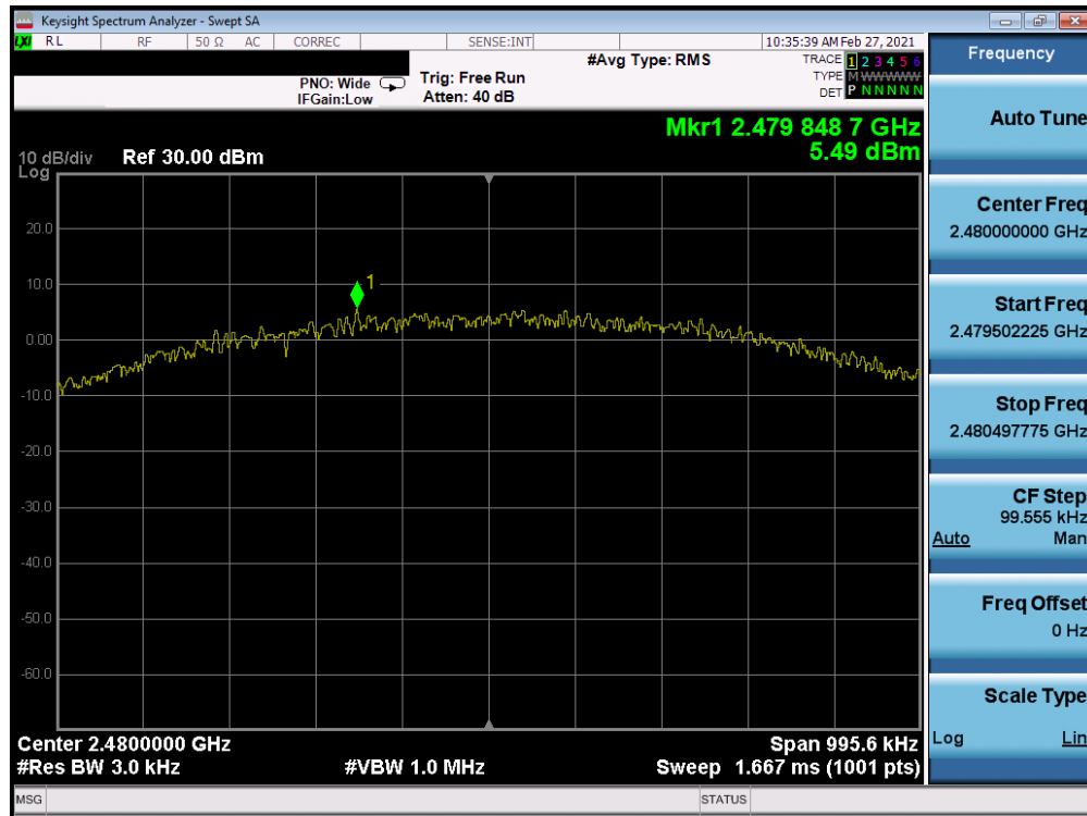
Plot 7-27. Power Spectral Density Plot Antenna 7 (Bluetooth (LE), 1Mbps, ePA – Ch. 39)
