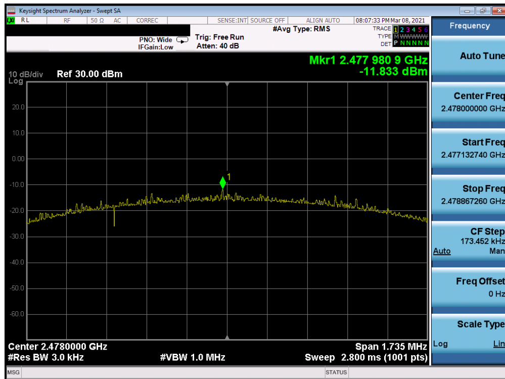
Plot 7-53. Power Spectral Density Plot Antenna 8 (Bluetooth (LE), 2Mbps, ePA – Ch. 38)
