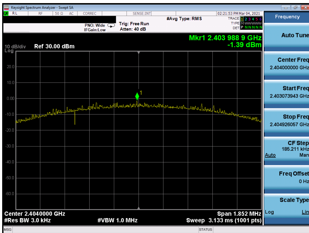
Plot 7-34. Power Spectral Density Plot Antenna 7 (Bluetooth (LE), 2Mbps, iPA – Ch. 1)
