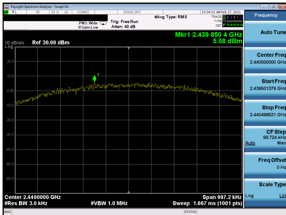
Plot 7-26. Power Spectral Density Plot Antenna 7 (Bluetooth (LE), 1Mbps, ePA – Ch. 19)
