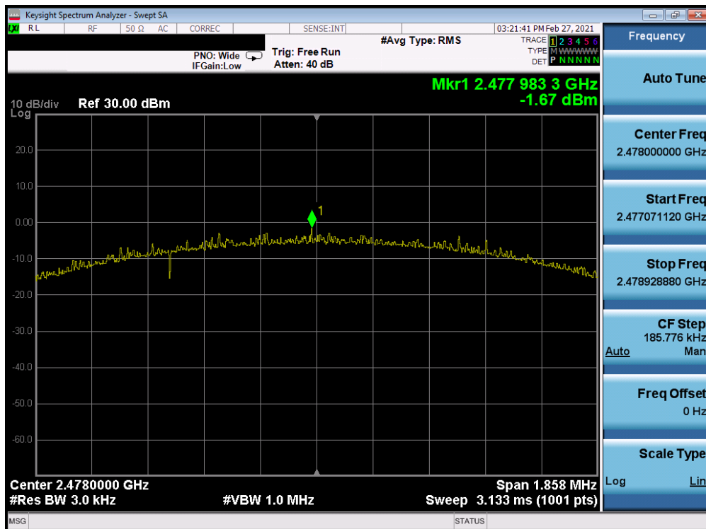
Plot 7-24. Power Spectral Density Plot Antenna 8 (Bluetooth (LE), 2Mbps, iPA – Ch. 38)
