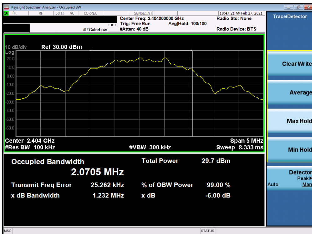
Plot 7-10. 6dB BW & 99% OBW Plot Antenna 7 (Bluetooth (LE), 2Mbps, ePA – Ch. 1)
