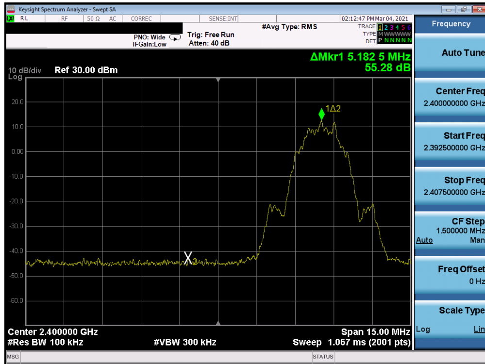
Plot 7-67. Band Edge Plot Antenna 7 (Bluetooth (LE), 2Mbps, ePA – Ch. 1)
