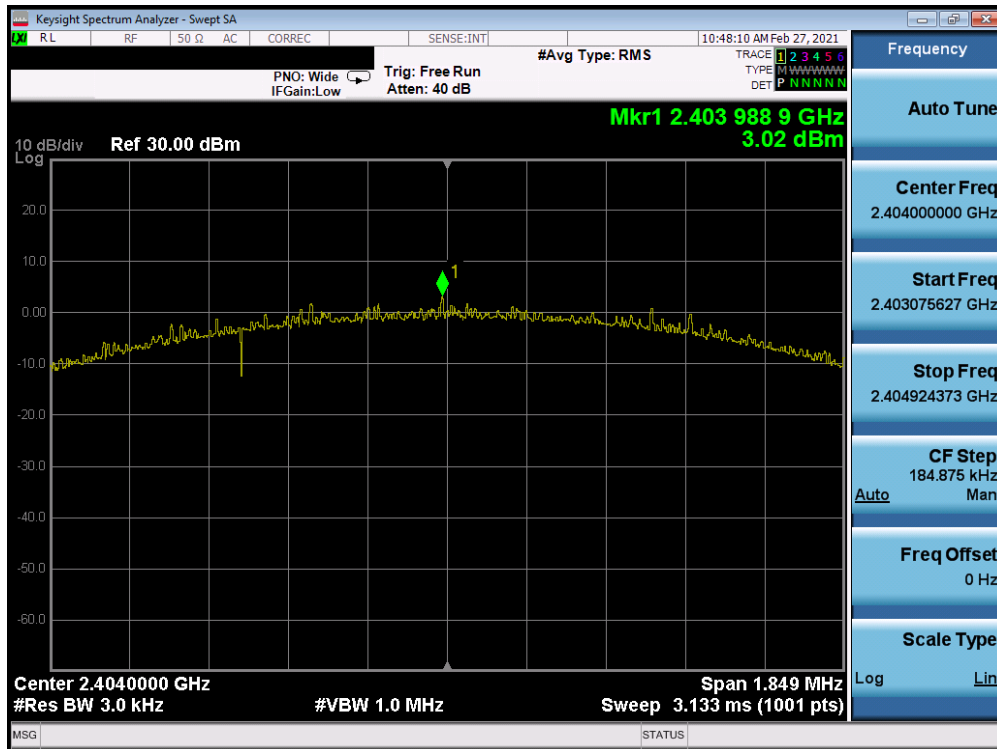
Plot 7-31. Power Spectral Density Plot Antenna 7 (Bluetooth (LE), 2Mbps, ePA – Ch. 1)
