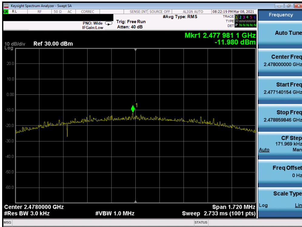
Plot 7-59. Power Spectral Density Plot Antenna 8 (Bluetooth (LE), 2Mbps, iPA – Ch. 38)
