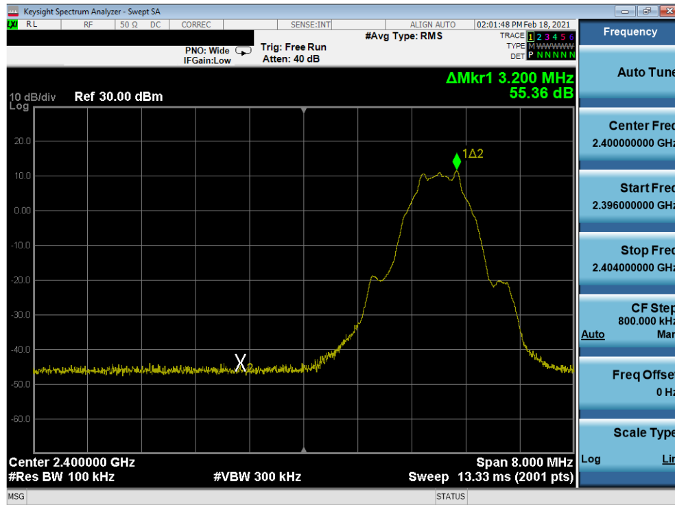
Plot 7-61. Band Edge Plot Antenna 8 (Bluetooth (LE), 1Mbps, ePA – Ch. 0)
