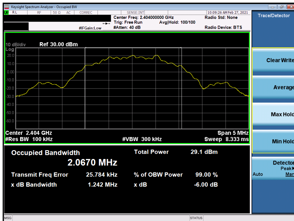
Plot 7-4. 6dB BW & 99% OBW Plot Antenna 8 (Bluetooth (LE), 2Mbps, ePA – Ch. 1)
