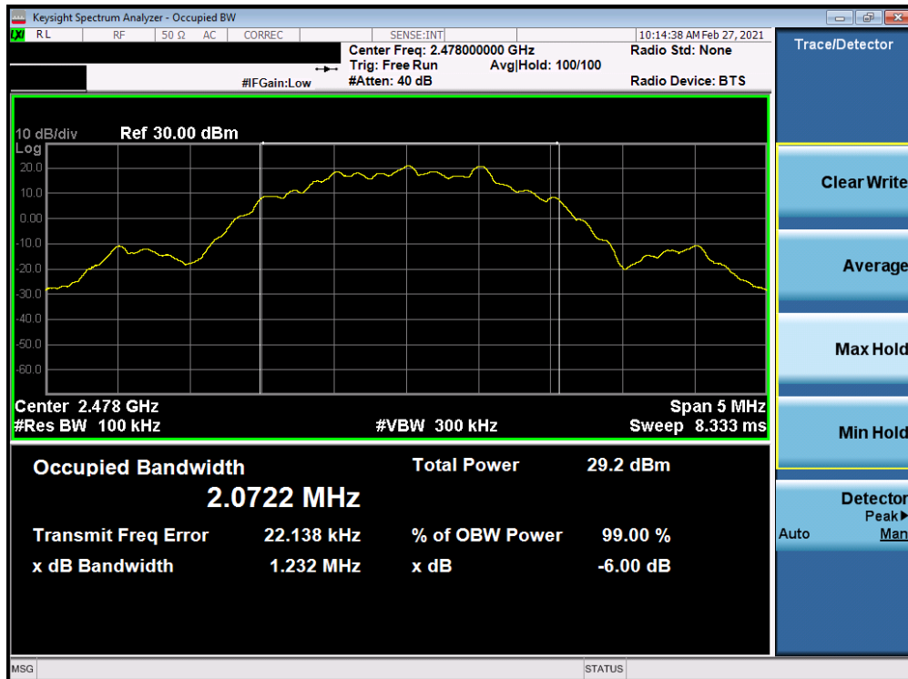
Plot 7-6. 6dB BW & 99% OBW Plot Antenna 8 (Bluetooth (LE), 2Mbps, ePA – Ch. 38)
