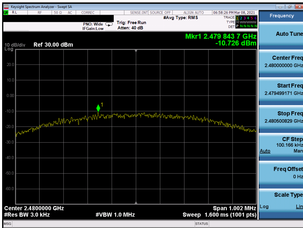
Plot 7-42. Power Spectral Density Plot Antenna 7 (Bluetooth (LE), 1Mbps, ePA – Ch. 39)
