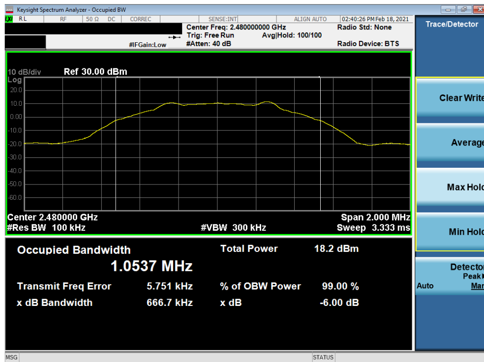
Plot 7-3. 6dB BW & 99% OBW Plot Antenna 8 (Bluetooth (LE), 1Mbps, ePA – Ch. 39)
