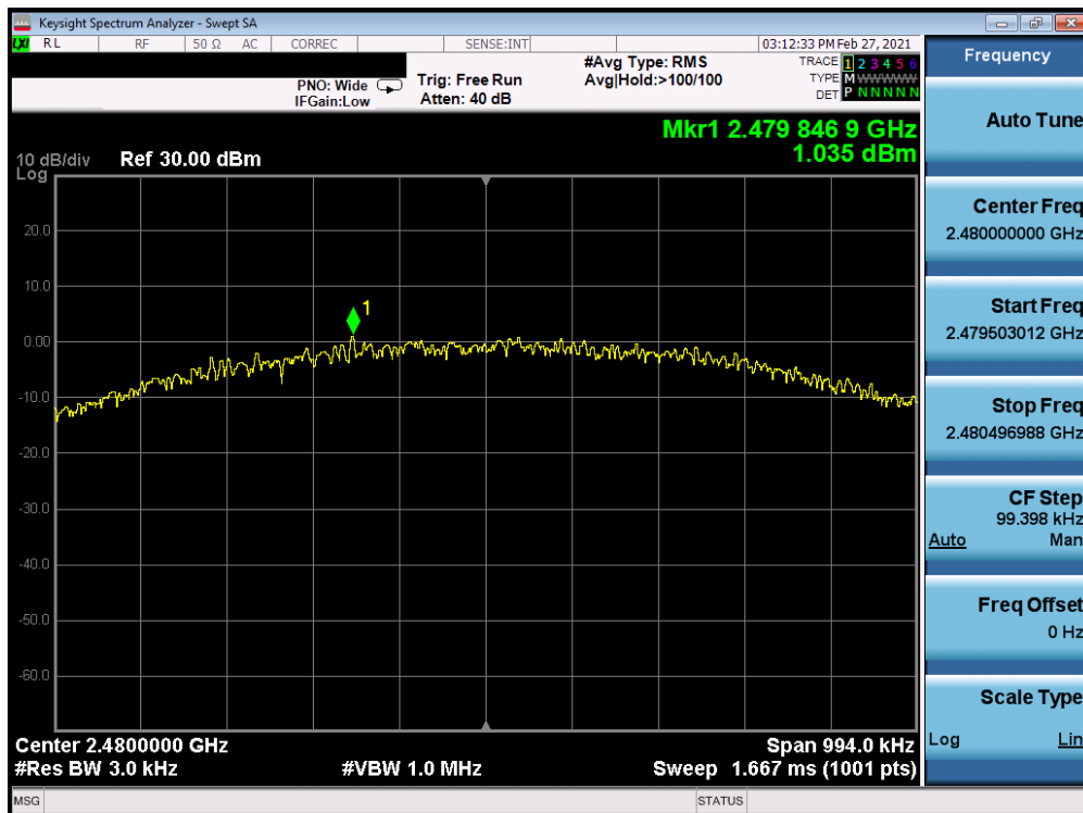
Plot 7-18. Power Spectral Density Plot Antenna 8 (Bluetooth (LE), 1Mbps, iPA – Ch. 39)
