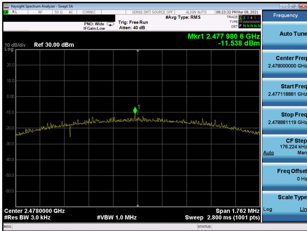
Plot 7-60. Power Spectral Density Plot Antenna 7 (Bluetooth (LE), 2Mbps, iPA – Ch. 38)
