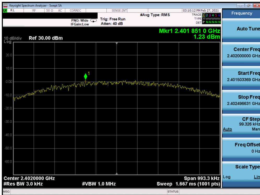
Plot 7-16. Power Spectral Density Plot Antenna 8 (Bluetooth (LE), 1Mbps, iPA – Ch. 0)
