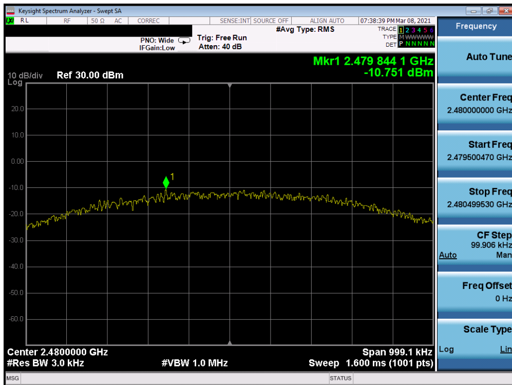
Plot 7-47. Power Spectral Density Plot Antenna 8 (Bluetooth (LE), 1Mbps, iPA – Ch. 39)
