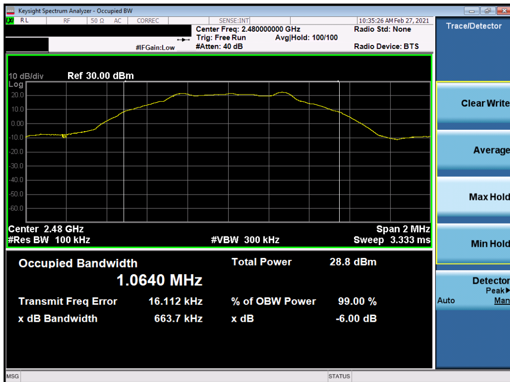
Plot 7-9. 6dB BW & 99% OBW Plot Antenna 7 (Bluetooth (LE), 1Mbps, ePA – Ch. 39)
