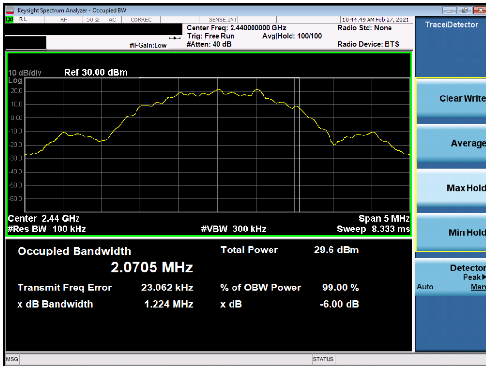
Plot 7-11. 6dB BW & 99% OBW Plot Antenna 7 (Bluetooth (LE), 2Mbps, ePA – Ch. 19)
