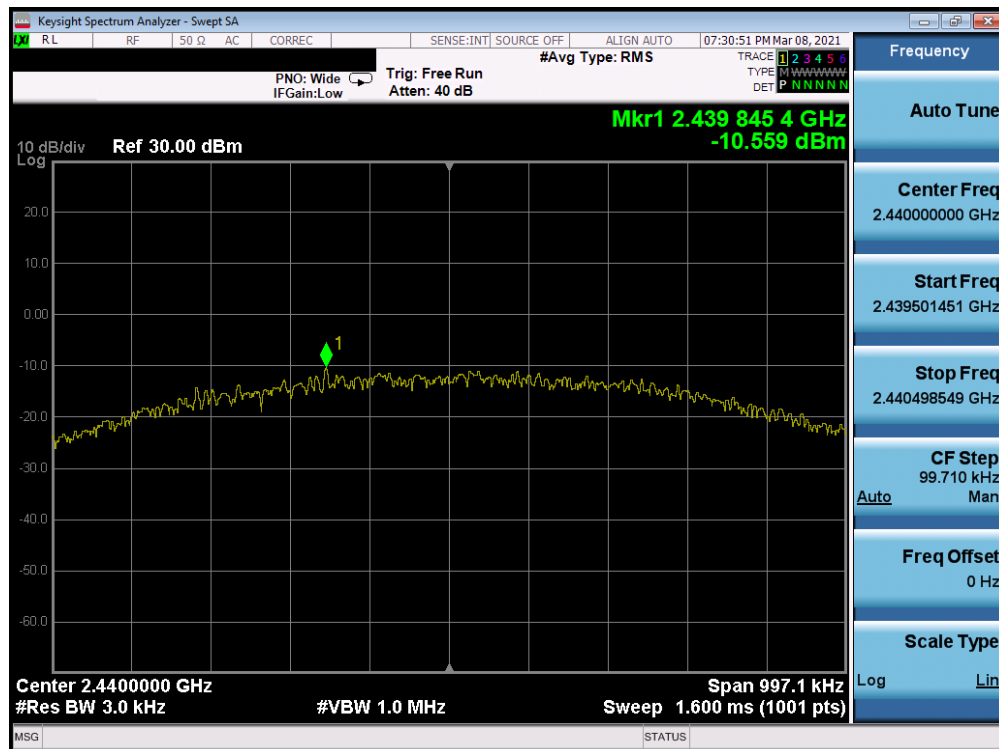
Plot 7-45. Power Spectral Density Plot Antenna 8 (Bluetooth (LE), 1Mbps, iPA – Ch. 19)
