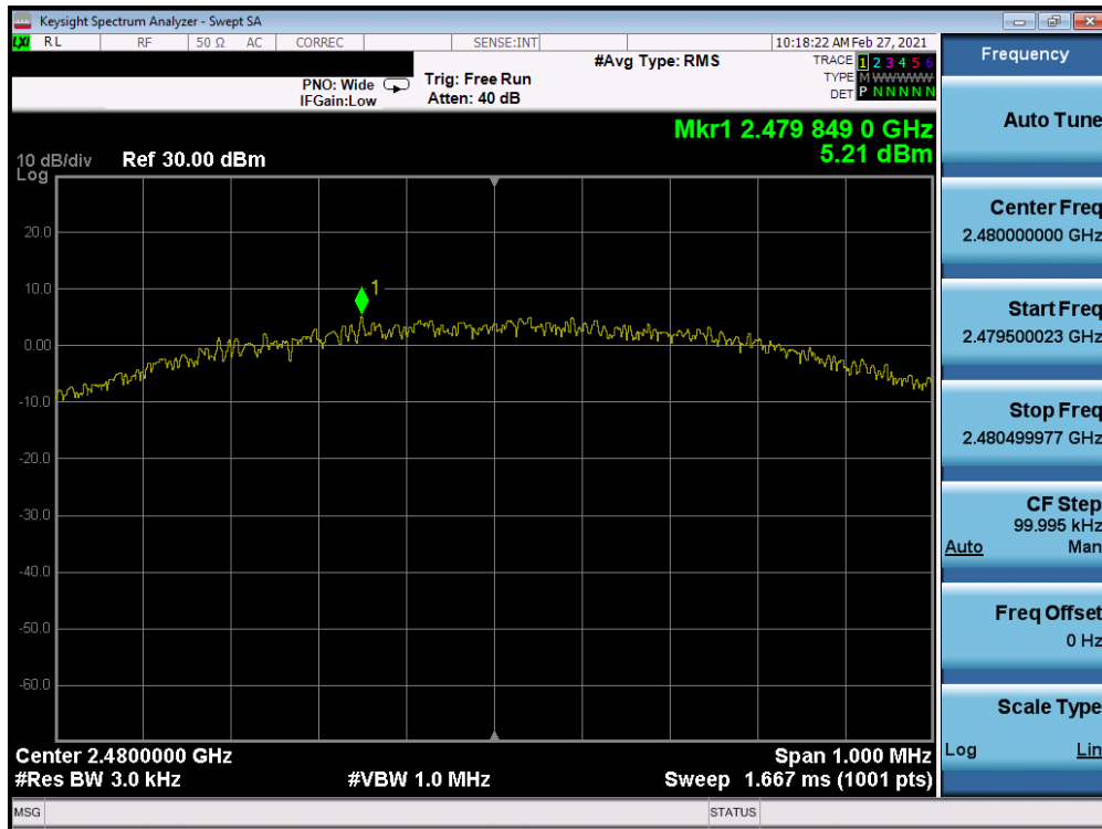
Plot 7-15. Power Spectral Density Plot Antenna 8 (Bluetooth (LE), 1Mbps, ePA – Ch. 39)
