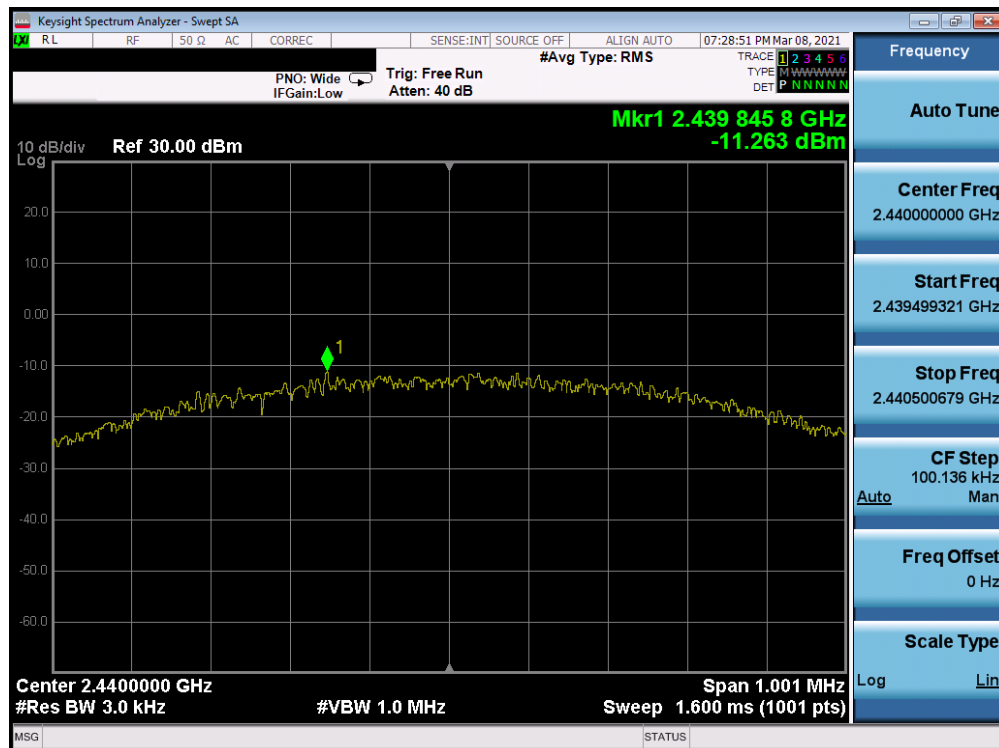
Plot 7-46. Power Spectral Density Plot Antenna 7 (Bluetooth (LE), 1Mbps, iPA – Ch. 19)
