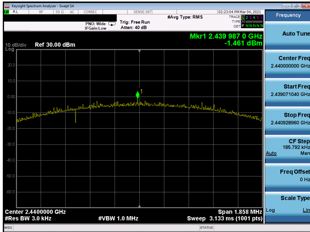
Plot 7-35. Power Spectral Density Plot Antenna 7 (Bluetooth (LE), 2Mbps, iPA – Ch. 19)
