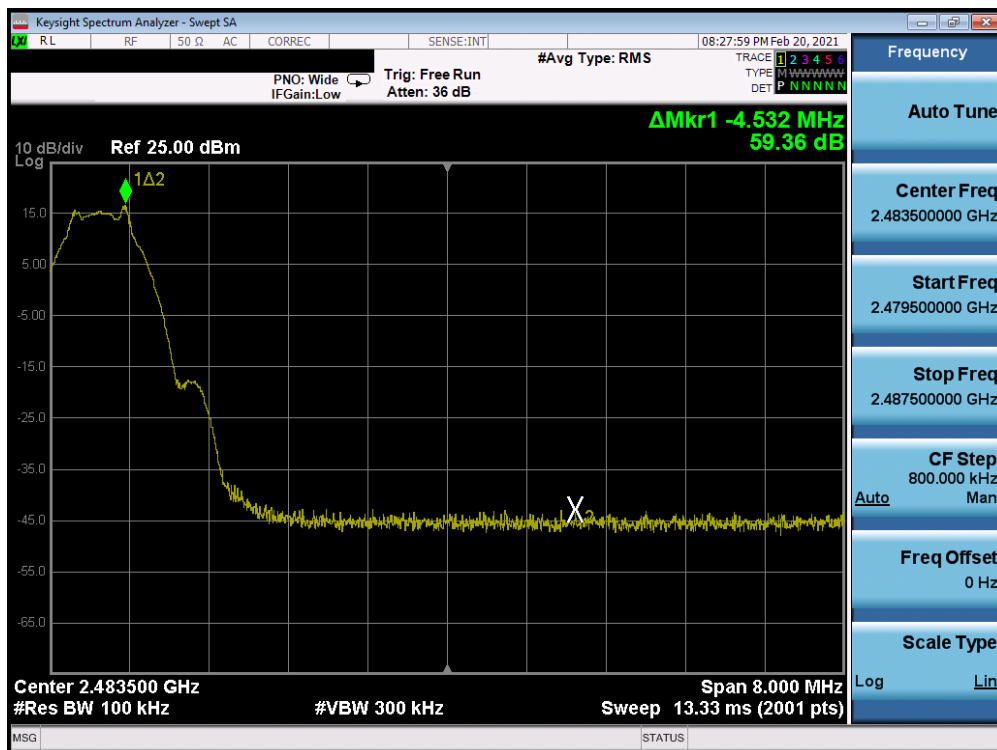
Plot 7-66. Band Edge Plot Antenna 7 (Bluetooth (LE), 1Mbps, ePA – Ch. 39)
