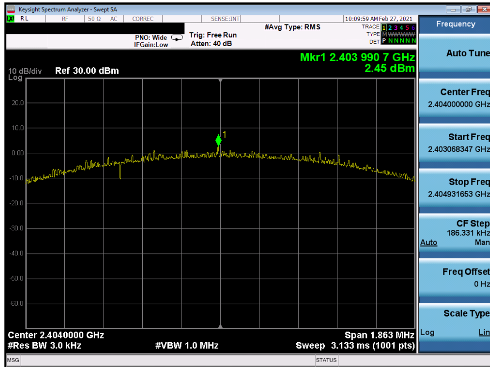
Plot 7-19. Power Spectral Density Plot Antenna 8 (Bluetooth (LE), 2Mbps, ePA – Ch. 1)
