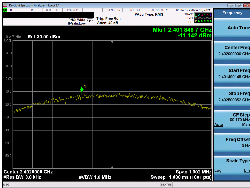
Plot 7-37. Power Spectral Density Plot Antenna 8 (Bluetooth (LE), 1Mbps, ePA – Ch. 0)
