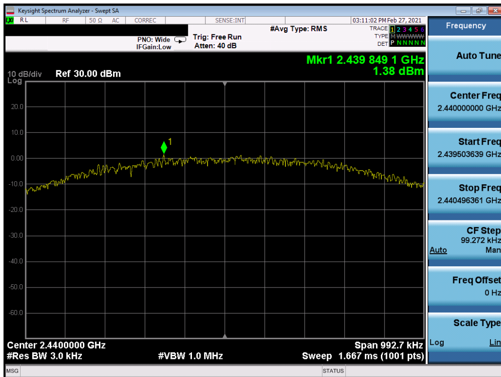
Plot 7-17. Power Spectral Density Plot Antenna 8 (Bluetooth (LE), 1Mbps, iPA – Ch. 19)
