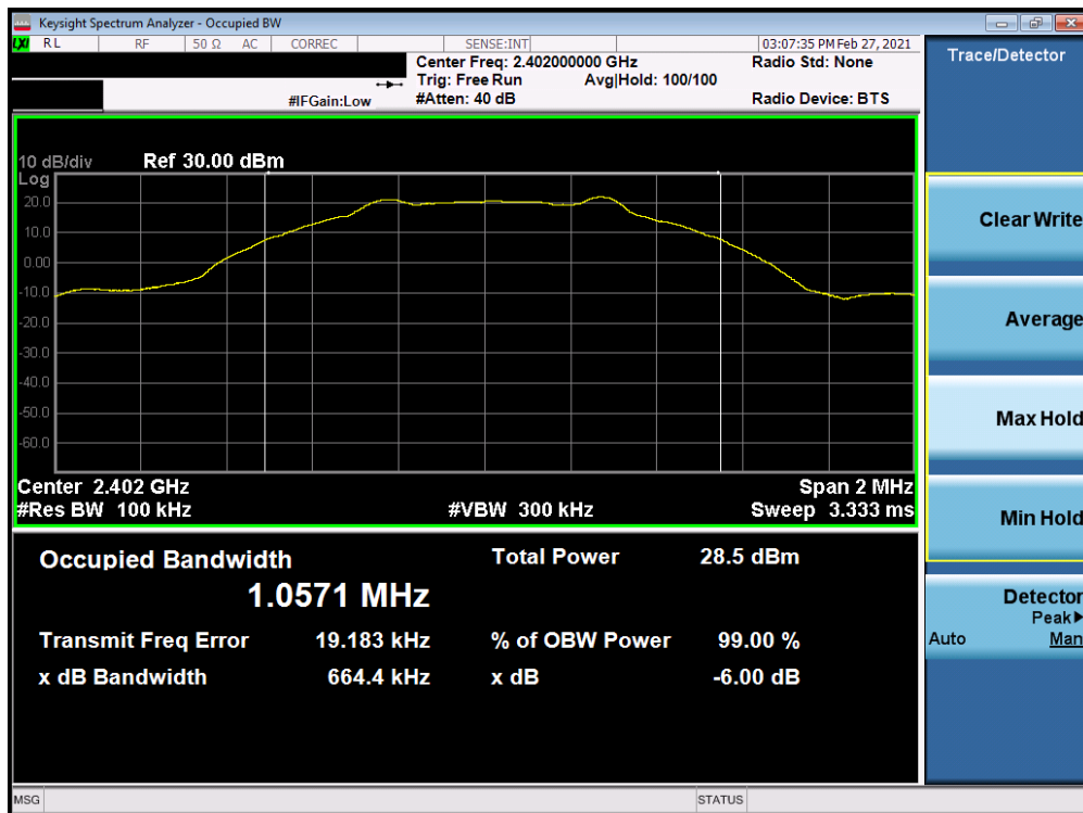
Plot 7-1. 6dB BW & 99% OBW Plot Antenna 8 (Bluetooth (LE), 1Mbps, ePA – Ch. 0)
