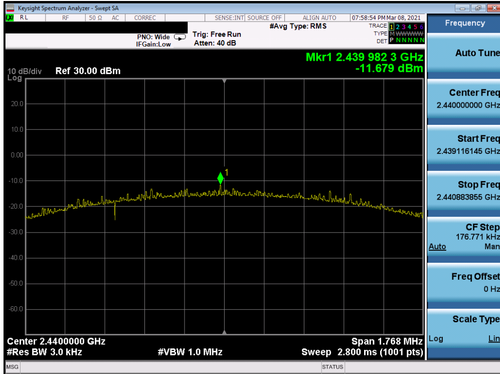
Plot 7-51. Power Spectral Density Plot Antenna 8 (Bluetooth (LE), 2Mbps, ePA – Ch. 19)
