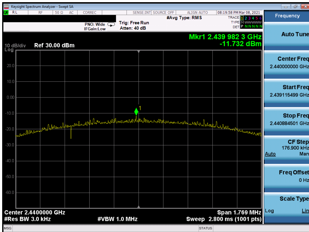
Plot 7-57. Power Spectral Density Plot Antenna 8 (Bluetooth (LE), 2Mbps, iPA – Ch. 19)
