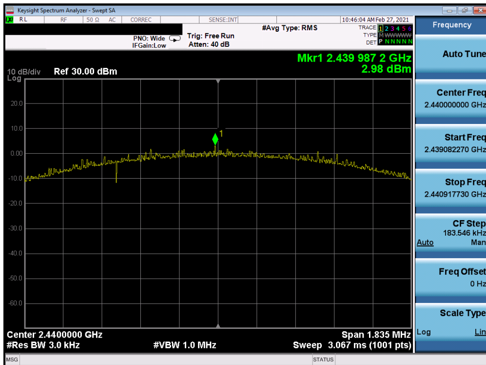
Plot 7-32. Power Spectral Density Plot Antenna 7 (Bluetooth (LE), 2Mbps, ePA – Ch. 19)
