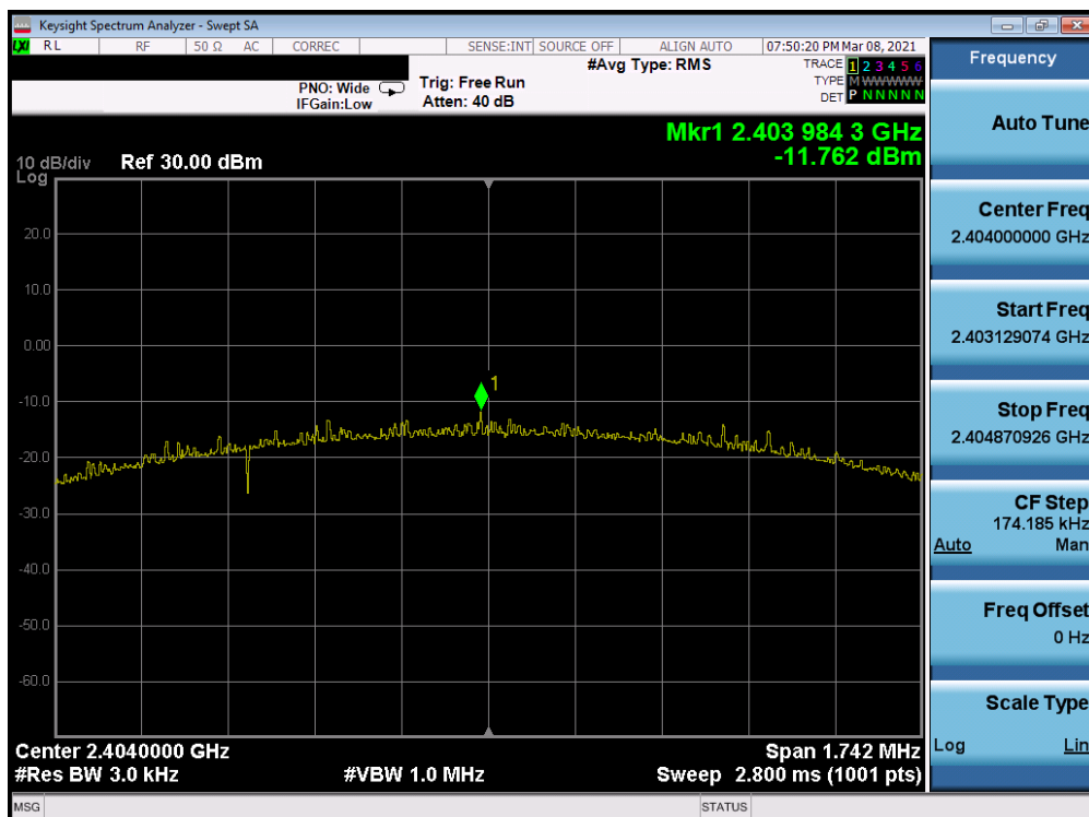
Plot 7-50. Power Spectral Density Plot Antenna 7 (Bluetooth (LE), 2Mbps, ePA – Ch. 1)
