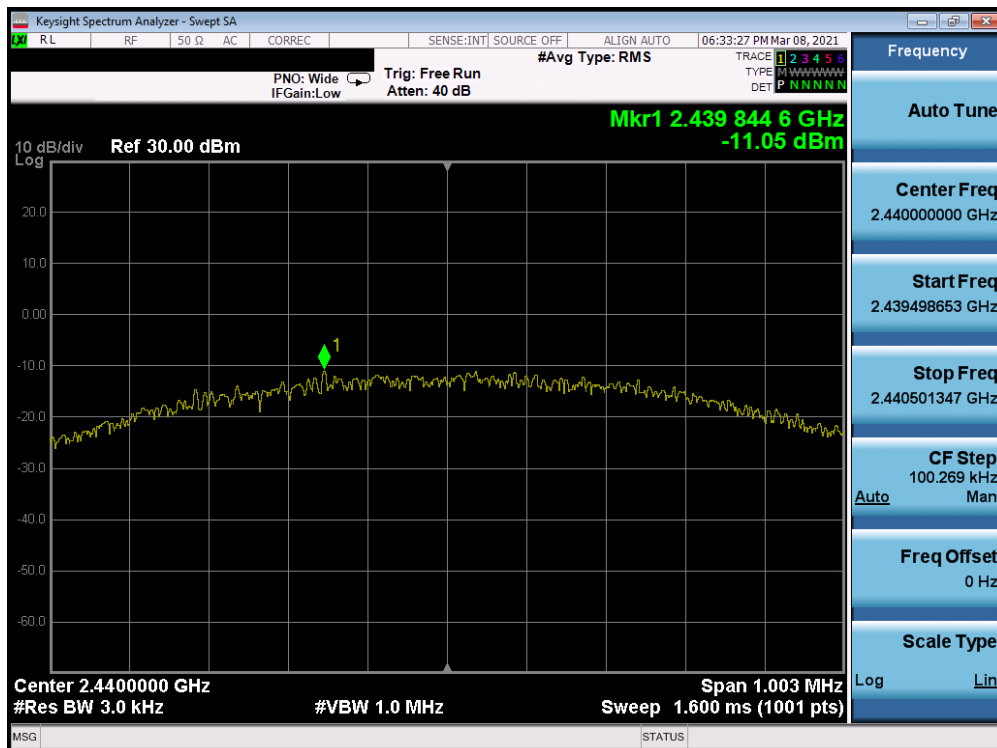
Plot 7-40. Power Spectral Density Plot Antenna 7 (Bluetooth (LE), 1Mbps, ePA – Ch. 19)
