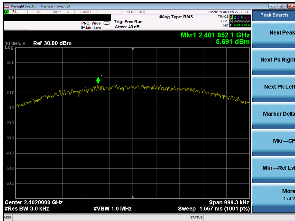
Plot 7-25. Power Spectral Density Plot Antenna 7 (Bluetooth (LE), 1Mbps, ePA – Ch. 0)
