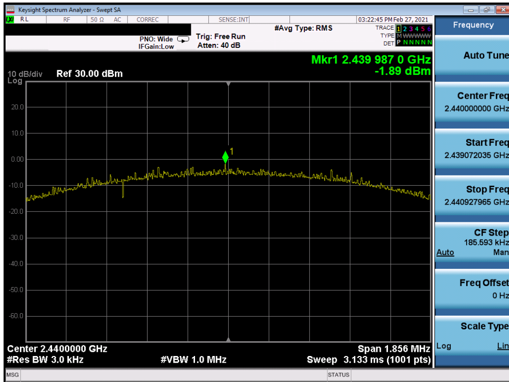
Plot 7-23. Power Spectral Density Plot Antenna 8 (Bluetooth (LE), 2Mbps, iPA – Ch. 19)
