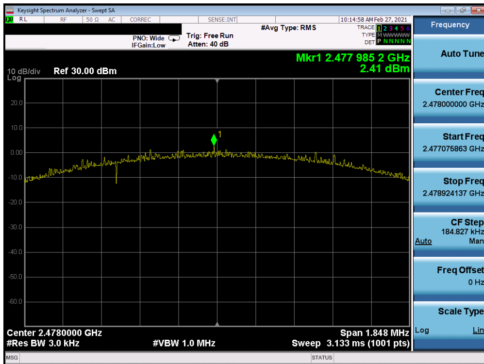
Plot 7-21. Power Spectral Density Plot Antenna 8 (Bluetooth (LE), 2Mbps, ePA – Ch. 38)
