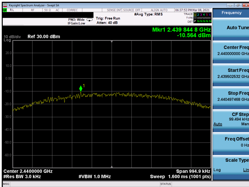
Plot 7-39. Power Spectral Density Plot Antenna 8 (Bluetooth (LE), 1Mbps, ePA – Ch. 19)
