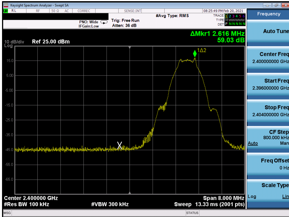
Plot 7-65. Band Edge Plot Antenna 7 (Bluetooth (LE), 1Mbps, ePA – Ch. 0)
