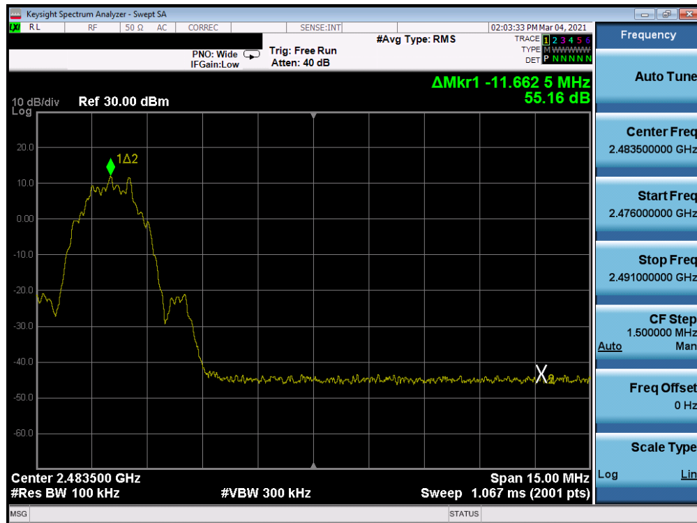
Plot 7-64. Band Edge Plot Antenna 8 (Bluetooth (LE), 2Mbps, ePA – Ch. 38)
