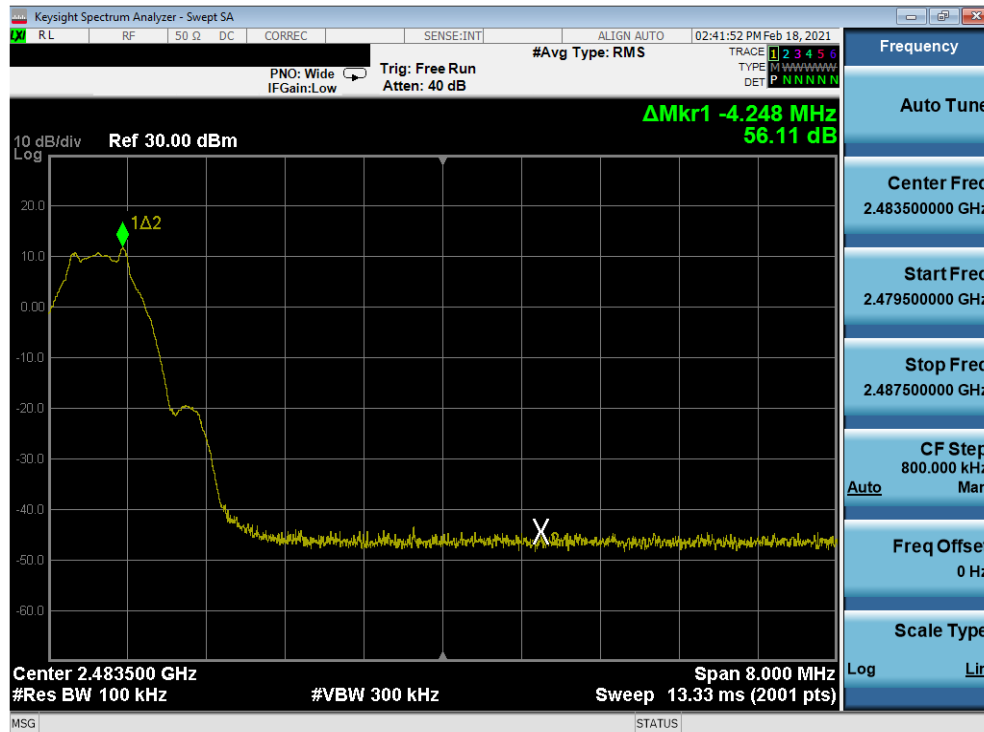
Plot 7-62. Band Edge Plot Antenna 8 (Bluetooth (LE), 1Mbps, ePA – Ch. 39)
