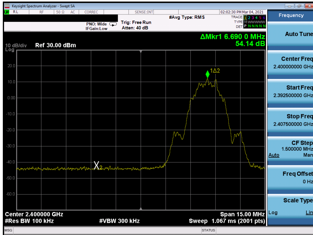
Plot 7-63. Band Edge Plot Antenna 8 (Bluetooth (LE), 2Mbps, ePA – Ch. 1)
