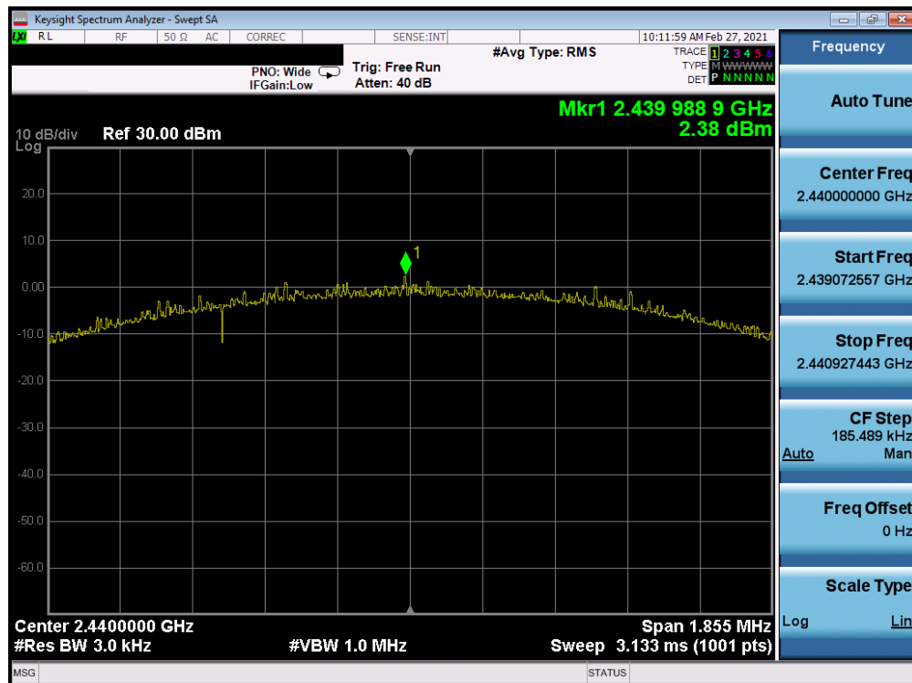
Plot 7-20. Power Spectral Density Plot Antenna 8 (Bluetooth (LE), 2Mbps, ePA – Ch. 19)
