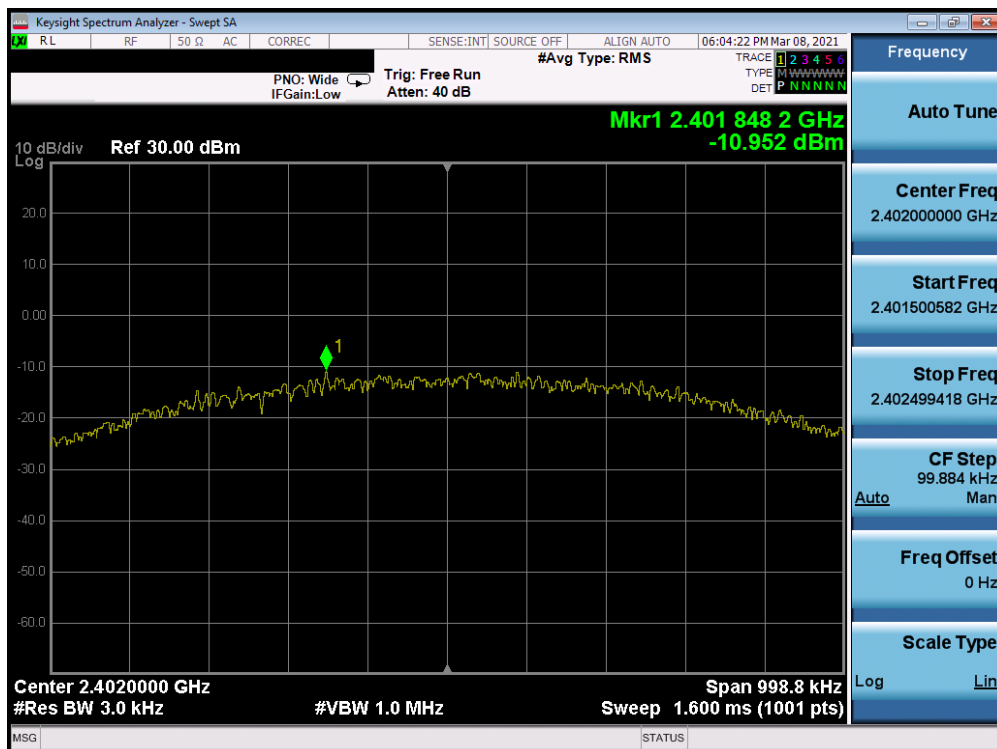
Plot 7-38. Power Spectral Density Plot Antenna 7 (Bluetooth (LE), 1Mbps, ePA – Ch. 0)
