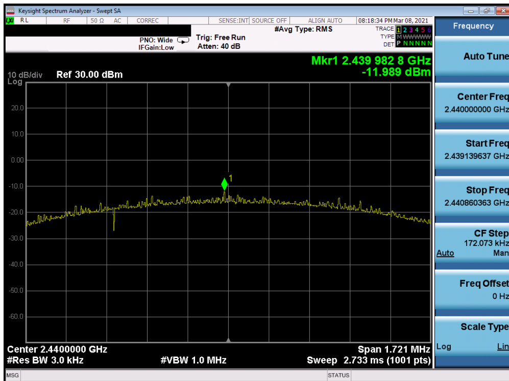
Plot 7-58. Power Spectral Density Plot Antenna 7 (Bluetooth (LE), 2Mbps, iPA – Ch. 19)
