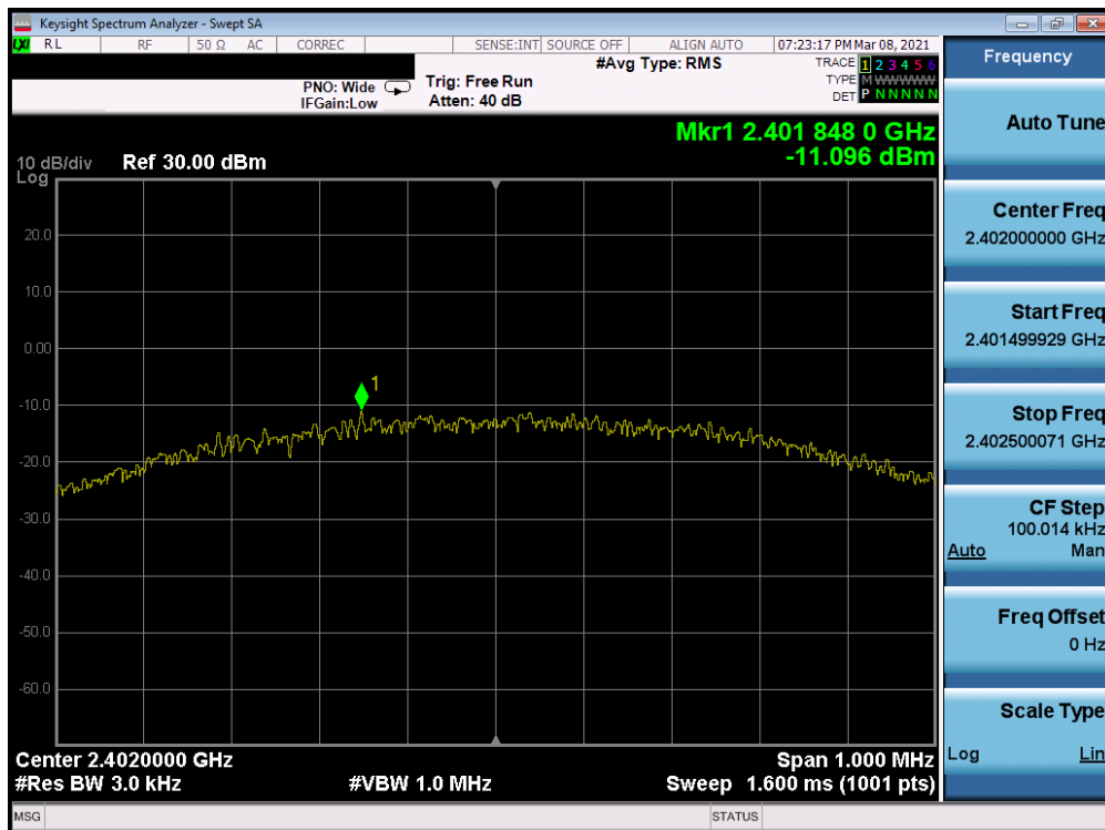
Plot 7-43. Power Spectral Density Plot Antenna 8 (Bluetooth (LE), 1Mbps, iPA – Ch. 0)
