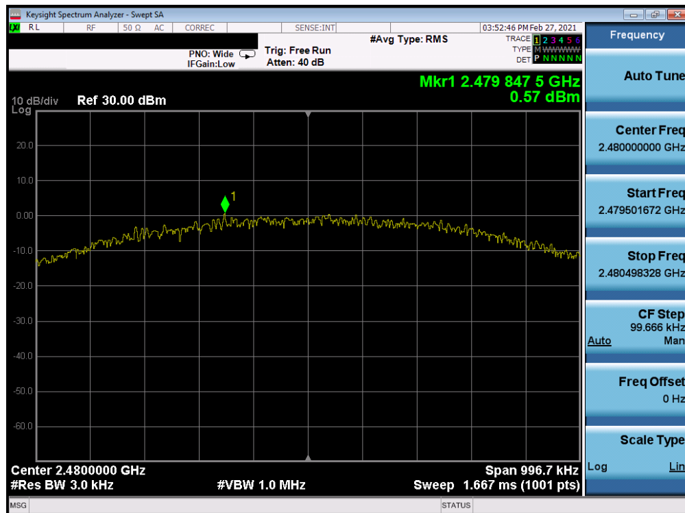
Plot 7-30. Power Spectral Density Plot Antenna 7 (Bluetooth (LE), 1Mbps, iPA – Ch. 39)
