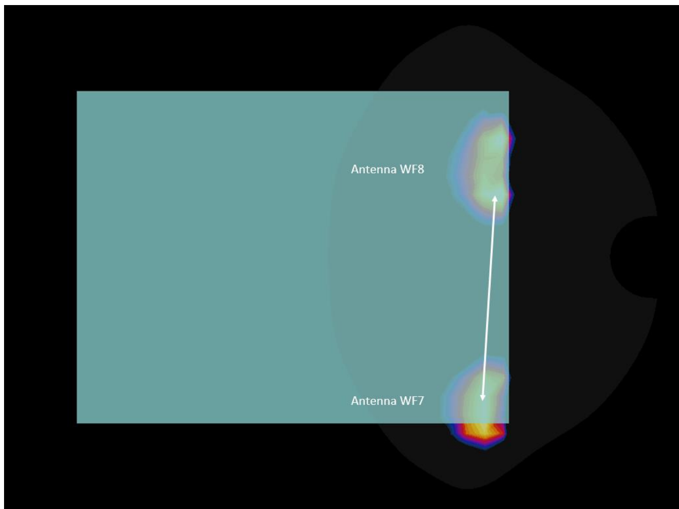
Figure 10-1 Backside Spatial Separation for Antenna WF8 and Antenna WF7
