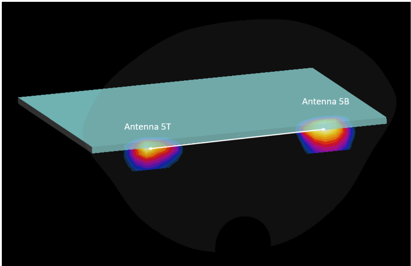
Figure 10-2 Right Edge Spatial Separation for Antenna 5T and Antenna 5B
