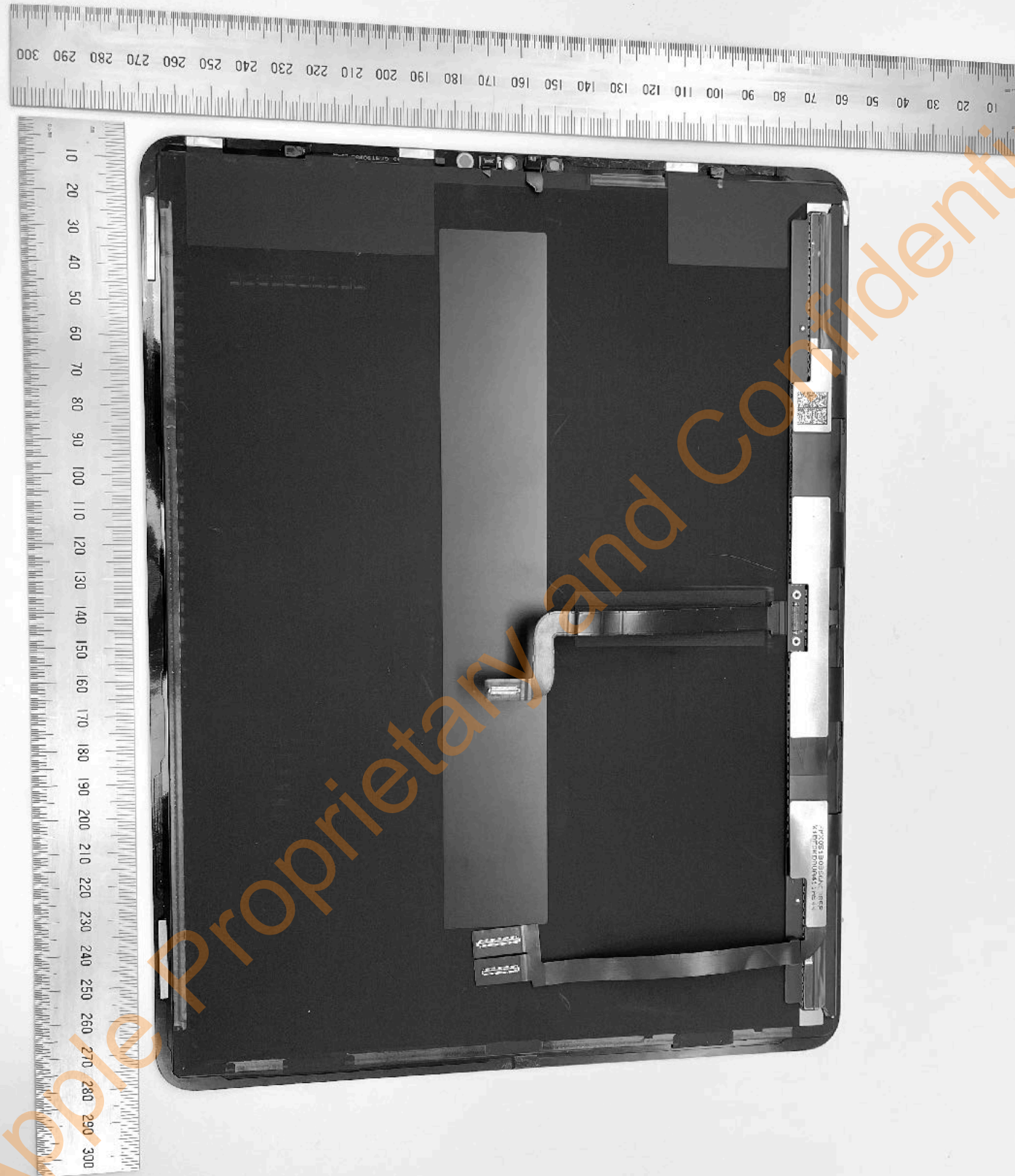
A2378 Display Panel - Back
