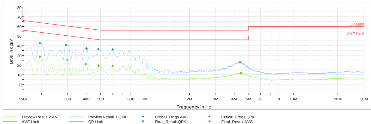
Plot 6-6. AC Line Conducted Plot (N, Charging Rate 10C, with AC/DC Adapter)
