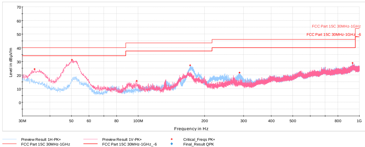
Plot 6-4. Radiated Spurious Emissions 30MHz-1GHz (Charging Rate 10C, with AC/DC Adapter)
