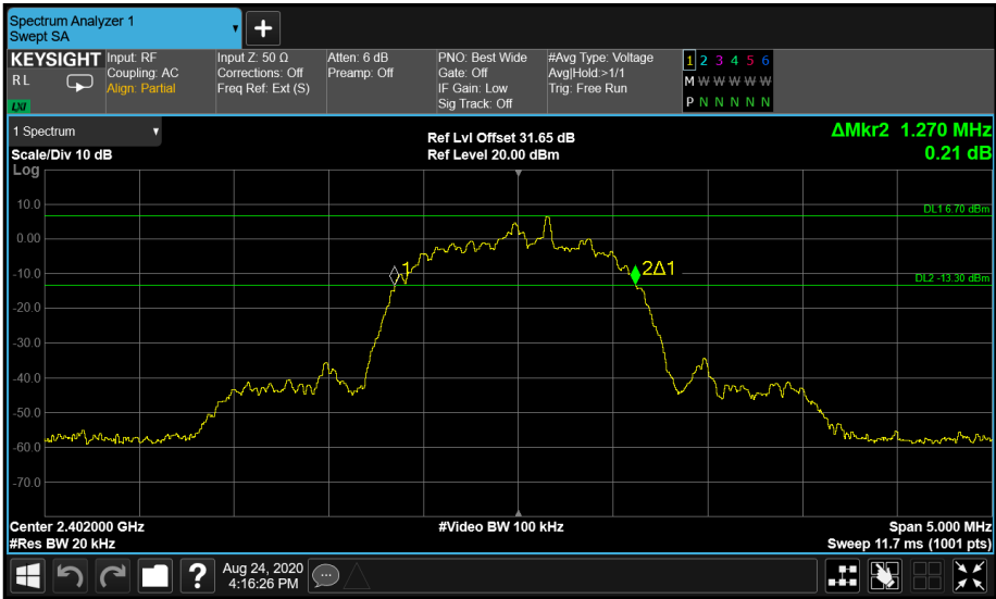
Figure 19 - Core 2 8DPSK 2402 MHz (CH0)
