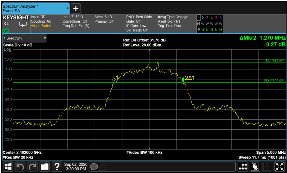
Figure 36 - Core 0 8DPSK 2402 MHz (CH0)
