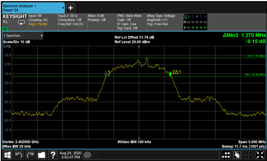
Figure 18 - Core 0 8DPSK 2402 MHz (CH0)
