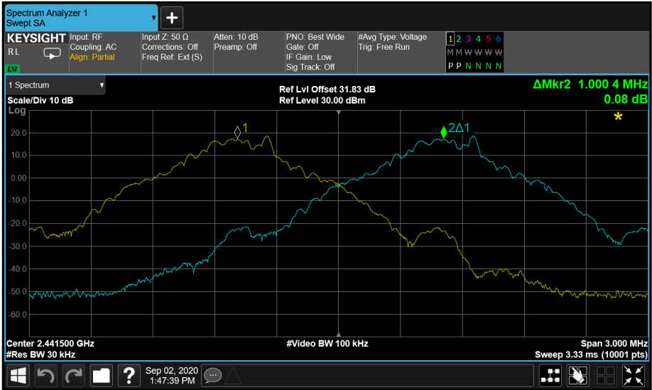
Figure 2- GFSK - 2441 MHz (CH 39)
