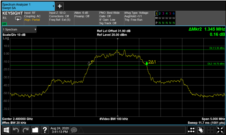
Figure 16 - Core 0 \pi/4 DQPSK 2480 MHz (CH78)
