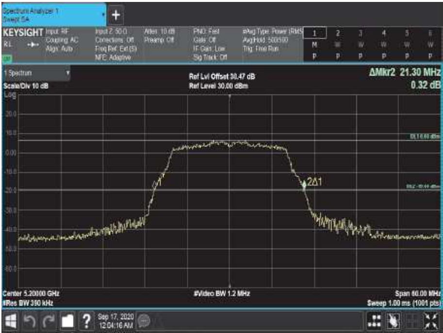
Figure 3 - 5200 MHz - 26 dB Emission Bandwidth h
