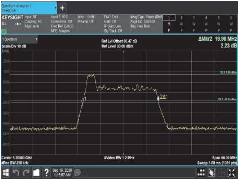
Figure 111 - 5200 MHz - 26 dB Emission Bandwidth
