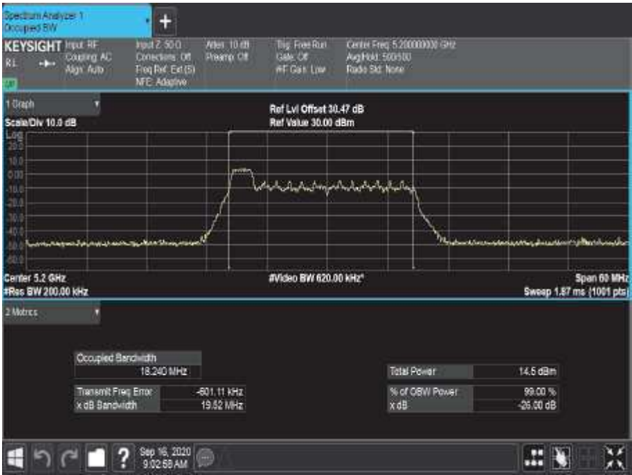
Figure 112 - 5200 MHz - 99% Occupied Bandwidth
