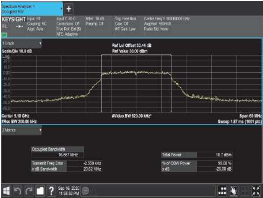
Figure 2 - 5180 MHz - 99 % Occupied Bandwidth h
