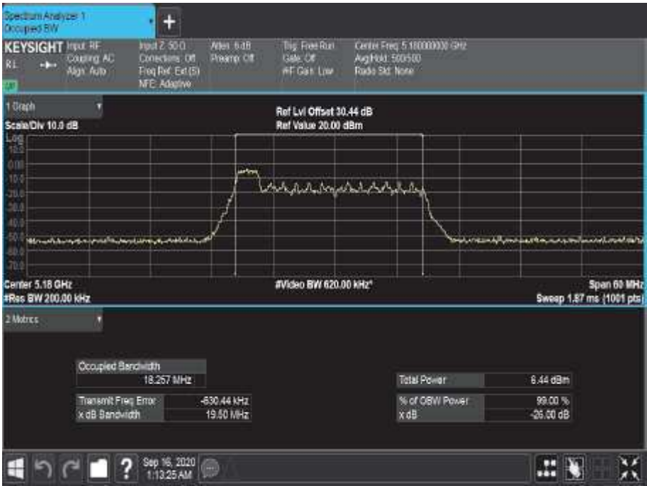
Figure 116 - 5180 MHz - 99% Occupied Bandwidth
