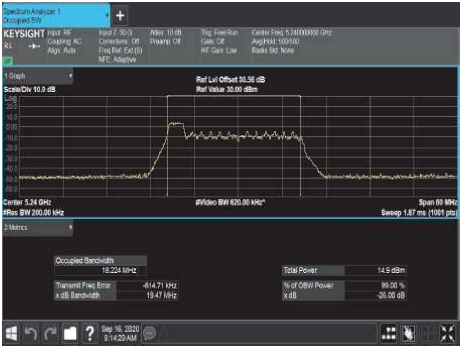
Figure 114 - 5240 MHz - 99% Occupied Bandwidth
