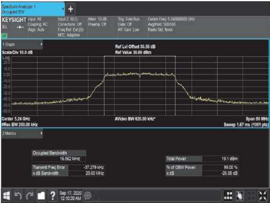
Figure 6 - 5240 M Hz - 99 % Occupied Bandwidth h
