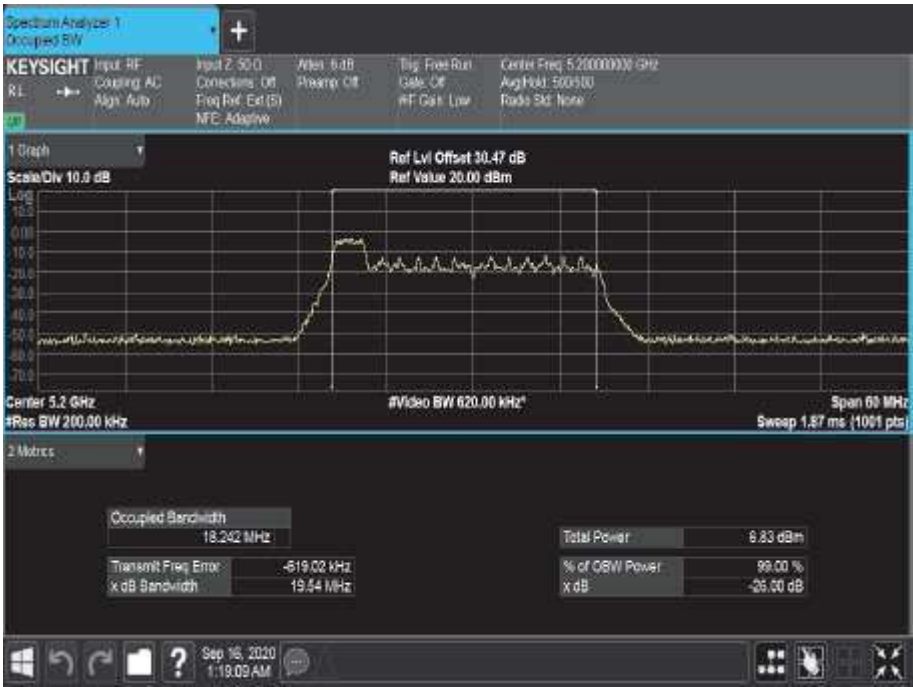
Figure 118 - 5200 MHz - 99% Occupied Bandwidth
