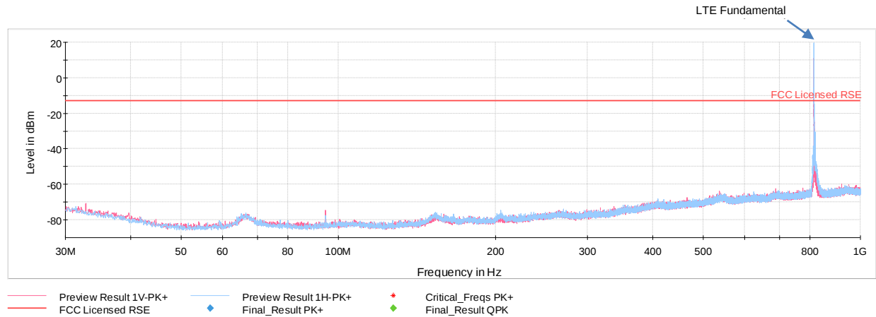
Plot 7-43. Radiated Spurious Emissions Below 1GHz (Band 26)
