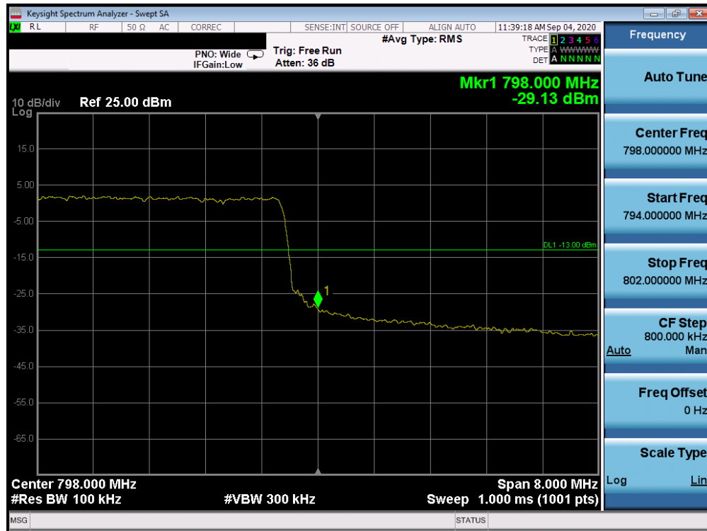
Plot 7-37. Upper Band Edge Plot (Band 14 - 10MHz QPSK - Full RB Configuration)
