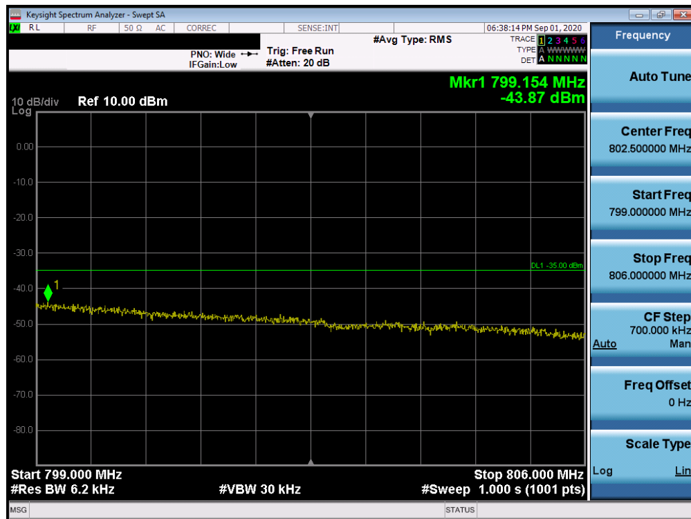
Plot 7-38. Upper Extended Band Edge Plot (Band 14 - 10MHz QPSK - Full RB Configuration)
