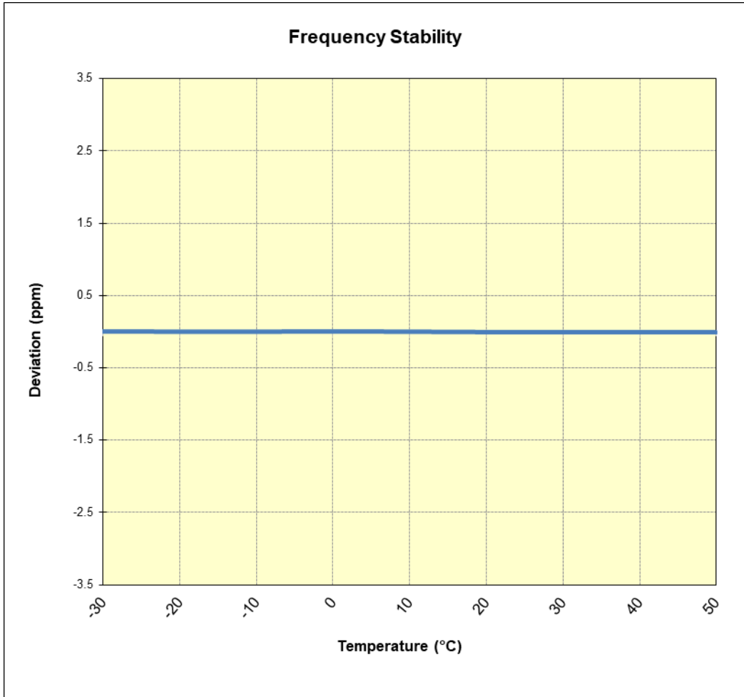
Figure 7-9. Frequency Stability Chart (LTE Band 26 – 10MHz QPSK – Full RB Configuration)
