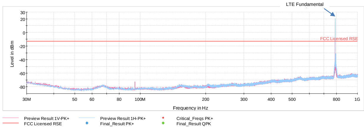
Plot 7-45. Radiated Spurious Emissions Below 1GHz (Band 14)
