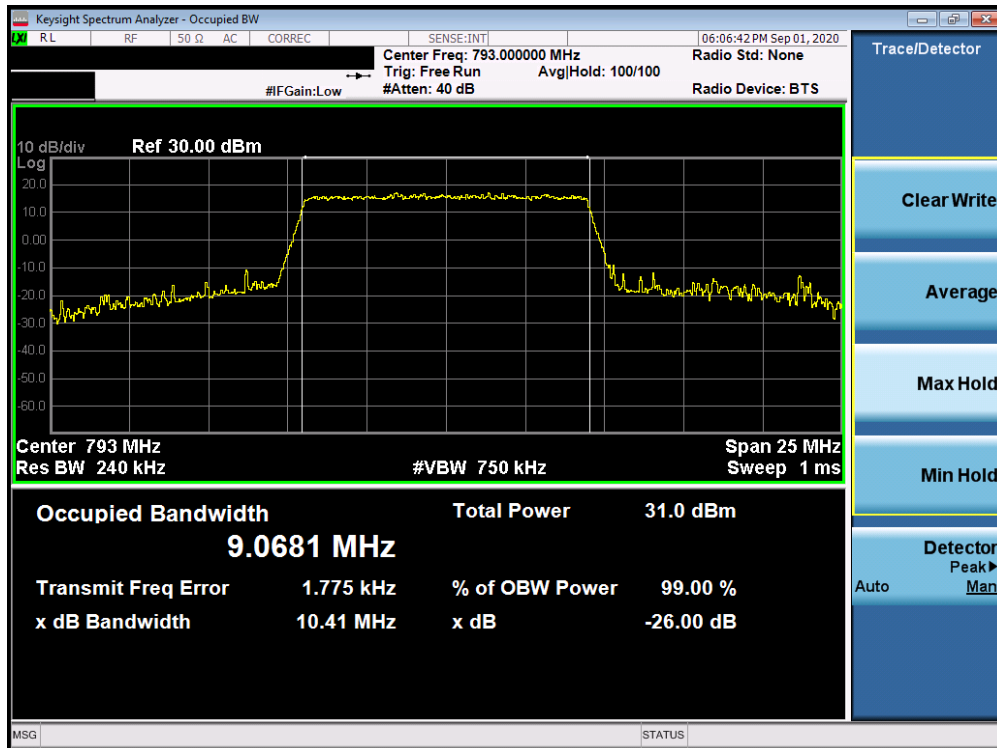
Plot 7-14. Occupied Bandwidth Plot (Band 14 - 10MHz 16-QAM - Full RB Configuration)
