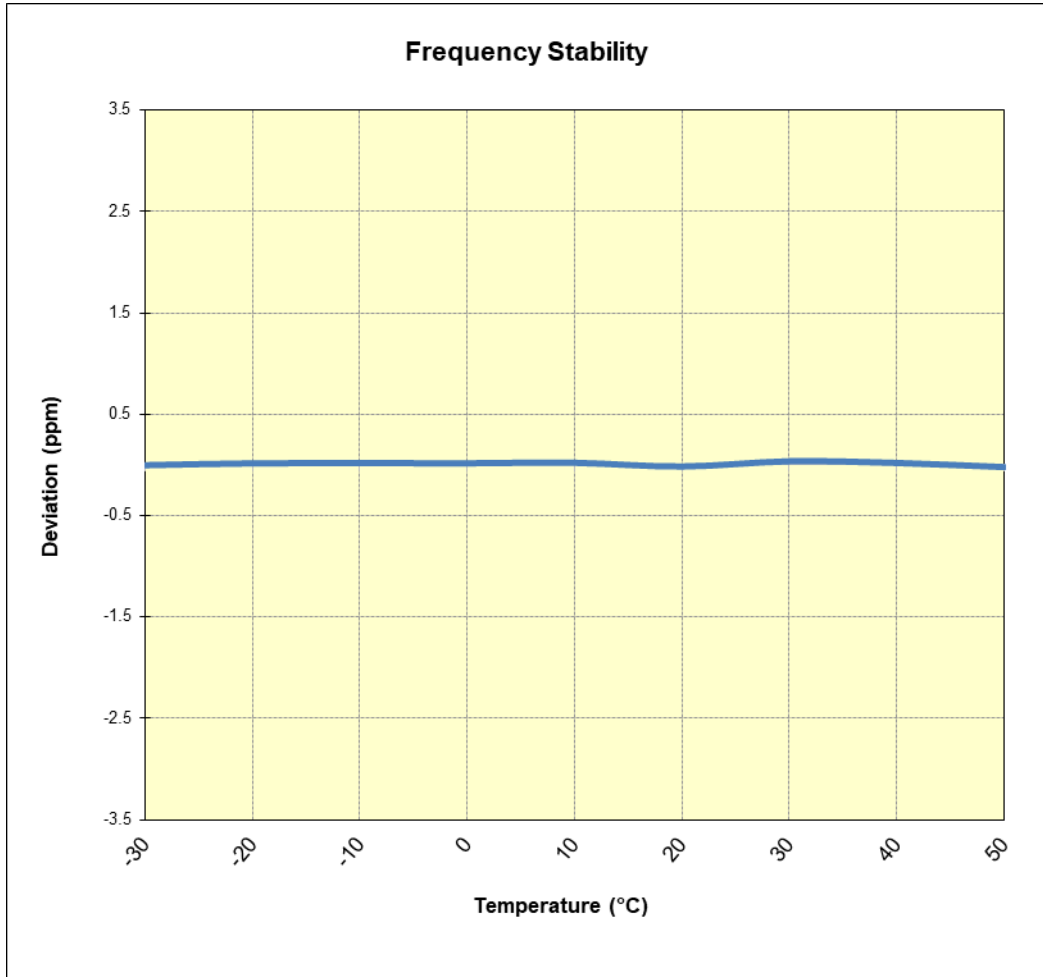
Figure 7-10. Frequency Stability Chart (LTE Band 14 – 10MHz QPSK – Full RB Configuration)
