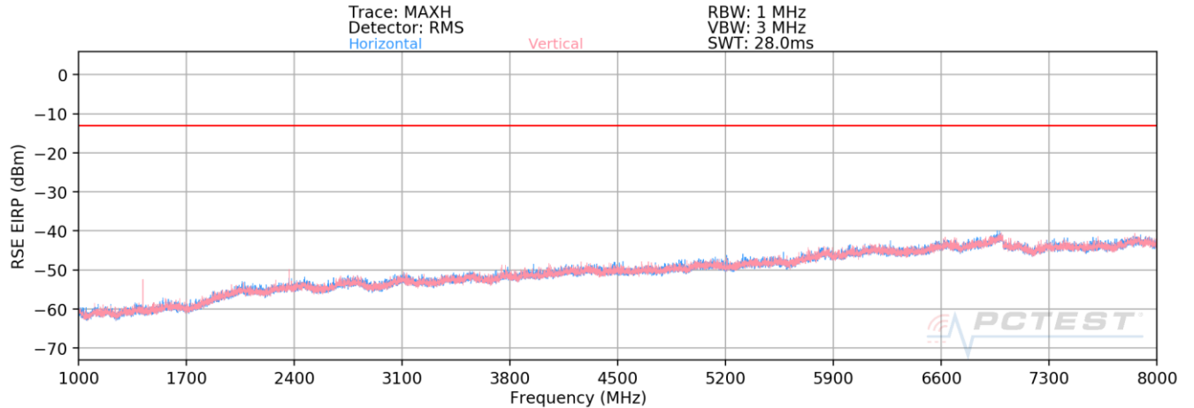
Plot 7-46. Radiated Spurious Emissions Above 1GHz (Band 14)
