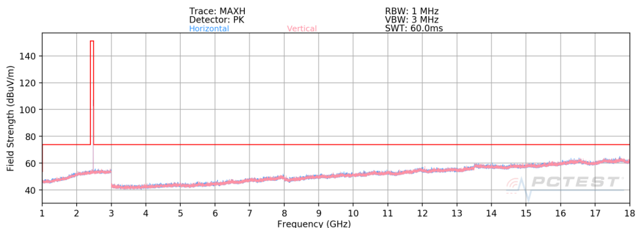
Plot 7-83. Radiated Spurious Emissions Above 1GHz Antenna WF8 (4Mbps, HDR4, ePA – Ch. 75)
