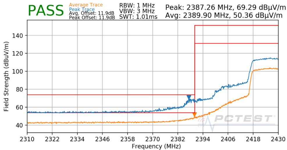
Plot 7-197. Radiated Restricted Lower Band Edge Measurement ANT WF7b (Peak & Average – RU242)
