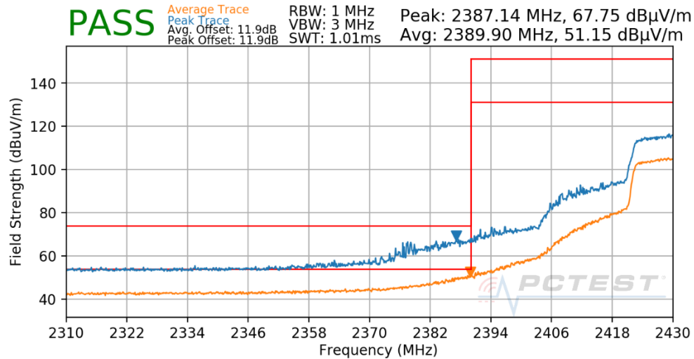
Plot 7-198. Radiated Restricted Lower Band Edge Measurement ANT WF7b (Peak & Average – RU242)
