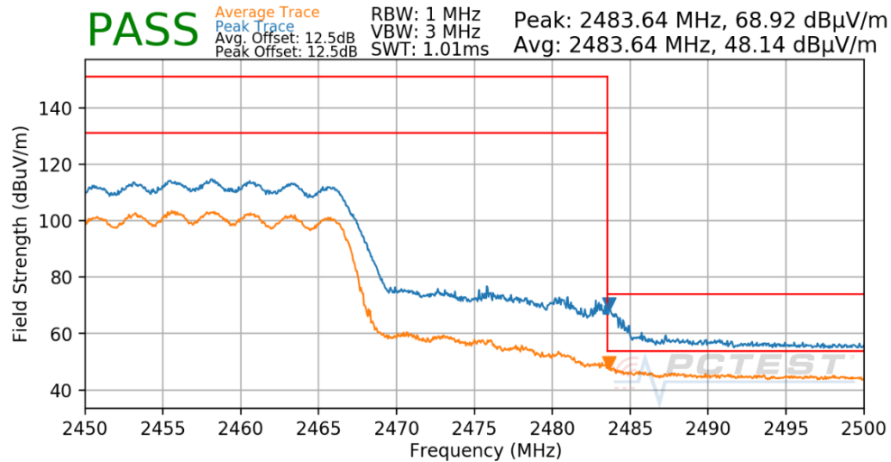
Plot 7-220. Radiated Restricted Upper Band Edge Measurement CDD (Peak & Average – RU242)
