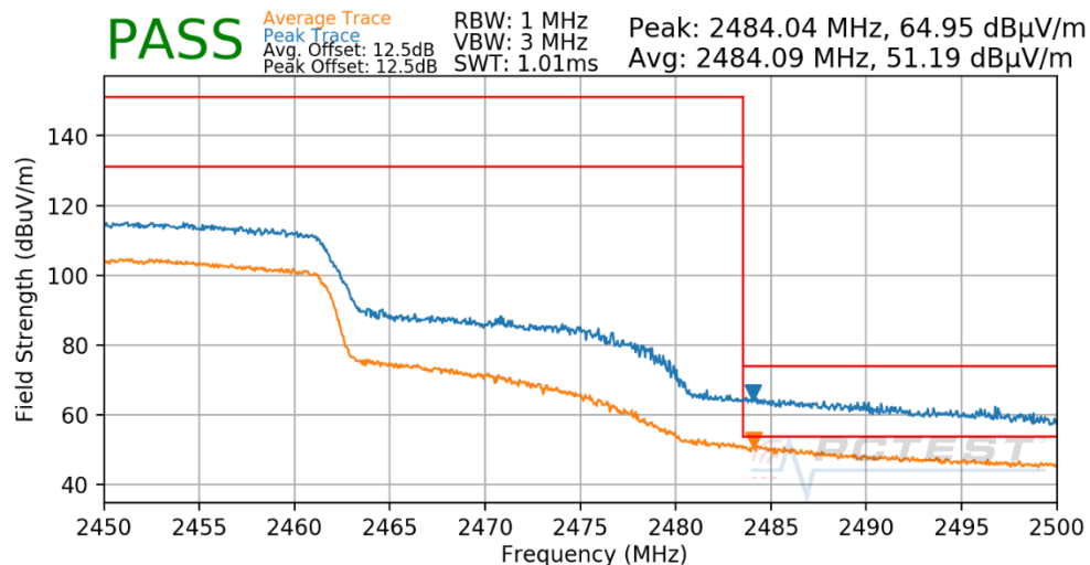
Plot 7-201. Radiated Restricted Upper Band Edge Measurement ANT WF7b (Peak & Average – RU242)
