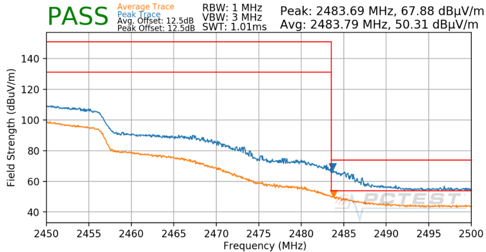
Plot 7-200. Radiated Restricted Upper Band Edge Measurement ANT WF7b (Peak & Average – RU242)
