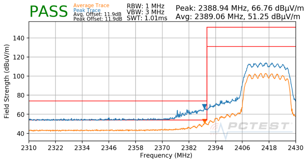
Plot 7-215. Radiated Restricted Lower Band Edge Measurement CDD (Peak & Average – RU242)
