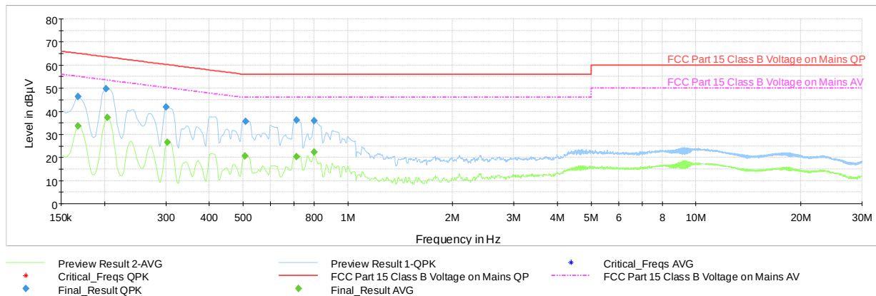
Plot 7-228. AC Line Conducted Emissions with 802.11ax (RU242) Ch.6 (N, with AC/DC Adapter)
