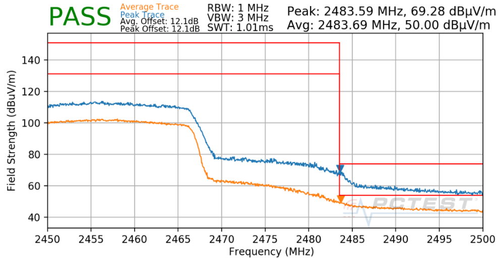
Plot 7-202. Radiated Restricted Upper Band Edge Measurement ANT WF7b (Peak & Average – RU242)
