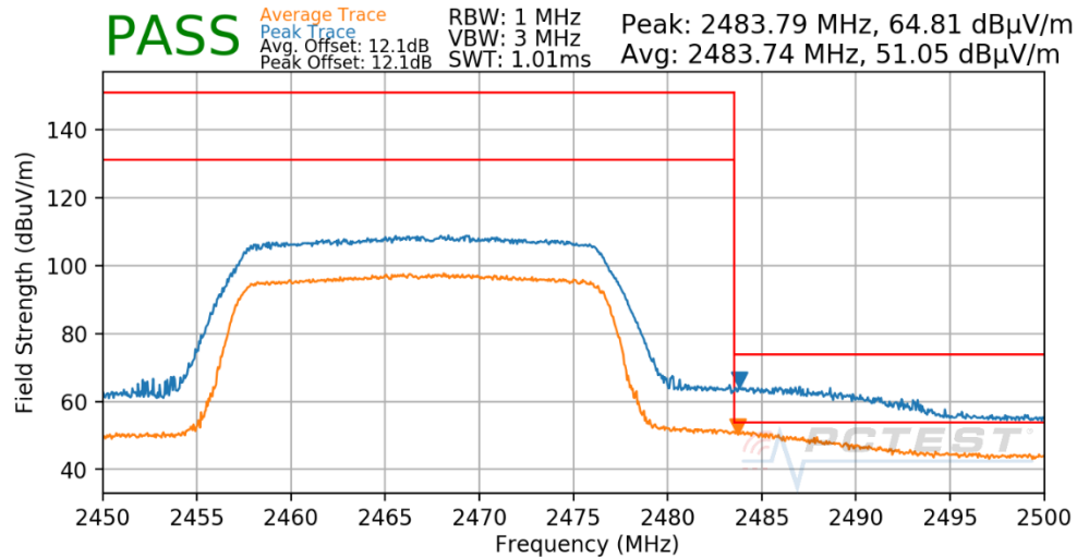
Plot 7-204. Radiated Restricted Upper Band Edge Measurement ANT WF7b (Peak & Average – RU242)
