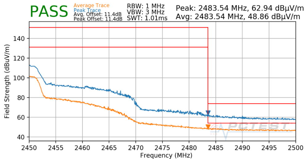
Plot 7-199. Radiated Restricted Upper Band Edge Measurement ANT WF7b (Peak & Average – RU242)
