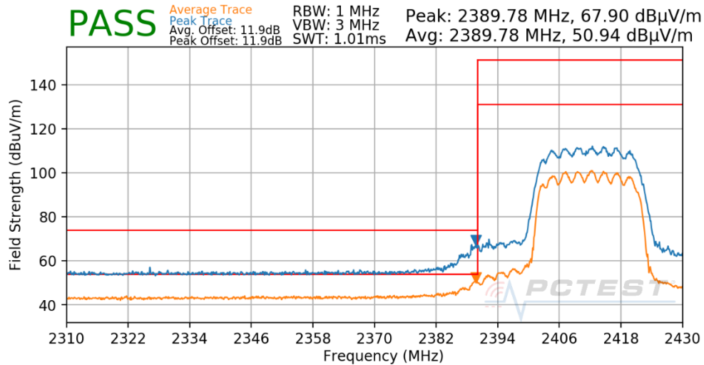
Plot 7-214. Radiated Restricted Lower Band Edge Measurement CDD (Peak & Average – RU242)
