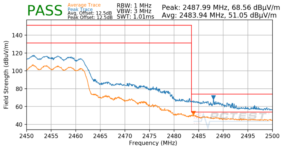
Plot 7-219. Radiated Restricted Upper Band Edge Measurement CDD (Peak & Average – RU242)
