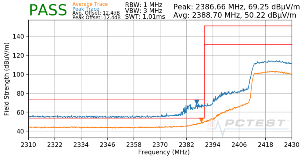
Plot 7-196. Radiated Restricted Lower Band Edge Measurement ANT WF7b (Peak & Average – RU242)
