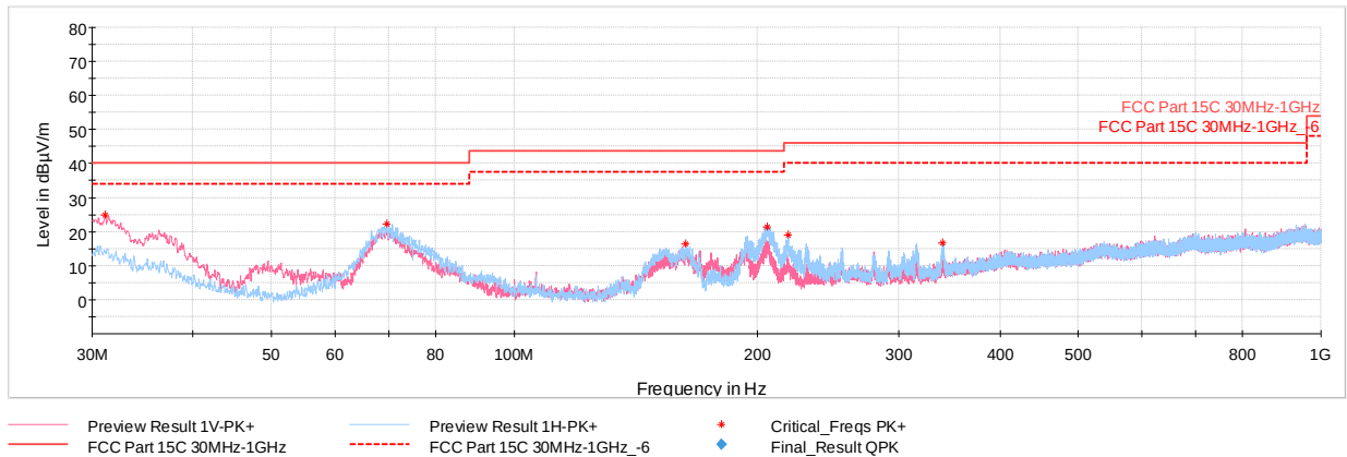
Plot 7-224. Radiated Spurious Emissions below 1GHz CDD Ch.6 (RU242), with AC/DC Adapter
