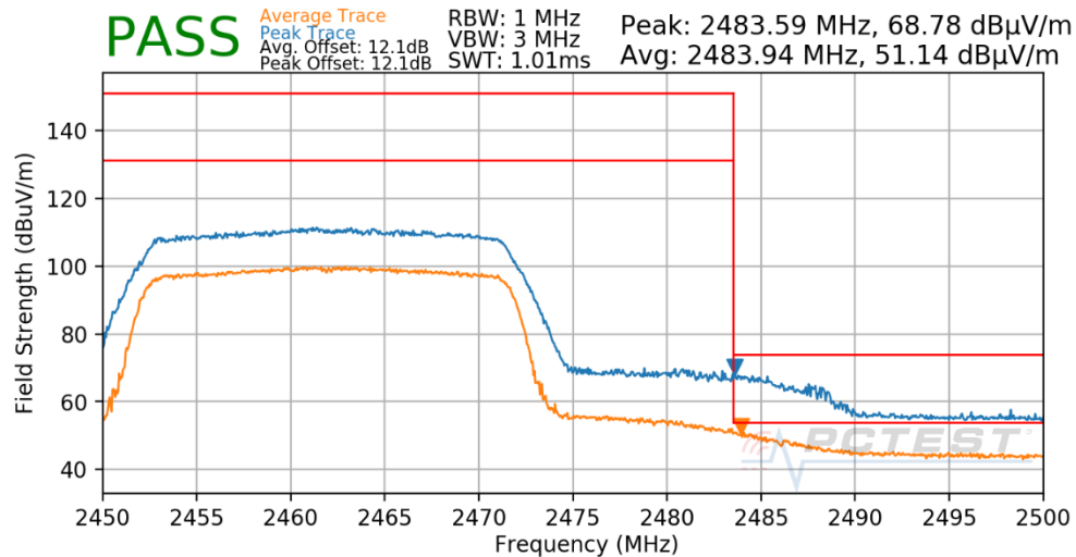
Plot 7-203. Radiated Restricted Upper Band Edge Measurement ANT WF7b (Peak & Average – RU242)
