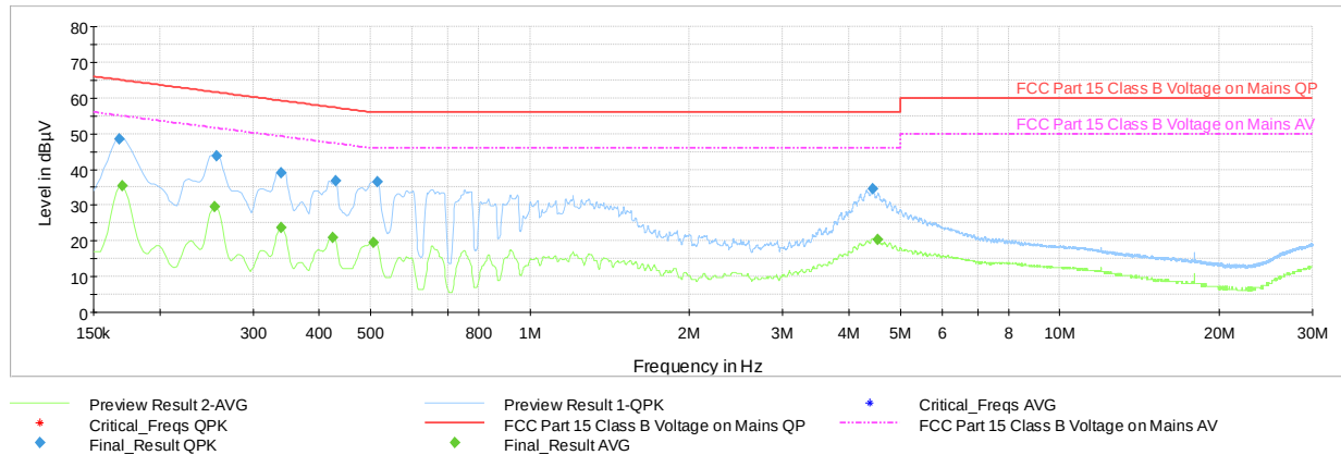
Plot 7-226. AC Line Conducted Emissions with 802.11ax (RU26) Ch.6 (N, with AC/DC Adapter)
