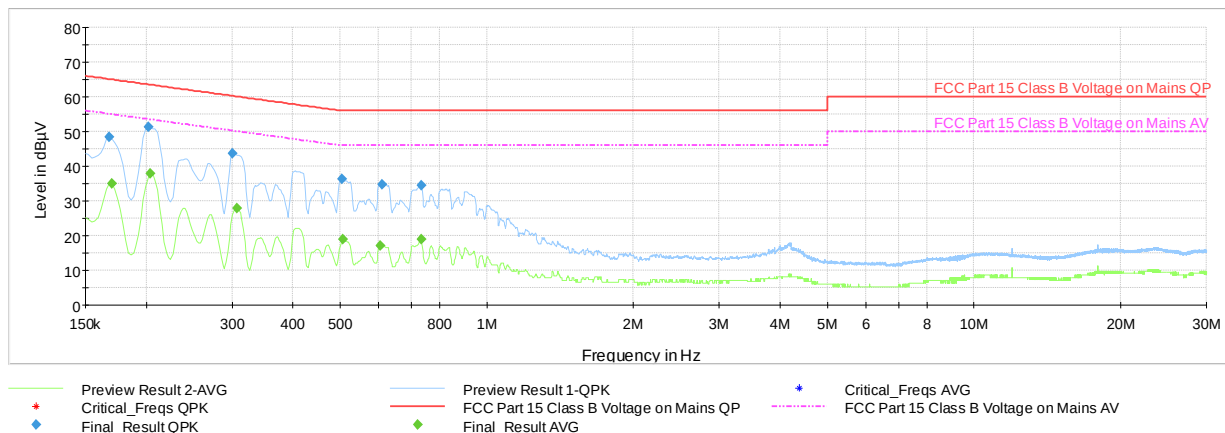
Plot 7-227. AC Line Conducted Emissions with 802.11ax (RU242) Ch.6 (L1, with AC/DC Adapter)
