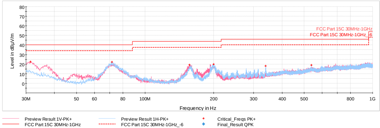
Plot 7-223. Radiated Spurious Emissions below 1GHz CDD Ch.6 (RU26), with AC/DC Adapter
