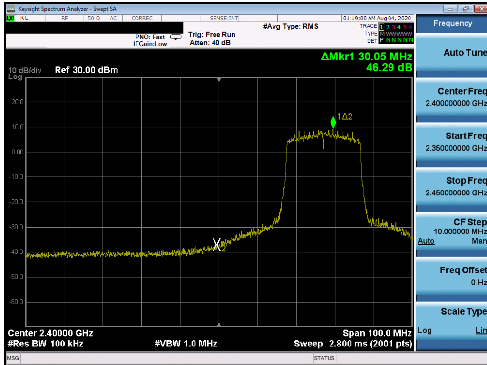
Plot 7-109. Band Edge ANT WF7b (802.11ax OFDMA – RU242 – Ch. 4)
