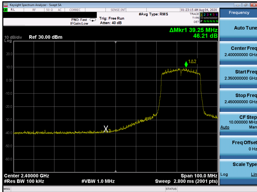
Plot 7-110. Band Edge ANT WF7b (802.11ax OFDMA – RU242 – Ch. 5)
