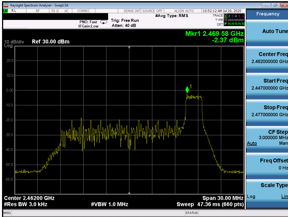
Plot 7-33. Power Spectral Density Plot ANT WF8 (802.11ax OFDMA – RU26 Index 8 – Ch. 11)
