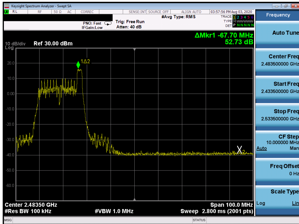
Plot 7-80. Band Edge ANT WF8 (802.11ax OFDMA – RU26 Index 8 – Ch. 9)
