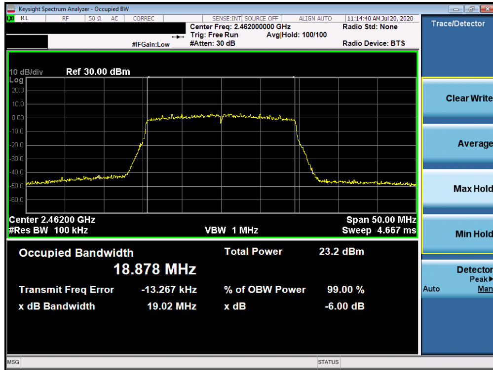
Plot 7-12. 6dB Bandwidth Plot ANT WF8 (802.11ax OFDMA – RU242 – Ch. 11)
