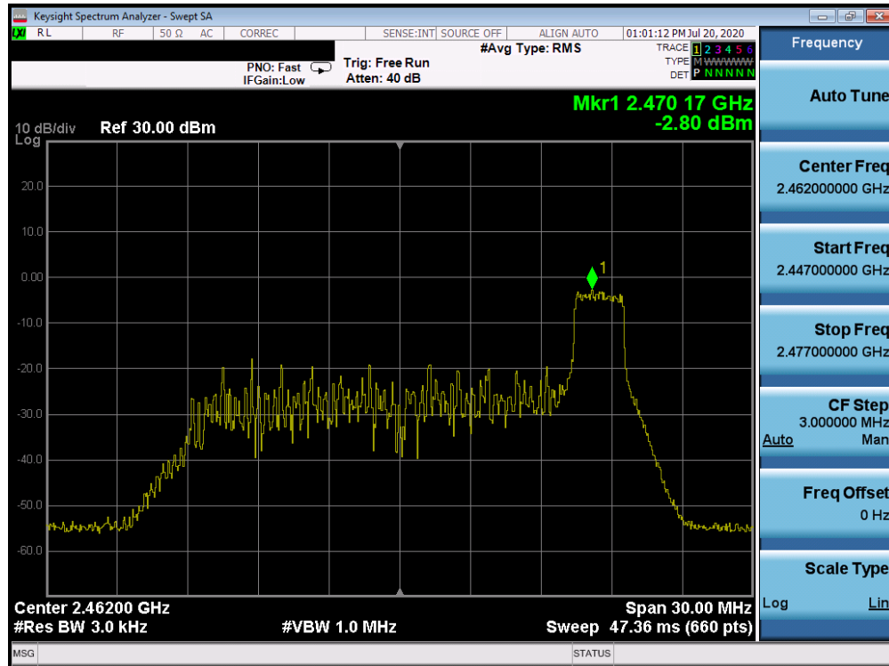
Plot 7-45. Power Spectral Density Plot ANT WF7b (802.11ax OFDMA – RU26 Index 8 – Ch. 11)
