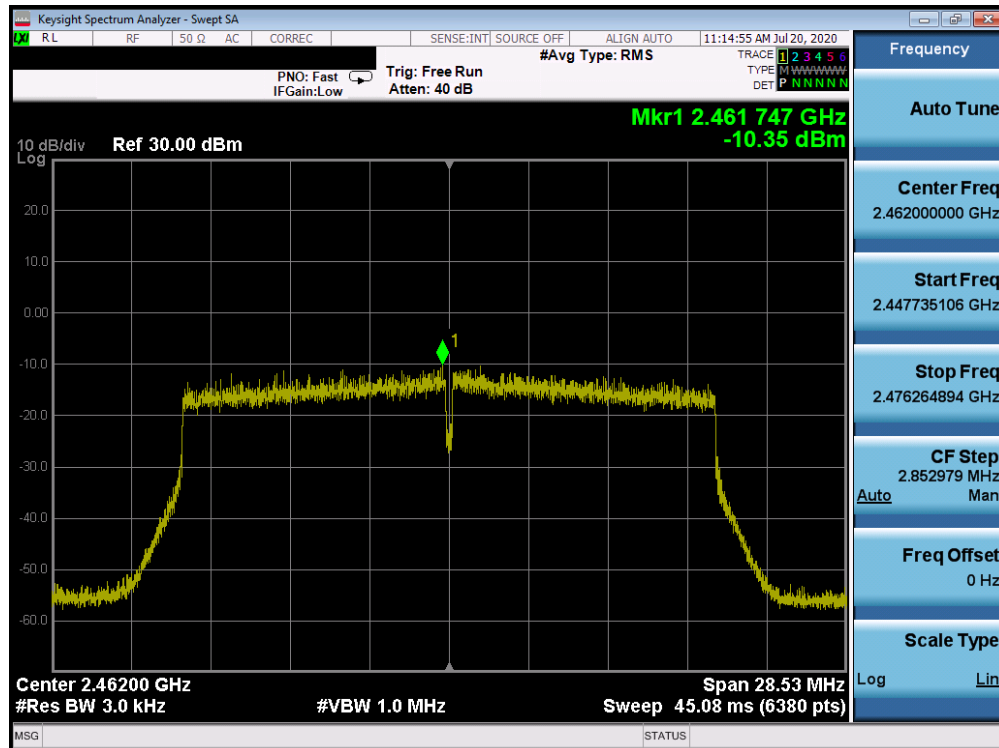
Plot 7-36. Power Spectral Density Plot ANT WF8 (802.11ax OFDMA – RU242 – Ch. 11)
