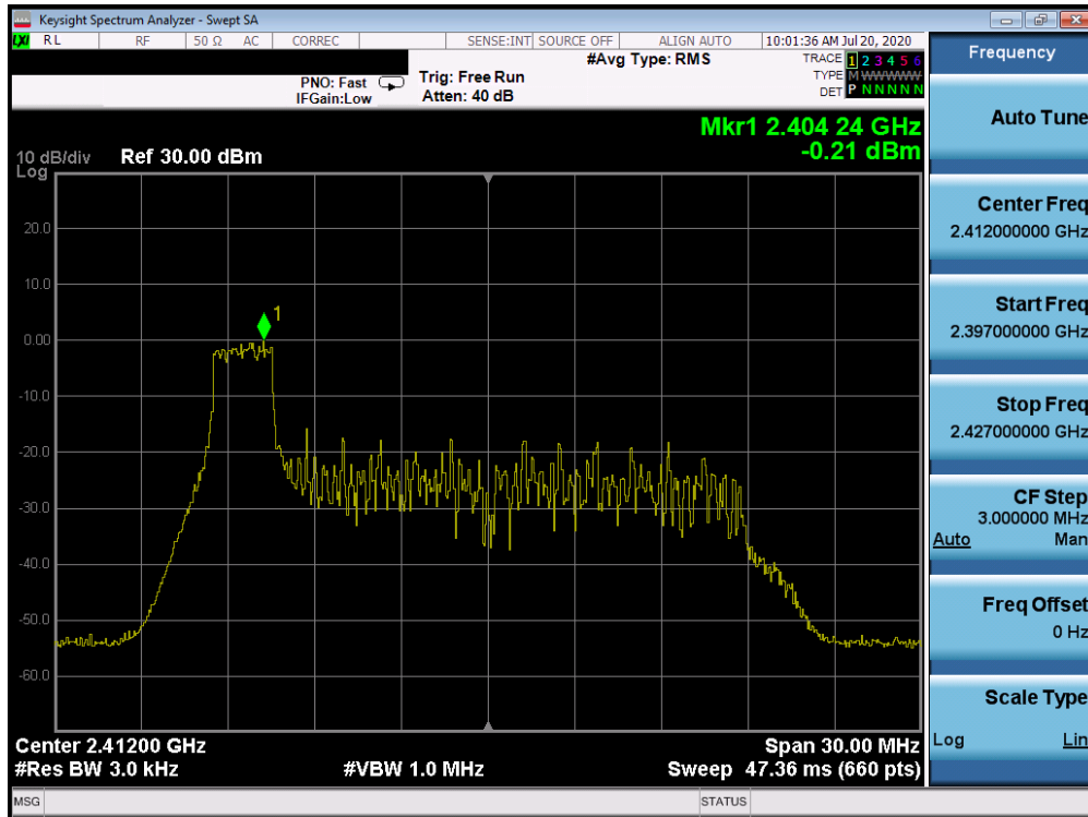
Plot 7-25. Power Spectral Density Plot ANT WF8 (802.11ax OFDMA – RU26 Index 0 – Ch. 1)
