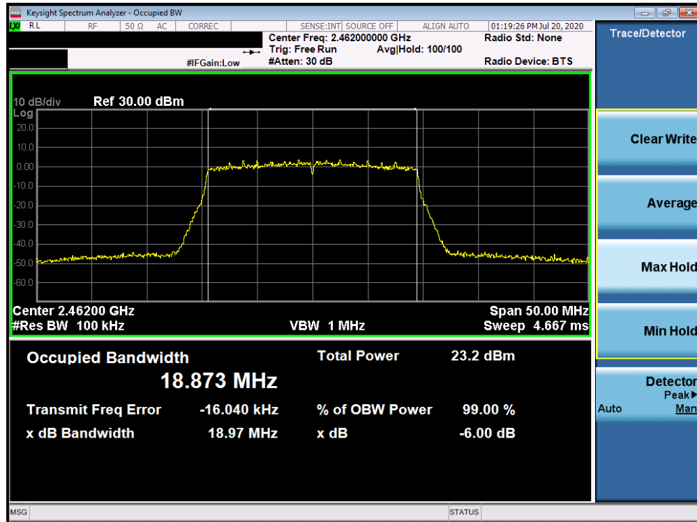
Plot 7-24. 6dB Bandwidth Plot ANT WF7b (802.11ax OFDMA – RU242 – Ch. 11)
