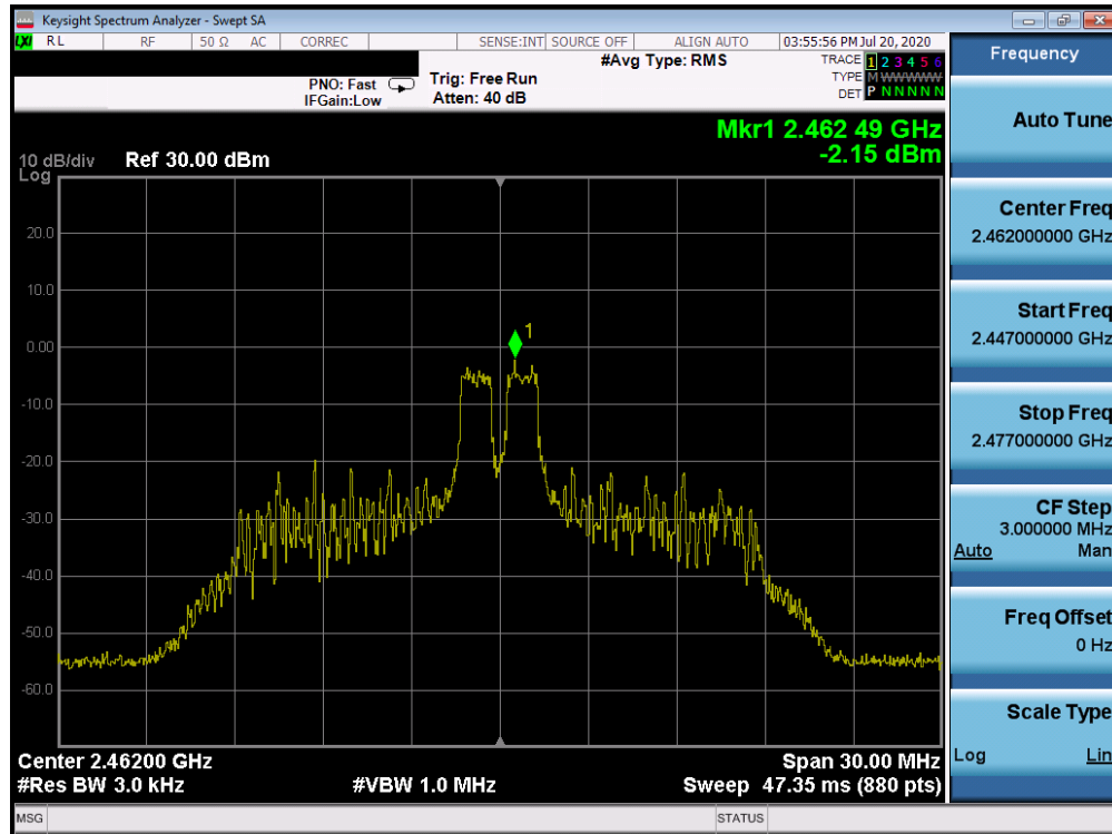
Plot 7-63. Power Spectral Density Plot CDD ANT WF8 (802.11ax OFDMA – RU26 Index 4 – Ch. 11)
