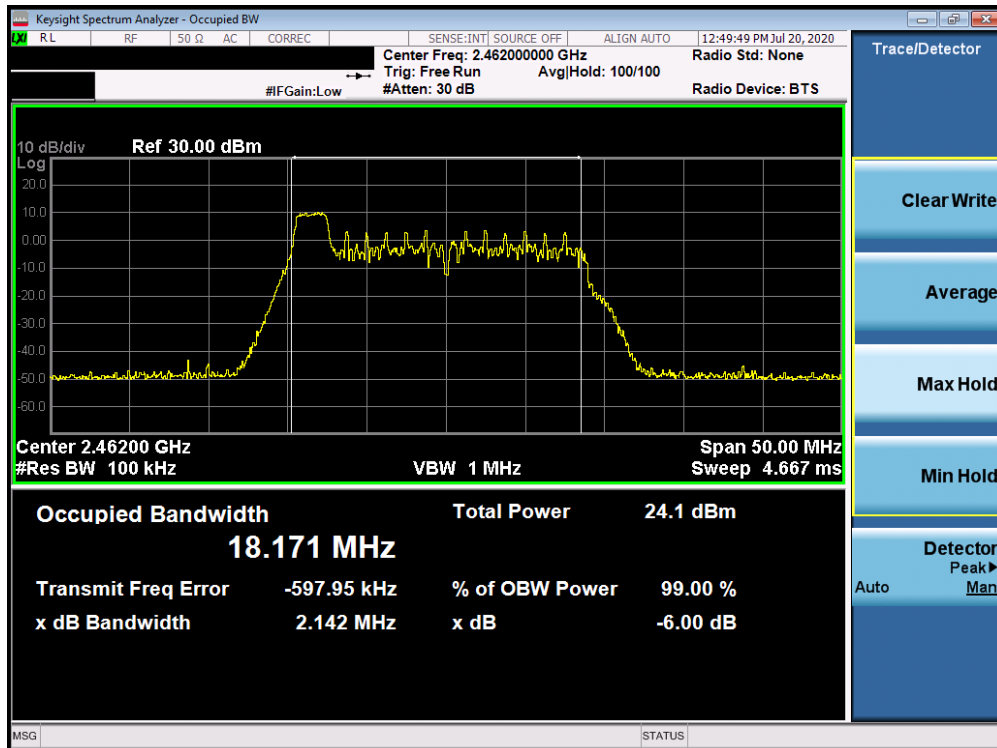
Plot 7-19. 6dB Bandwidth Plot ANT WF7b (802.11ax OFDMA – RU26 Index 0 – Ch. 11)
