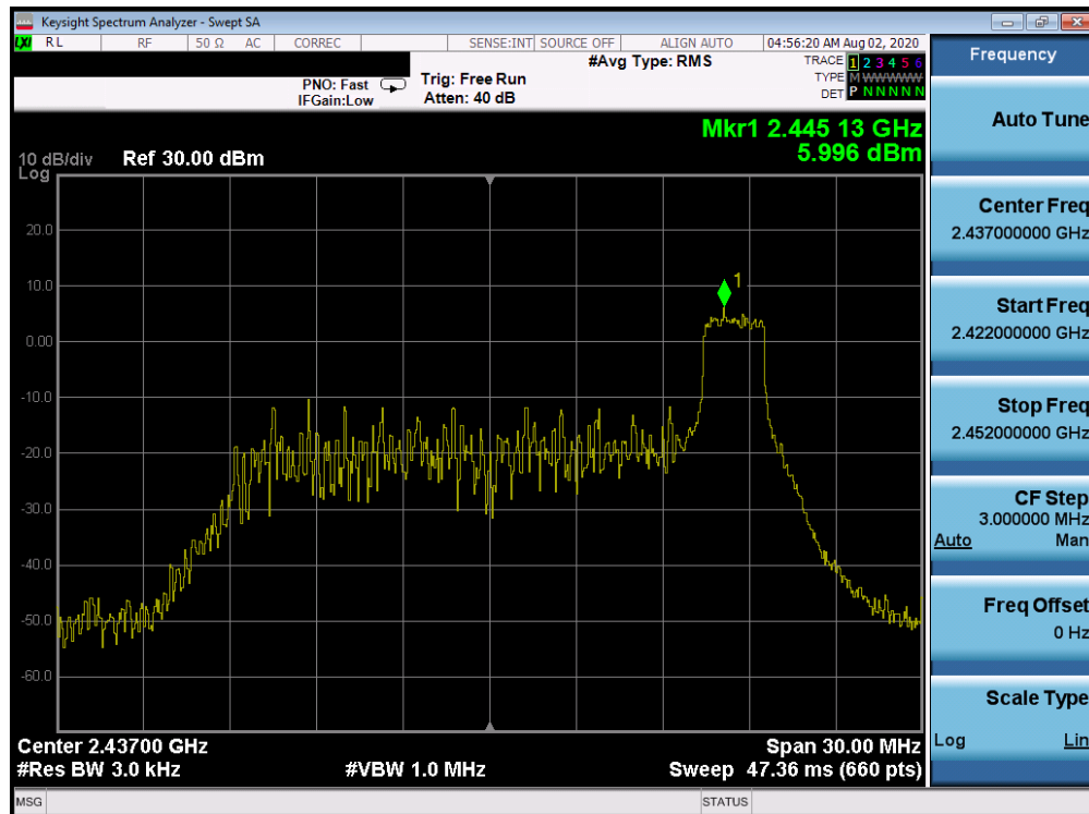
Plot 7-42. Power Spectral Density Plot ANT WF7b (802.11ax OFDMA – RU26 Index 8 – Ch. 6)
