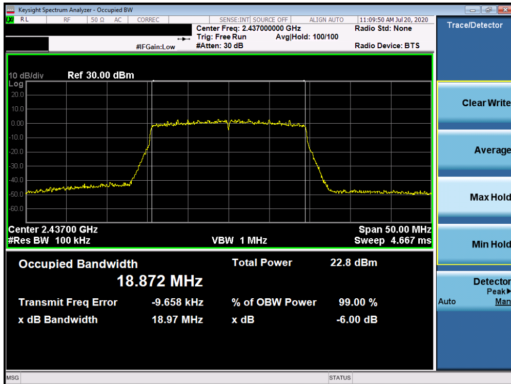
Plot 7-11. 6dB Bandwidth Plot ANT WF8 (802.11ax OFDMA – RU242 – Ch. 6)
