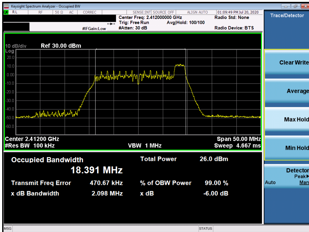
Plot 7-15. 6dB Bandwidth Plot ANT WF7b (802.11ax OFDMA – RU26 Index 8 – Ch. 1)
