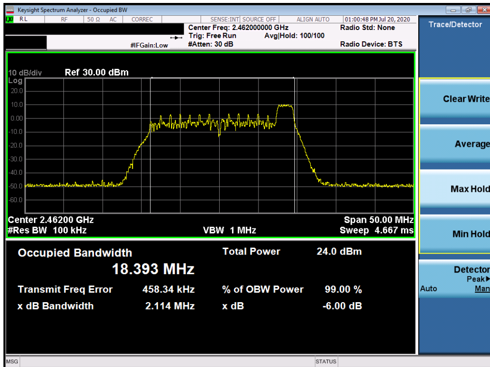
Plot 7-21. 6dB Bandwidth Plot ANT WF7b (802.11ax OFDMA – RU26 Index 8 – Ch. 11)
