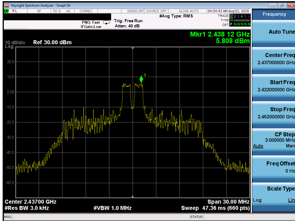
Plot 7-41. Power Spectral Density Plot ANT WF7b (802.11ax OFDMA – RU26 Index 4 – Ch. 6)
