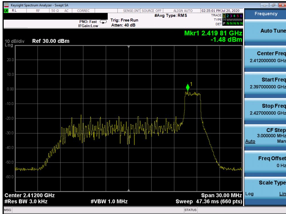
Plot 7-53. Power Spectral Density Plot CDD ANT WF8 (802.11ax OFDMA – RU26 Index 8 – Ch. 1)
