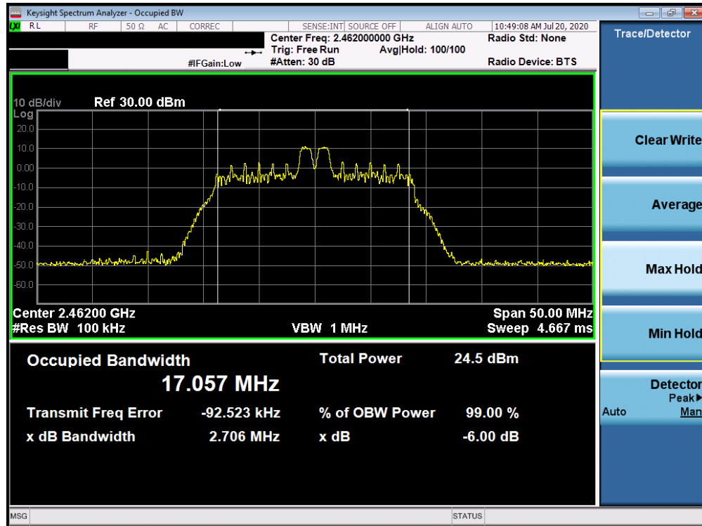
Plot 7-8. 6dB Bandwidth Plot ANT WF8 (802.11ax OFDMA – RU26 Index 4 – Ch. 11)
