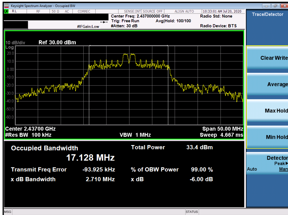
Plot 7-5. 6dB Bandwidth Plot ANT WF8 (802.11ax OFDMA – RU26 Index 4 – Ch. 6)
