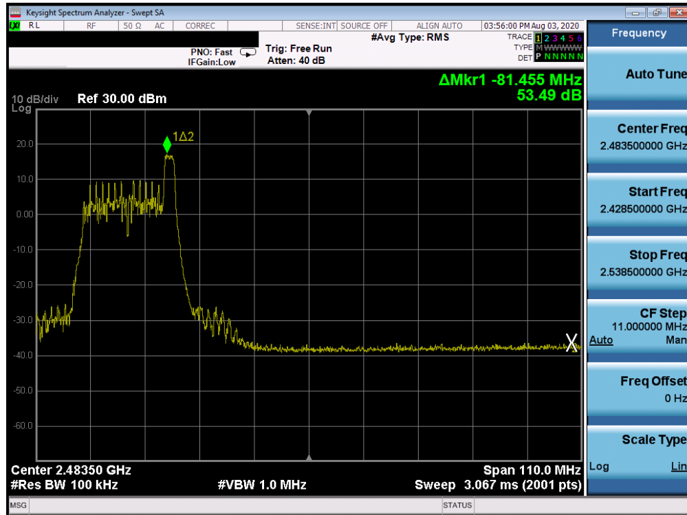
Plot 7-79. Band Edge ANT WF8 (802.11ax OFDMA – RU26 Index 8 – Ch. 8)
