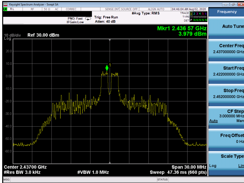
Plot 7-57. Power Spectral Density Plot CDD ANT WF8 (802.11ax OFDMA – RU26 Index 4 – Ch. 6)
