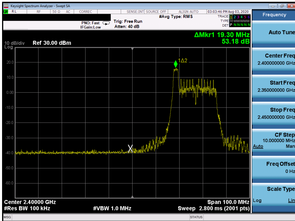
Plot 7-76. Band Edge ANT WF8 (802.11ax OFDMA – RU26 Index 0 – Ch. 4)
