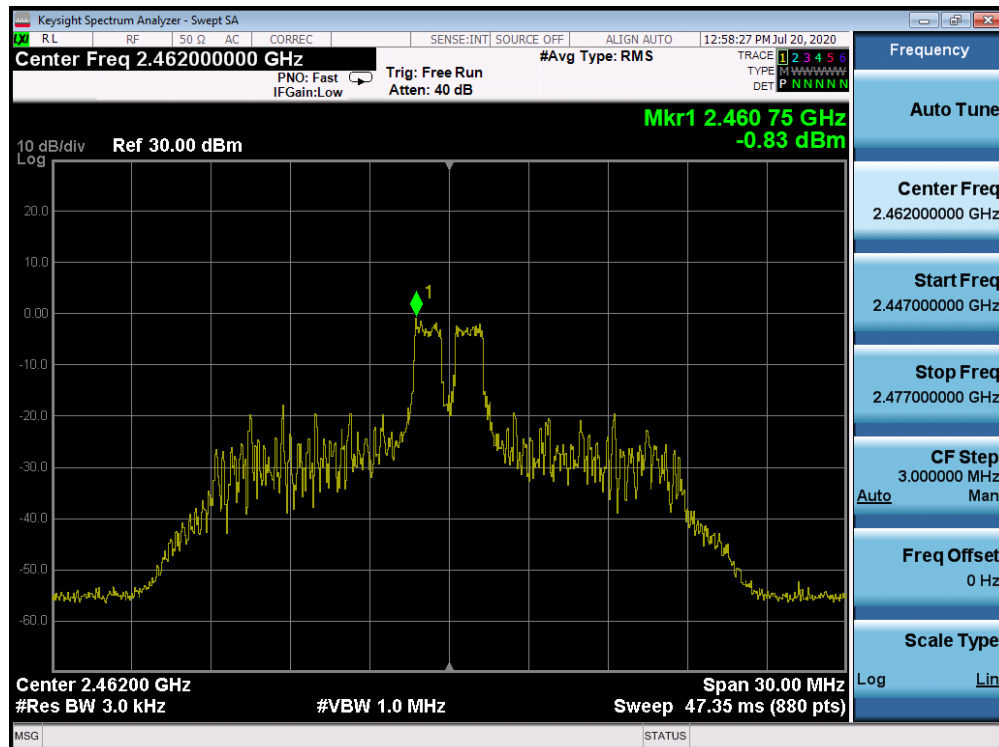
Plot 7-44. Power Spectral Density Plot ANT WF7b (802.11ax OFDMA – RU26 Index 4 – Ch. 11)
