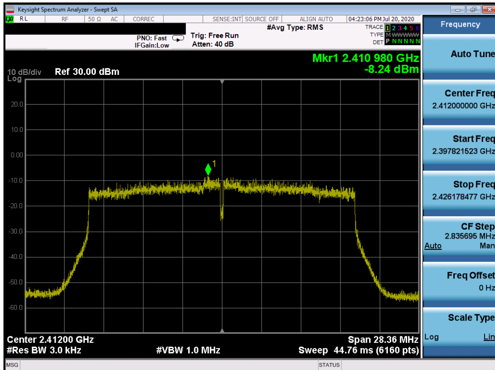
Plot 7-68. Power Spectral Density Plot CDD ANT WF7b (802.11ax OFDMA – RU242 – Ch. 1)
