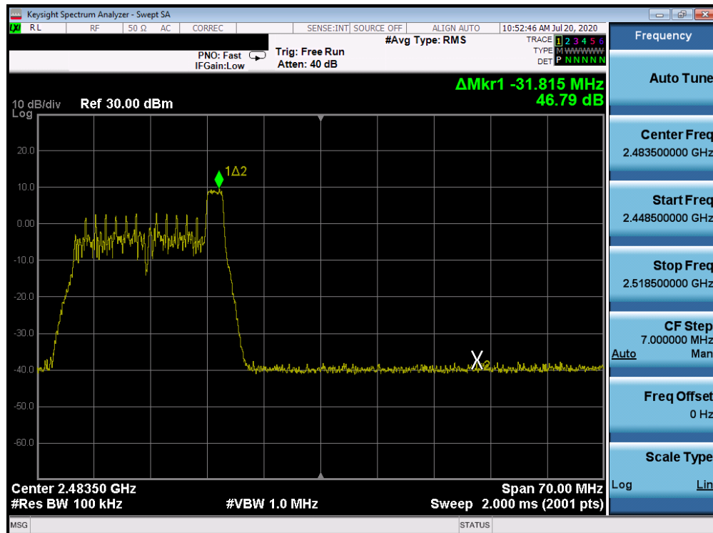
Plot 7-82. Band Edge ANT WF8 (802.11ax OFDMA – RU26 Index 8 – Ch. 11)
