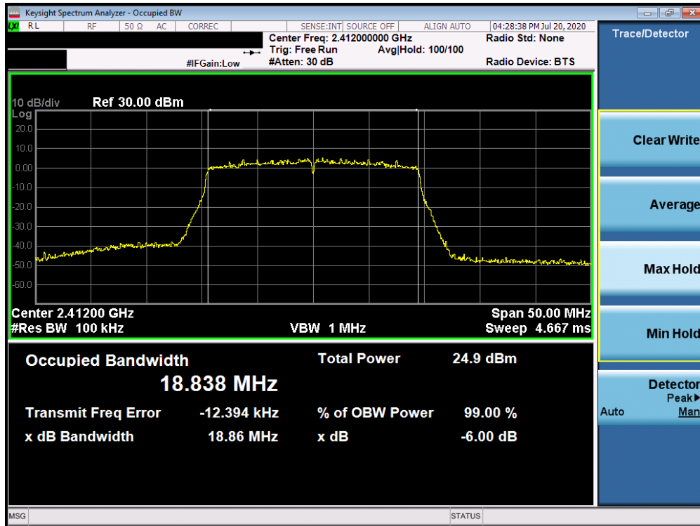
Plot 7-10. 6dB Bandwidth Plot ANT WF8 (802.11ax OFDMA – RU242 – Ch. 1)
