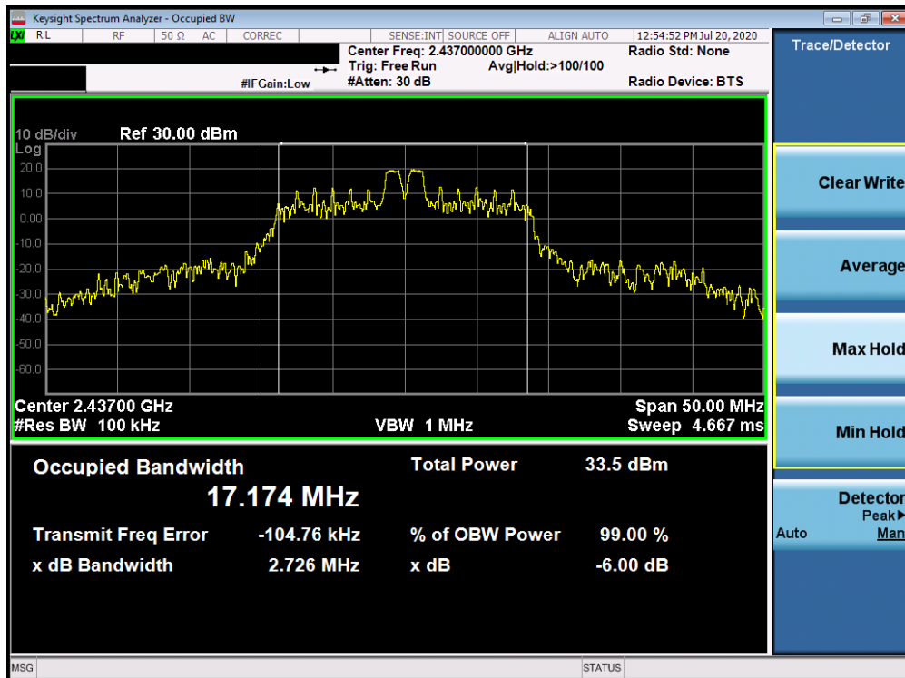
Plot 7-17. 6dB Bandwidth Plot ANT WF7b (802.11ax OFDMA – RU26 Index 4 – Ch. 6)
