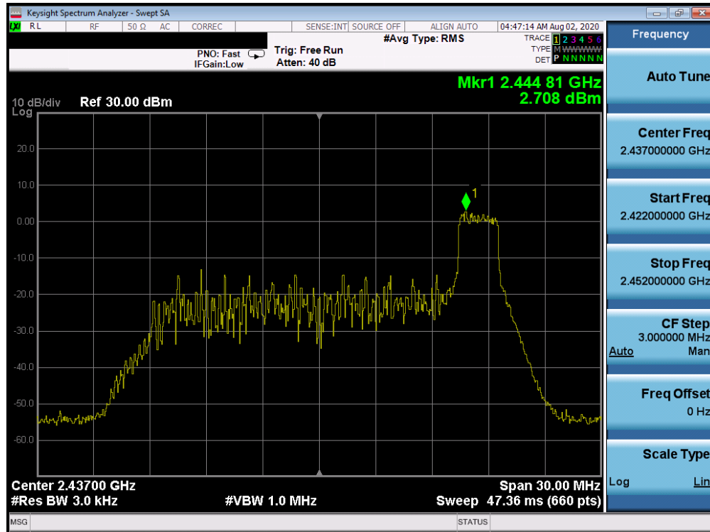
Plot 7-59. Power Spectral Density Plot CDD ANT WF8 (802.11ax OFDMA – RU26 Index 8 – Ch. 6)
