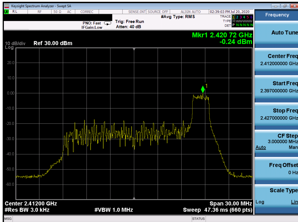
Plot 7-54. Power Spectral Density Plot CDD ANT WF7b (802.11ax OFDMA – RU26 Index 8 – Ch. 1)
