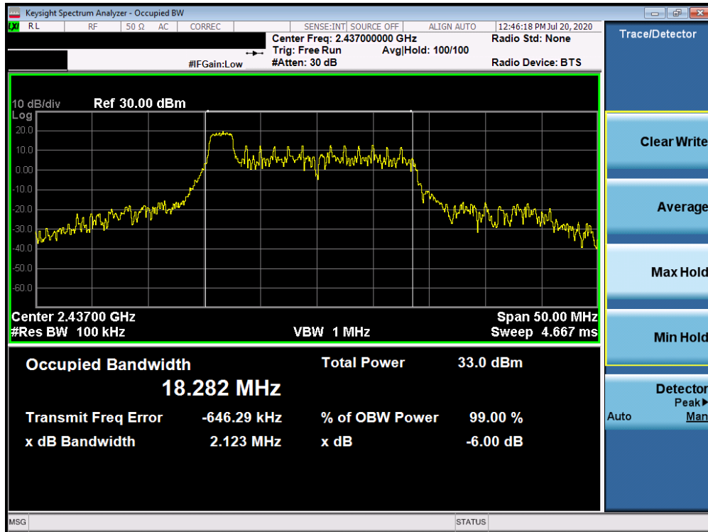
Plot 7-16. 6dB Bandwidth Plot ANT WF7b (802.11ax OFDMA – RU26 Index 0 – Ch. 6)
