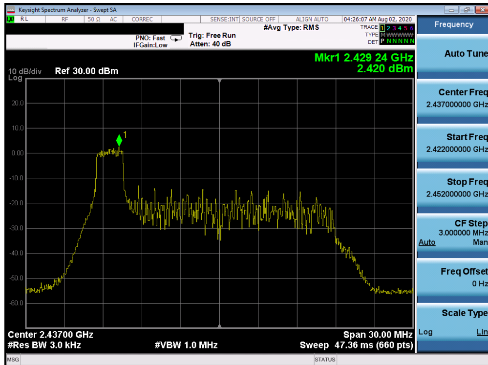
Plot 7-56. Power Spectral Density Plot CDD ANT WF7b (802.11ax OFDMA – RU26 Index 0 – Ch. 6)
