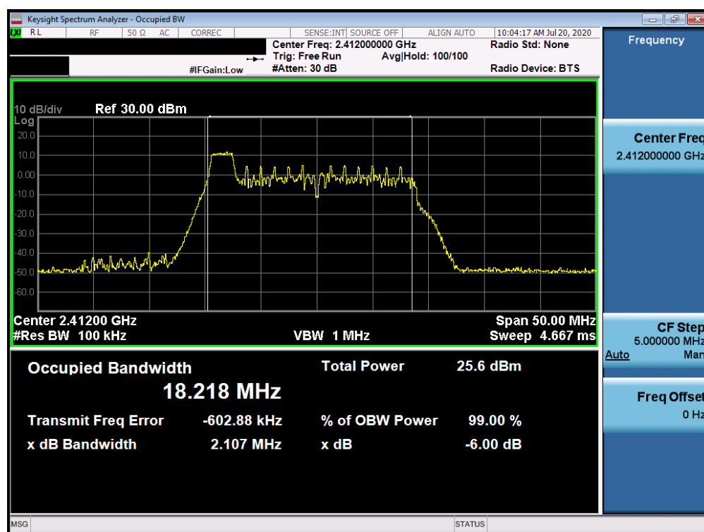
Plot 7-1. 6dB Bandwidth Plot ANT WF8 (802.11ax OFDMA – RU26 Index 0 – Ch. 1)
