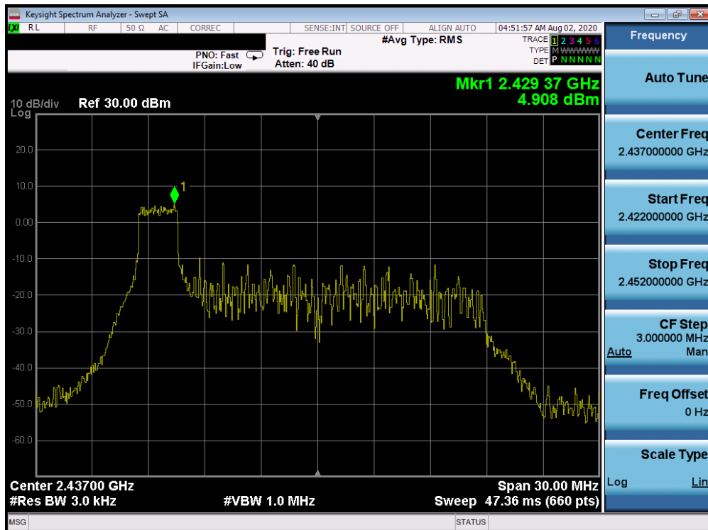
Plot 7-40. Power Spectral Density Plot ANT WF7b (802.11ax OFDMA – RU26 Index 0 – Ch. 6)
