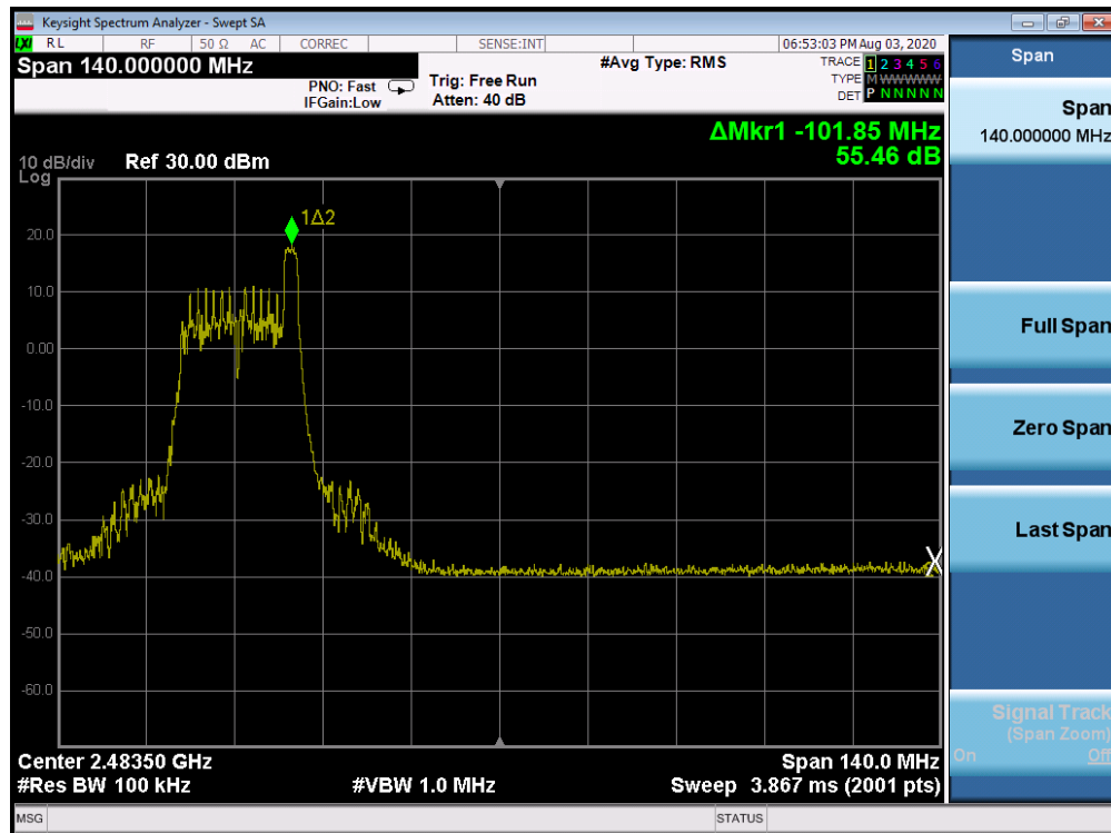
Plot 7-78. Band Edge ANT WF8 (802.11ax OFDMA – RU26 Index 8 – Ch. 7)
