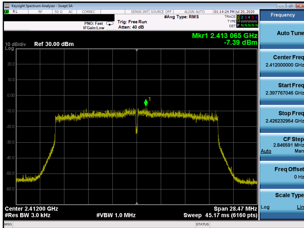
Plot 7-46. Power Spectral Density Plot ANT WF7b (802.11ax OFDMA – RU242 – Ch. 1)
