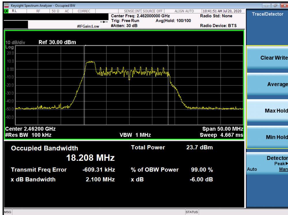
Plot 7-7. 6dB Bandwidth Plot ANT WF8 (802.11ax OFDMA – RU26 Index 0 – Ch. 11)
