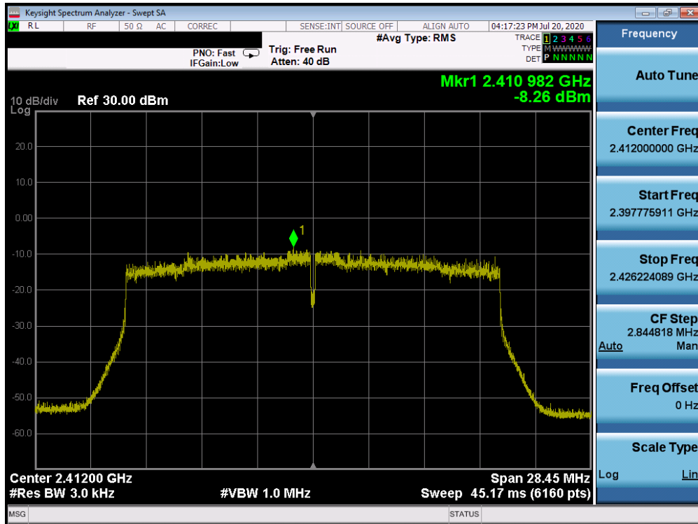
Plot 7-67. Power Spectral Density Plot CDD ANT WF8 (802.11ax OFDMA – RU242 – Ch. 1)
