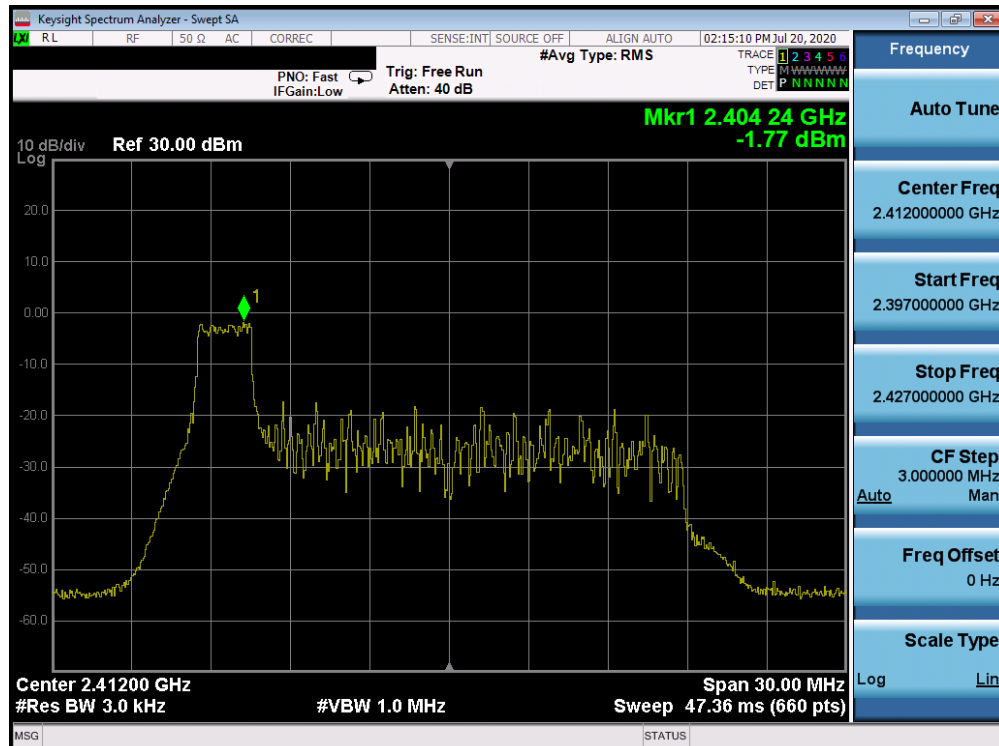
Plot 7-50. Power Spectral Density Plot CDD ANT WF7b (802.11ax OFDMA – RU26 Index 0 – Ch. 1)
