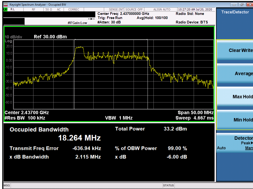
Plot 7-4. 6dB Bandwidth Plot ANT WF8 (802.11ax OFDMA – RU26 Index 0 – Ch. 6)
