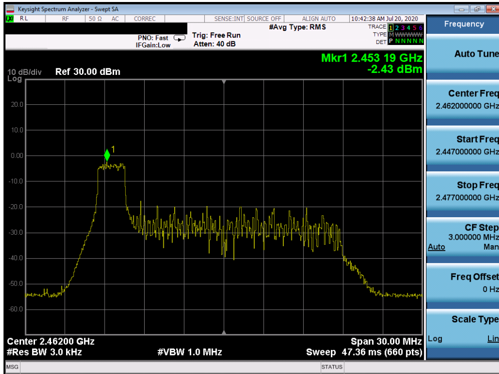
Plot 7-31. Power Spectral Density Plot ANT WF8 (802.11ax OFDMA – RU26 Index 0 – Ch. 11)
