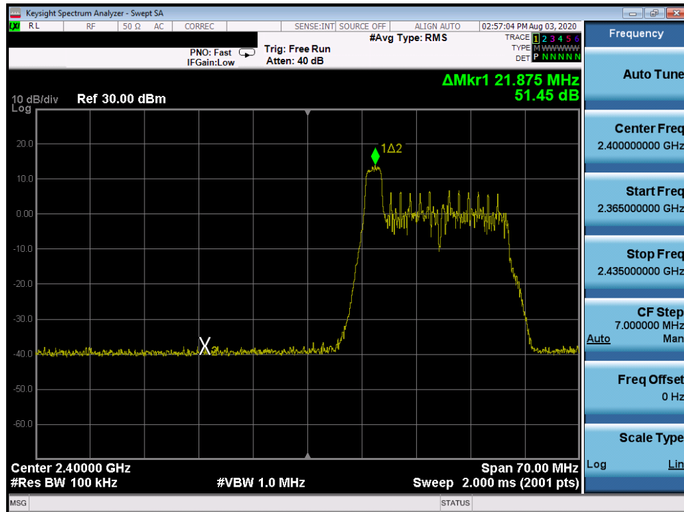
Plot 7-74. Band Edge ANT WF8 (802.11ax OFDMA – RU26 Index 0 – Ch. 2)
