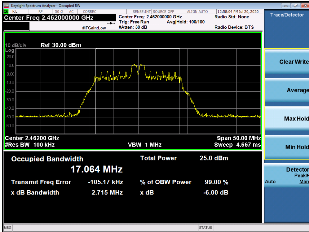
Plot 7-20. 6dB Bandwidth Plot ANT WF7b (802.11ax OFDMA – RU26 Index 4 – Ch. 11)
