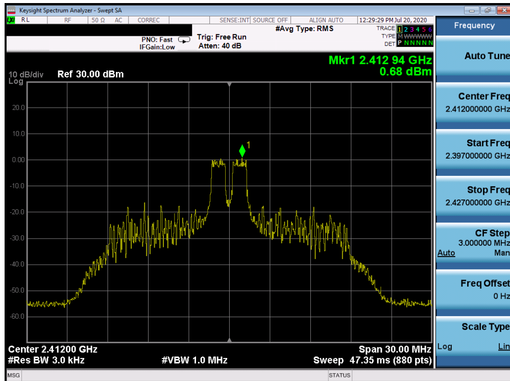
Plot 7-38. Power Spectral Density Plot ANT WF7b (802.11ax OFDMA – RU26 Index 4 – Ch. 1)
