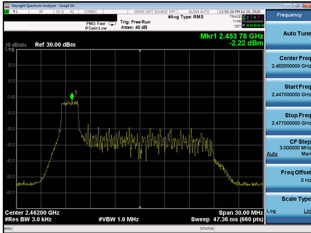
Plot 7-43. Power Spectral Density Plot ANT WF7b (802.11ax OFDMA – RU26 Index 0 – Ch. 11)
