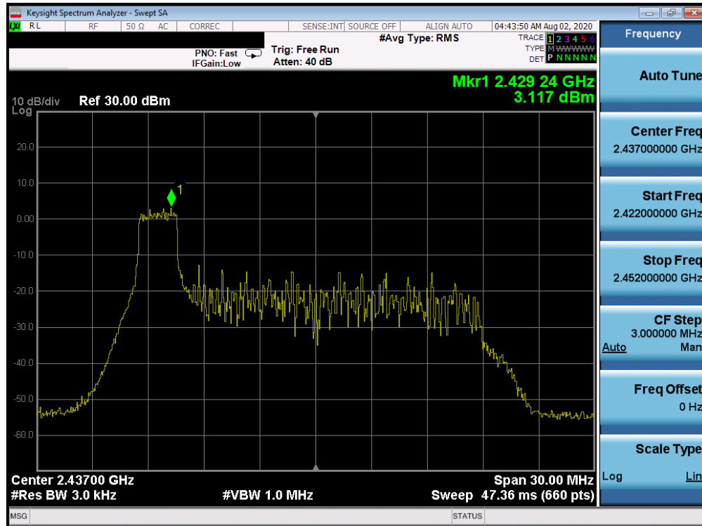
Plot 7-55. Power Spectral Density Plot CDD ANT WF8 (802.11ax OFDMA – RU26 Index 0 – Ch. 6)
