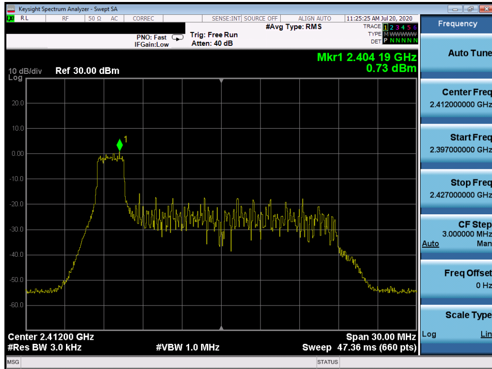
Plot 7-37. Power Spectral Density Plot ANT WF7b (802.11ax OFDMA – RU26 Index 0 – Ch. 1)
