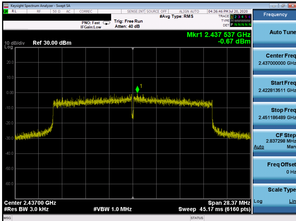
Plot 7-70. Power Spectral Density Plot CDD ANT WF7b (802.11ax OFDMA – RU242 – Ch. 6)
