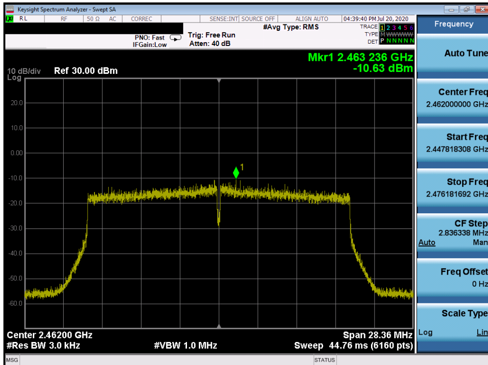
Plot 7-72. Power Spectral Density Plot CDD ANT WF7b (802.11ax OFDMA – RU242 – Ch. 11)
