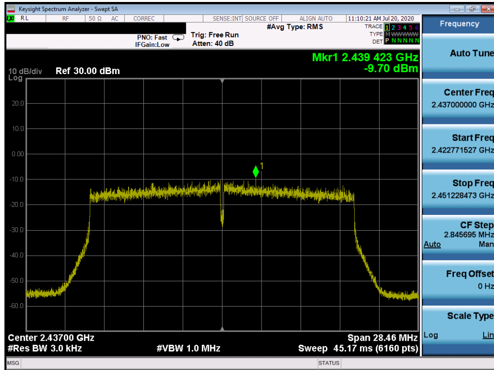
Plot 7-35. Power Spectral Density Plot ANT WF8 (802.11ax OFDMA – RU242 – Ch. 6)
