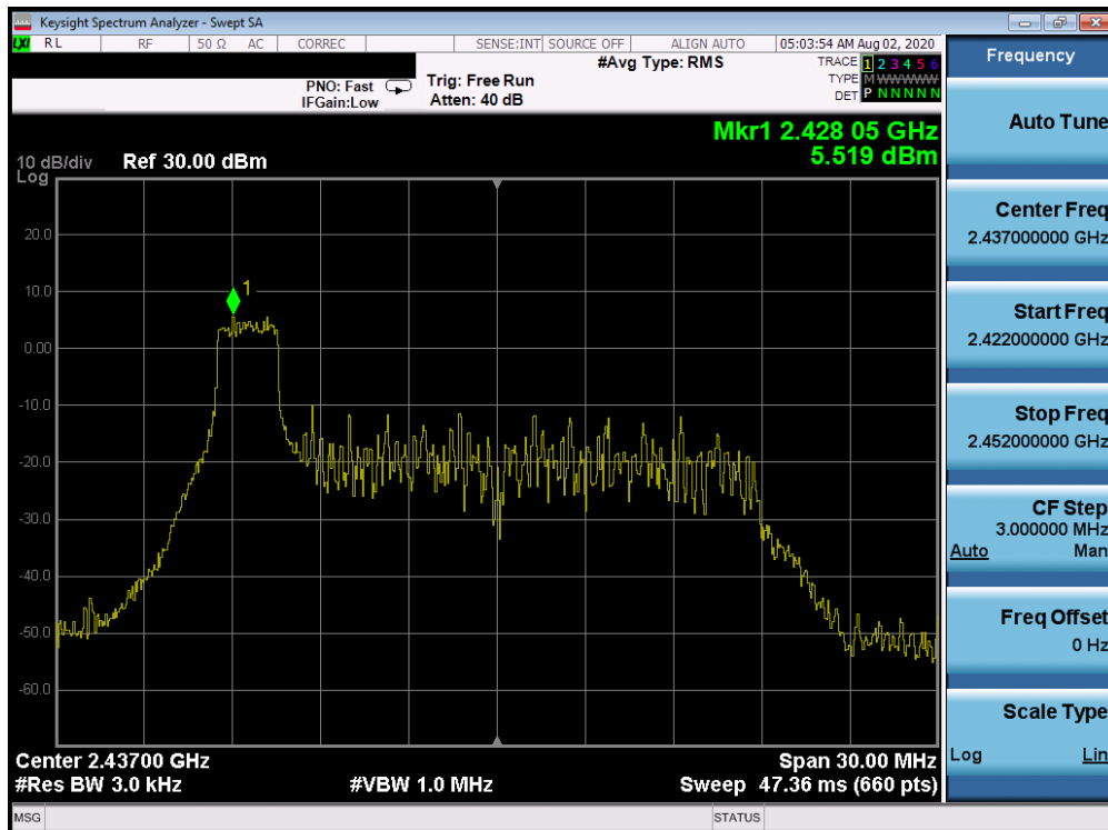
Plot 7-28. Power Spectral Density Plot ANT WF8 (802.11ax OFDMA – RU26 Index 0 – Ch. 6)
