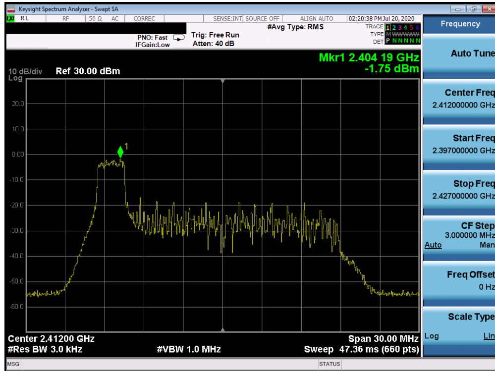
Plot 7-49. Power Spectral Density Plot CDD ANT WF8 (802.11ax OFDMA – RU26 Index 0 – Ch. 1)
