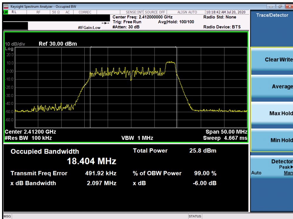
Plot 7-3. 6dB Bandwidth Plot ANT WF8 (802.11ax OFDMA – RU26 Index 8 – Ch. 1)
