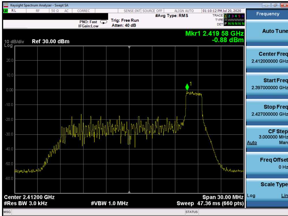
Plot 7-39. Power Spectral Density Plot ANT WF7b (802.11ax OFDMA – RU26 Index 8 – Ch. 1)
