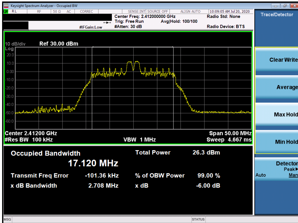
Plot 7-2. 6dB Bandwidth Plot ANT WF8 (802.11ax OFDMA – RU26 Index 4 – Ch. 1)
