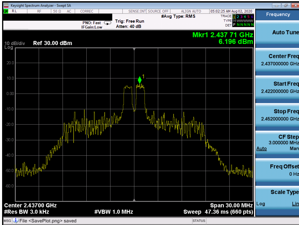
Plot 7-29. Power Spectral Density Plot ANT WF8 (802.11ax OFDMA – RU26 Index 4 – Ch. 6)
