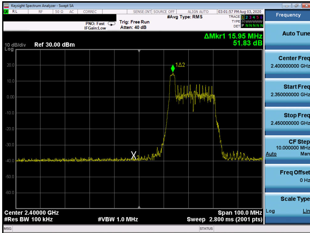
Plot 7-75. Band Edge ANT WF8 (802.11ax OFDMA – RU26 Index 0 – Ch. 3)
