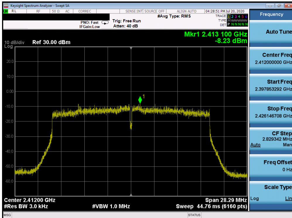
Plot 7-34. Power Spectral Density Plot ANT WF8 (802.11ax OFDMA – RU242 – Ch. 1)
