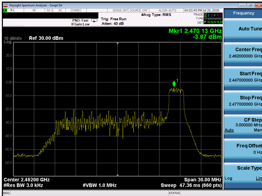
Plot 7-66. Power Spectral Density Plot CDD ANT WF7b (802.11ax OFDMA – RU26 Index 8 – Ch. 11)
