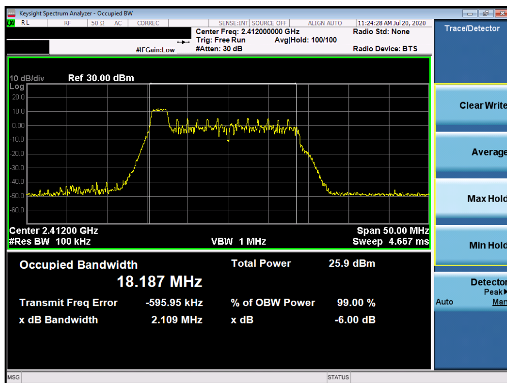
Plot 7-13. 6dB Bandwidth Plot ANT WF7b (802.11ax OFDMA – RU26 Index 0 – Ch. 1)
