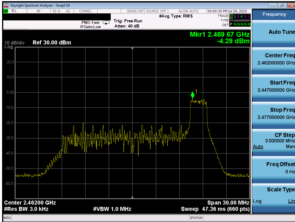
Plot 7-65. Power Spectral Density Plot CDD ANT WF8 (802.11ax OFDMA – RU26 Index 8 – Ch. 11)
