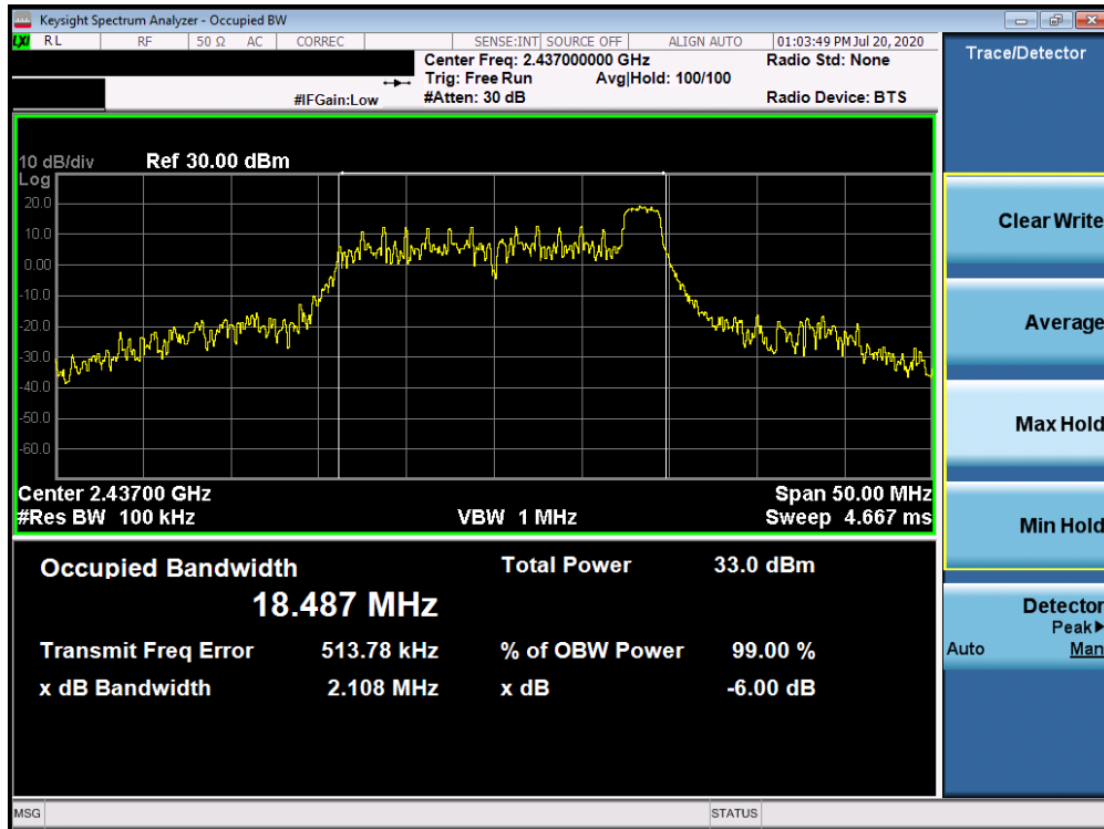
Plot 7-18. 6dB Bandwidth Plot ANT WF7b (802.11ax OFDMA – RU26 Index 8 – Ch. 6)
