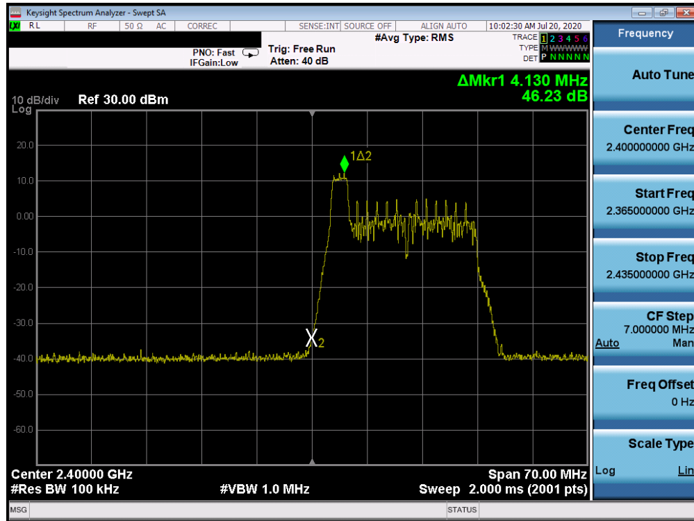
Plot 7-73. Band Edge ANT WF8 (802.11ax OFDMA – RU26 Index 0 – Ch. 1)
