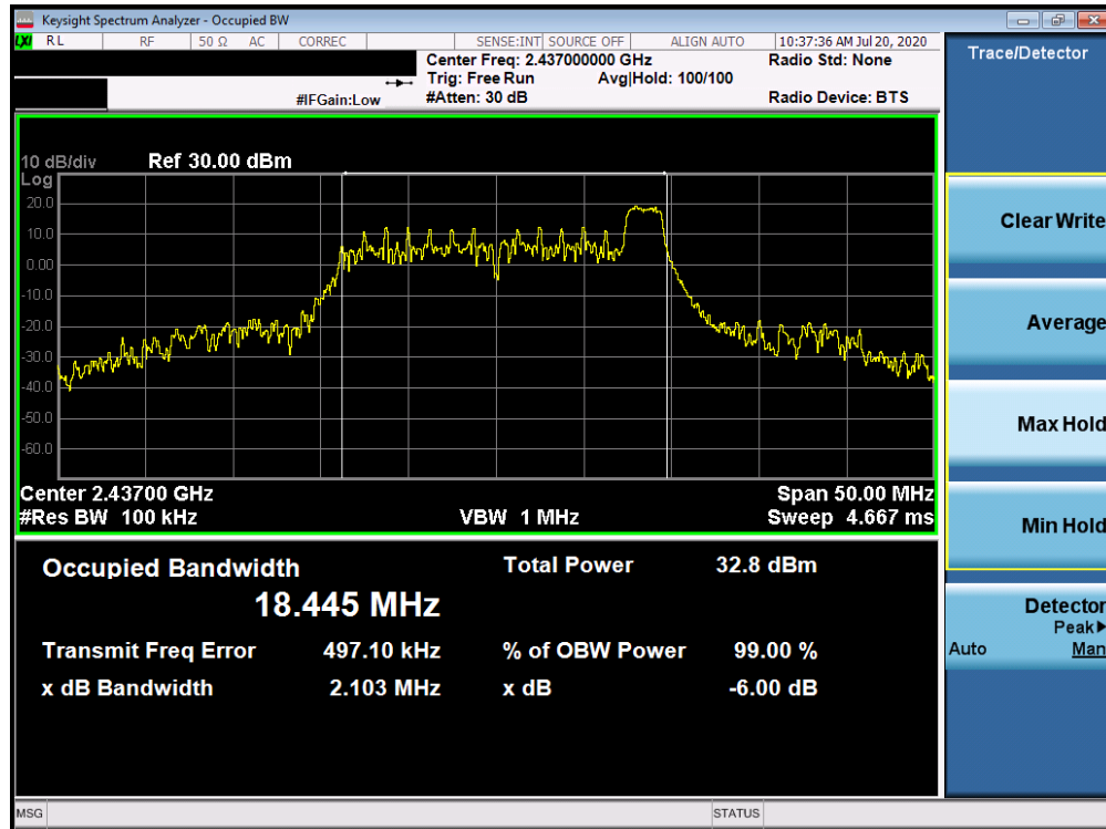
Plot 7-6. 6dB Bandwidth Plot ANT WF8 (802.11ax OFDMA – RU26 Index 8 – Ch. 6)
