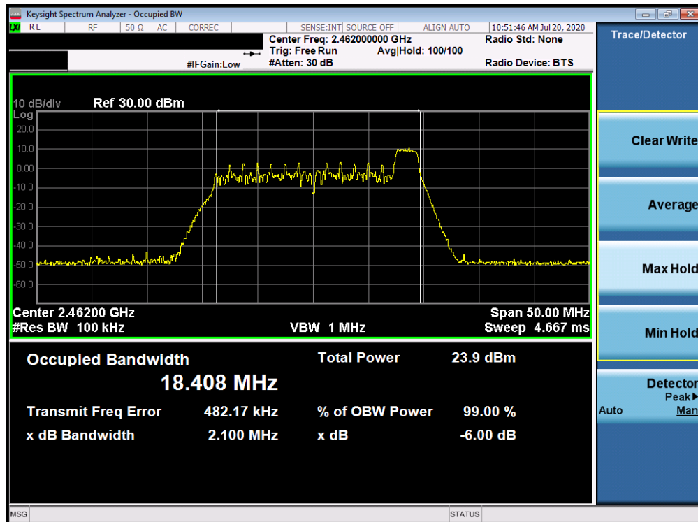
Plot 7-9. 6dB Bandwidth Plot ANT WF8 (802.11ax OFDMA – RU26 Index 8 – Ch. 11)
