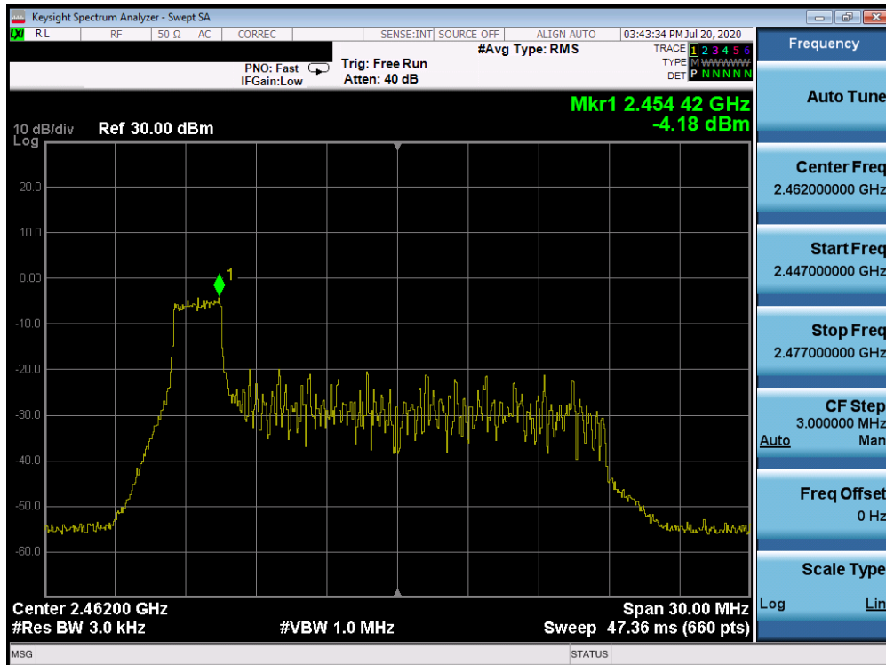
Plot 7-62. Power Spectral Density Plot CDD ANT WF7b (802.11ax OFDMA – RU26 Index 0 – Ch. 11)
