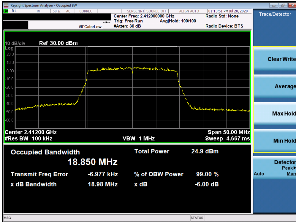
Plot 7-22. 6dB Bandwidth Plot ANT WF7b (802.11ax OFDMA – RU242 – Ch. 1)
