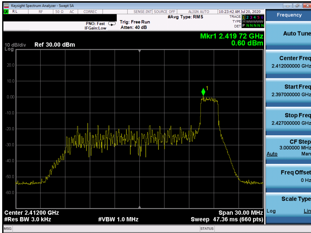
Plot 7-27. Power Spectral Density Plot ANT WF8 (802.11ax OFDMA – RU26 Index 8 – Ch. 1)
