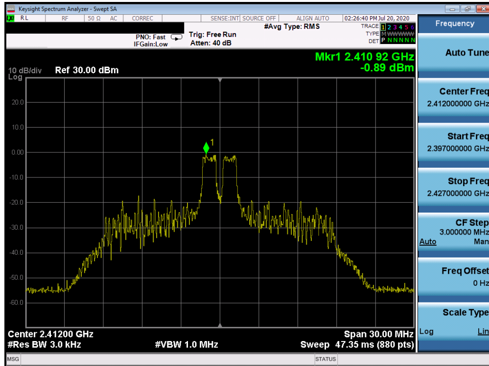
Plot 7-51. Power Spectral Density Plot CDD ANT WF8 (802.11ax OFDMA – RU26 Index 4 – Ch. 1)
