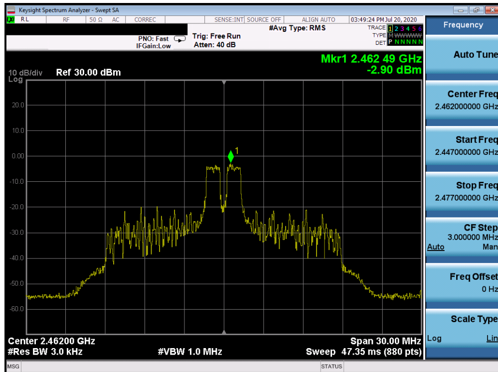
Plot 7-64. Power Spectral Density Plot CDD ANT WF7b (802.11ax OFDMA – RU26 Index 4 – Ch. 11)
