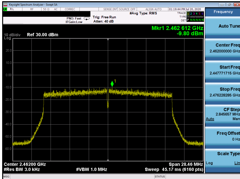
Plot 7-48. Power Spectral Density Plot ANT WF7b (802.11ax OFDMA – RU242 – Ch. 11)
