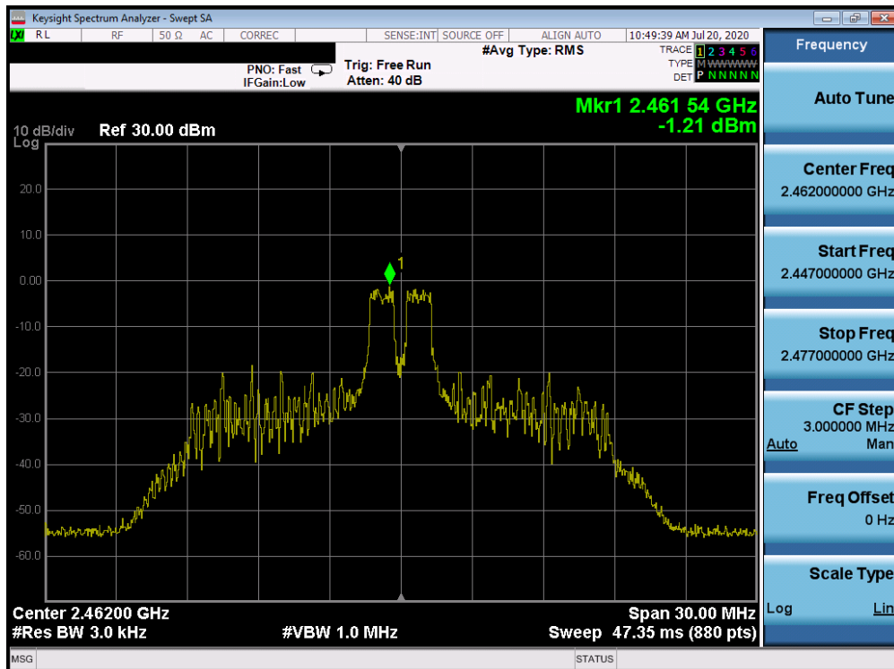
Plot 7-32. Power Spectral Density Plot ANT WF8 (802.11ax OFDMA – RU26 Index 4 – Ch. 11)
