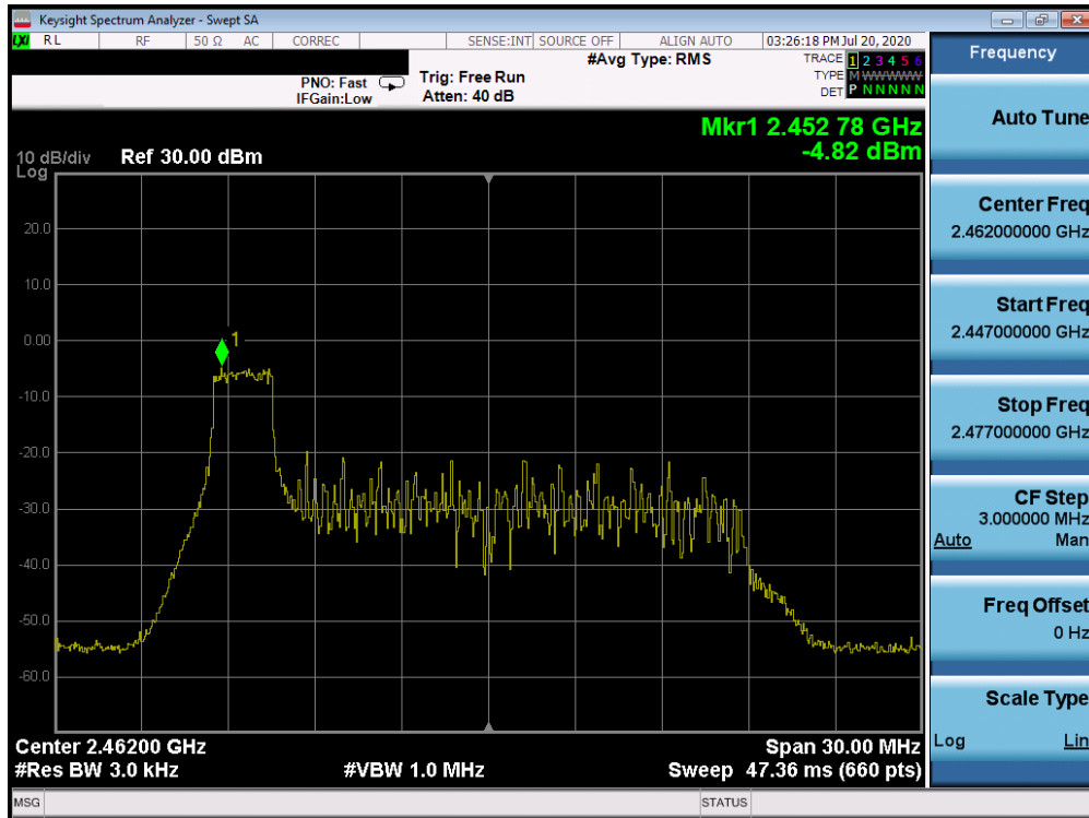
Plot 7-61. Power Spectral Density Plot CDD ANT WF8 (802.11ax OFDMA – RU26 Index 0 – Ch. 11)
