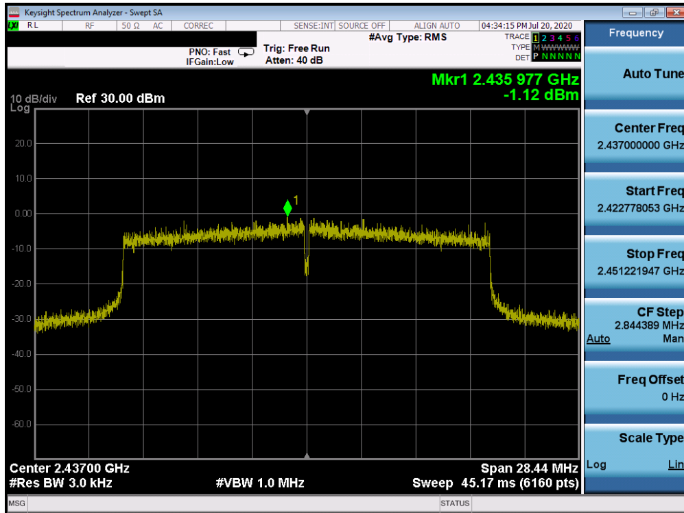
Plot 7-69. Power Spectral Density Plot CDD ANT WF8 (802.11ax OFDMA – RU242 – Ch. 6)
