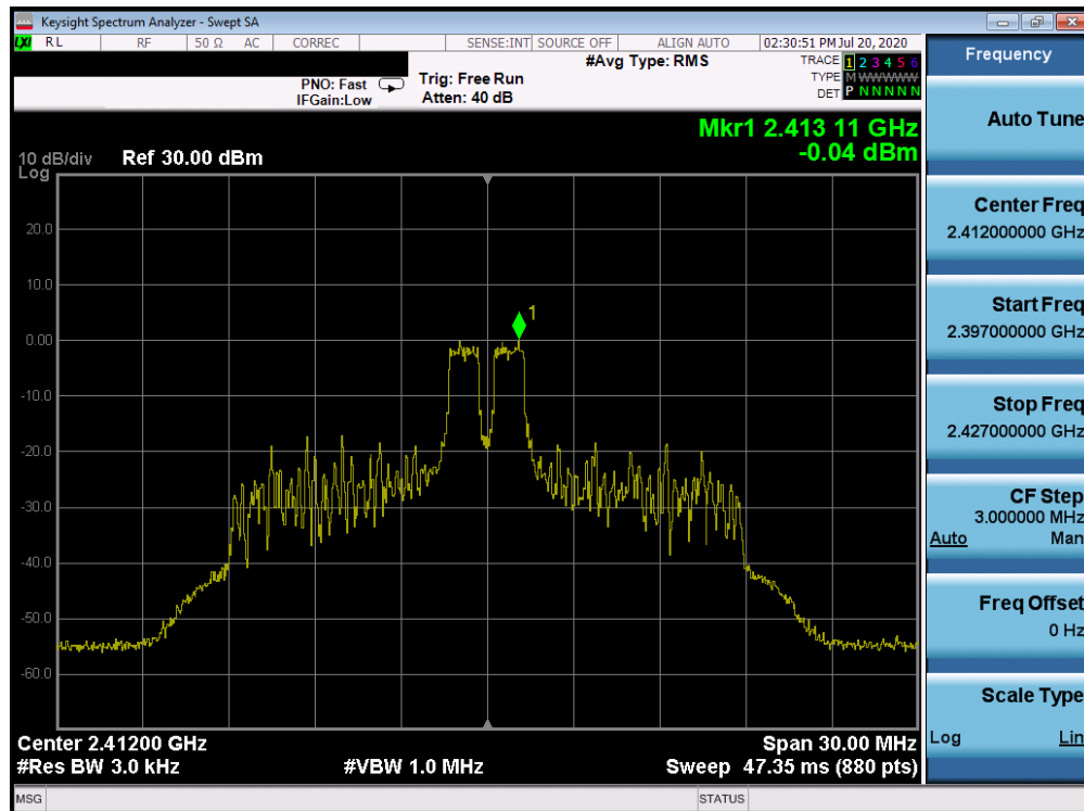
Plot 7-52. Power Spectral Density Plot CDD ANT WF7b (802.11ax OFDMA – RU26 Index 4 – Ch. 1)
