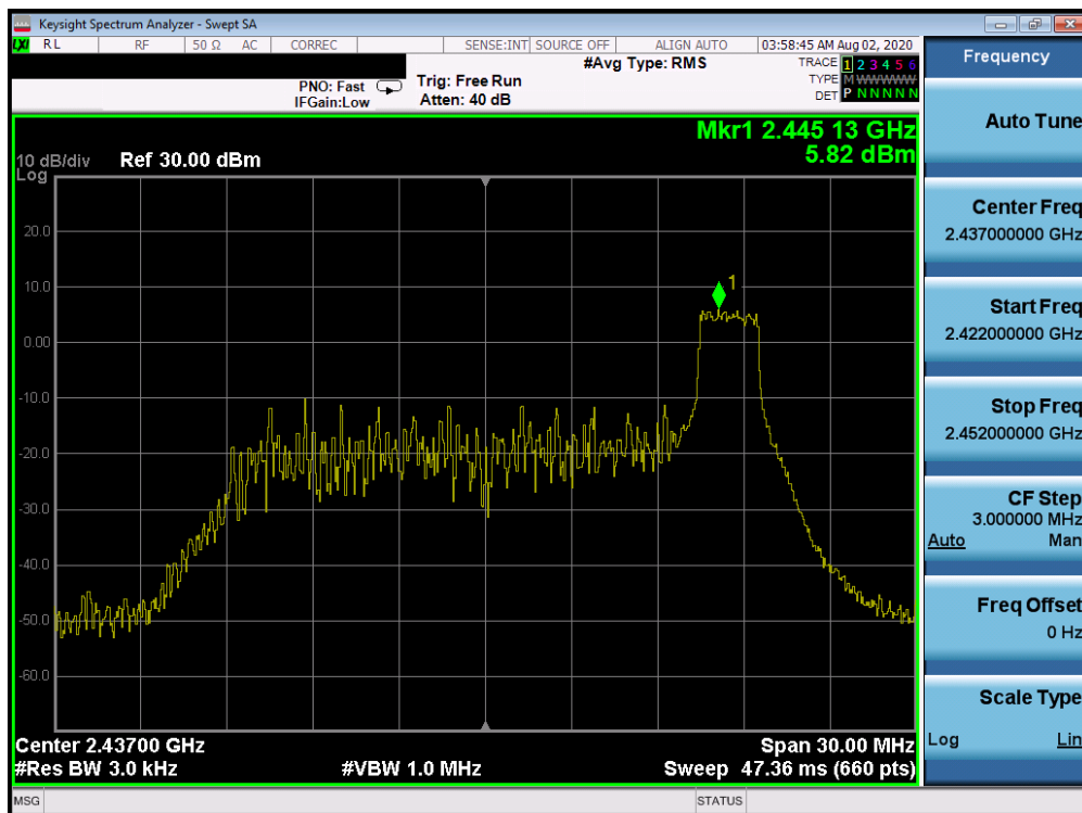
Plot 7-30. Power Spectral Density Plot ANT WF8 (802.11ax OFDMA – RU26 Index 8 – Ch. 6)
