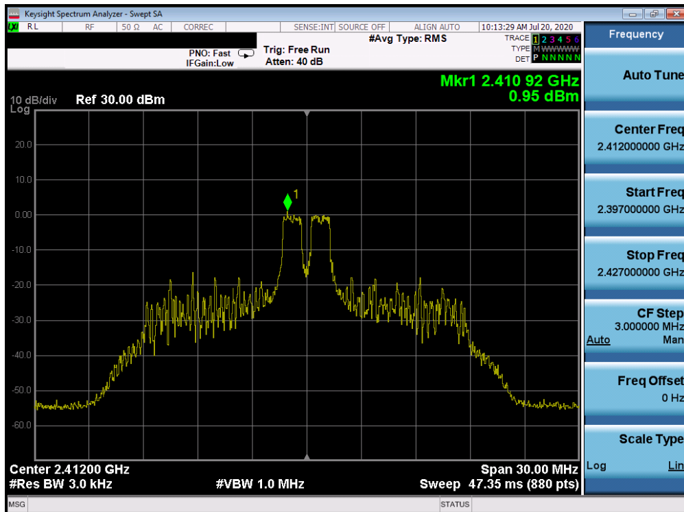
Plot 7-26. Power Spectral Density Plot ANT WF8 (802.11ax OFDMA – RU26 Index 4 – Ch. 1)
