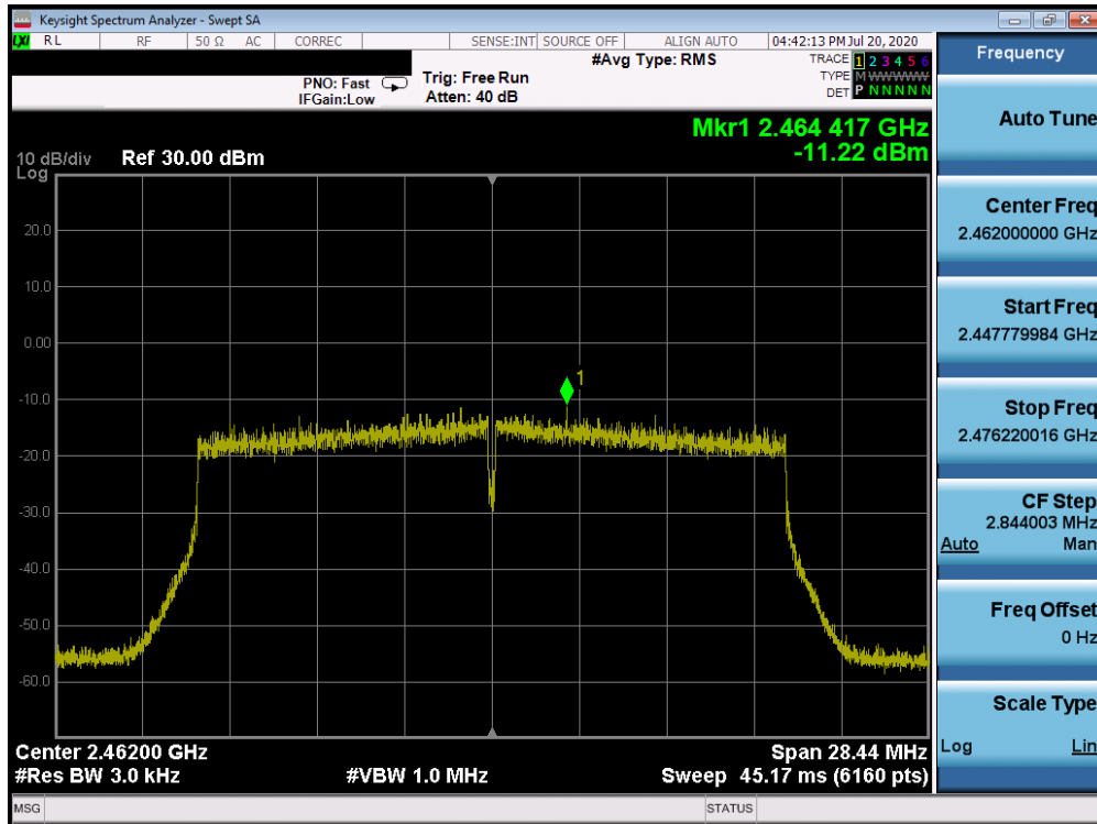
Plot 7-71. Power Spectral Density Plot CDD ANT WF8 (802.11ax OFDMA – RU242 – Ch. 11)
