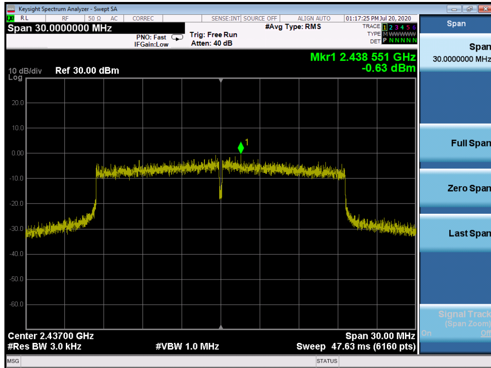
Plot 7-47. Power Spectral Density Plot ANT WF7b (802.11ax OFDMA – RU242 – Ch. 6)
