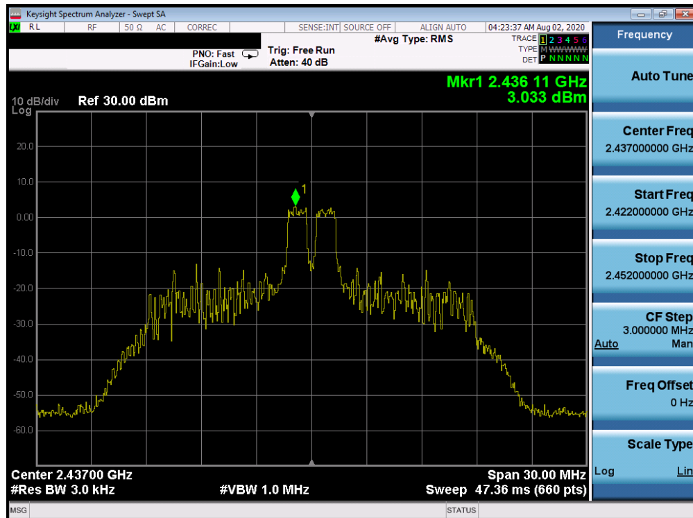
Plot 7-58. Power Spectral Density Plot CDD ANT WF7b (802.11ax OFDMA – RU26 Index 4 – Ch. 6)
