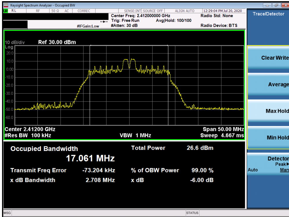
Plot 7-14. 6dB Bandwidth Plot ANT WF7b (802.11ax OFDMA – RU26 Index 4 – Ch. 1)
