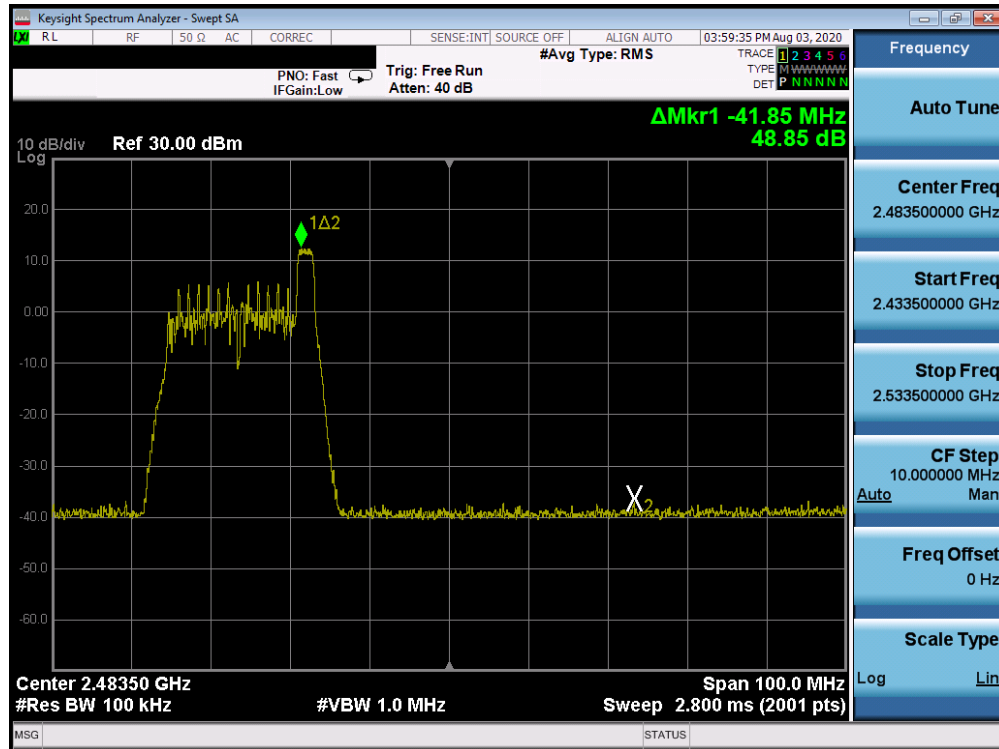
Plot 7-81. Band Edge ANT WF8 (802.11ax OFDMA – RU26 Index 8 – Ch. 10)
