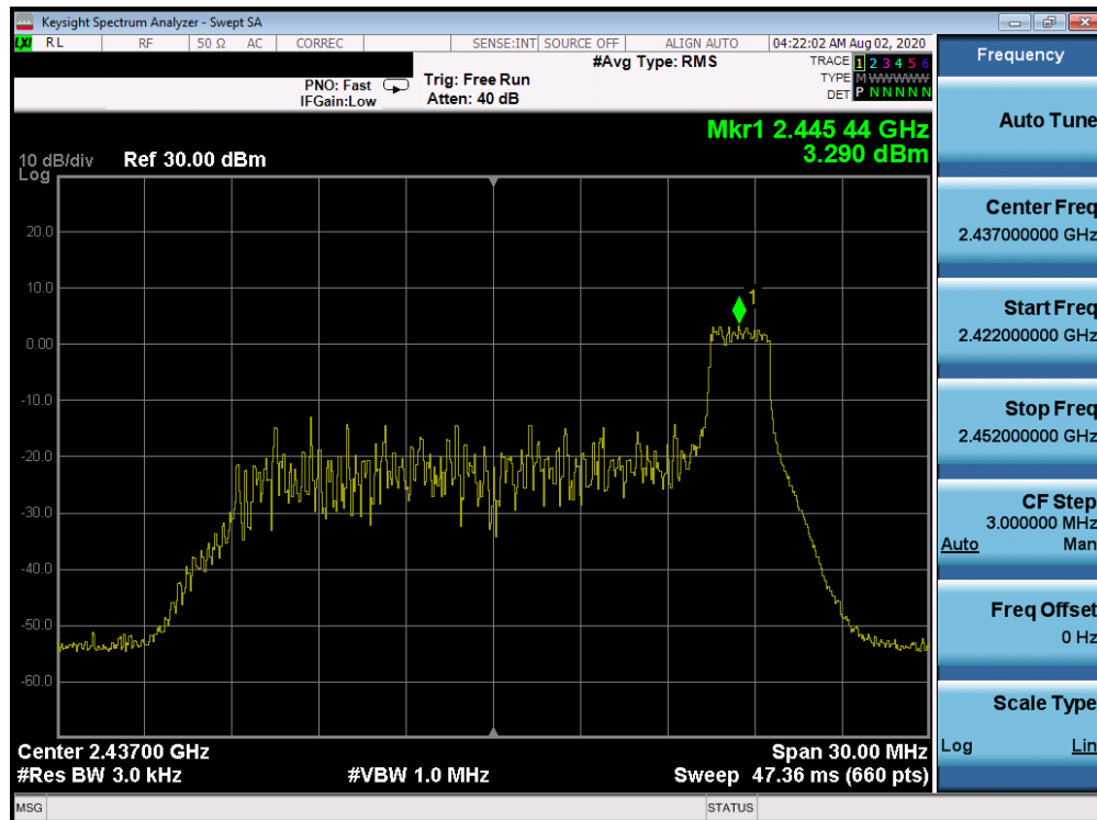
Plot 7-60. Power Spectral Density Plot CDD ANT WF7b (802.11ax OFDMA – RU26 Index 8 – Ch. 6)
