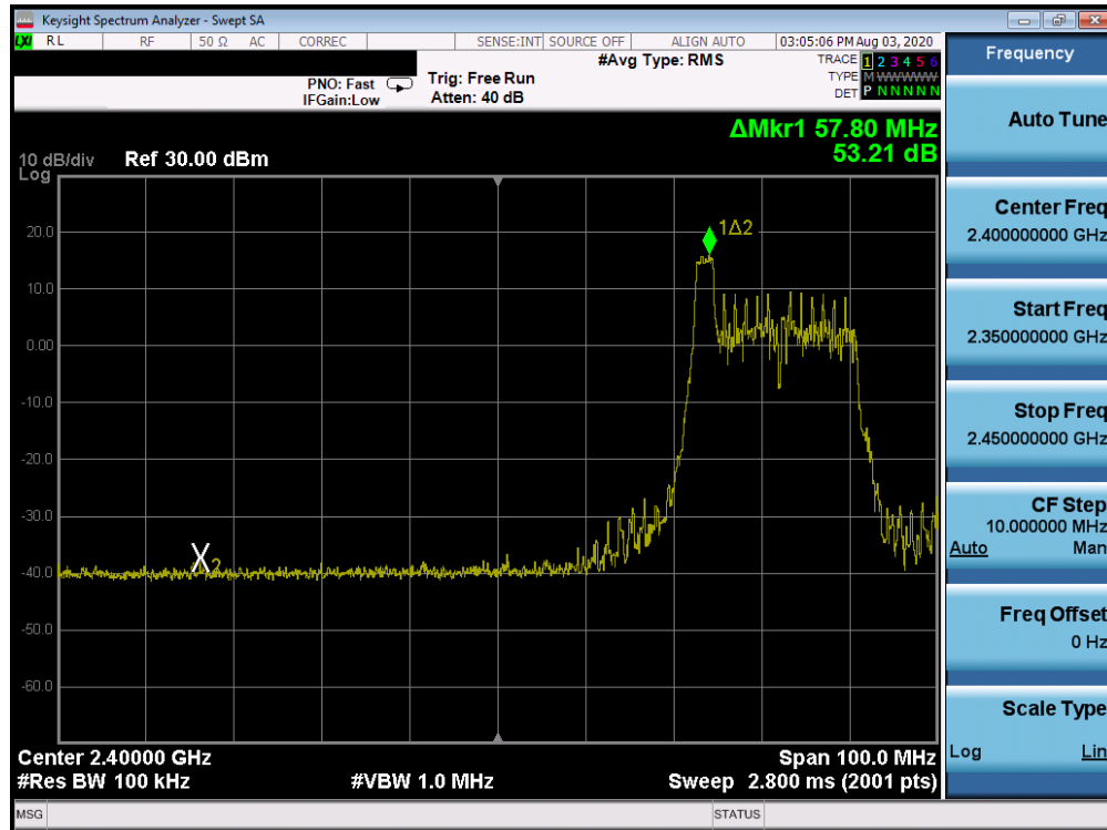
Plot 7-77. Band Edge ANT WF8 (802.11ax OFDMA – RU26 Index 0 – Ch. 5)
