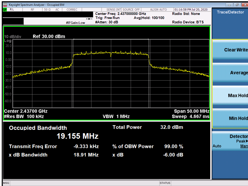
Plot 7-23. 6dB Bandwidth Plot ANT WF7b (802.11ax OFDMA – RU242 – Ch. 6)
