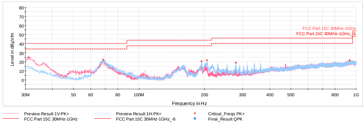
Plot 7-181. Radiated Spurious Emissions below 1GHz CDD Ch.6, with AC/DC Adapter
