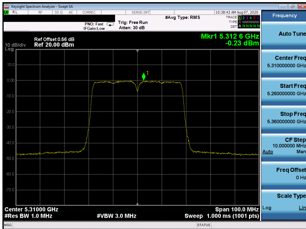
Plot 7-95. Power Spectral Density Plot ANT WF7a (40MHz BW 802.11n (UNII Band 2A) – Ch. 62)
