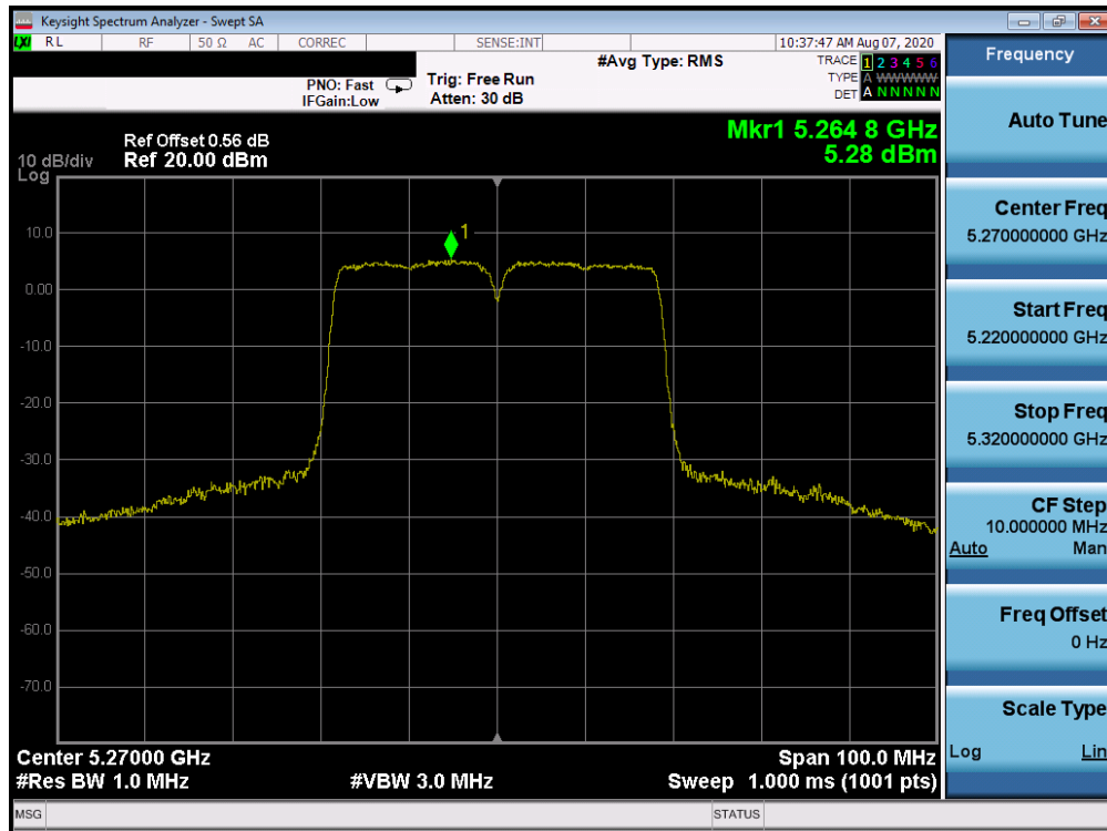
Plot 7-94. Power Spectral Density Plot ANT WF7a (40MHz BW 802.11n (UNII Band 2A) – Ch. 54)
