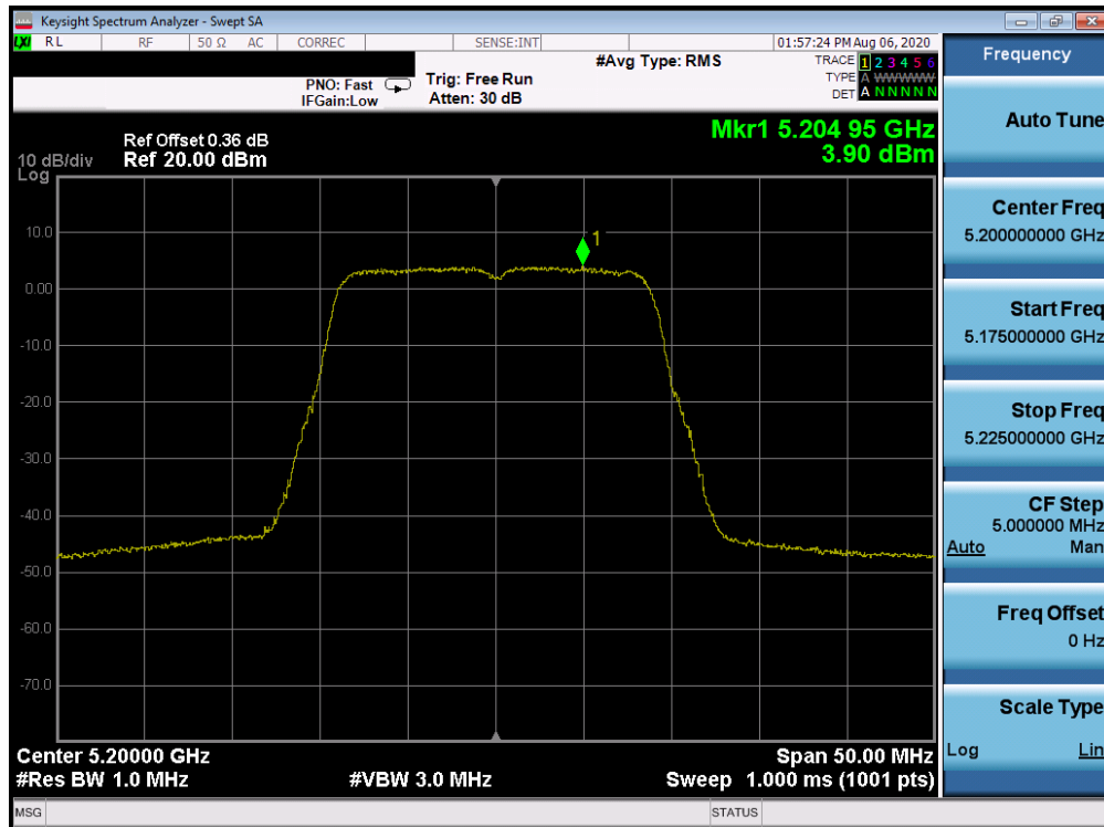
Plot 7-56. ISED Power Spectral Density Plot ANT WF8 (20MHz BW 802.11n (UNII Band 1) – Ch. 40)
