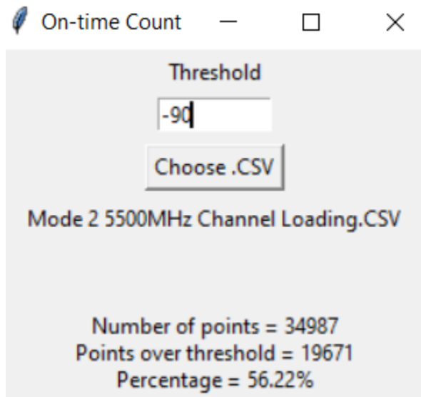
Figure 9-8. 5500MHz - Channel Loading Calculation - Mode 2 (20MHz)
