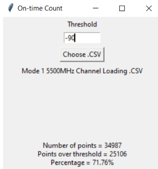
Figure 9-2. 5500MHz - Channel Loading Calculation - Mode 1 (20MHz)
