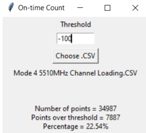
Figure 9-22. 5510MHz - Channel Loading Calculation - Mode 4 (40MHz)
