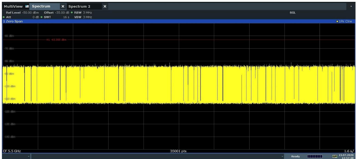
Figure 9-1. 5500MHz - Channel Loading - Mode 1 (20MHz)
