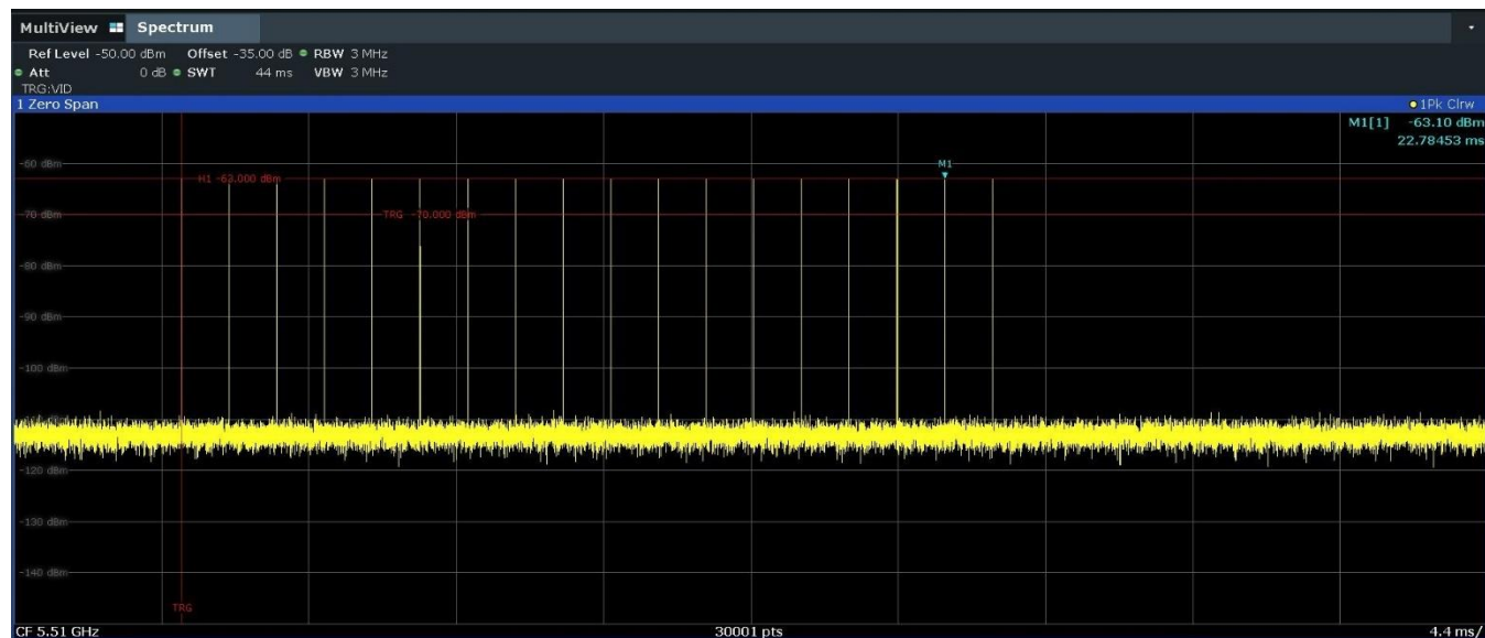
Figure 7-4. 5510MHz – Radar Pulse Type 0 (40MHz)
