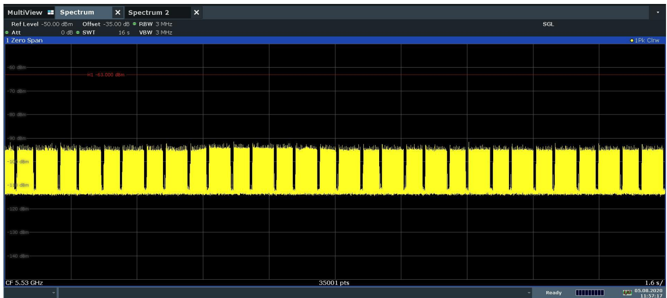
Figure 9-23. 5530MHz - Channel Loading - Mode 4 (80MHz)
