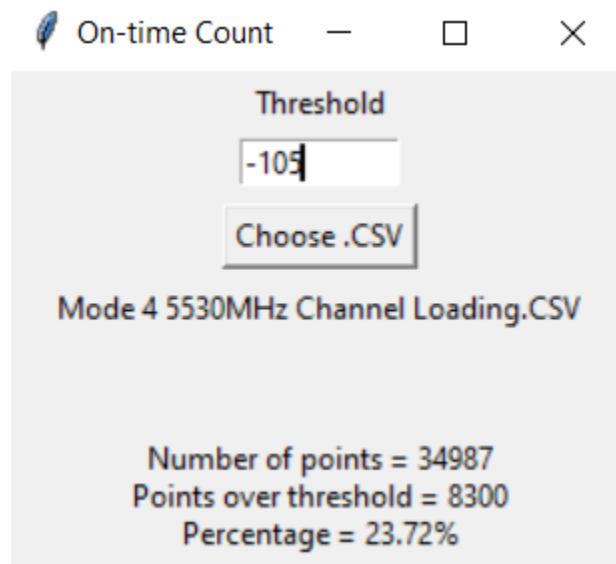
Figure 9-24. 5530MHz - Channel Loading Calculation - Mode 4 (80MHz)
