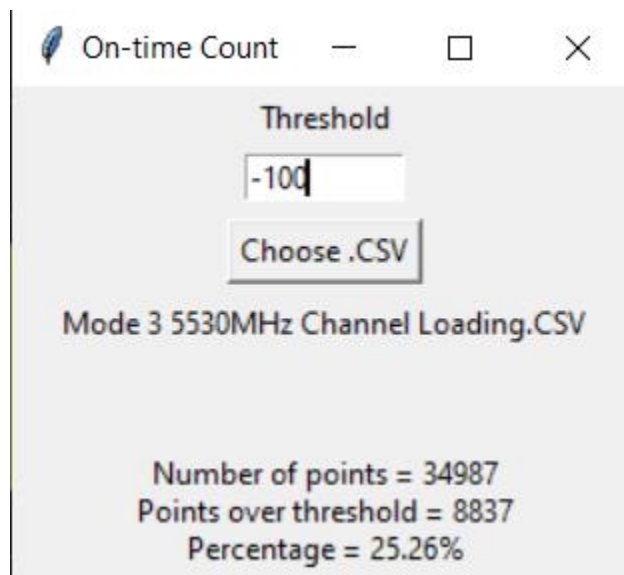
Figure 9-18. 5530MHz - Channel Loading Calculation - Mode 3 (80MHz)
