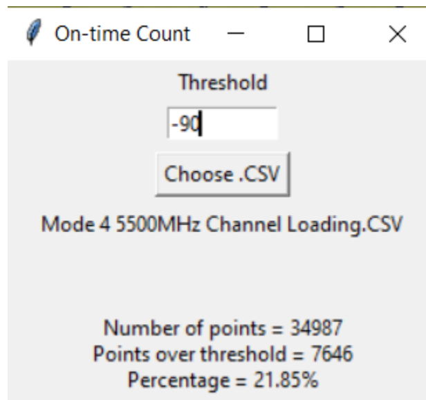
Figure 9-20. 5500MHz - Channel Loading Calculation - Mode 4 (20MHz)
