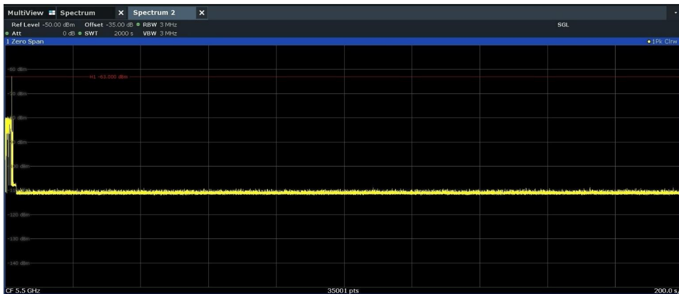
Figure 9-40. 5500MHz - Non-Occupancy Period (30 Minutes) - Mode 2 (20MHz)
