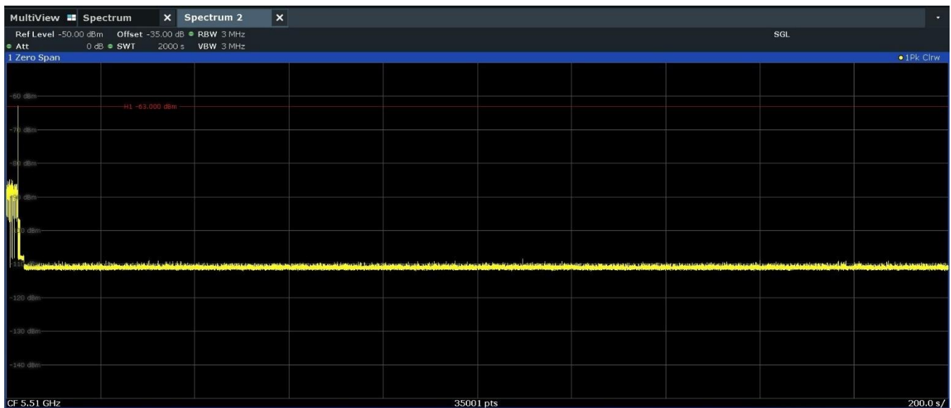
Figure 9-44. 5510MHz - Non-Occupancy Period (30 Minutes) - Mode 3 (40MHz)
