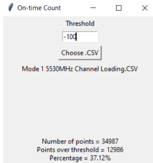
Figure 9-6. 5530MHz - Channel Loading Calculation - Mode 1 (80MHz)
