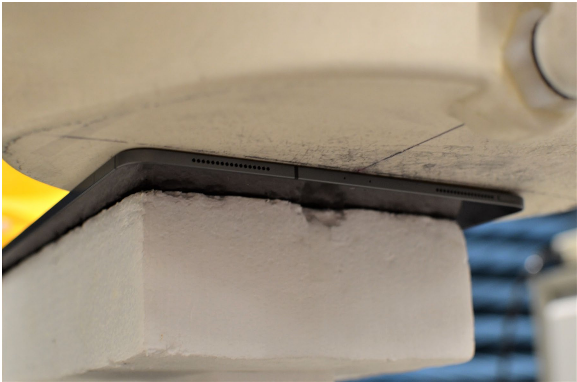
SAR Test Setup Photo 2: Back Side at 0.0 cm – 5GHz ANTupper
