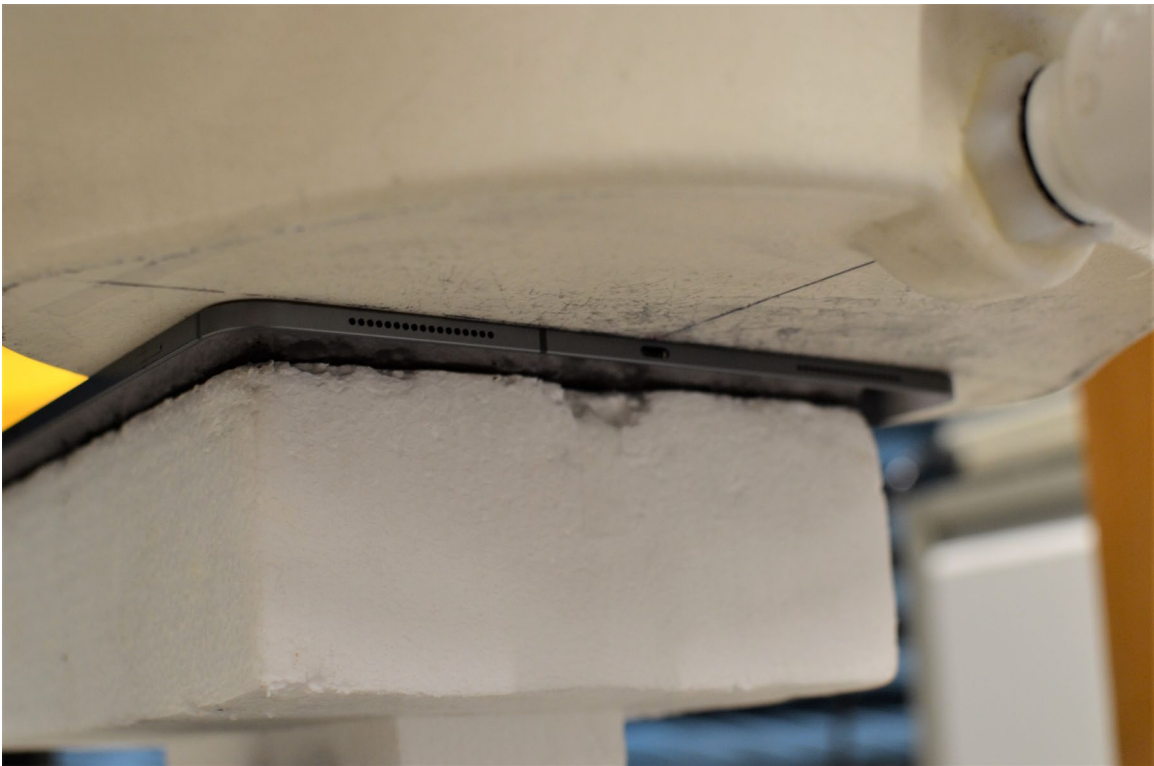
SAR Test Setup Photo 4: Back Side at 0.0 cm – 5GHz ANTlower
