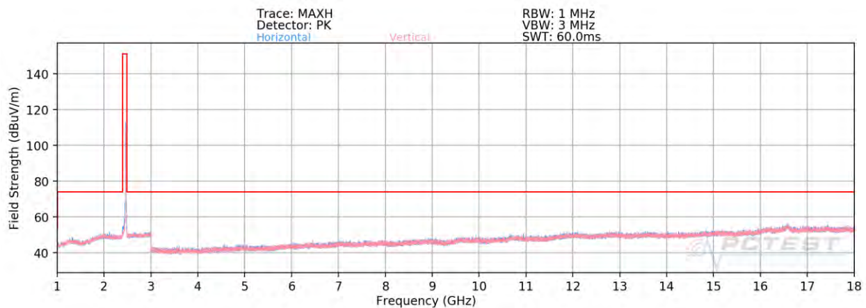
Plot 7-86. Radiated Spurious Plot above 1GHz SISO CORE 0 (802.11b – Ch. 11)
