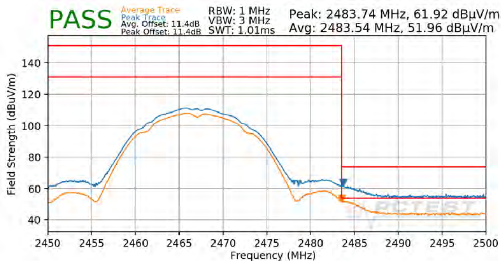
Plot 7-96. Radiated Restricted Upper Band Edge Measurement SISO CORE0
