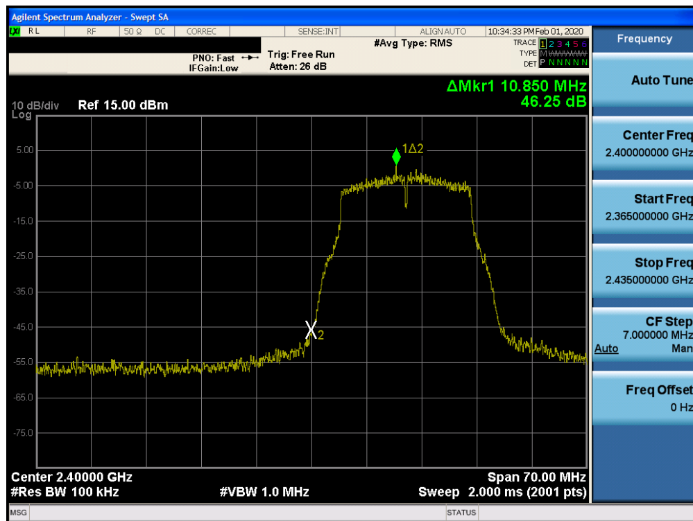
Plot 7-64. Band Edge Plot SISO CORE 1 (802.11g- Ch. 1)
