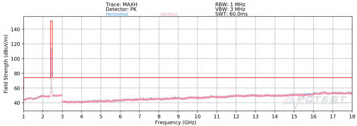
Plot 7-91. Radiated Spurious Plot above 1GHz CDD (802.11n – Ch. 6)
