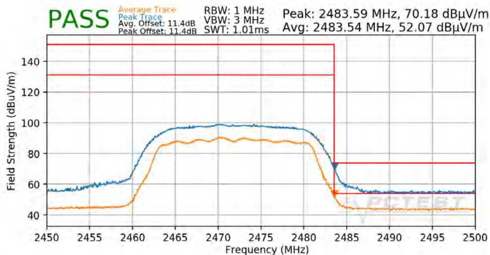
Plot 7-113. Radiated Restricted Upper Band Edge Measurement CDD
