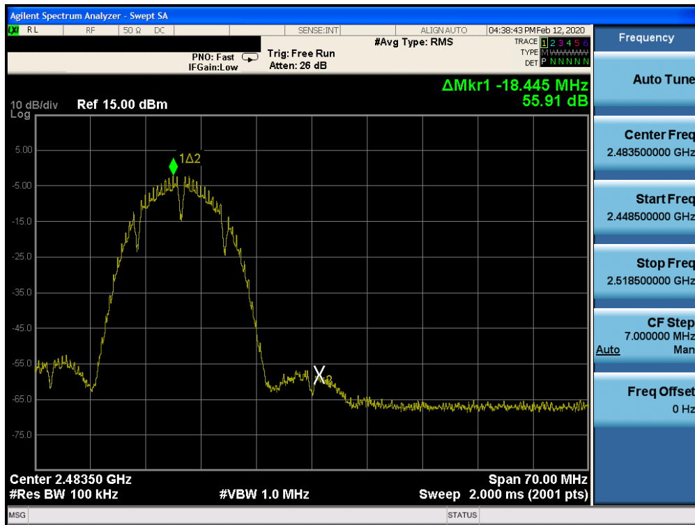
Plot 7-63. Band Edge Plot SISO CORE 1 (802.11b – Ch. 13)
