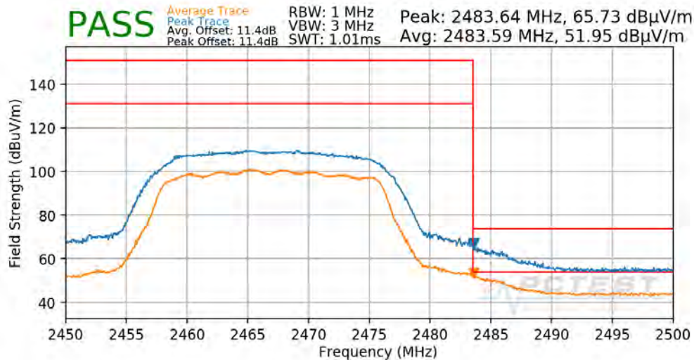
Plot 7-112. Radiated Restricted Upper Band Edge Measurement CDD
