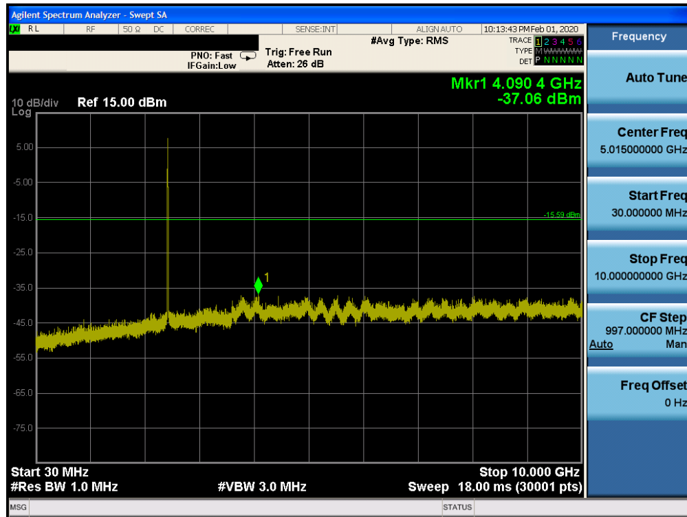
Plot 7-74. Conducted Spurious Plot SISO CORE0 (802.11b – Ch. 6)
