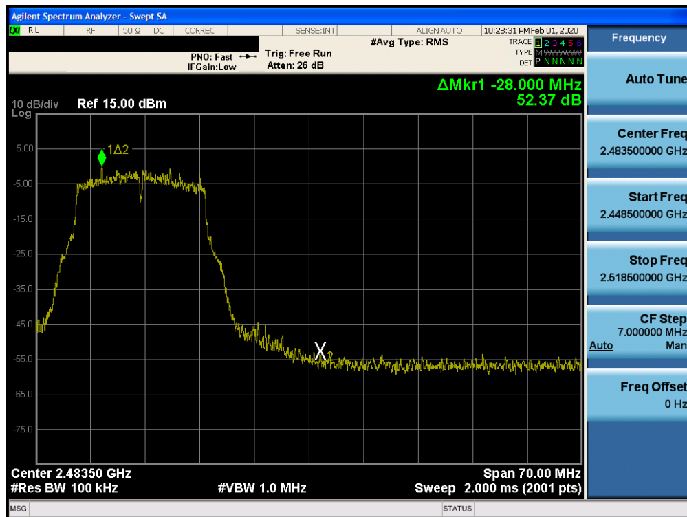
Plot 7-65. Band Edge Plot SISO CORE 1 (802.11g – Ch. 11)
