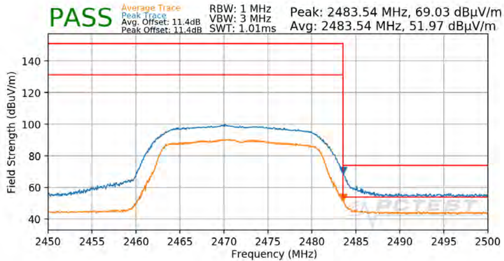
Plot 7-108. Radiated Restricted Upper Band Edge Measurement SISO CORE 1
