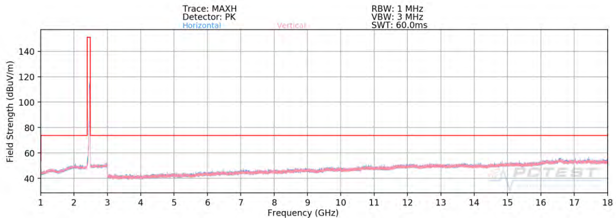
Plot 7-92. Radiated Spurious Plot above 1GHz CDD (802.11n – Ch. 11)
