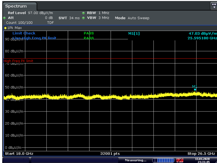
Plot 7-93. Radiated Spurious Plot above 18GHz CDD (802.11n, Pol. H)
