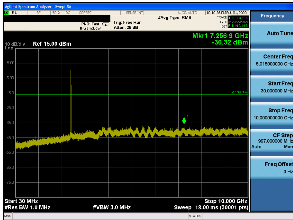
Plot 7-72. Conducted Spurious Plot SISO CORE0 (802.11b – Ch. 1)
