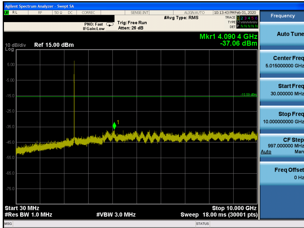
Plot 7-80. Conducted Spurious Plot SISO CORE1 (802.11b – Ch. 6)
