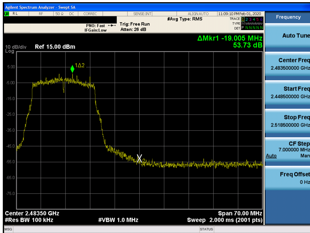
Plot 7-69. Band Edge Plot SISO CORE 1 (802.11n (2.4GHz) – Ch. 11)
