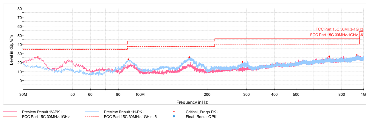
Plot 7-114. Radiated Spurious Plot below 1GHz CDD Ch.6, with AC/DC Adapter
