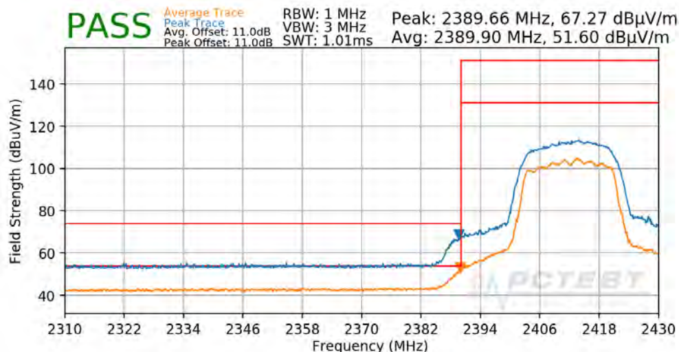
Plot 7-109. Radiated Restricted Lower Band Edge Measurement CDD
