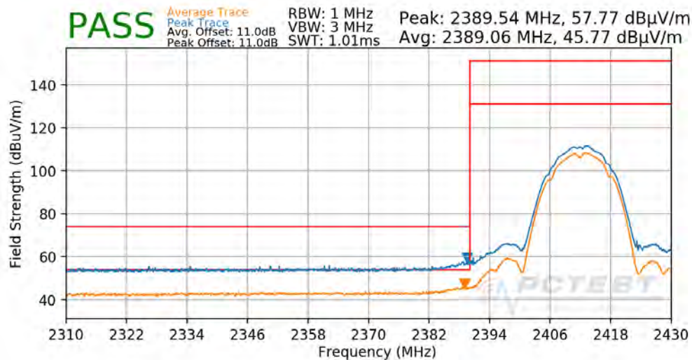
Plot 7-95. Radiated Restricted Lower Band Edge Measurement SISO CORE0
