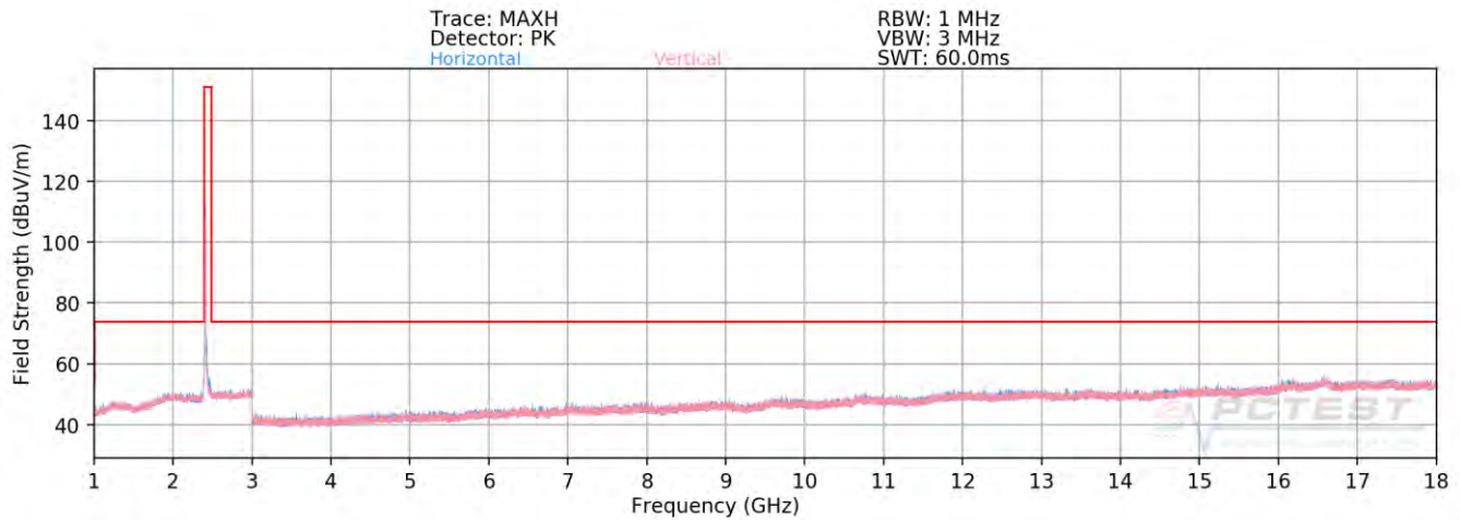
Plot 7-84. Radiated Spurious Plot above 1GHz SISO CORE 0 (802.11b – Ch. 1)
