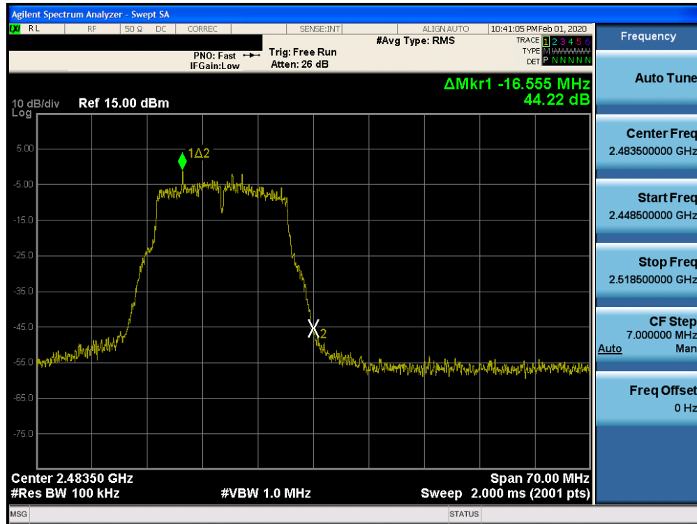
Plot 7-67. Band Edge Plot SISO CORE 1 (802.11g – Ch. 13)
