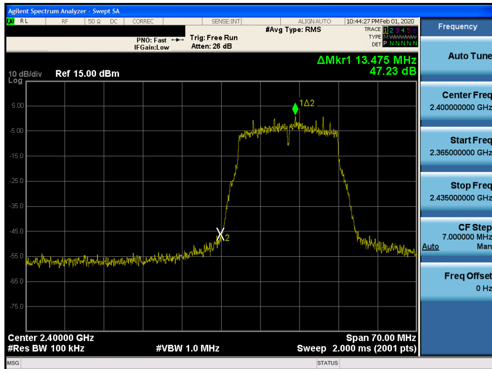
Plot 7-68. Band Edge Plot SISO CORE 1 (802.11n (2.4GHz) – Ch. 1)
