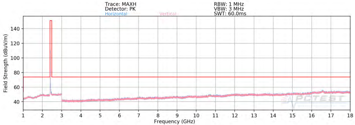
Plot 7-87. Radiated Spurious Plot above 1GHz SISO CORE 1 (802.11b – Ch. 1)
