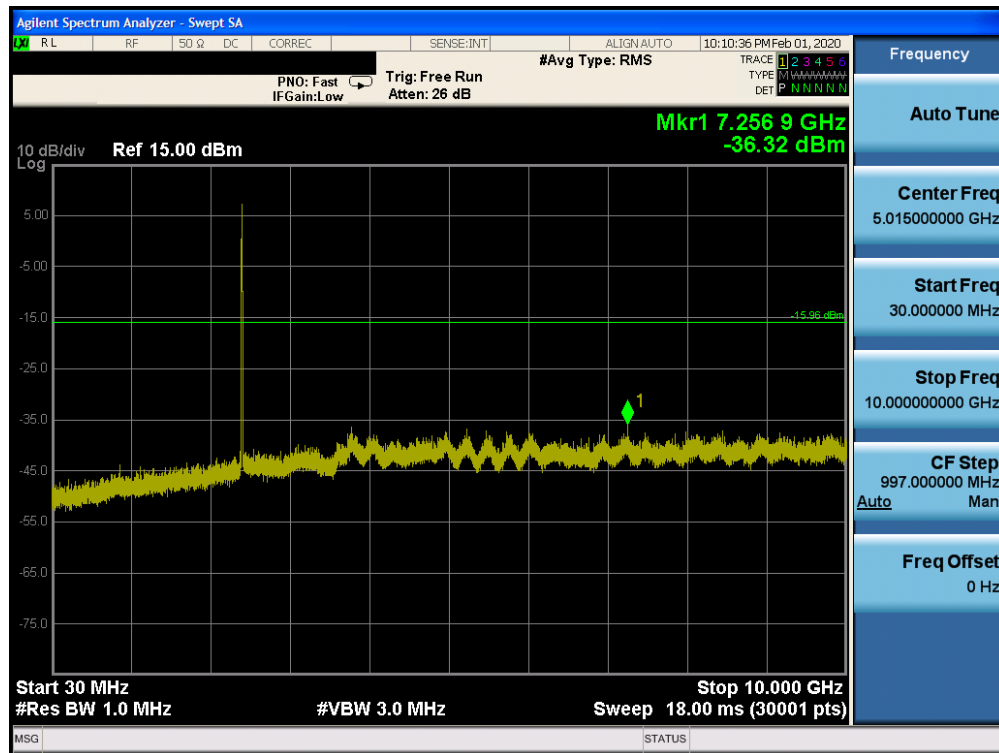
Plot 7-78. Conducted Spurious Plot SISO CORE1 (802.11b – Ch. 1)
