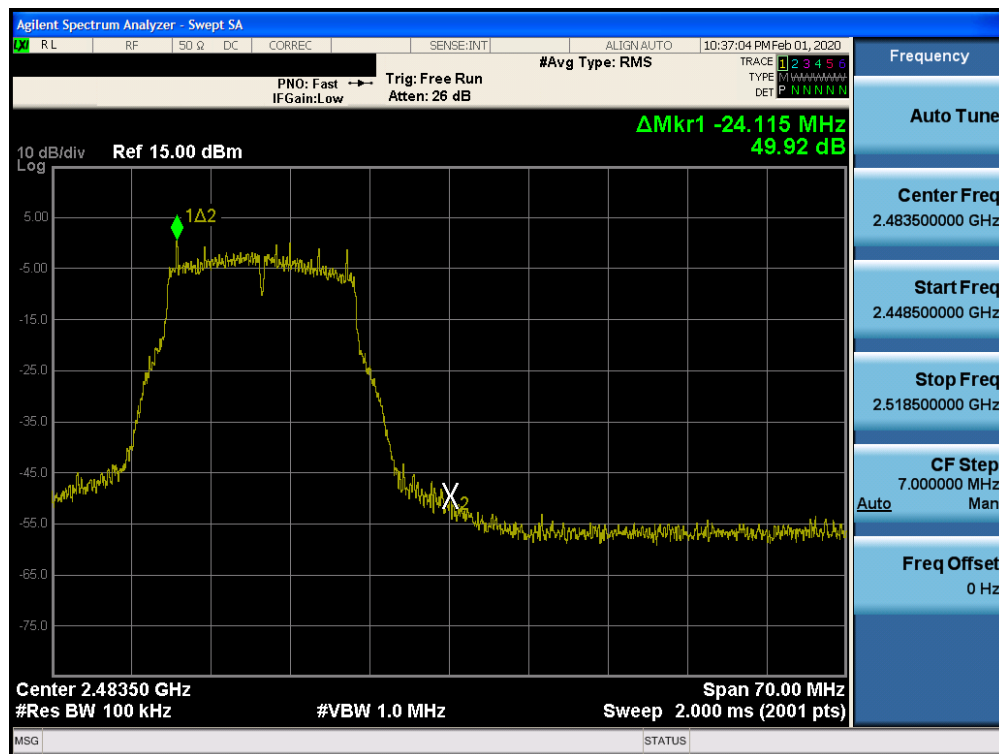
Plot 7-66. Band Edge Plot SISO CORE 1 (802.11g – Ch. 12)
