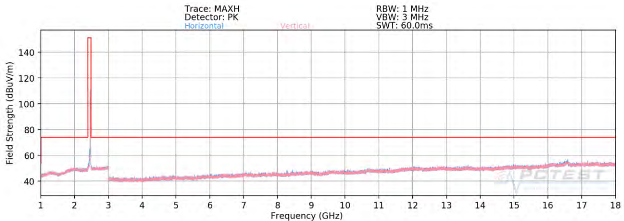
Plot 7-89. Radiated Spurious Plot above 1GHz SISO CORE 1 (802.11b – Ch. 11)
