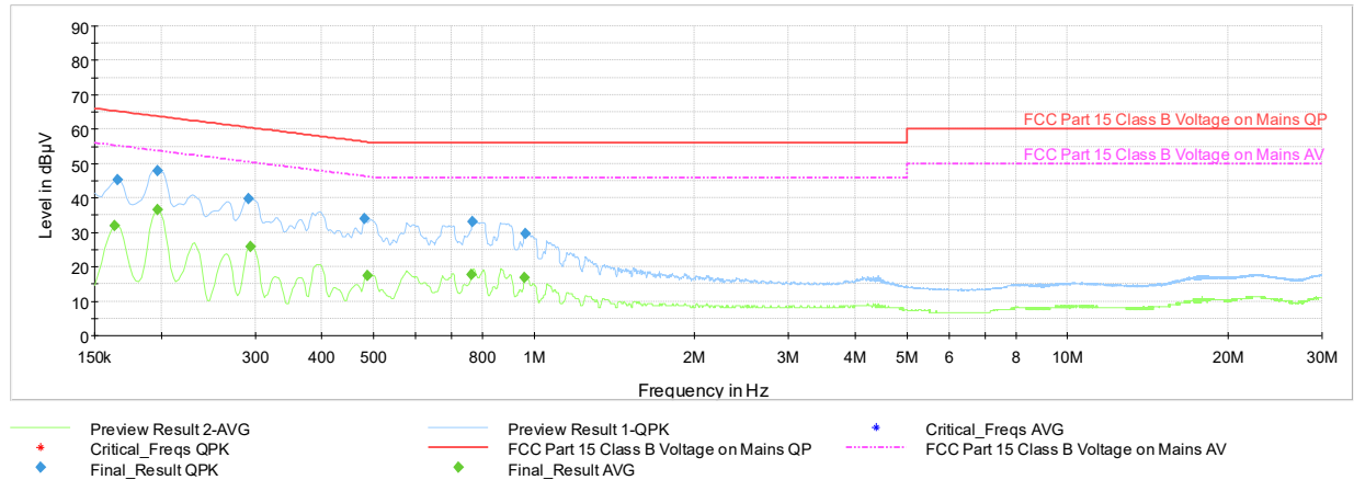
Plot 7-116. Line Conducted Plot with 802.11n CDD Ch.6 (N, with AC/DC Adapter)
