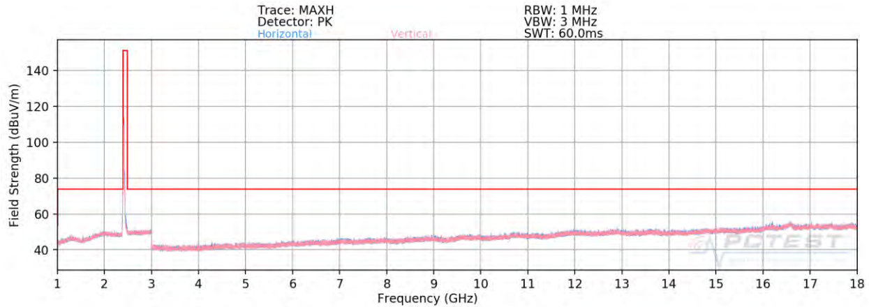
Plot 7-90. Radiated Spurious Plot above 1GHz CDD (802.11n – Ch. 1)
