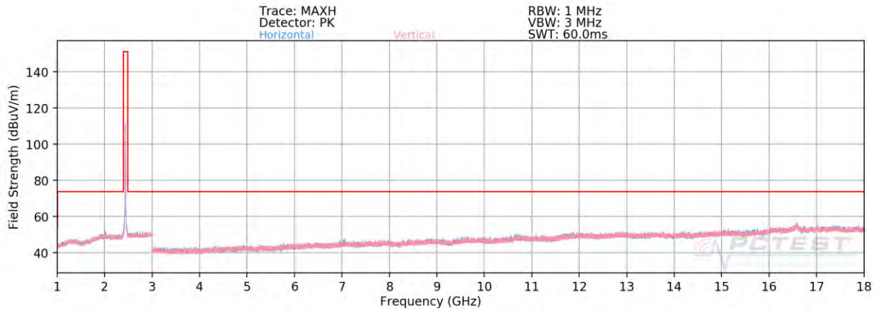
Plot 7-88. Radiated Spurious Plot above 1GHz SISO CORE 1 (802.11b – Ch. 6)
