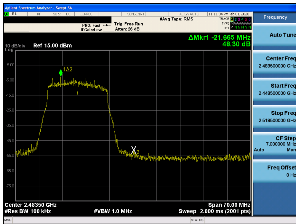
Plot 7-70. Band Edge Plot SISO CORE 1 (802.11n – Ch. 12)
