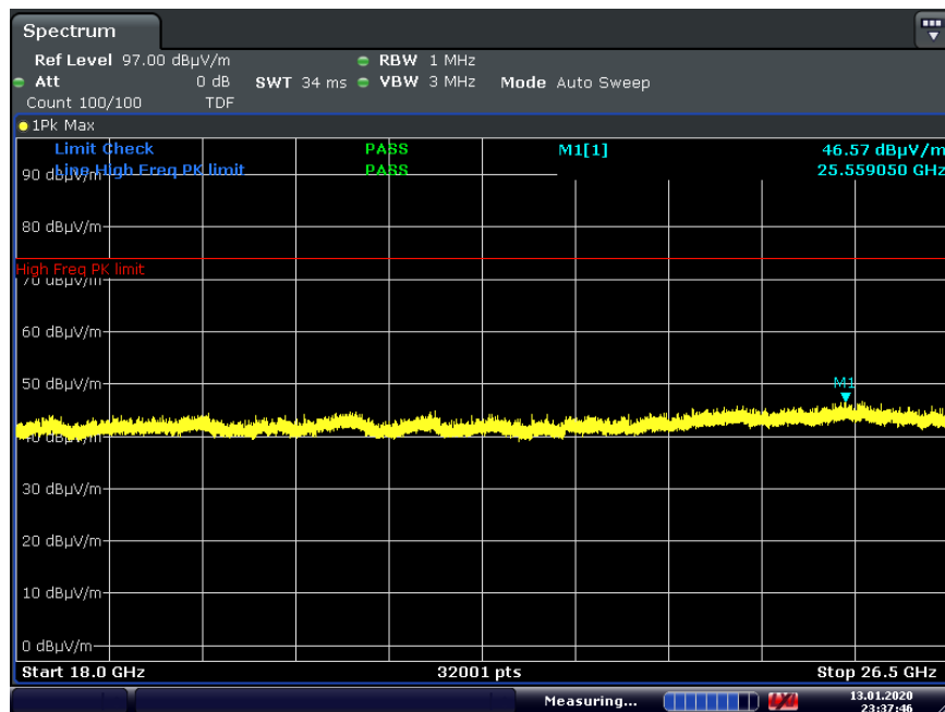
Plot 7-94. Radiated Spurious Plot above 18GHz CDD (802.11n, Pol. V)
