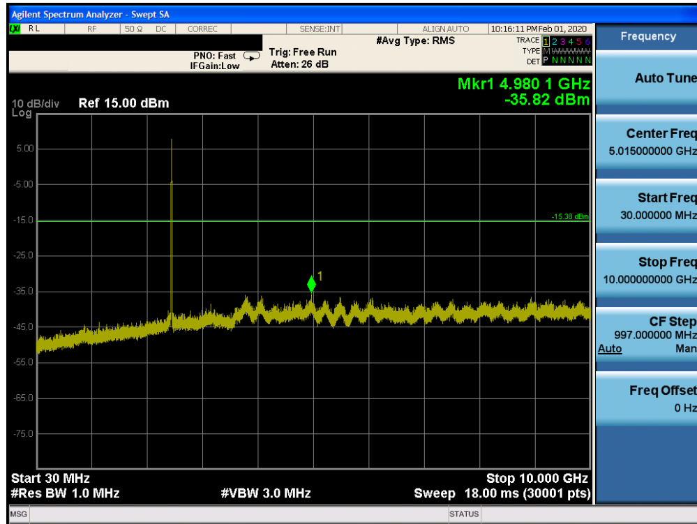
Plot 7-82. Conducted Spurious Plot SISO CORE1 (802.11b – Ch. 11)
