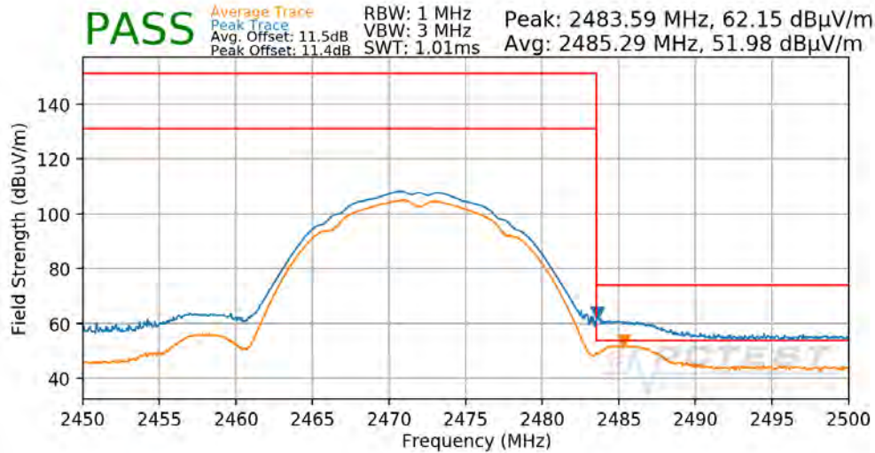
Plot 7-104. Radiated Restricted Upper Band Edge Measurement SISO CORE 1
