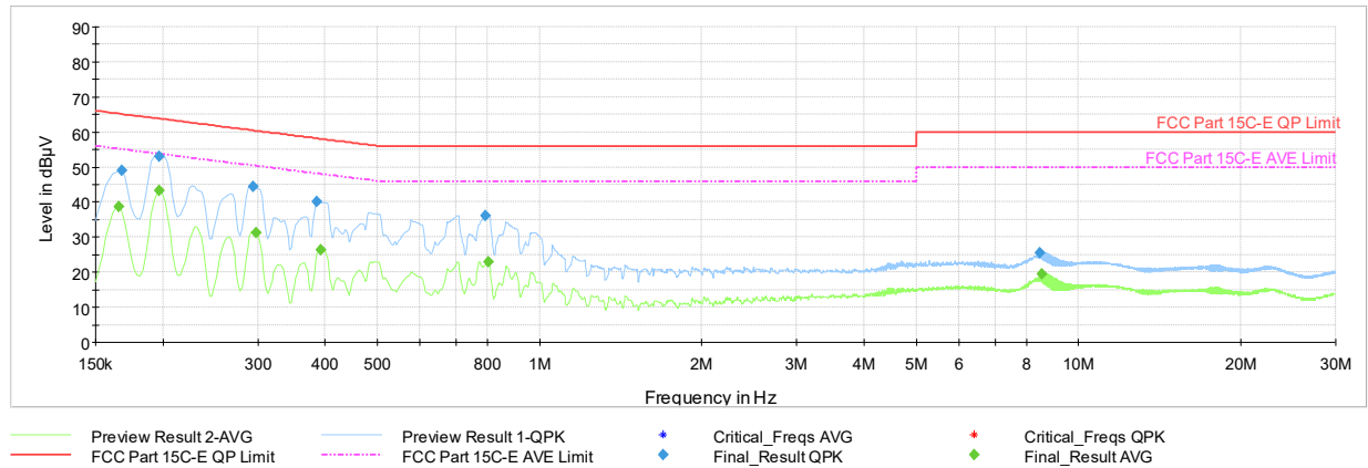
Plot 7-115. Line Conducted Plot with 802.11n CDD Ch.6 (L1, with AC/DC Adapter)
