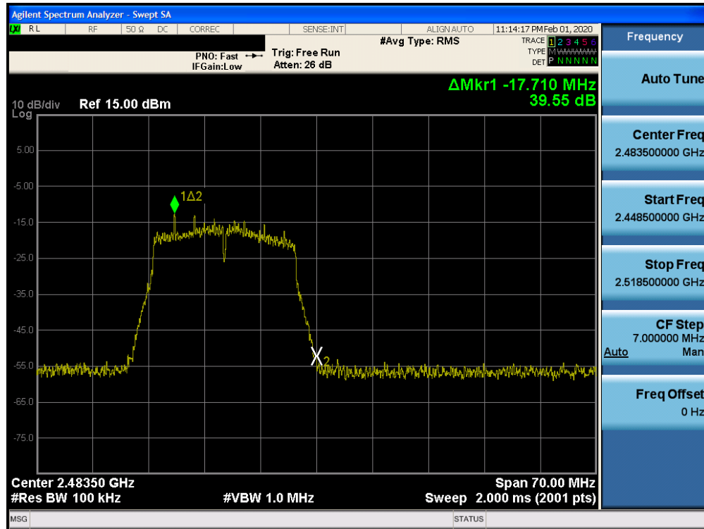
Plot 7-71. Band Edge Plot SISO CORE 1 (802.11n – Ch. 13)
