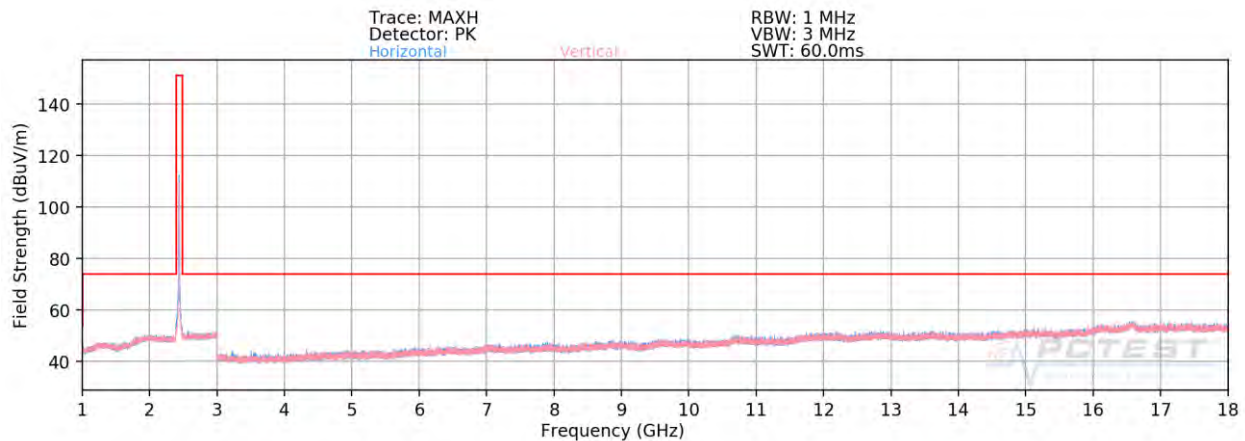
Plot 7-85. Radiated Spurious Plot above 1GHz SISO CORE 0 (802.11b – Ch. 6)
