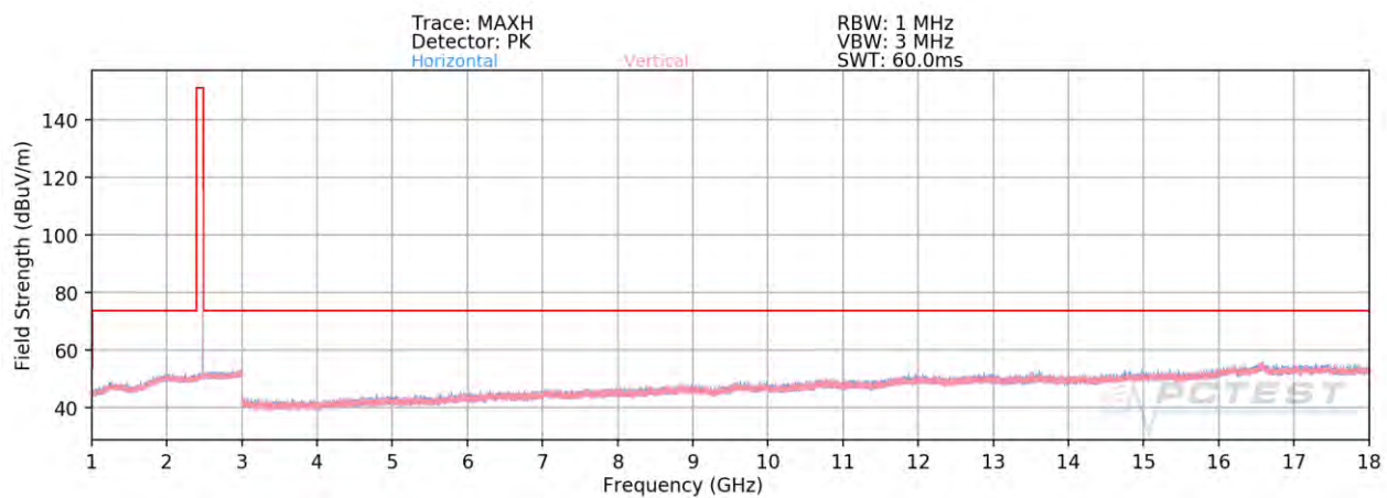
Plot 7-86. Radiated Spurious Plot Above 1GHz Ant 2a (1Mbps, ePA – Ch. 39)
