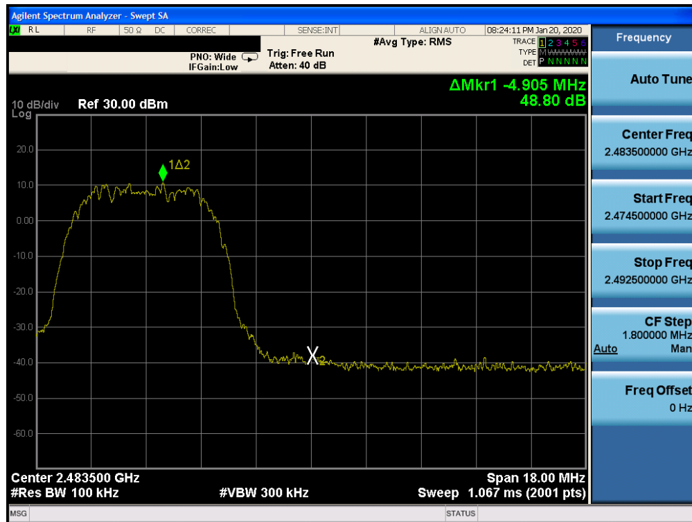
Plot 7-64. Band Edge Plot Ant WF8 (Bluetooth (HDR8), ePA – Ch. 75)
