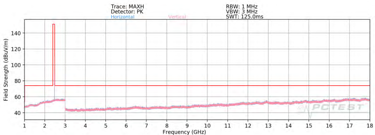
Plot 7-86. Radiated Spurious Plot Above 1GHz Ant WF7 (4Mbps, HDR4 ePA – Ch. 75, Ant. Pol. H & V)
