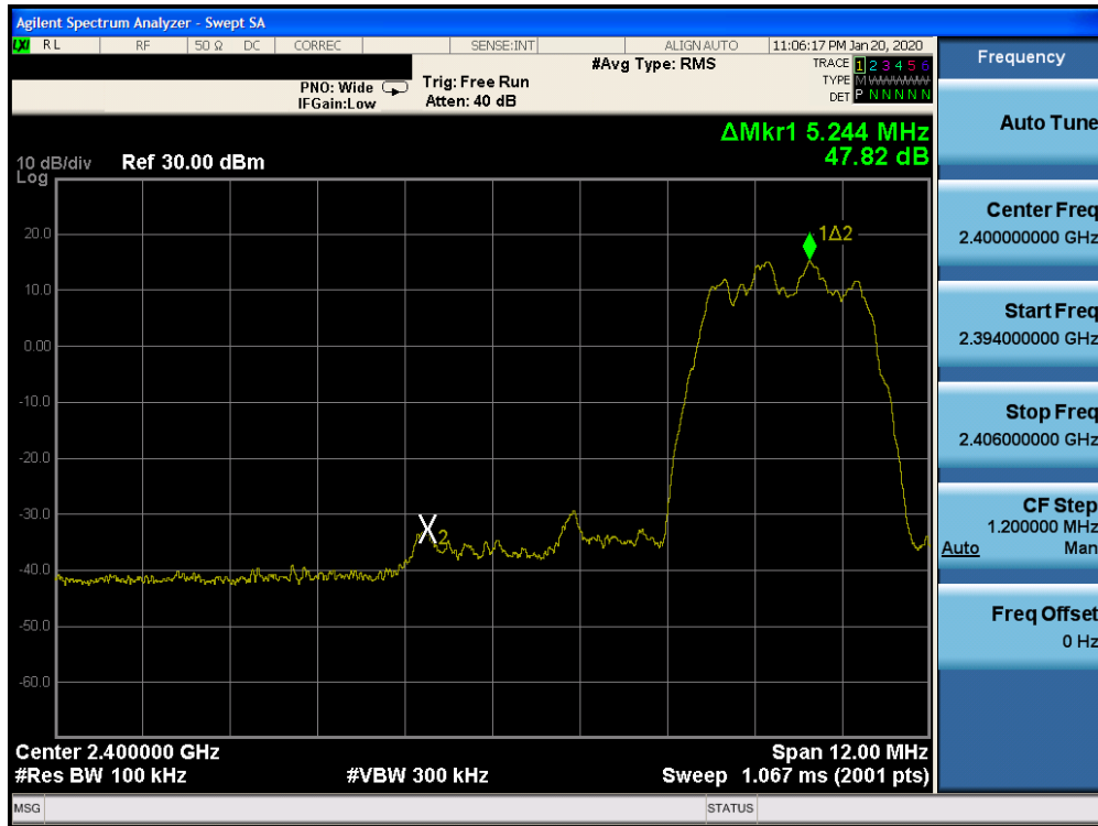
Plot 7-65. Band Edge Plot Ant WF7 (Bluetooth (HDR4), ePA – Ch. 1)
