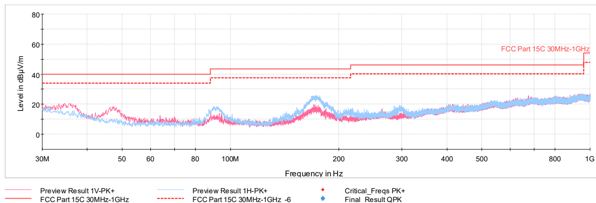
Plot 7-104. Radiated Spurious Plot below 1GHz (4Mbps, ePA – Ch.38 with AC/DC Adapter)
