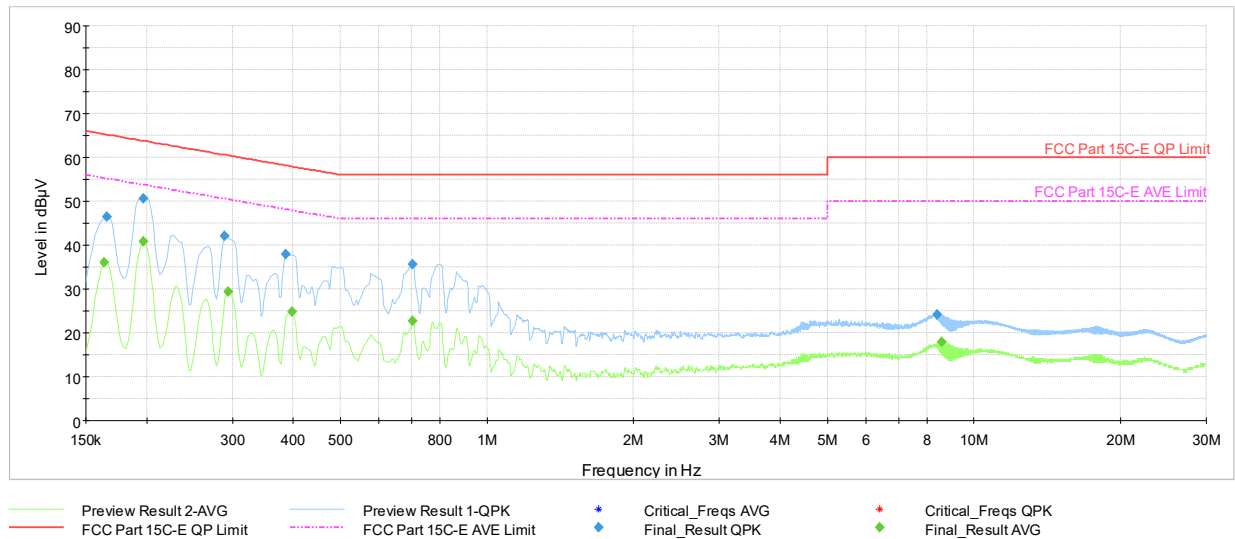
Plot 7-105. Line Conducted Plot with Bluetooth HDR (L1, 4Mbps ePA – Ch.38 with AC/DC Adapter)
