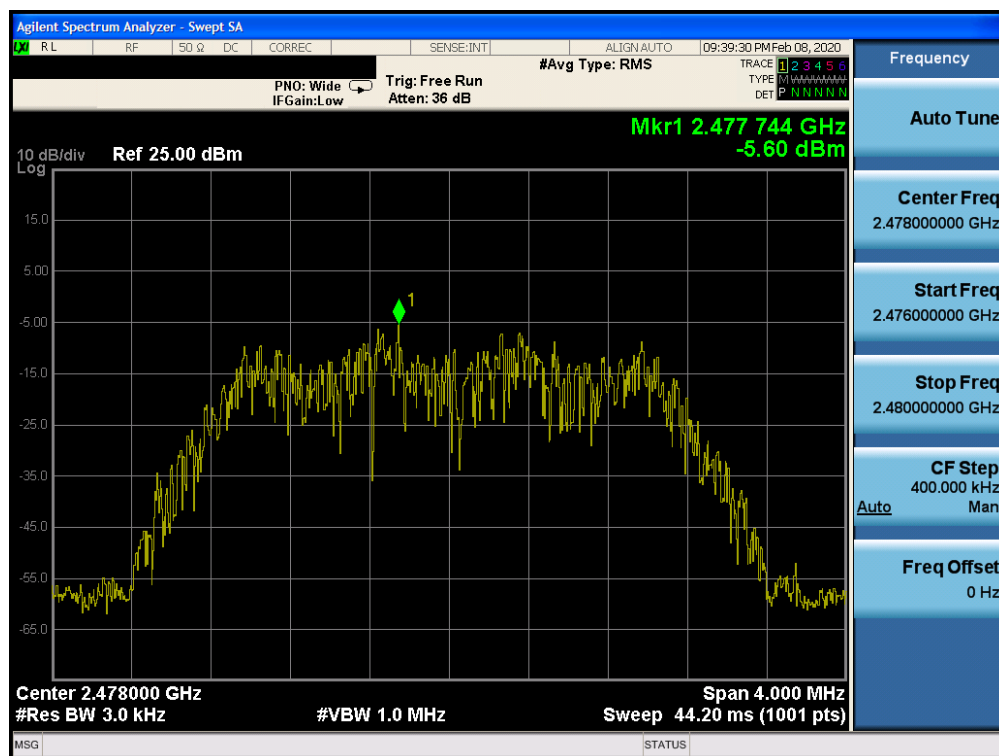
Plot 7-48. Power Spectral Density Plot TxBF Ant WF7 (Bluetooth (HDR4), 4Mbps, iPA – Ch. 75)
