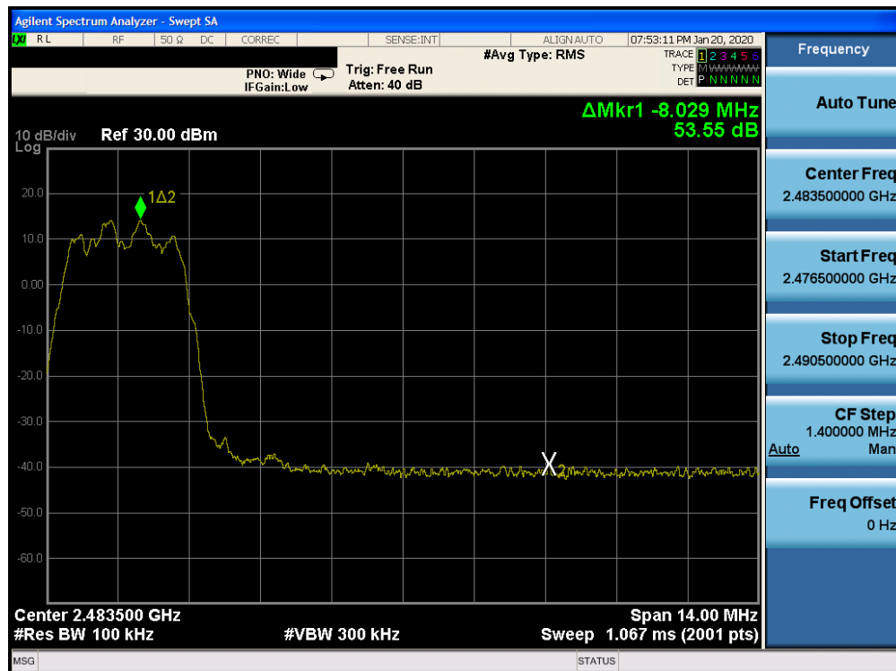
Plot 7-62. Band Edge Plot Ant WF8 (Bluetooth (HDR4), ePA – Ch. 75)
