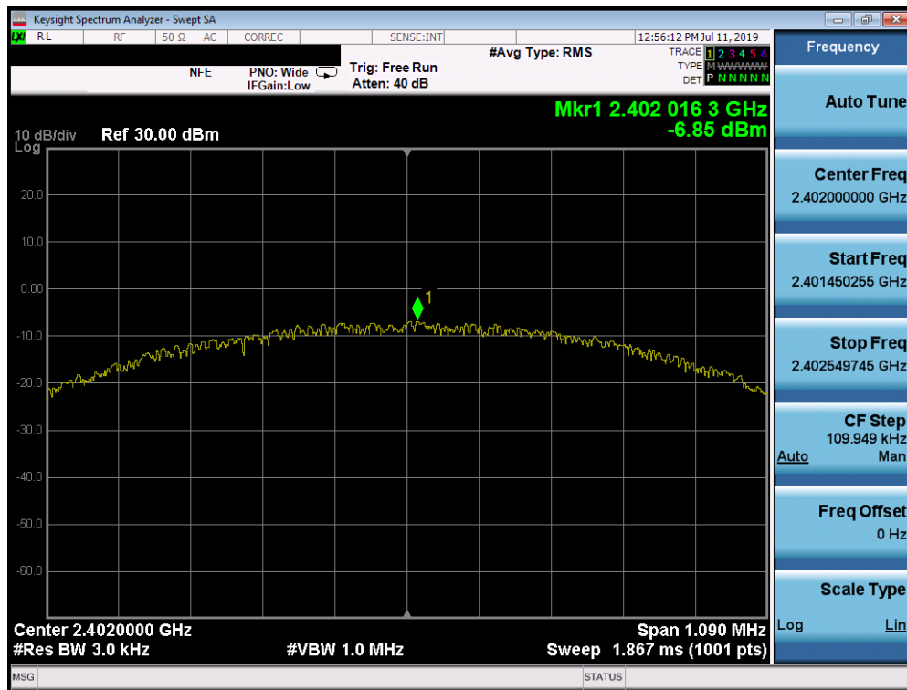
Plot 7-10. Power Spectral Density Plot (Bluetooth (LE), iPA – Ch. 0)
