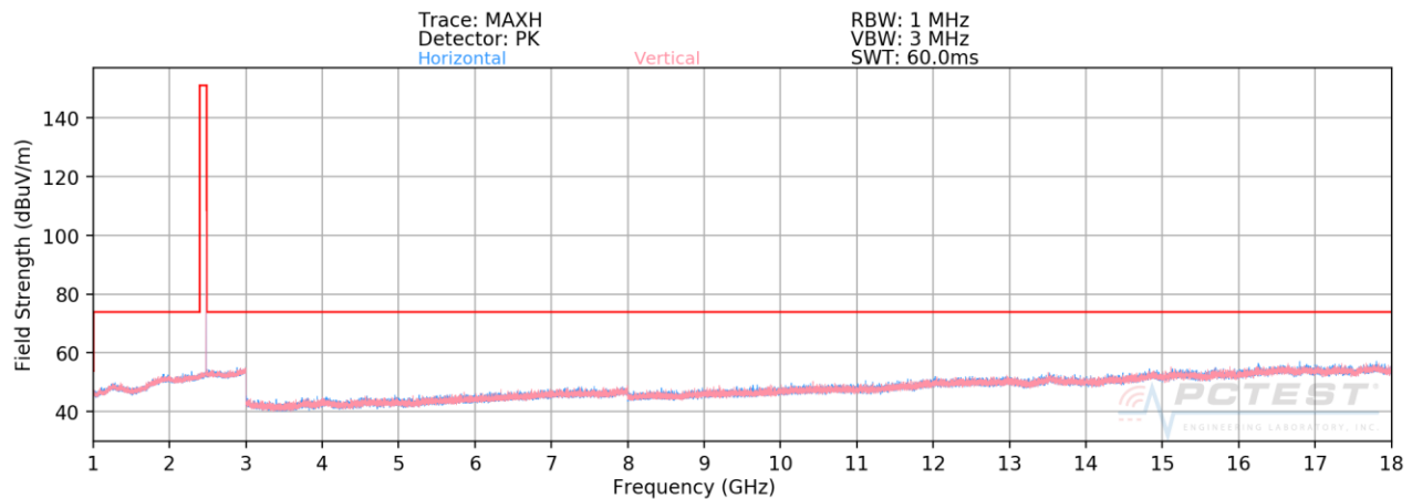
Plot 7-23. Radiated Spurious Plot Above 1GHz (1Mbps, ePA – Ch. 39)
