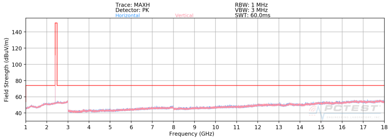
Plot 7-21. Radiated Spurious Plot Above 1GHz (1Mbps, ePA – Ch. 0)
