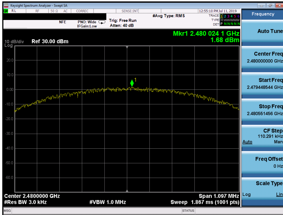
Plot 7-9. Power Spectral Density Plot (Bluetooth (LE), ePA – Ch. 39)
