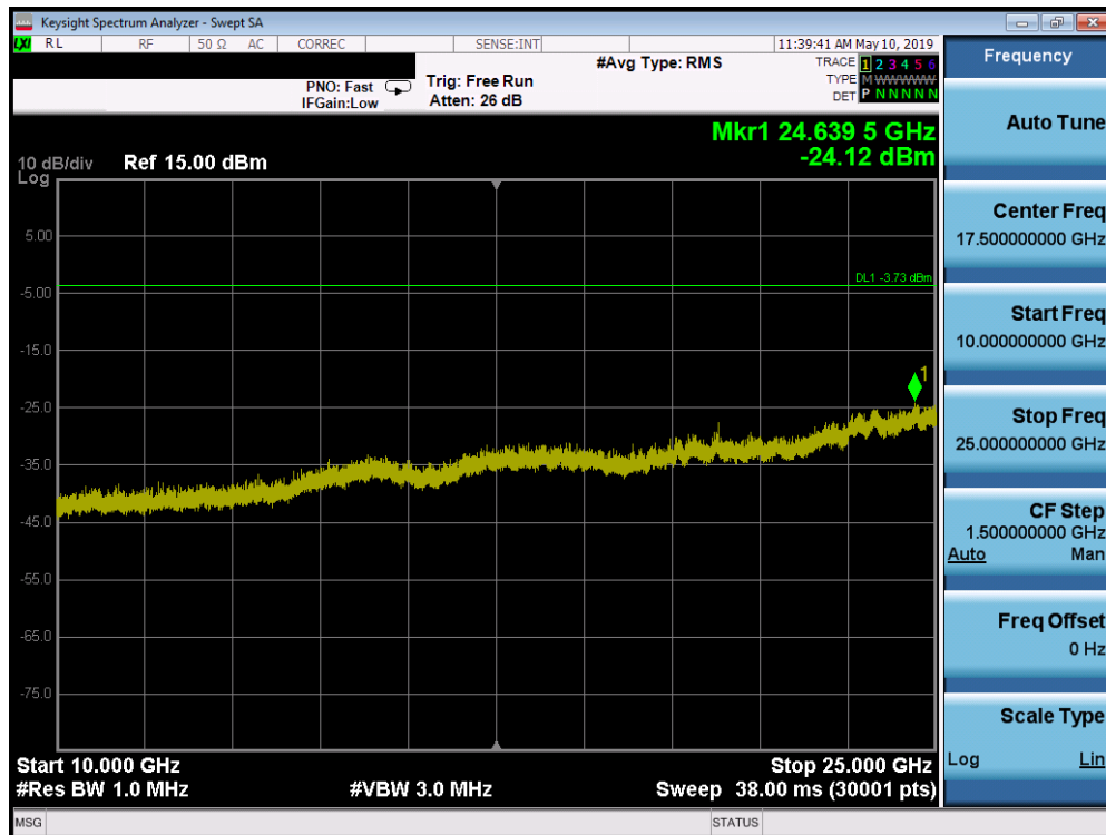
Plot 7-20. Conducted Spurious Plot (Bluetooth (LE), ePA – Ch. 39)
