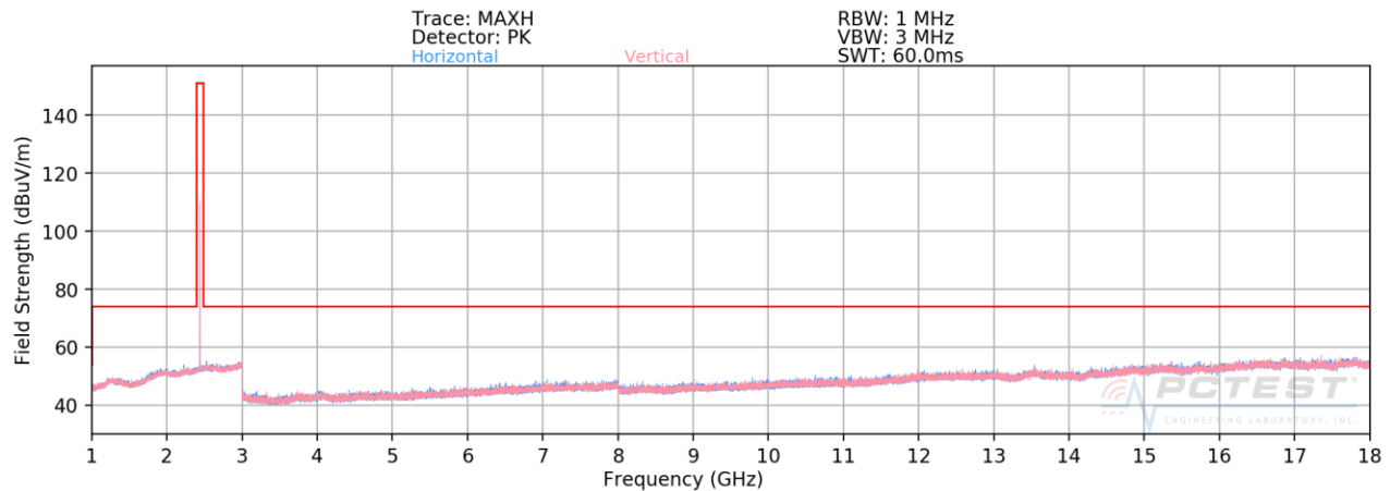
Plot 7-22. Radiated Spurious Plot Above 1GHz (1Mbps, ePA – Ch. 19)
