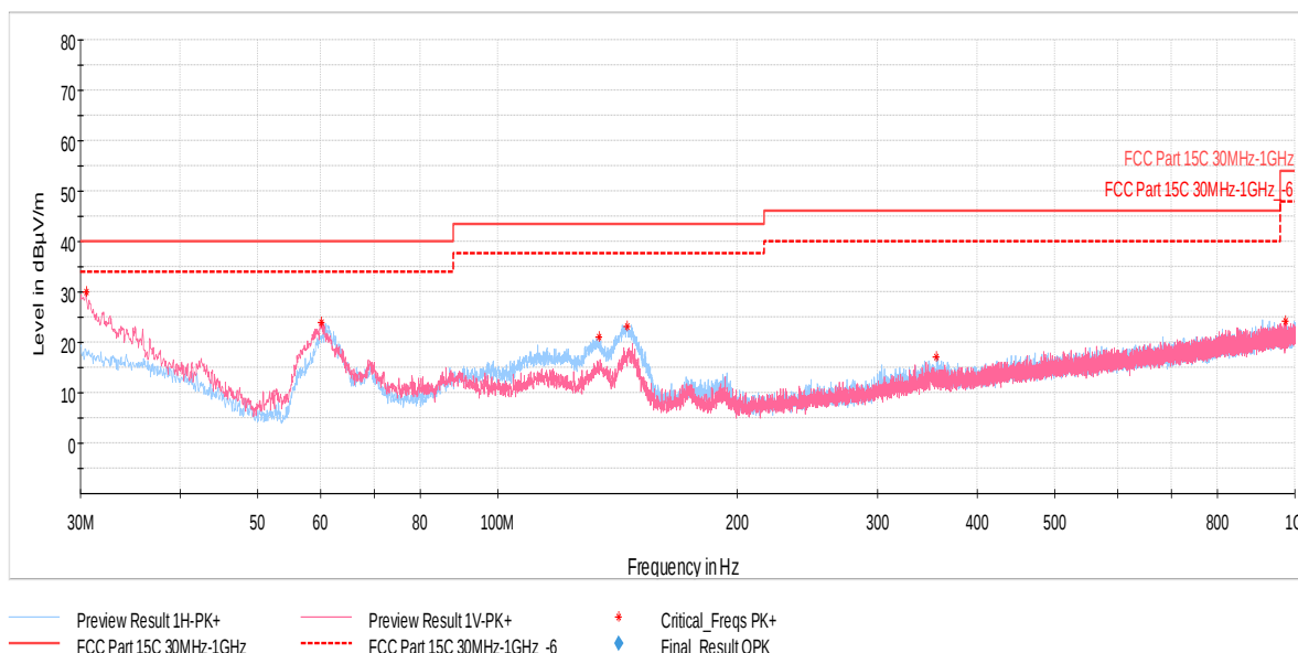
Plot 7-28. Radiated Spurious Plot below 1GHz (ePA – Ch.39, Pol. H & V, with AC/DC Adapter)
