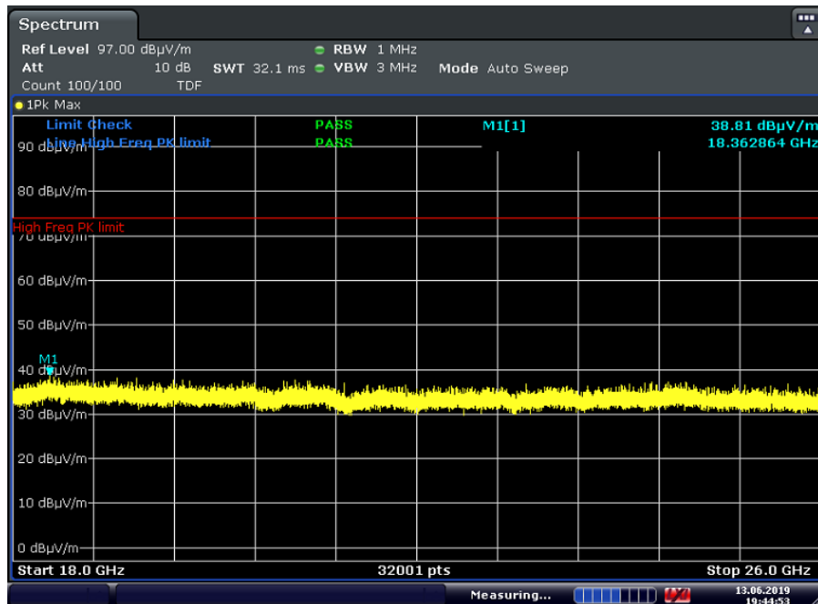
Plot 7-24. Radiated Spurious Plot Above 18GHz (ePA – Ch. 19, Ant. Pol. H)
