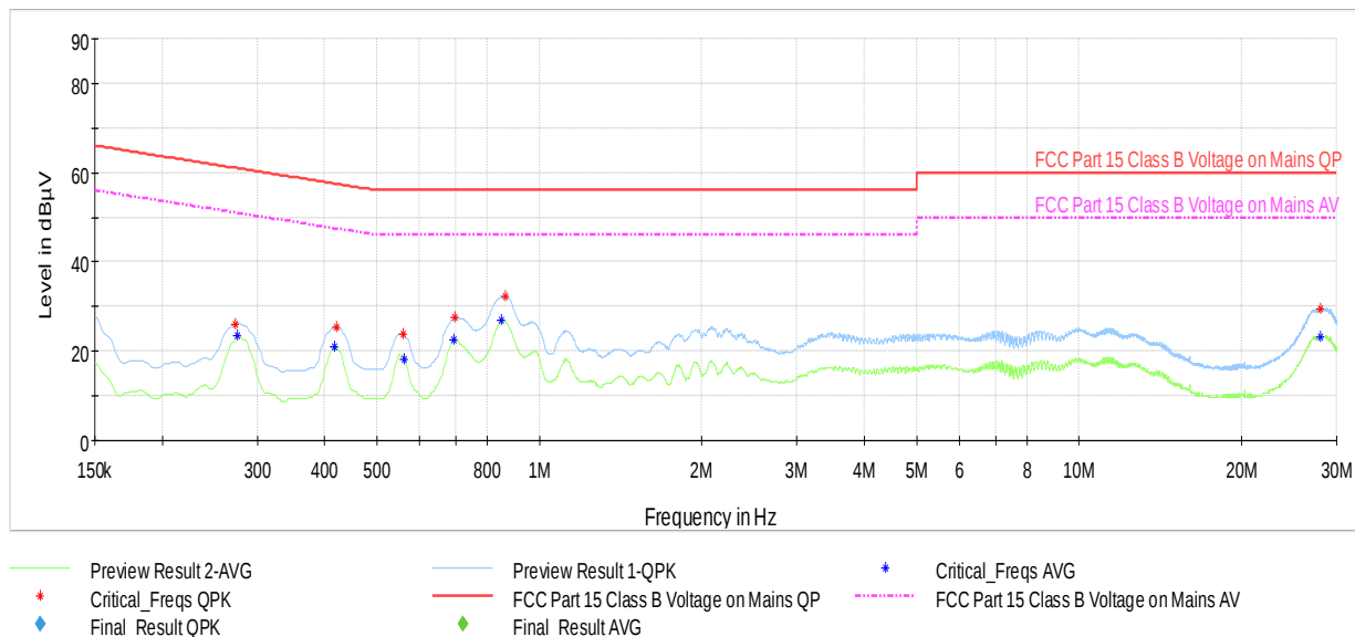
Plot 7-30. AC Line Conducted Plot with Bluetooth LE (N, with AC/DC Adapter)
