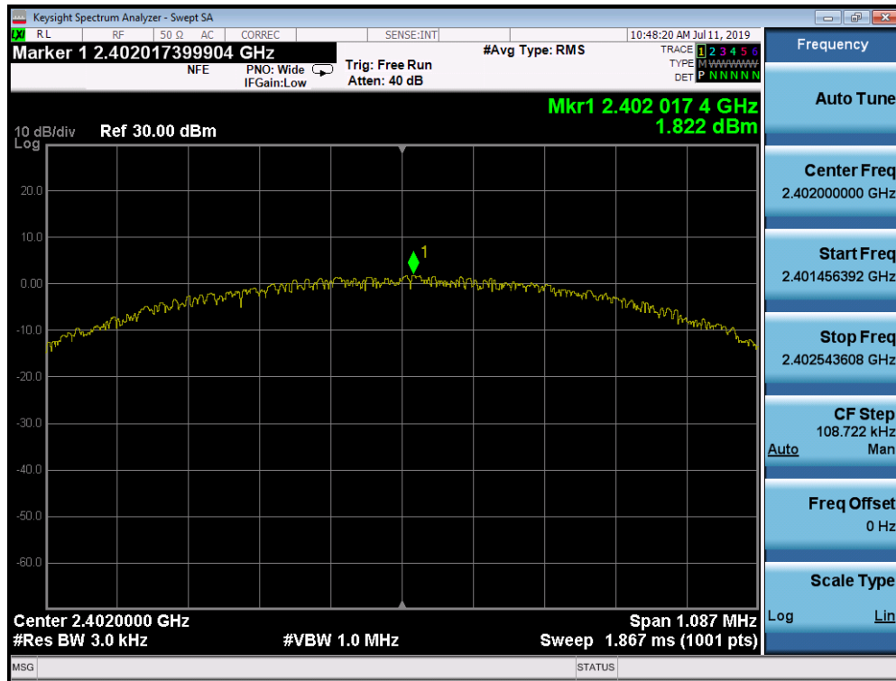
Plot 7-7. Power Spectral Density Plot (Bluetooth (LE), ePA – Ch. 0)
