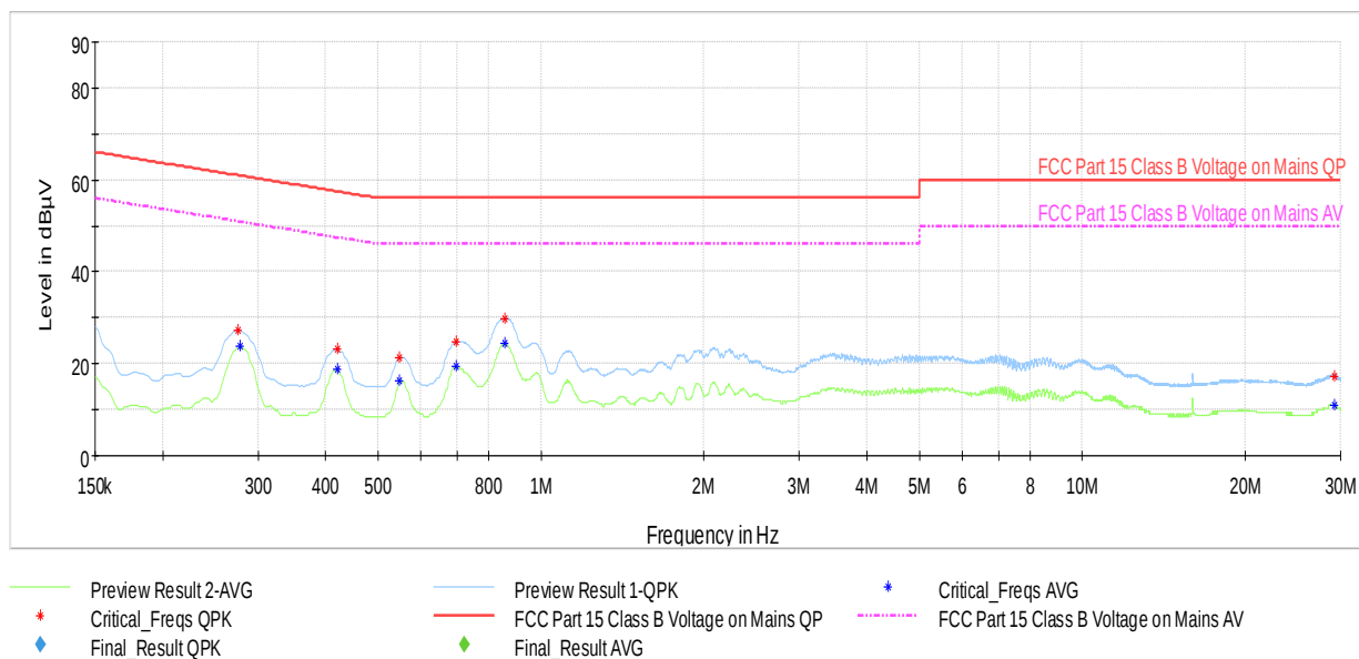
Plot 7-29. AC Line Conducted Plot with Bluetooth LE (L1, with AC/DC Adapter)
