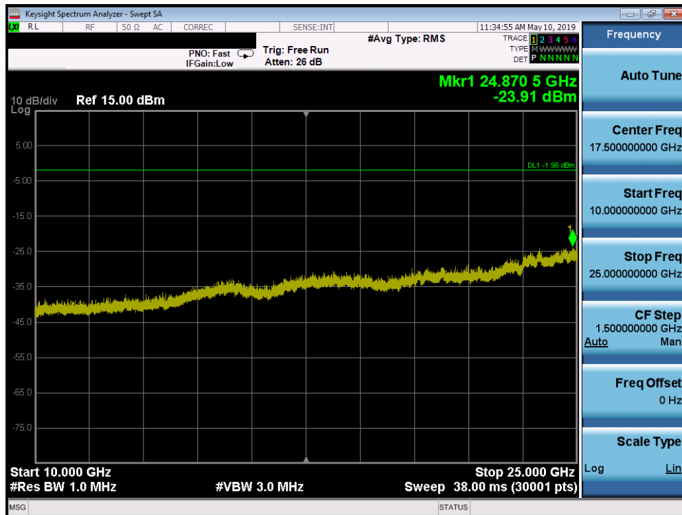
Plot 7-18. Conducted Spurious Plot (Bluetooth (LE), ePA – Ch. 19)
