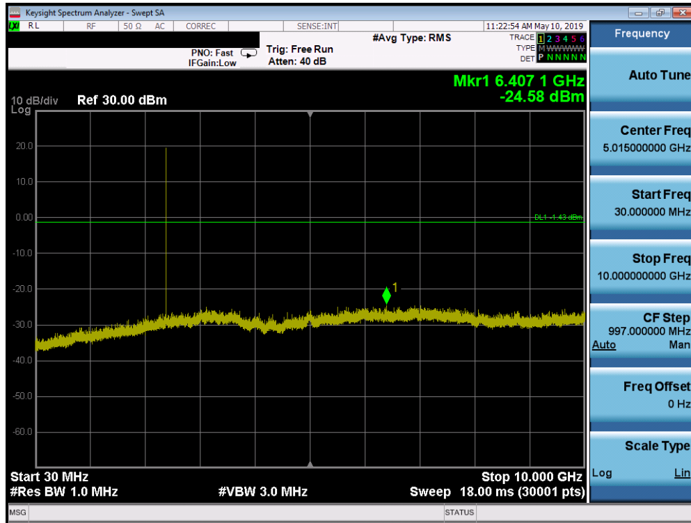
Plot 7-15. Conducted Spurious Plot (Bluetooth (LE), ePA – Ch. 0)
