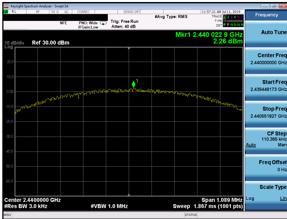
Plot 7-8. Power Spectral Density Plot (Bluetooth (LE), ePA – Ch. 19)
