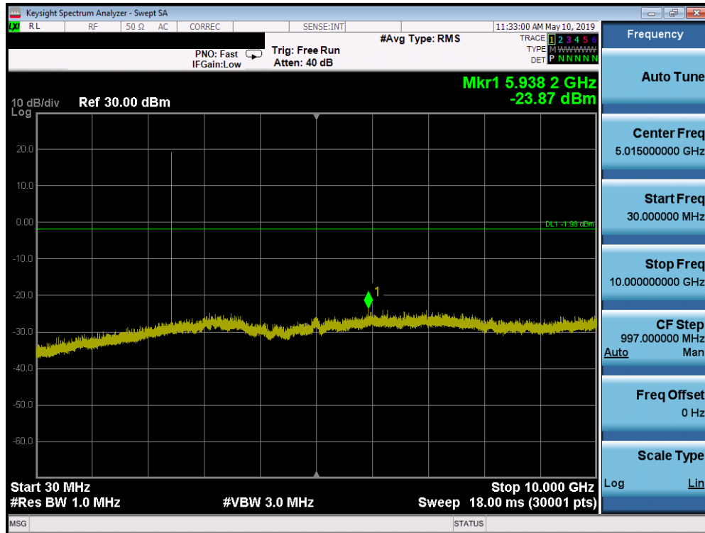
Plot 7-17. Conducted Spurious Plot (Bluetooth (LE), ePA – Ch. 19)
