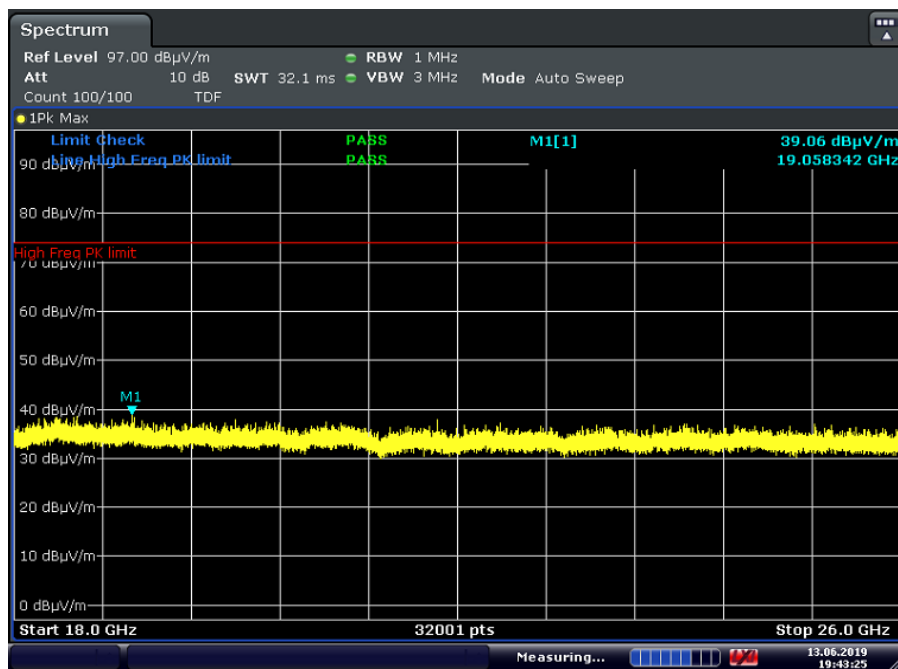
Plot 7-25. Radiated Spurious Plot Above 18GHz (ePA – Ch. 19, Ant. Pol. V)
