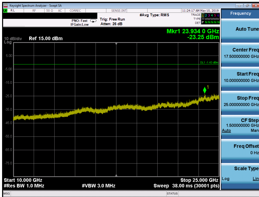
Plot 7-16. Conducted Spurious Plot (Bluetooth (LE), ePA – Ch. 0)
