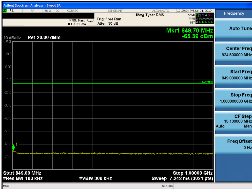
Plot 7-116. Conducted Spurious Plot (Band 5 - 10.0MHz QPSK - RB Size 1, RB Offset 0 - Low Channel)
