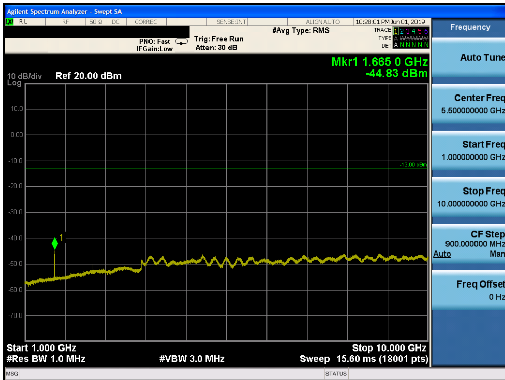
Plot 7-120. Conducted Spurious Plot (Band 5 - 10.0MHz QPSK - RB Size 1, RB Offset 0 - Mid Channel)
