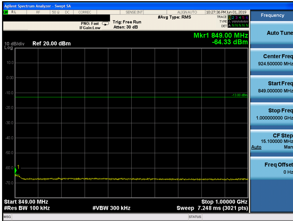
Plot 7-119. Conducted Spurious Plot (Band 5 - 10.0MHz QPSK - RB Size 1, RB Offset 0 - Mid Channel)
