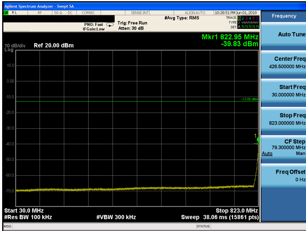
Plot 7-115. Conducted Spurious Plot (Band 5 - 10.0MHz QPSK - RB Size 1, RB Offset 0 - Low Channel)
