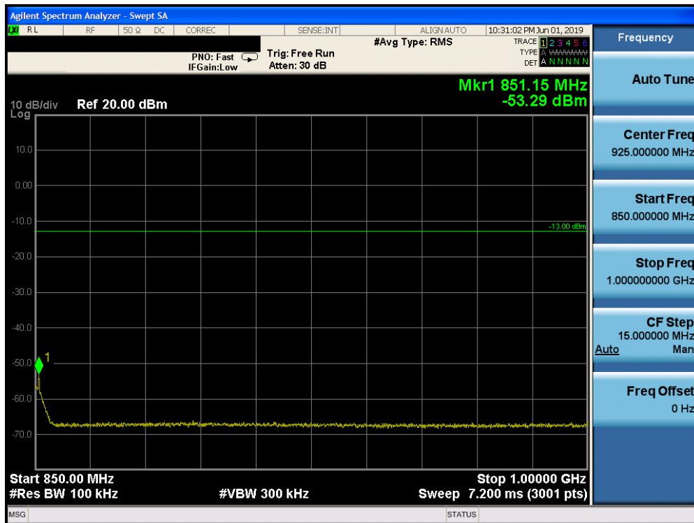
Plot 7-122. Conducted Spurious Plot (Band 5 - 10.0MHz QPSK - RB Size 1, RB Offset 0 - High Channel)
