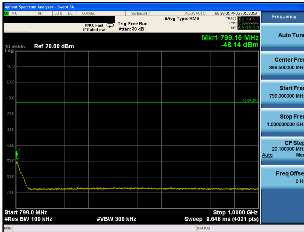
Plot 7-29. Conducted Spurious Plot (LTE Band 14, 5MHz QPSK – RB Size 1, RB Offset 0 – High Channel)
