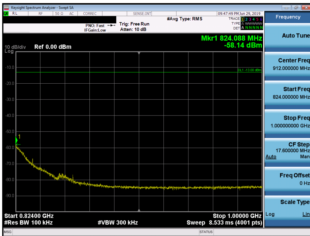
Plot 7-20. Conducted Spurious Plot (LTE Band 26, 5MHz QPSK – RB Size 1, RB Offset 0 – Low Channel)
