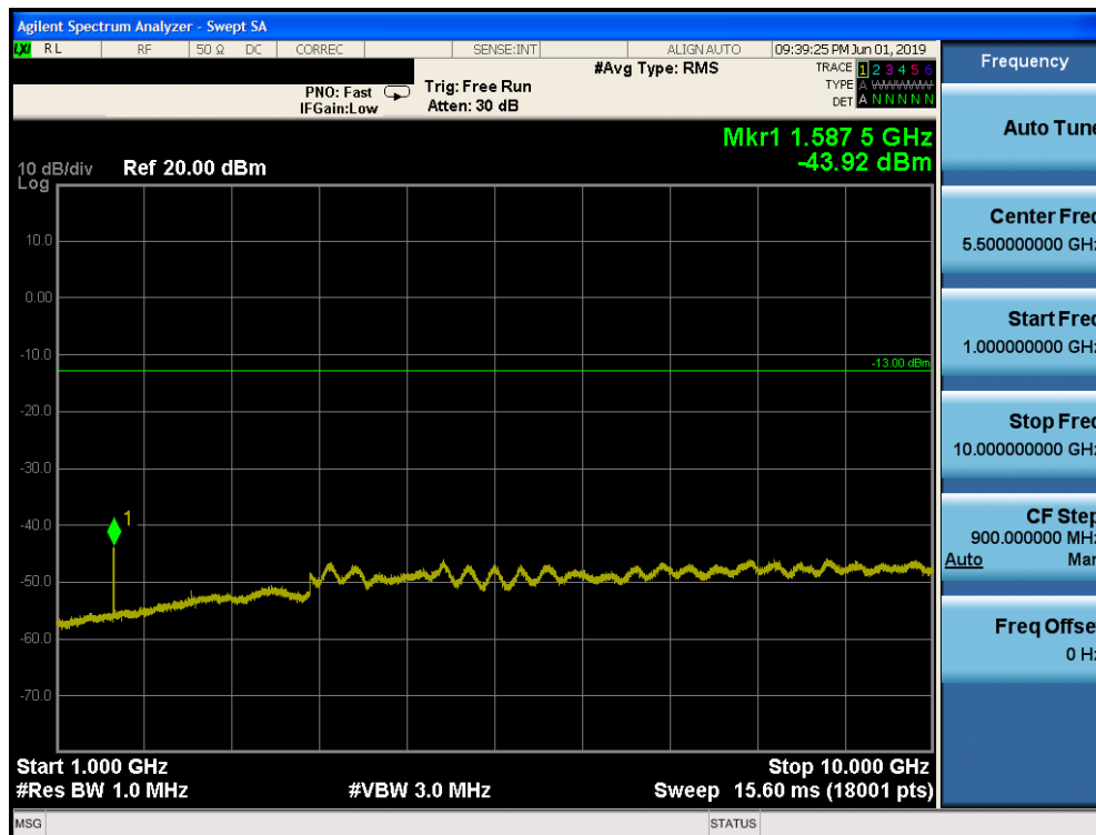
Plot 7-30. Conducted Spurious Plot (LTE Band 14, 5MHz QPSK – RB Size 1, RB Offset 0 – High Channel)
