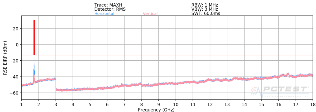
Plot 7-84. Radiated Spurious Plot above 1GHz (AWS WCDMA Mode)
