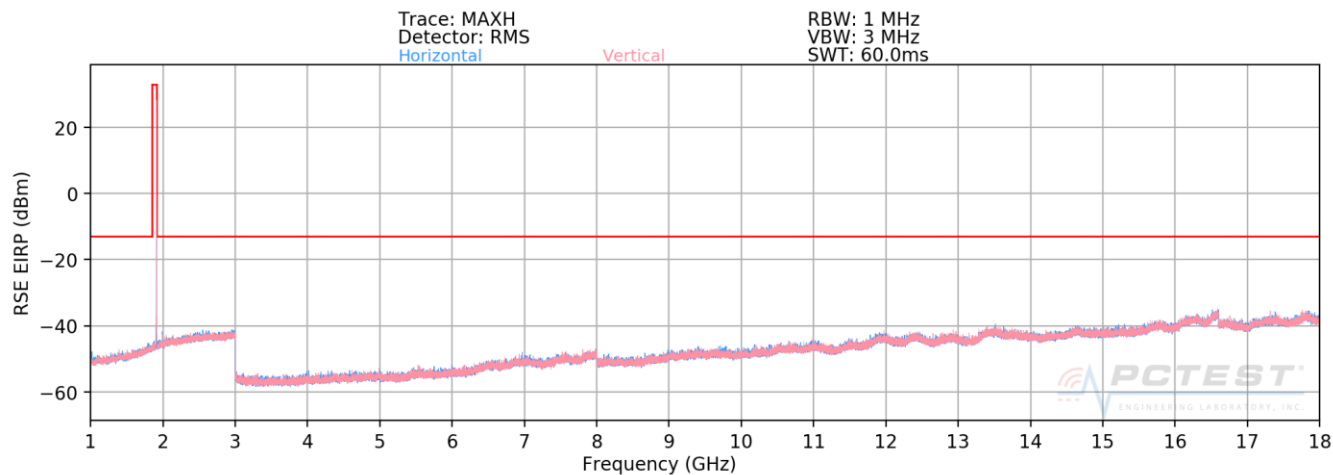
Plot 7-85. Radiated Spurious Plot above 1GHz (PCS GPRS Mode)
