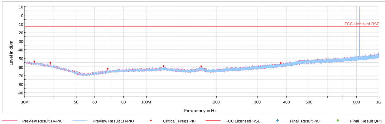
Plot 7-76. Radiated Spurious Plot below 1GHz (Cellular GPRS Mode) with Laptop
