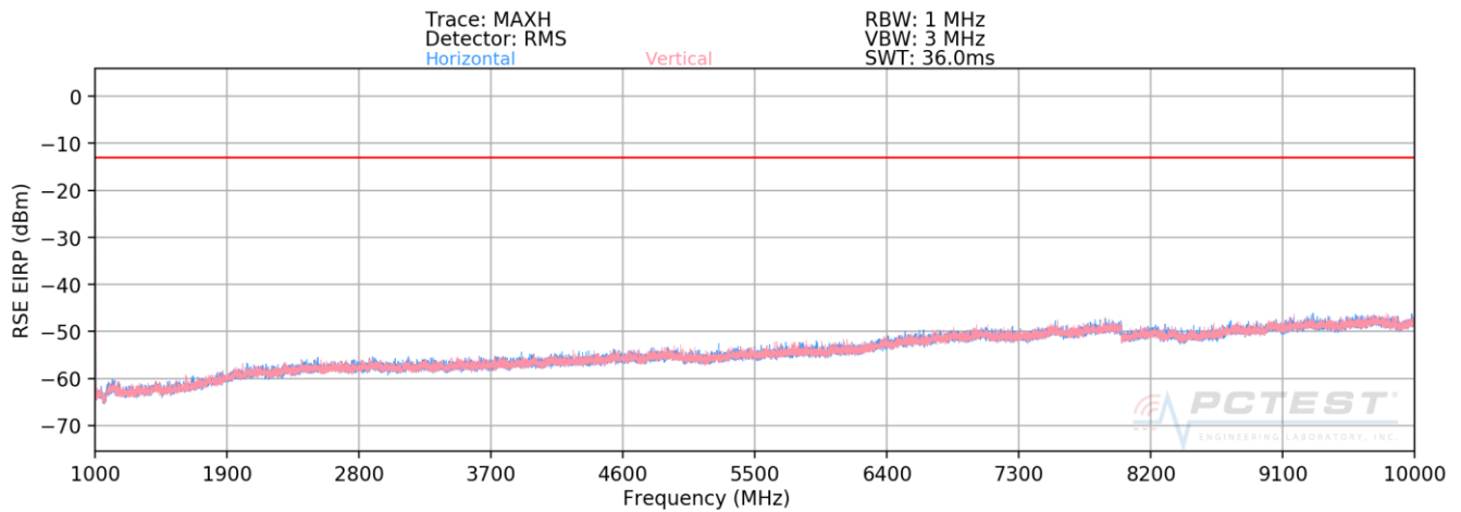
Plot 7-82. Radiated Spurious Plot above 1GHz (Cellular GPRS Mode)
