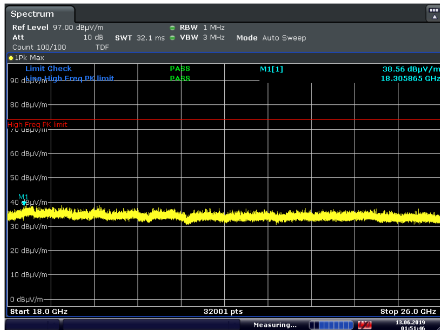
Plot 7-39. Radiated Spurious Plot above 18GHz (GFSK ePA – Ch. 39, Pol. V)
