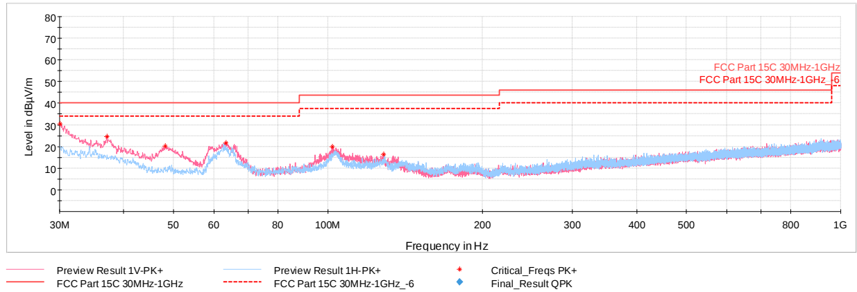
Plot 7-48. Radiated Spurious Plot below 1GHz (2.4GHz – 5GHz), with AC/DC Adapter
