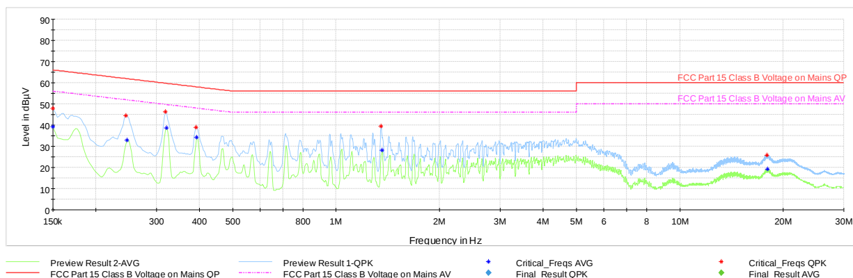
Plot 7-50. AC Line-Conducted Test Plot - Ch.39 (N, with Laptop)
