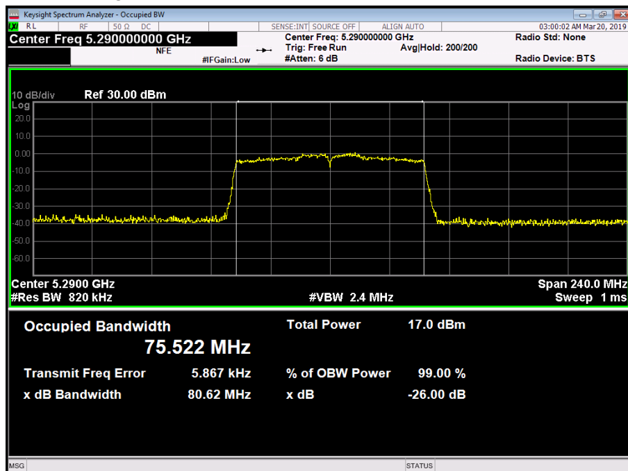
Figure 164 - 5290 MHz - 99% Occupied Bandwidth
