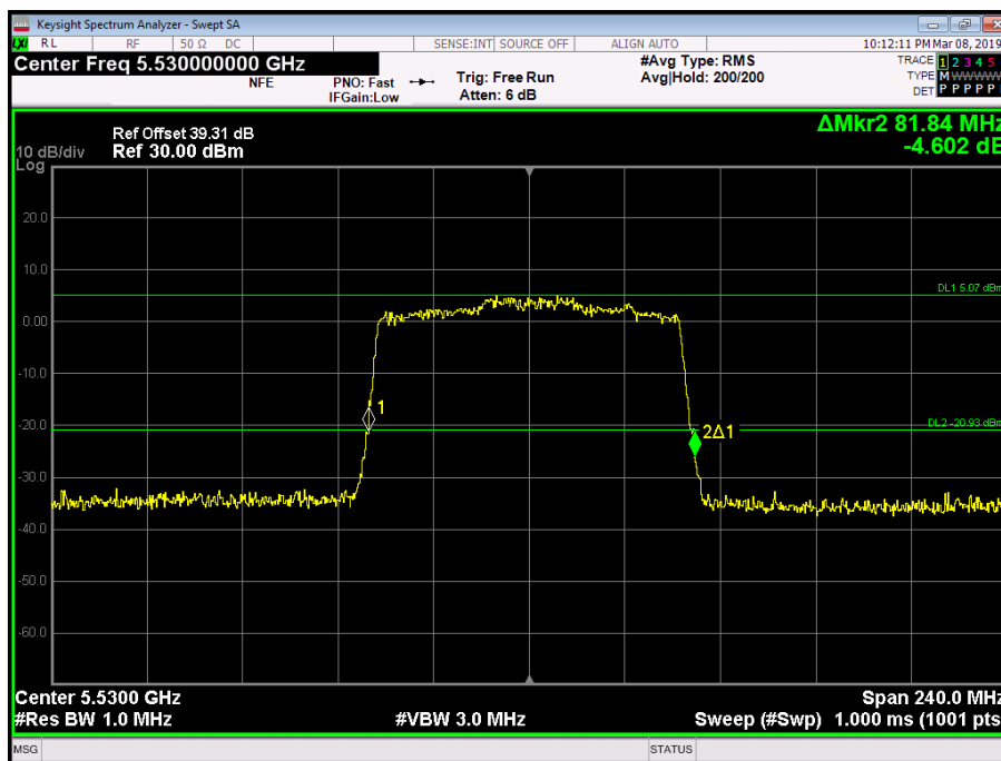
Figure 251 - 5530 MHz - 26 dB Emission Bandwidth
