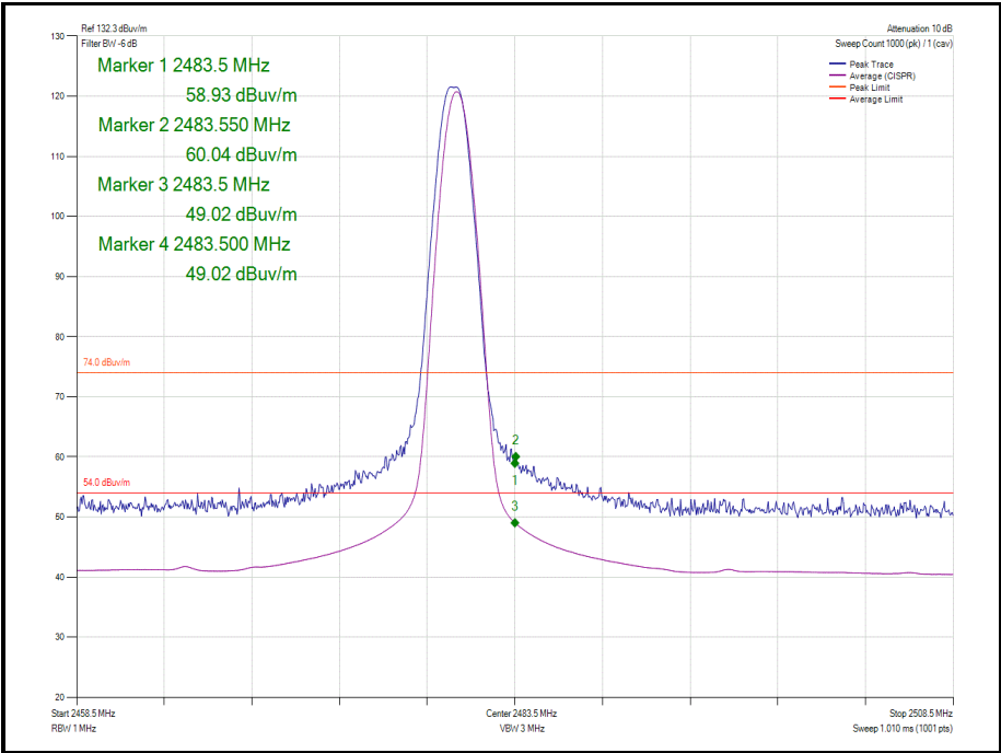
Static - GFSK/DH5 - 2480 MHz - Band Edge Frequency 2483.5 MHz
