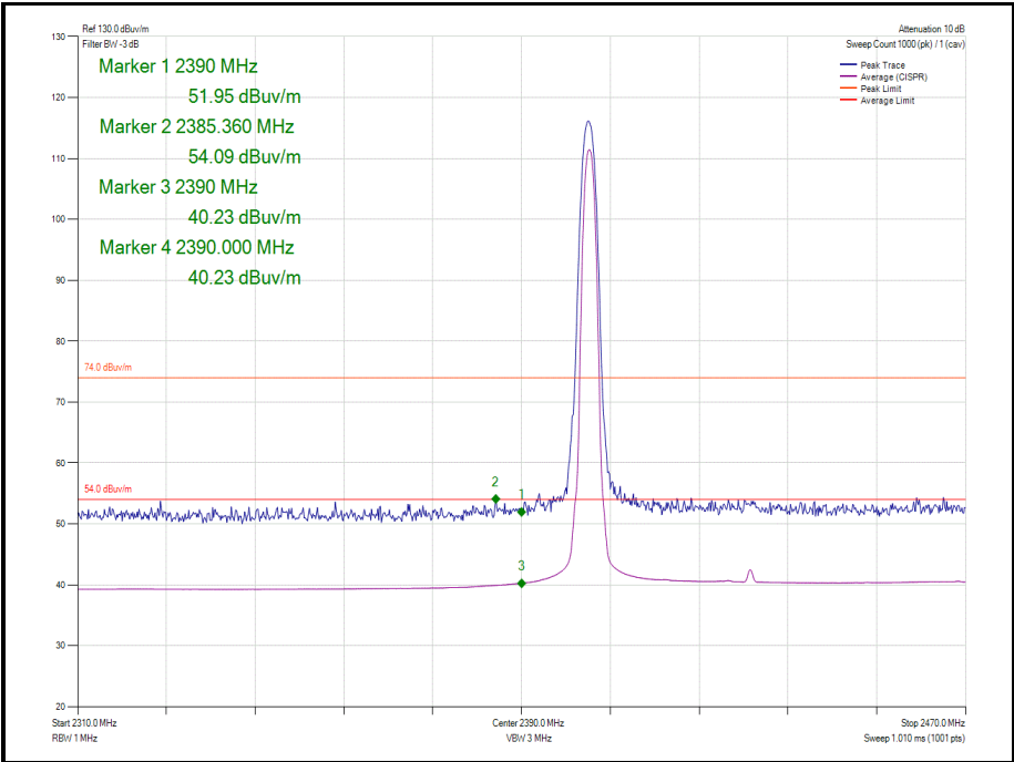
Static - 8-DPSK/3DH5 - 2402 MHz - Band Edge Frequency 2390.0 MHz
