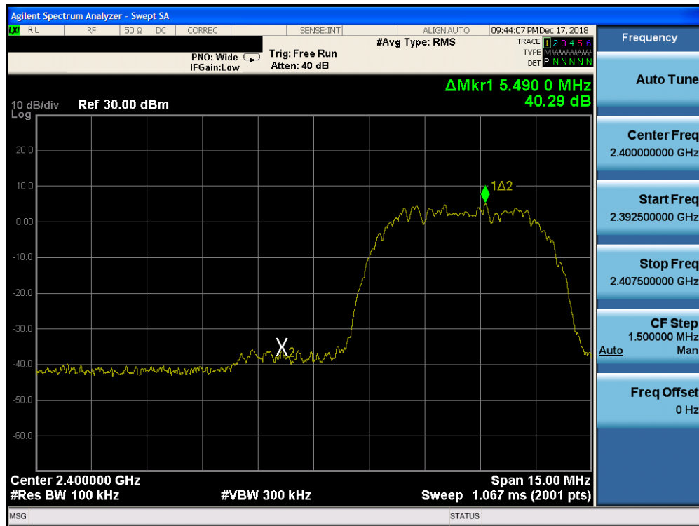
Plot 7-39. Band Edge Plot Ant-0 (Bluetooth (HDR8), ePA - Ch. 1)
