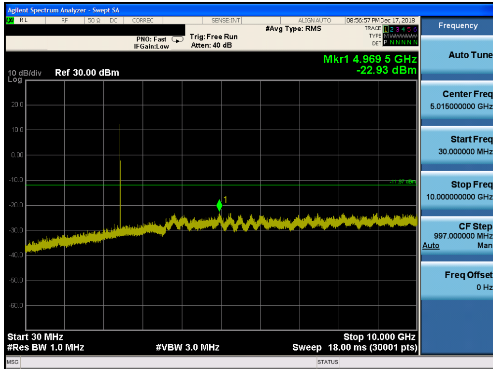
Plot 7-47. Conducted Spurious Plot Ant-0 (Bluetooth (HDR4), Mbps, ePA – Ch. 38)
