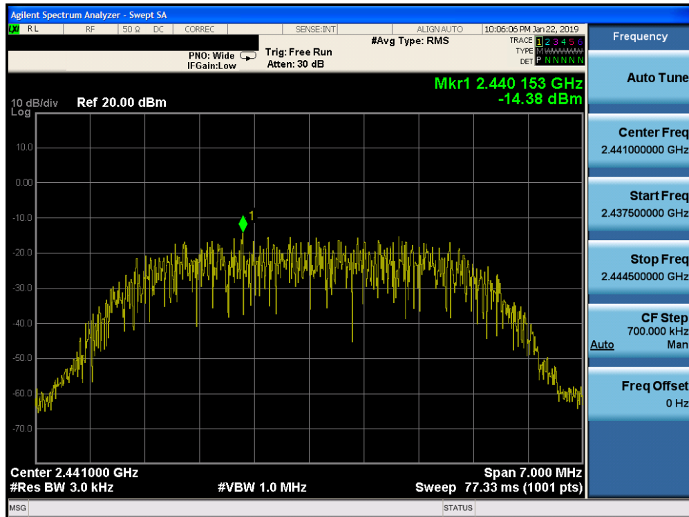
Plot 7-35. Power Spectral Density Plot Ant-1 (Bluetooth (HDR8), 8Mbps, iPA – Ch. 38)
