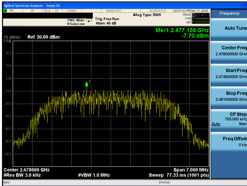
Plot 7-21. Power Spectral Density Plot Ant-0 (Bluetooth (HDR8), 8Mbps, ePA – Ch. 75)
