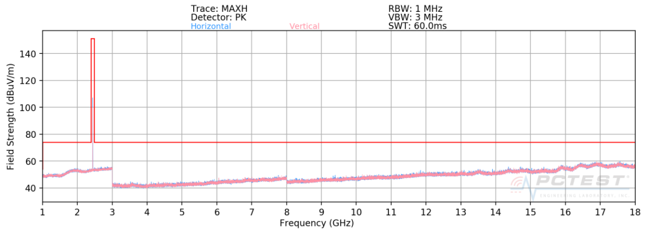
Plot 7-58. Radiated Spurious Plot Above 1GHz Ant-0 (4Mbps, HDR4, ePA – Ch. 38, Ant. Pol. H & V)
