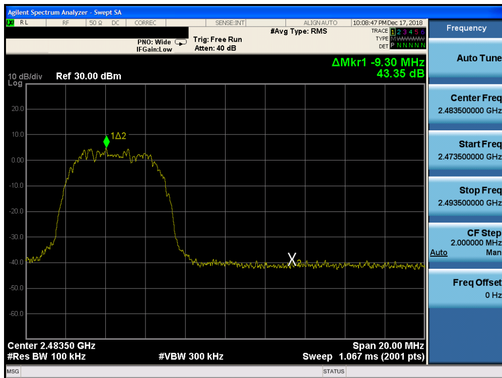
Plot 7-40. Band Edge Plot Ant-0 (Bluetooth (HDR8), ePA - Ch. 75)
