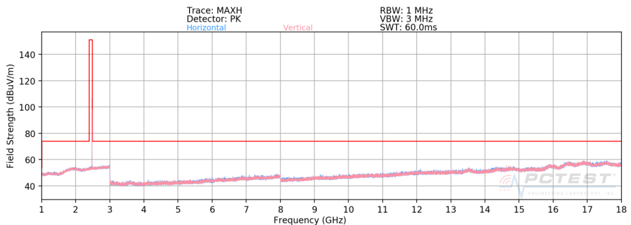
Plot 7-62. Radiated Spurious Plot Above 1GHz Ant-1 (4Mbps, HDR4, ePA – Ch. 75, Ant. Pol. H & V)
