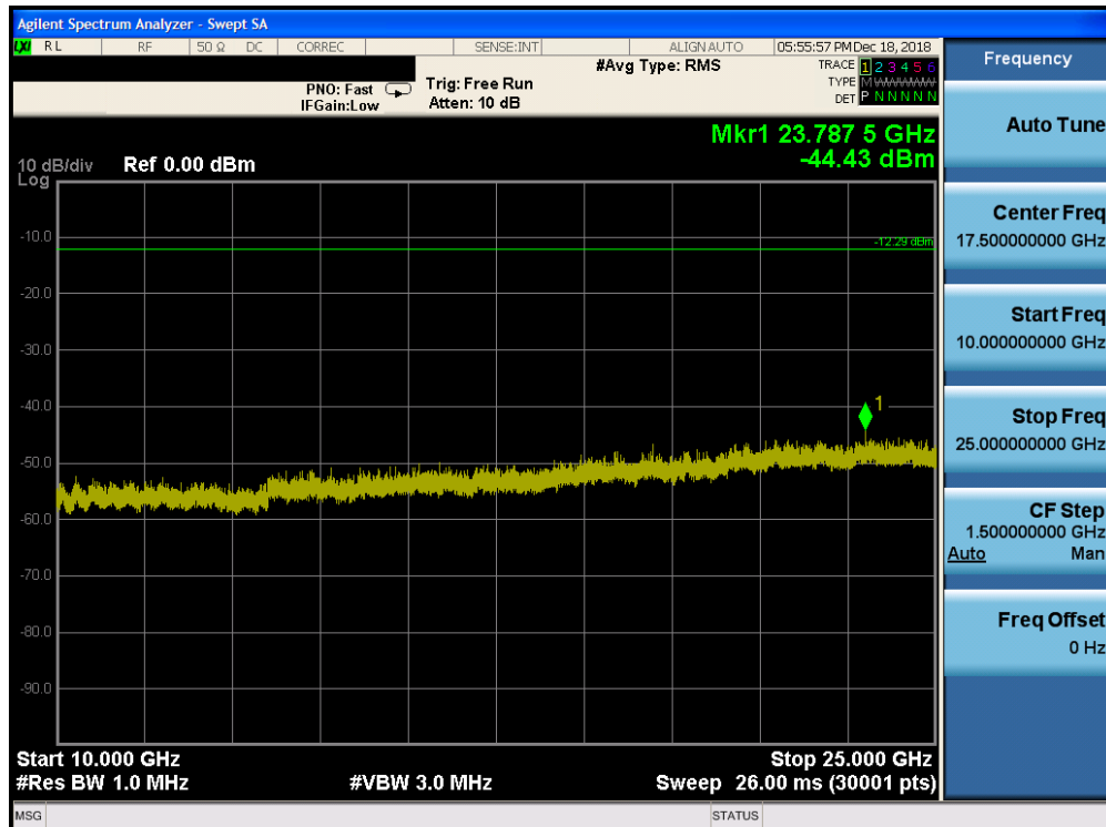
Plot 7-52. Conducted Spurious Plot Ant-1 (Bluetooth (HDR4), Mbps, ePA – Ch. 1)
