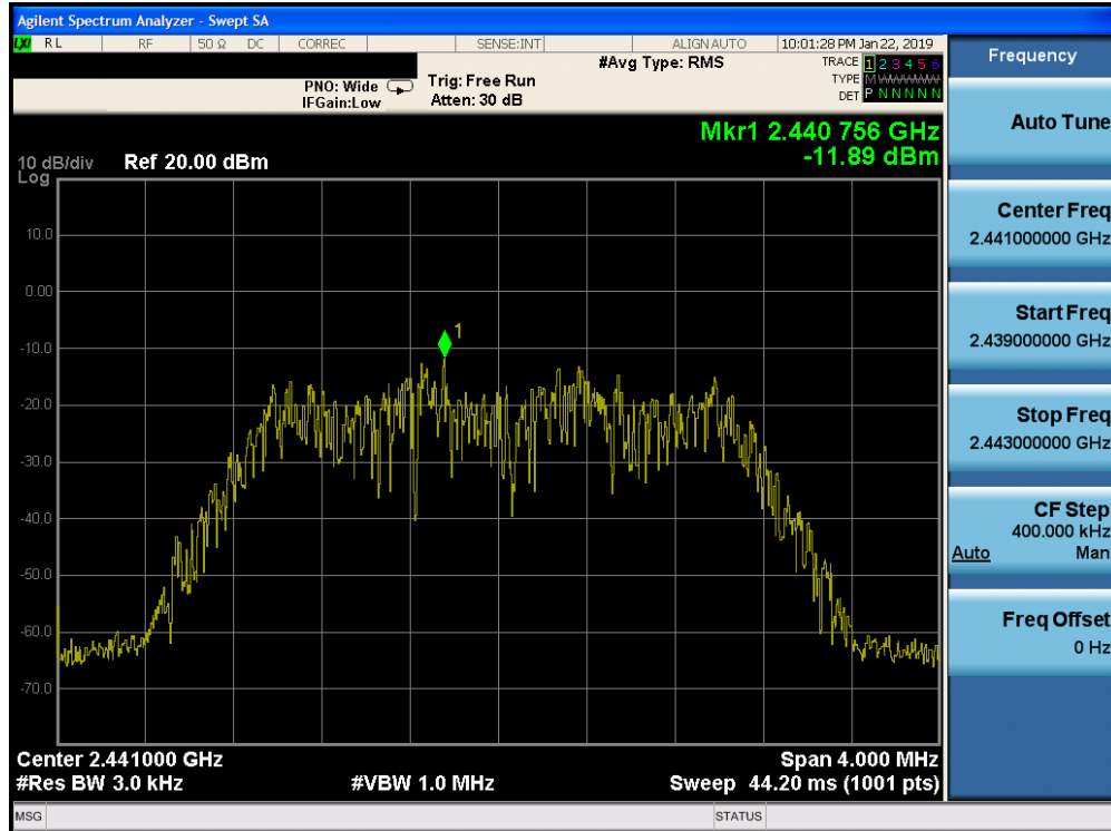
Plot 7-29. Power Spectral Density Plot Ant-1 (Bluetooth (HDR4), 4Mbps, iPA – Ch. 38)
