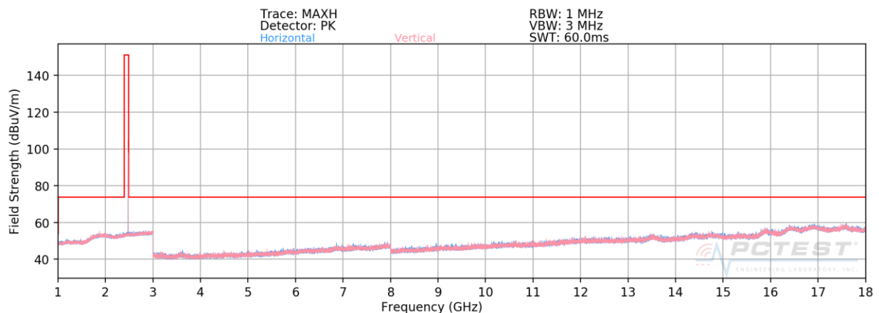
Plot 7-59. Radiated Spurious Plot Above 1GHz Ant-0 (4Mbps, HDR4, ePA – Ch. 75, Ant. Pol. H & V)
