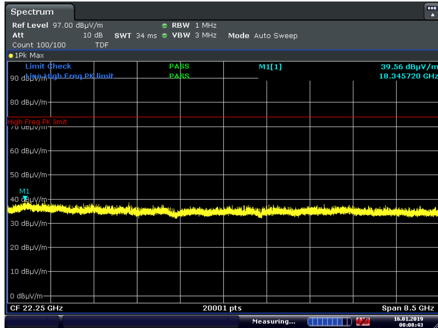
Plot 7-63. Radiated Spurious Plot Above 18GHz Ant-0 (4Mbps, HDR, ePA – Ch.38, Ant. Pol. H)
