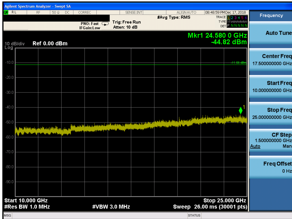
Plot 7-46. Conducted Spurious Plot Ant-0 (Bluetooth (HDR4), Mbps, ePA – Ch. 1)
