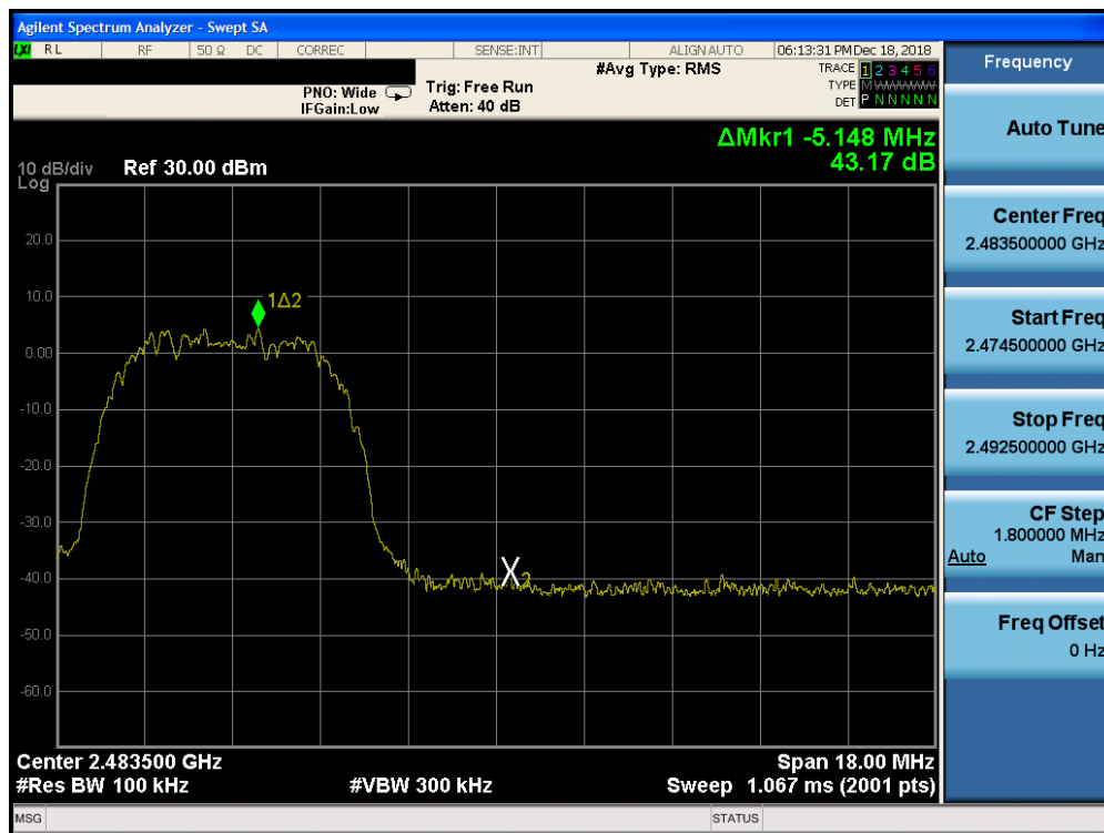
Plot 7-44. Band Edge Plot Ant-1 (Bluetooth (HDR8), ePA - Ch. 75)
