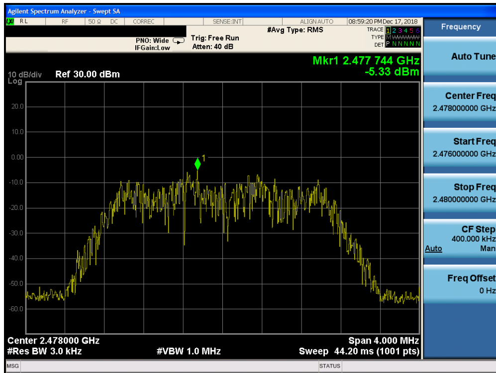
Plot 7-15. Power Spectral Density Plot Ant-0 (Bluetooth (HDR4), 4Mbps, ePA – Ch. 75)
