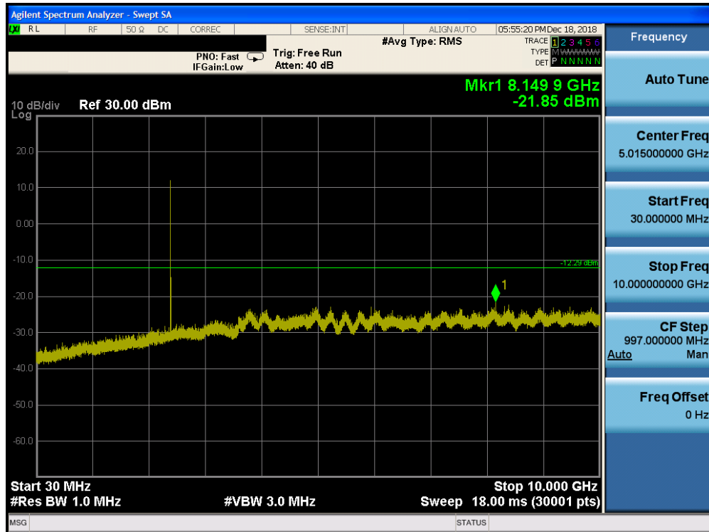
Plot 7-51. Conducted Spurious Plot Ant-1 (Bluetooth (HDR4), Mbps, ePA – Ch. 1)
