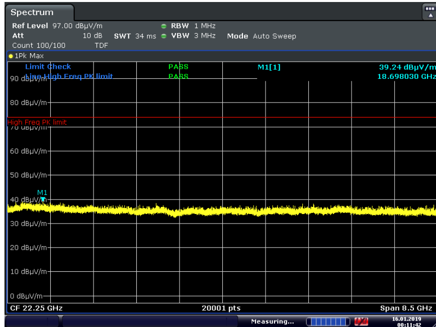
Plot 7-64. Radiated Spurious Plot Above 18GHz Ant-0 (4Mbps, HDR, ePA – Ch.38, Ant. Pol. V)
