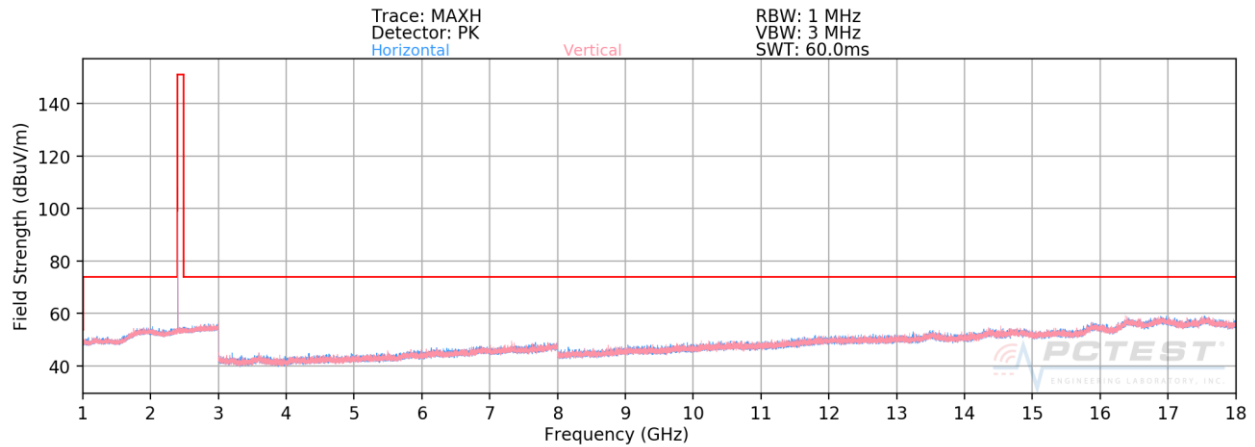
Plot 7-60. Radiated Spurious Plot Above 1GHz Ant-1 (4Mbps, HDR4, ePA – Ch. 1, Ant. Pol. H & V)
