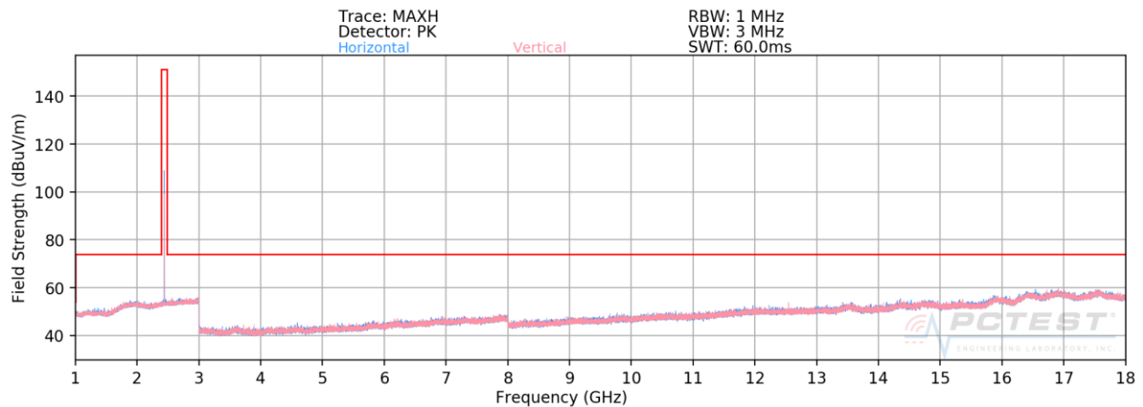
Plot 7-61. Radiated Spurious Plot Above 1GHz Ant-1 (4Mbps, HDR4, ePA – Ch. 38, Ant. Pol. H & V)
