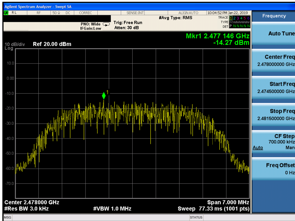
Plot 7-36. Power Spectral Density Plot Ant-1 (Bluetooth (HDR8), 8Mbps, iPA – Ch. 75)
