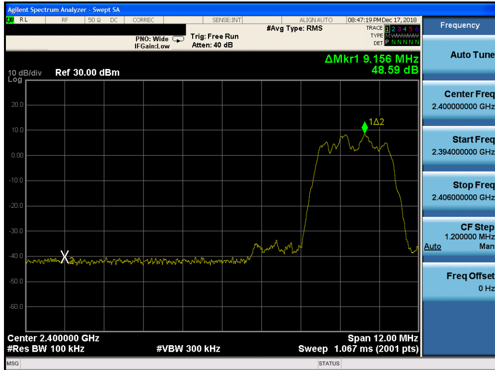
Plot 7-37. Band Edge Plot Ant-0 (Bluetooth (HDR4), ePA – Ch. 1)
