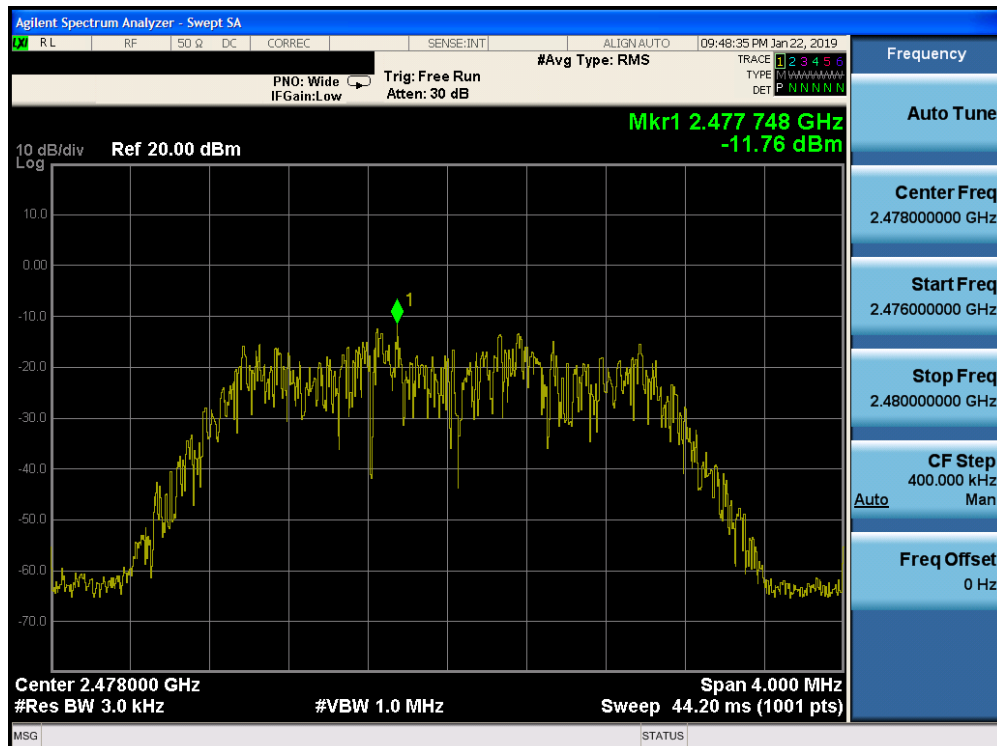
Plot 7-18. Power Spectral Density Plot Ant-0 (Bluetooth (HDR4), 4Mbps, iPA – Ch. 75)
