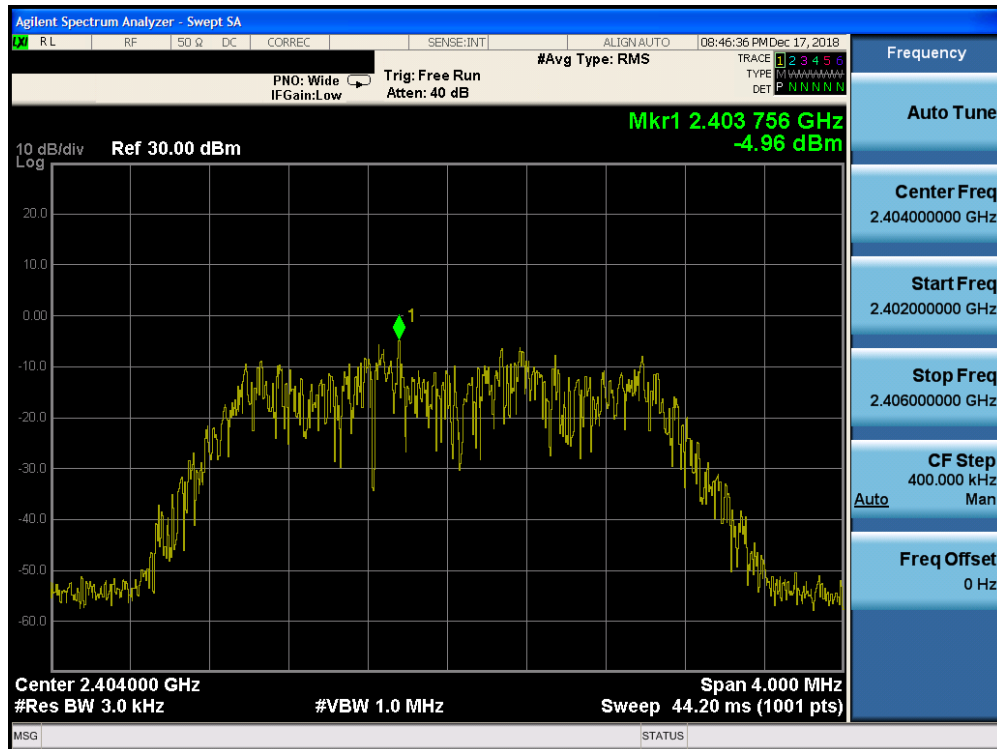
Plot 7-13. Power Spectral Density Plot Ant-0 (Bluetooth (HDR4), 4Mbps, ePA – Ch. 1)
