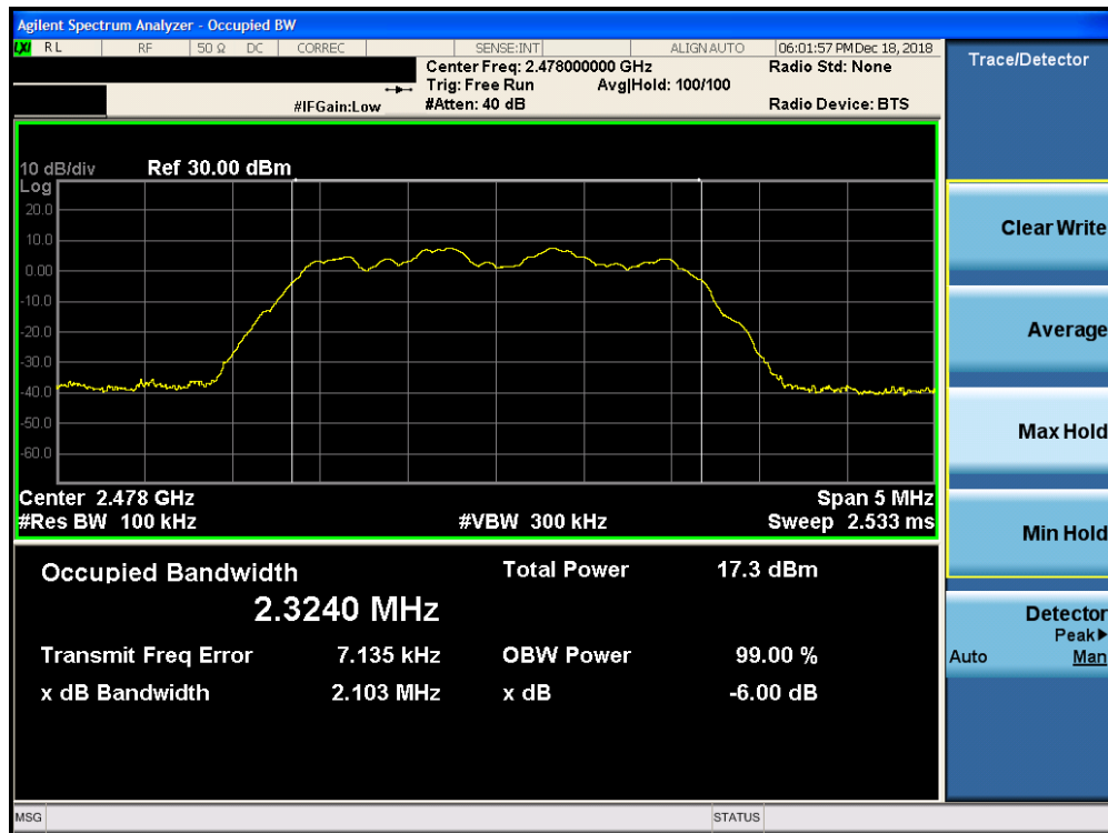
Plot 7-9. 6dB Bandwidth Plot Ant-1 (Bluetooth (HDR4), 4Mbps, ePA - Ch. 75)
