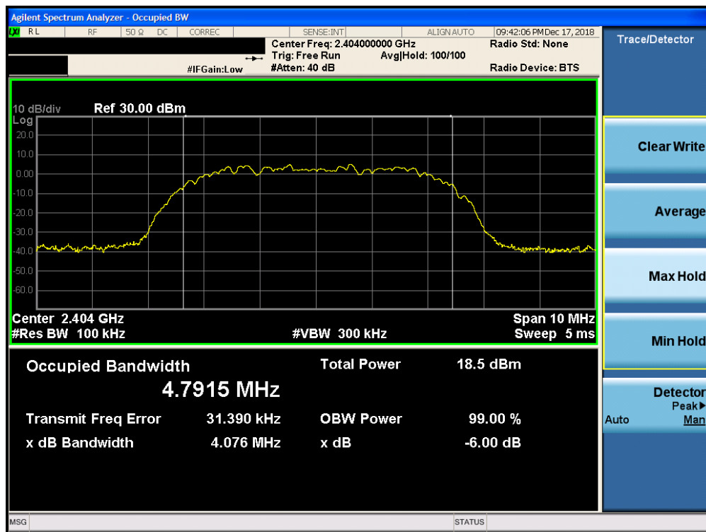
Plot 7-4. 6dB Bandwidth Plot Ant-0 (Bluetooth (HDR8), 8Mbps, ePA – Ch. 1)
