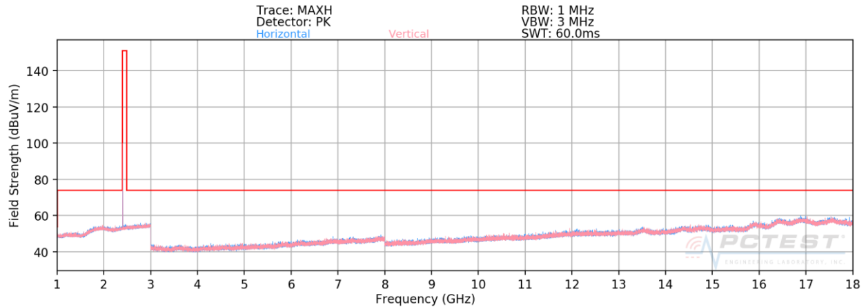
Plot 7-57. Radiated Spurious Plot Above 1GHz Ant-0 (4Mbps, HDR4, ePA – Ch. 1, Ant. Pol. H & V)
