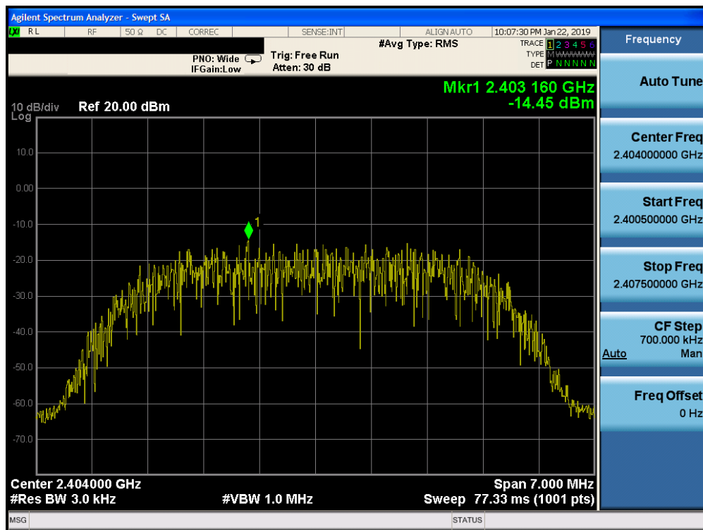
Plot 7-34. Power Spectral Density Plot Ant-1 (Bluetooth (HDR8), 8Mbps, iPA – Ch. 1)
