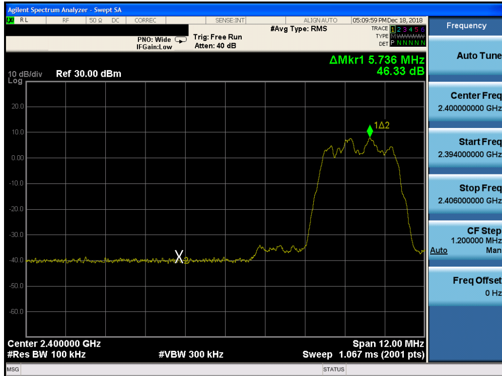
Plot 7-41. Band Edge Plot Ant-1 (Bluetooth (HDR4), ePA – Ch. 1)
