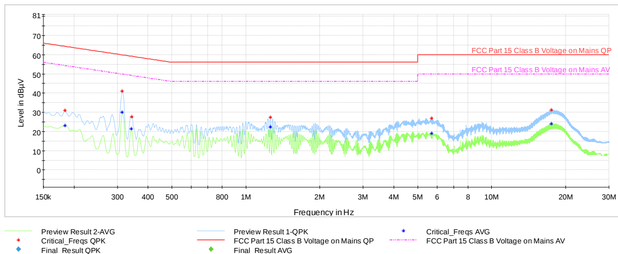
Plot 7-74. AC Line Conducted Plot with Bluetooth HDR4 ePA – Ch.1 (L1, with Laptop)
