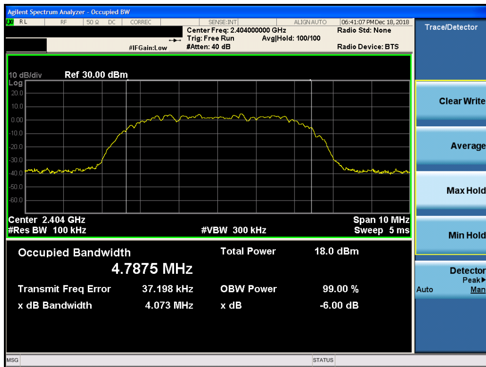
Plot 7-10. 6dB Bandwidth Plot Ant-1 (Bluetooth (HDR8), 8Mbps, ePA - Ch. 1)
