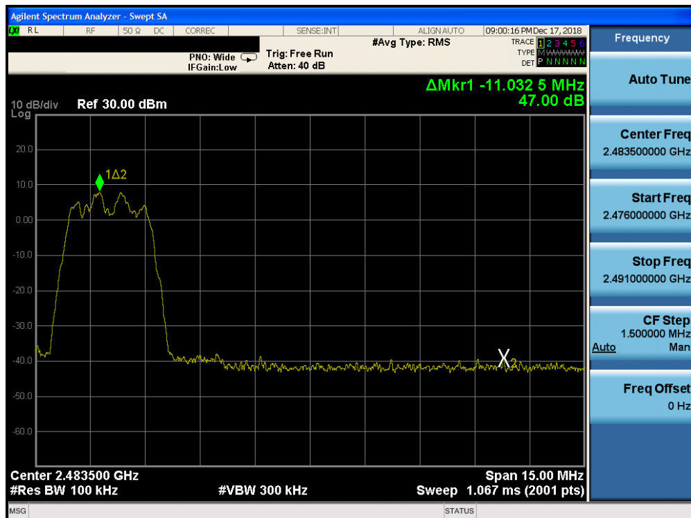
Plot 7-38. Band Edge Plot Ant-0 (Bluetooth (HDR4), ePA – Ch. 75)
