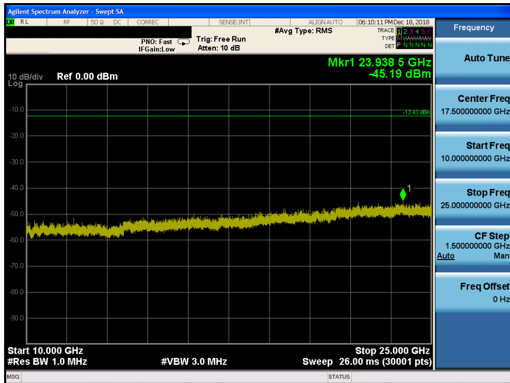
Plot 7-56. Conducted Spurious Plot Ant-1 (Bluetooth (HDR4), Mbps, ePA – Ch. 75)
