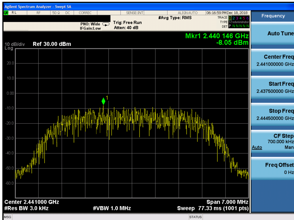
Plot 7-32. Power Spectral Density Plot Ant-1 (Bluetooth (HDR8), 8Mbps, ePA – Ch. 38)
