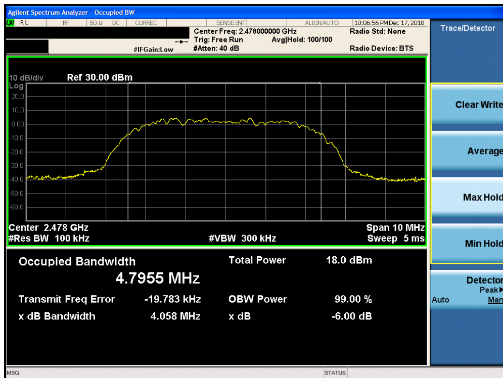
Plot 7-6. 6dB Bandwidth Plot Ant-0 (Bluetooth (HDR8), 8Mbps, ePA – Ch. 75)
