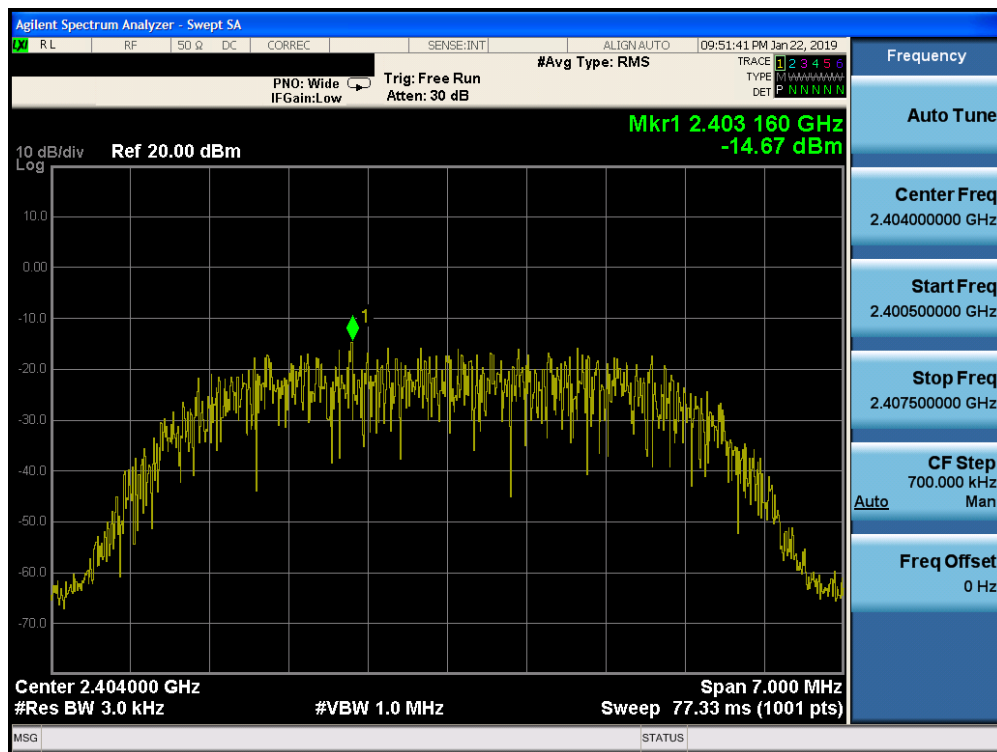
Plot 7-22. Power Spectral Density Plot Ant-0 (Bluetooth (HDR8), 8Mbps, iPA – Ch. 1)
