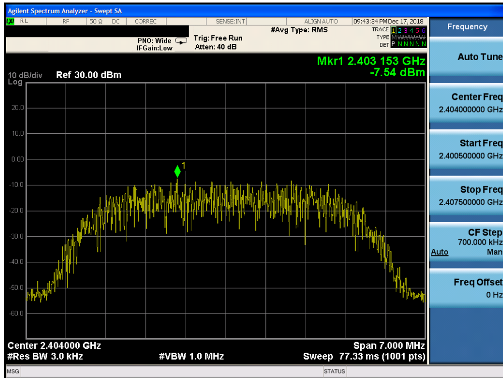
Plot 7-19. Power Spectral Density Plot Ant-0 (Bluetooth (HDR8), 8Mbps, ePA – Ch. 1)
