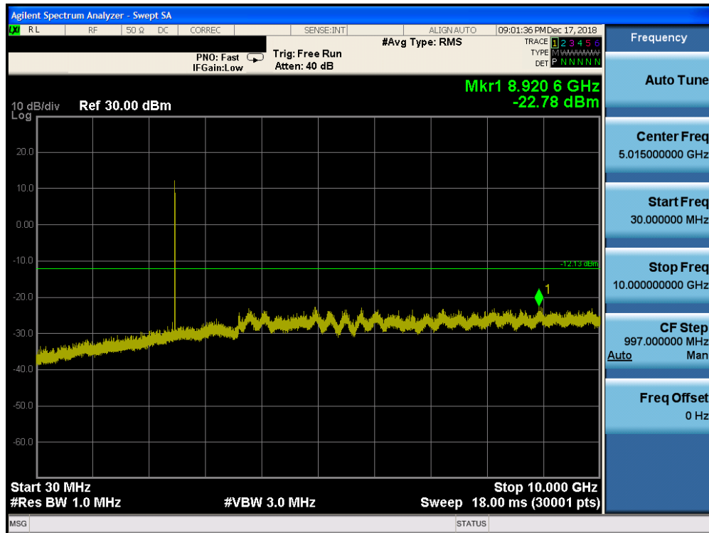
Plot 7-49. Conducted Spurious Plot Ant-0 (Bluetooth (HDR4), Mbps, ePA – Ch. 75)
