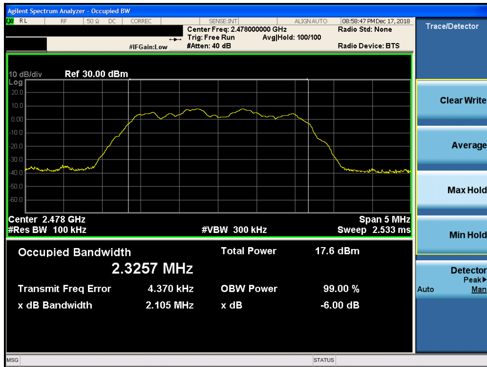
Plot 7-3. 6dB Bandwidth Plot Ant-0 (Bluetooth (HDR4), 4Mbps, ePA – Ch. 75)
