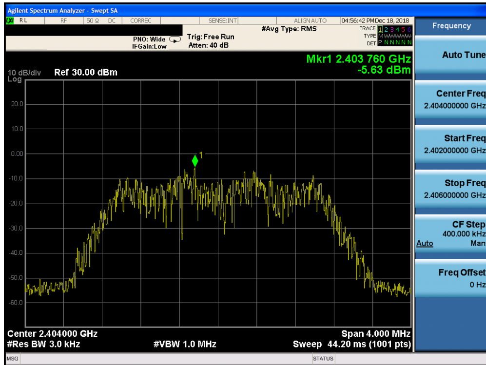
Plot 7-25. Power Spectral Density Plot Ant-1 (Bluetooth (HDR4), 4Mbps, ePA – Ch. 1)
