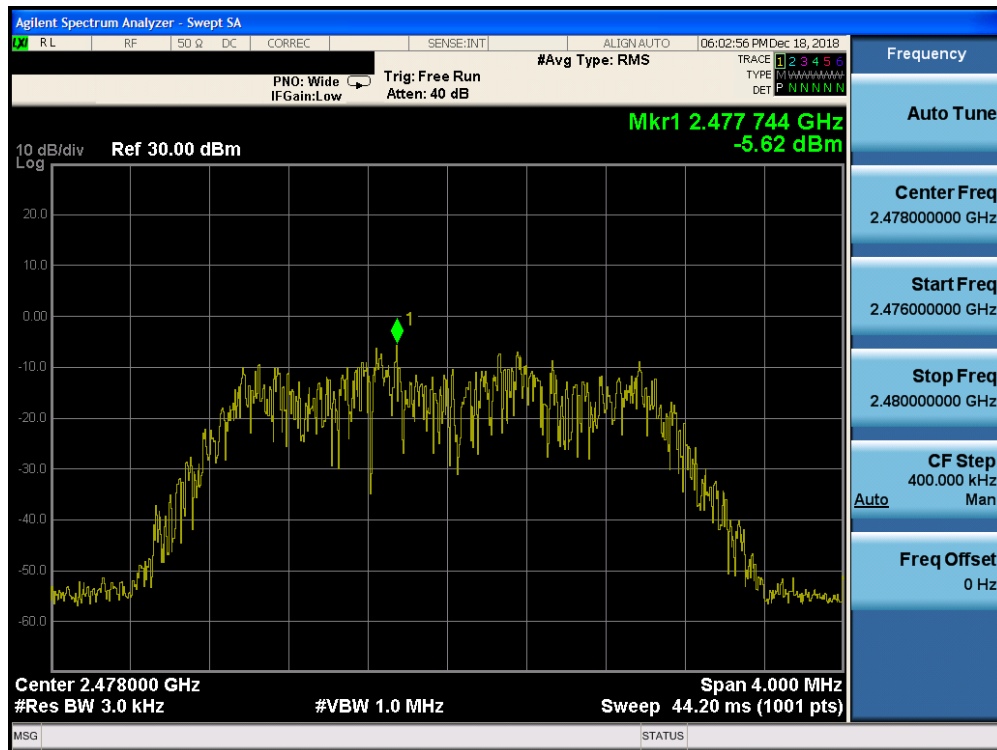
Plot 7-27. Power Spectral Density Plot Ant-1 (Bluetooth (HDR4), 4Mbps, ePA – Ch. 75)
