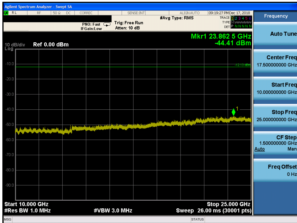
Plot 7-50. Conducted Spurious Plot Ant-0 (Bluetooth (HDR4), Mbps, ePA – Ch. 75)
