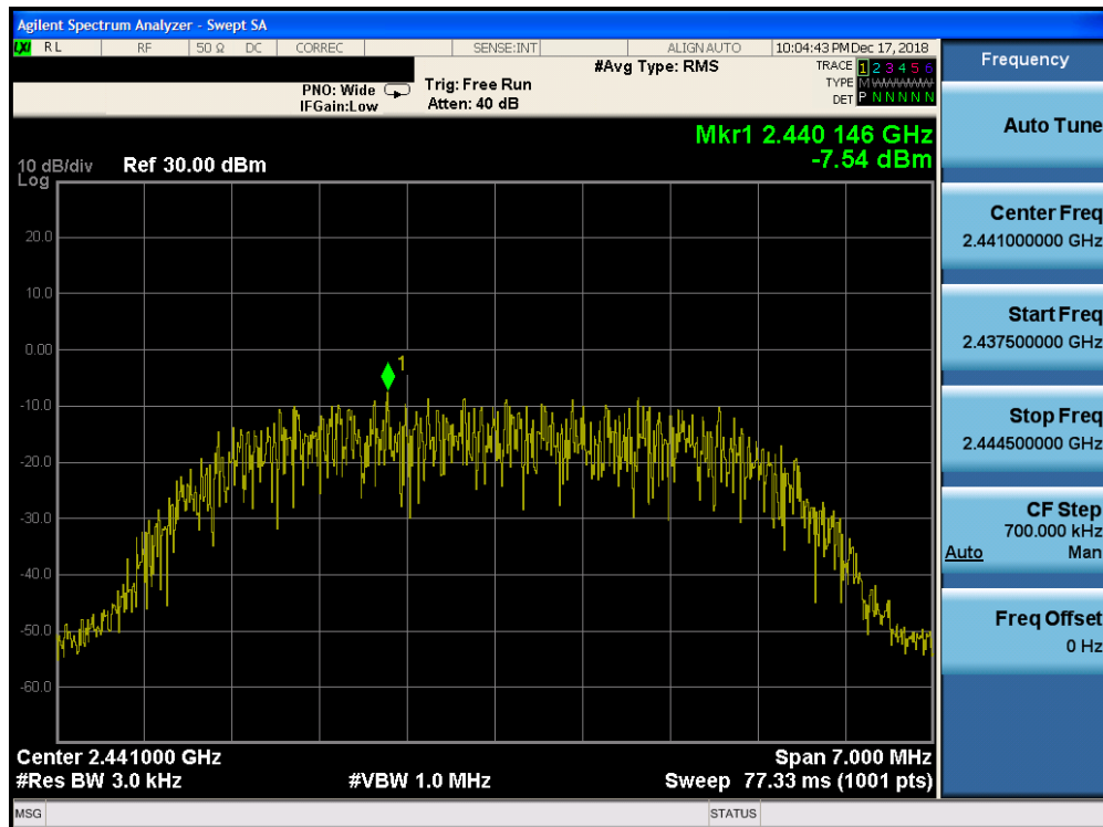
Plot 7-20. Power Spectral Density Plot Ant-0 (Bluetooth (HDR8), 8Mbps, ePA – Ch. 38)
