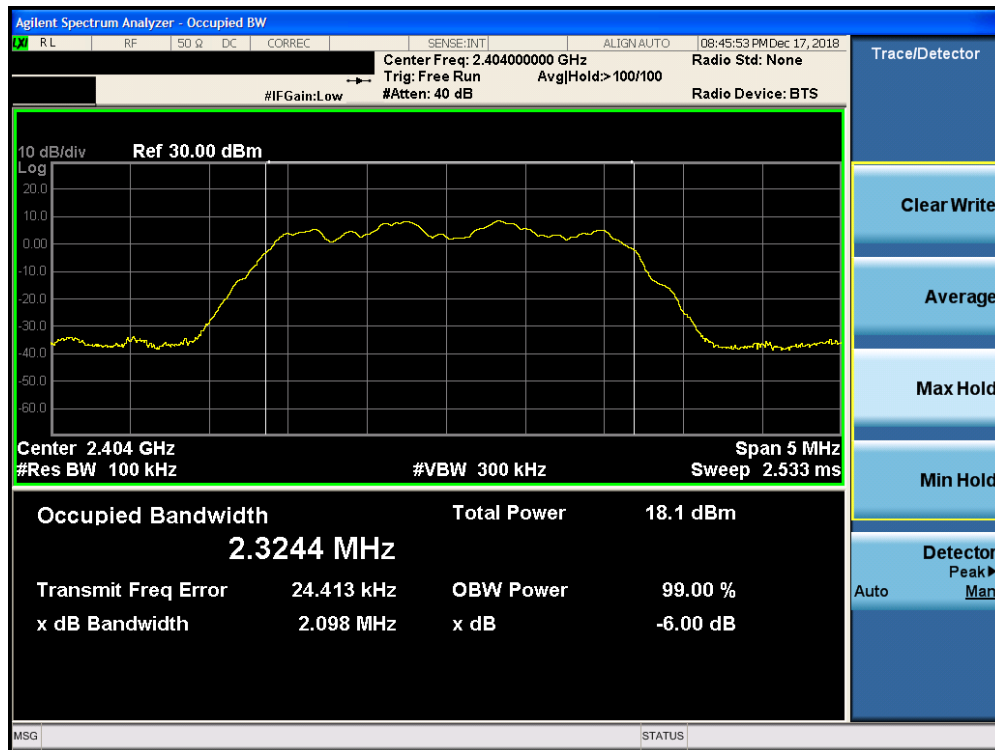
Plot 7-1. 6dB Bandwidth Plot Ant-0 (Bluetooth (HDR4), 4Mbps, ePA – Ch. 1)
