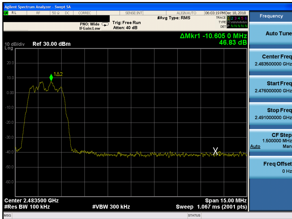
Plot 7-42. Band Edge Plot Ant-1 (Bluetooth (HDR4), ePA – Ch. 75)
