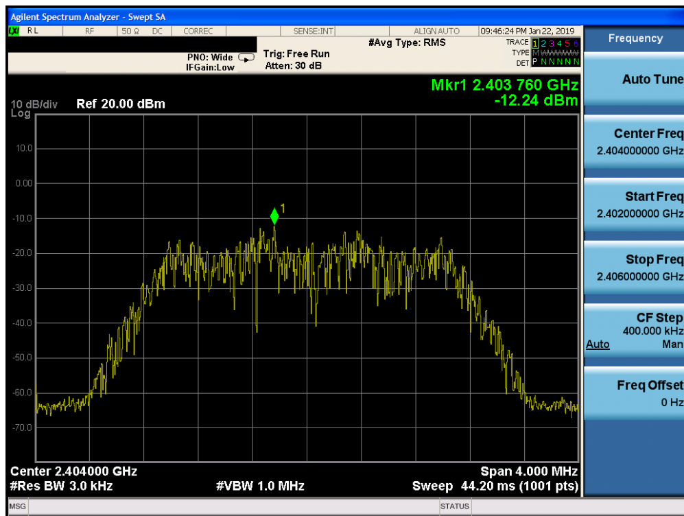
Plot 7-16. Power Spectral Density Plot Ant-0 (Bluetooth (HDR4), 4Mbps, iPA – Ch. 1)
