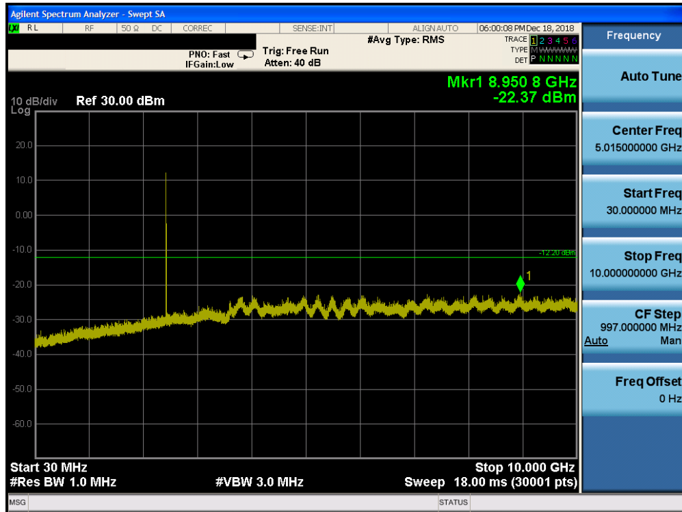
Plot 7-53. Conducted Spurious Plot Ant-1 (Bluetooth (HDR4), Mbps, ePA – Ch. 38)
