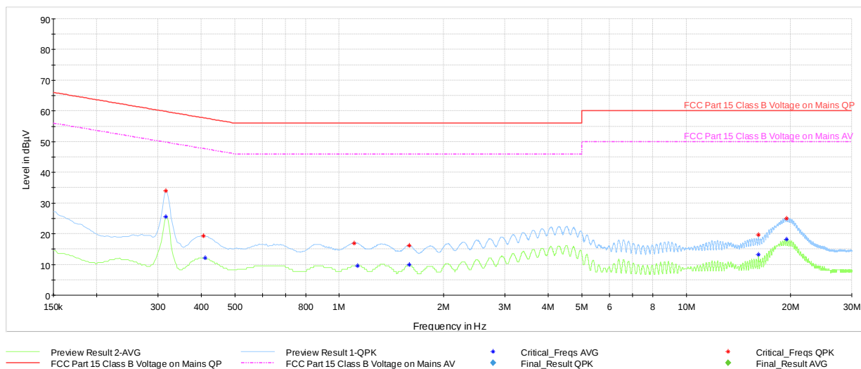
Plot 7-75. AC Line Conducted Plot with Bluetooth HDR4 ePA – Ch.1 (N, with Laptop)
