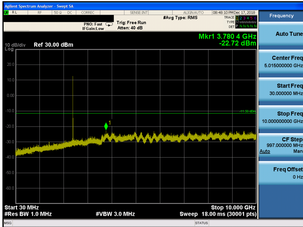
Plot 7-45. Conducted Spurious Plot Ant-0 (Bluetooth (HDR4), Mbps, ePA – Ch. 1)
