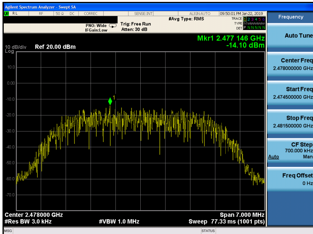
Plot 7-24. Power Spectral Density Plot Ant-0 (Bluetooth (HDR8), 8Mbps, iPA – Ch. 75)
