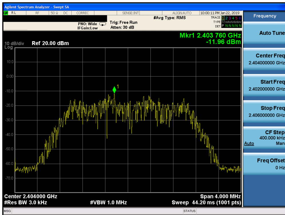
Plot 7-28. Power Spectral Density Plot Ant-1 (Bluetooth (HDR4), 4Mbps, iPA – Ch. 1)
