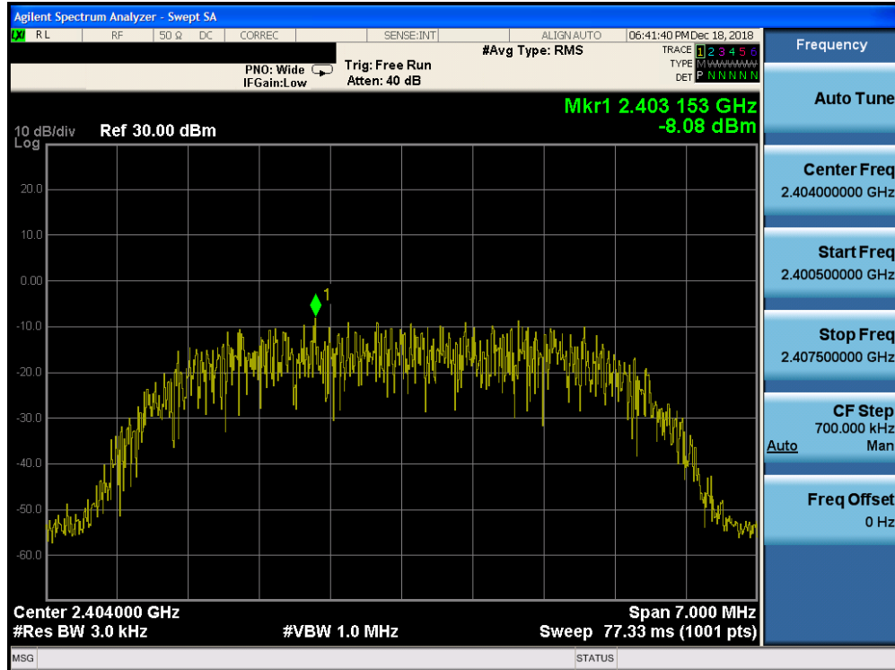
Plot 7-31. Power Spectral Density Plot Ant-1 (Bluetooth (HDR8), 8Mbps, ePA – Ch. 1)
