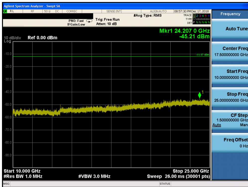
Plot 7-48. Conducted Spurious Plot Ant-0 (Bluetooth (HDR4), Mbps – Ch. 38)
