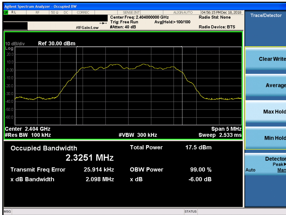
Plot 7-7. 6dB Bandwidth Plot Ant-1 (Bluetooth (HDR4), 4Mbps, ePA – Ch. 1)
