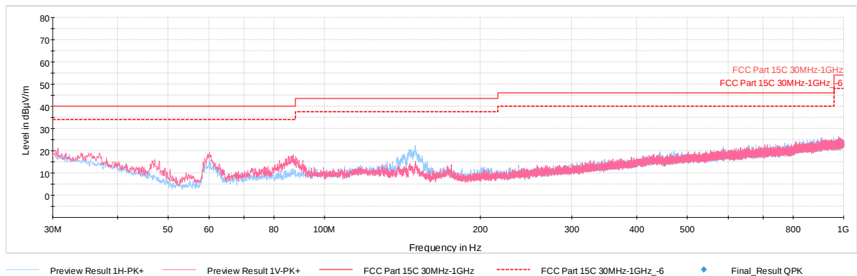
Plot 7-73. Radiated Spurious Plot below 1GHz (4Mbps, HDR4 ePA – Ch.38, Pol. H & V, with Charger)
