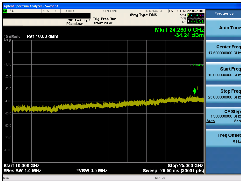
Plot 7-54. Conducted Spurious Plot Ant-1 (Bluetooth (HDR4), Mbps – Ch. 38)
