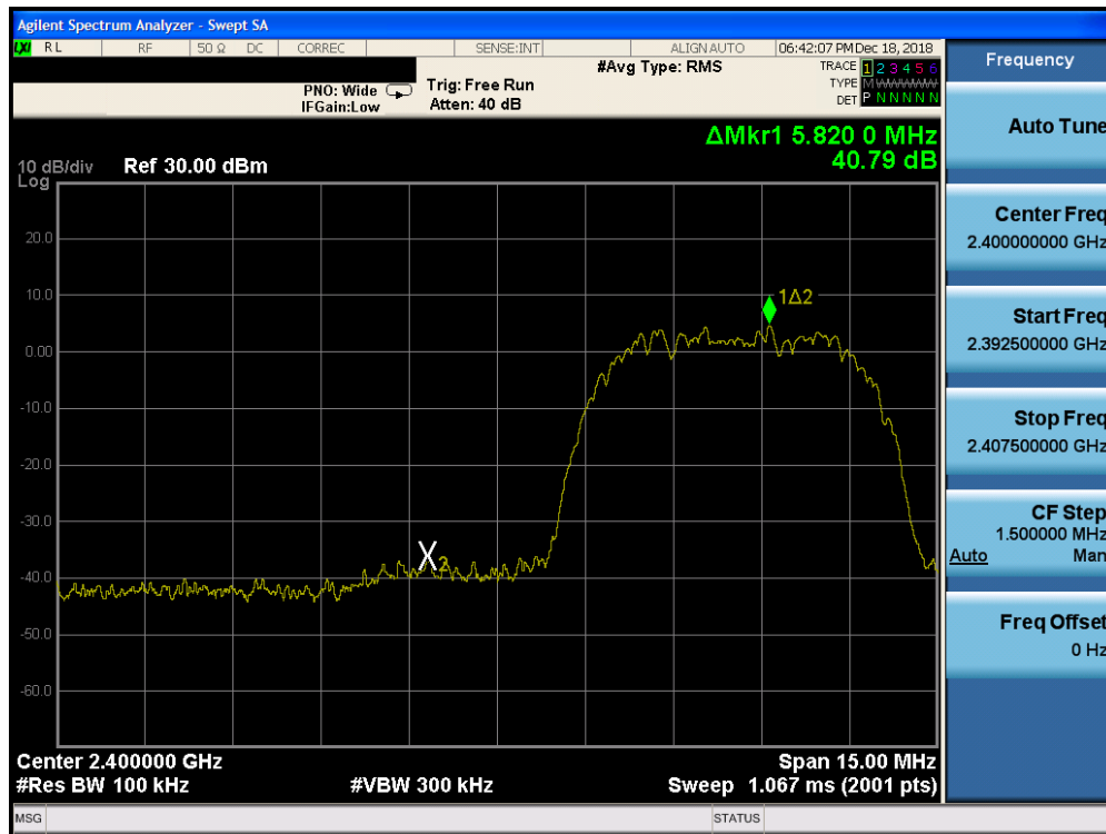
Plot 7-43. Band Edge Plot Ant-1 (Bluetooth (HDR8), ePA - Ch. 1)
