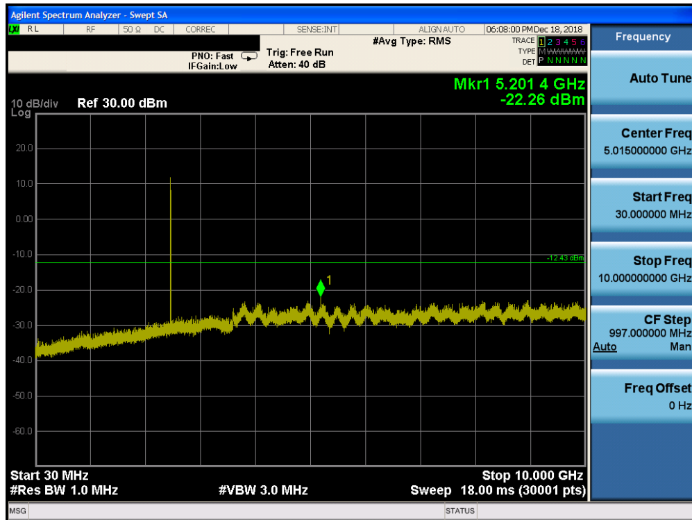
Plot 7-55. Conducted Spurious Plot Ant-1 (Bluetooth (HDR4), Mbps, ePA – Ch. 75)
