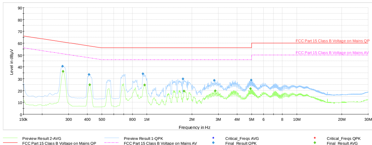
Plot 7-91. Line-Conducted Test Plot - Ch.0 (N, with AC/DC Adapter)
