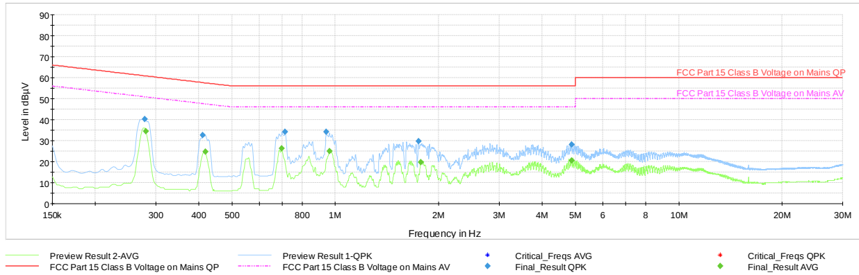
Plot 7-90. Line-Conducted Test Plot – Ch.0 (L1, with AC/DC Adapter)
