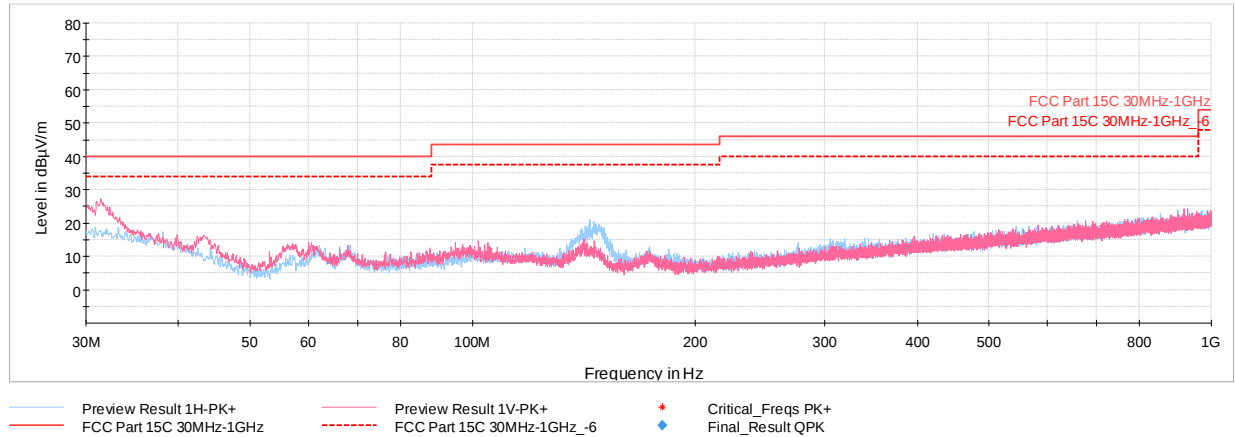
Plot 7-89. Radiated Spurious Plot below 1GHz (2.4GHz – 5GHz), with AC/DC Adapter
