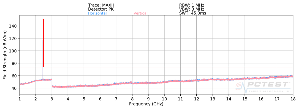
Plot 7-70. Radiated Spurious Plot above 1GHz ANT 0 (BT GFSK ePA – Ch. 39)
