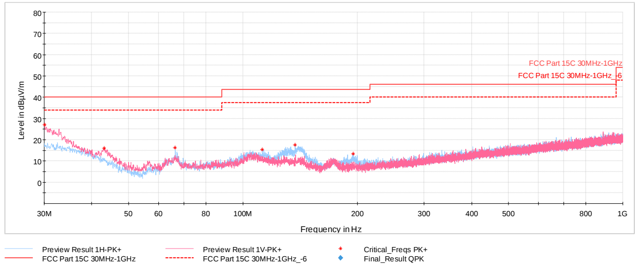
Plot 7-88. Radiated Spurious Plot below 1GHz GFSK ePA – Ch.0, with AC/DC Adapter
