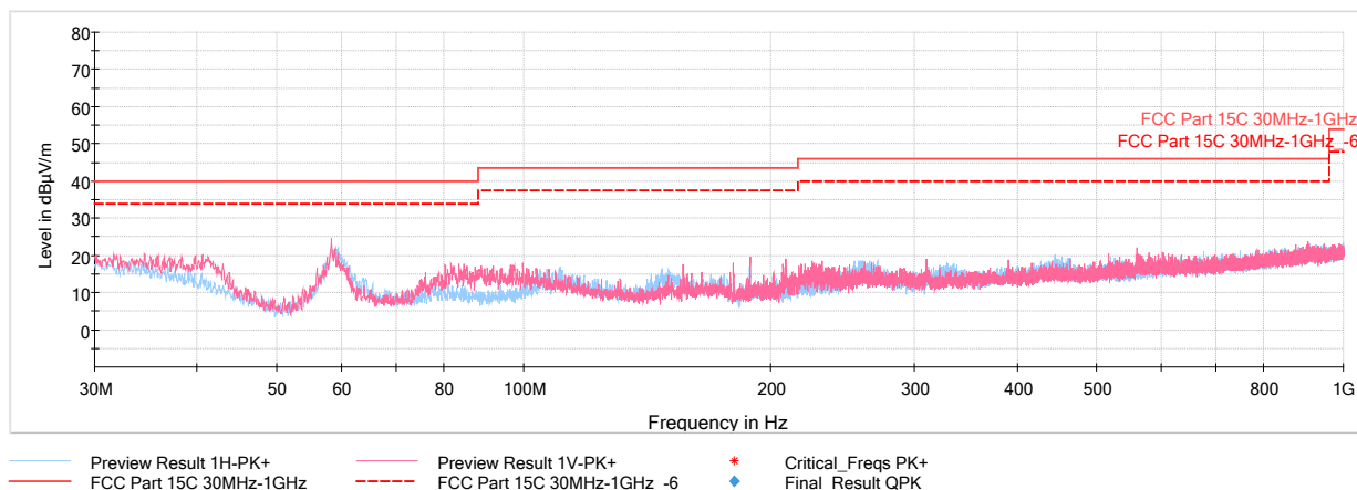
Plot 7-279. Radiated Spurious Plot below 1GHz (2.4GHz Ch 78– 5GHz Ch 36), with Laptop
