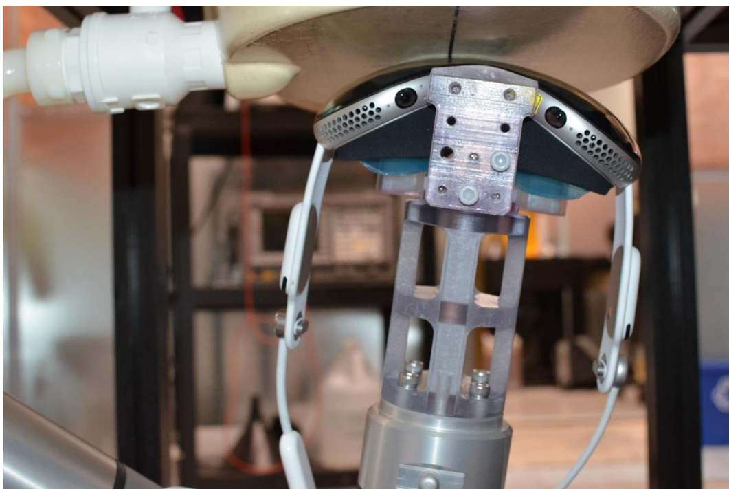
SAR Test Setup Photo 19: Antenna 1 Point 36 Extremity SAR at 0.0 cm
