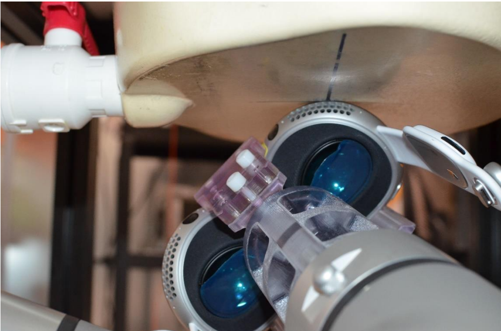
SAR Test Setup Photo 40: Antenna NB UNII_L Point 7 Extremity SAR at 0.0 cm
