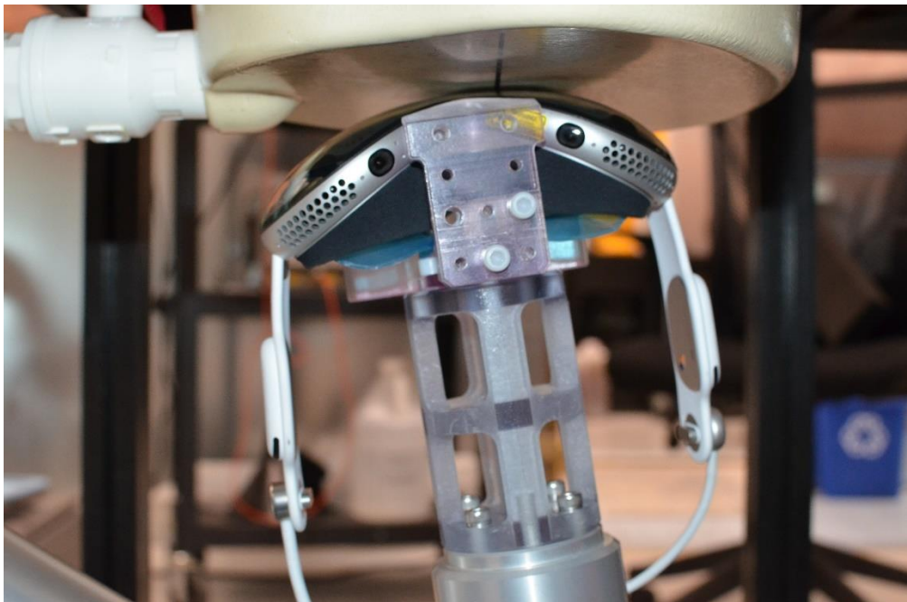
SAR Test Setup Photo 33: Antenna 2 Point 21 Extremity SAR at 0.0 cm
