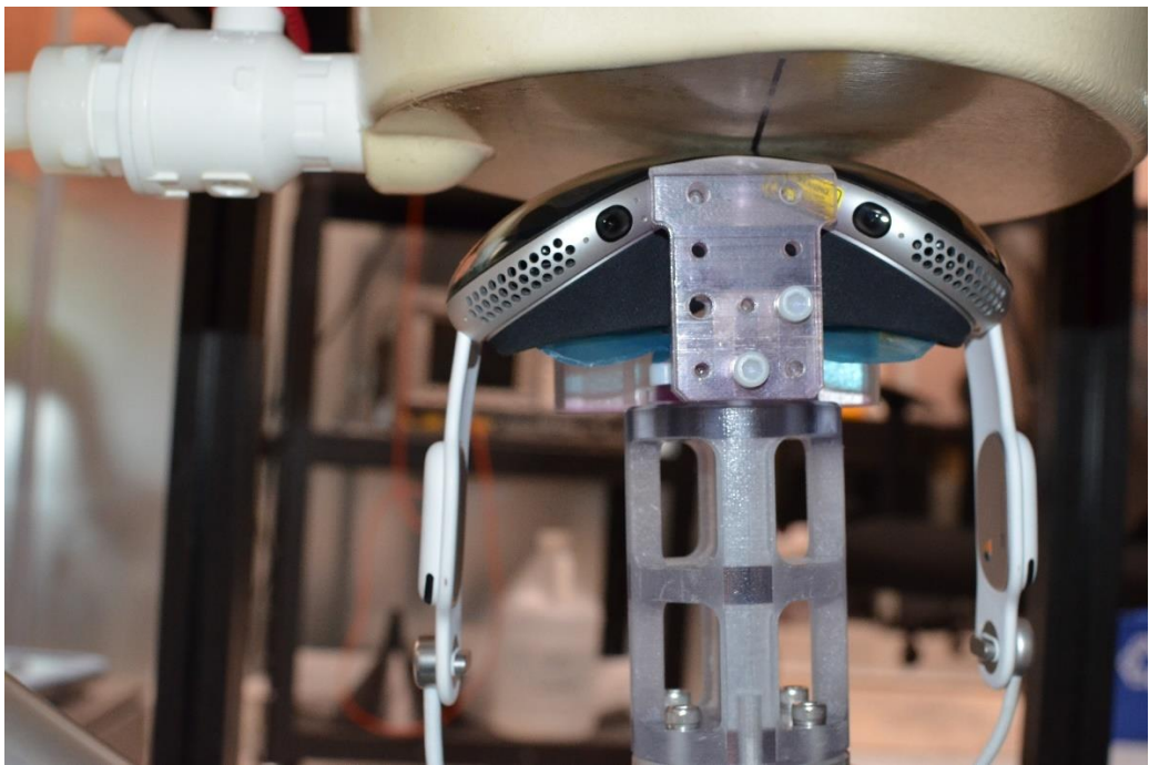
SAR Test Setup Photo 32: Antenna 2 Point 20 Extremity SAR at 0.0 cm
