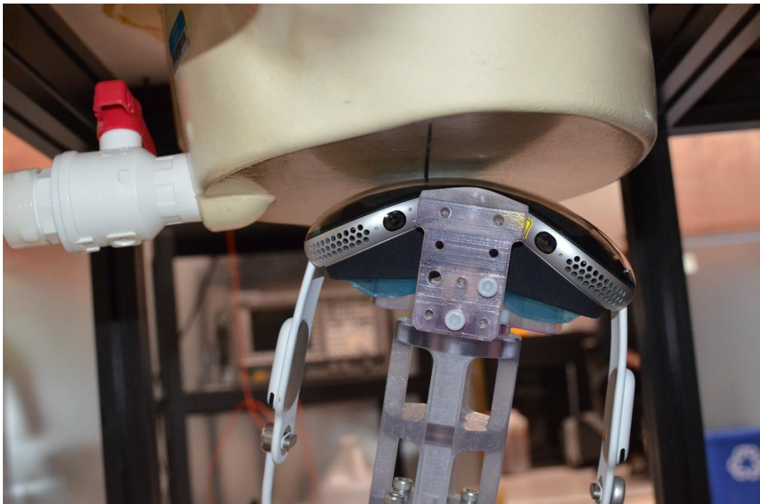
SAR Test Setup Photo 11: Antenna 1 Point 13 Extremity SAR at 0.0 cm
