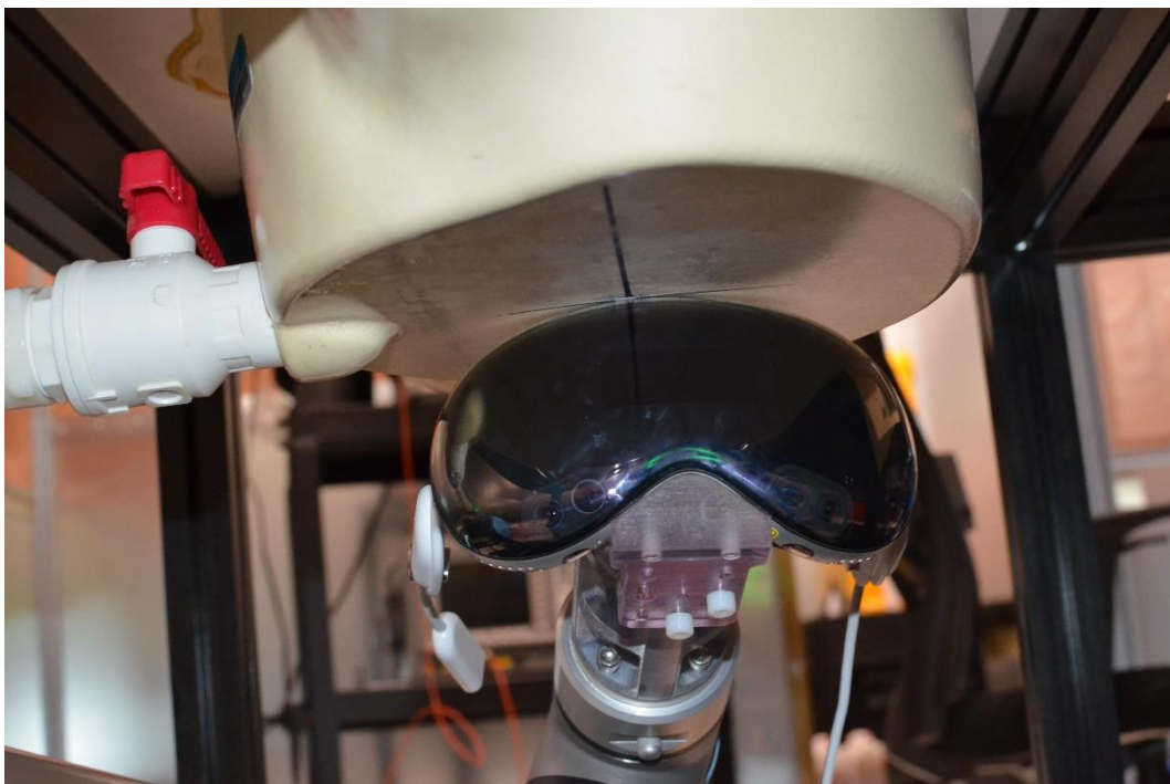
SAR Test Setup Photo 13: Antenna 1 Point 25 Extremity SAR at 0.0 cm
