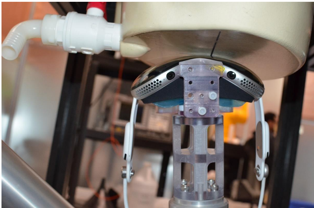
SAR Test Setup Photo 26: Antenna 2 Point 6 Extremity SAR at 0.0 cm
