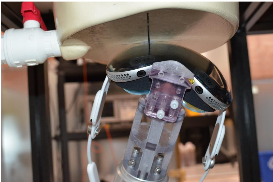
SAR Test Setup Photo 17: Antenna 1 Point 33 Extremity SAR at 0.0 cm
