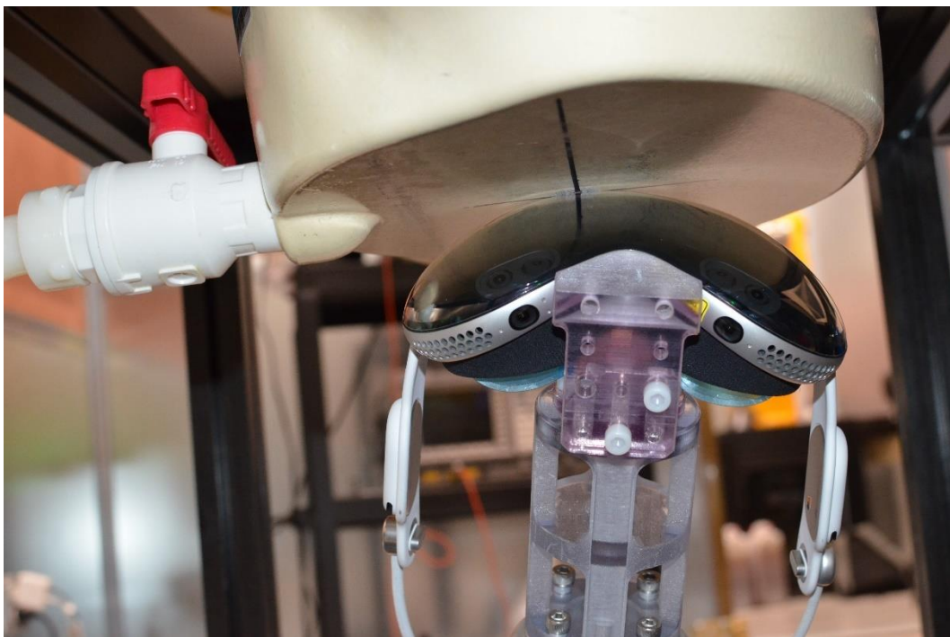
SAR Test Setup Photo 15: Antenna 1 Point 31 Extremity SAR at 0.0 cm
