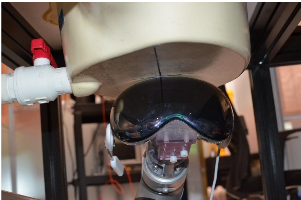
SAR Test Setup Photo 6: Antenna 1 Point 8 Extremity SAR at 0.0 cm
