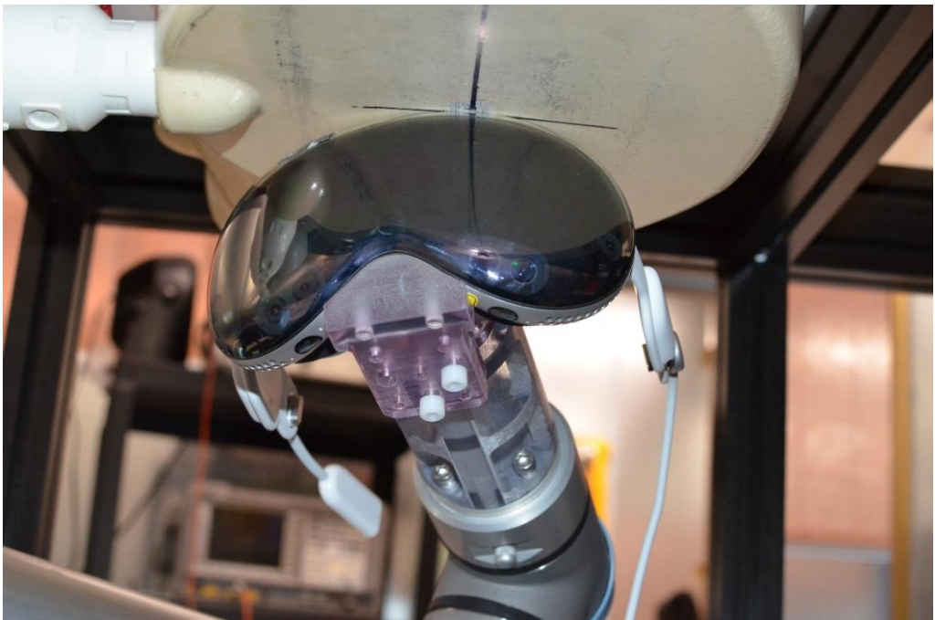
SAR Test Setup Photo 22: Antenna 2 Point 2 Extremity SAR at 0.0 cm
