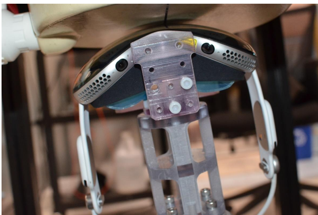
SAR Test Setup Photo 30: Antenna 2 Point 14 Extremity SAR at 0.0 cm
