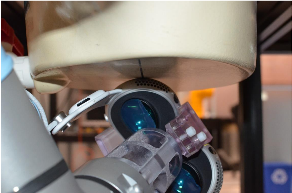
SAR Test Setup Photo 37: Antenna NB UNII_R Point 25 Extremity SAR at 0.0 cm
