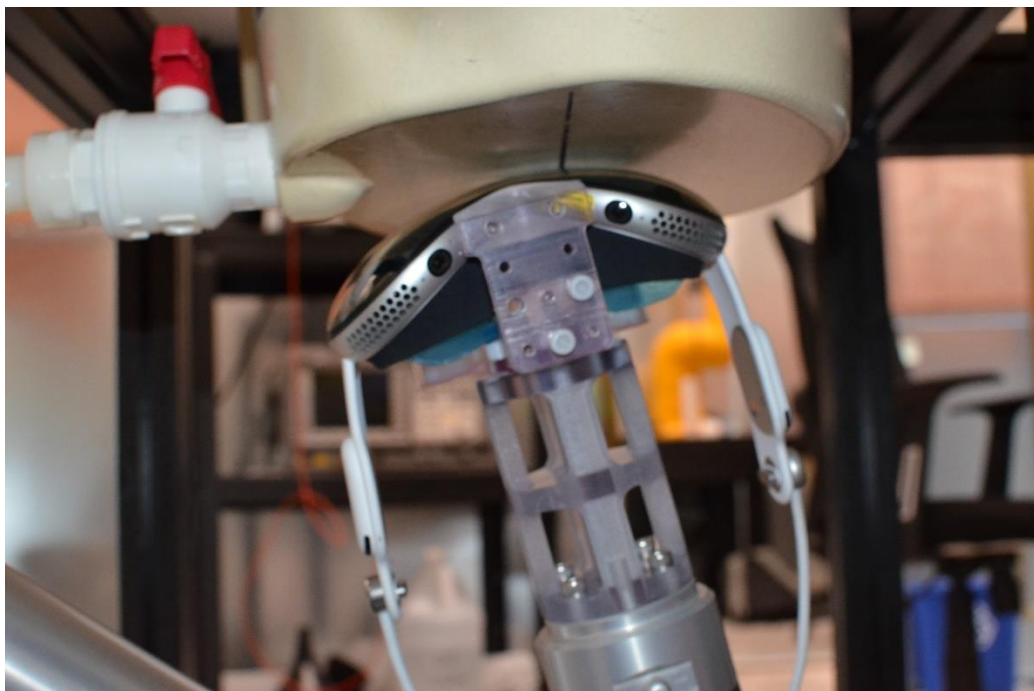
SAR Test Setup Photo 27: Antenna 2 Point 7 Extremity SAR at 0.0 cm
