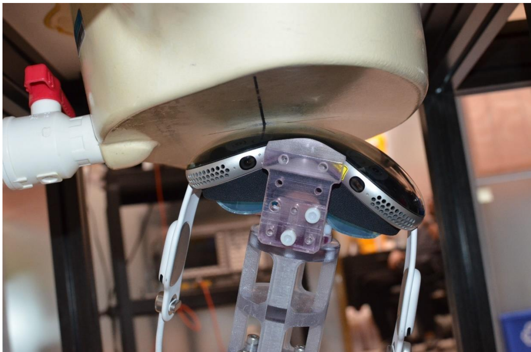
SAR Test Setup Photo 10: Antenna 1 Point 12 Extremity SAR at 0.0 cm
