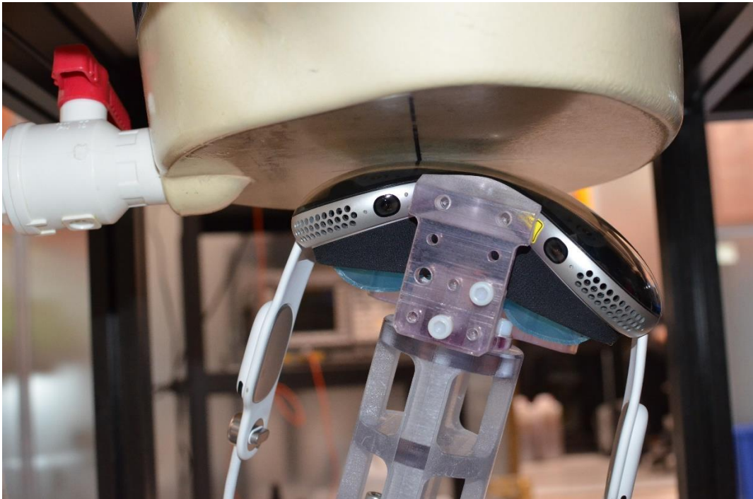
SAR Test Setup Photo 12: Antenna 1 Point 14 Extremity SAR at 0.0 cm
