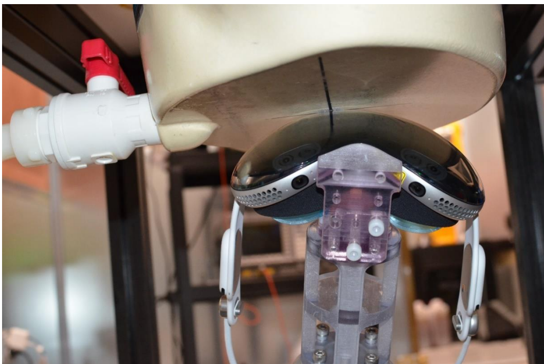
SAR Test Setup Photo 14: Antenna 1 Point 30 Extremity SAR at 0.0 cm
