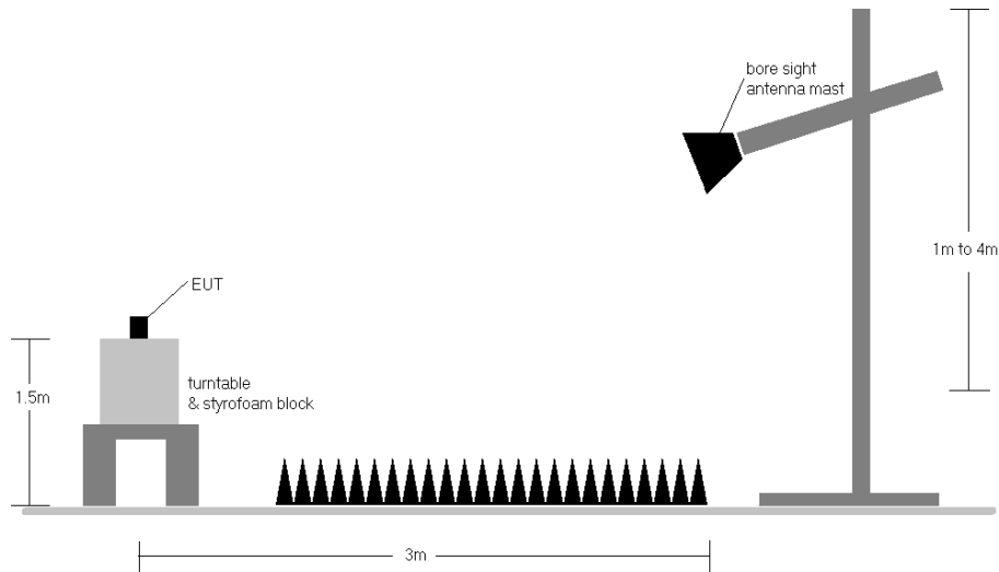
Figure 7-6. Test Instrument & Measurement Setup >1 GHz
