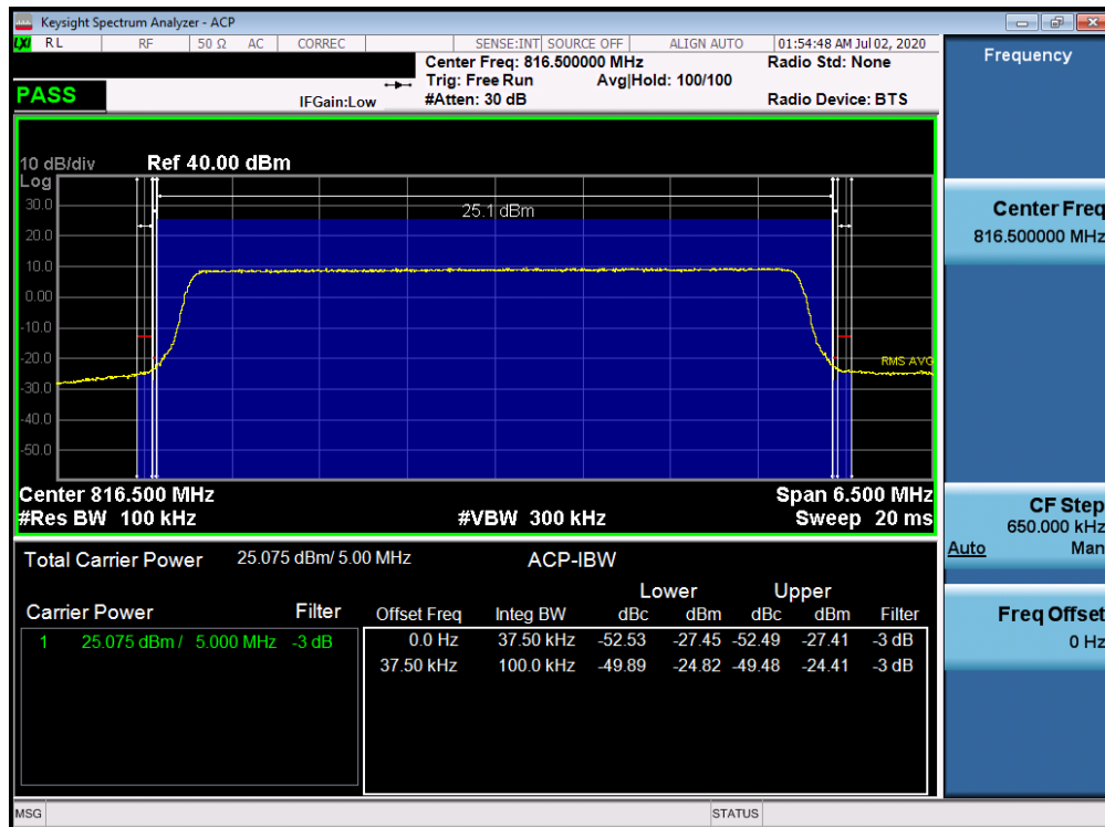
Plot 7-20. Channel Edge Plot (LTE Band 26 - 5MHz QPSK - Low Channel)
