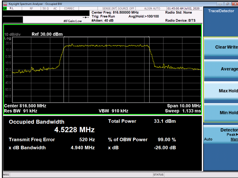
Plot 7-5. Occupied Bandwidth Plot (LTE Band 26 - 5MHz 16-QAM - Full RB Configuration)
