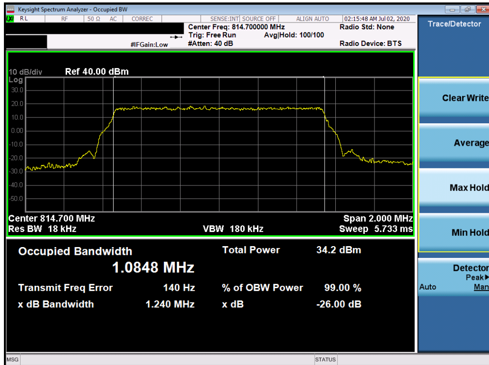
Plot 7-10. Occupied Bandwidth Plot (LTE Band 26 - 1.4MHz QPSK - Full RB Configuration)
