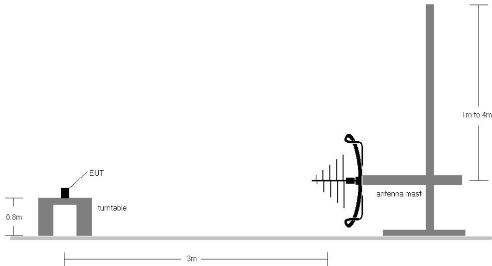
Figure 7-5. Test Instrument & Measurement Setup < 1GHz
