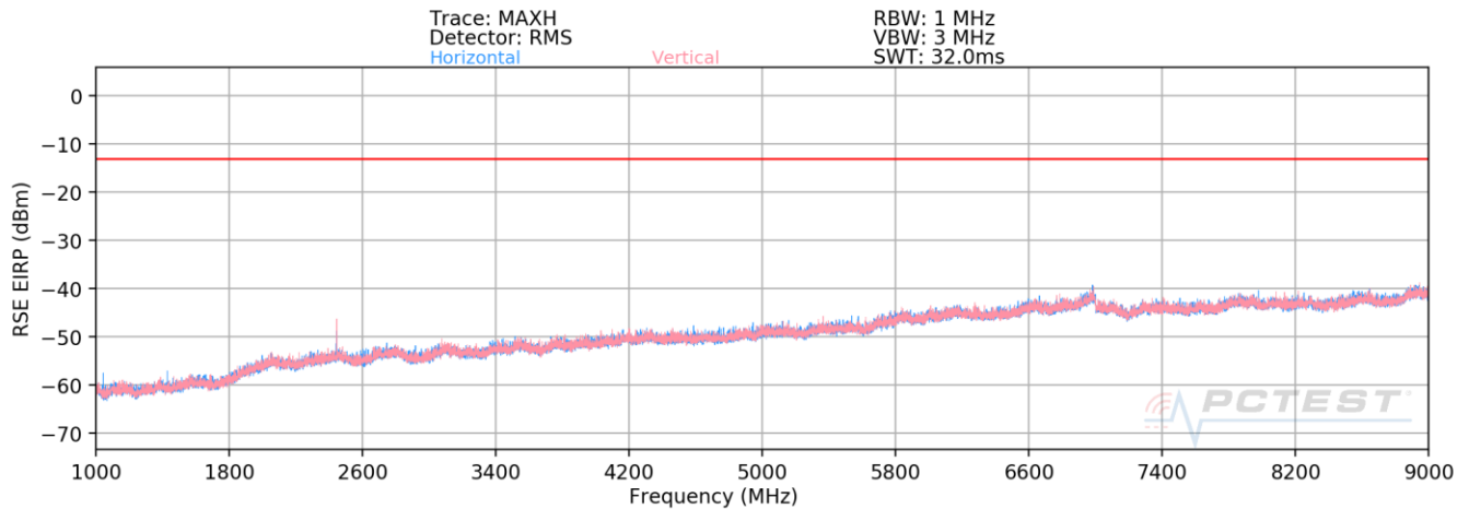
Plot 7-27. Radiated Spurious Emissions Above 1GHz (Band 26)
