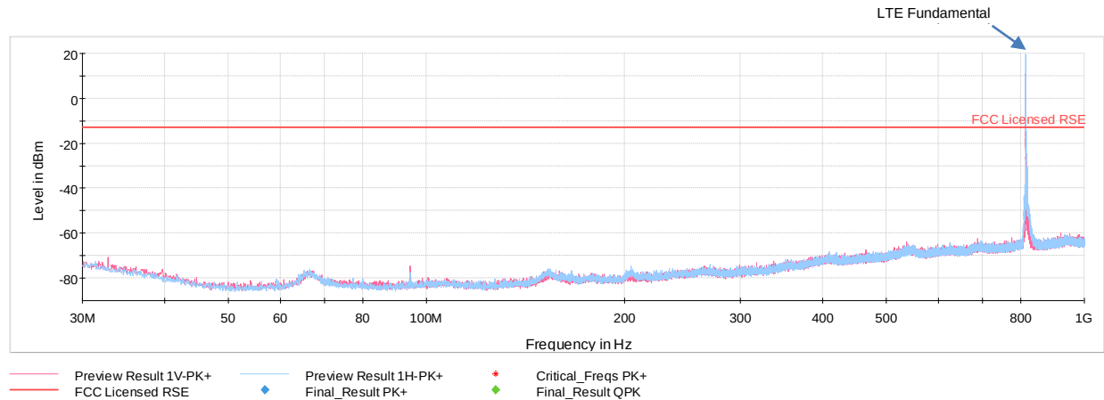
Plot 7-26. Radiated Spurious Emissions Below 1GHz (Band 26)
