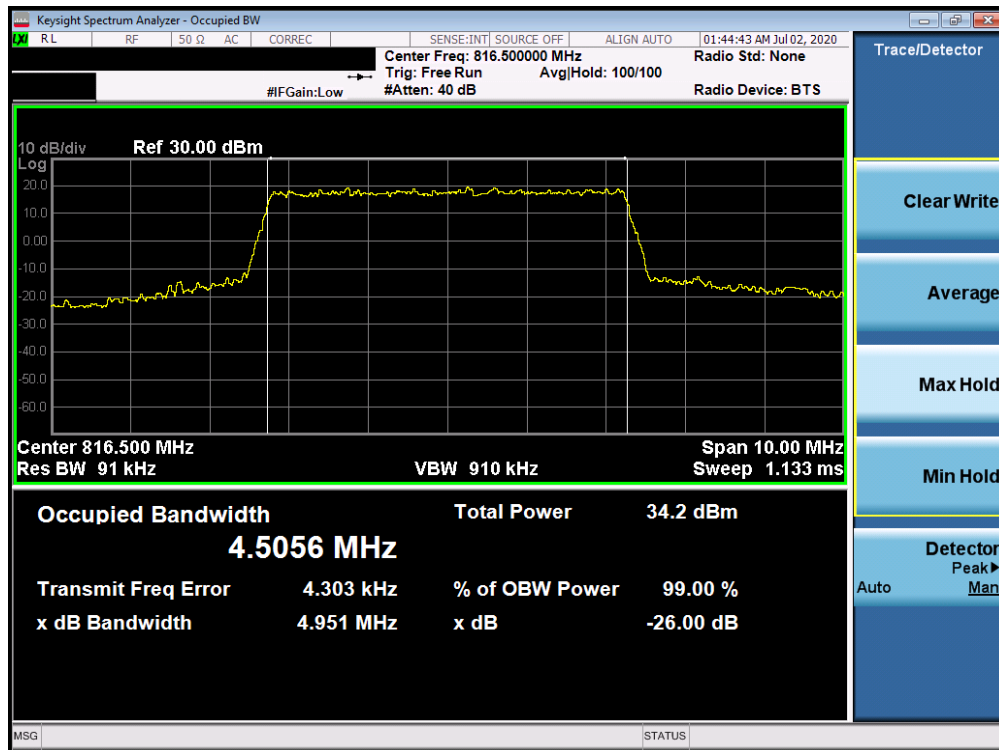
Plot 7-4. Occupied Bandwidth Plot (LTE Band 26 - 5MHz QPSK - Full RB Configuration)
