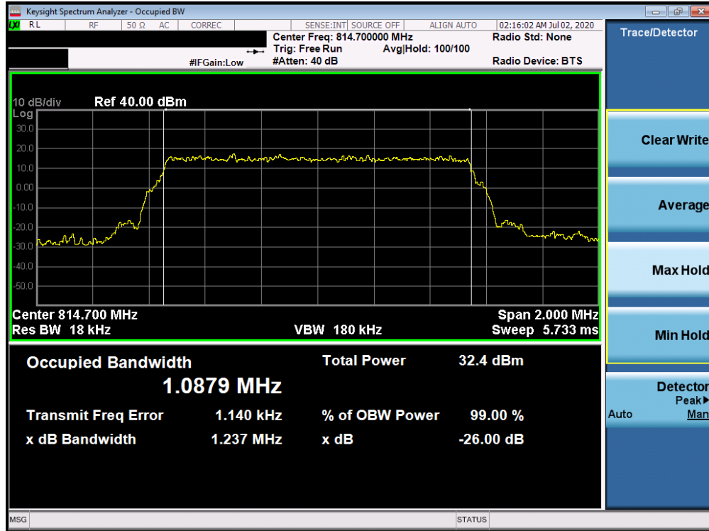
Plot 7-11. Occupied Bandwidth Plot (LTE Band 26 - 1.4MHz 16-QAM - Full RB Configuration)
