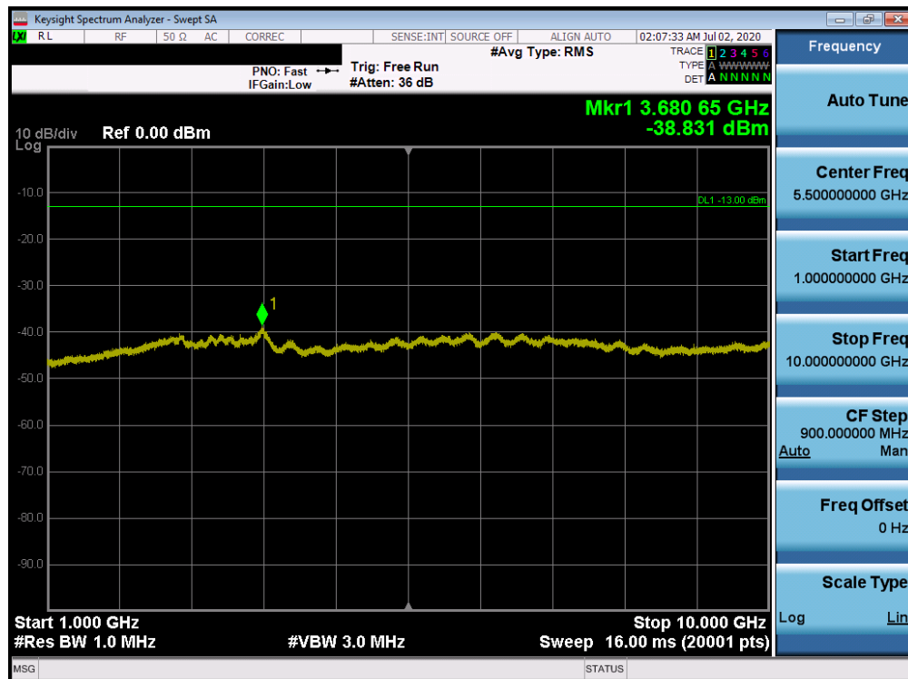
Plot 7-18. Conducted Spurious Plot (LTE Band 26 - 5MHz QPSK - RB Size 1, RB Offset 0 - High Channel)
