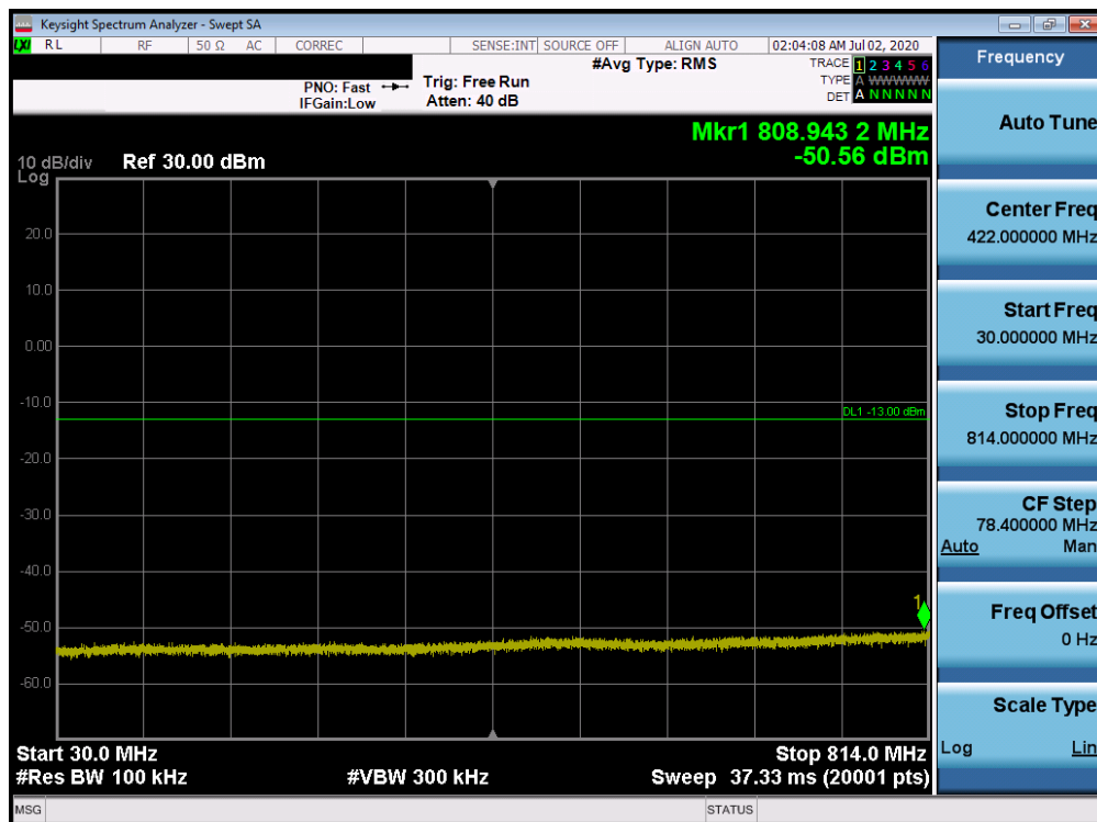
Plot 7-16. Conducted Spurious Plot (LTE Band 26 - 5MHz QPSK - RB Size 1, RB Offset 0 - High Channel)
