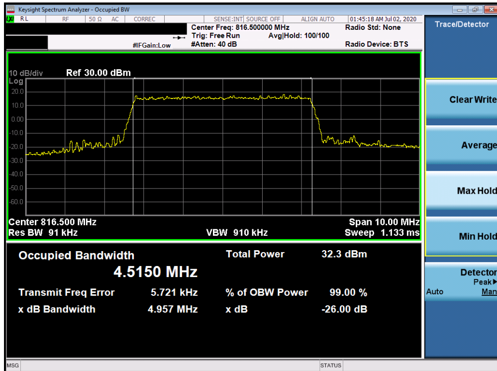
Plot 7-6. Occupied Bandwidth Plot (LTE Band 26 - 5MHz 64-QAM - Full RB Configuration)
