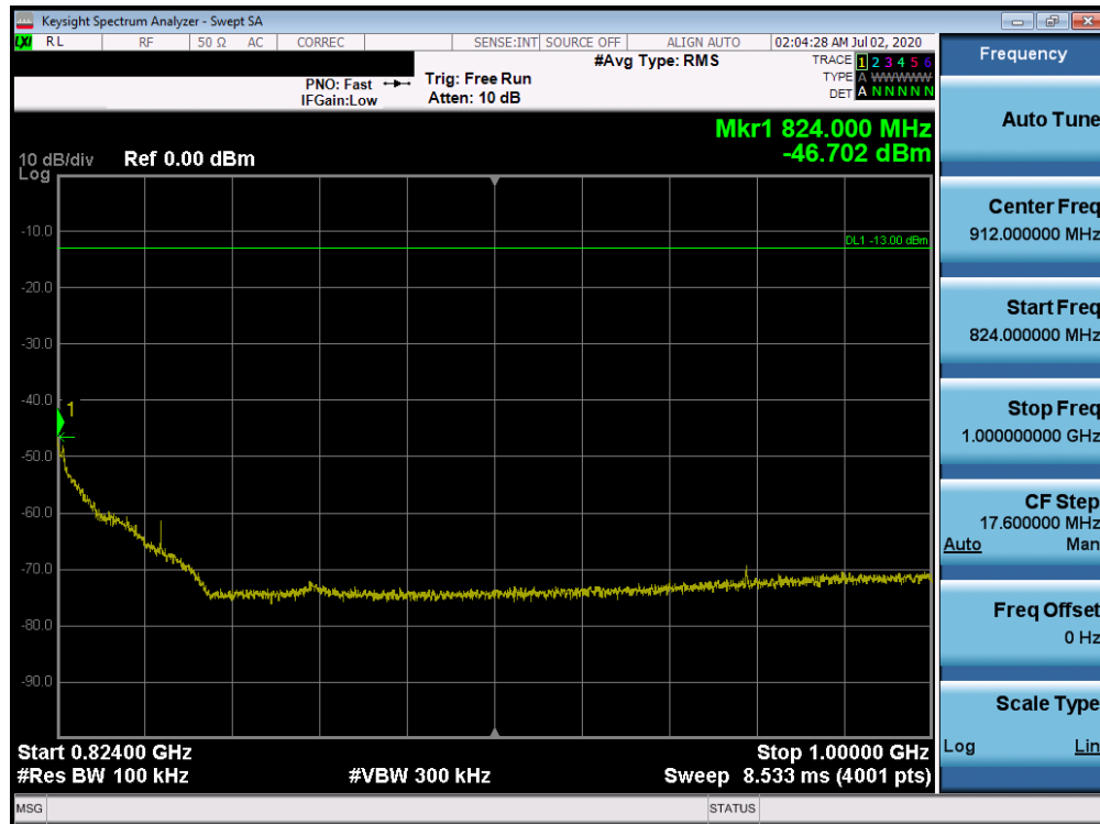
Plot 7-17. Conducted Spurious Plot (LTE Band 26 - 5MHz QPSK - RB Size 1, RB Offset 0 - High Channel)
