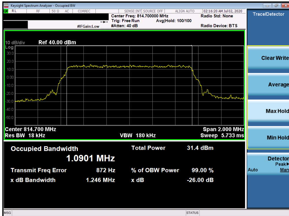
Plot 7-12. Occupied Bandwidth Plot (LTE Band 26 - 1.4MHz 64-QAM - Full RB Configuration)
