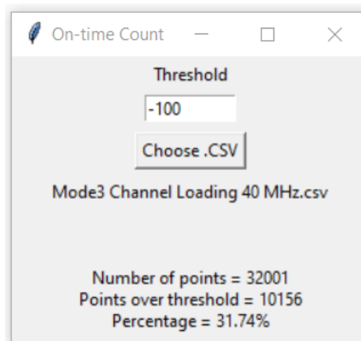
Figure 9-16 5510MHz - Channel Loading Calculation - Mode 3 (40MHz)
