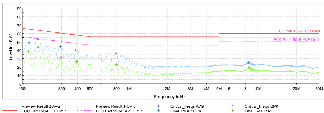
Plot 7-114. Line Conducted Plot with 802.11n CDD Ch.6 (L1, with AC/DC Adapter)
