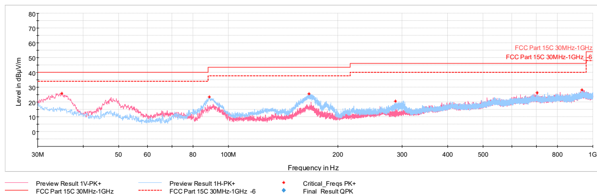
Plot 7-113. Radiated Spurious Plot below 1GHz CDD Ch.6, with AC/DC Adapter
