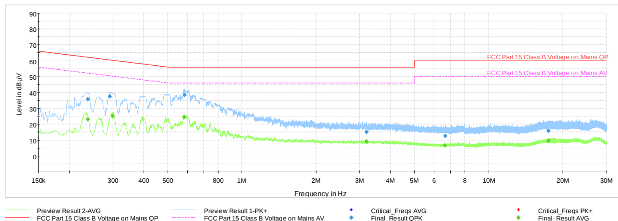
Plot 7-188. Line Conducted Plot with CDD Primary 802.11n – Ch. 6 (N, with Adapter)
