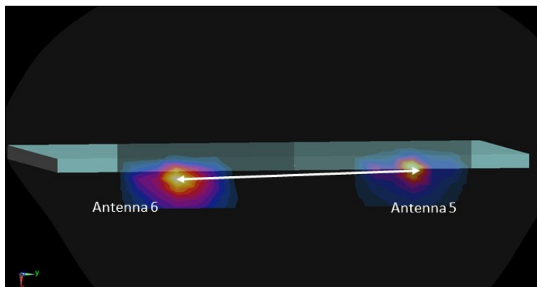
Figure 11-29 Right Edge Spatial Separation for Antenna 5 and Antenna 6
