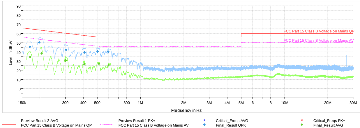
Plot 7-114. Line-Conducted Test Plot (L1, with AC/DC Adapter)
