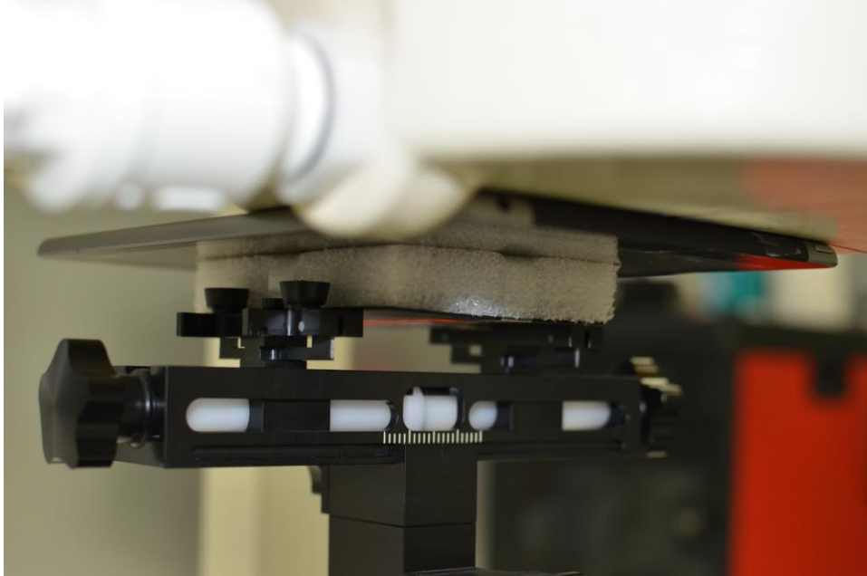
SAR Test Setup Photo 1: Back Side at 0.0 cm – 2G/3G/4G
