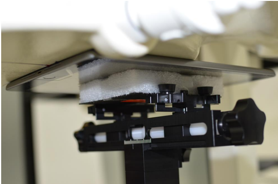
SAR Test Setup Photo 2: Back Side at 0.0 cm – WLAN/Bluetooth
