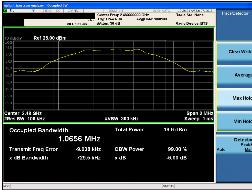
Plot 7-3. 6dB Bandwidth Plot (Bluetooth (LE), ePA – Ch. 39)
