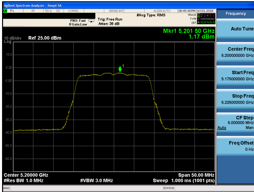
Plot 7-107. Power Spectral Density Plot CDD CORE 0 (20MHz BW 802.11n (UNII Band 1) – Ch. 40) - ISED
