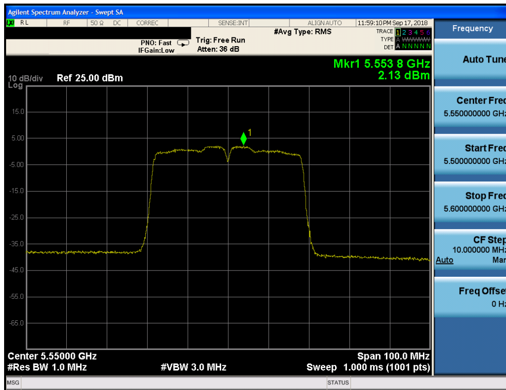
Plot 7-147. Power Spectral Density Plot CDD CORE 0 (40MHz BW 802.11n (UNII Band 2C) – Ch. 110)
