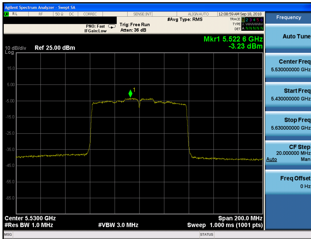
Plot 7-151. Power Spectral Density Plot CDD CORE 0 (80MHz BW 802.11ac (UNII Band 2C) – Ch. 106)
