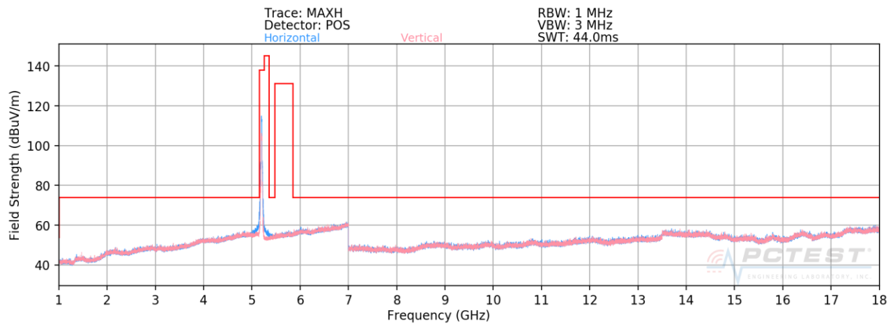
Plot 7-181. Radiated Spurious Plot above 1GHz SISO CORE 1 (802.11n – U1 Ch. 40)
