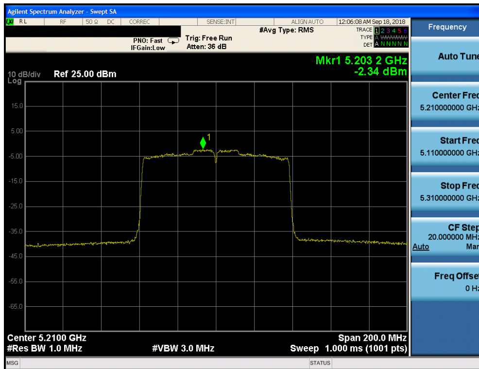
Plot 7-125. Power Spectral Density Plot CDD CORE 0 (80MHz BW 802.11ac (UNII Band 1) – Ch. 42)
