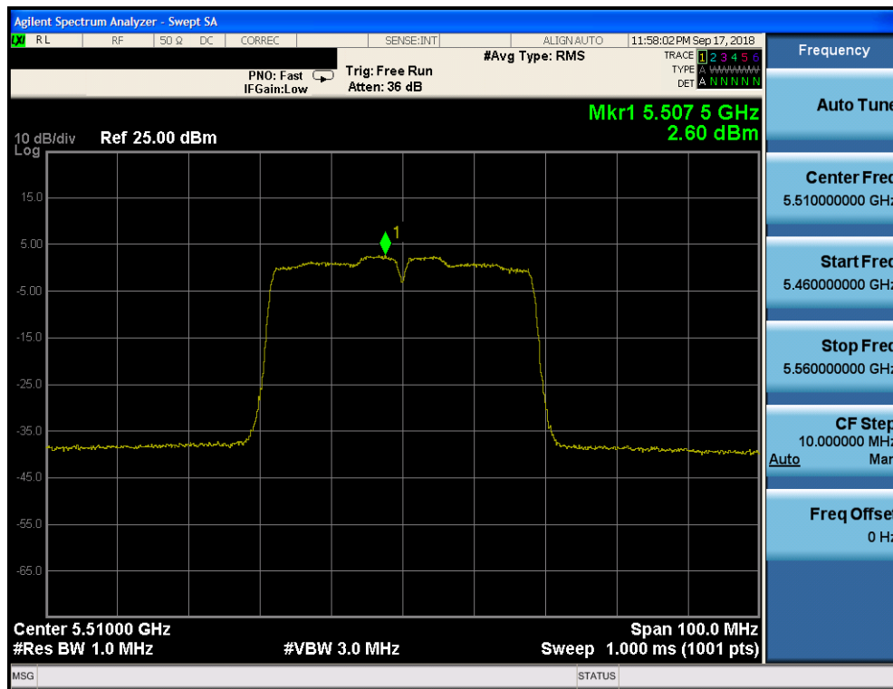
Plot 7-145. Power Spectral Density Plot CDD CORE 0 (40MHz BW 802.11n (UNII Band 2C) – Ch. 102)
