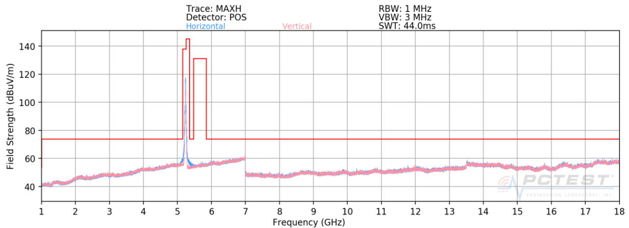
Plot 7-169. Radiated Spurious Plot above 1GHz SISO CORE 0 (802.11n – U1 Ch. 48)
