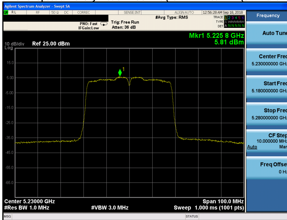
Plot 7-124. Power Spectral Density Plot CDD CORE 1 (40MHz BW 802.11n (UNII Band 1) – Ch. 46)
