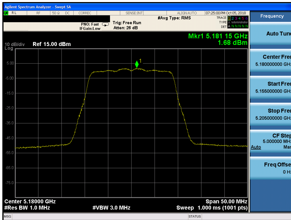
Plot 7-105. Power Spectral Density Plot CDD CORE 0 (20MHz BW 802.11n (UNII Band 1) – Ch. 36) - ISED
