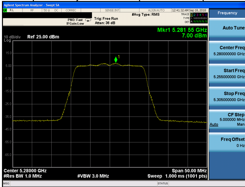
Plot 7-130. Power Spectral Density Plot CDD CORE 1 (20MHz BW 802.11n (UNII Band 2A) – Ch. 56)
