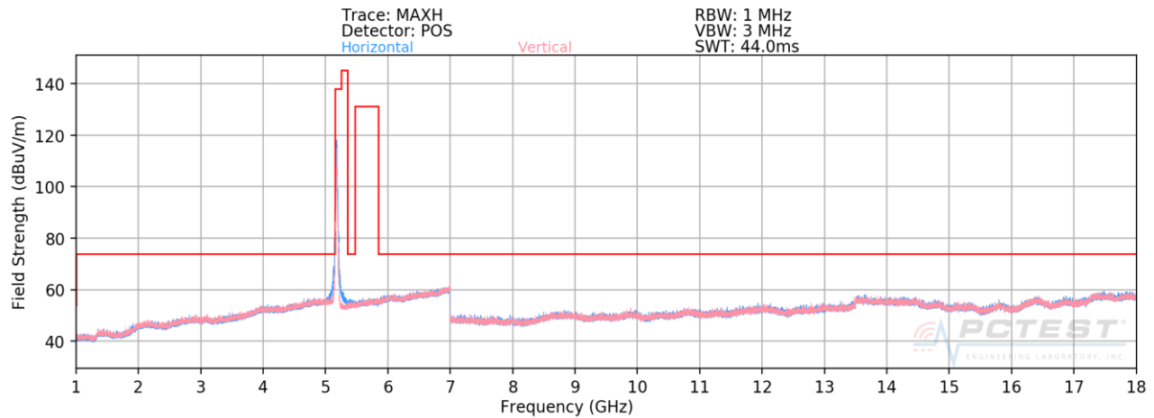
Plot 7-167. Radiated Spurious Plot above 1GHz SISO Core 0 (802.11n – U1 Ch. 36)
