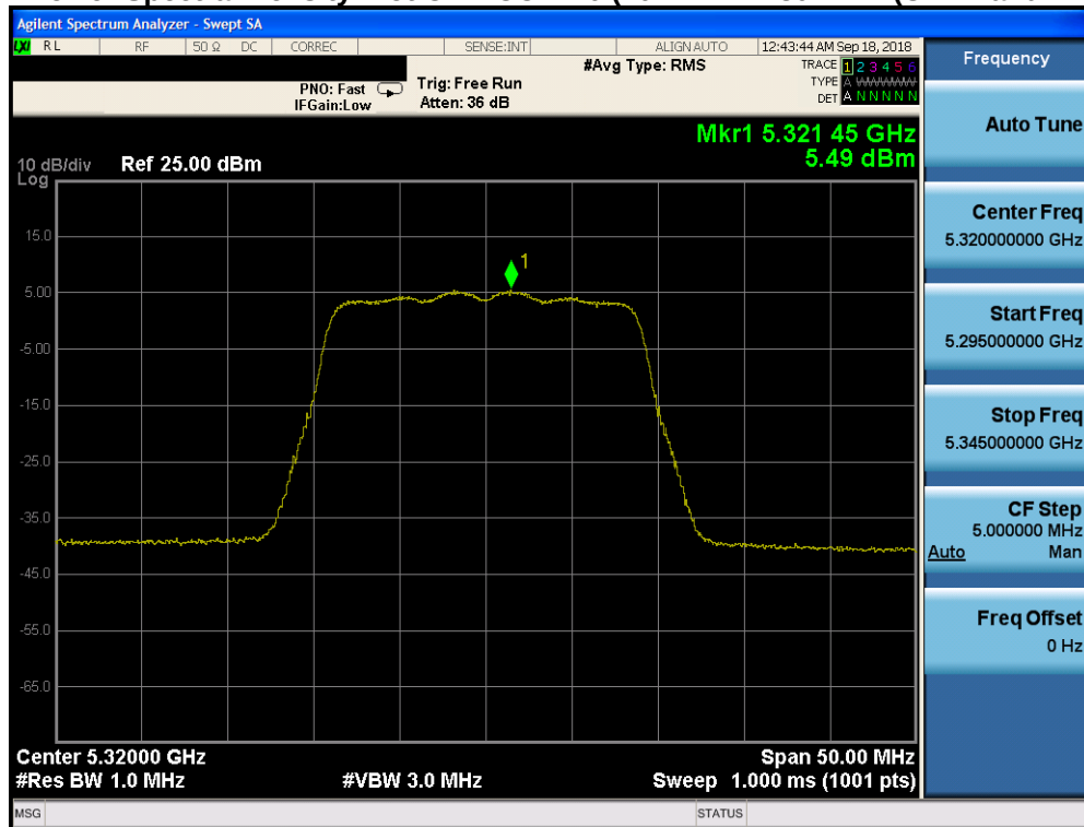
Plot 7-132. Power Spectral Density Plot CDD CORE 1 (20MHz BW 802.11n (UNII Band 2A) – Ch. 64)
