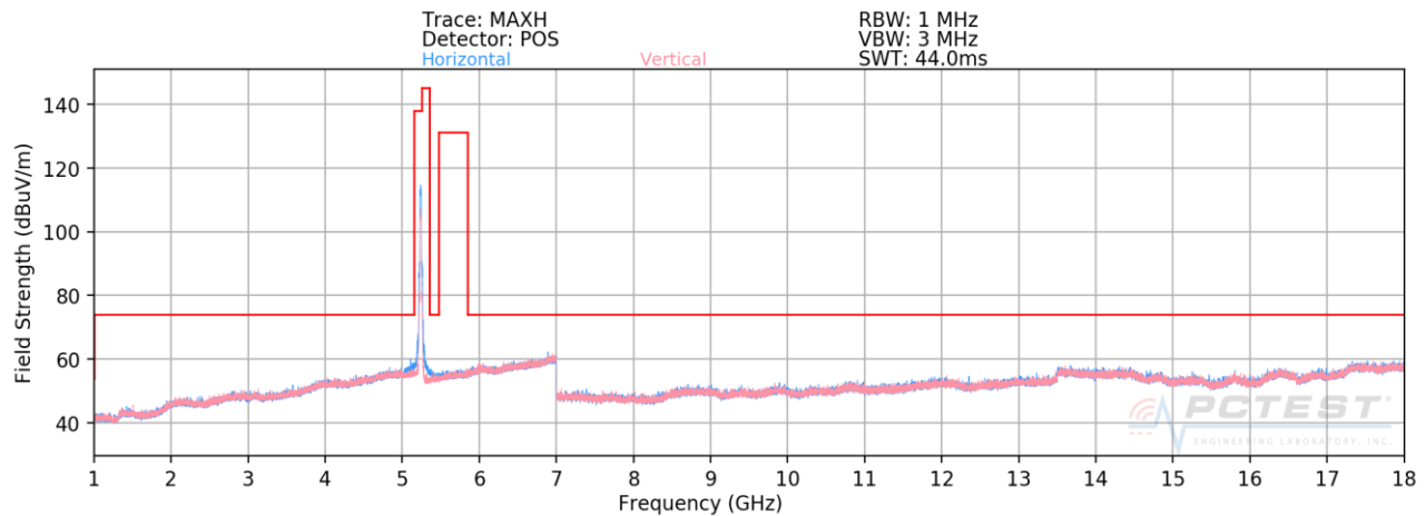
Plot 7-182. Radiated Spurious Plot above 1GHz SISO CORE 1 (802.11n – U1 Ch. 48)
