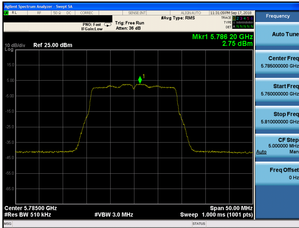
Plot 7-157. Power Spectral Density Plot CDD CORE 0 (20MHz BW 802.11n (UNII Band 3) – Ch. 157)
