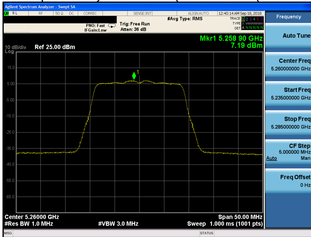
Plot 7-128. Power Spectral Density Plot CDD CORE 1 (20MHz BW 802.11n (UNII Band 2A) – Ch. 52)
