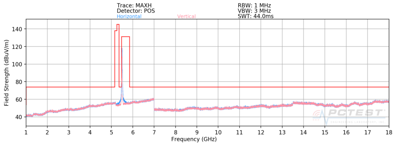
Plot 7-173. Radiated Spurious Plot above 1GHz SISO Core 0 (802.11n – U2C Ch. 100)
