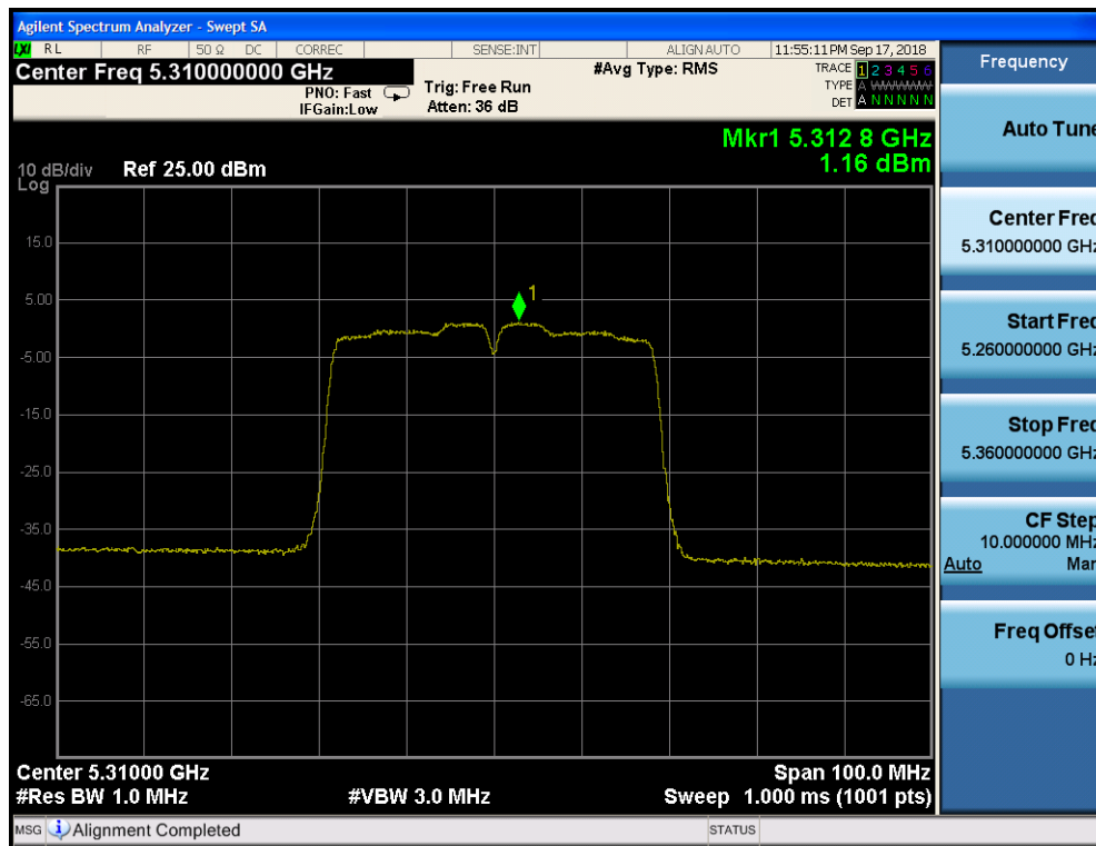
Plot 7-135. Power Spectral Density Plot CDD CORE 0 (40MHz BW 802.11n (UNII Band 2A) – Ch. 62)
