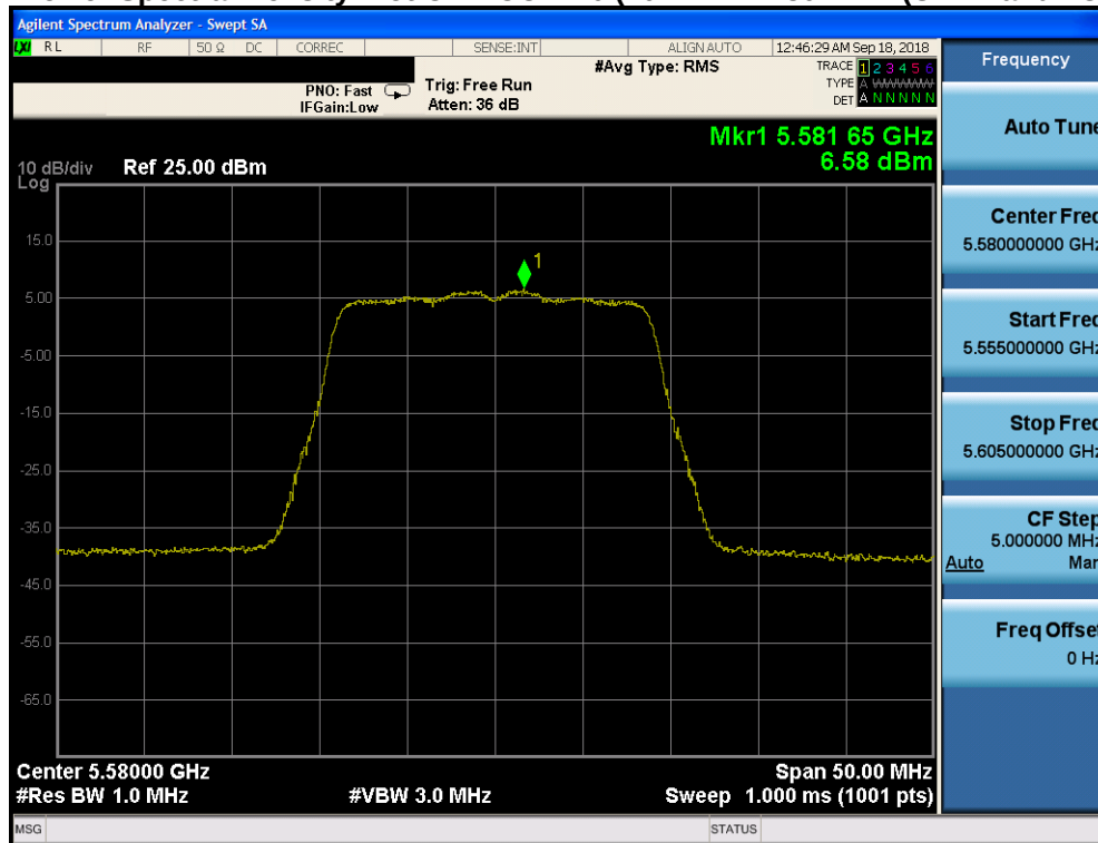
Plot 7-142. Power Spectral Density Plot CDD CORE 1 (20MHz BW 802.11n (UNII Band 2C) – Ch. 116)
