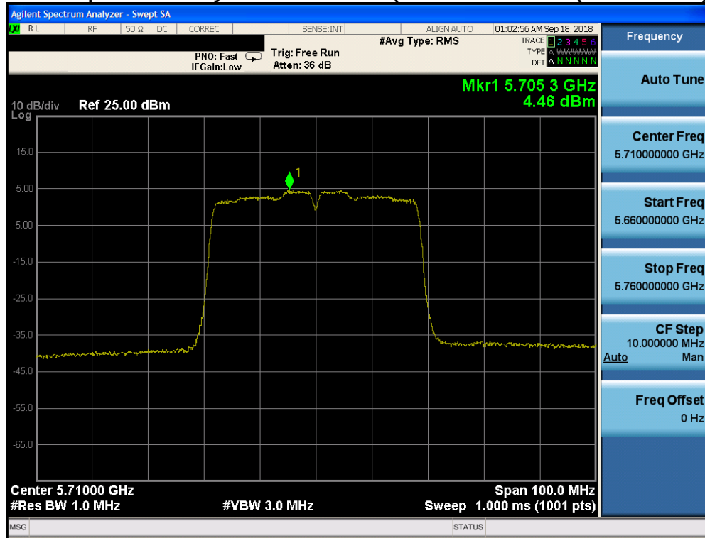
Plot 7-150. Power Spectral Density Plot CDD CORE 1 (40MHz BW 802.11n (UNII Band 2C) – Ch. 142)
