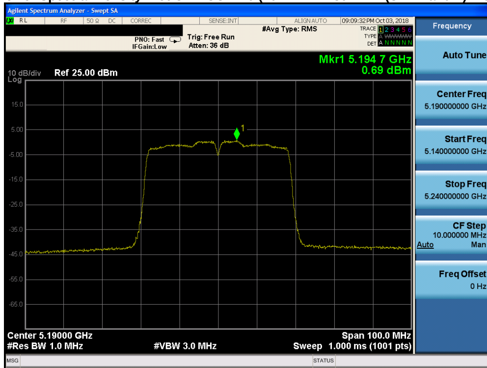
Plot 7-112. Power Spectral Density Plot CDD CORE 1 (40MHz BW 802.11n (UNII Band 1) – Ch. 38) - ISED
