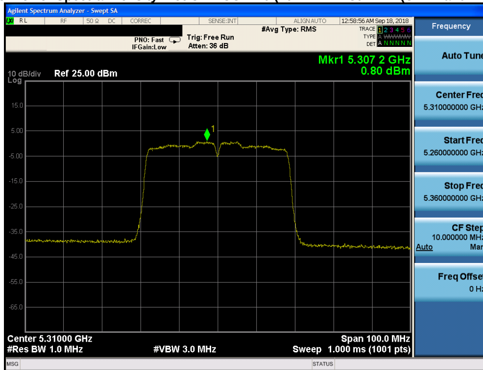
Plot 7-136. Power Spectral Density Plot CDD CORE 1 (40MHz BW 802.11n (UNII Band 2A) – Ch. 62)
