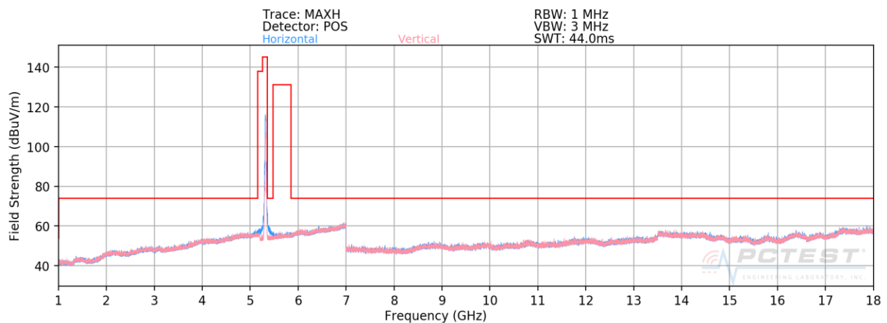
Plot 7-172. Radiated Spurious Plot above 1GHz SISO CORE 0 (802.11n – U2A Ch. 64)
