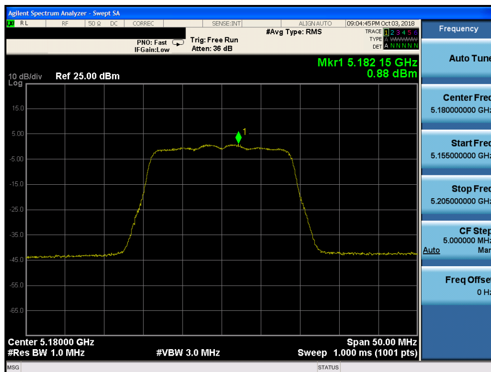
Plot 7-106. Power Spectral Density Plot CDD CORE 1 (20MHz BW 802.11n (UNII Band 1) – Ch. 36) - ISED
