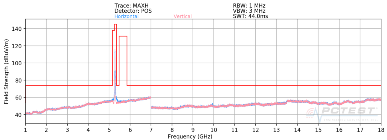
Plot 7-184. Radiated Spurious Plot above 1GHz SISO CORE 1 (802.11n – U2A Ch. 56)
