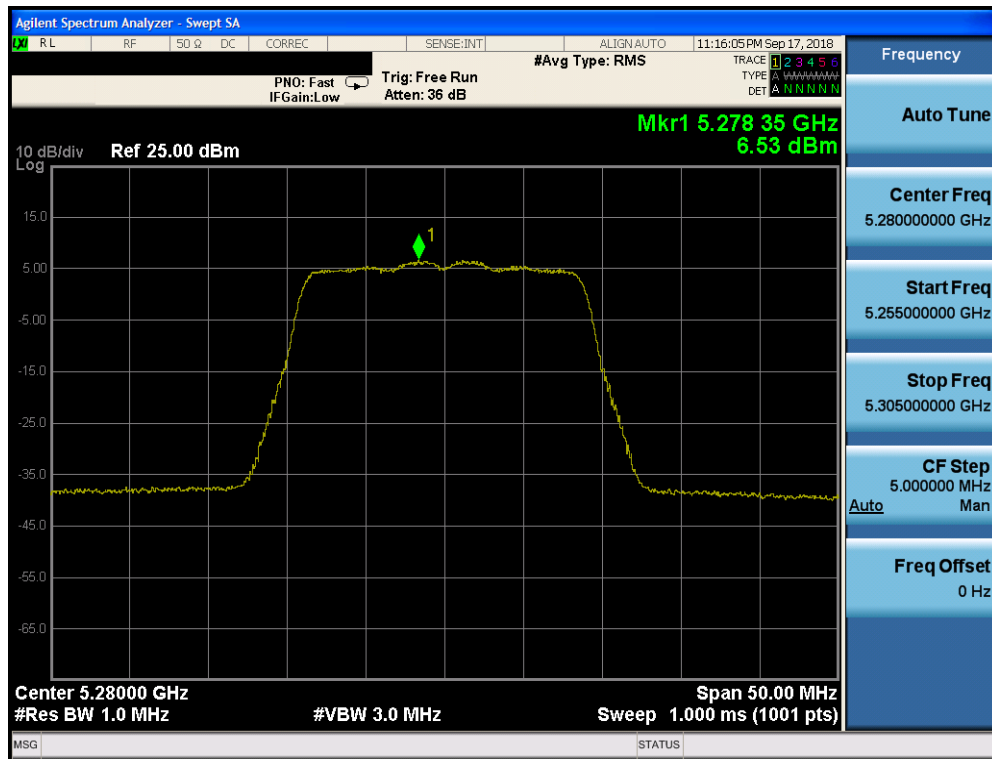
Plot 7-129. Power Spectral Density Plot CDD CORE 0 (20MHz BW 802.11n (UNII Band 2A) – Ch. 56)
