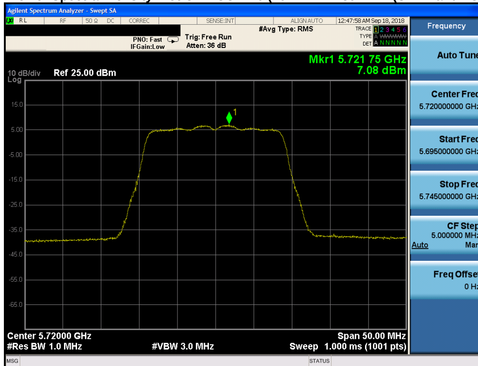
Plot 7-144. Power Spectral Density Plot CDD CORE 1 (20MHz BW 802.11n (UNII Band 2C) – Ch. 144)
