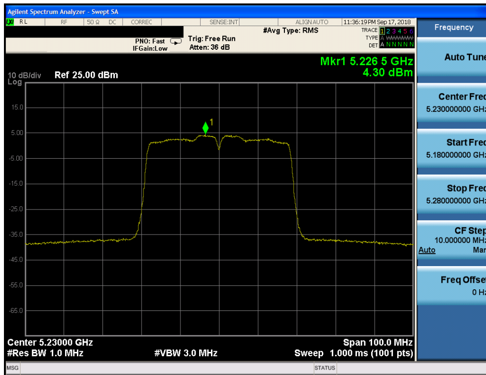
Plot 7-123. Power Spectral Density Plot CDD CORE 0 (40MHz BW 802.11n (UNII Band 1) – Ch. 46)
