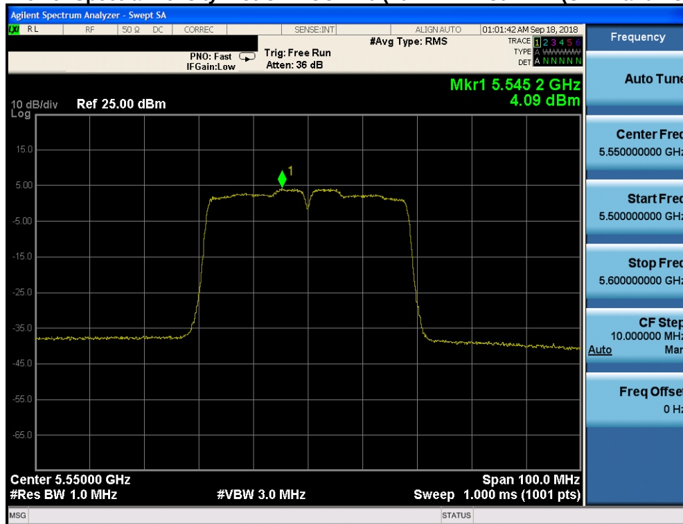
Plot 7-148. Power Spectral Density Plot CDD CORE 1 (40MHz BW 802.11n (UNII Band 2C) – Ch. 110)
