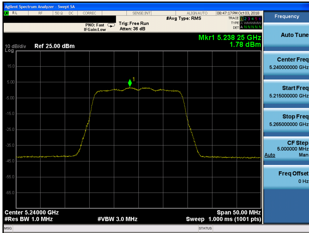
Plot 7-109. Power Spectral Density Plot CDD CORE 0 (20MHz BW 802.11n (UNII Band 1) – Ch. 48) - ISED
