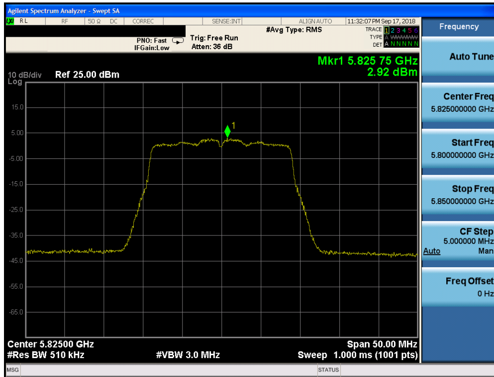
Plot 7-159. Power Spectral Density Plot CDD CORE 0 (20MHz BW 802.11n (UNII Band 3) – Ch. 165)
