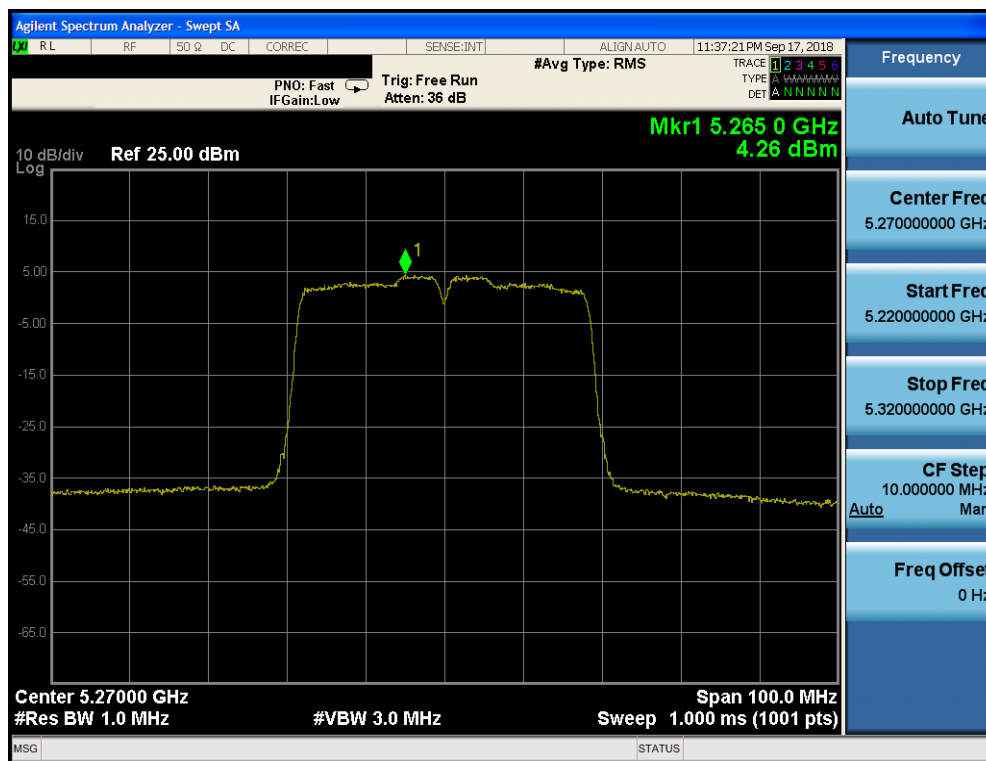
Plot 7-133. Power Spectral Density Plot CDD CORE 0 (40MHz BW 802.11n (UNII Band 2A) – Ch. 54)
