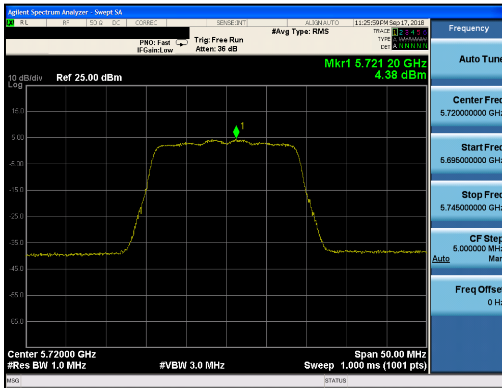
Plot 7-143. Power Spectral Density Plot CDD CORE 0 (20MHz BW 802.11n (UNII Band 2C) – Ch. 144)
