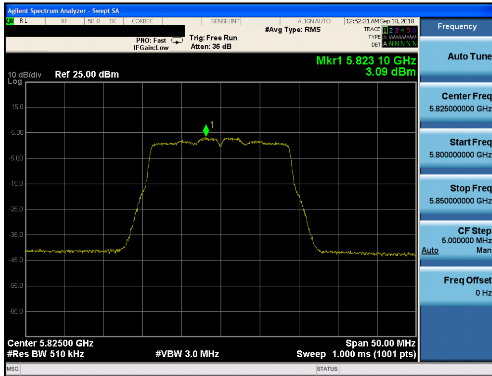
Plot 7-160. Power Spectral Density Plot CDD CORE 1 (20MHz BW 802.11n (UNII Band 3) – Ch. 165)
