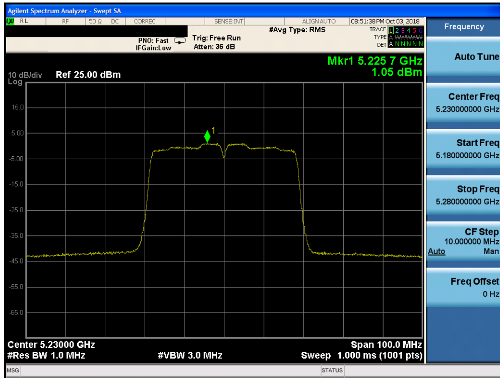
Plot 7-113. Power Spectral Density Plot CDD CORE 0 (40MHz BW 802.11n (UNII Band 1) – Ch. 46) - ISED
