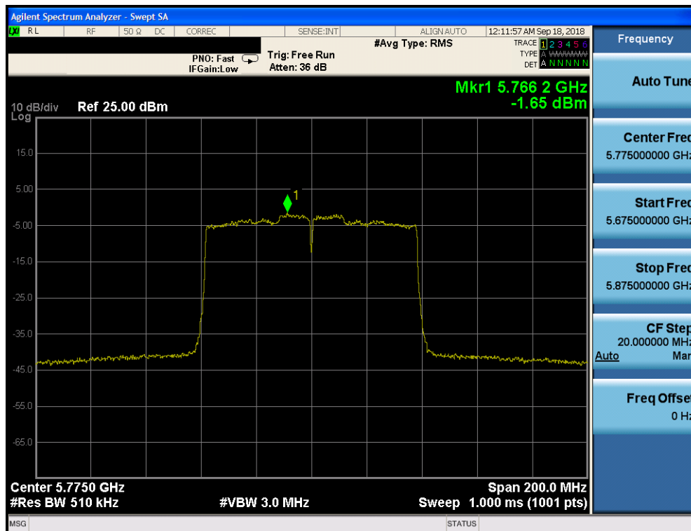
Plot 7-165. Power Spectral Density Plot CDD CORE 0 (80MHz BW 802.11ac (UNII Band 3) – Ch. 155)
