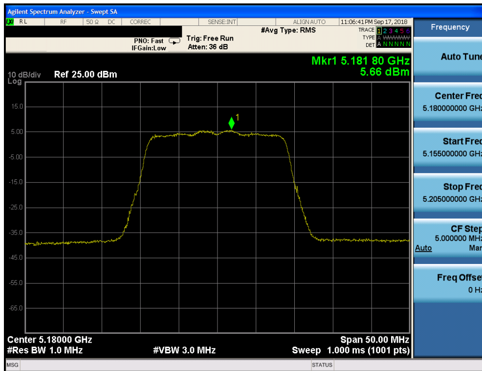
Plot 7-115. Power Spectral Density Plot CDD CORE 0 (20MHz BW 802.11n (UNII Band 1) – Ch. 36)
