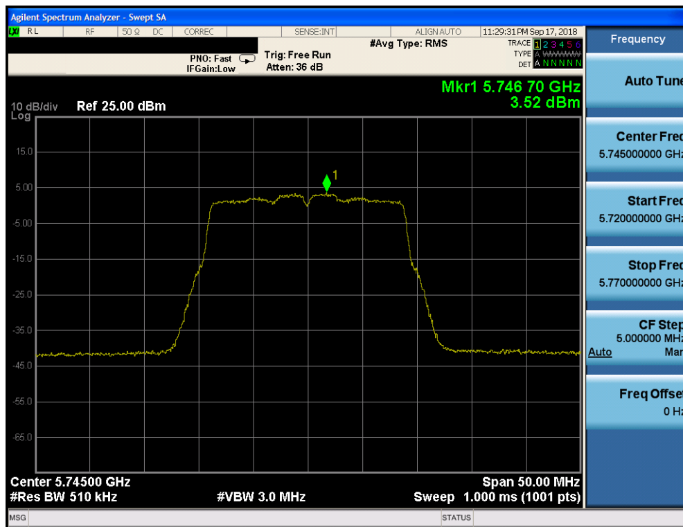
Plot 7-155. Power Spectral Density Plot CDD CORE 0 (20MHz BW 802.11n (UNII Band 3) – Ch. 149)
