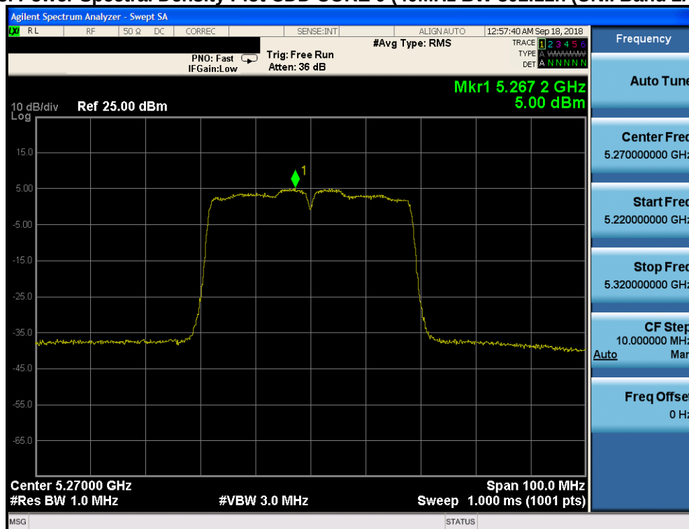
Plot 7-134. Power Spectral Density Plot CDD CORE 1 (40MHz BW 802.11n (UNII Band 2A) – Ch. 54)
