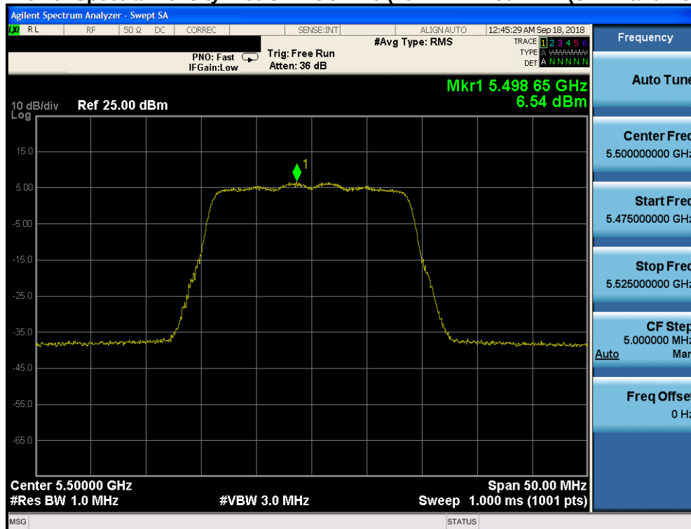
Plot 7-140. Power Spectral Density Plot CDD CORE 1 (20MHz BW 802.11n (UNII Band 2C) – Ch. 100)
