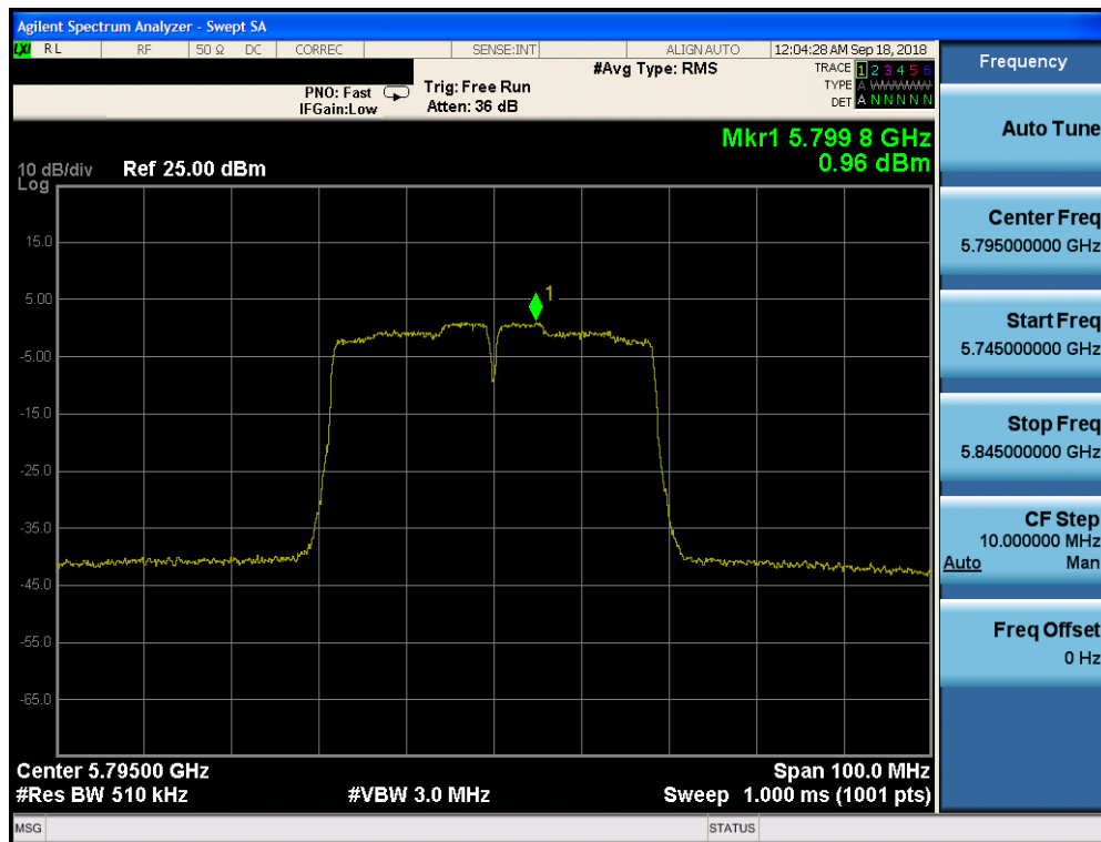
Plot 7-163. Power Spectral Density Plot CDD CORE 0 (40MHz BW 802.11n (UNII Band 3) – Ch. 159)
