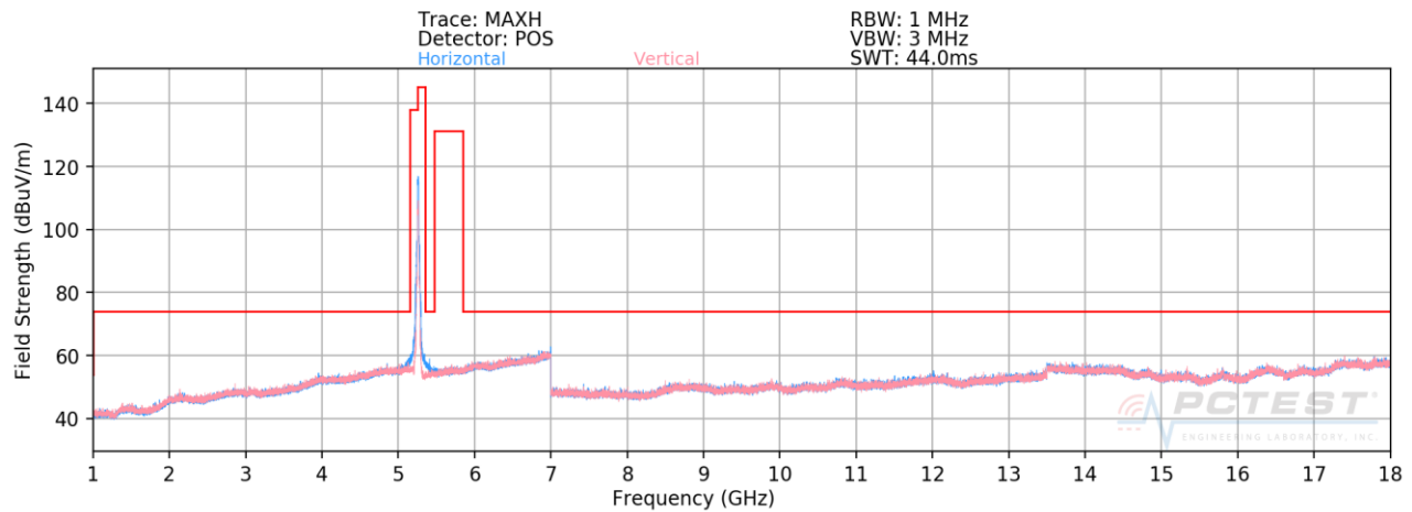
Plot 7-170. Radiated Spurious Plot above 1GHz SISO Core 0 (802.11n – U2A Ch. 52)
