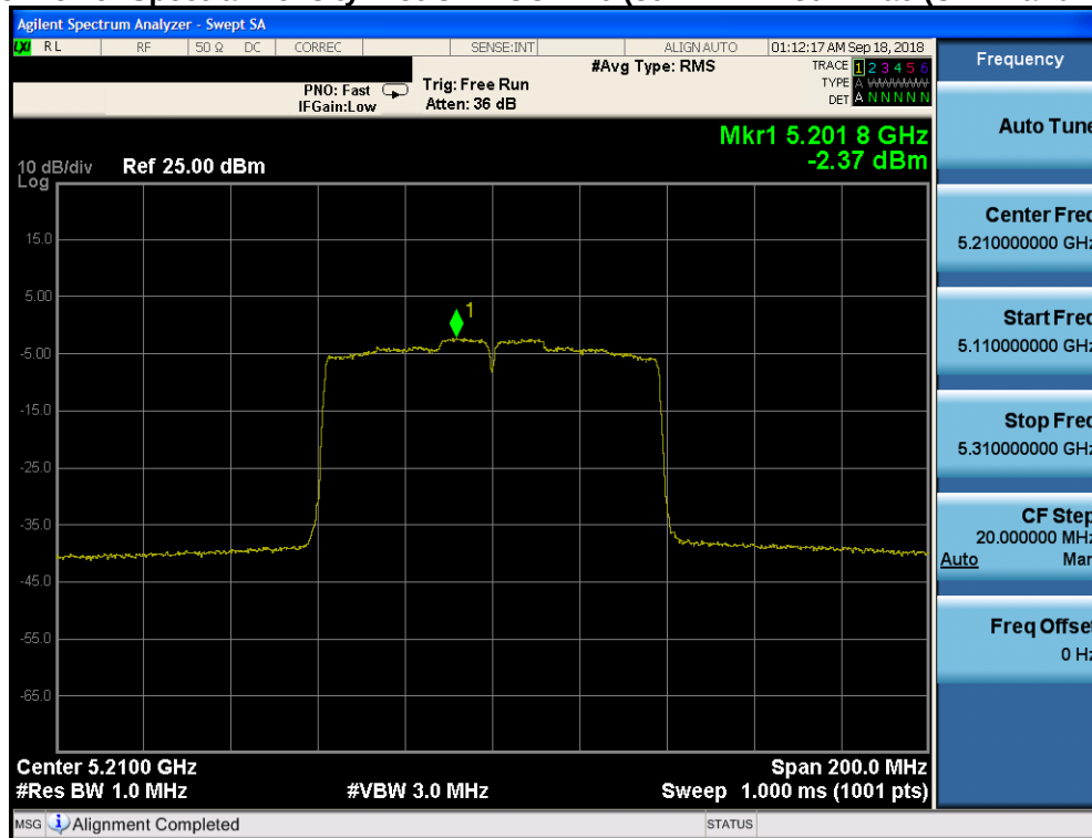
Plot 7-126. Power Spectral Density Plot CDD CORE 1 (80MHz BW 802.11ac (UNII Band 1) – Ch. 42)
