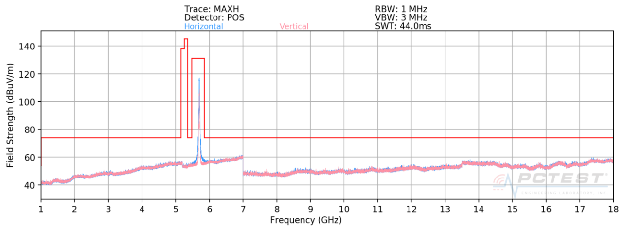
Plot 7-175. Radiated Spurious Plot above 1GHz SISO CORE 0 (802.11n – U2C Ch. 140)
