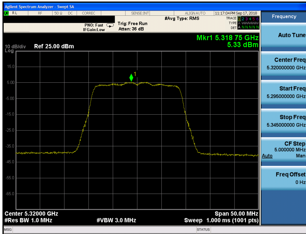
Plot 7-131. Power Spectral Density Plot CDD CORE 0 (20MHz BW 802.11n (UNII Band 2A) – Ch. 64)
