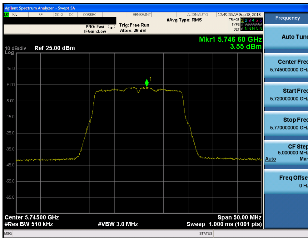
Plot 7-156. Power Spectral Density Plot CDD CORE 1 (20MHz BW 802.11n (UNII Band 3) – Ch. 149)
