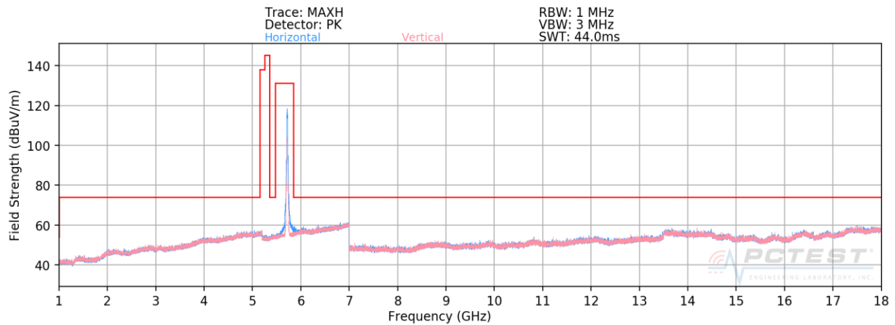
Plot 7-176. Radiated Spurious Plot above 1GHz SISO Core 0 (802.11n – U2C Ch. 144)
