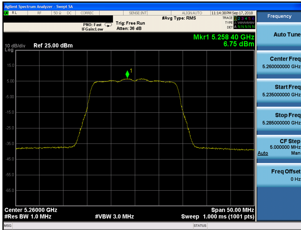
Plot 7-127. Power Spectral Density Plot CDD CORE 0 (20MHz BW 802.11n (UNII Band 2A) – Ch. 52)
