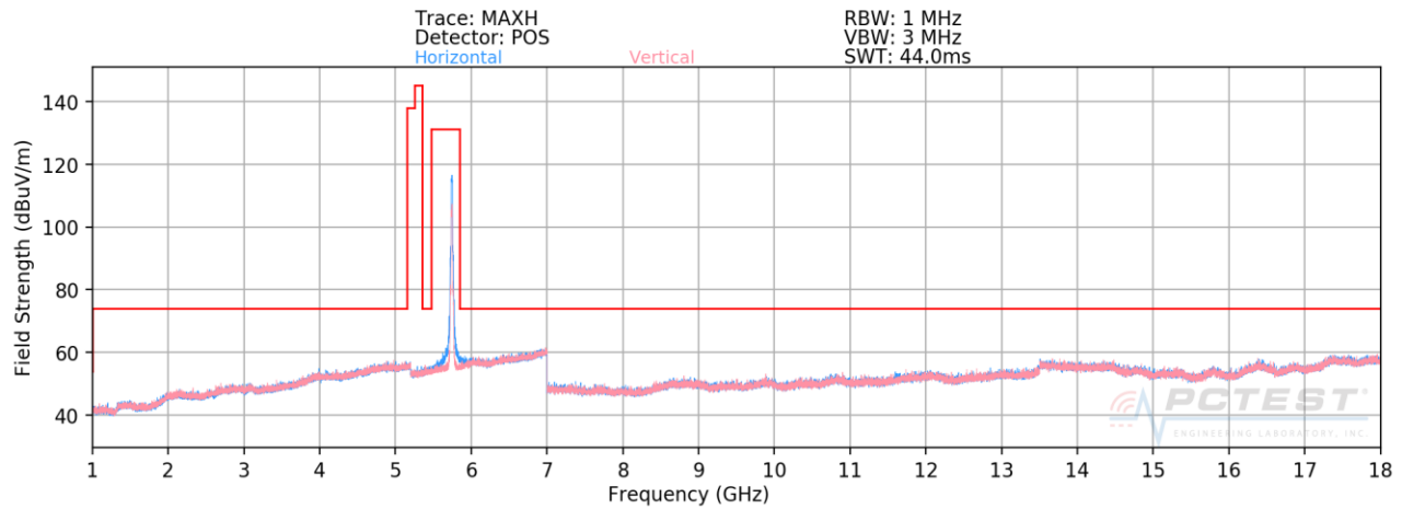
Plot 7-177. Radiated Spurious Plot above 1GHz SISO CORE 0 (802.11n – U3 Ch. 149)
