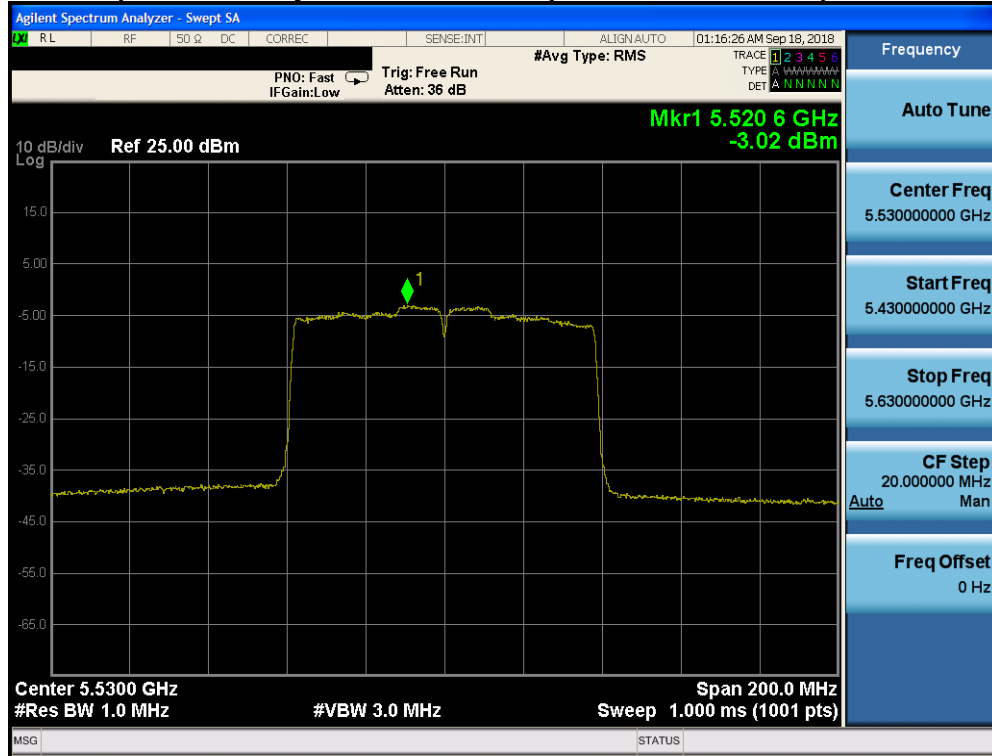
Plot 7-152. Power Spectral Density Plot CDD CORE 1 (80MHz BW 802.11ac (UNII Band 2C) – Ch. 106)
