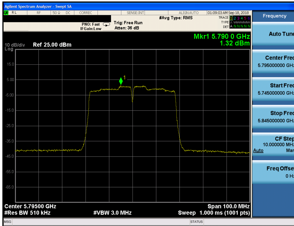
Plot 7-164. Power Spectral Density Plot CDD CORE 1 (40MHz BW 802.11n (UNII Band 3) – Ch. 159)
