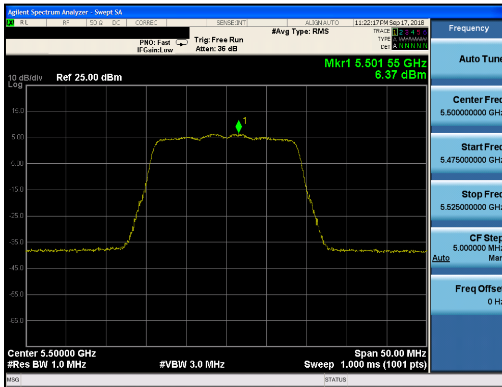
Plot 7-139. Power Spectral Density Plot CDD CORE 0 (20MHz BW 802.11n (UNII Band 2C) – Ch. 100)
