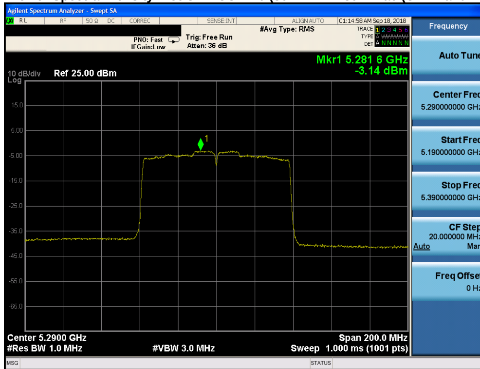
Plot 7-138. Power Spectral Density Plot CDD CORE 1 (80MHz BW 802.11ac (UNII Band 2A) – Ch. 58)
