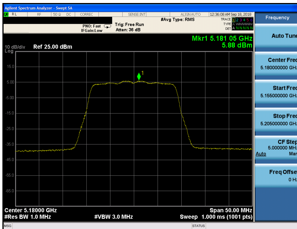
Plot 7-116. Power Spectral Density Plot CDD CORE 1 (20MHz BW 802.11n (UNII Band 1) – Ch. 36)
