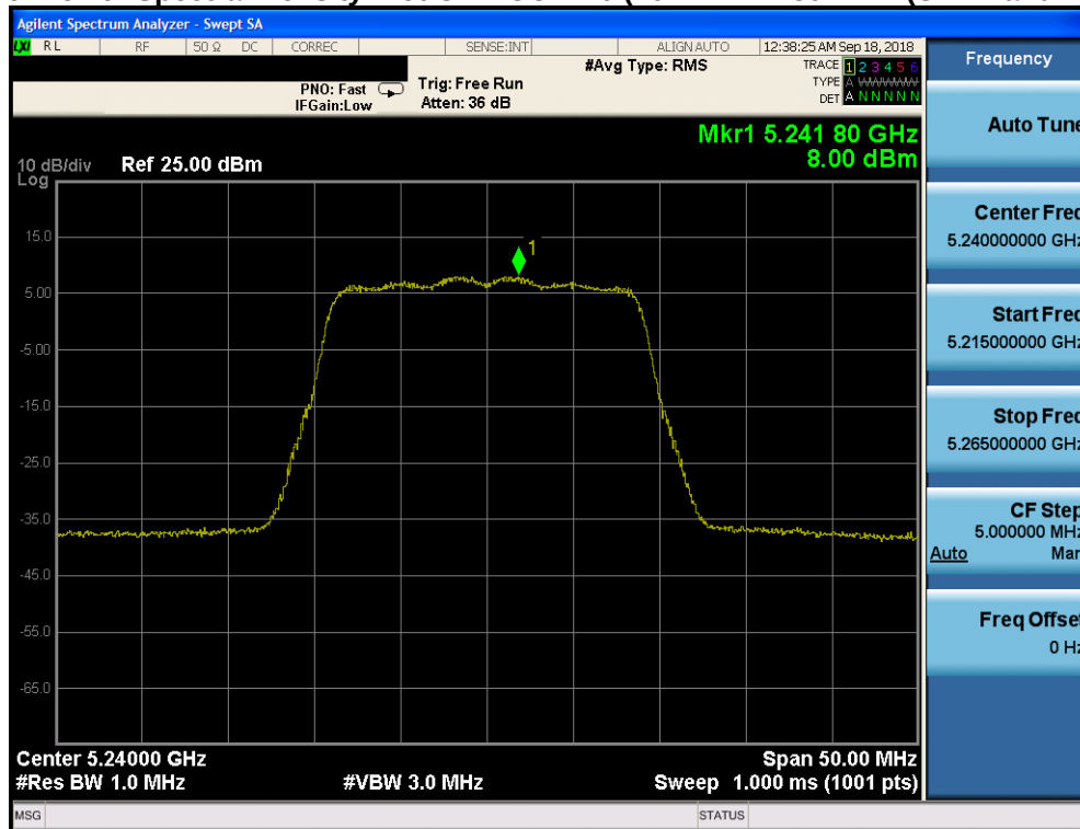
Plot 7-120. Power Spectral Density Plot CDD CORE 1 (20MHz BW 802.11n (UNII Band 1) – Ch. 48)
