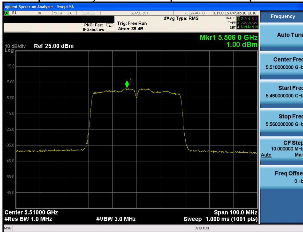
Plot 7-146. Power Spectral Density Plot CDD CORE 1 (40MHz BW 802.11n (UNII Band 2C) – Ch. 102)
