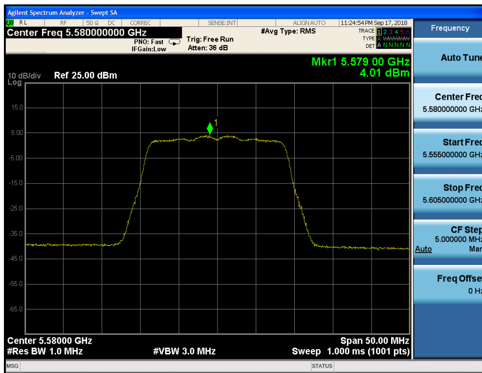
Plot 7-141. Power Spectral Density Plot CDD CORE 0 (20MHz BW 802.11n (UNII Band 2C) – Ch. 116)
