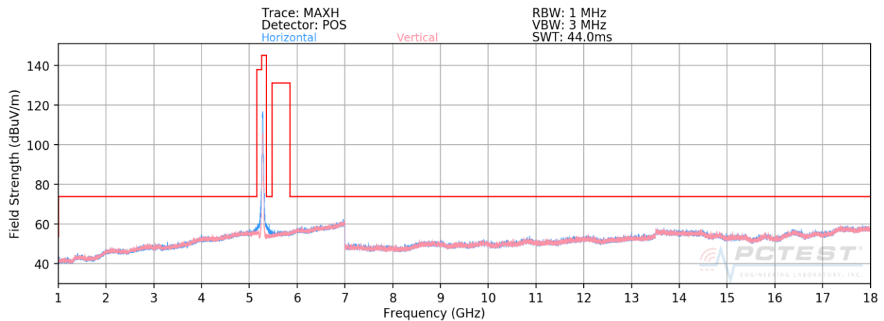
Plot 7-171. Radiated Spurious Plot above 1GHz SISO CORE 0 (802.11n – U2A Ch. 56)
