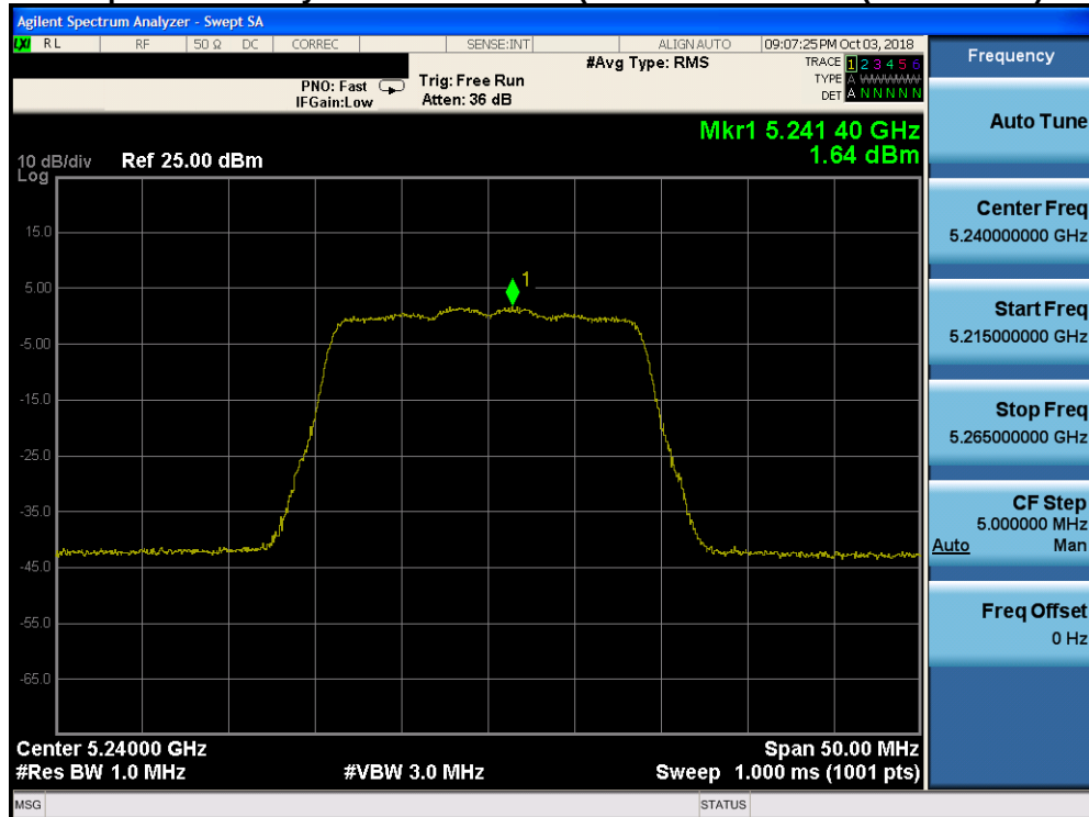
Plot 7-110. Power Spectral Density Plot CDD CORE 1 (20MHz BW 802.11n (UNII Band 1) – Ch. 48) - ISED
