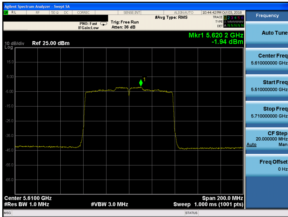
Plot 7-153. Power Spectral Density Plot CDD CORE 0 (80MHz BW 802.11ac (UNII Band 2C) – Ch. 122)
