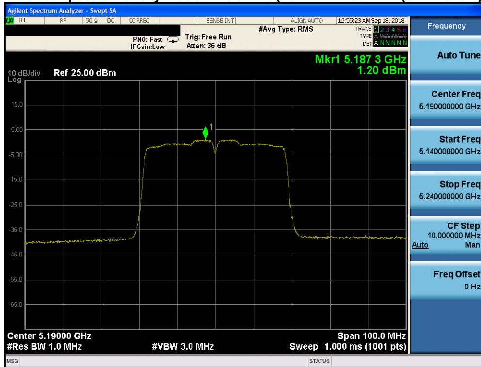
Plot 7-122. Power Spectral Density Plot CDD CORE 1 (40MHz BW 802.11n (UNII Band 1) – Ch. 38)
