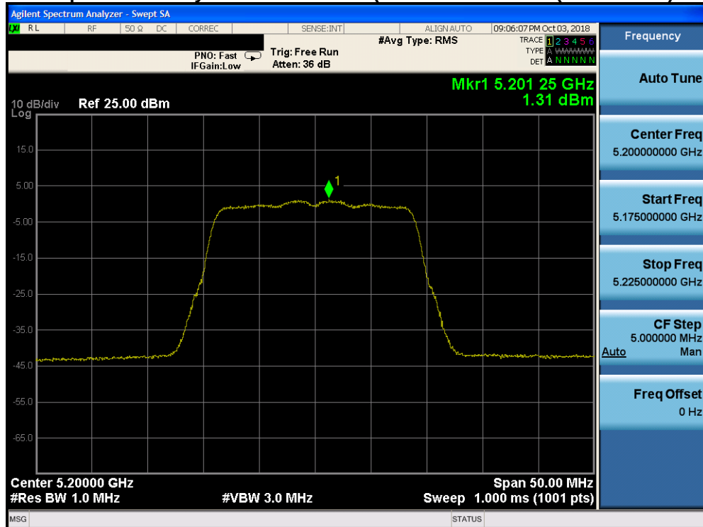
Plot 7-108. Power Spectral Density Plot CDD CORE 1 (20MHz BW 802.11n (UNII Band 1) – Ch. 40) - ISED
