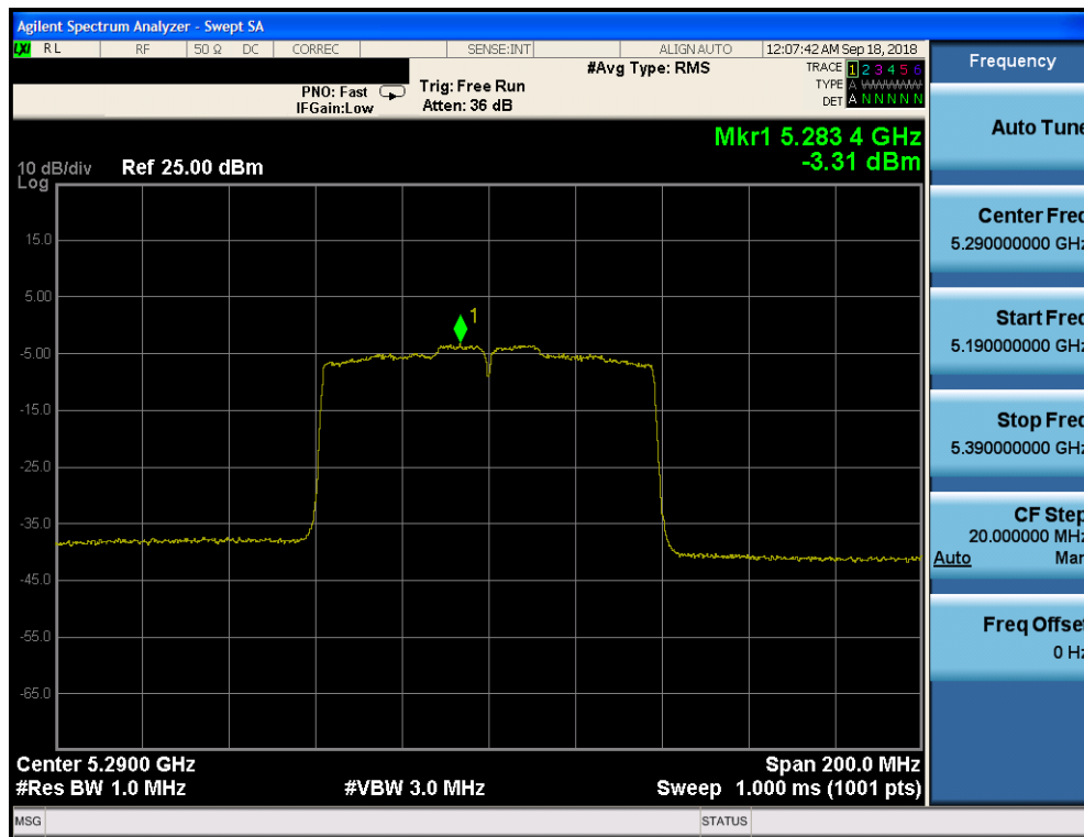
Plot 7-137. Power Spectral Density Plot CDD CORE 0 (80MHz BW 802.11ac (UNII Band 2A) – Ch. 58)
