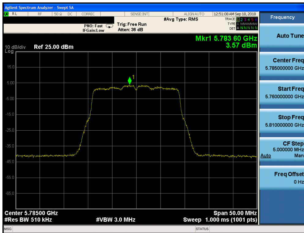
Plot 7-158. Power Spectral Density Plot CDD CORE 1 (20MHz BW 802.11n (UNII Band 3) – Ch. 157)
