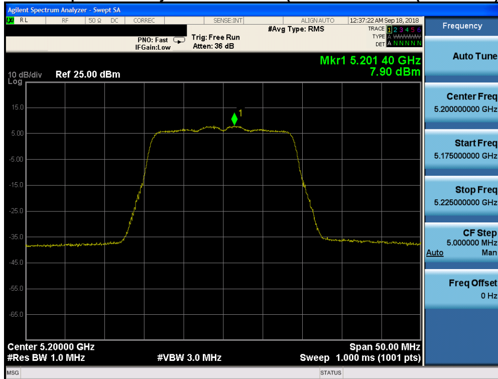
Plot 7-118. Power Spectral Density Plot CDD CORE 1 (20MHz BW 802.11n (UNII Band 1) – Ch. 40)
