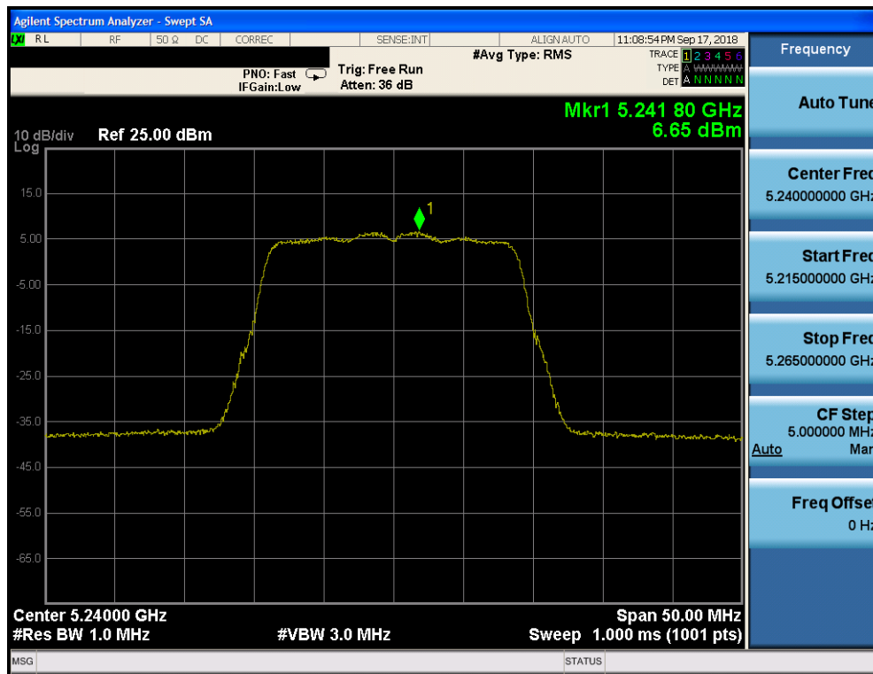
Plot 7-119. Power Spectral Density Plot CDD CORE 0 (20MHz BW 802.11n (UNII Band 1) – Ch. 48)
