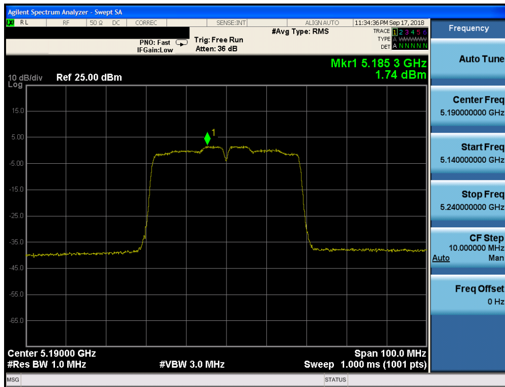
Plot 7-121. Power Spectral Density Plot CDD CORE 0 (40MHz BW 802.11n (UNII Band 1) – Ch. 38)
