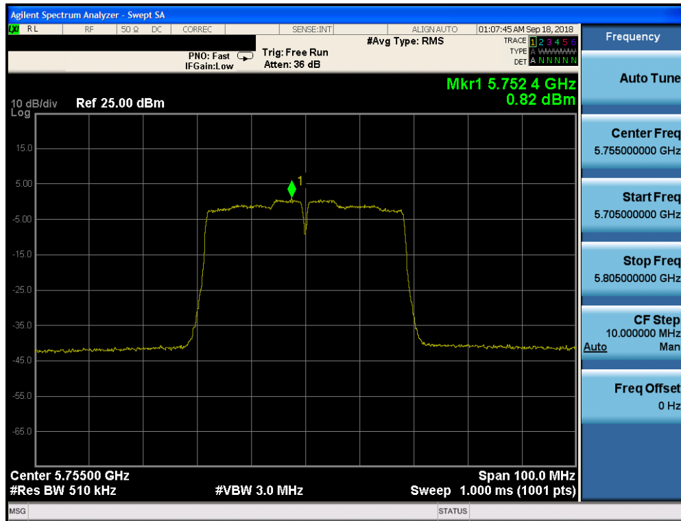
Plot 7-162. Power Spectral Density Plot CDD CORE 1 (40MHz BW 802.11n (UNII Band 3) – Ch. 151)
