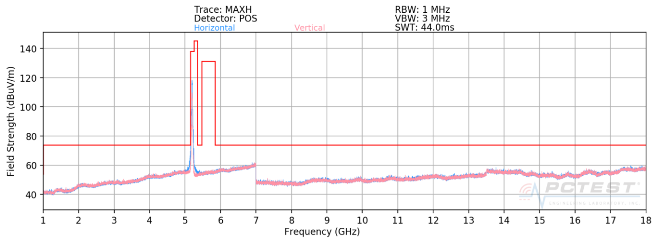
Plot 7-168. Radiated Spurious Plot above 1GHz SISO CORE 0 (802.11n – U1 Ch. 40)
