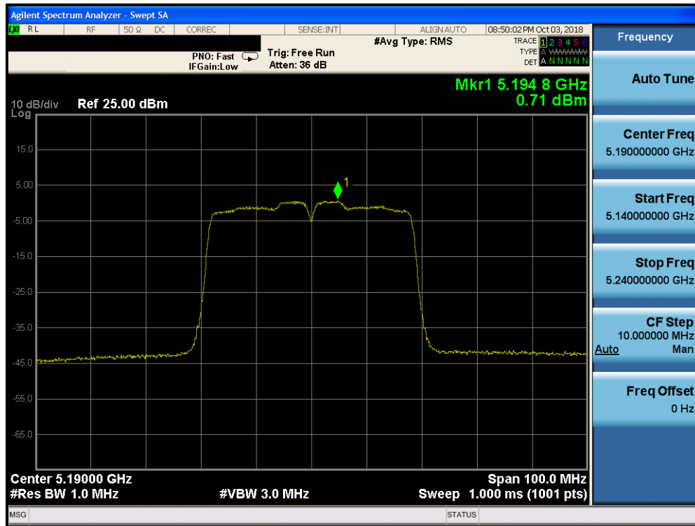
Plot 7-111. Power Spectral Density Plot CDD CORE 0 (40MHz BW 802.11n (UNII Band 1) – Ch. 38) - ISED
