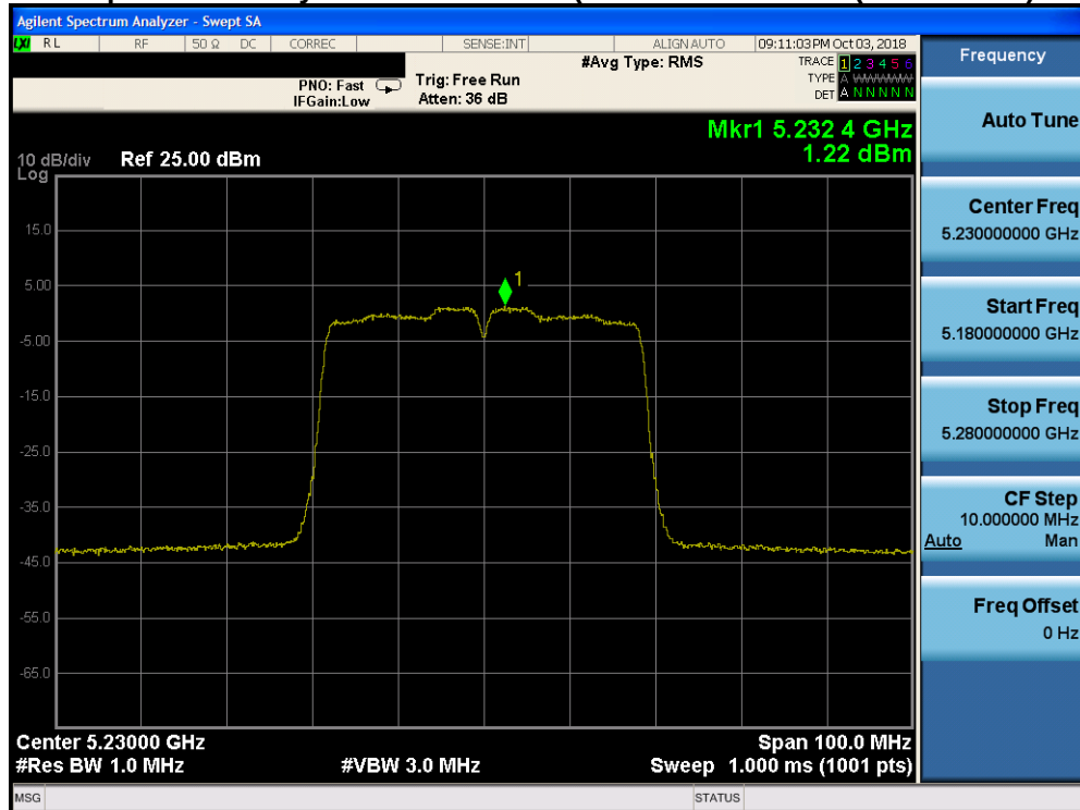
Plot 7-114. Power Spectral Density Plot CDD CORE 1 (40MHz BW 802.11n (UNII Band 1) – Ch. 46) - ISED
