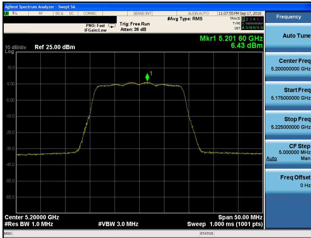
Plot 7-117. Power Spectral Density Plot CDD CORE 0 (20MHz BW 802.11n (UNII Band 1) – Ch. 40)
