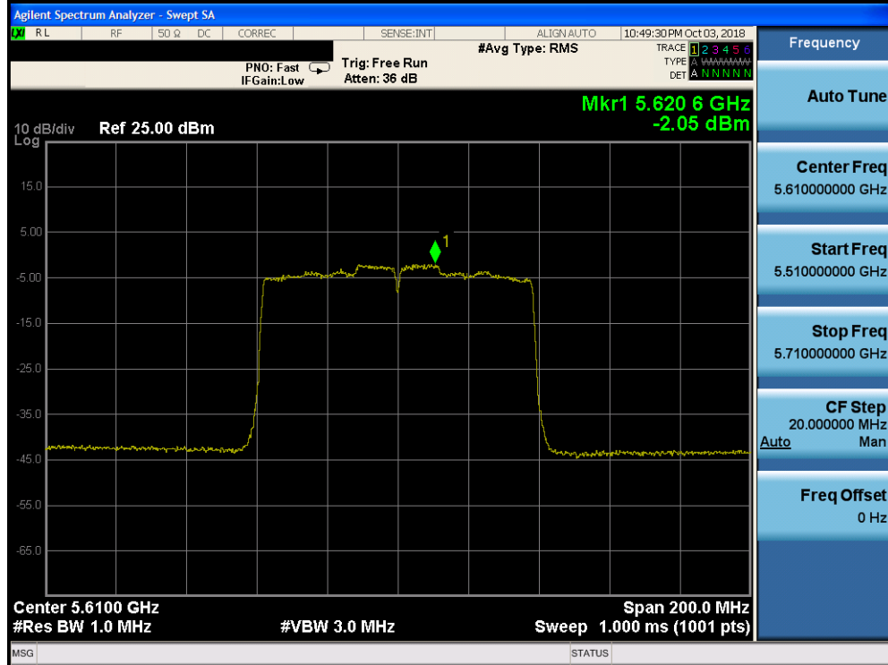
Plot 7-154. Power Spectral Density Plot CDD CORE 1 (80MHz BW 802.11ac (UNII Band 2C) – Ch. 122)
