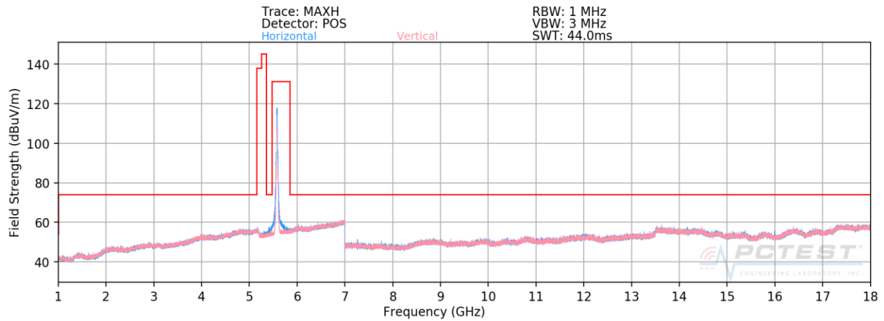
Plot 7-174. Radiated Spurious Plot above 1GHz SISO CORE 0 (802.11n – U2C Ch. 116)
