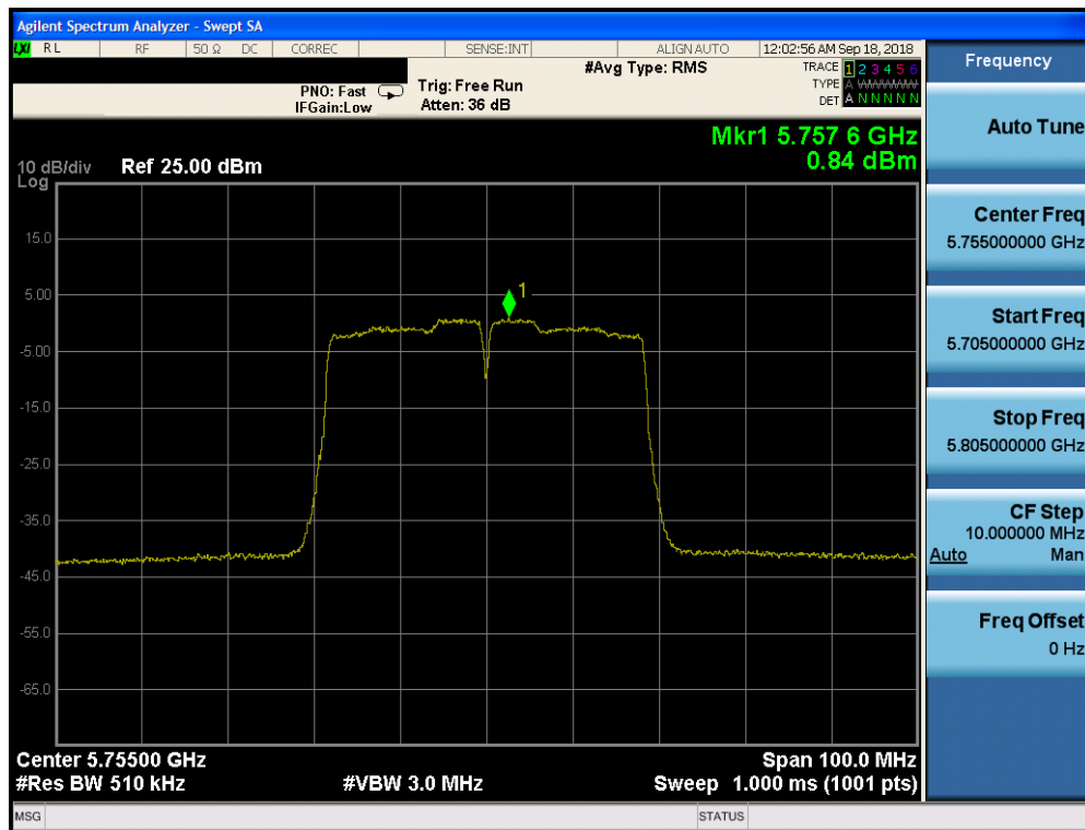
Plot 7-161. Power Spectral Density Plot CDD CORE 0 (40MHz BW 802.11n (UNII Band 3) – Ch. 151)
