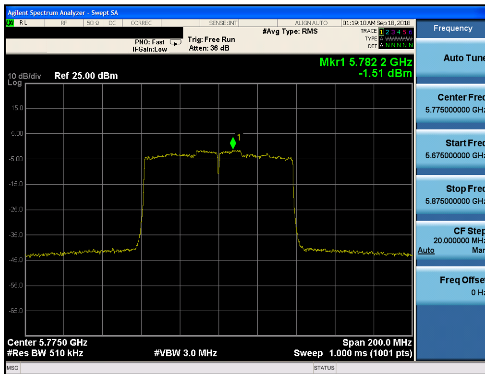
Plot 7-166. Power Spectral Density Plot CDD CORE 1 (80MHz BW 802.11ac (UNII Band 3) – Ch. 155)
