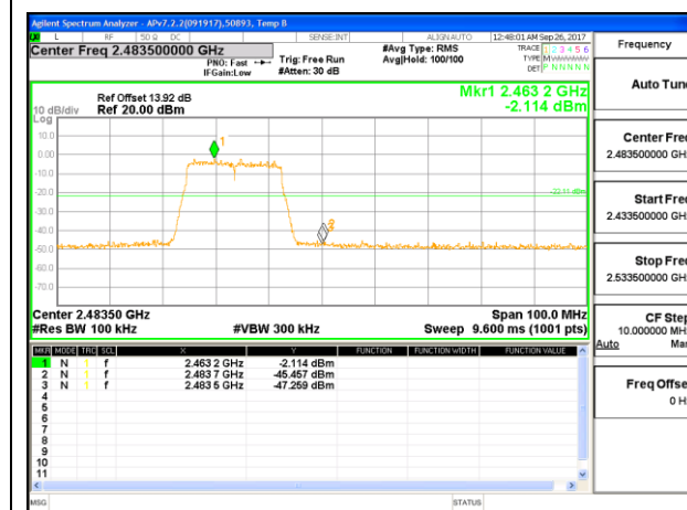
HIGH CHANNEL 12 BANDEDGE WF2
