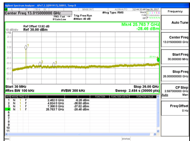
OUT-OF-BAND HIGH CHANNEL 11 WF2
