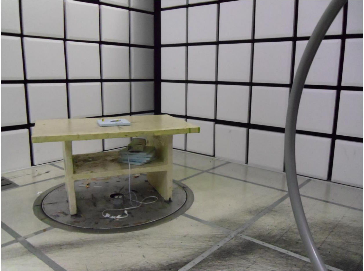
Radiated Test Setup: 9KHz-30MHz
