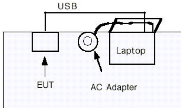
Radiated Test Setup - Top View
