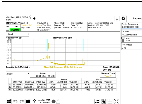
5G NR n77 50MHz BPSK High Channel RB1-0 Port A
