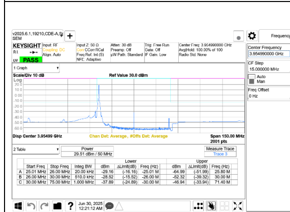
5G NR n77 50MHz BPSK High Channel RB1-0 Port A+B
