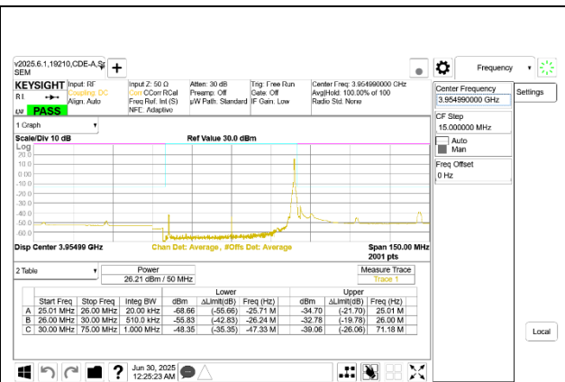
5G NR n77 50MHz BPSK High Channel RB1-132 Port A
