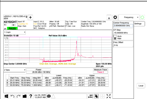
5G NR n77 50MHz BPSK High Channel RB1-132 Port B
