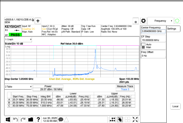
5G NR n77 50MHz BPSK High Channel RB1-132 Port A+B
