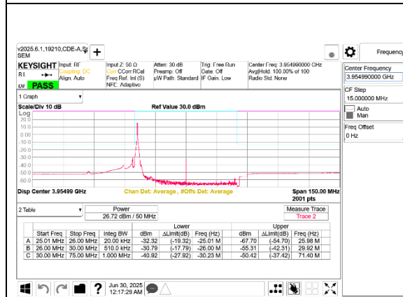
5G NR n77 50MHz BPSK High Channel RB1-0 Port B
