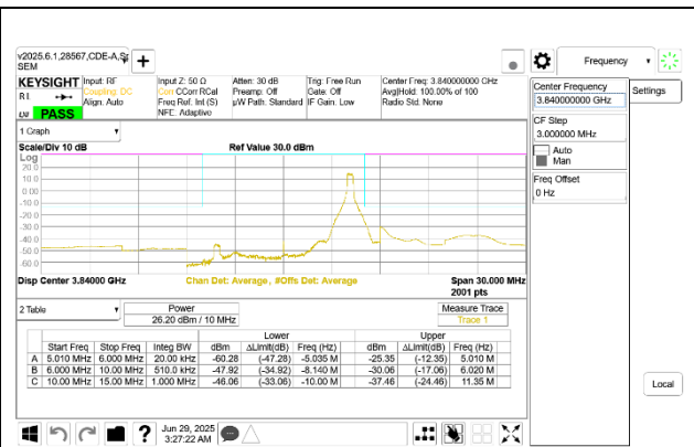
5G NR n77 10MHz BPSK Mid Channel RB1-23 Port A
