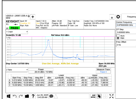
5G NR n77 10MHz BPSK High Channel RB1-0 Port A+B
