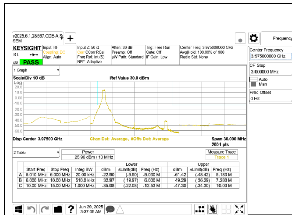
5G NR n77 10MHz BPSK High Channel RB1-0 Port A
