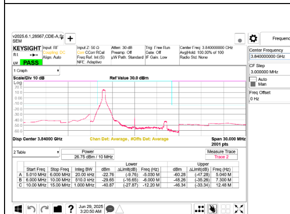
5G NR n77 10MHz BPSK Mid Channel RB1-0 Port B
