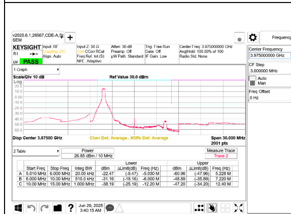
5G NR n77 10MHz BPSK High Channel RB1-0 Port B
