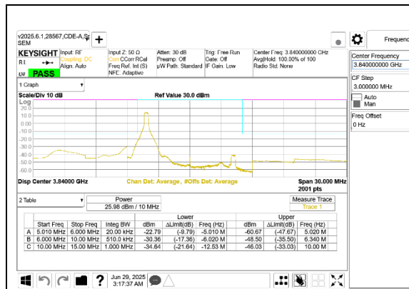
5G NR n77 10MHz BPSK Mid Channel RB1-0 Port A
