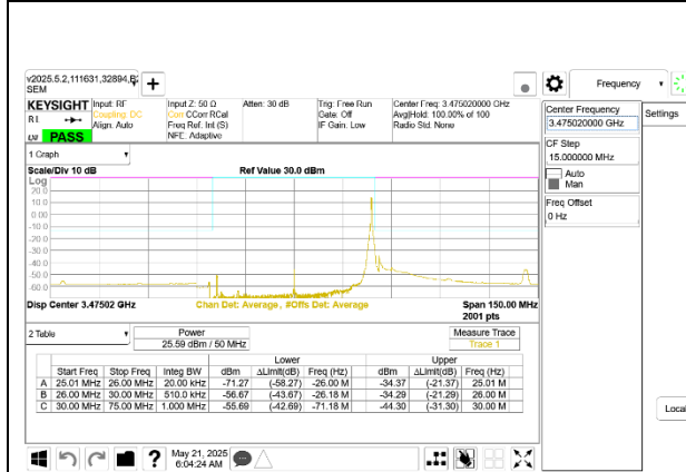
5G NR n77 50MHz BPSK Low Channel RB1-132
