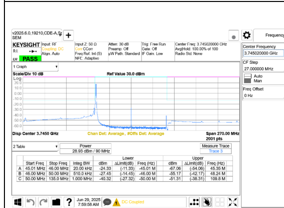
5G NR n77 90MHz BPSK Low Channel RB1-0 Port A+B
