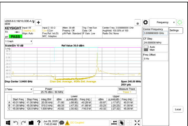
5G NR n77 80MHz BPSK High Channel RB1-216 Port A
