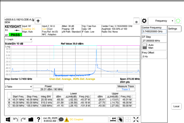
5G NR n77 90MHz BPSK Low Channel RB1-244 Port A+B
