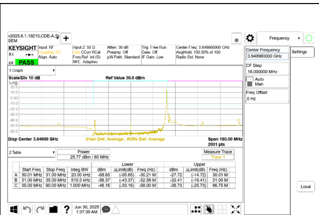
5G NR n77 60MHz BPSK High Channel RB1-161 Port A
