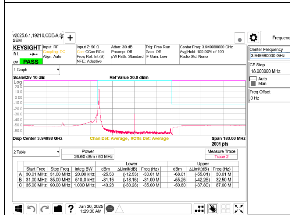
5G NR n77 60MHz BPSK High Channel RB1-0 Port B
