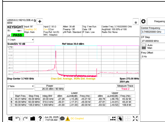
5G NR n77 90MHz BPSK Low Channel RB1-0 Port B
