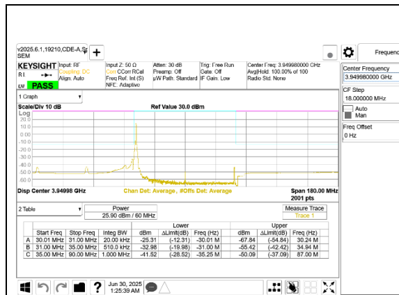
5G NR n77 60MHz BPSK High Channel RB1-0 Port A
