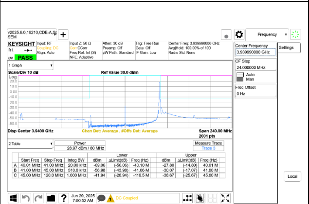
5G NR n77 80MHz BPSK High Channel RB1-216 Port A+B
