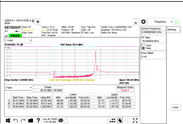
5G NR n77 60MHz BPSK High Channel RB1-161 Port B
