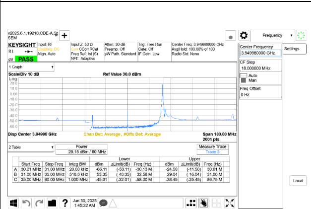
5G NR n77 60MHz BPSK High Channel RB1-161 Port A+B
