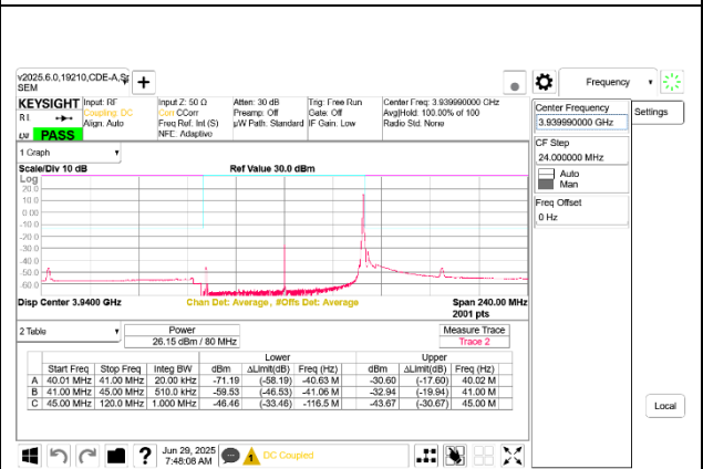
5G NR n77 80MHz BPSK High Channel RB1-216 Port B
