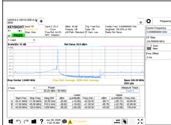
5G NR n77 80MHz BPSK High Channel RB1-0 Port A+B
