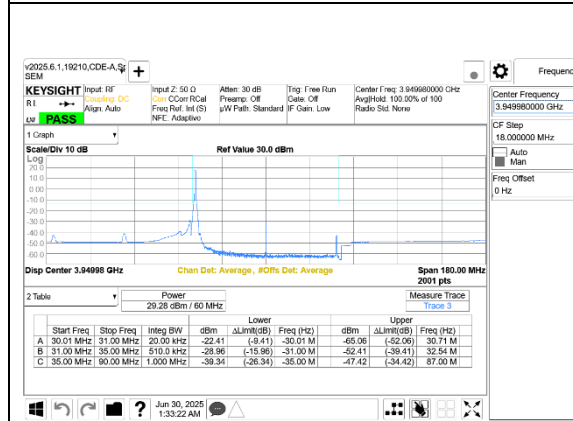
5G NR n77 60MHz BPSK High Channel RB1-0 Port A+B
