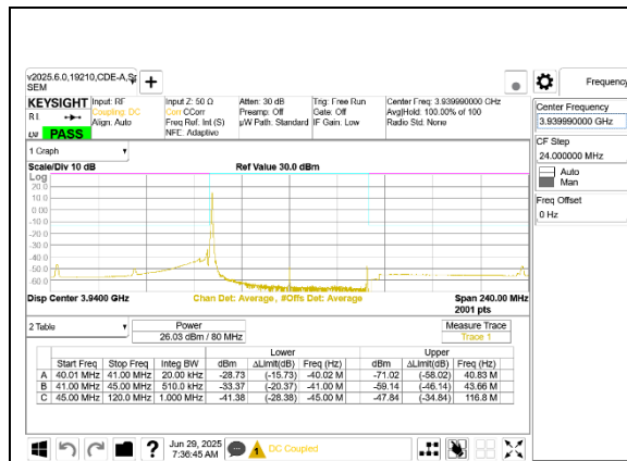
5G NR n77 80MHz BPSK High Channel RB1-0 Port A
