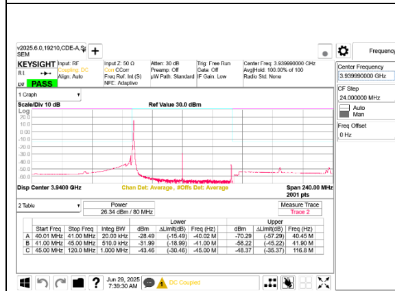
5G NR n77 80MHz BPSK High Channel RB1-0 Port B
