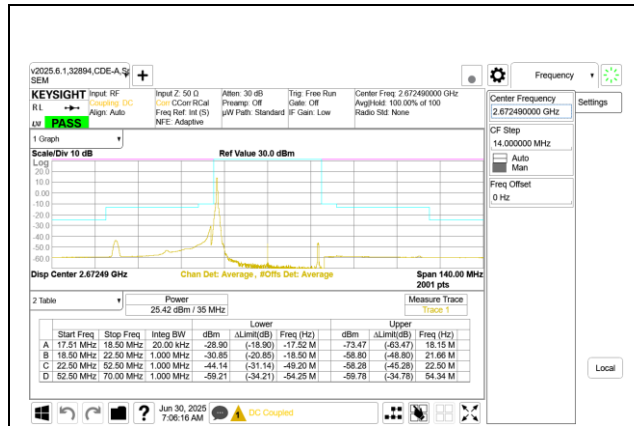
5G NR n41 35MHz BPSK High Channel RB1-0 Port A
