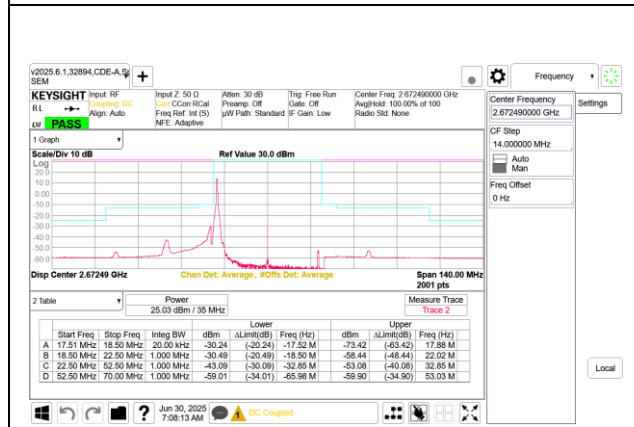
5G NR n41 35MHz BPSK High Channel RB1-0 Port B
