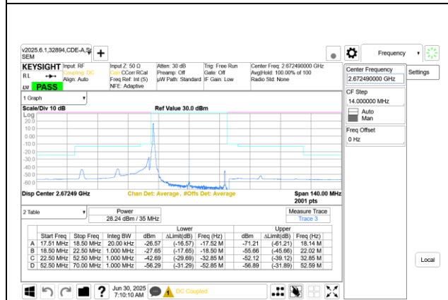
5G NR n41 35MHz BPSK High Channel RB1-0 Port A+B
